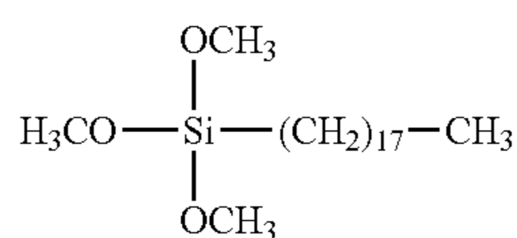
Octadecyltrimethoxysilane
