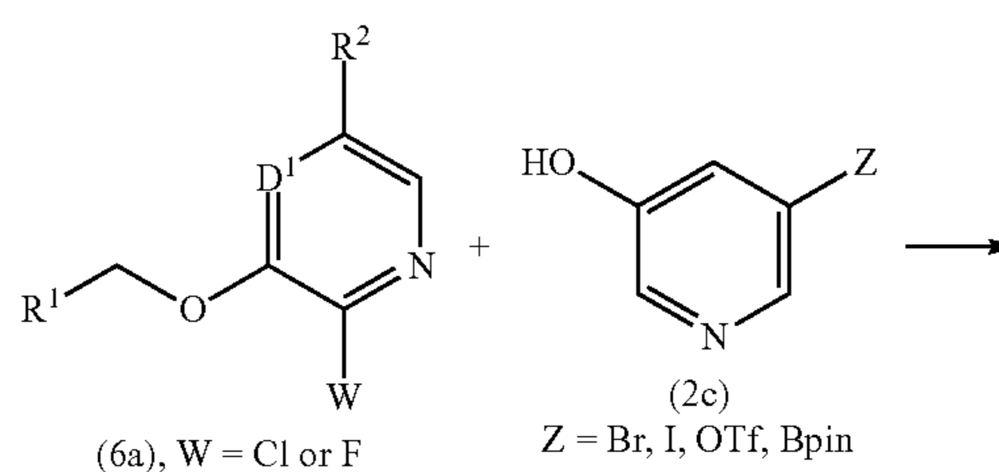
Reaction Scheme II
