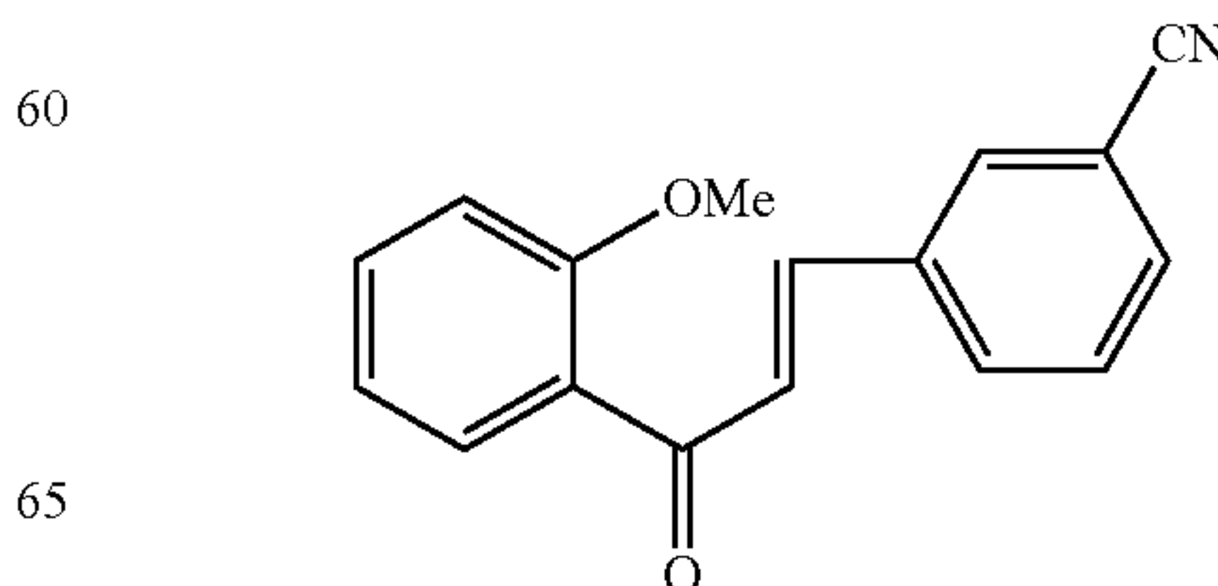
Compound 102
