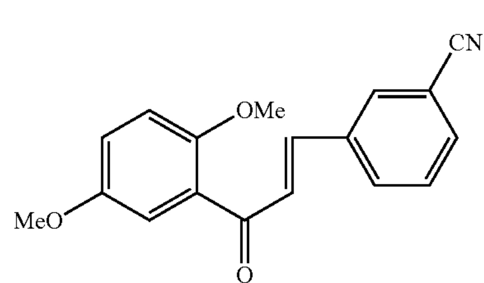
Compound 114
