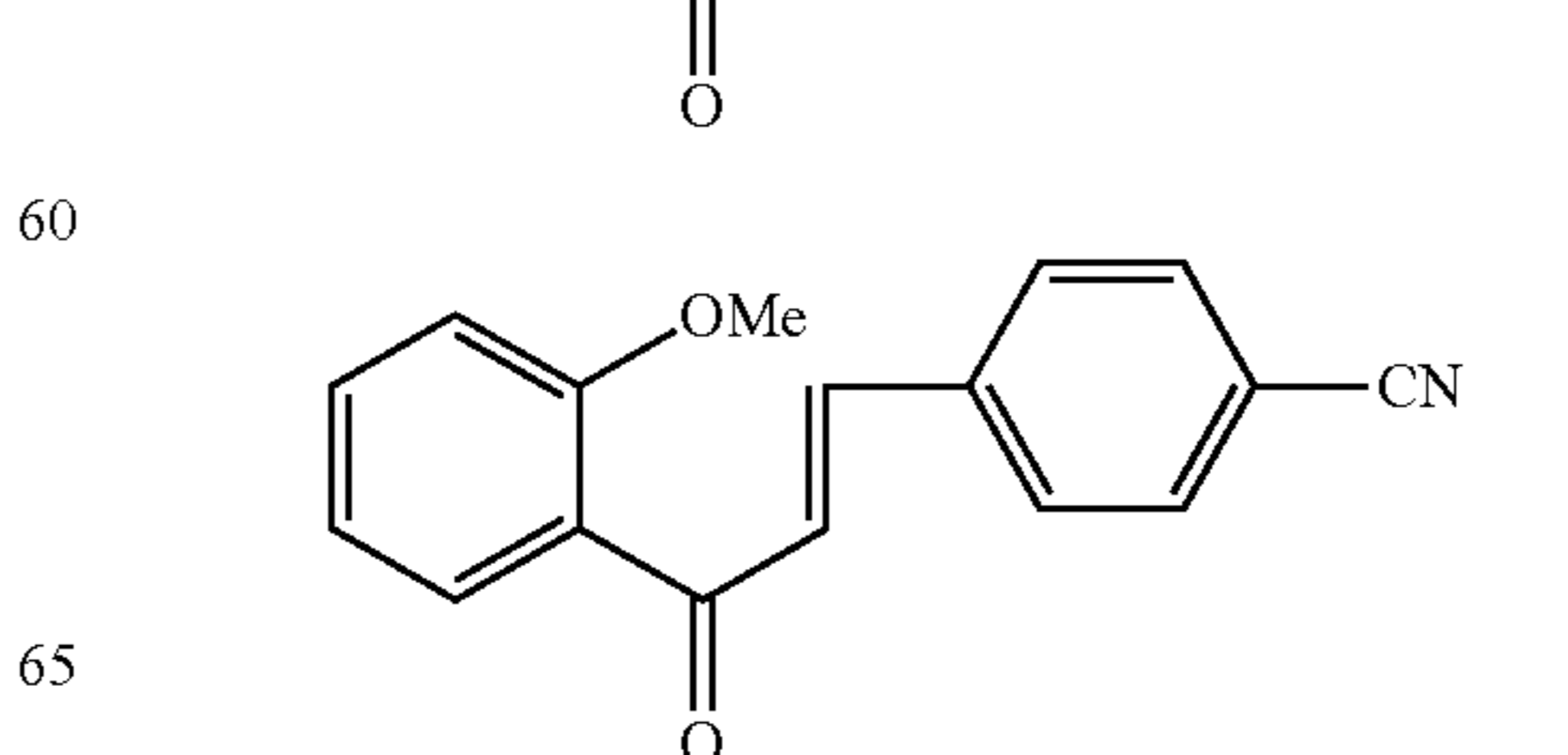
Compound 98
