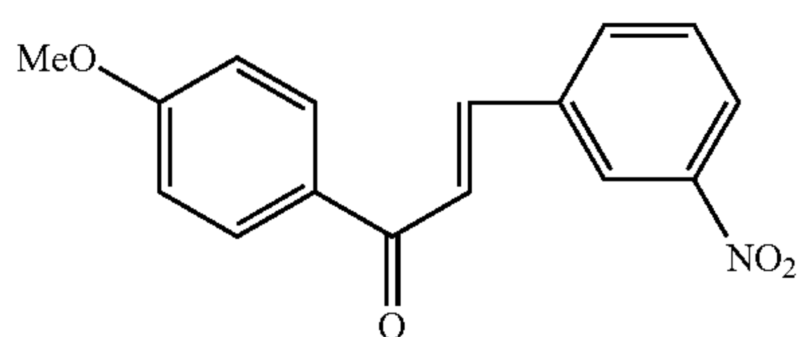
Compound 8
