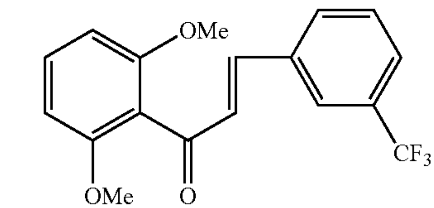
Compound 50
