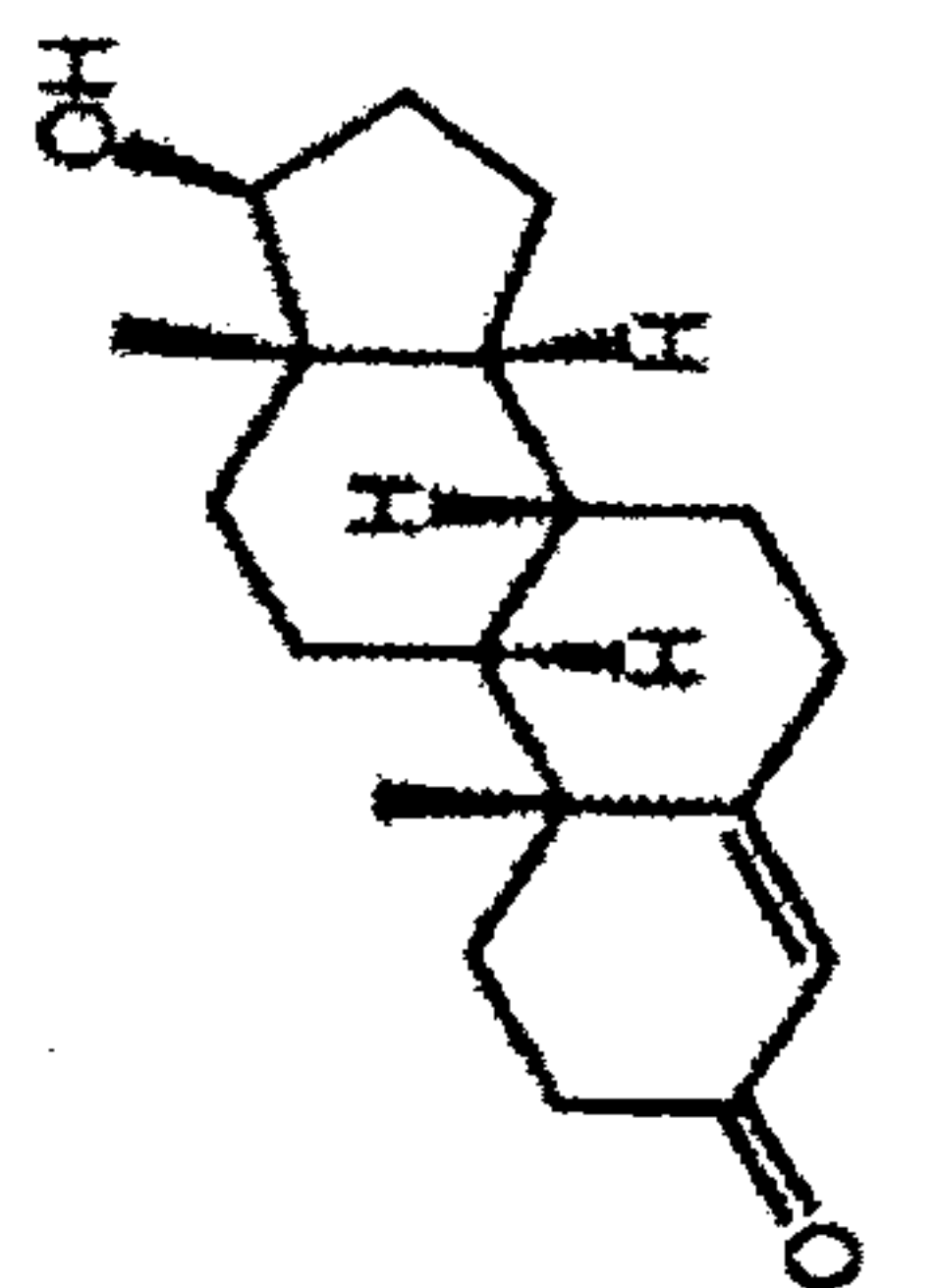
Testosterone
