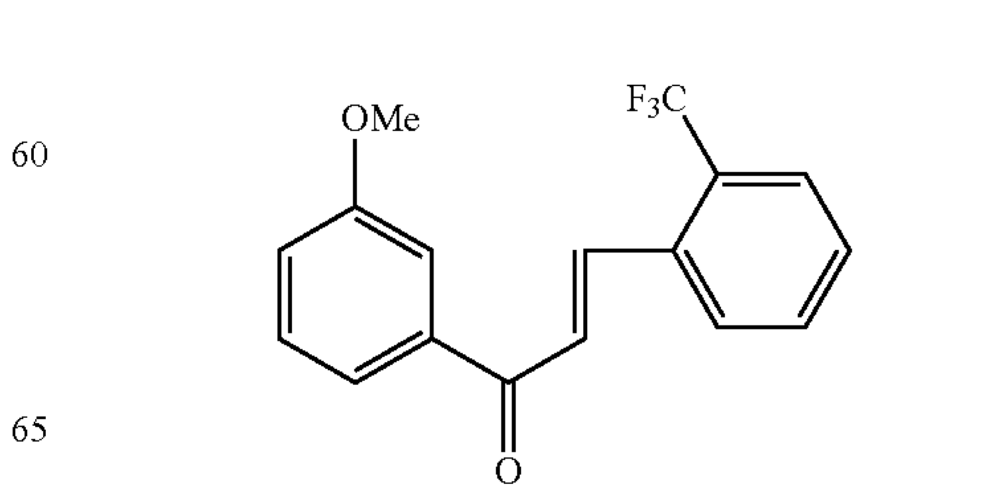
Compound 13
