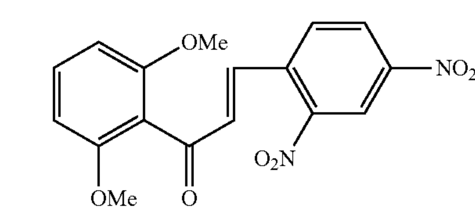
Compound 62
