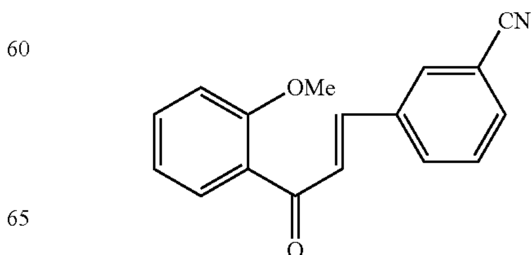
Compound 102
