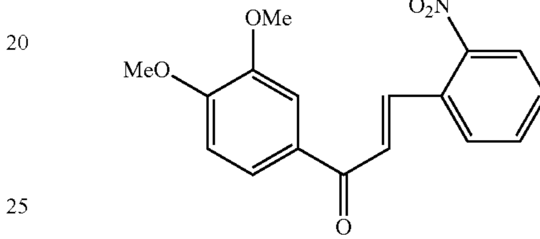
Compound 23
