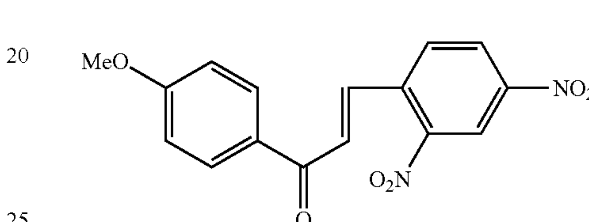
Compound 9
