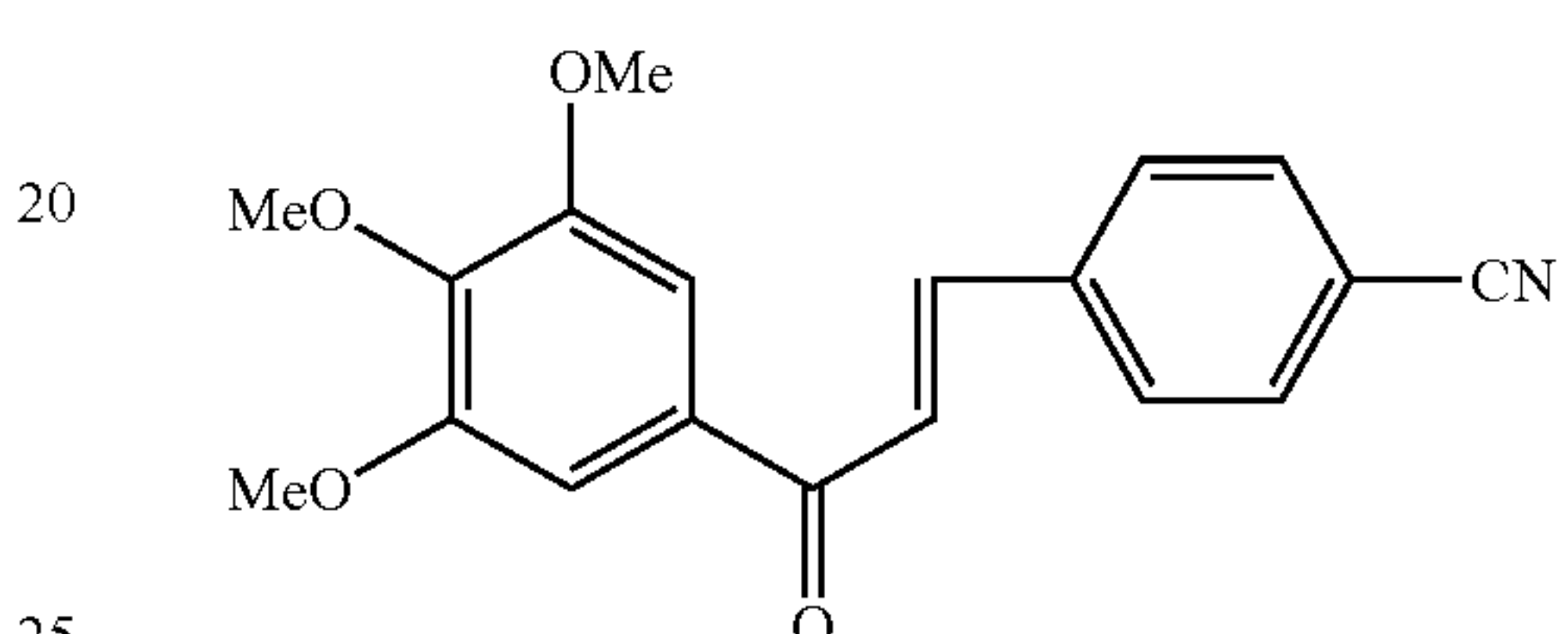
Compound 87
