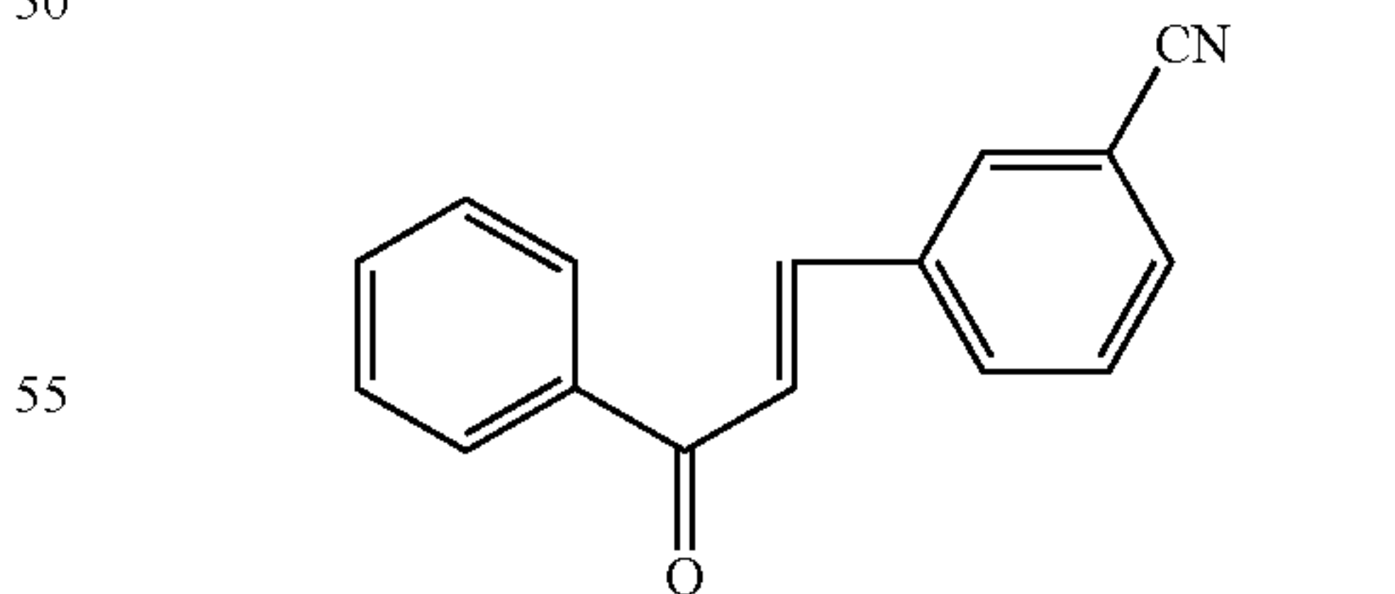
Compound 101
