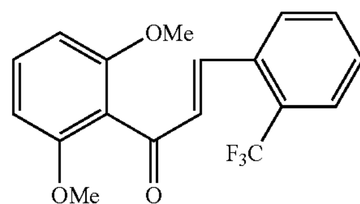
Compound 48
