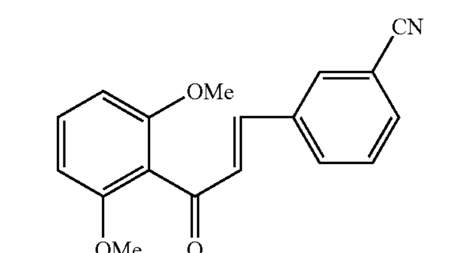
Compound 115
