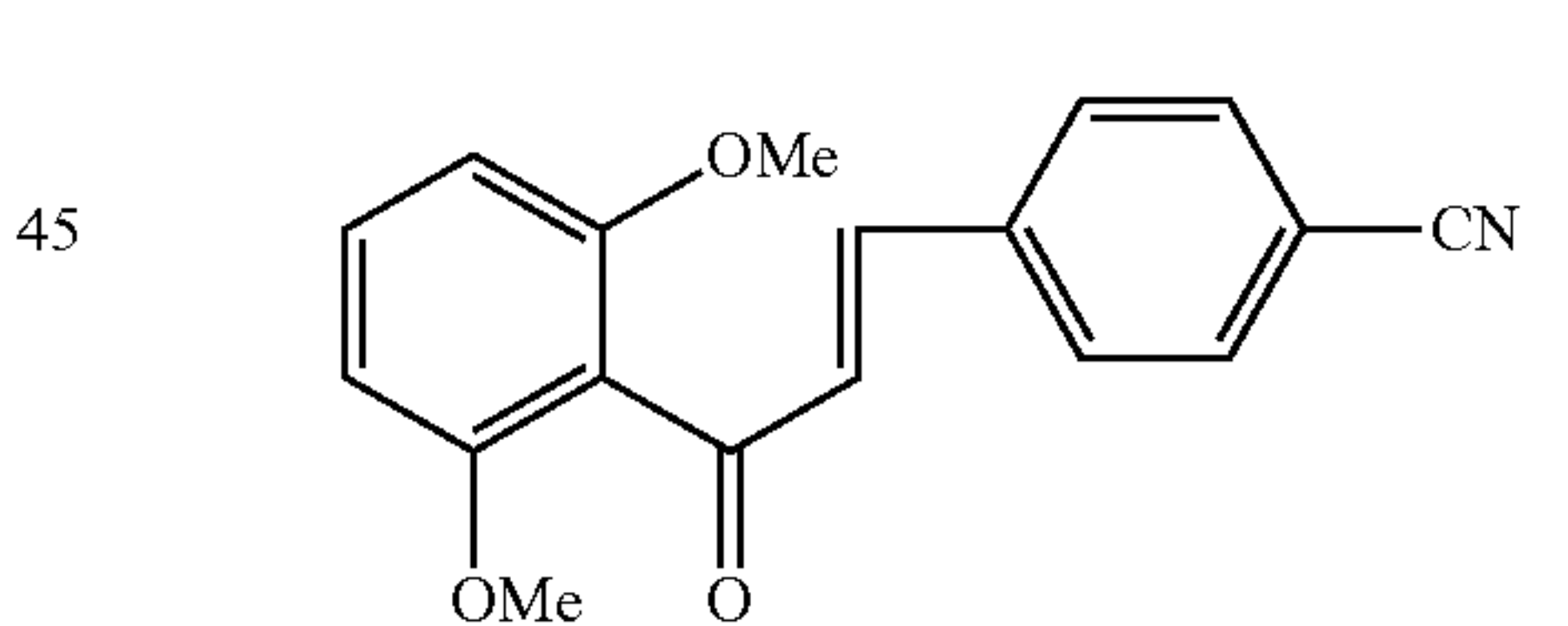
Compound 95
