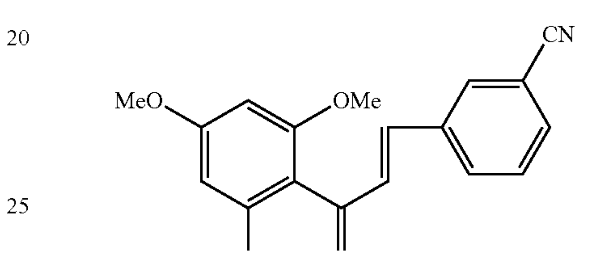
Compound 89
