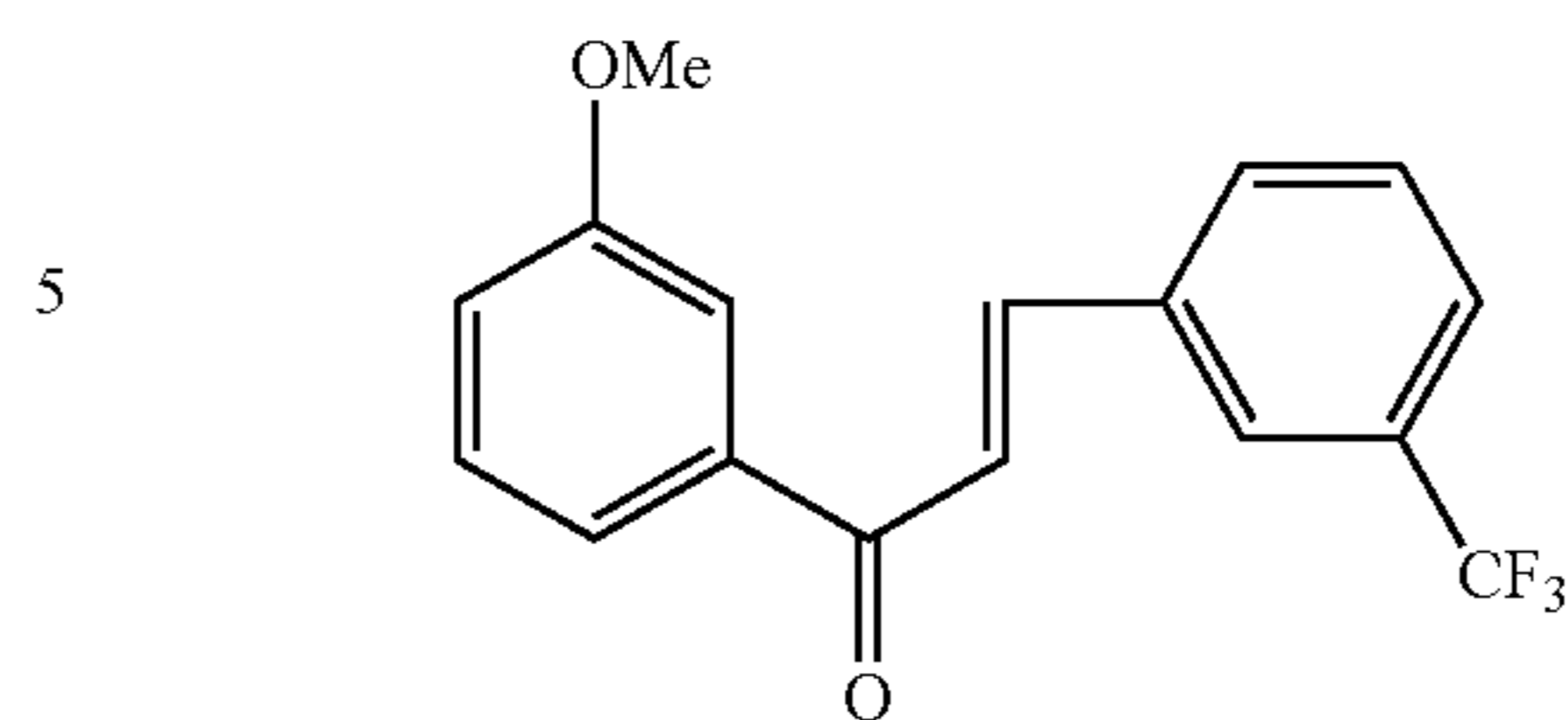
Compound 21
