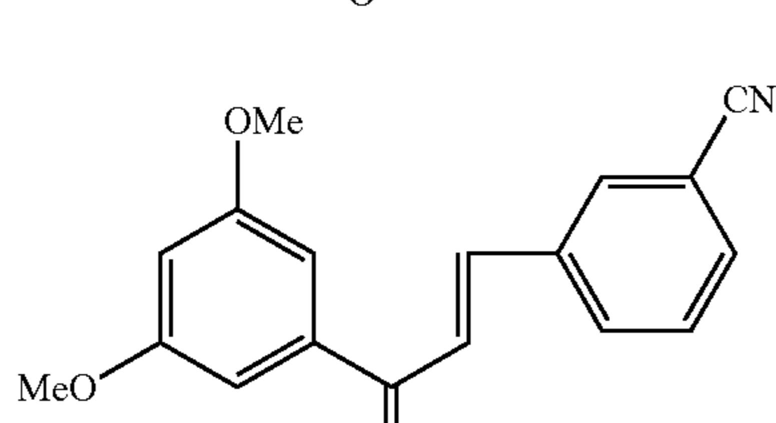
Compound 117
