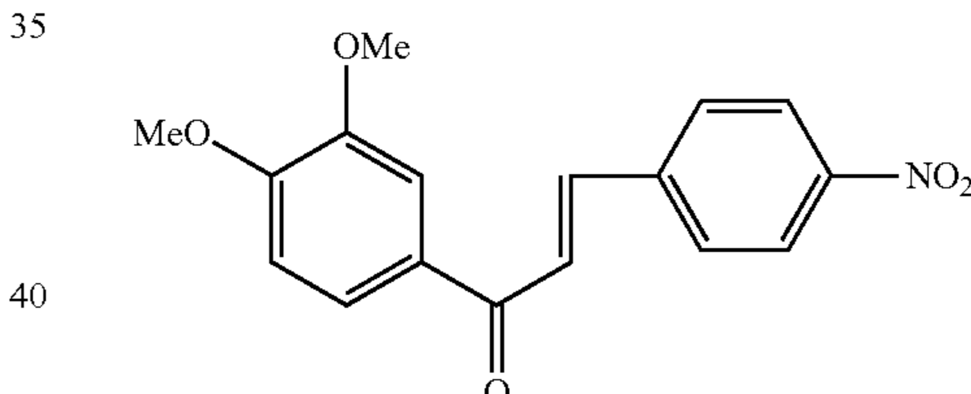
Compound 32
