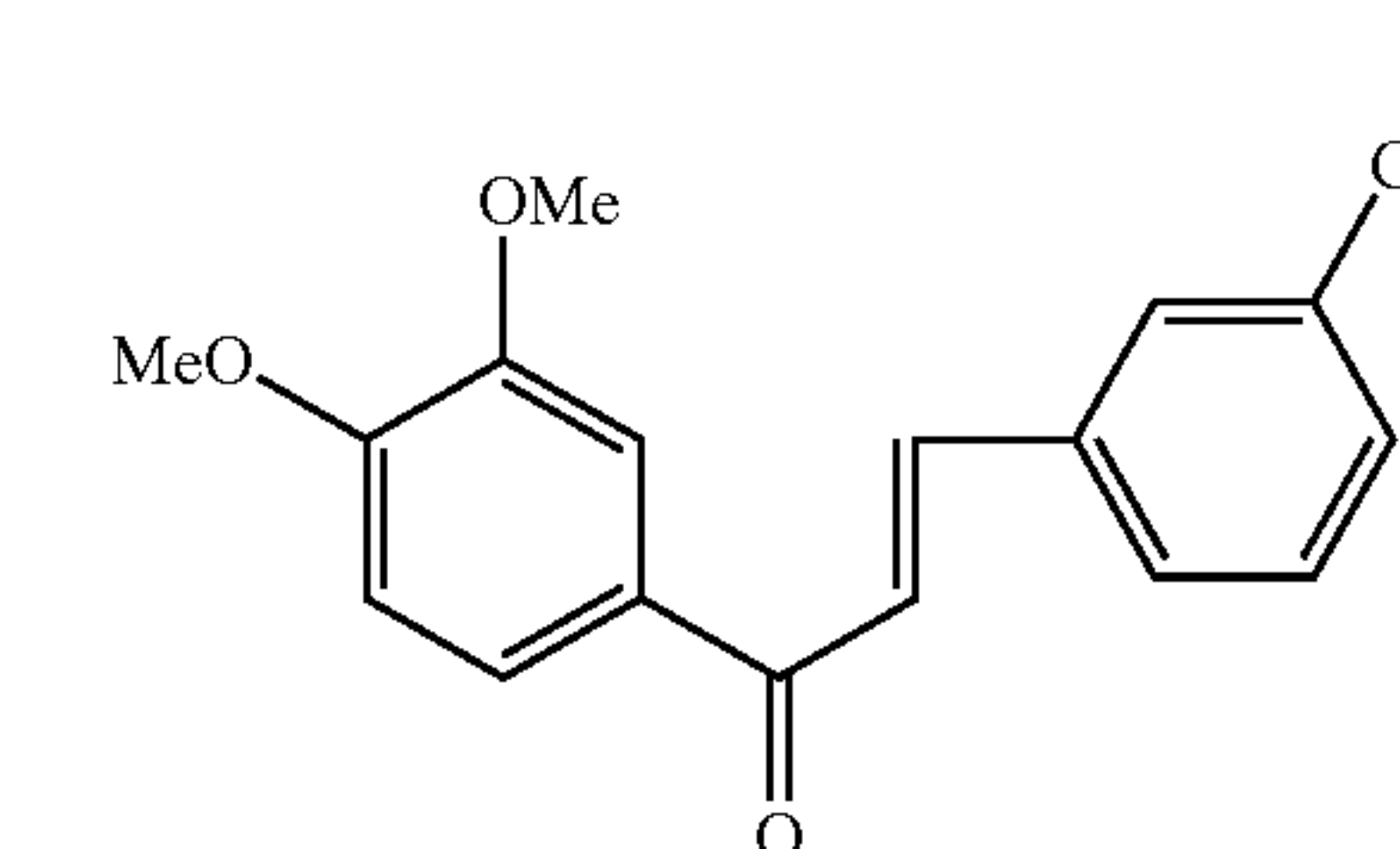
Compound 116
