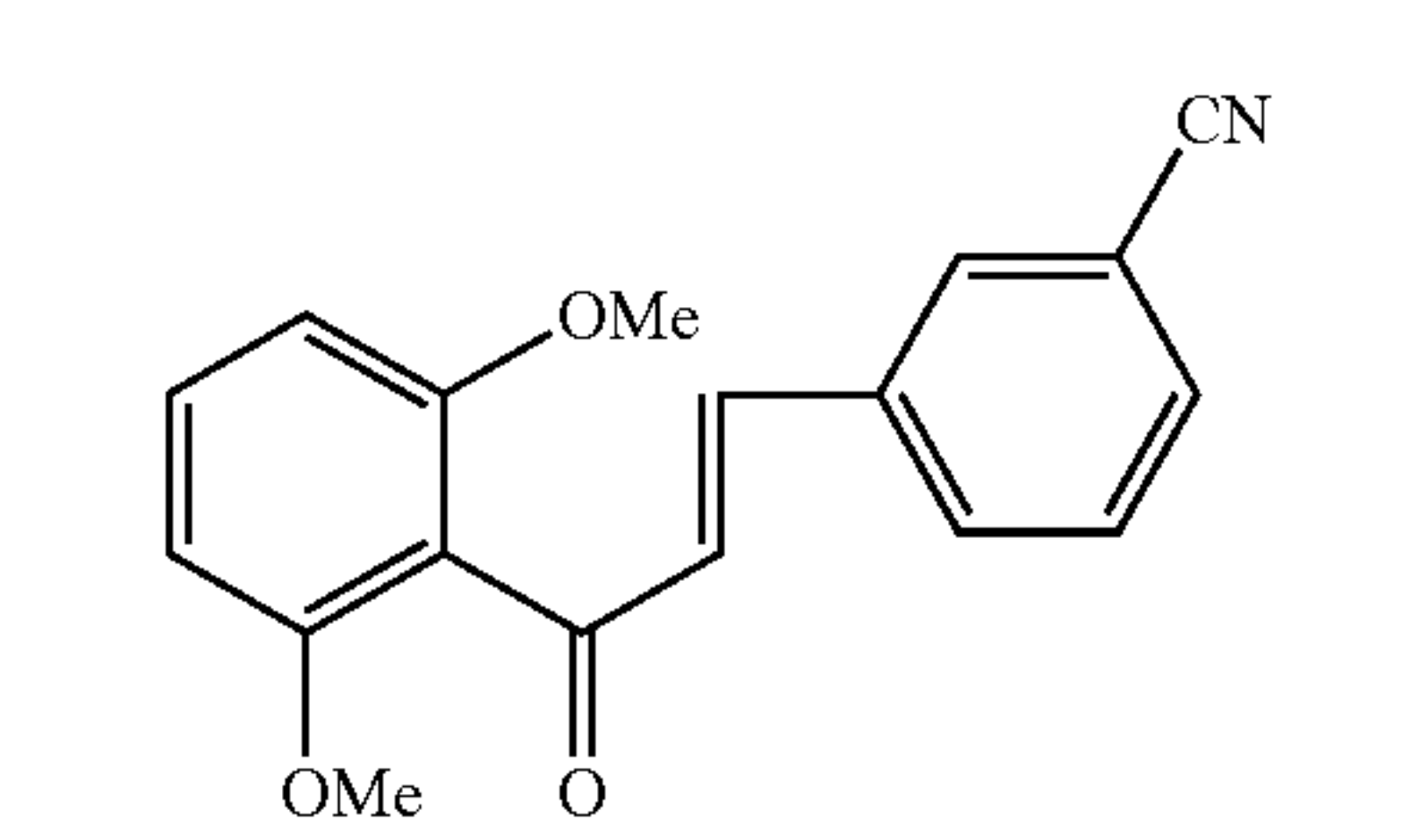
Compound 115
