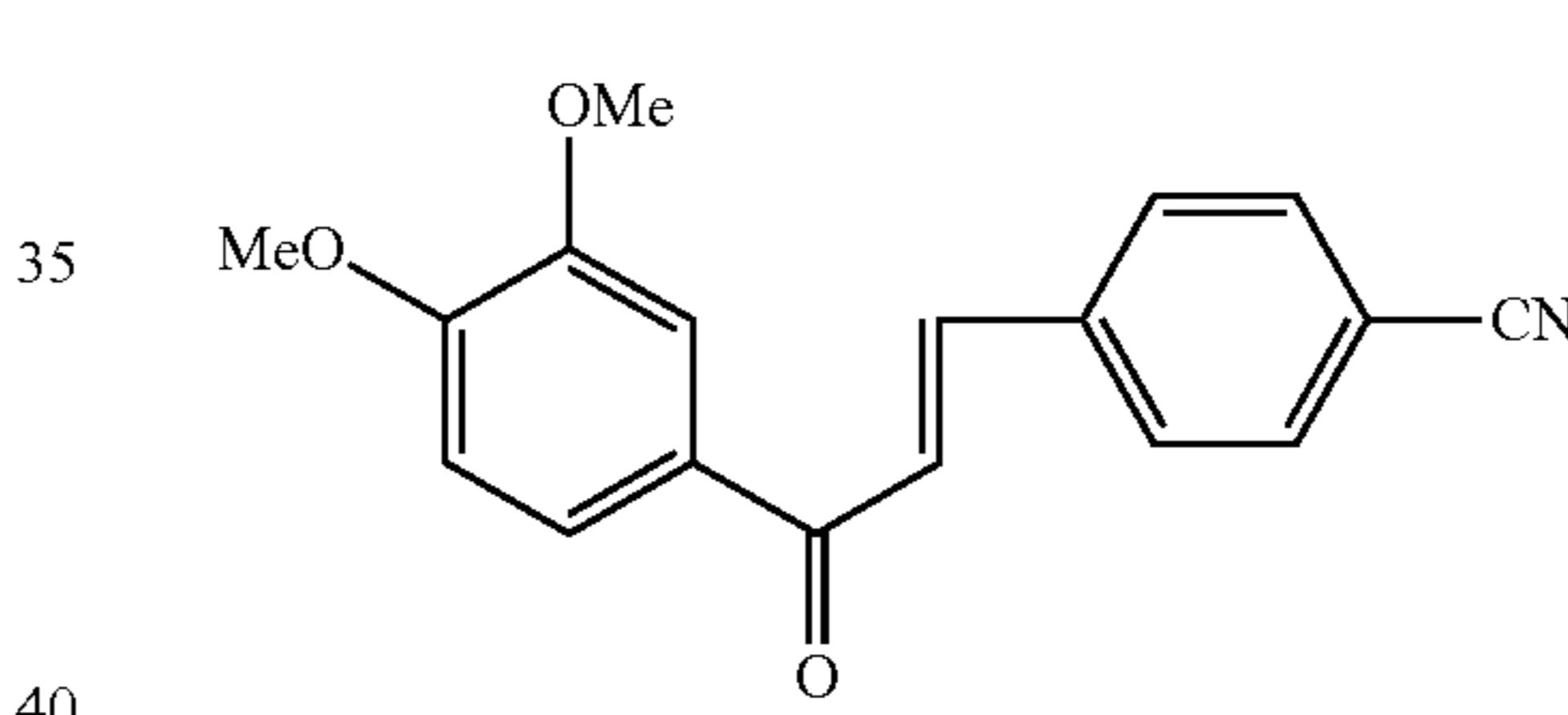
Compound 95
