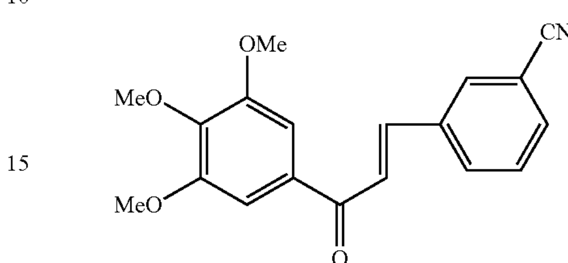
Compound 91
