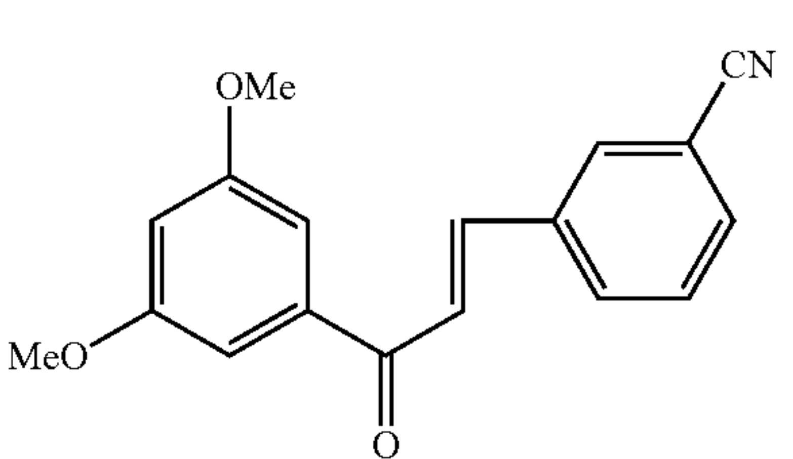
Compound 117
