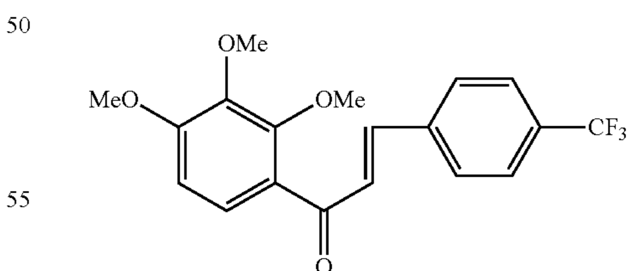
Compound 12
