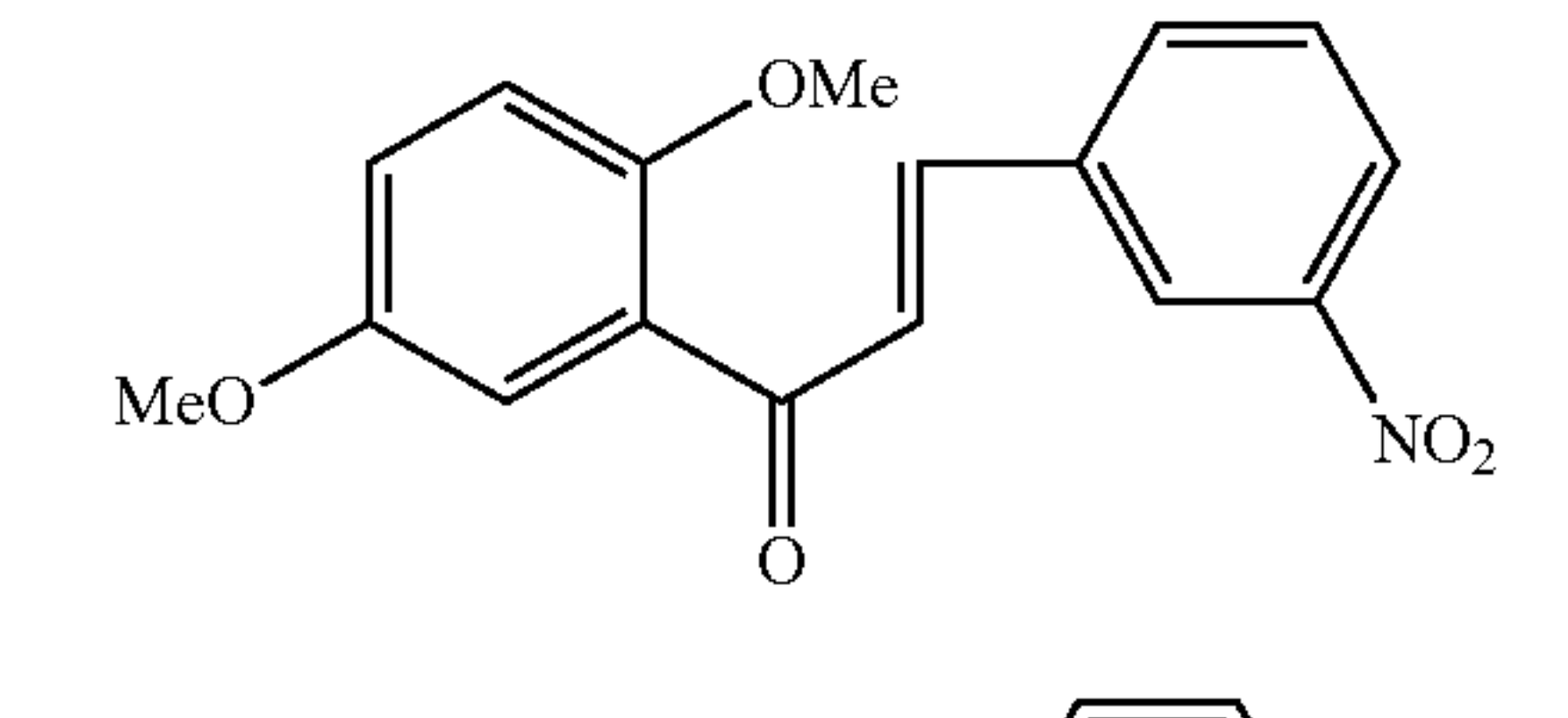
Compound 39
