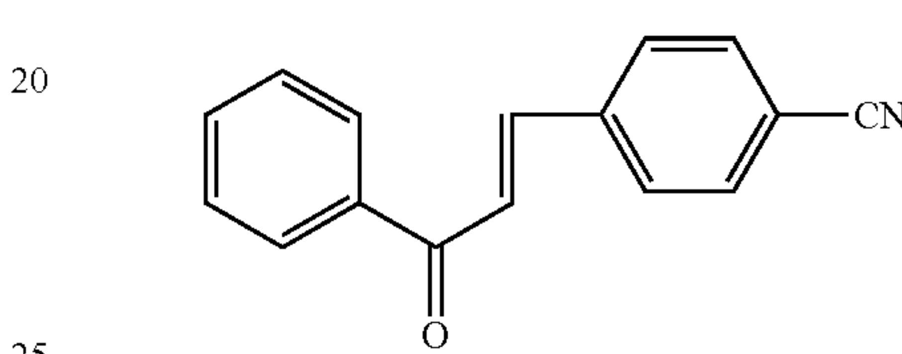
Compound 97
