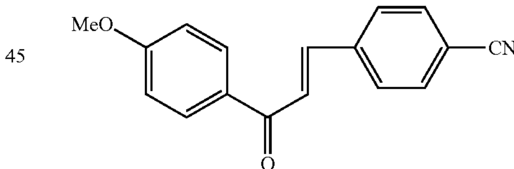
Compound 100
