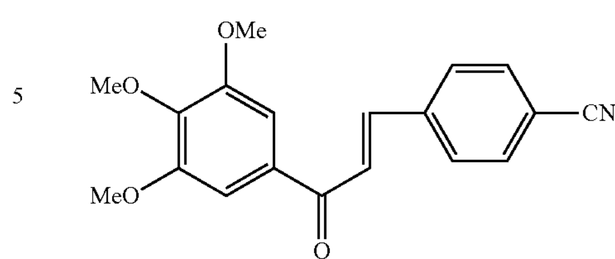
Compound 87
