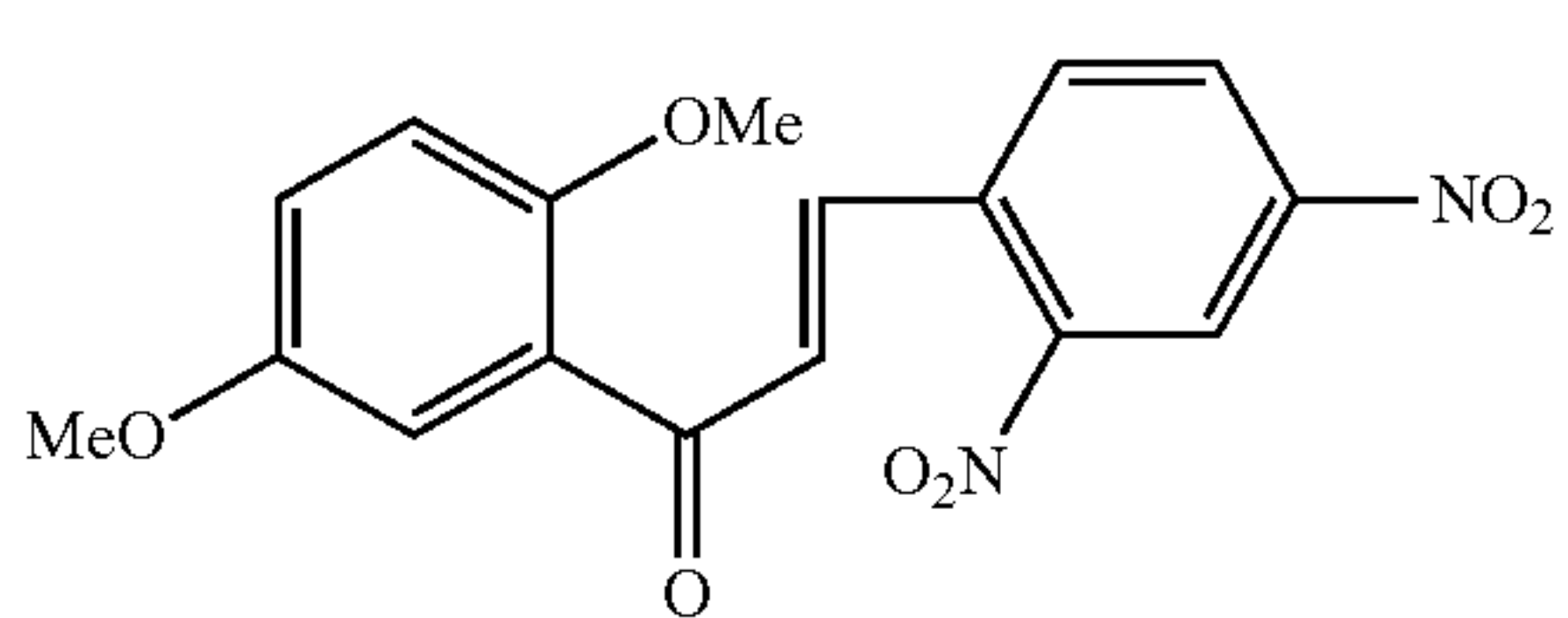
Compound 61
