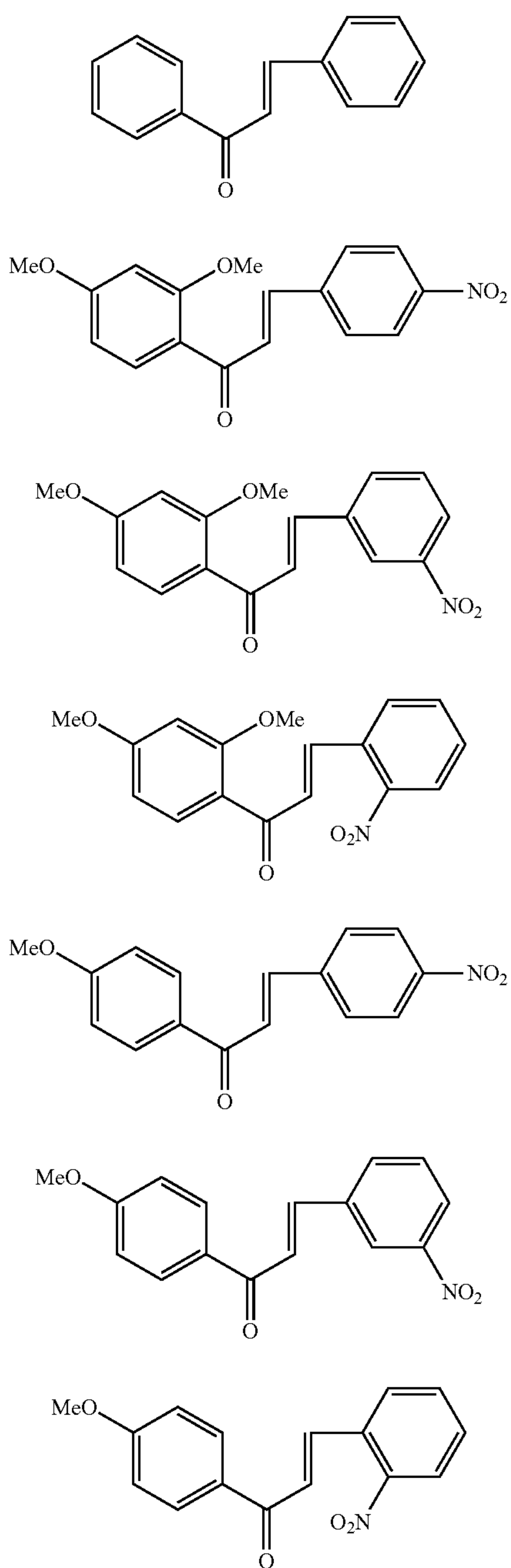
Compound 2
