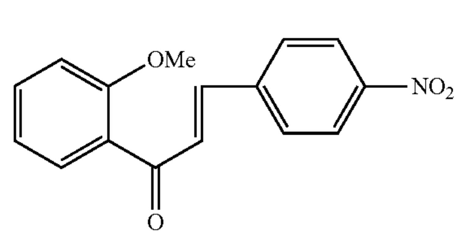
Compound 52
