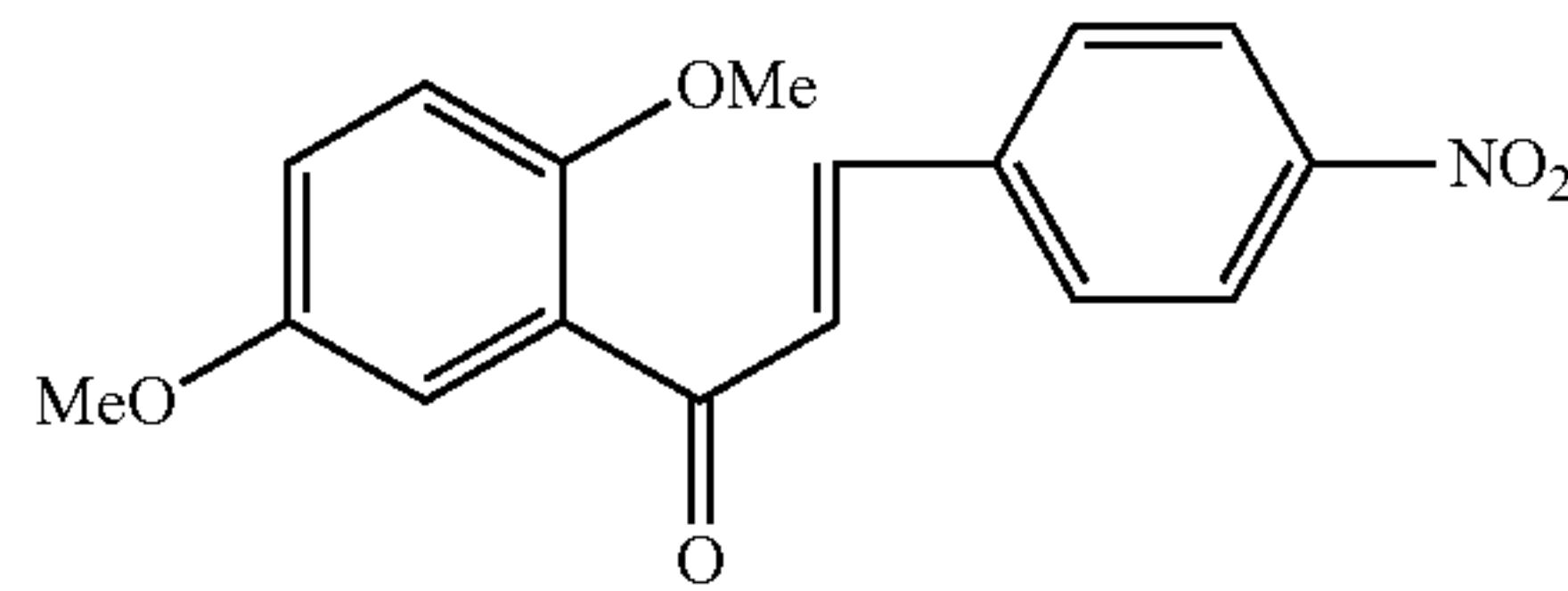
40
