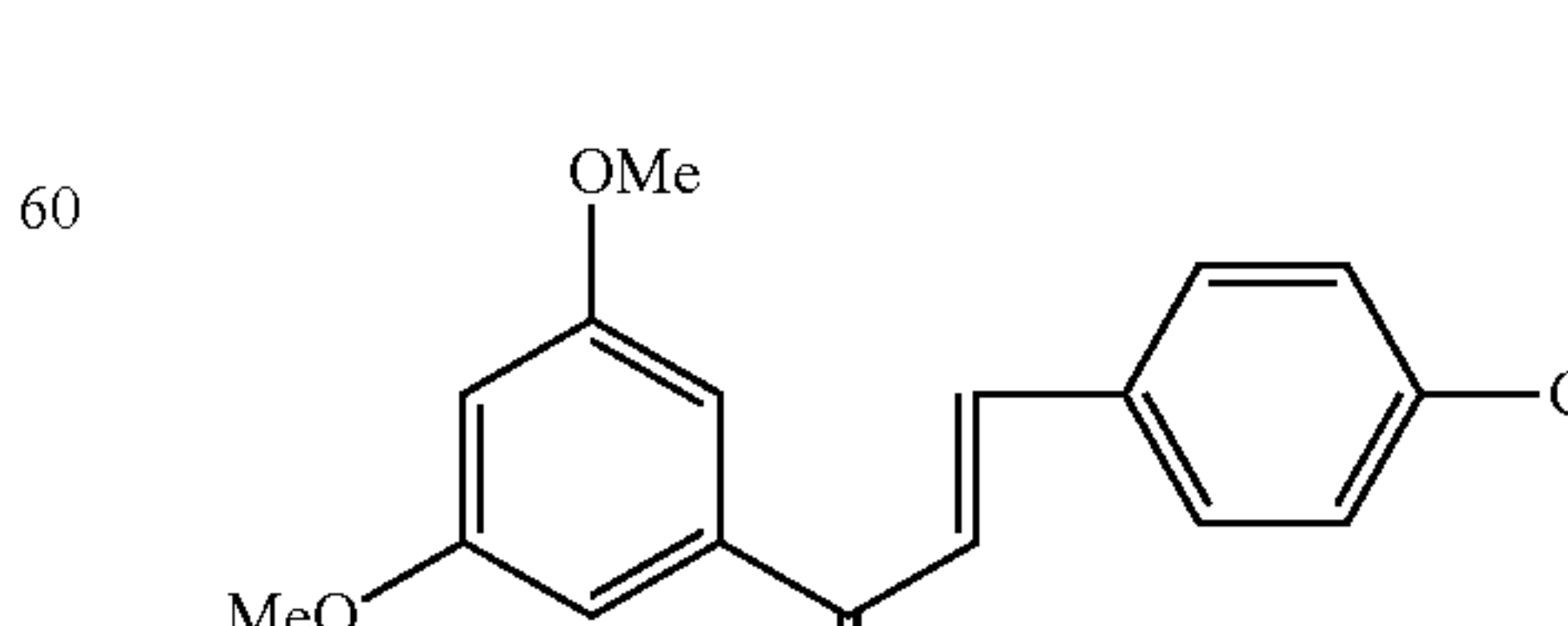
Compound 96
