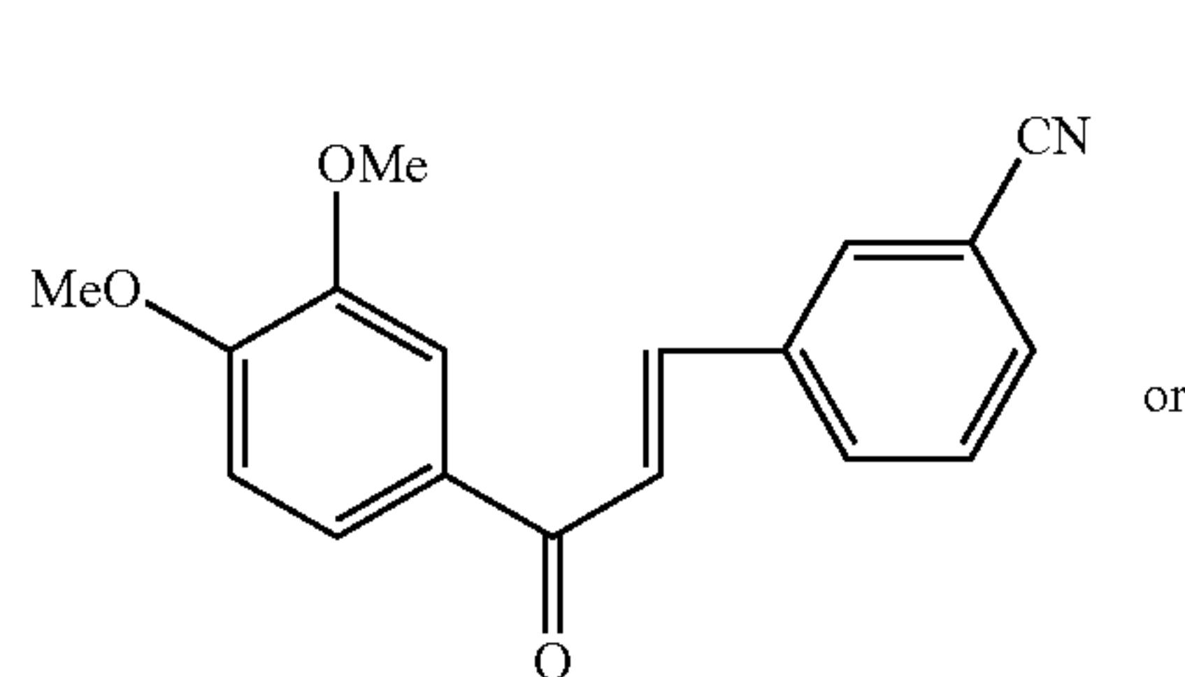
Compound 116
