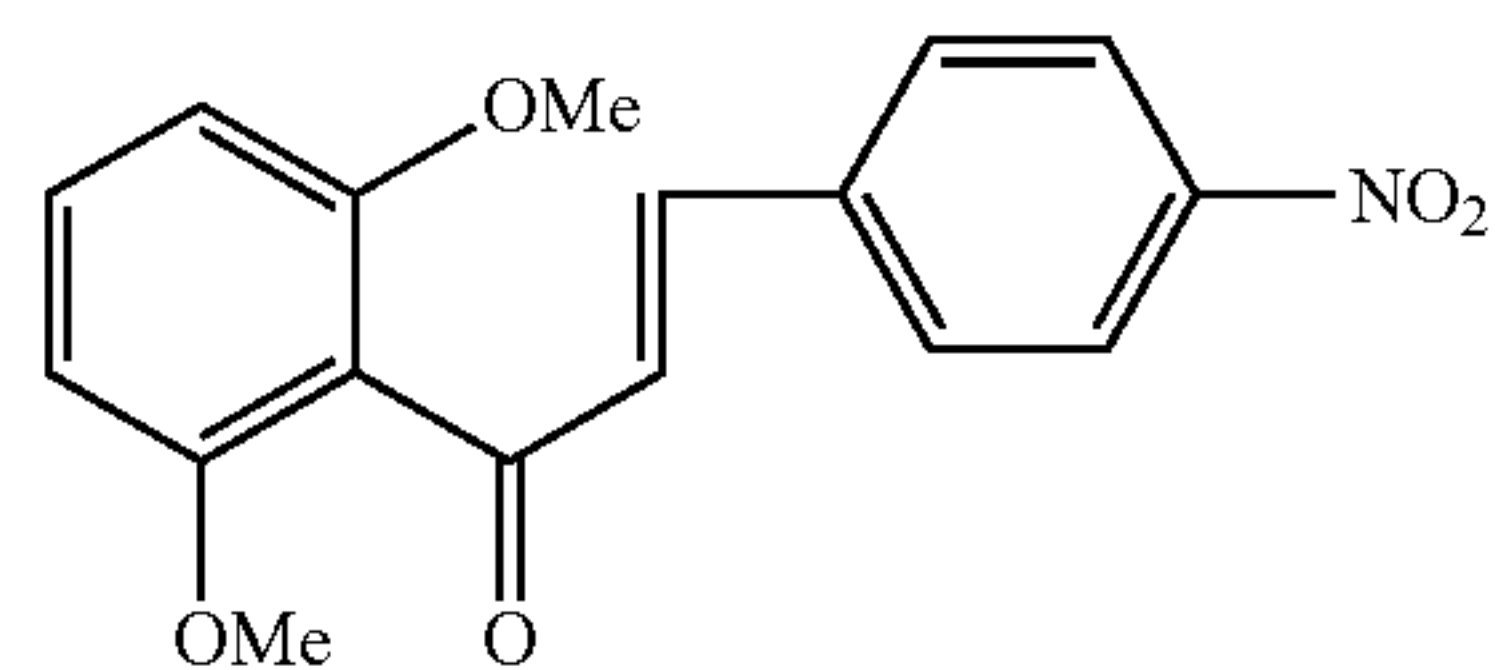
Compound 46
