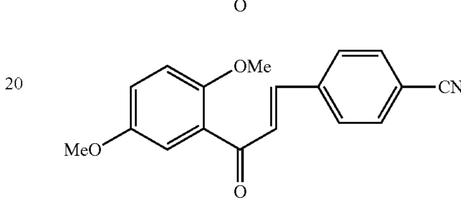
Compound 91
