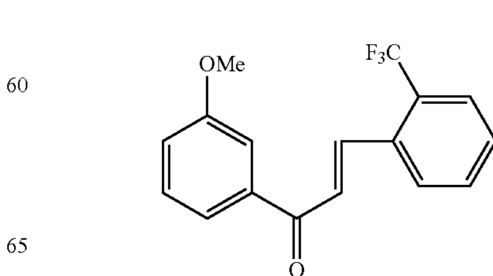
Compound 13
