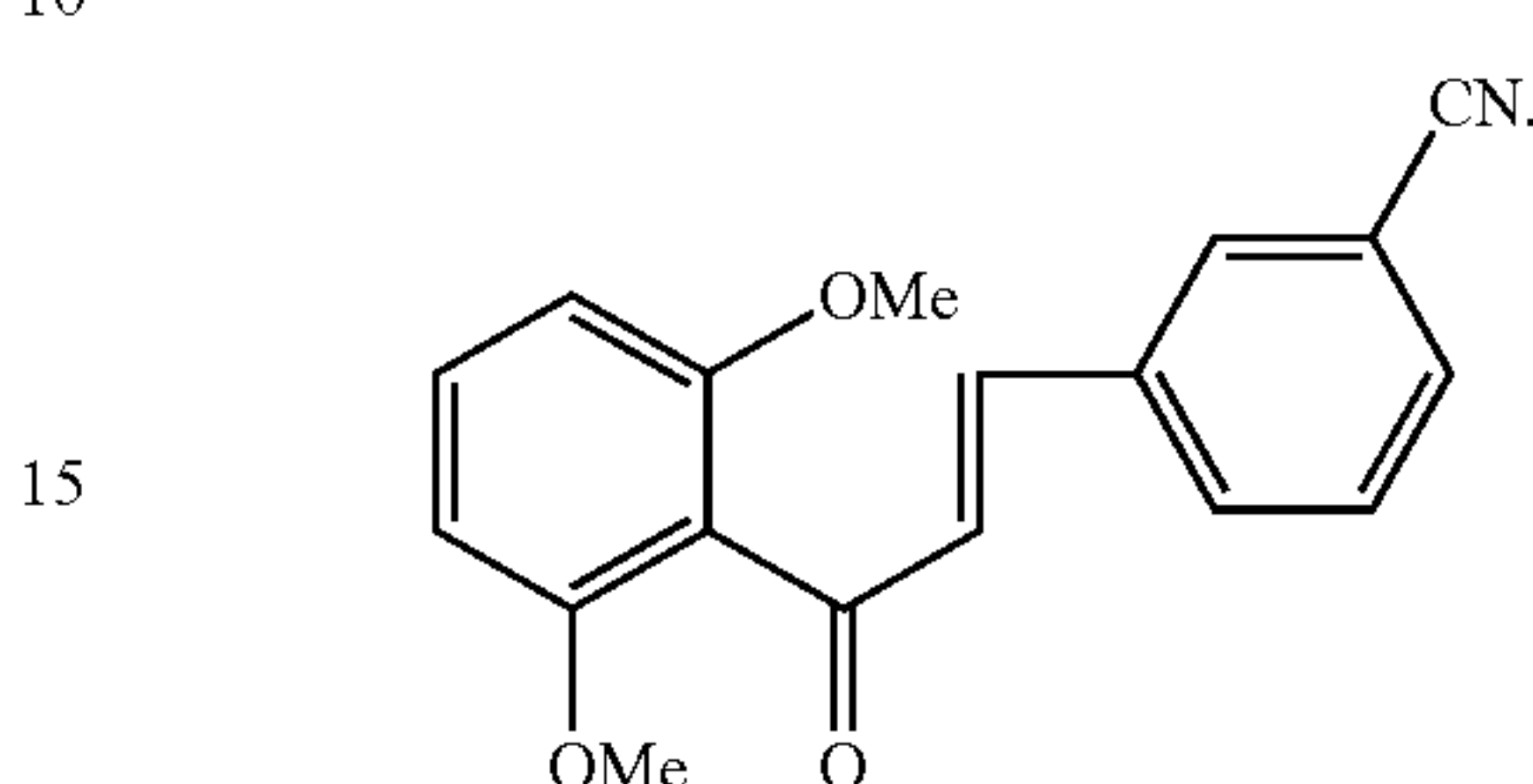
Compound 61
