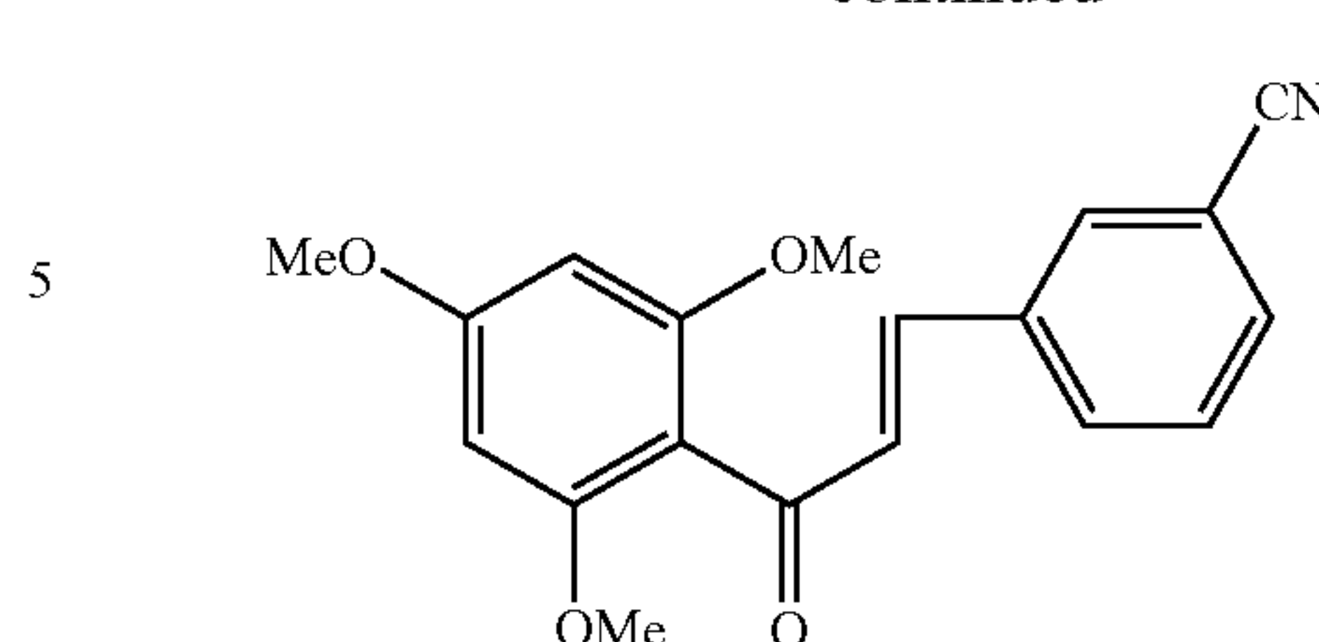
Compound 89
