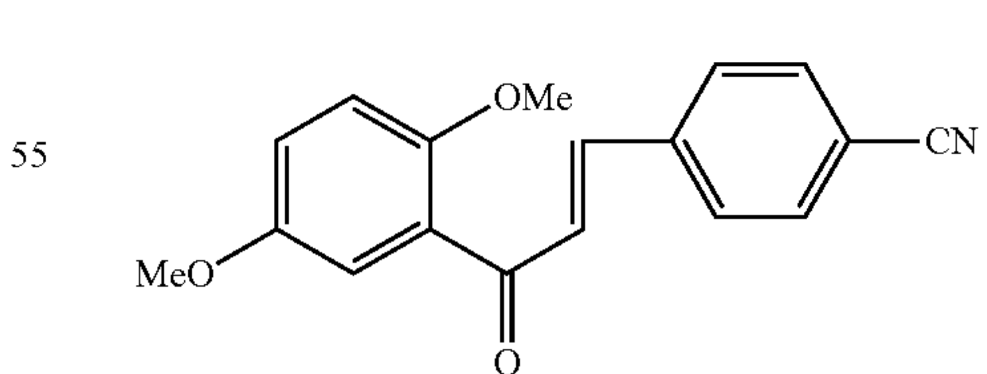
Compound 101
