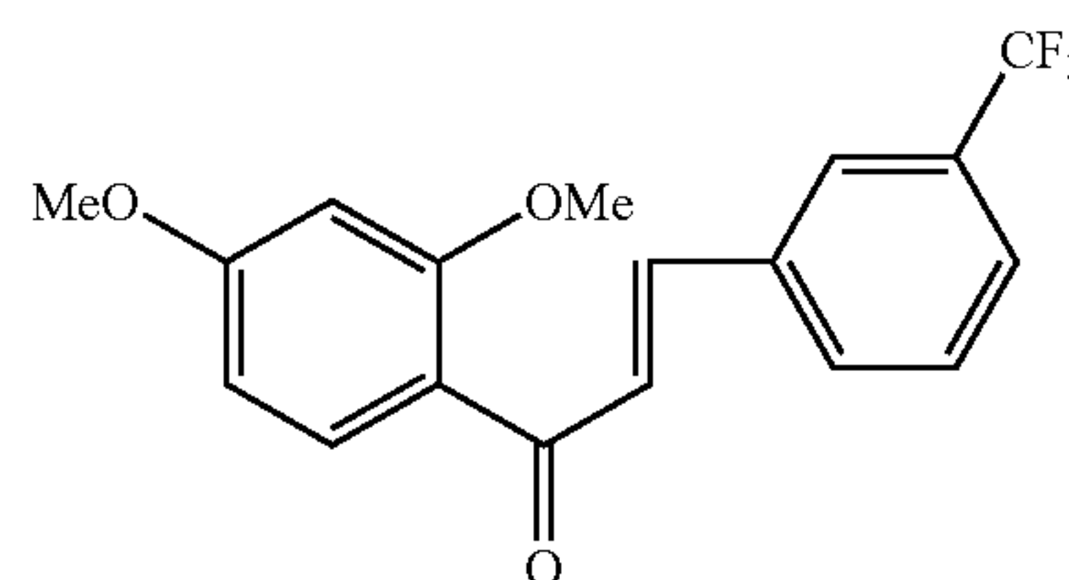
Compound 19
