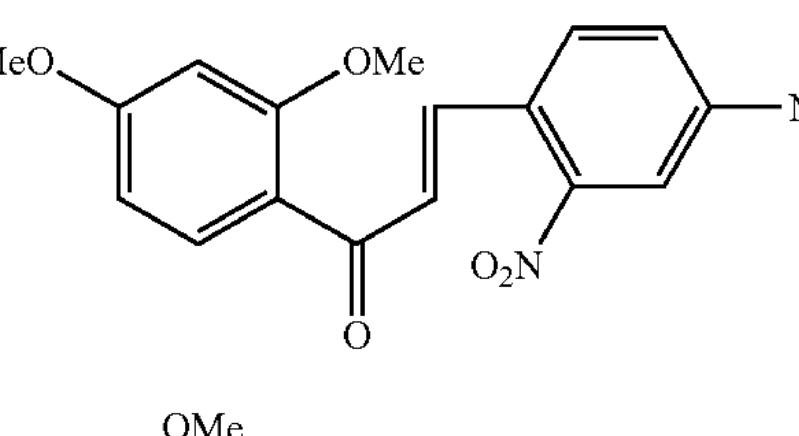
Compound 28
