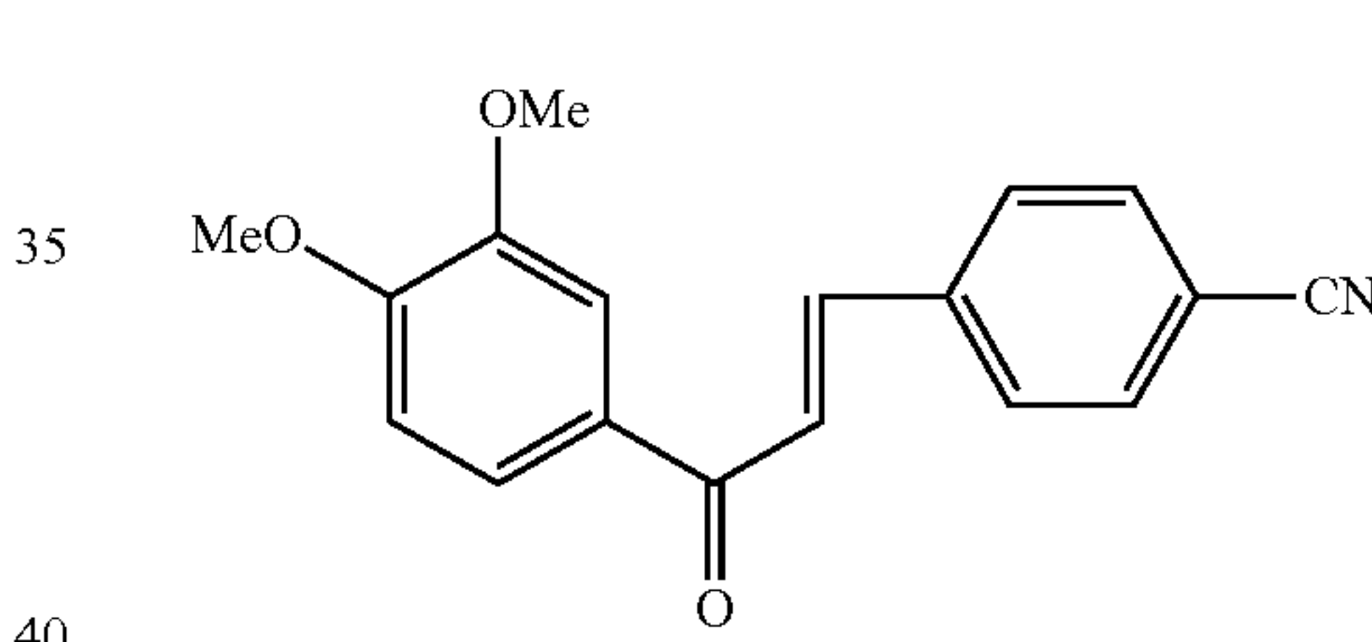
Compound 95
