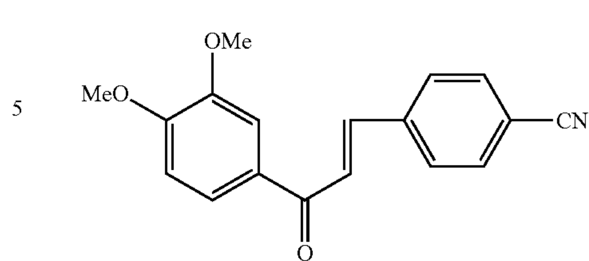
Compound 95
