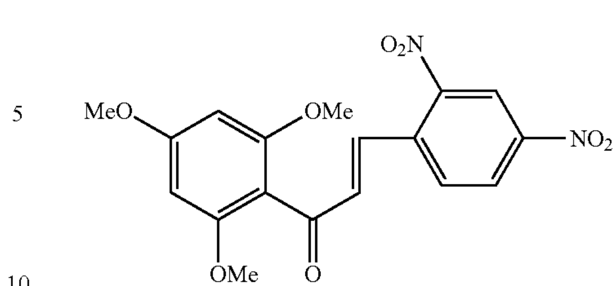
Compound 84
