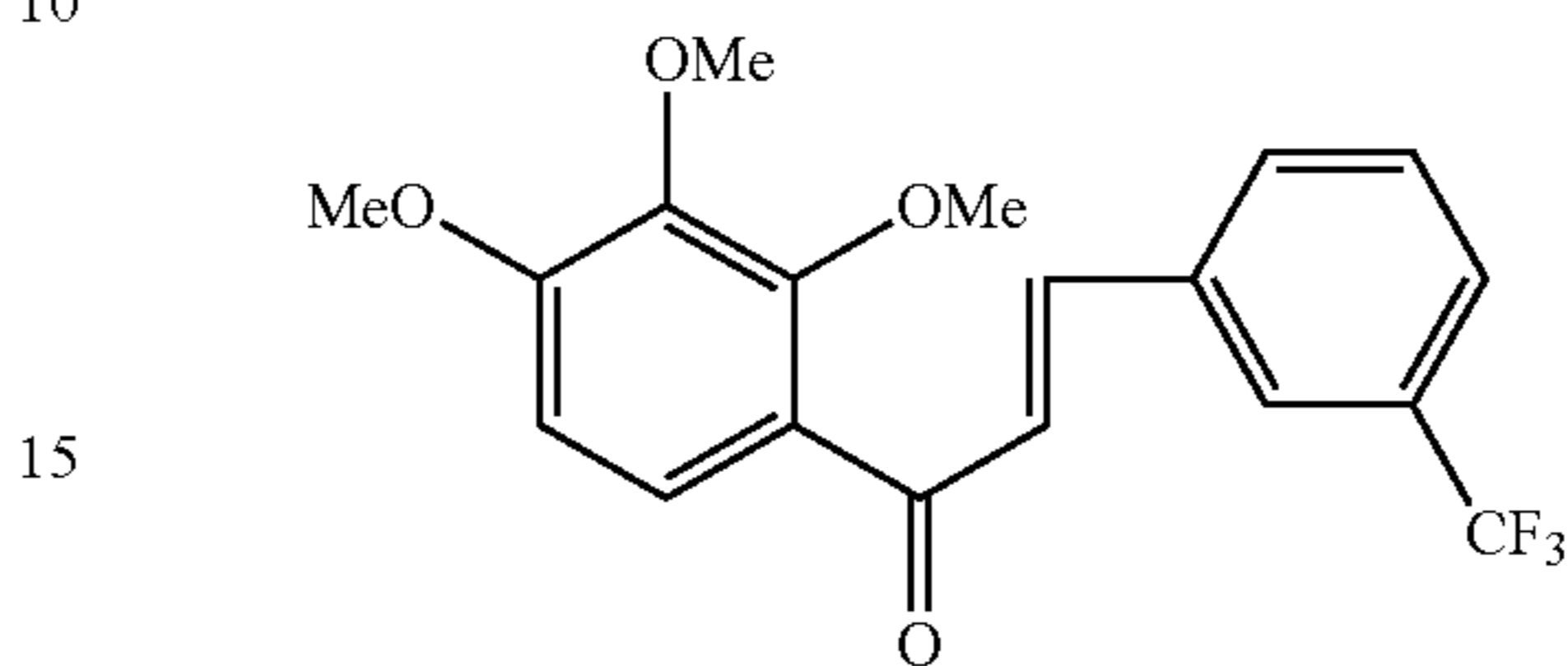
Compound 22
