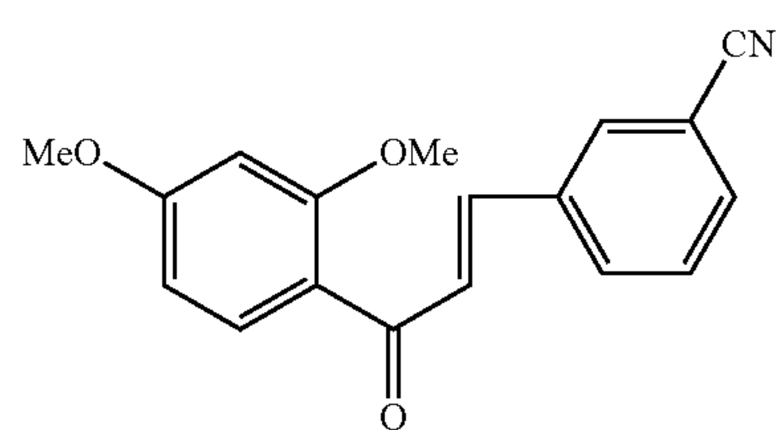
Compound 113
