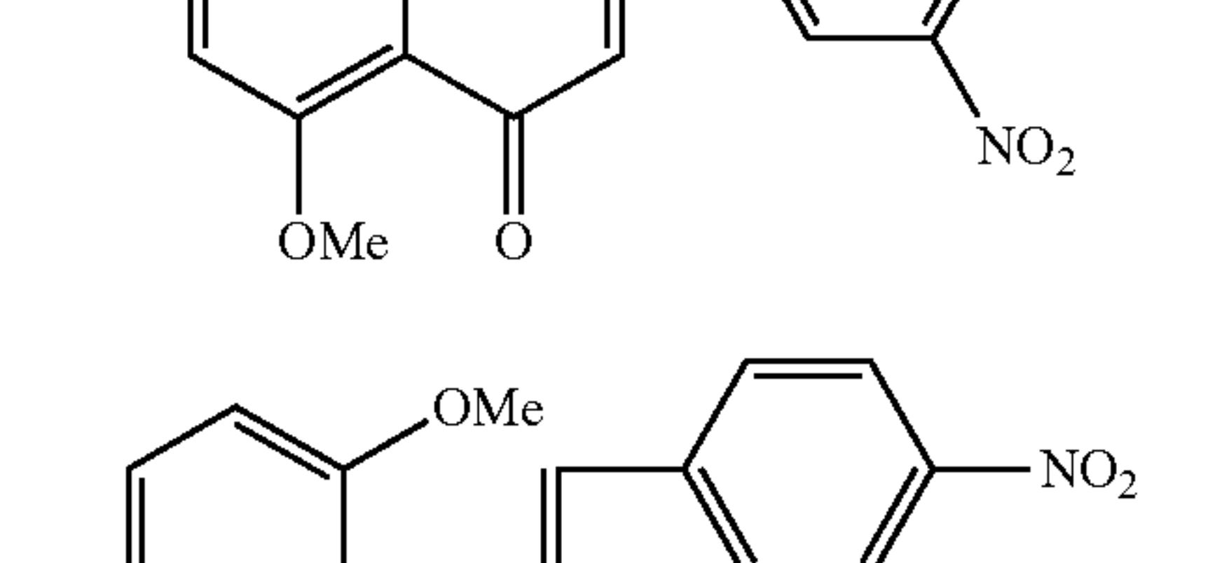
Compound 45
