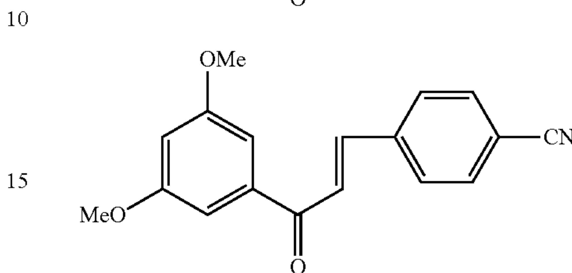
Compound 96
