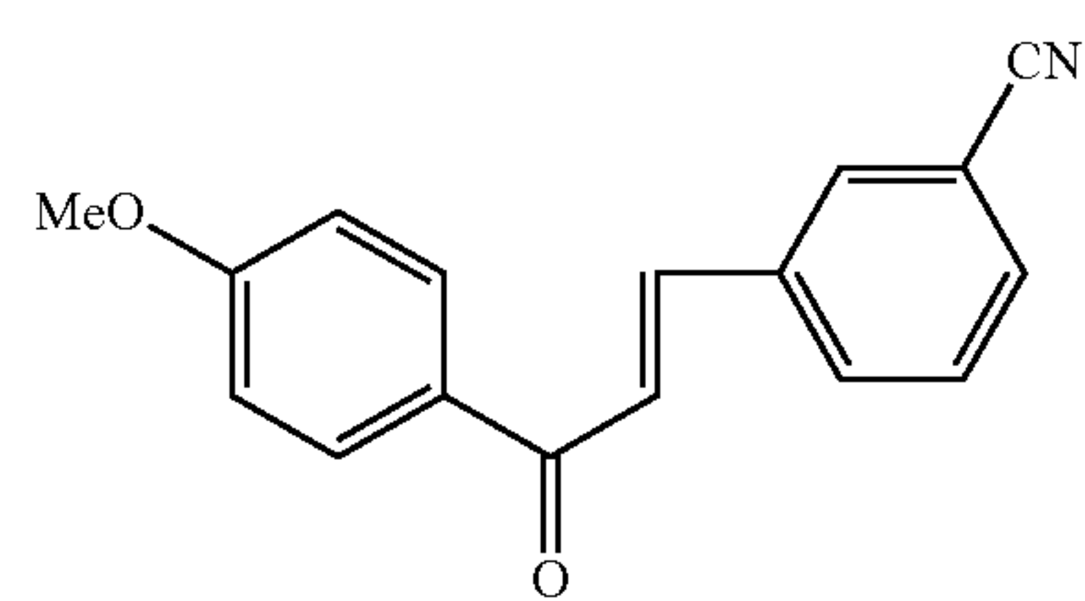
Compound 112
