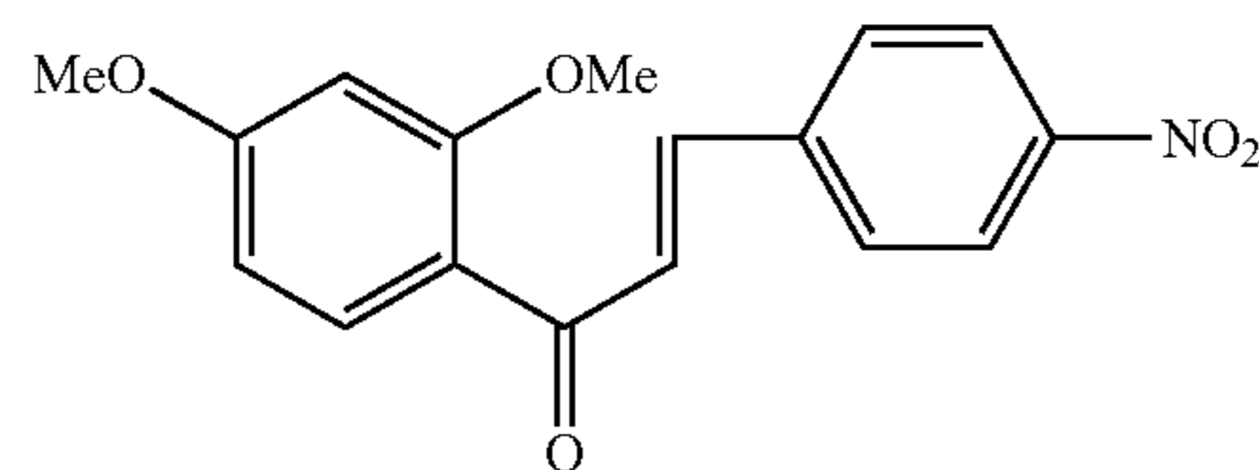
Compound 113
