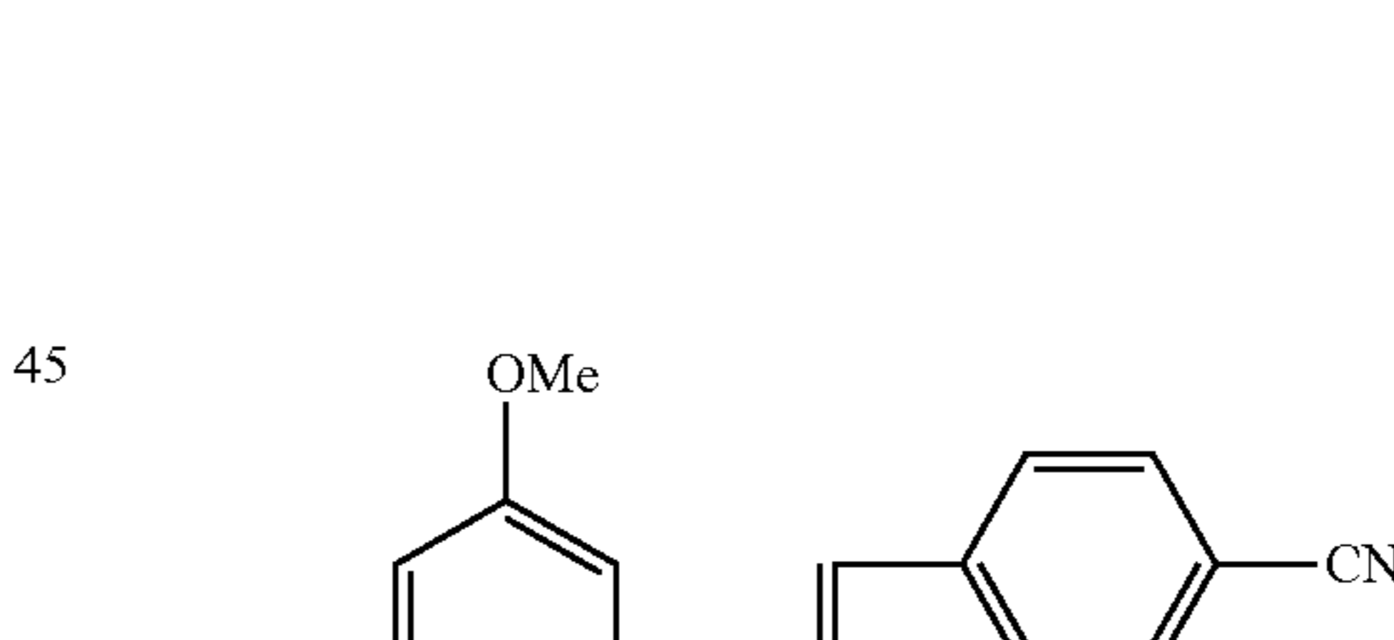
Compound 96
