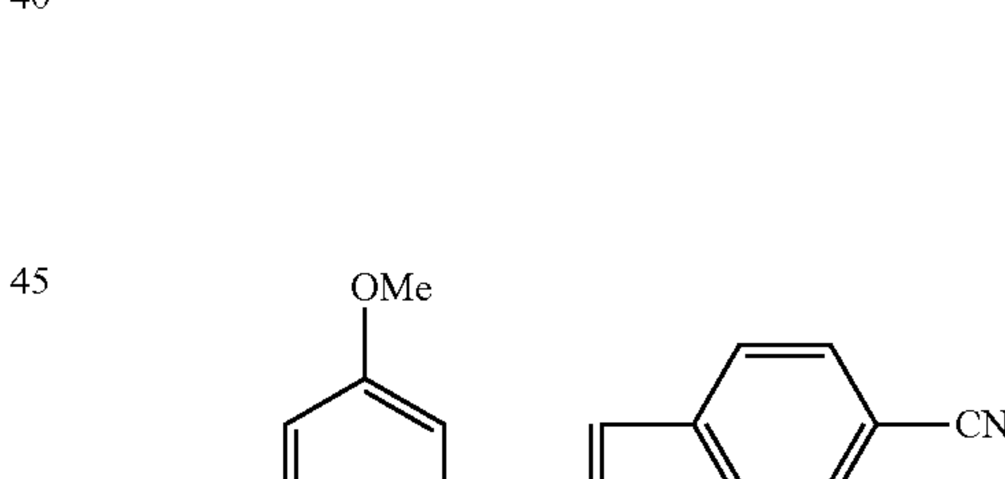
Compound 96
