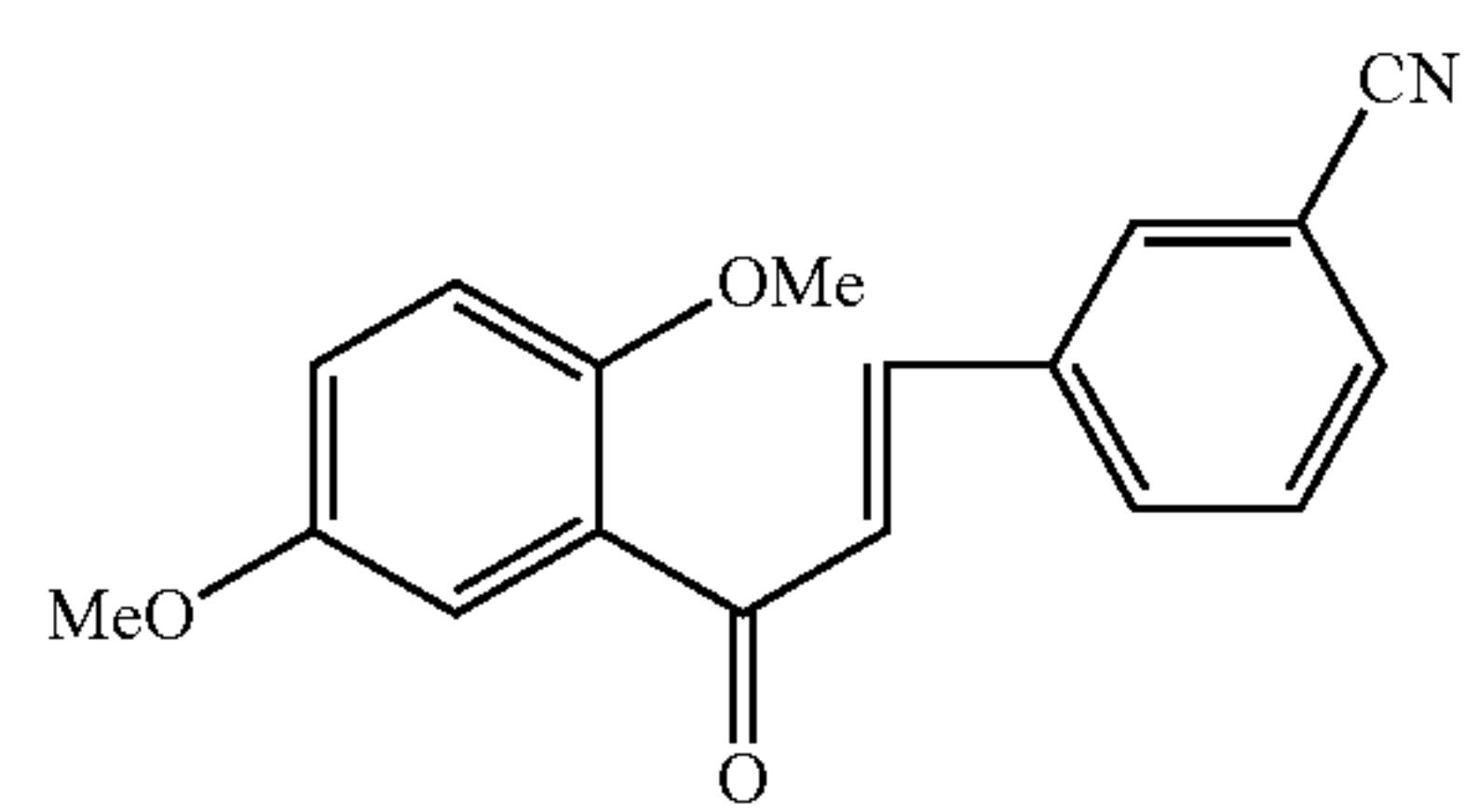
Compound 114
