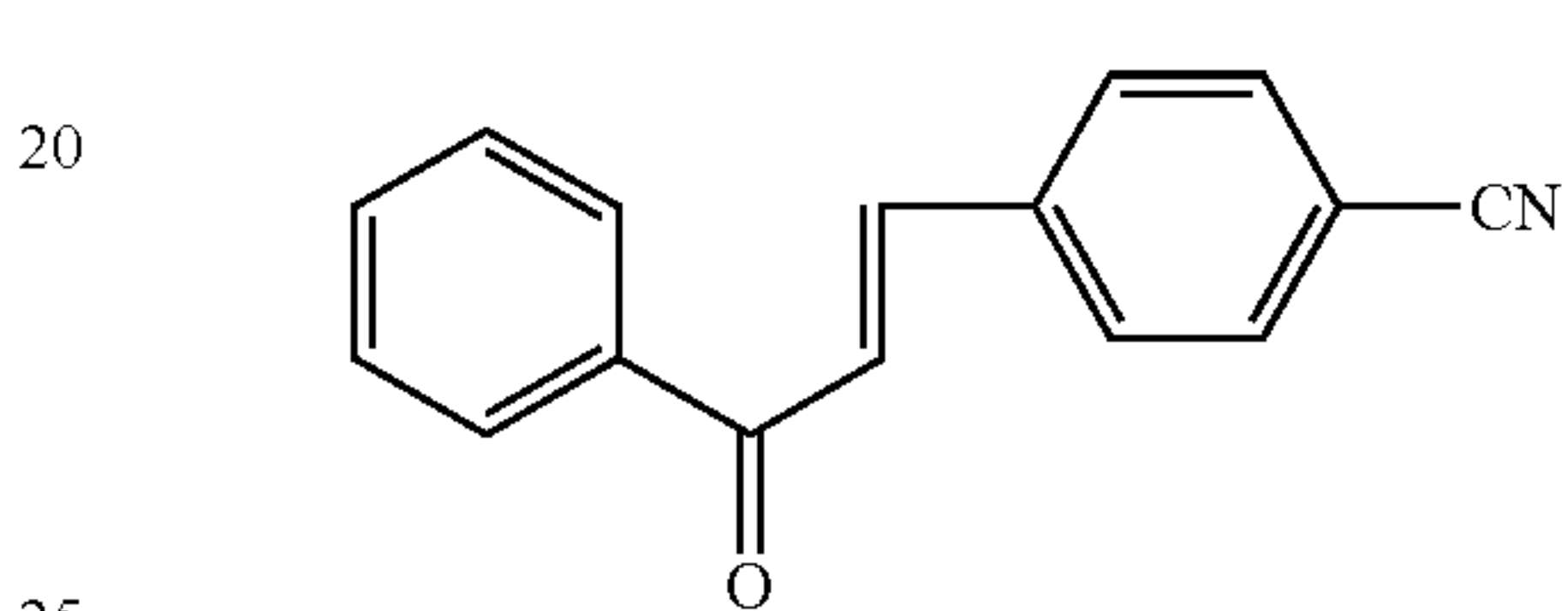
Compound 97
