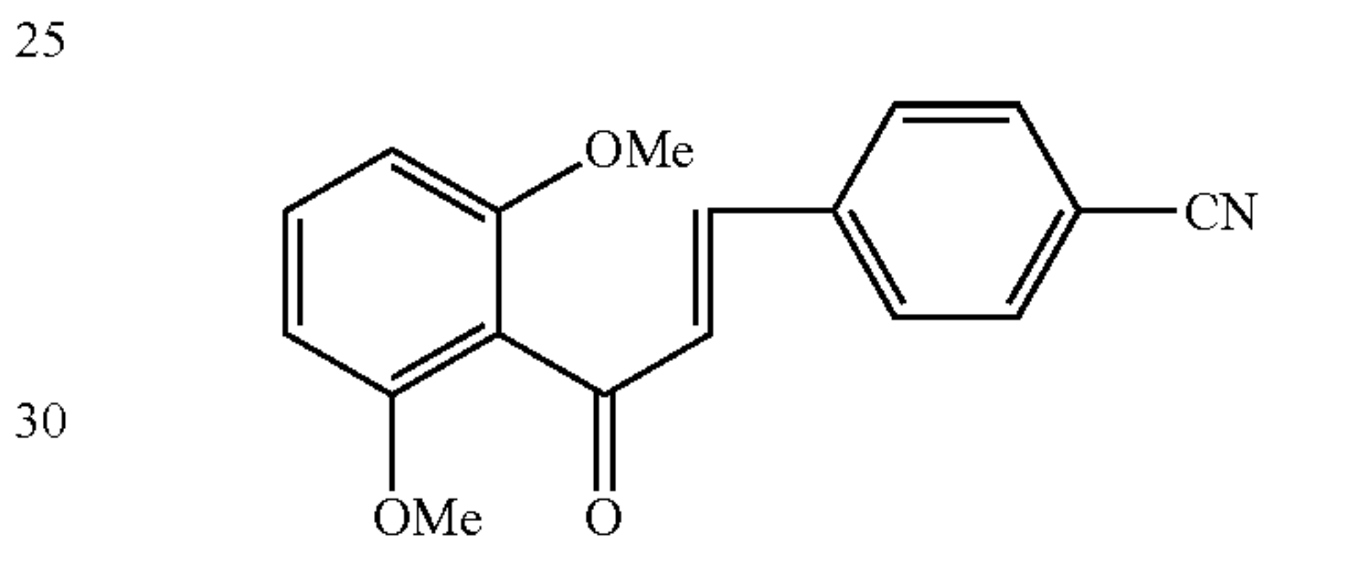
Compound 94
