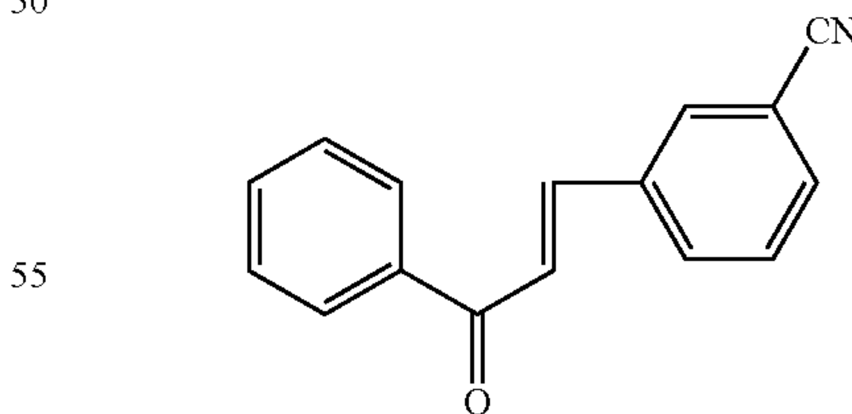
Compound 101
