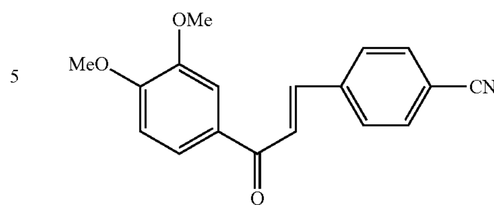
Compound 95
