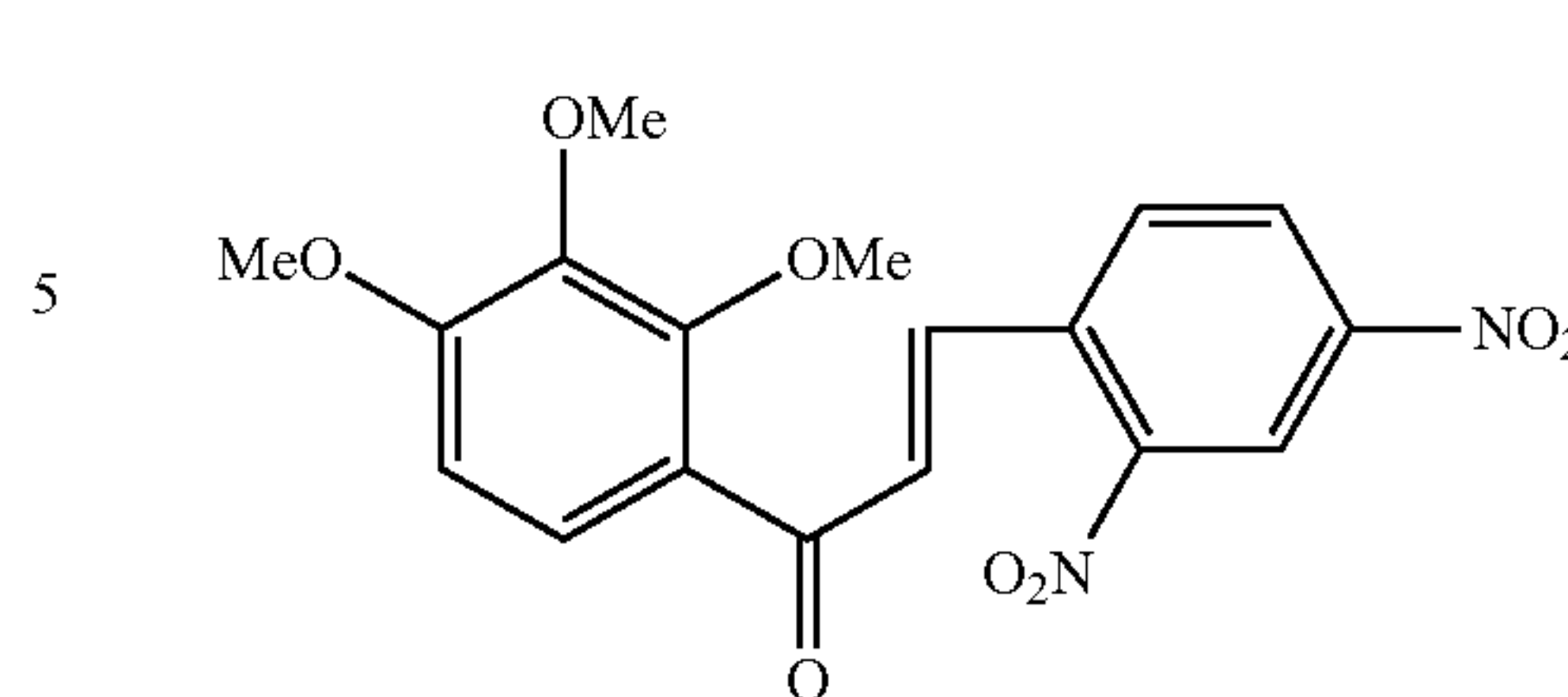
Compound 6
