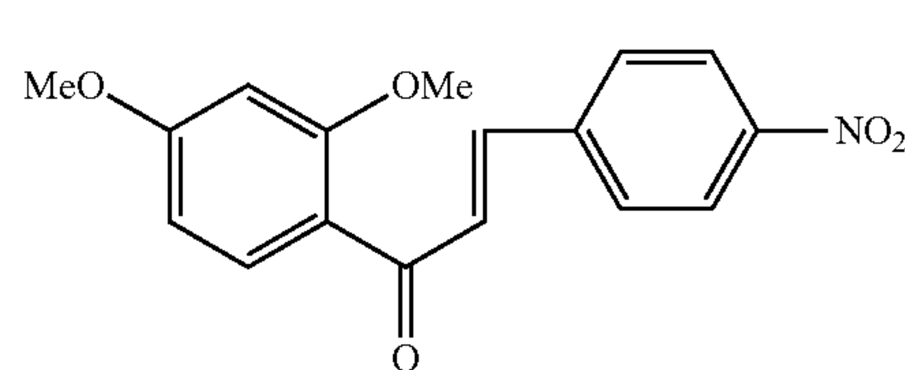
Compound 2
