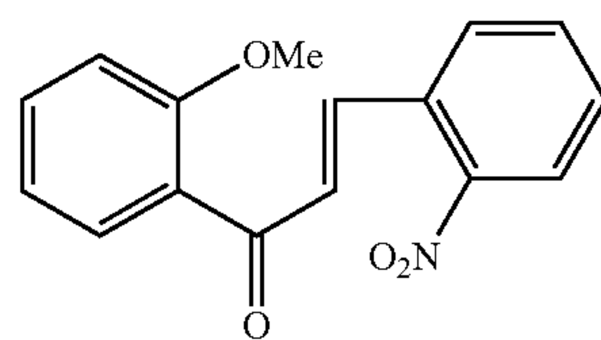
Compound 52
