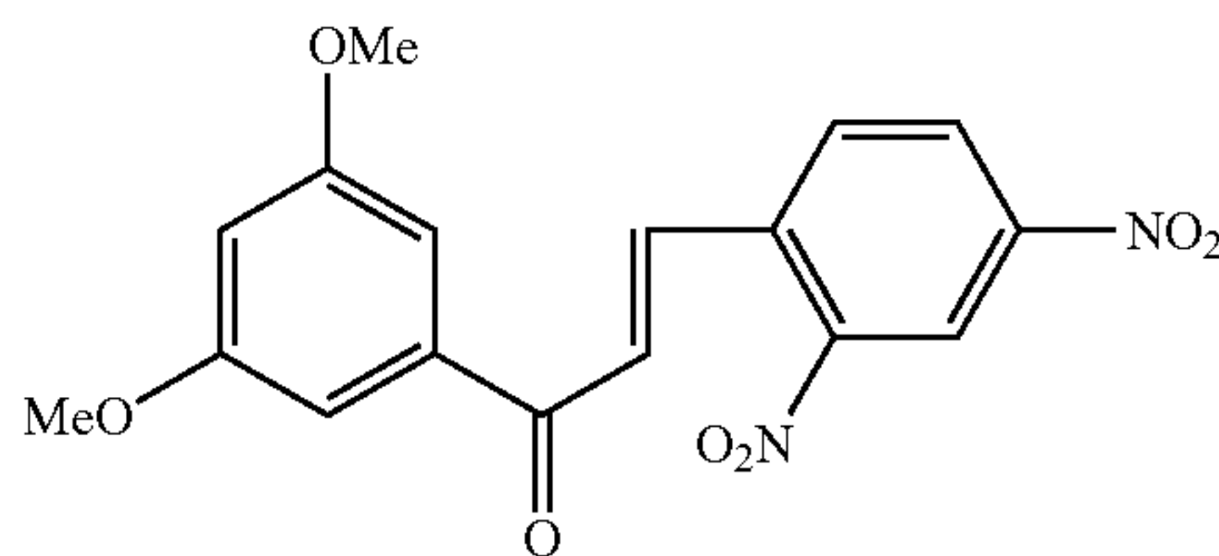
Compound 44
