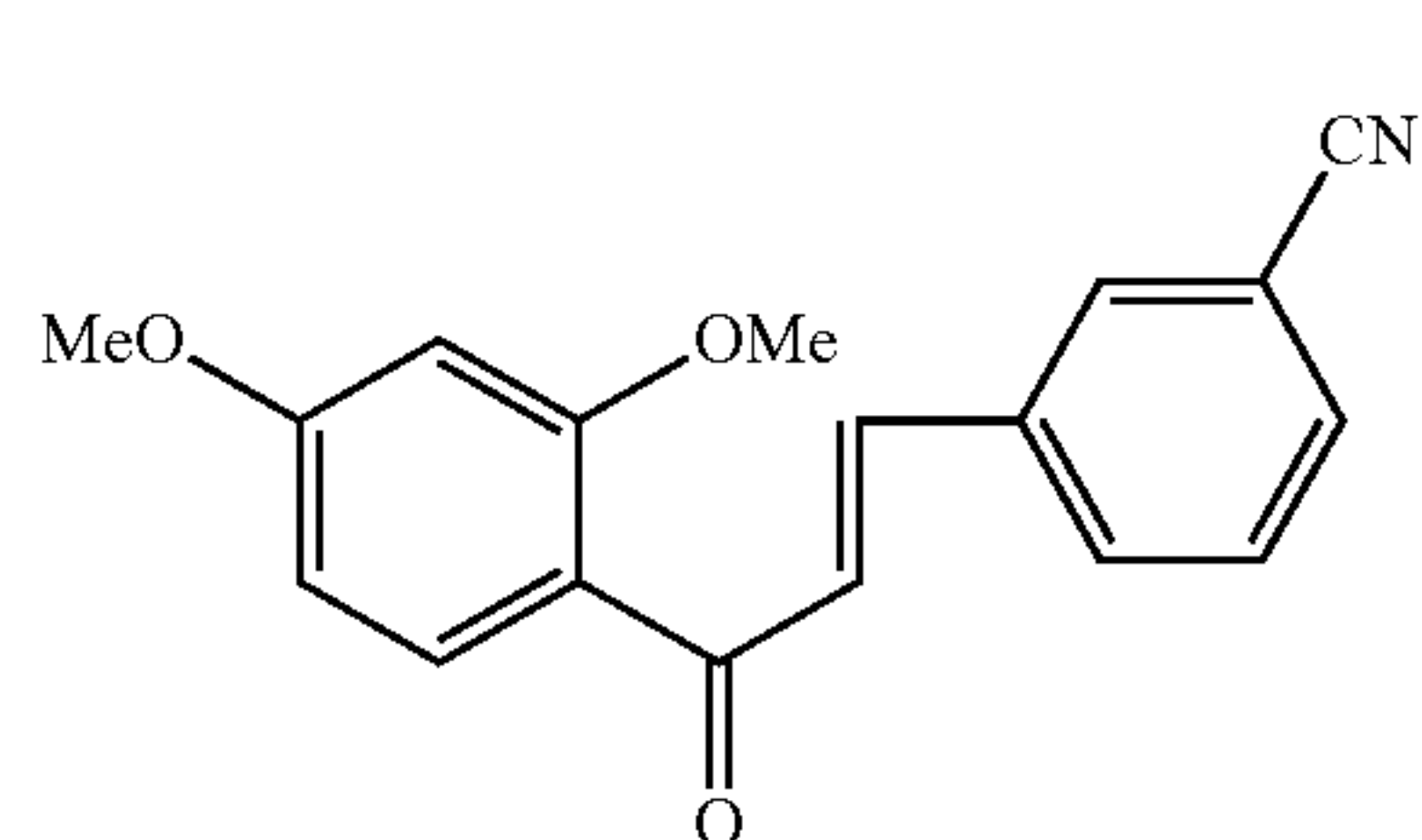
Compound 113
