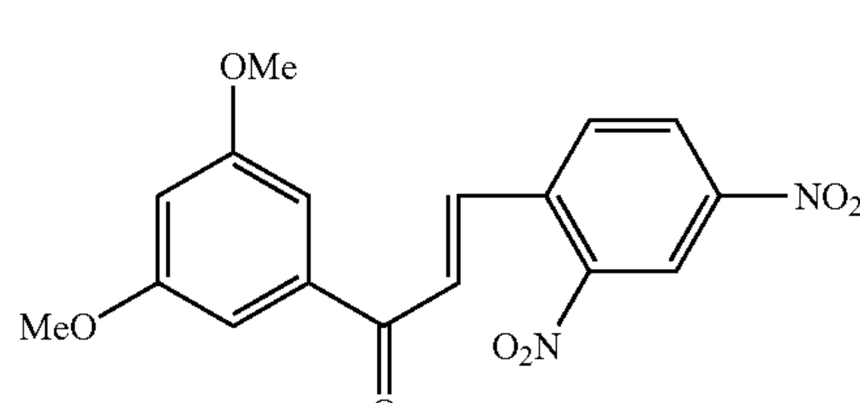
Compound 58
