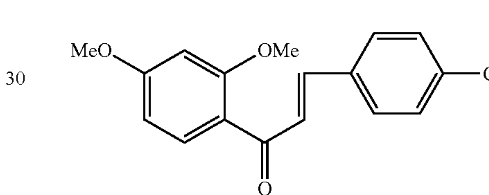
Compound 93
