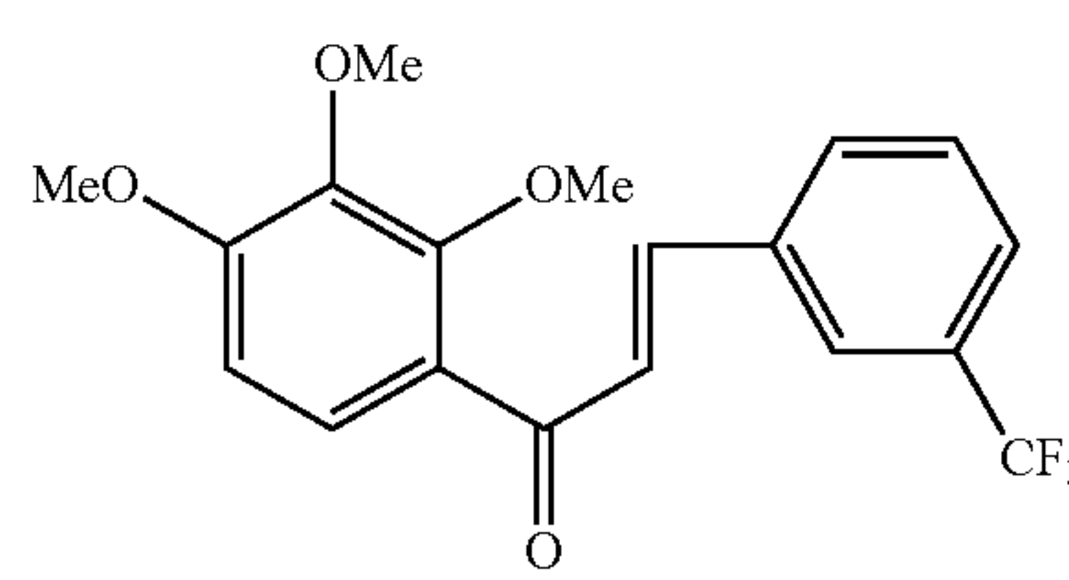
Compound 29
