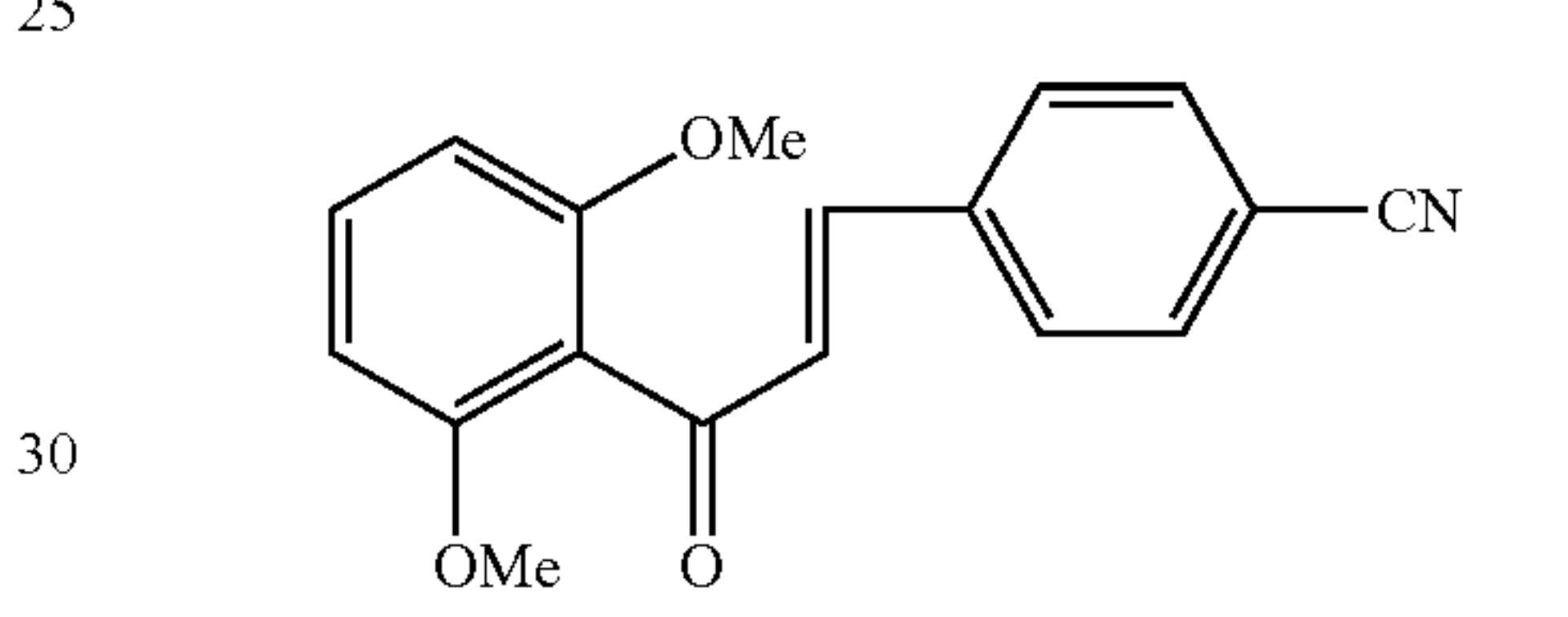
Compound 94
