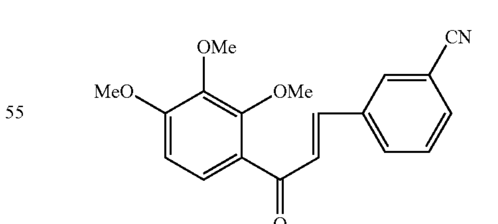
Compound 91
