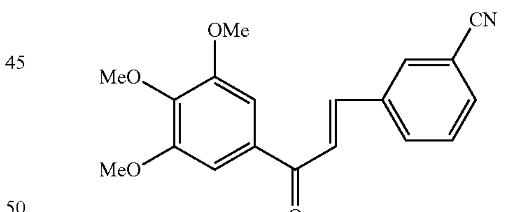
Compound 90
