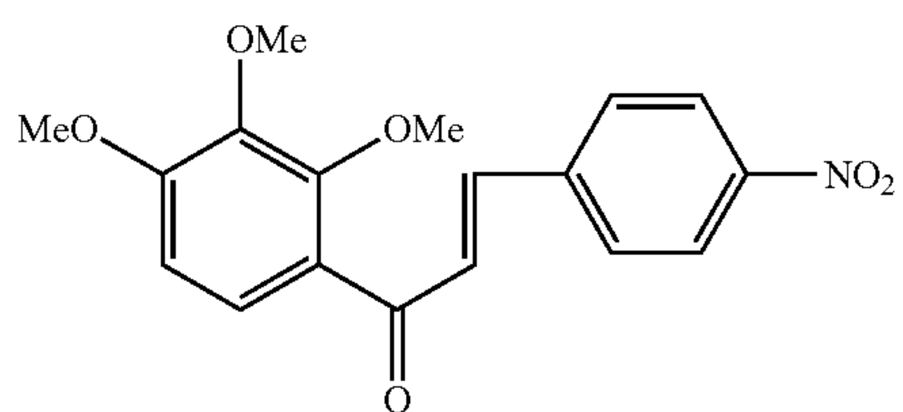
Compound 12
