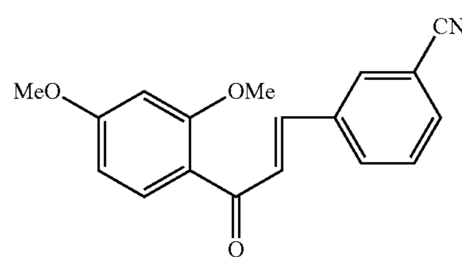
Compound 113
