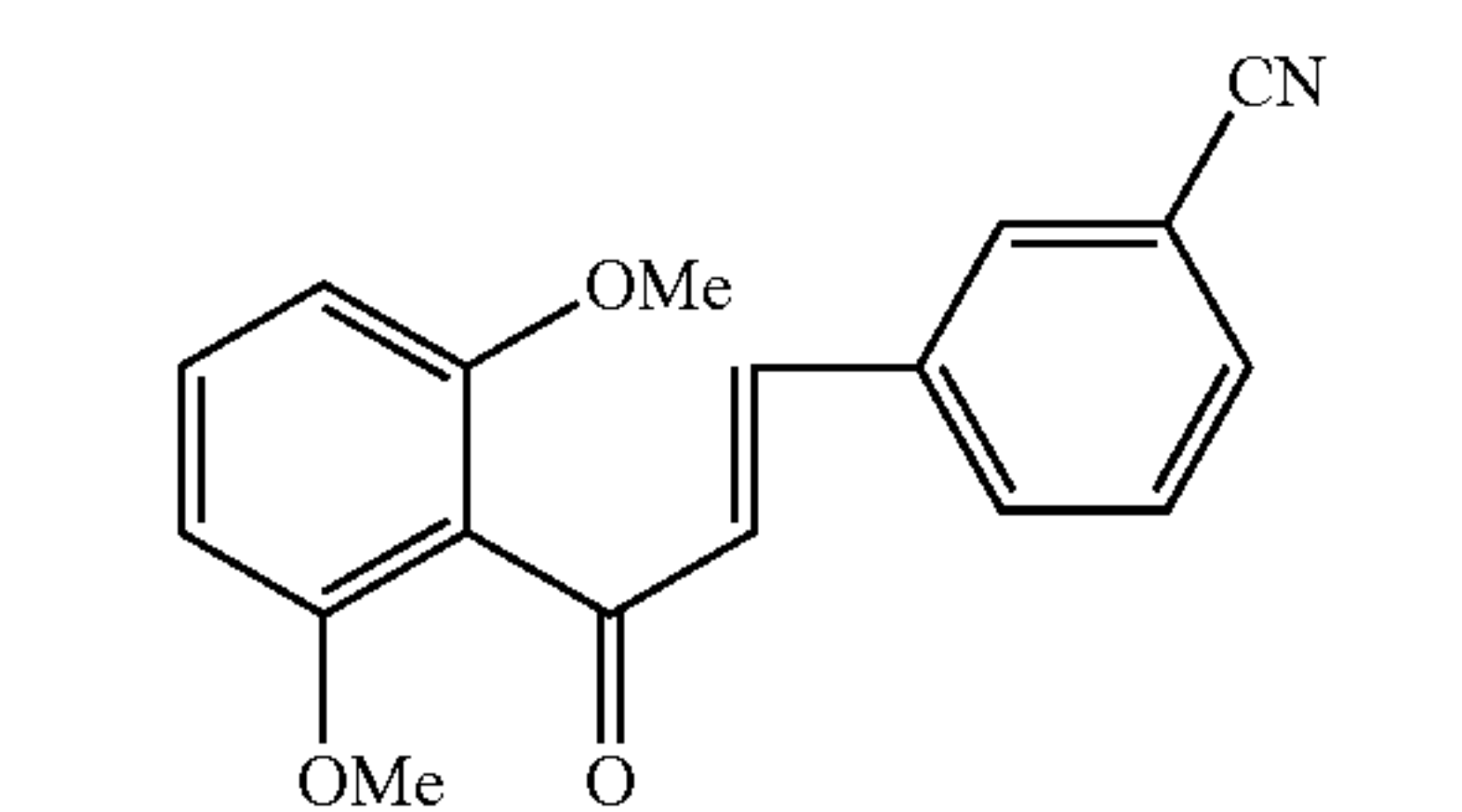
Compound 115
