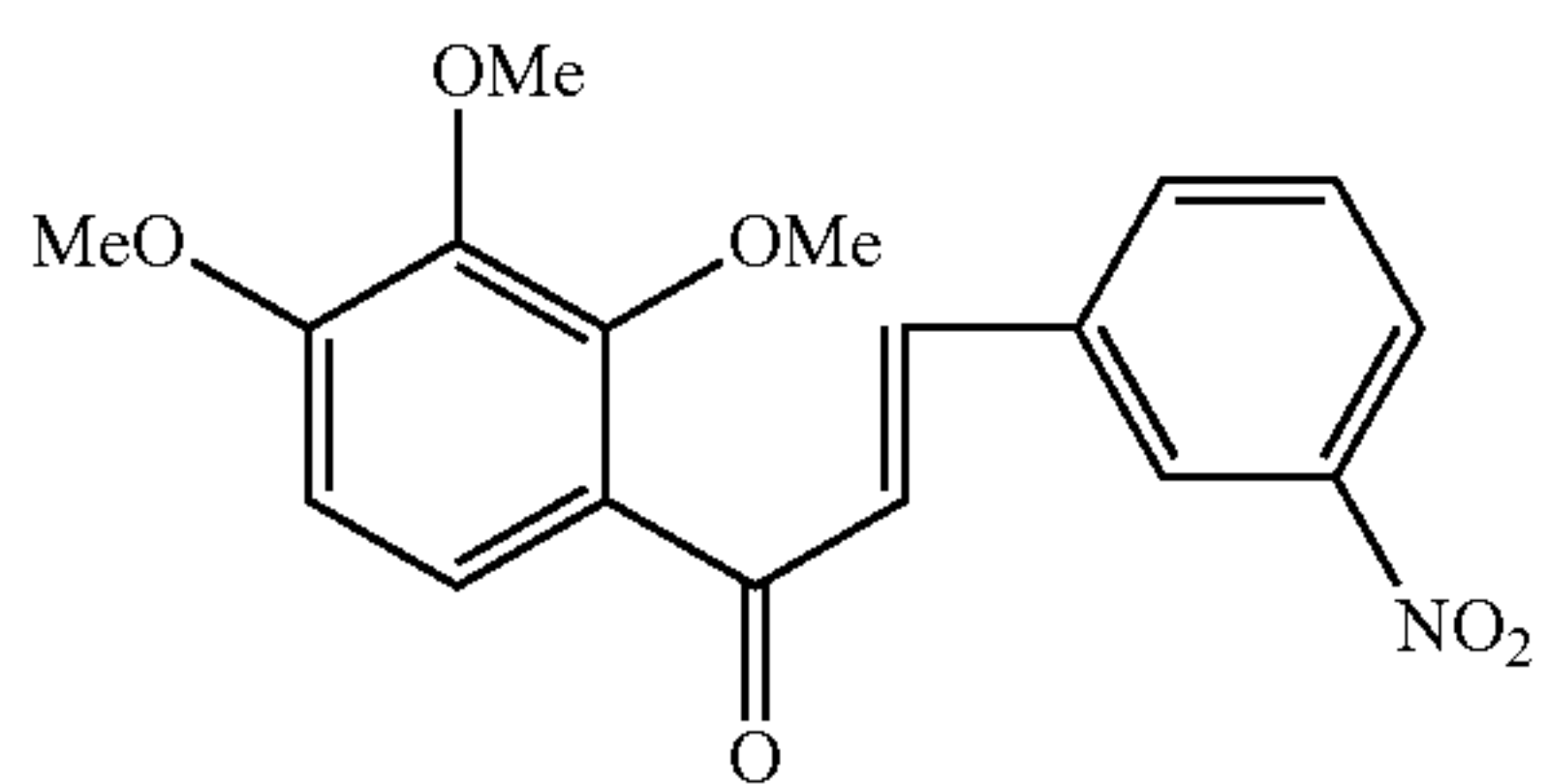
Compound 12
