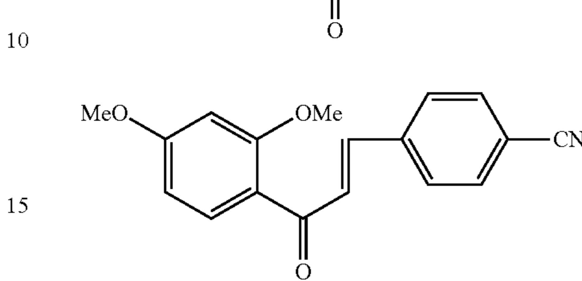
Compound 87
