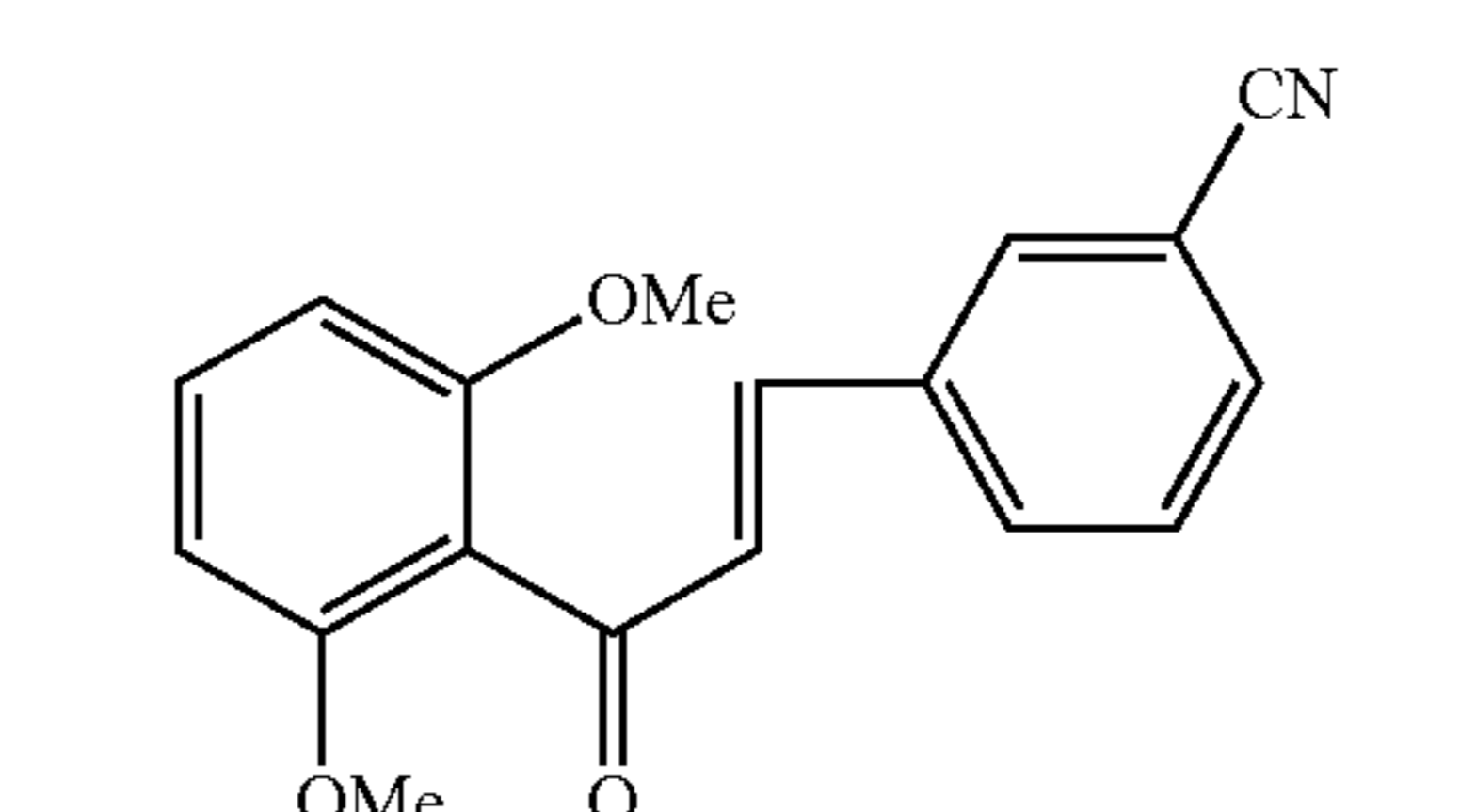
Compound 115
