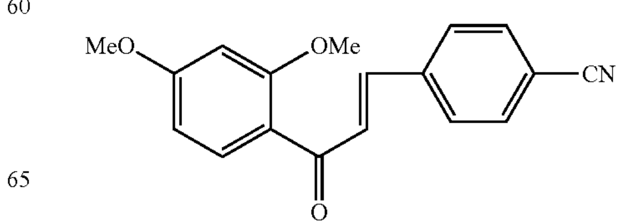
Compound 92
