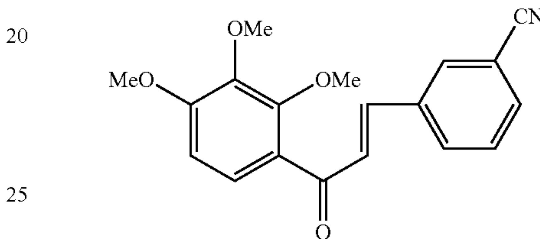
Compound 92
