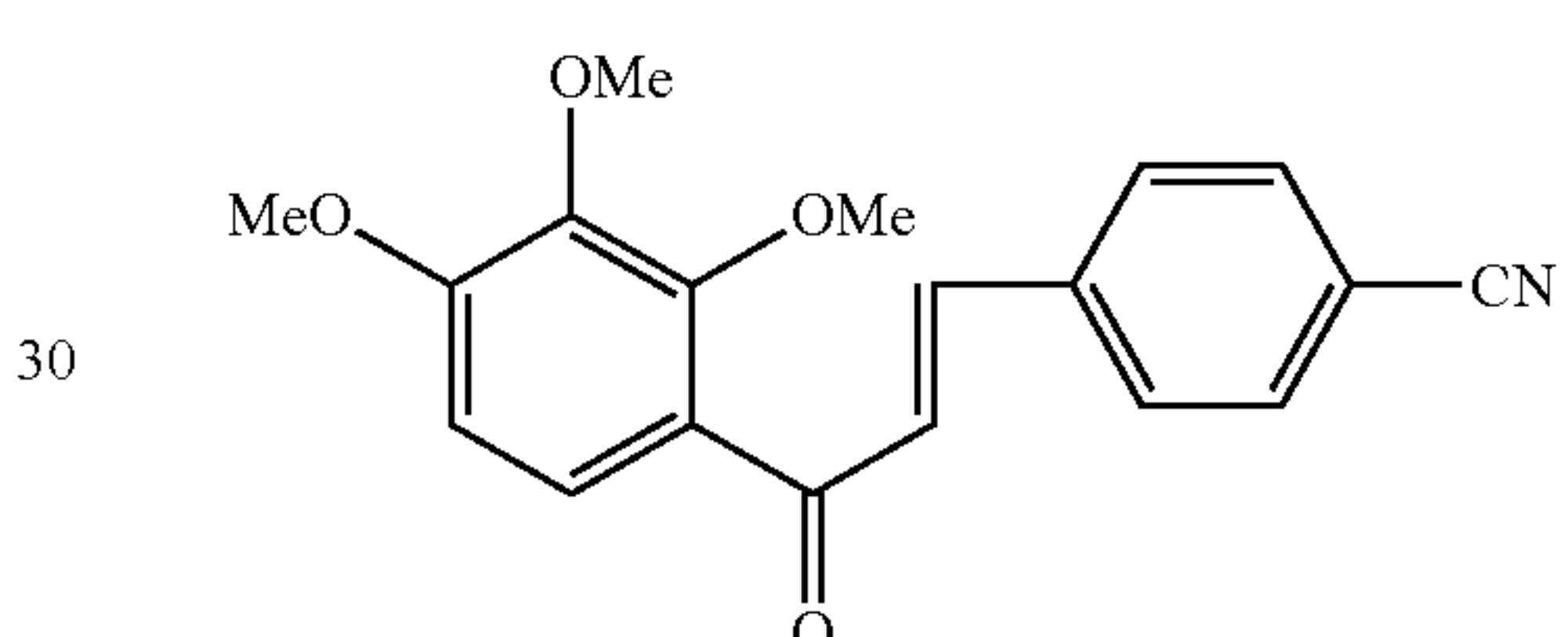
Compound 88
