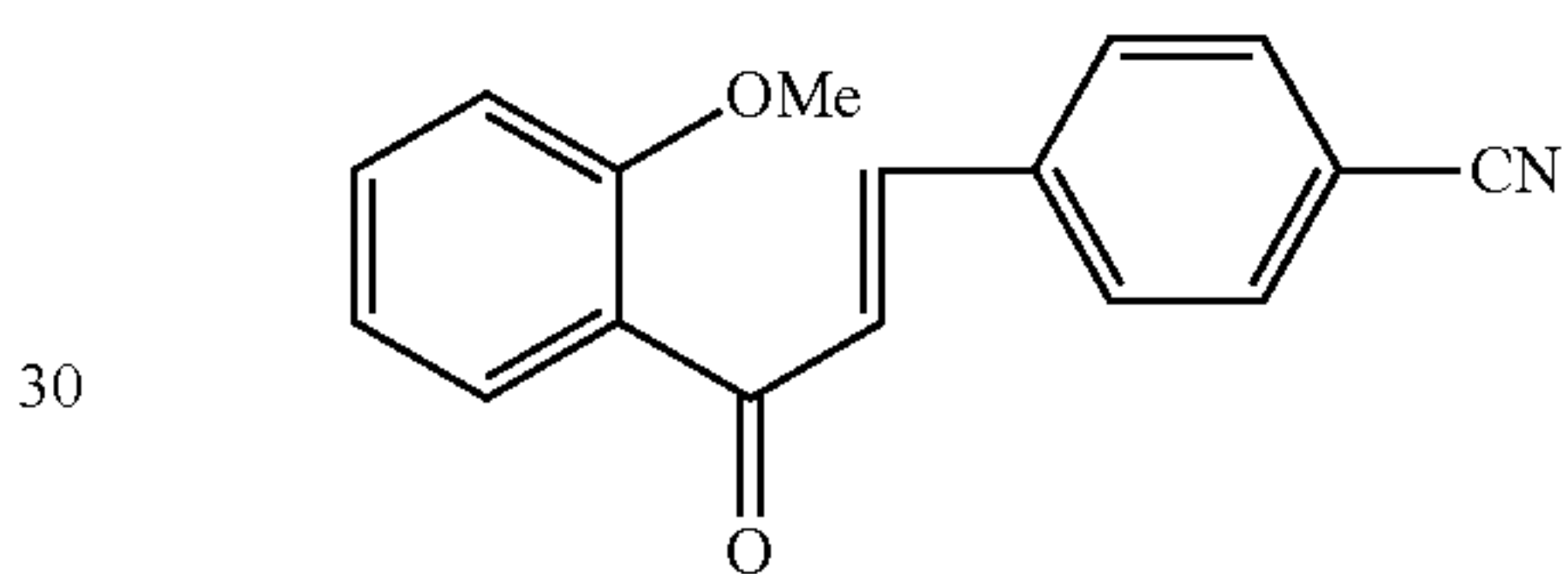
Compound 98
