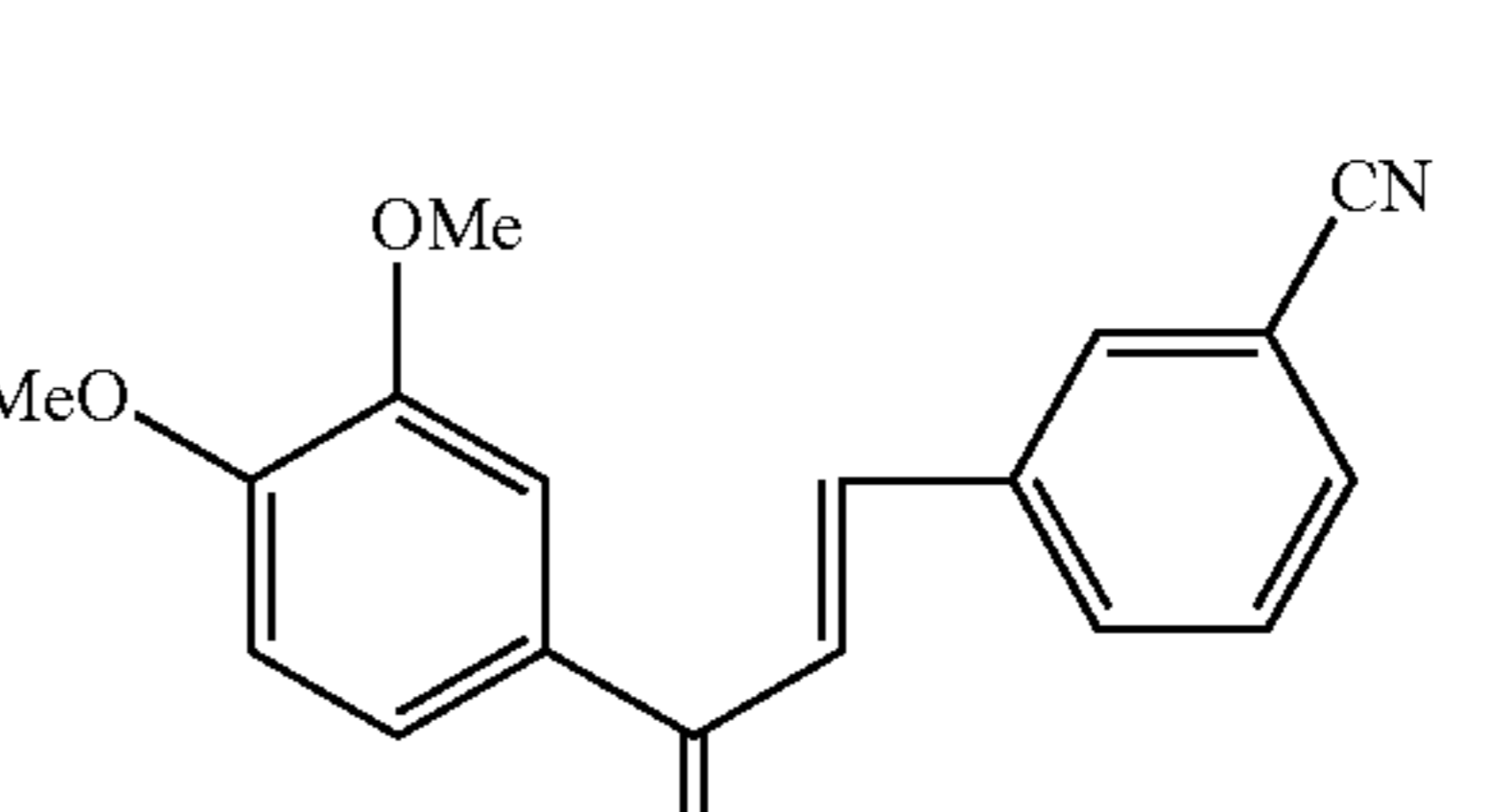
Compound 116
