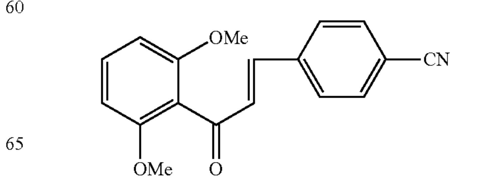
Compound 102
