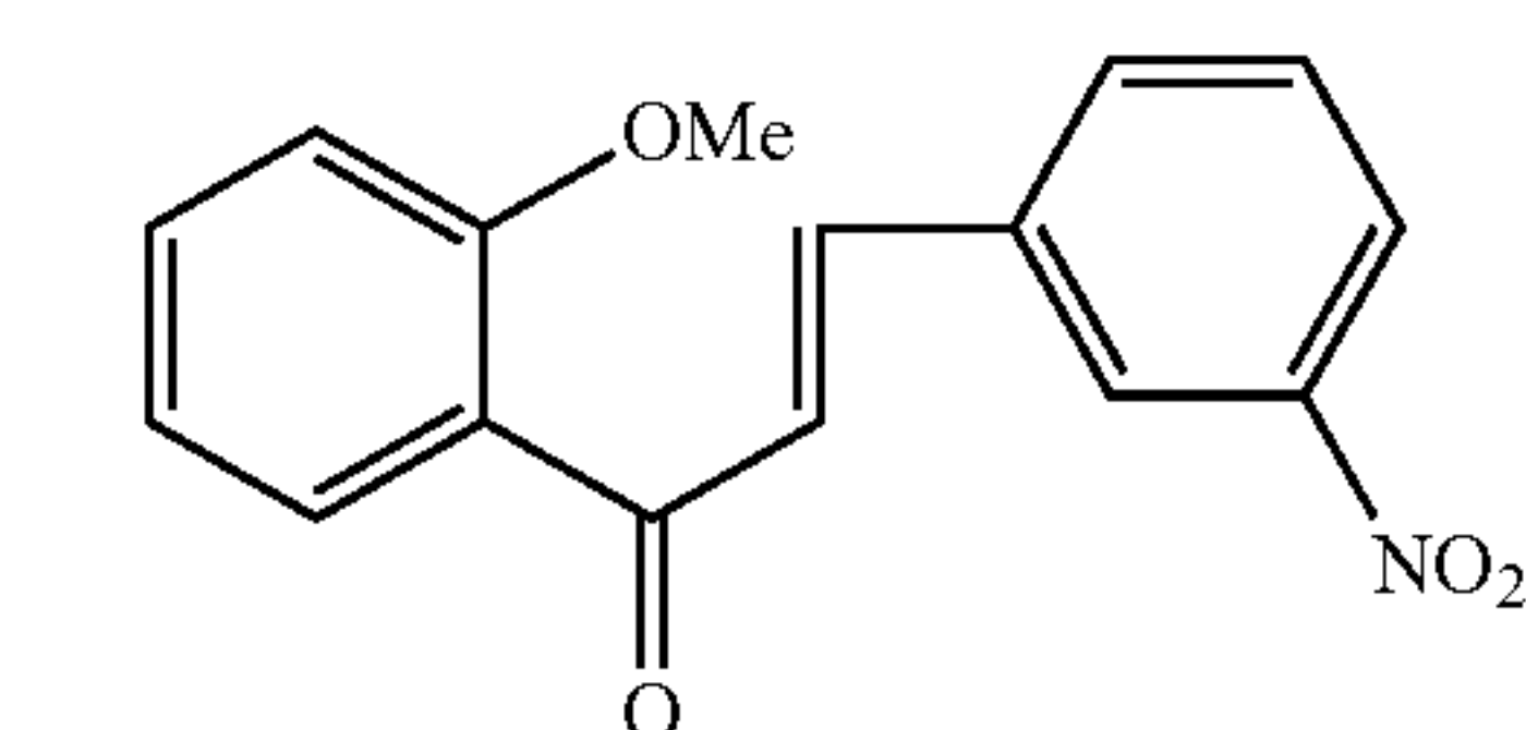
Compound 51
