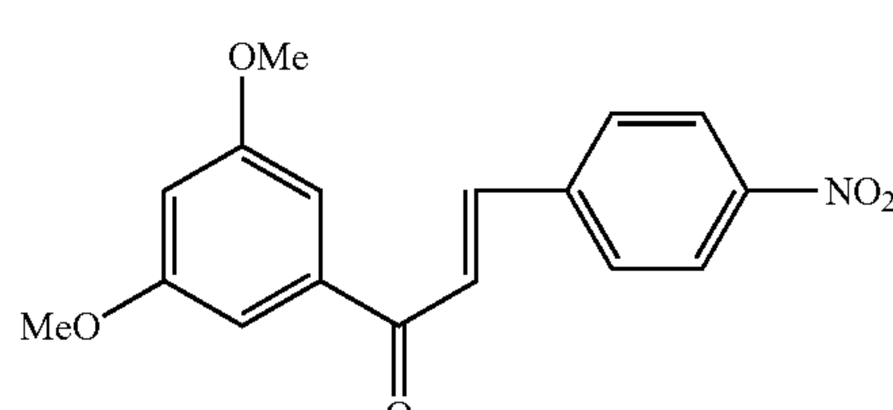
Compound 57
