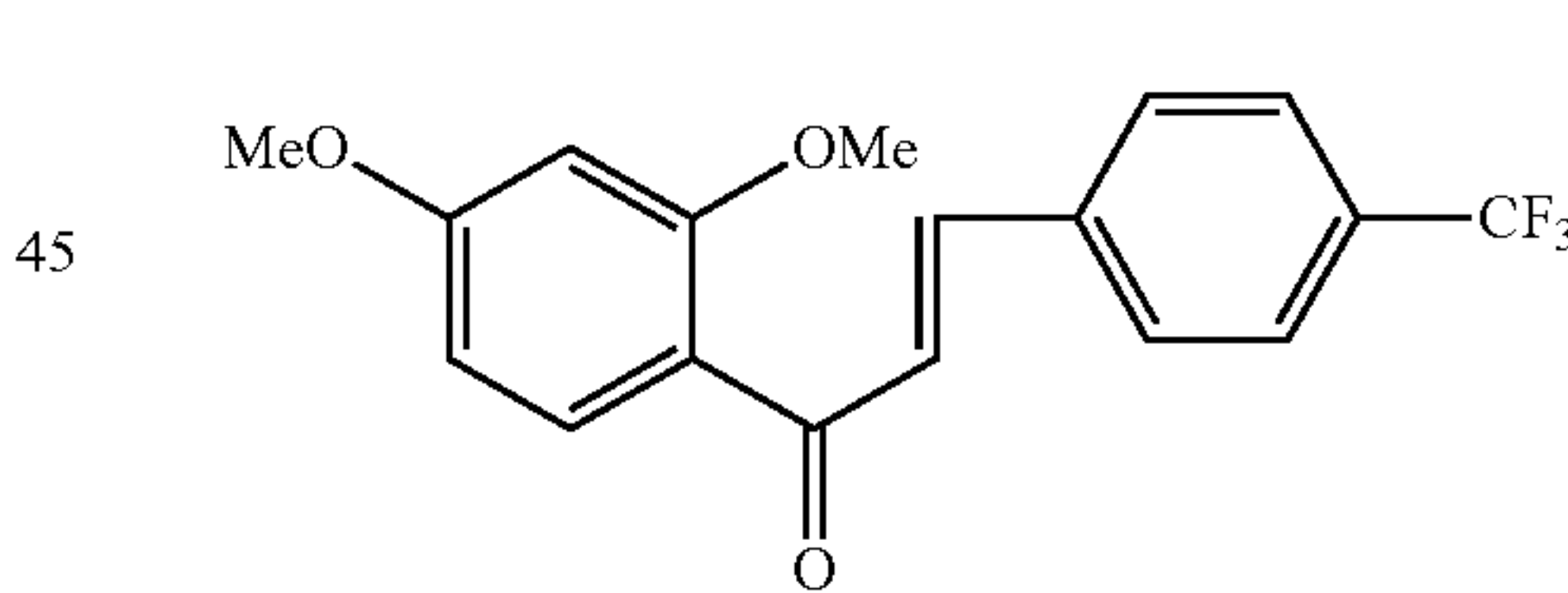
Compound 19
