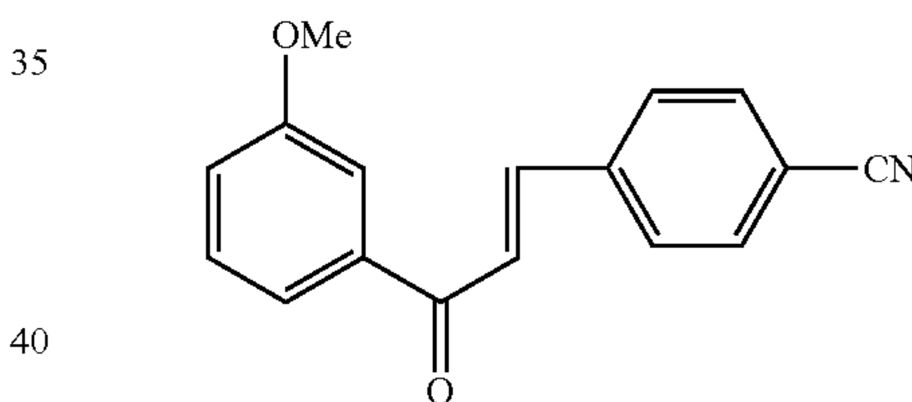
Compound 99
