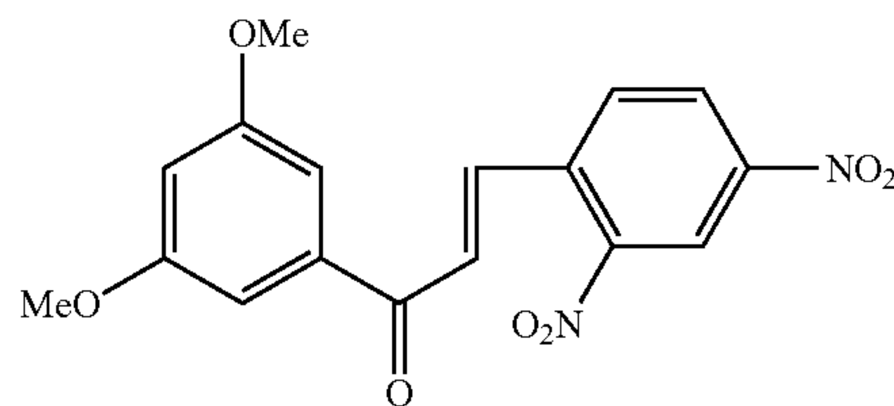
Compound 44
