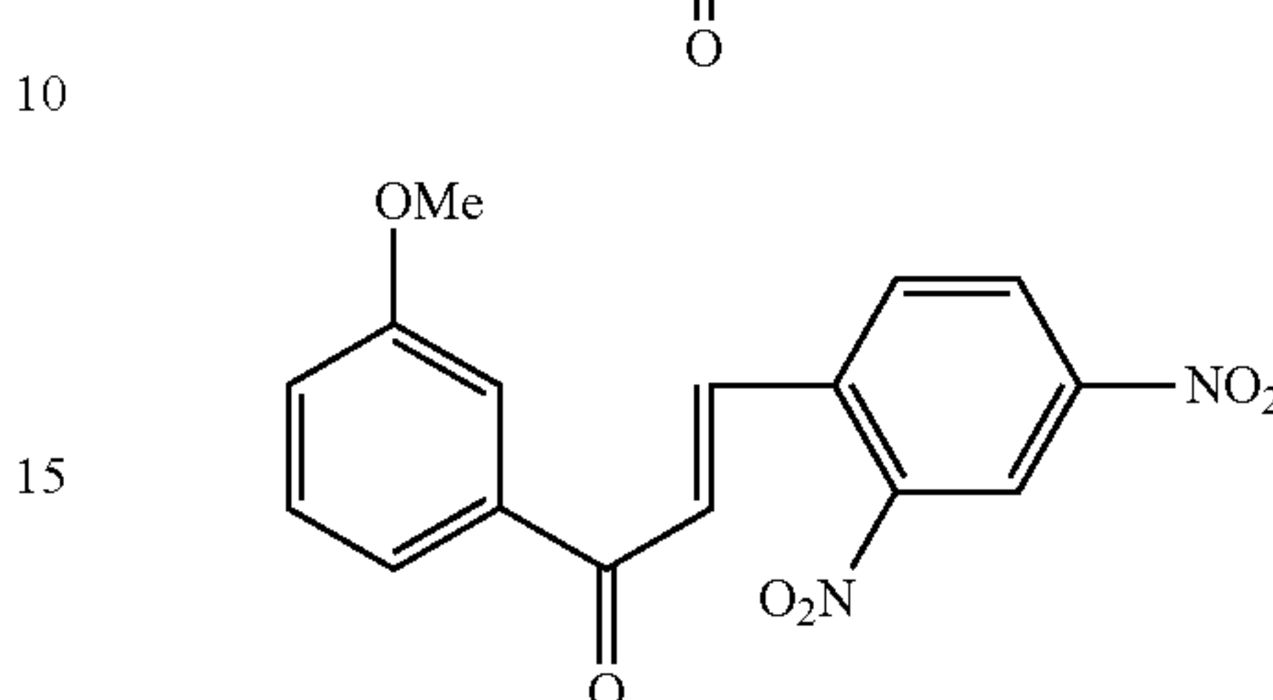
Compound 7
