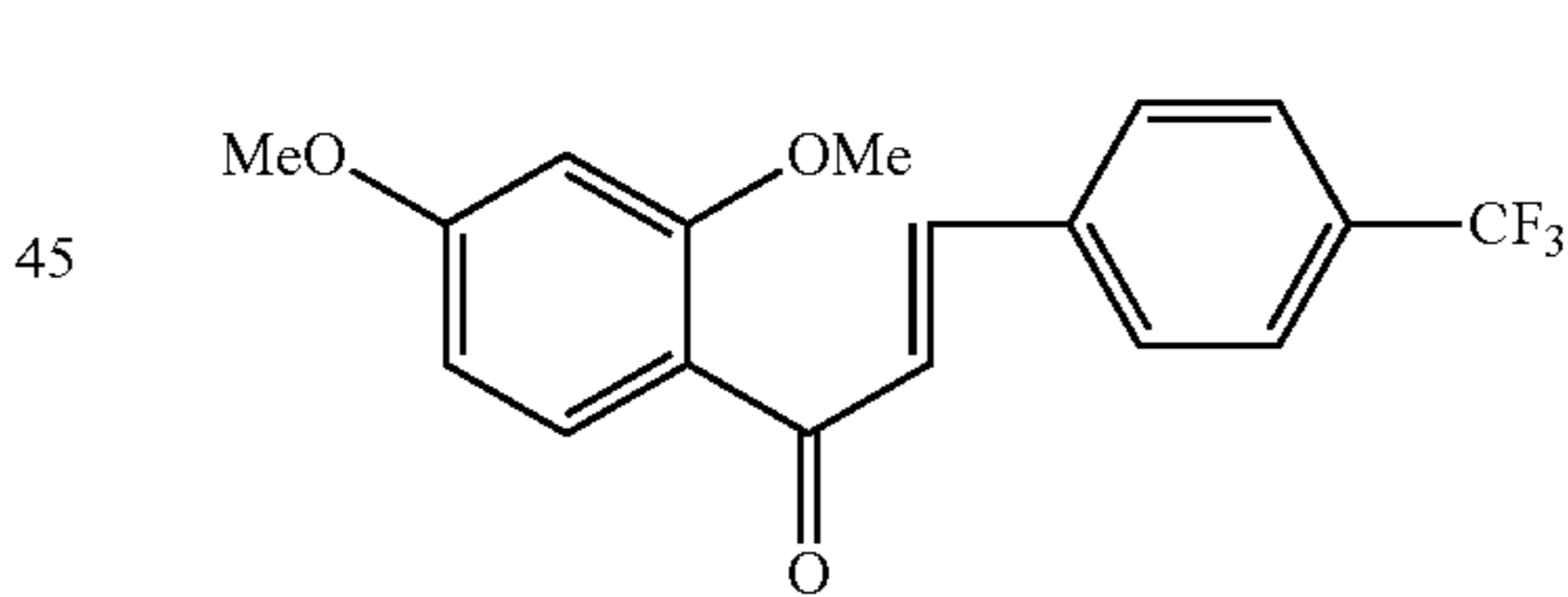
Compound 19
