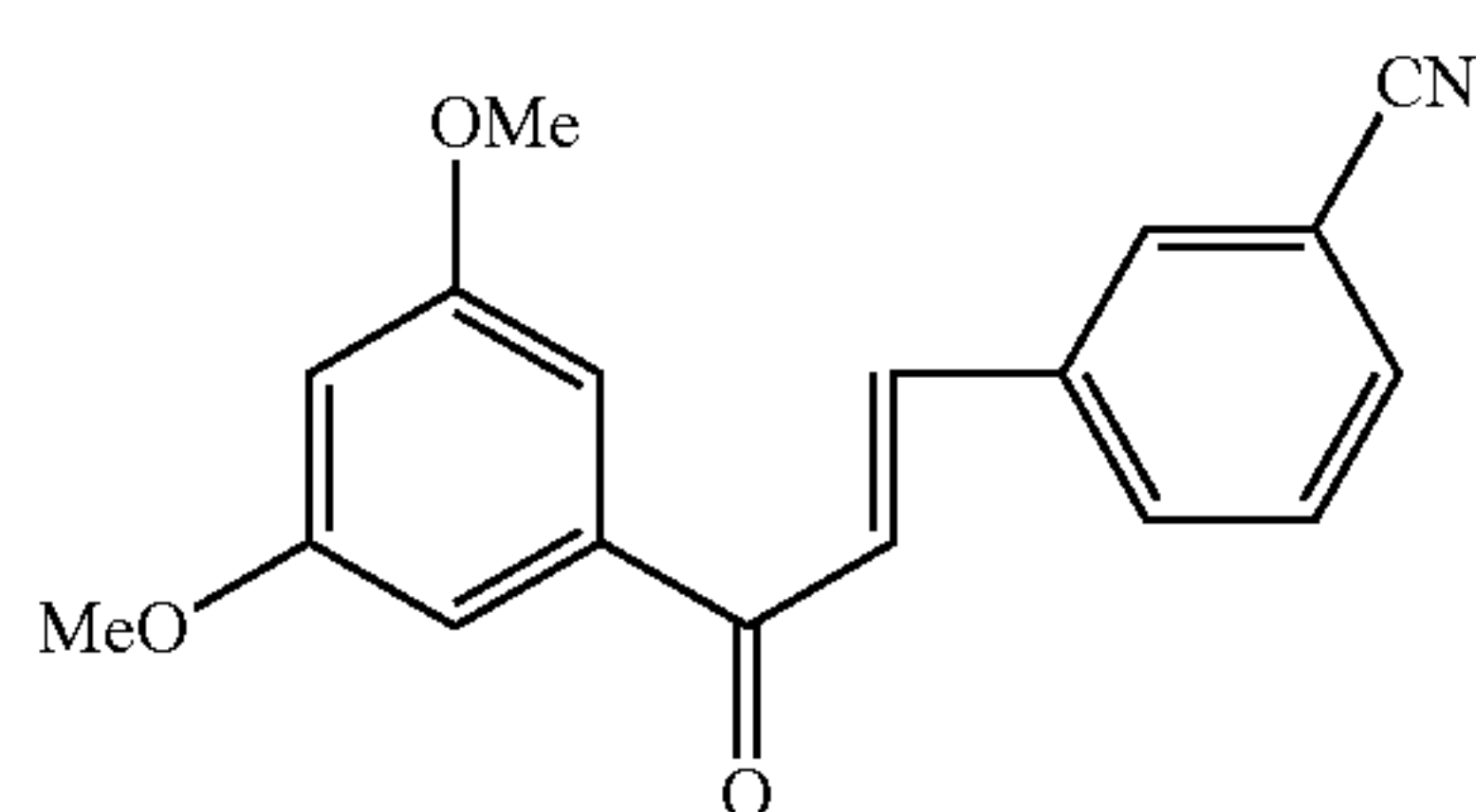
Compound 117
