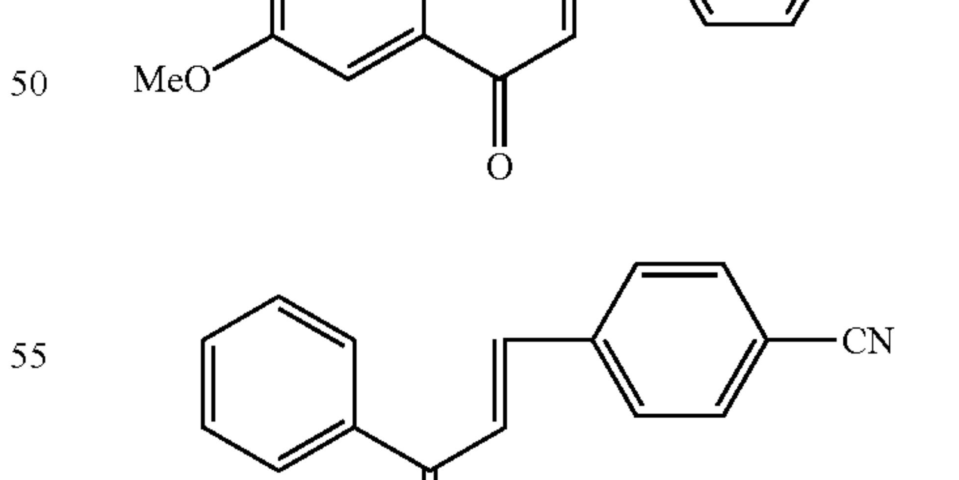
Compound 97
