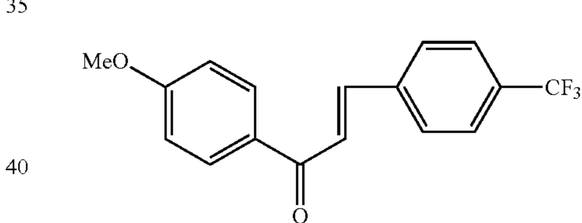
Compound 18
