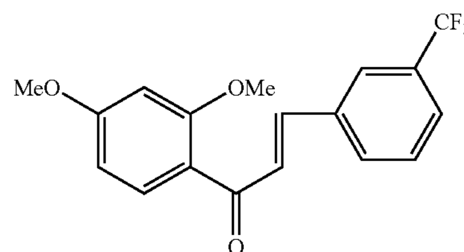
Compound 19
