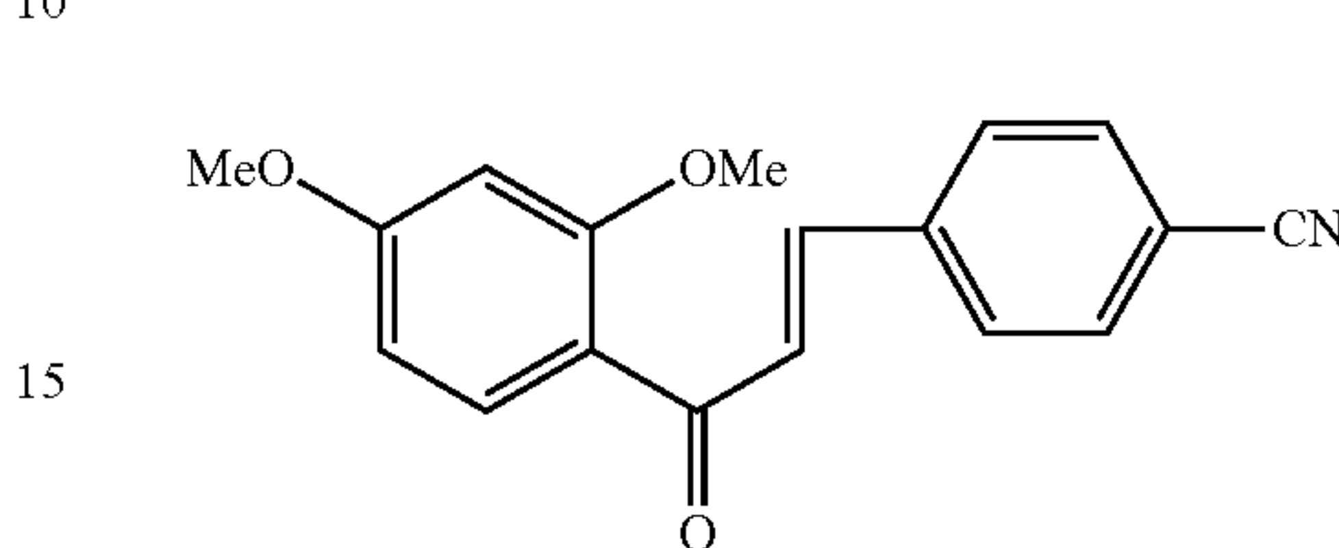
Compound 93
