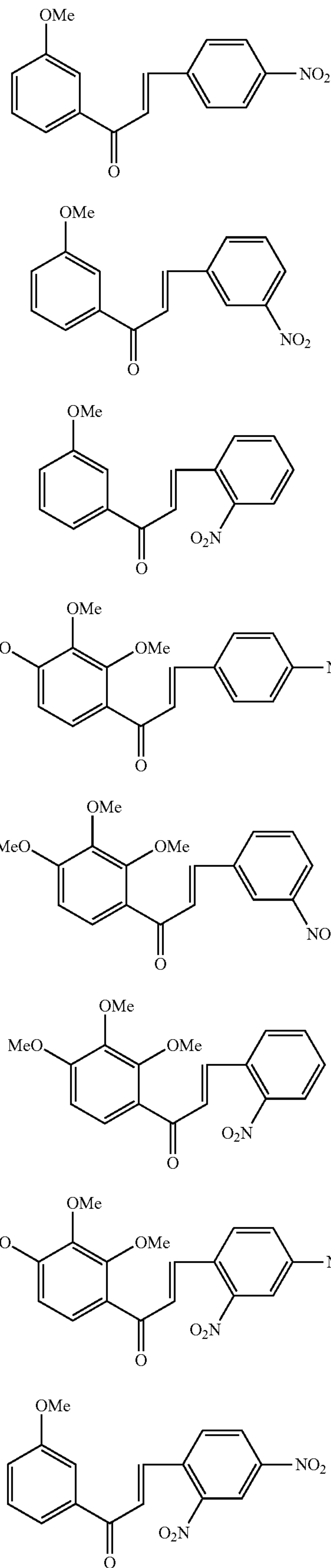
Compound 10
