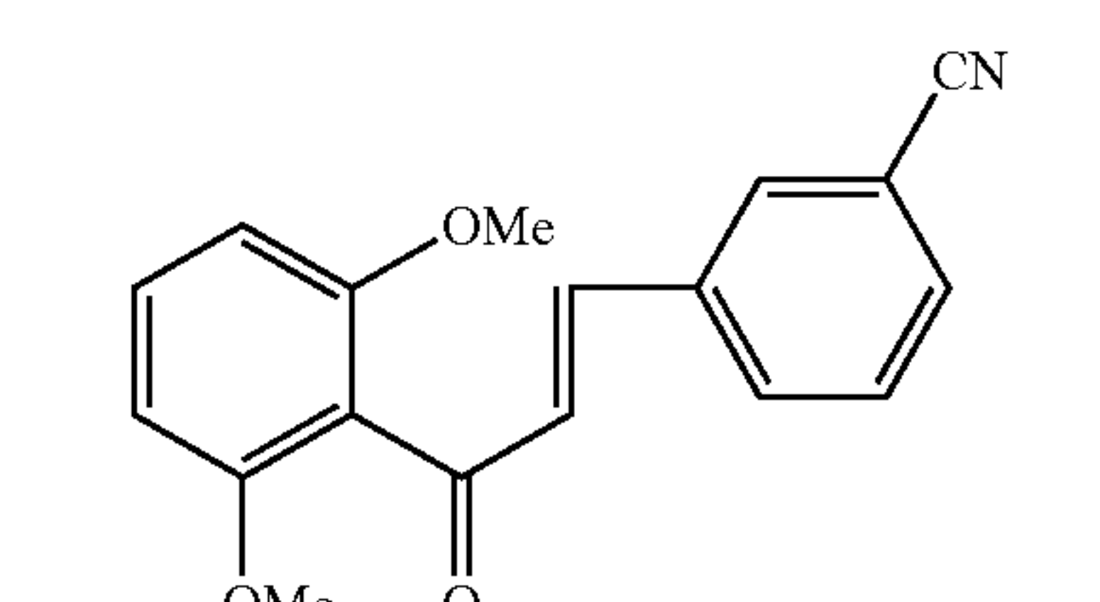
Compound 115
