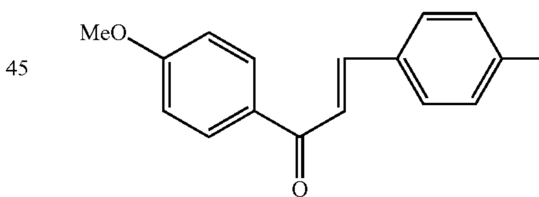
Compound 100
