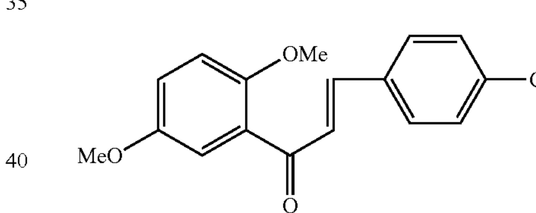
Compound 94
