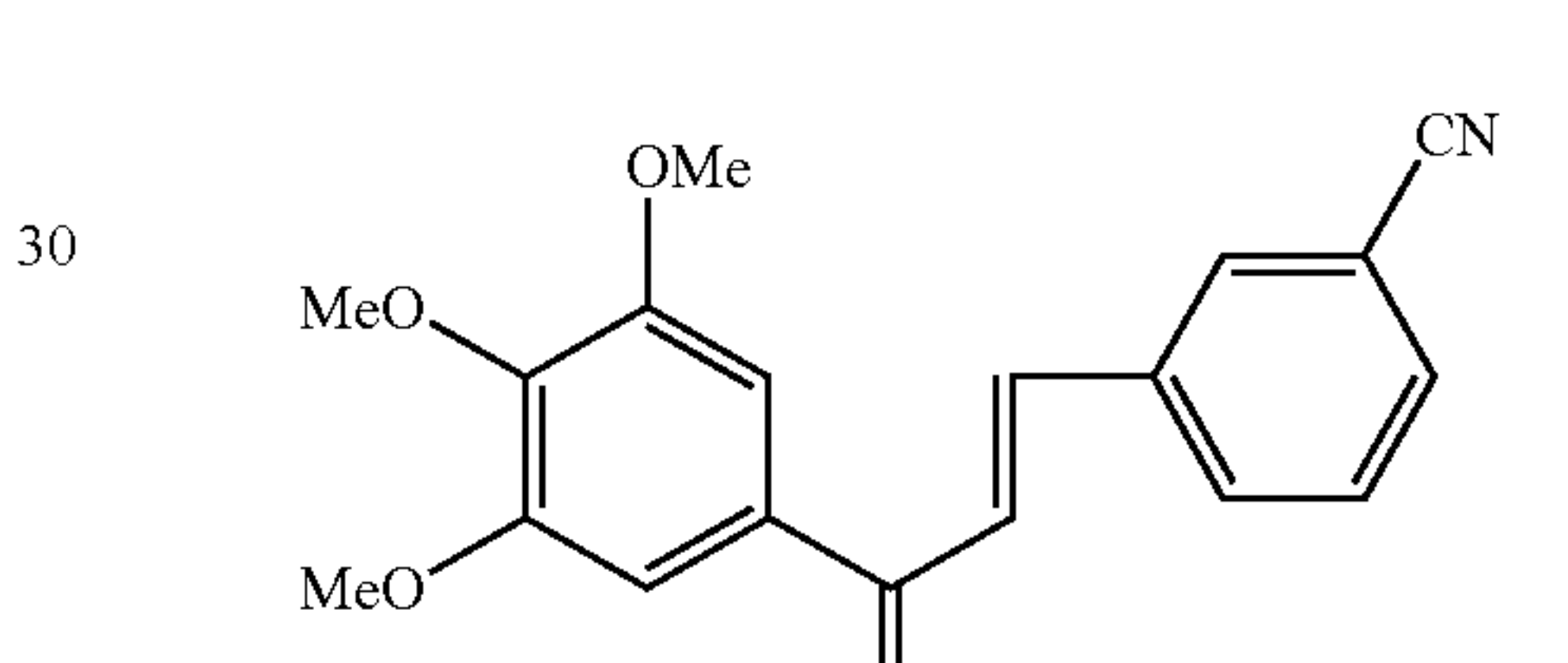
Compound 90
