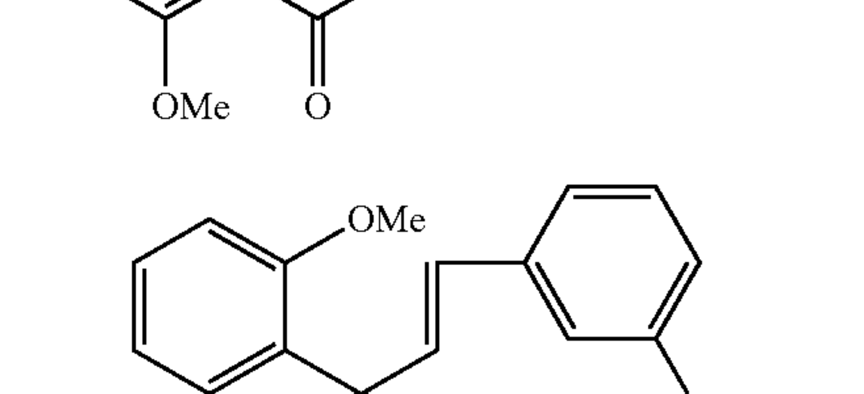
Compound 50
