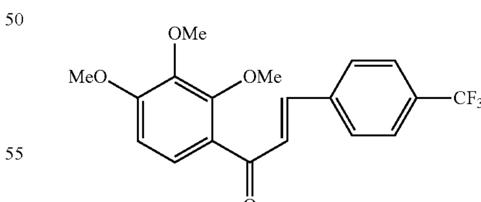
Compound 12
