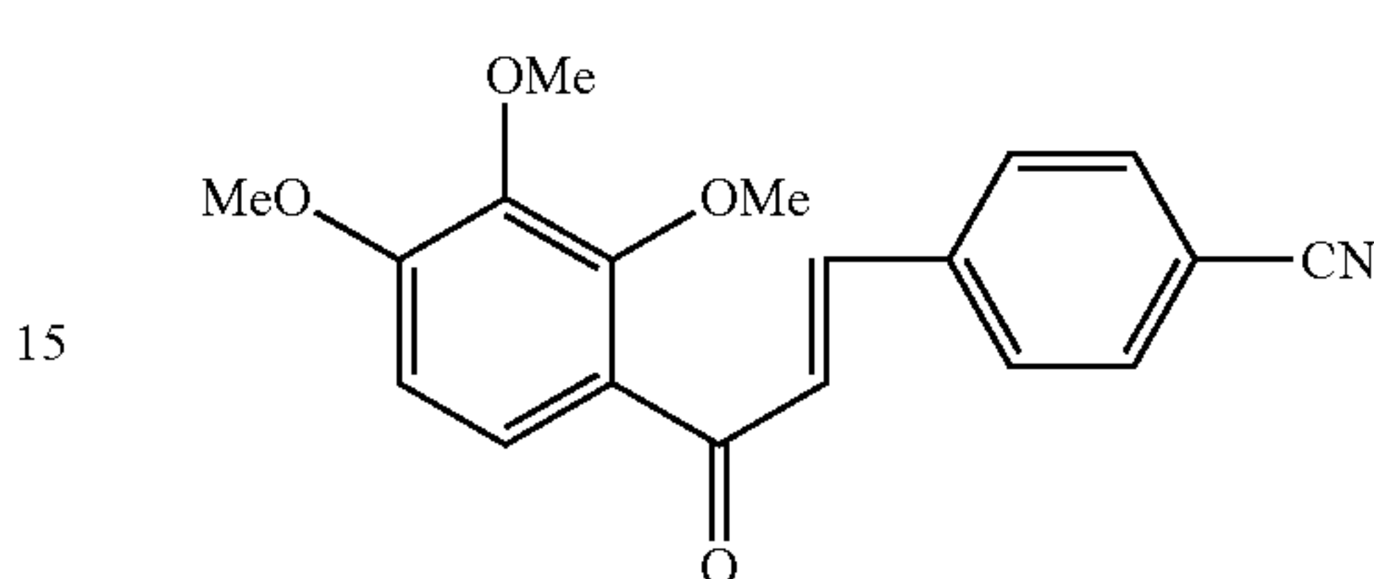
Compound 88
