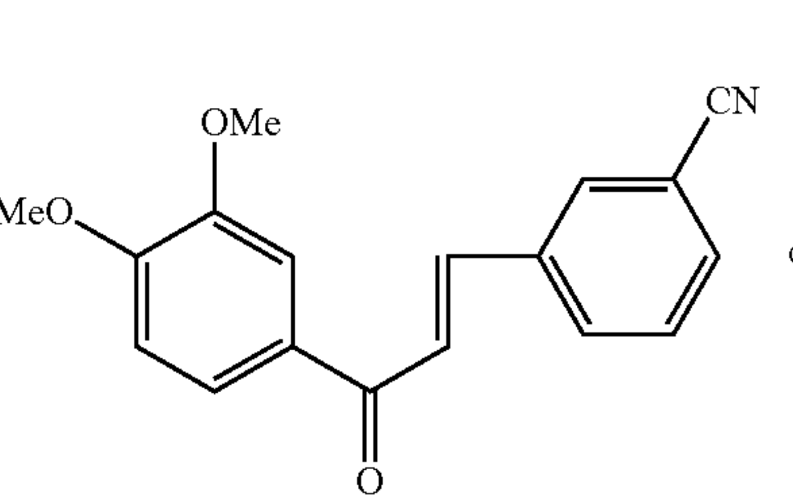
Compound 116
