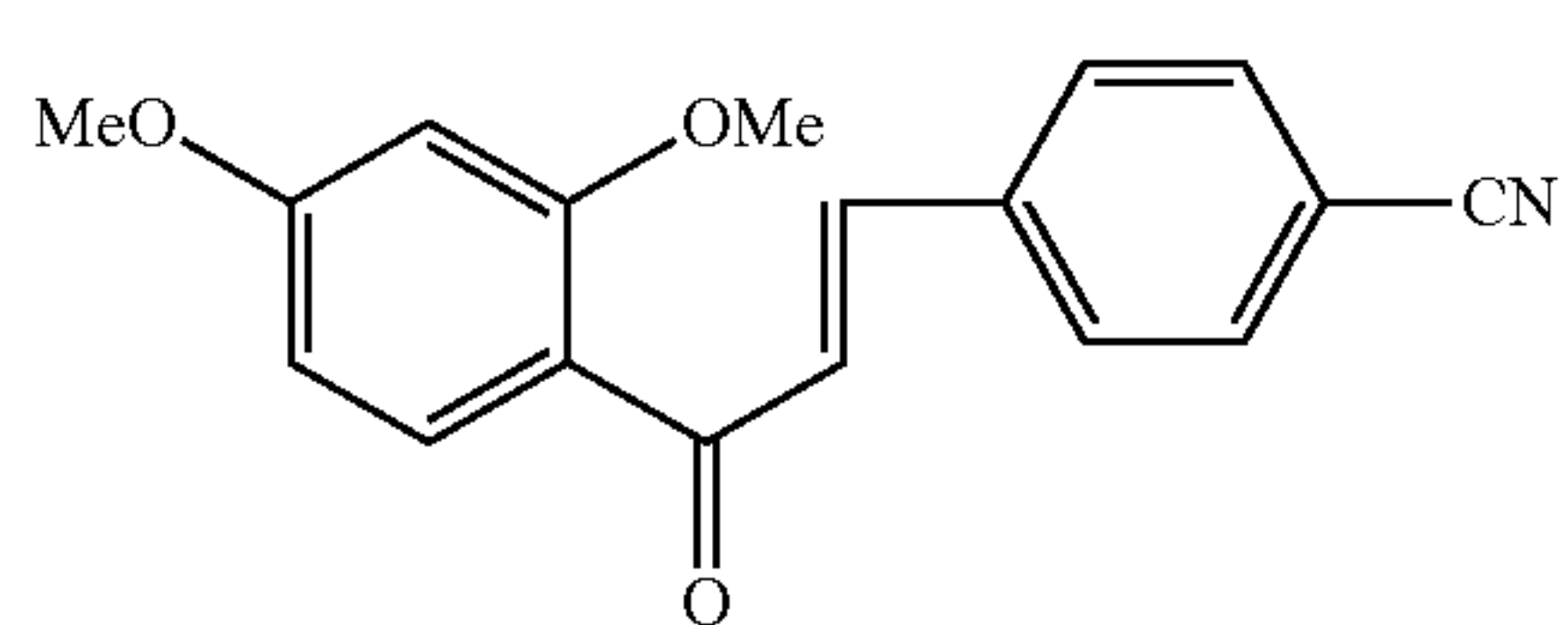
Compound 100
