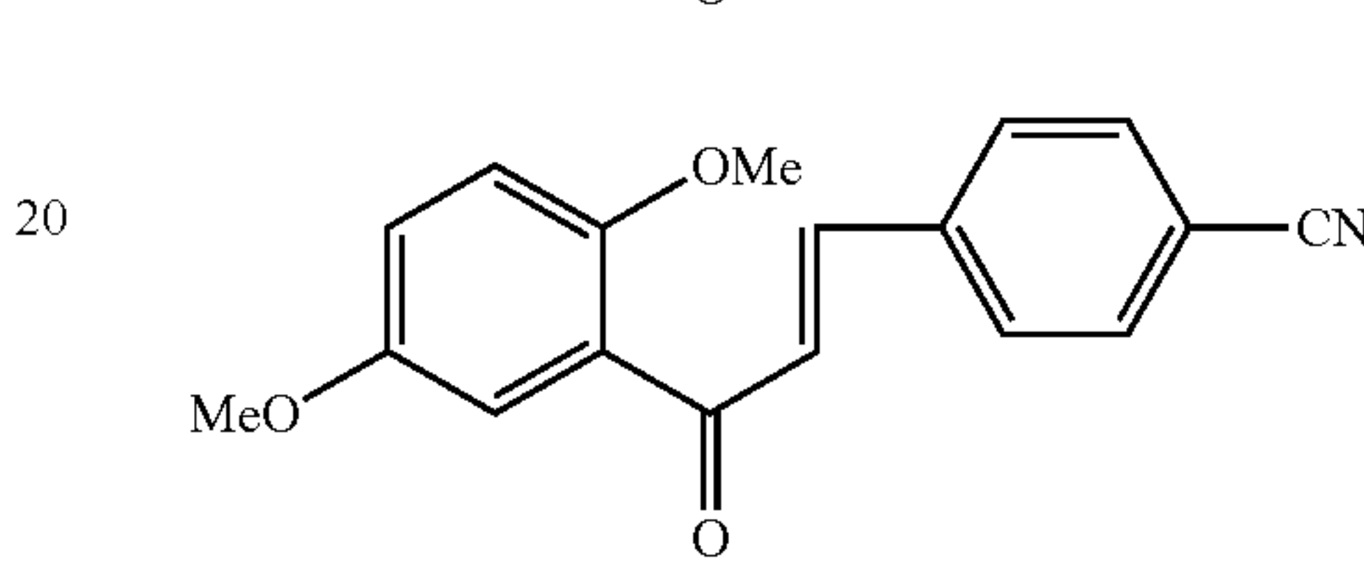
Compound 101
