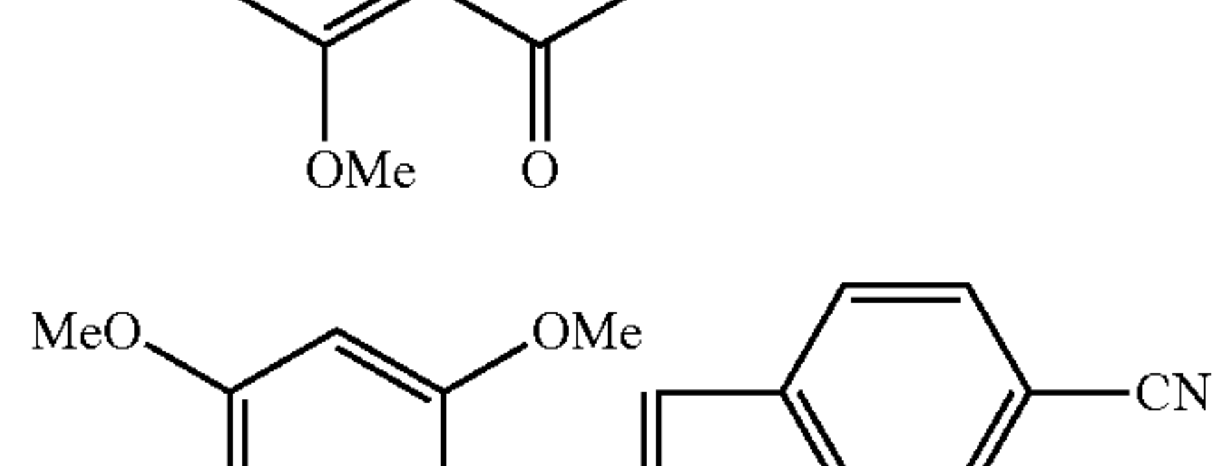
Compound 94
