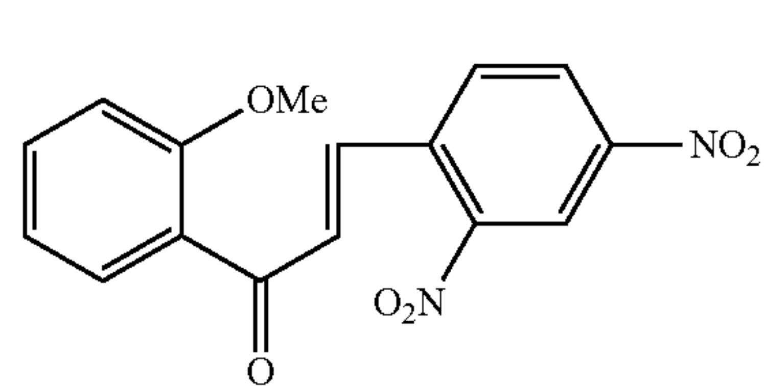
Compound 53
