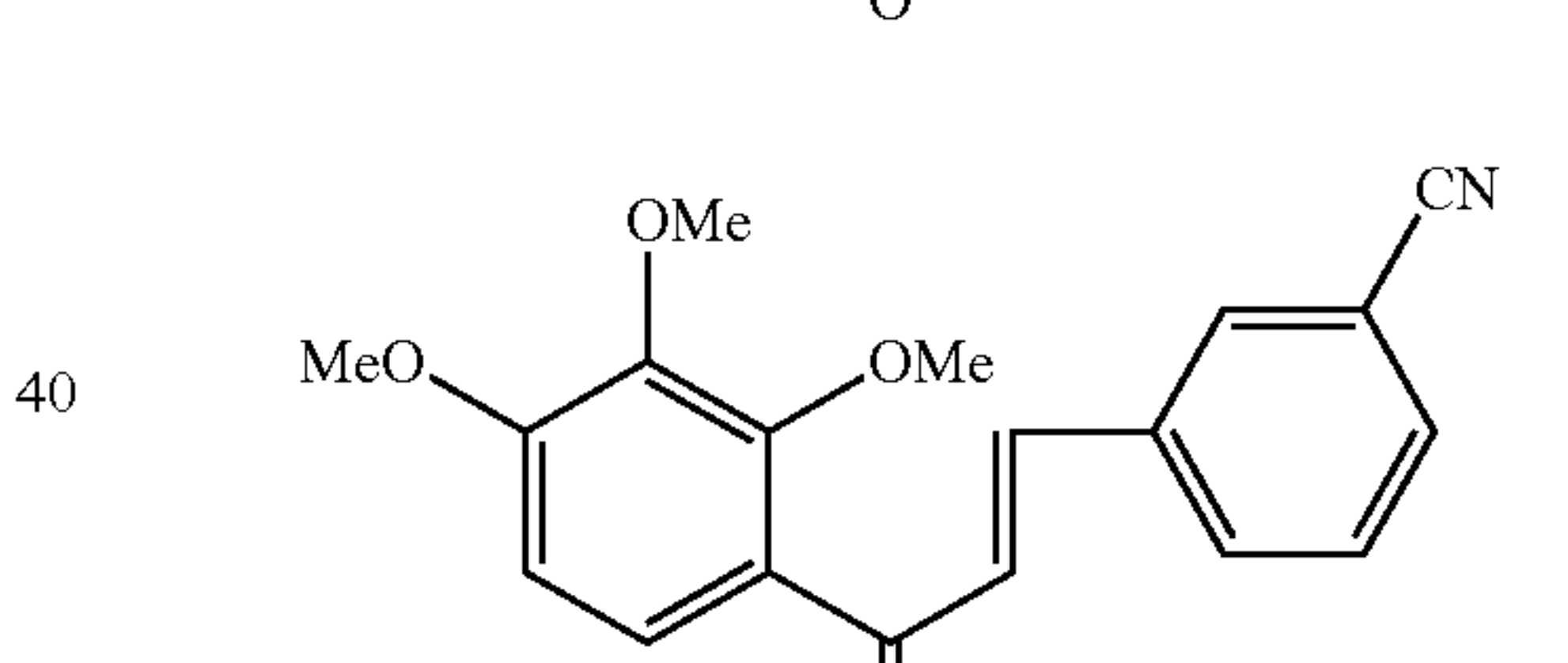
Compound 91
