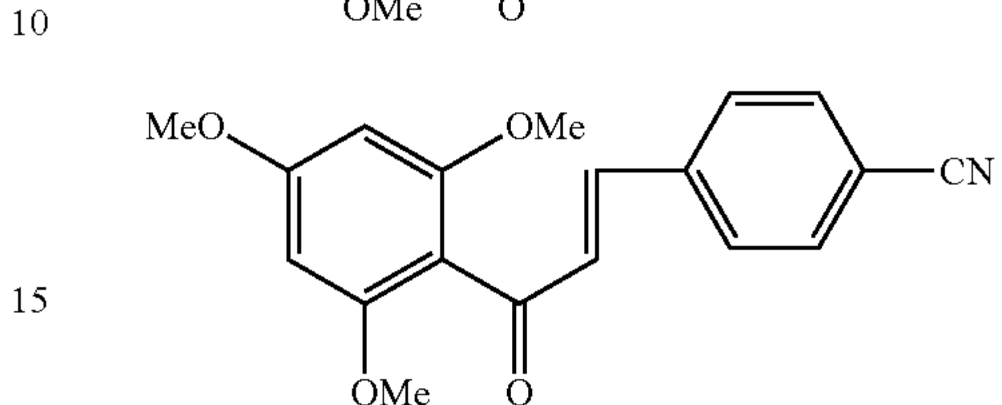
Compound 85
