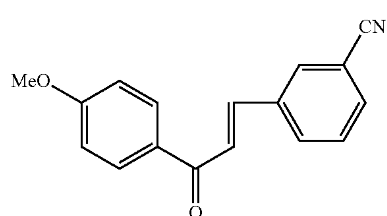
Compound 112
