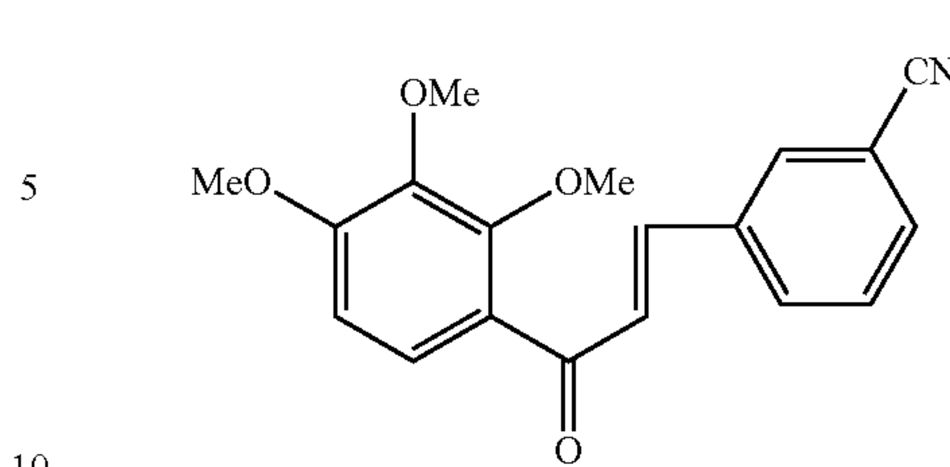
Compound 86
