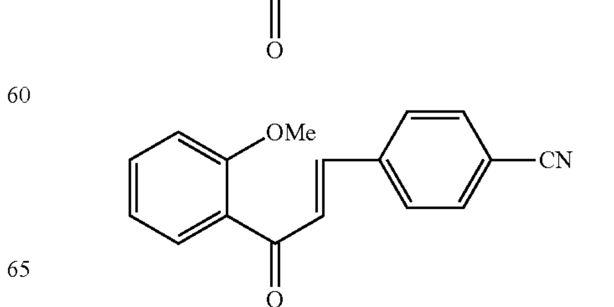
Compound 98
