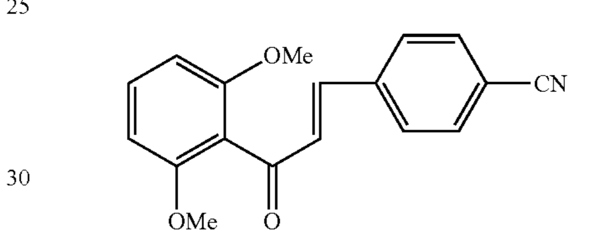
Compound 94
