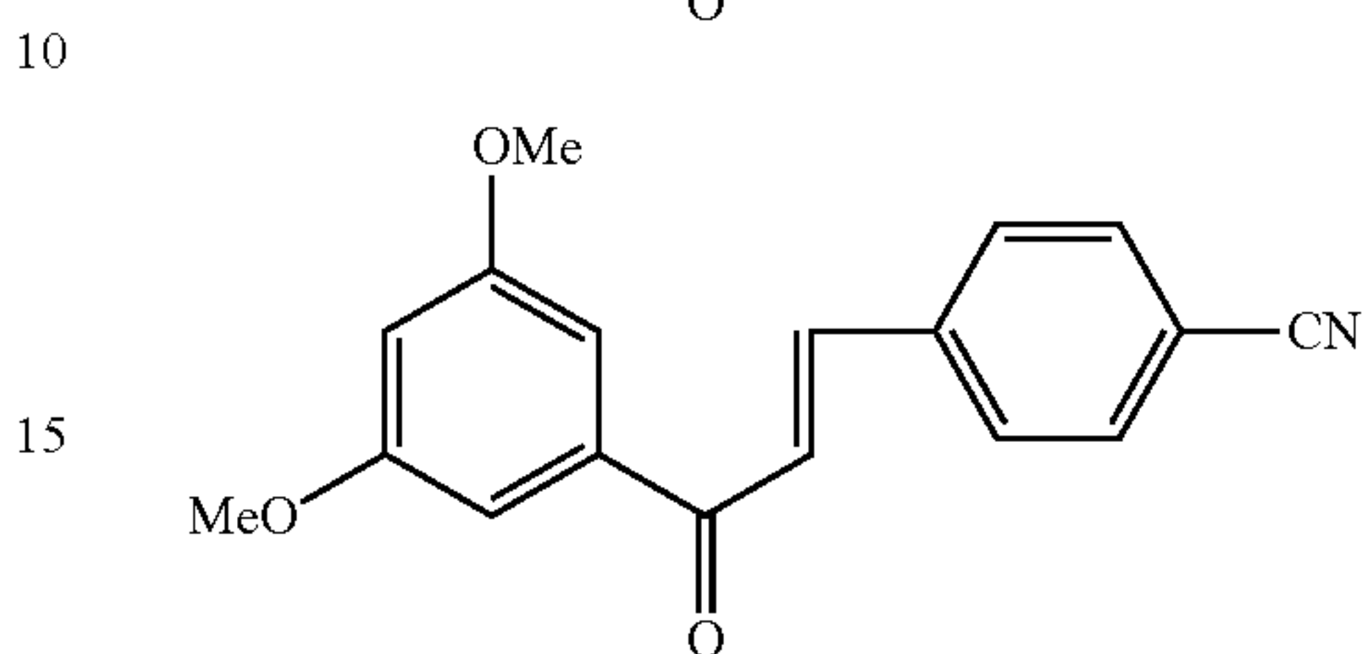
Compound 96
