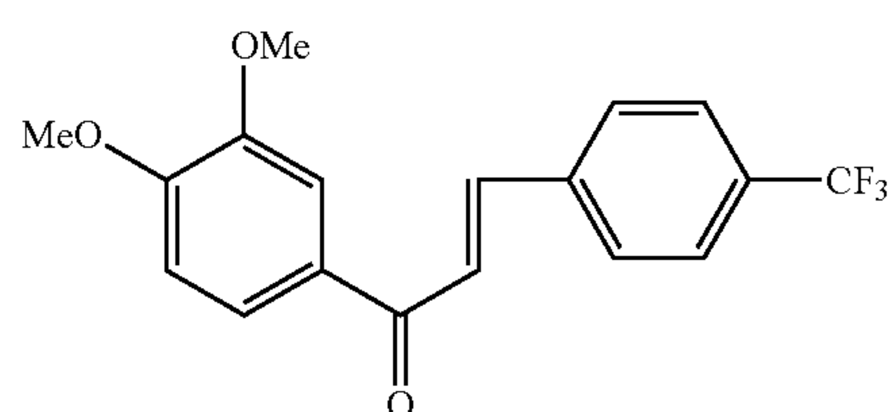
Compound 36
