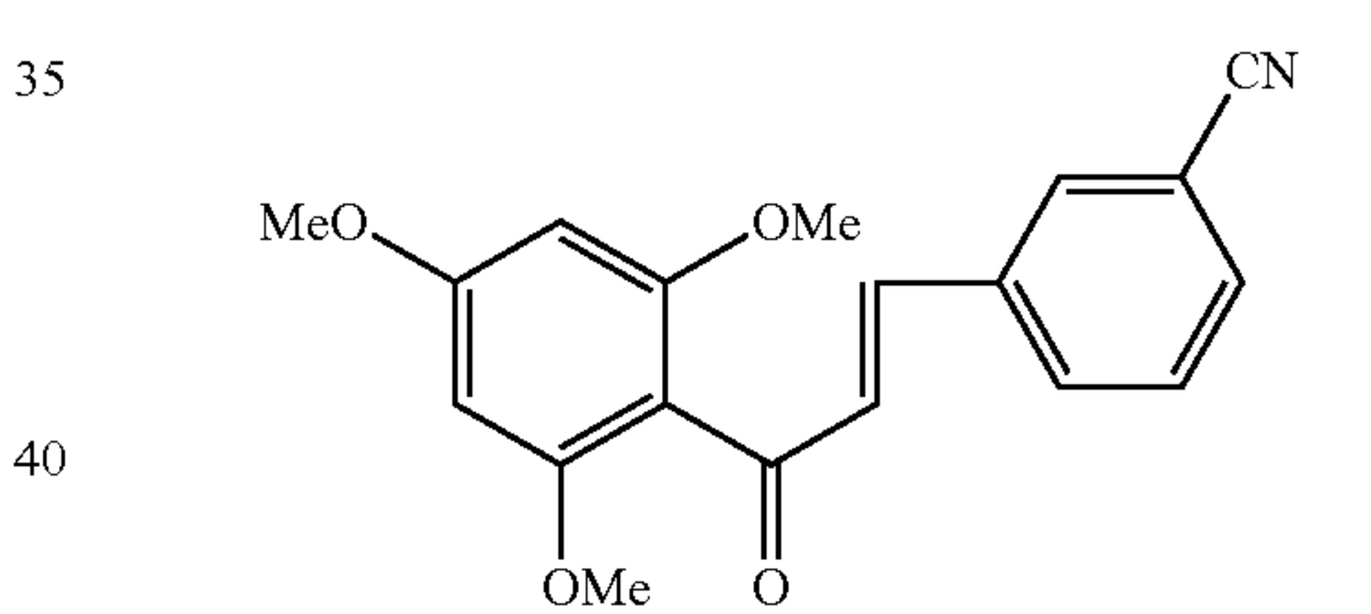
Compound 89
