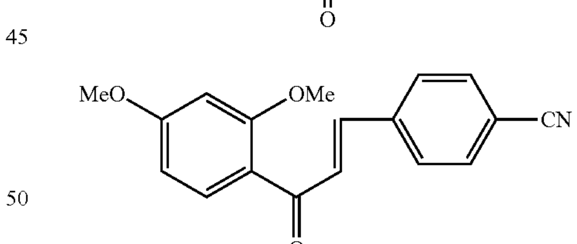
Compound 93
