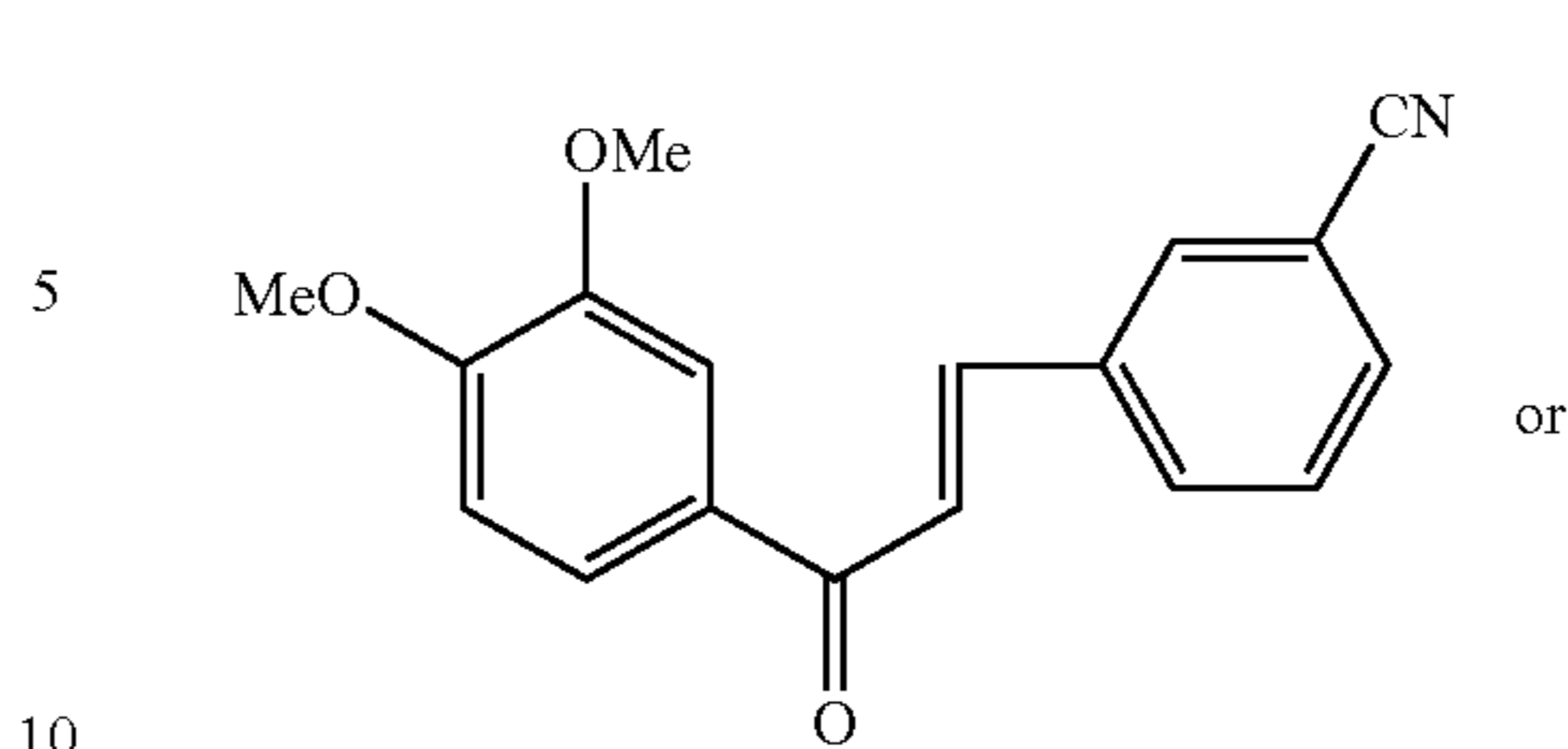
Compound 109
