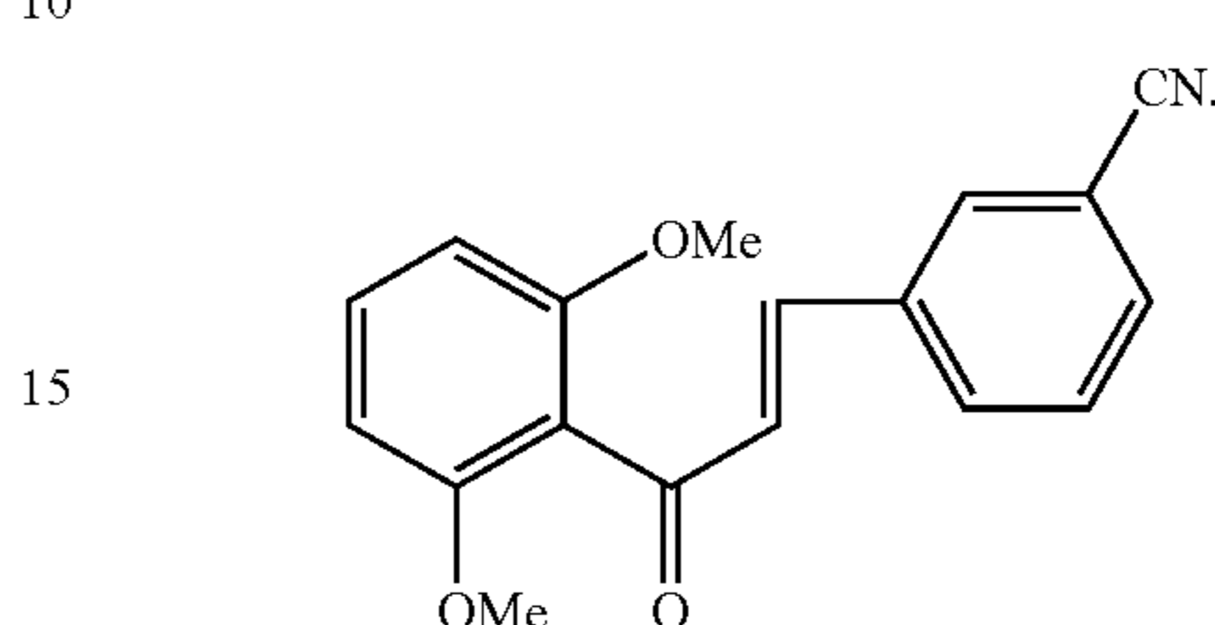
Compound 61
