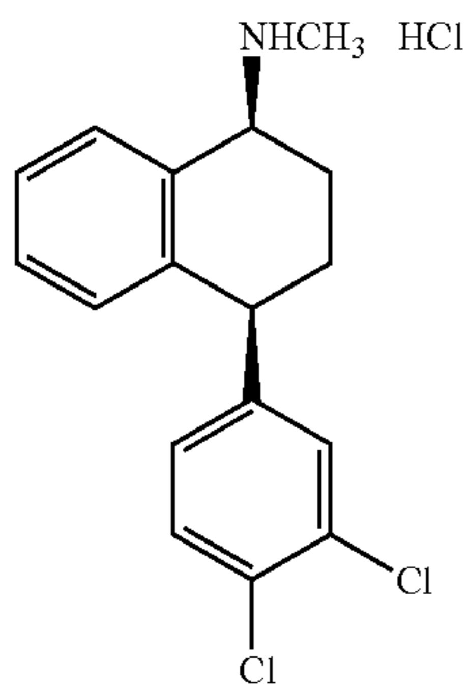
Sertraline hydrochloride
