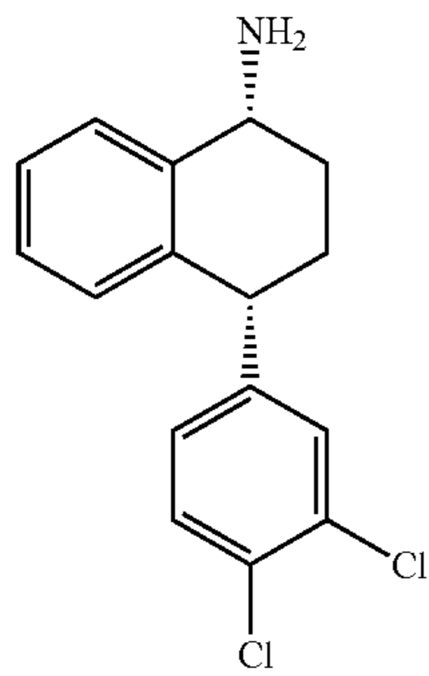
(1R, 4R)-desmethylsertraline
