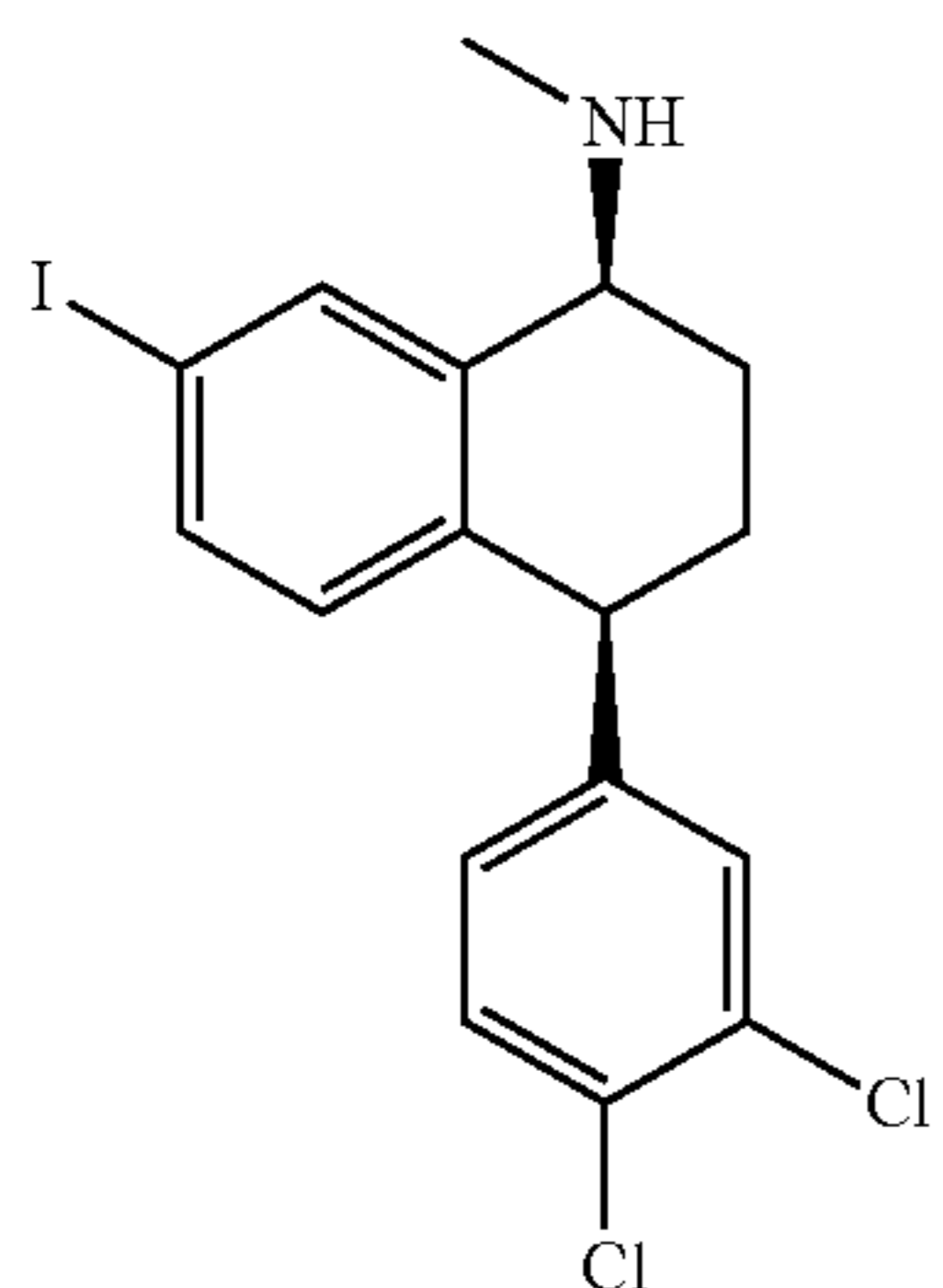
Sertraline iodide
