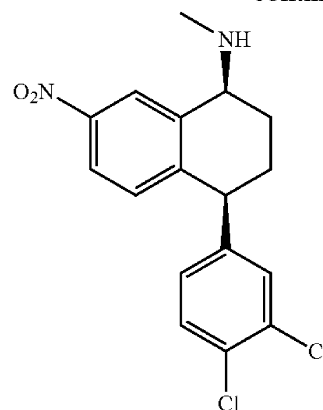
Nitro Sertraline
