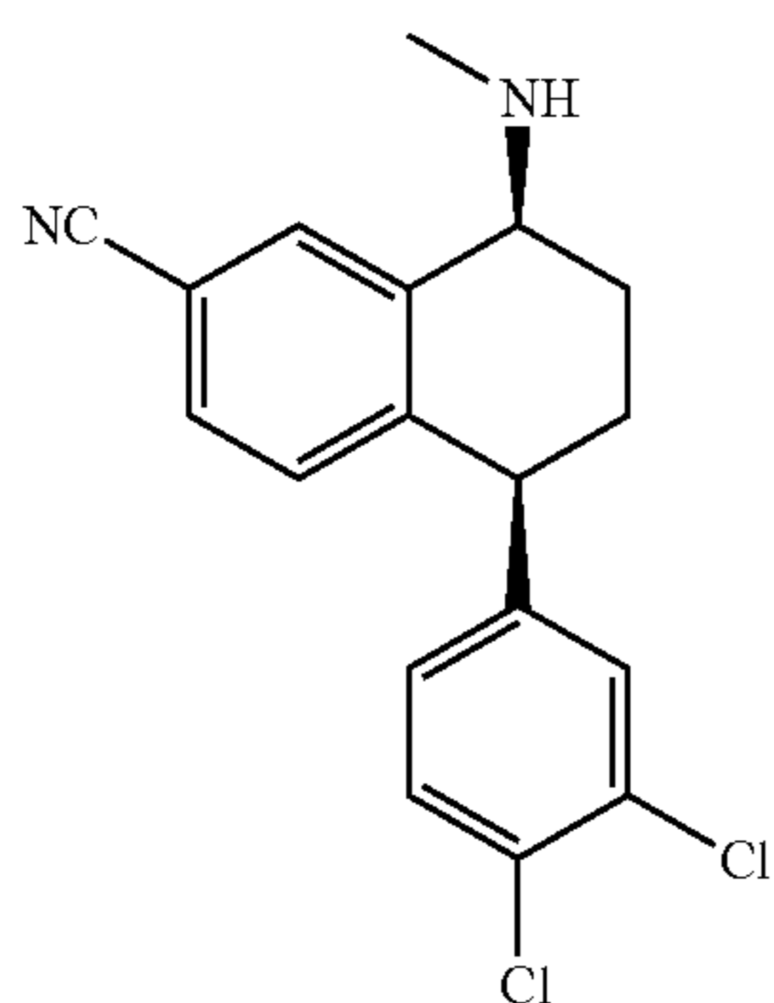
Sertraline nitrile
