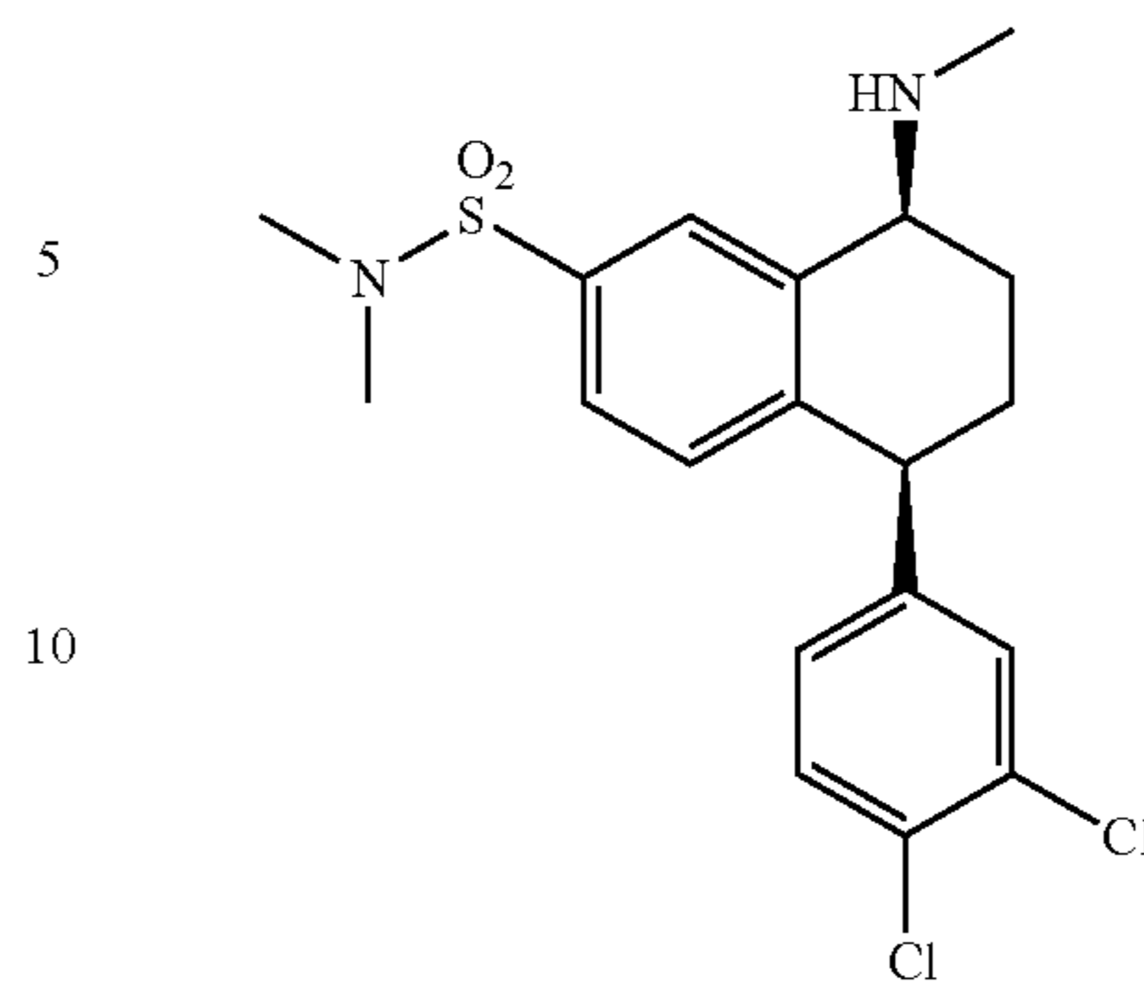
Sertraline N,N-Dimethylsulfonamide
