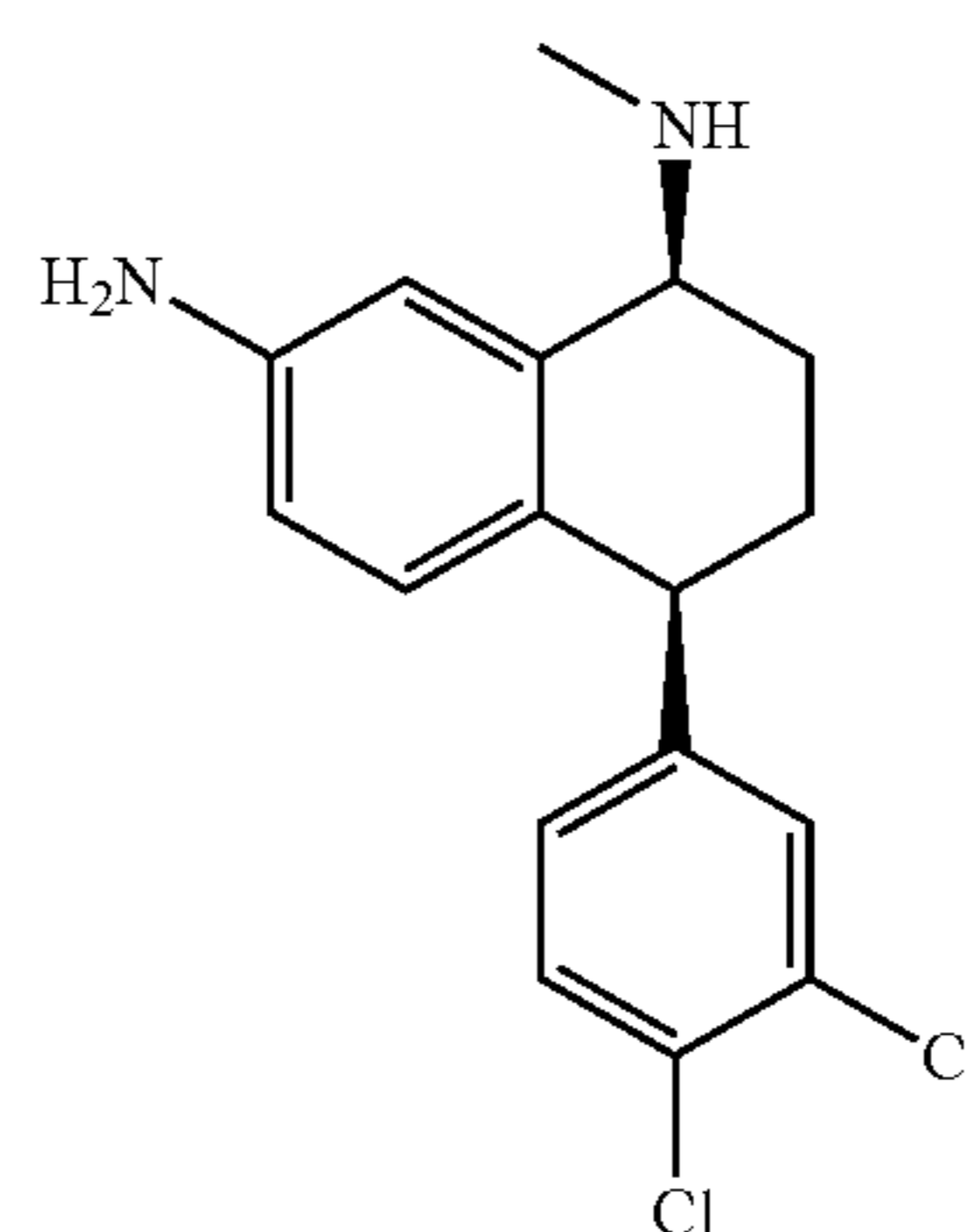
Sertraline aniline
