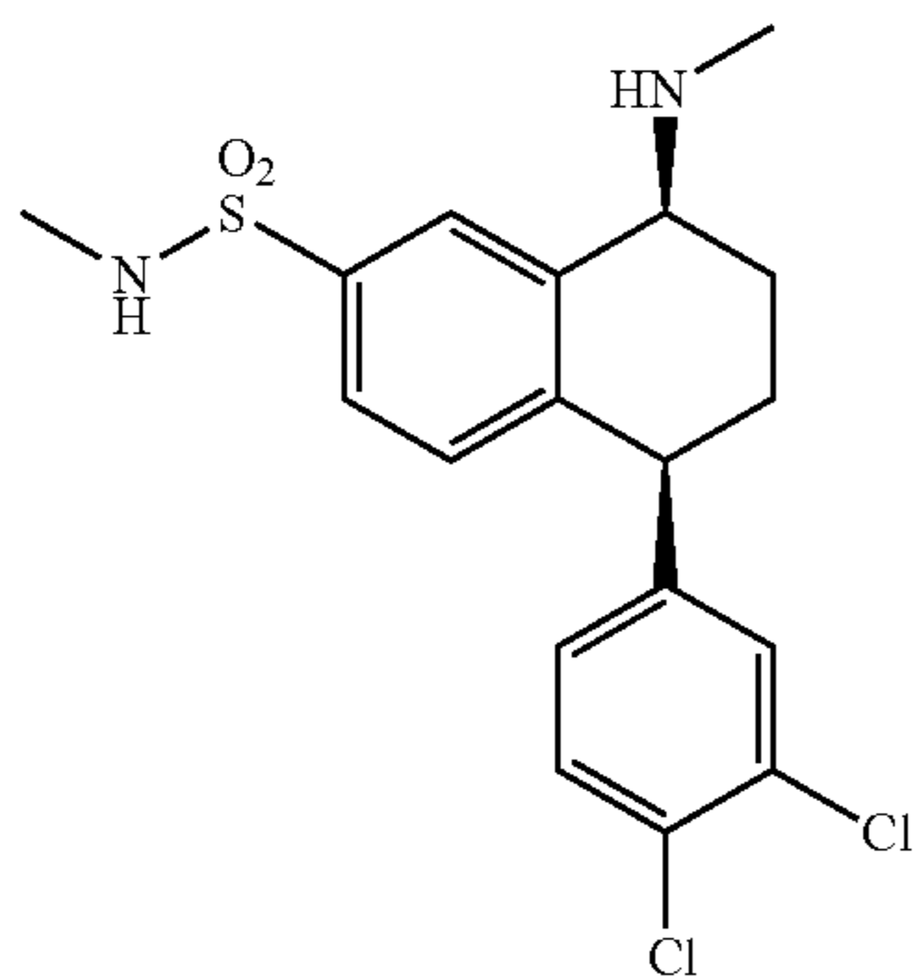
Sertraline sulfonamide
