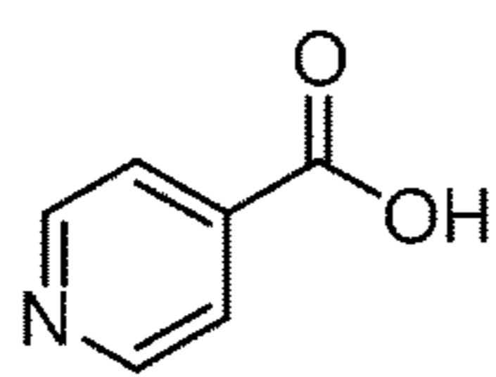
isonicotinic acid
