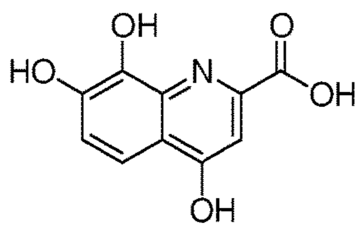
7,8-dihydroxykynurenic acid
