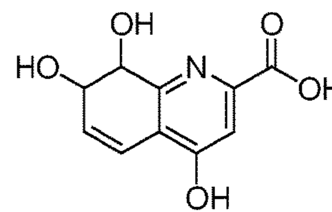
7,8-dihydro-7,8-dihydroxykynurenic acid
