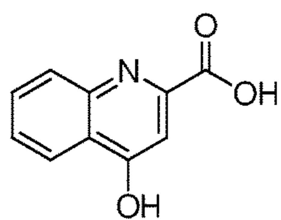
kynurenic acid
