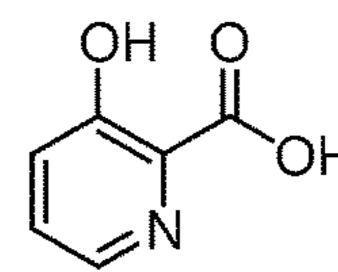
3-hydroxypicolinic acid
