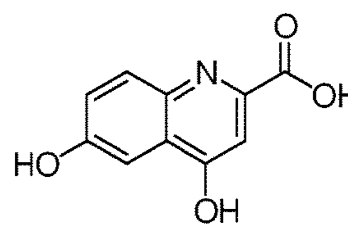
6-hydroxykynurenic acid
