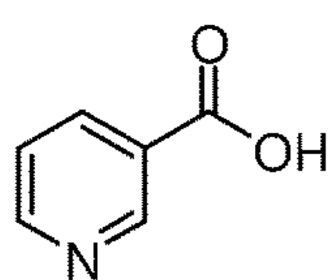
nicotinic acid
