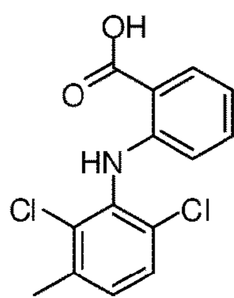
Meclofenamic acid
