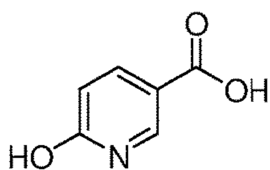
6-hydroxynicotinic acid
