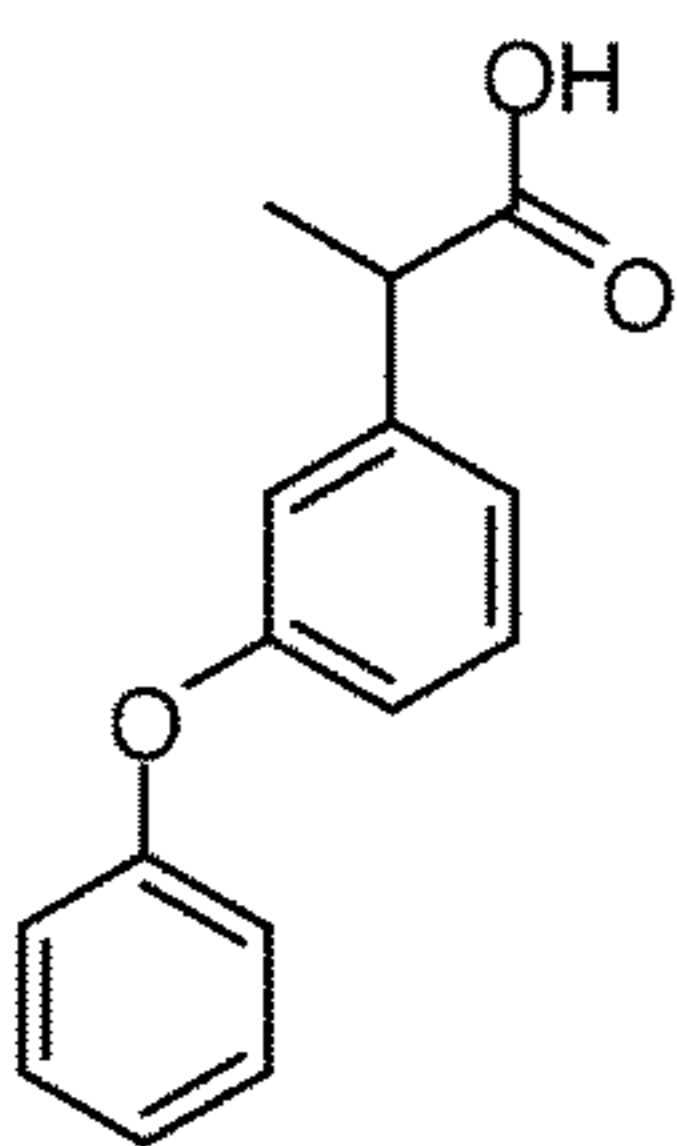
Fenoprofen
