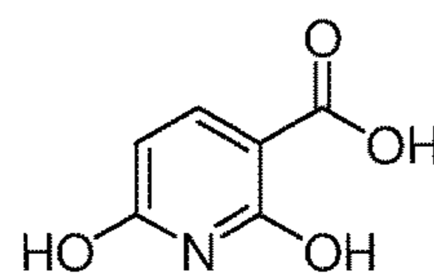
2,6-dihydroxynicotinic acid
