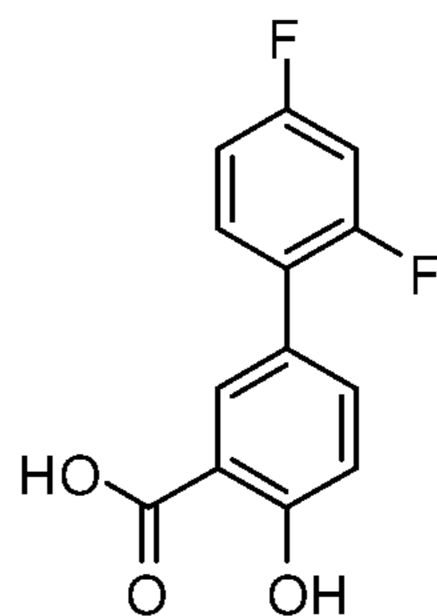
Diflusalol
