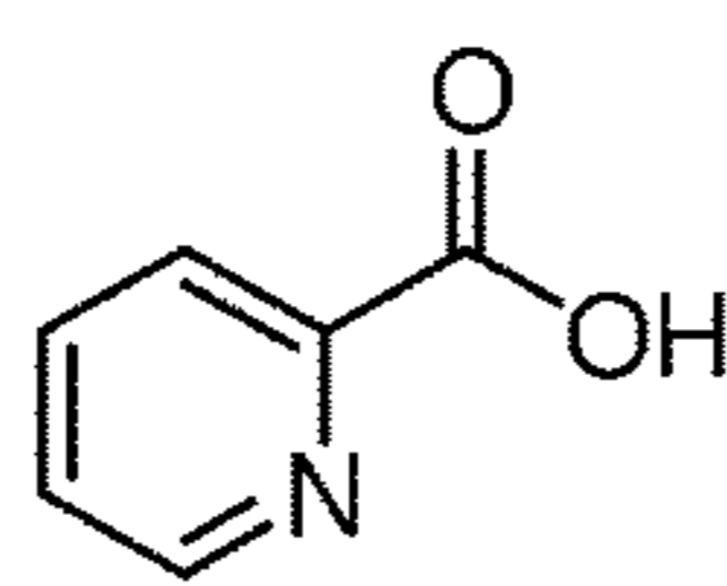
picolinic acid
