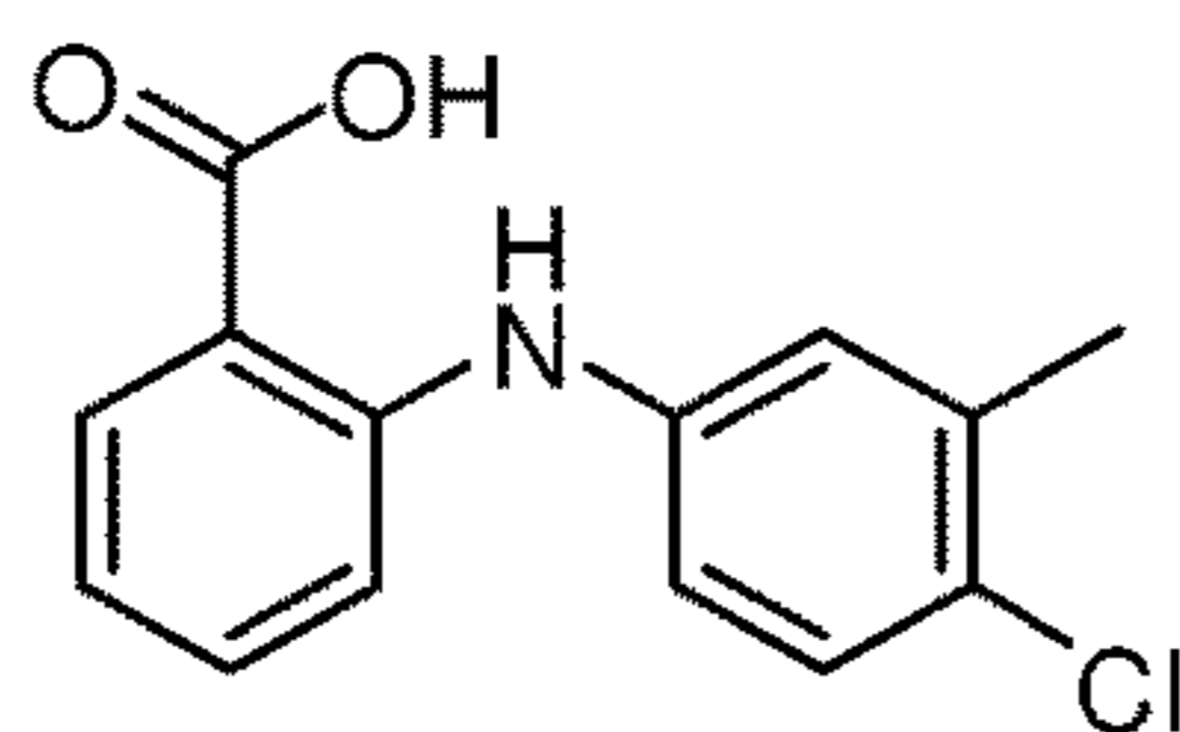
Tolfenamic acid
