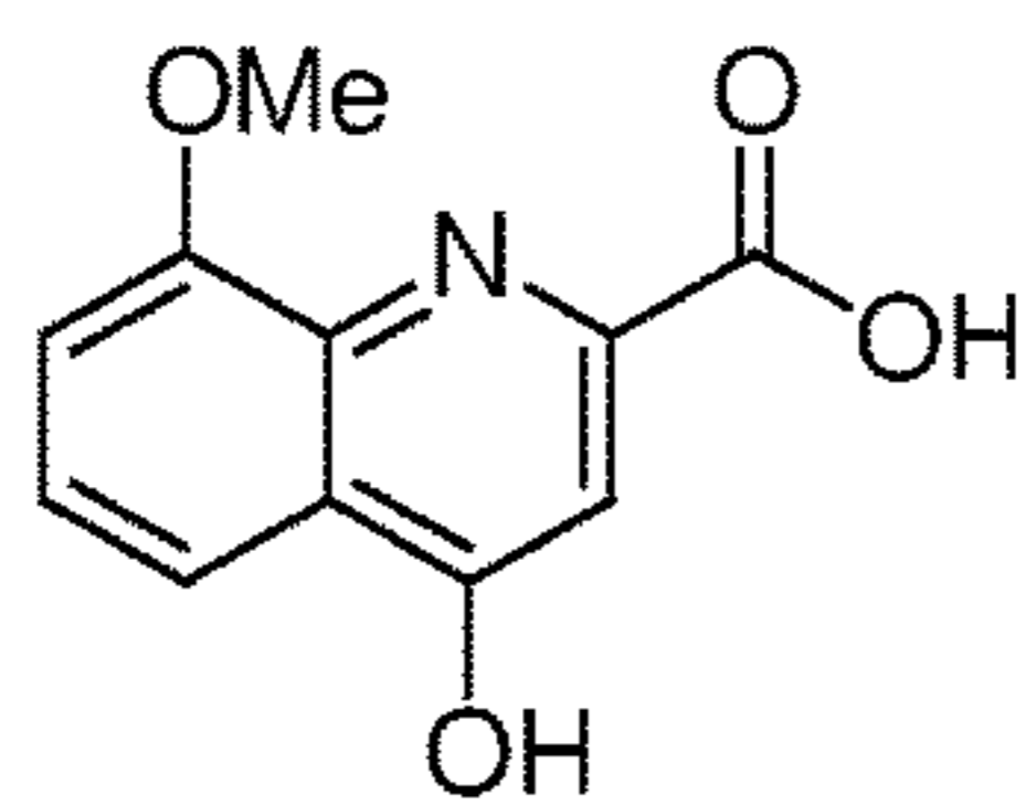
8-methoxykynurenic acid
