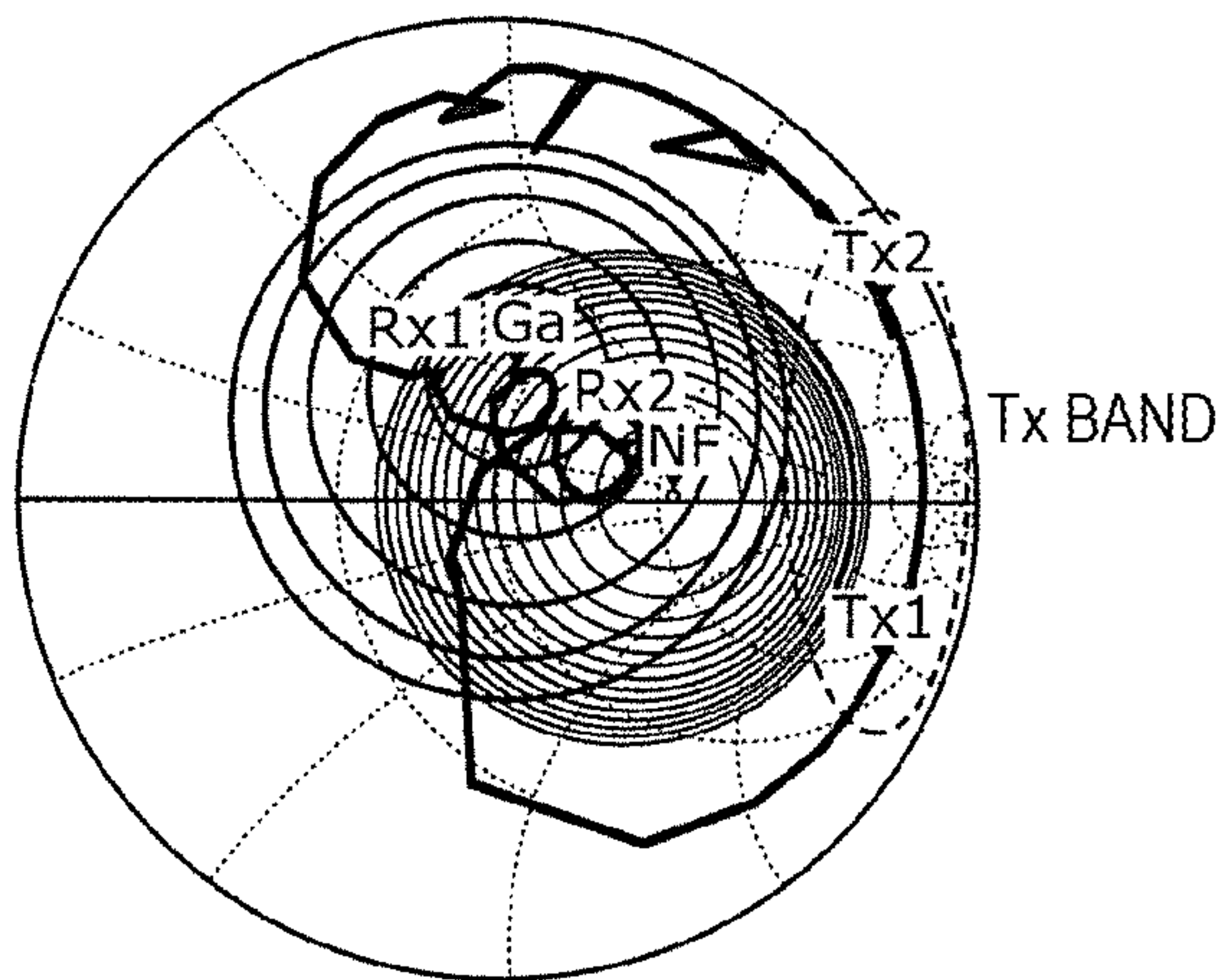
THIRD EXAMPLE DUPLEXER Rx IN-BAND IMPEDANCE: 110Ω
