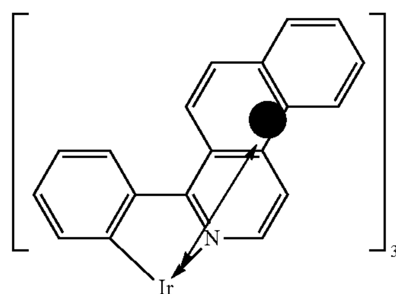
\text{Ir}(\text{piq})_3
