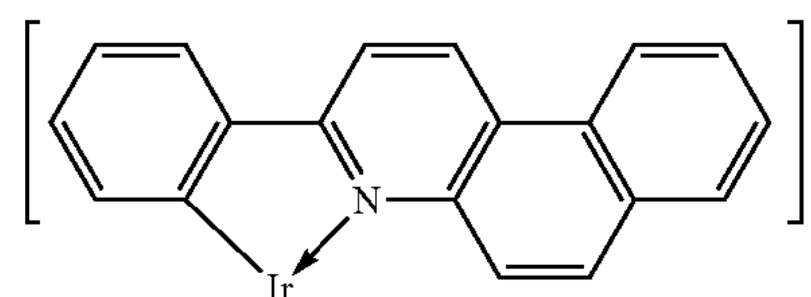
\text{Ir}(\text{pq})_3
