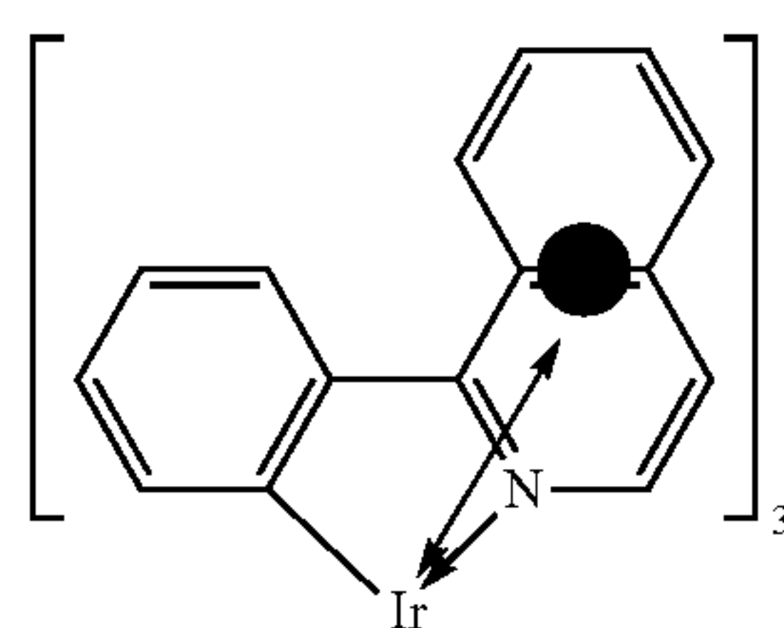
\text{Ir}(\text{piq})_3
