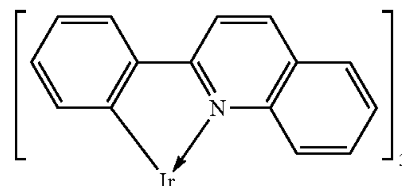
\text{Ir}(\text{pq})_3
