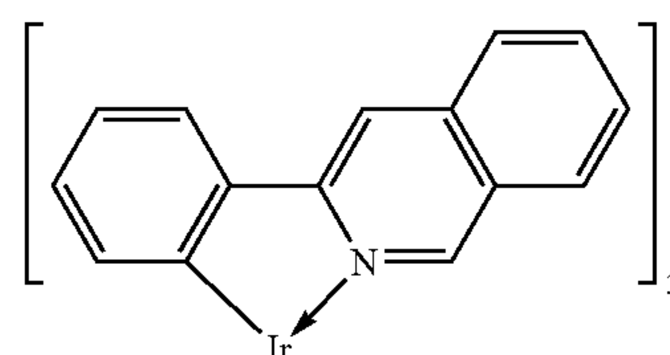
\text{Ir}(\text{p-3iq})_3
