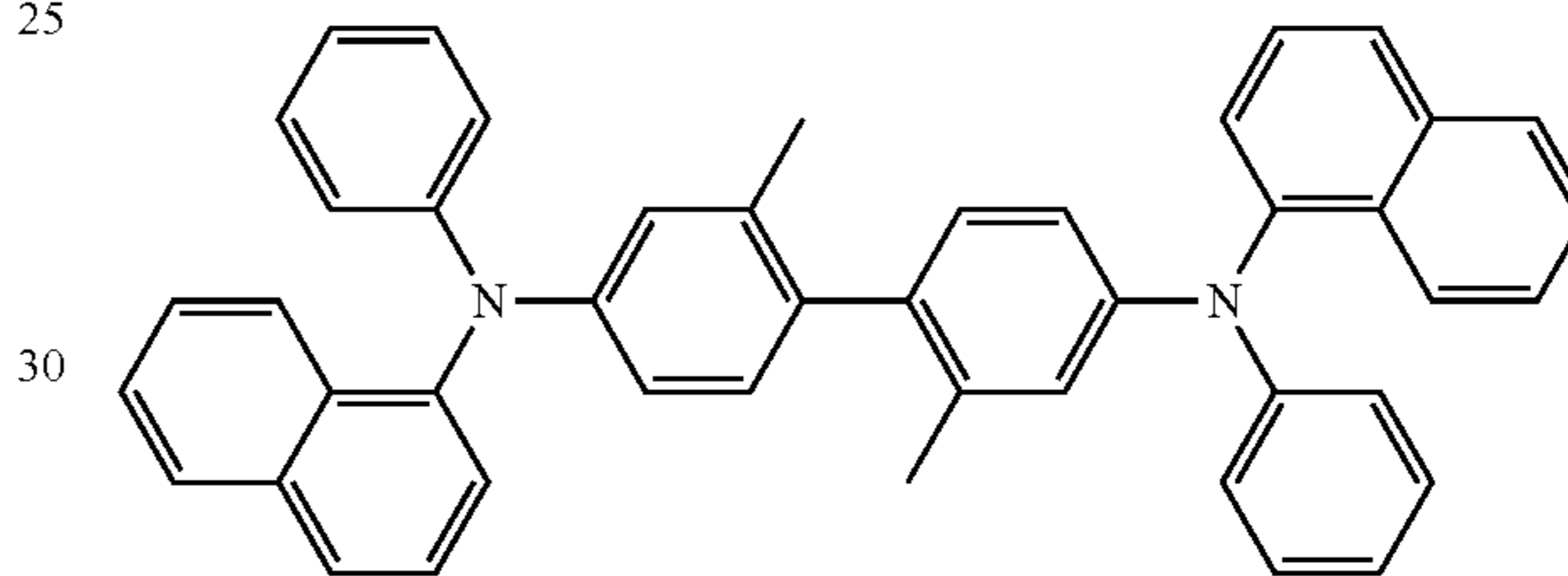
\alpha -NPB
