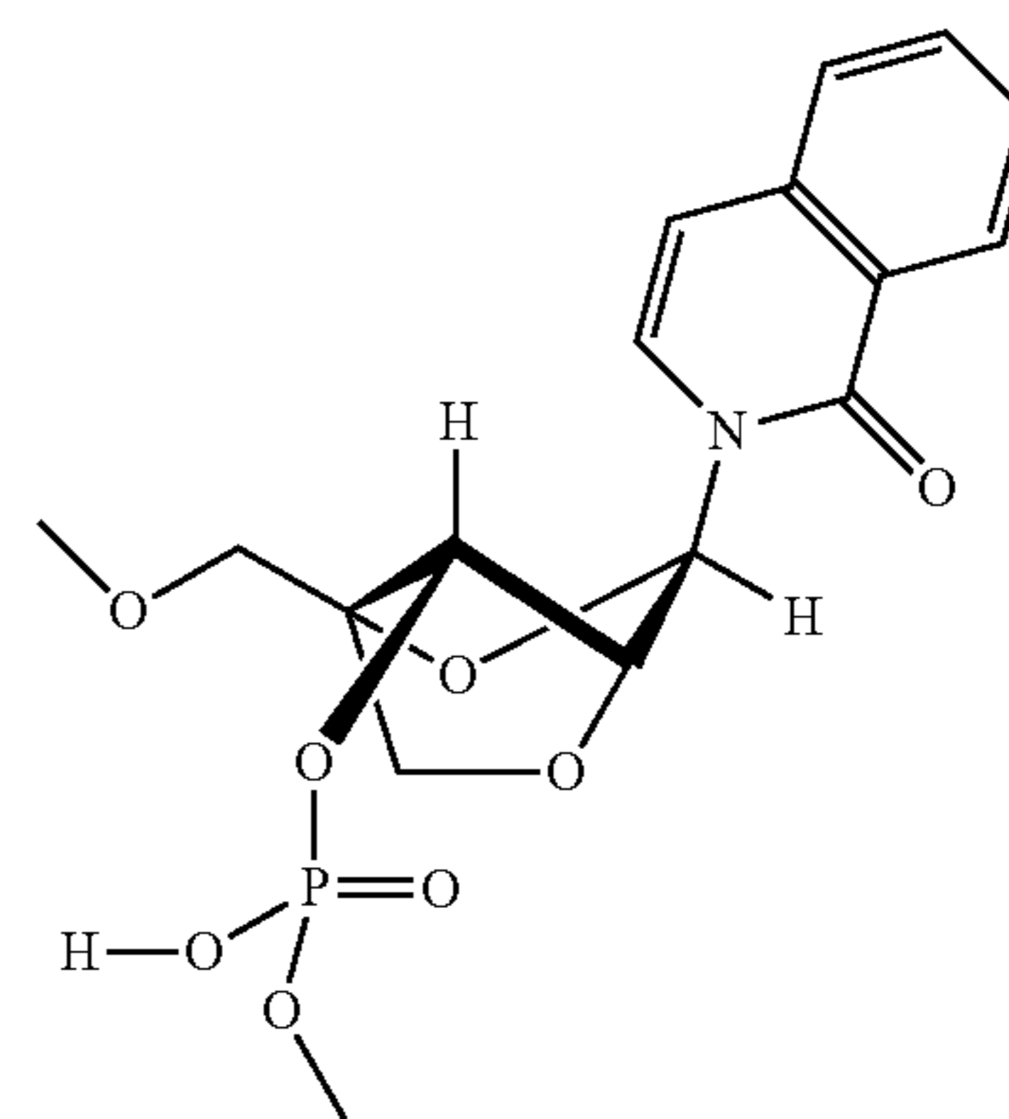
2',4'-BNA-1-isoquinolone
