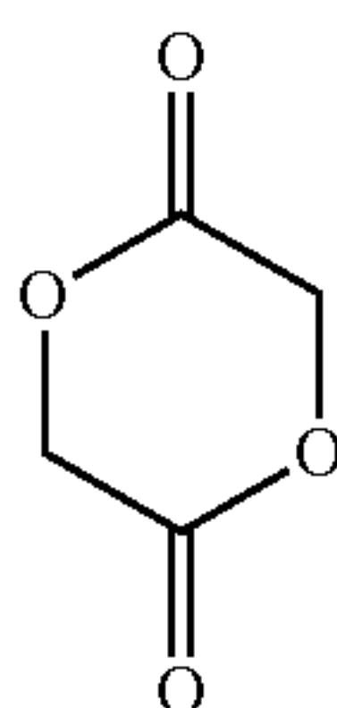
Glycolide (GLY)
