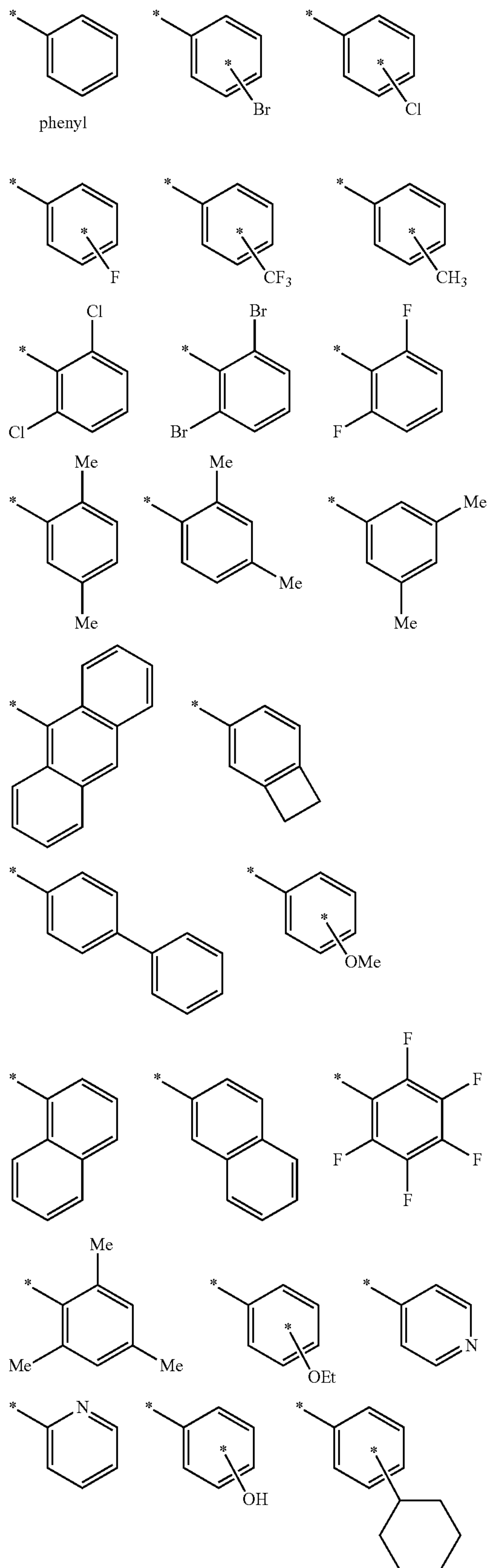
Scheme 10.
