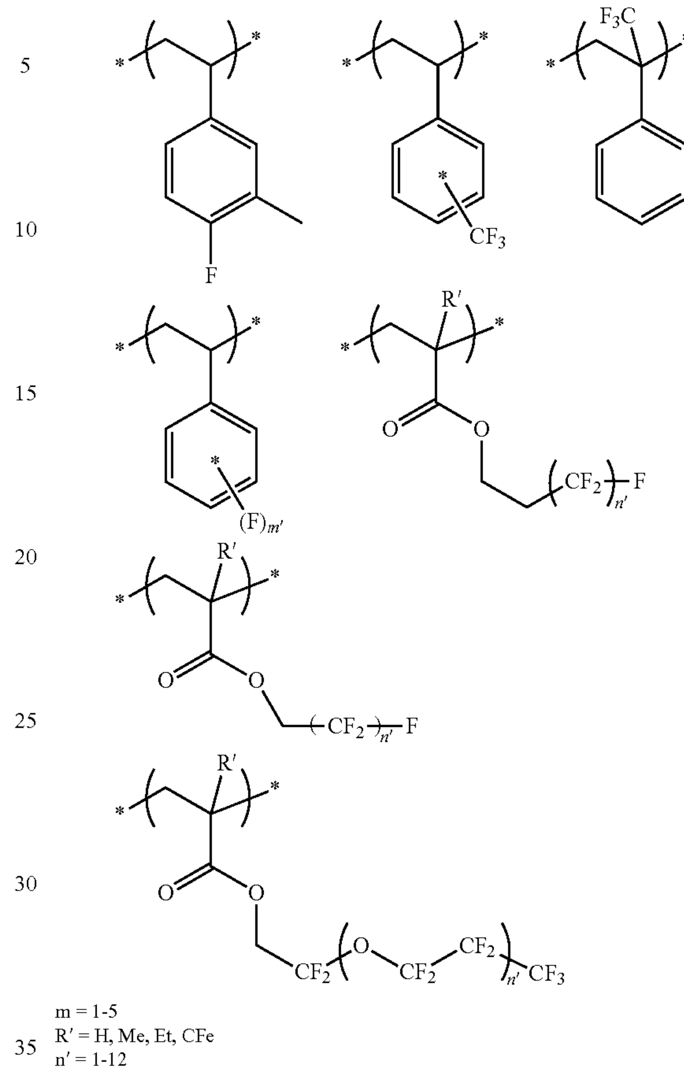
Scheme 4.
