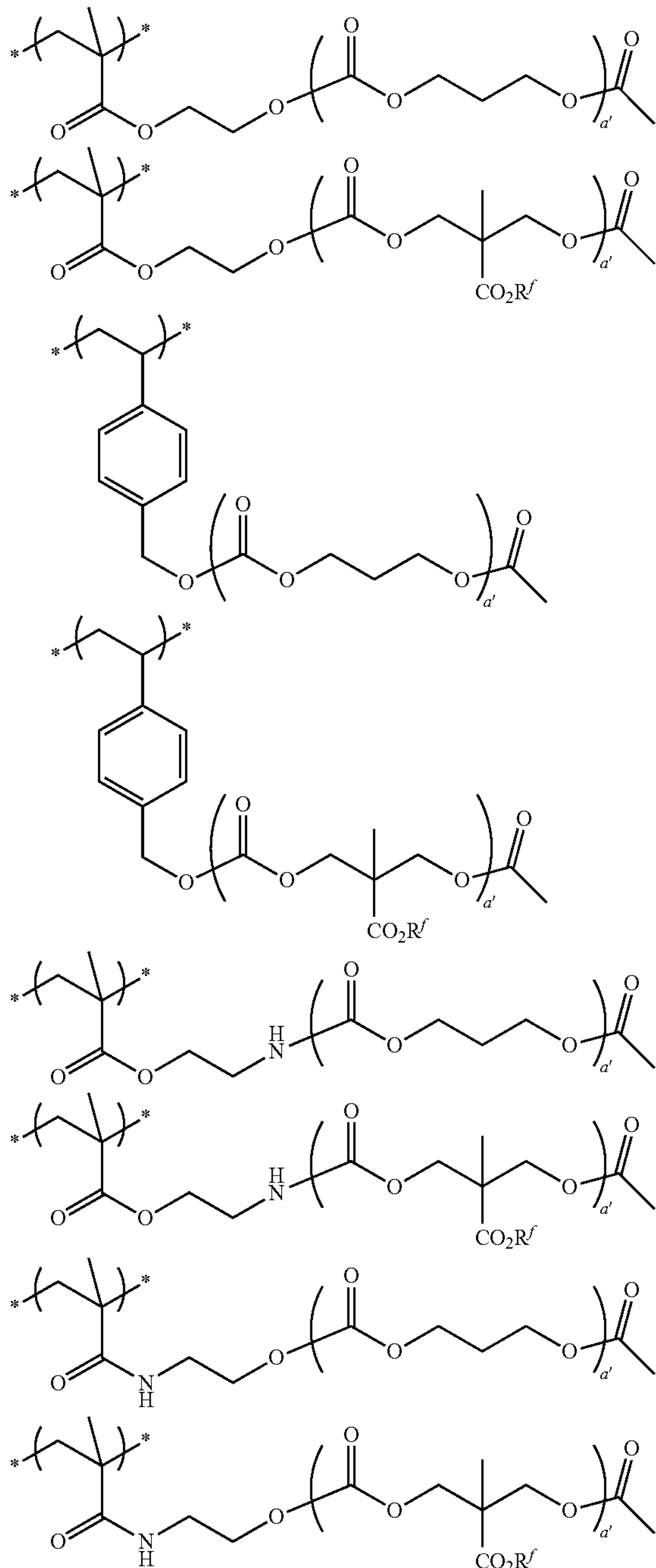
Scheme 13b.
