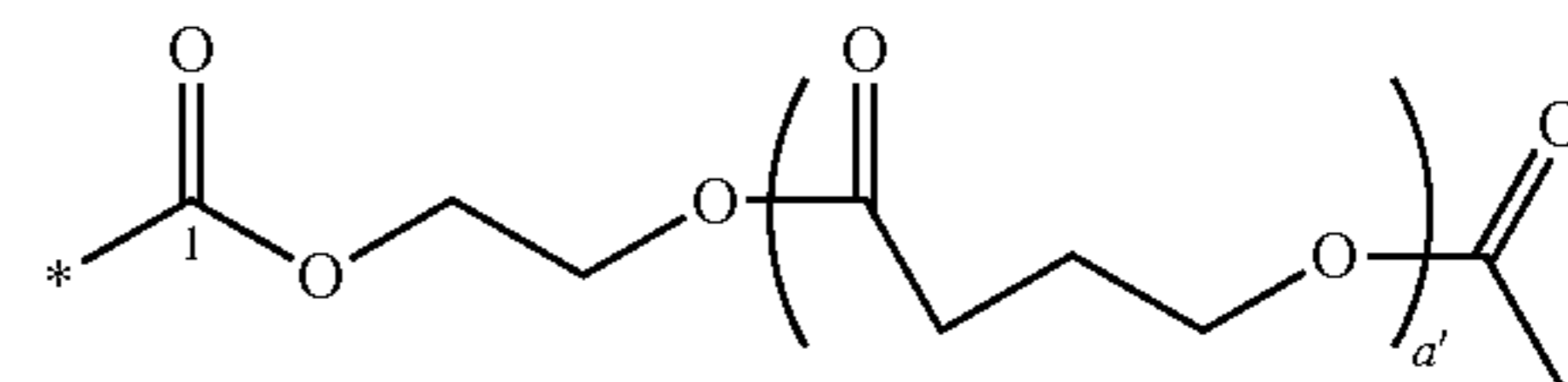
Scheme 12.
