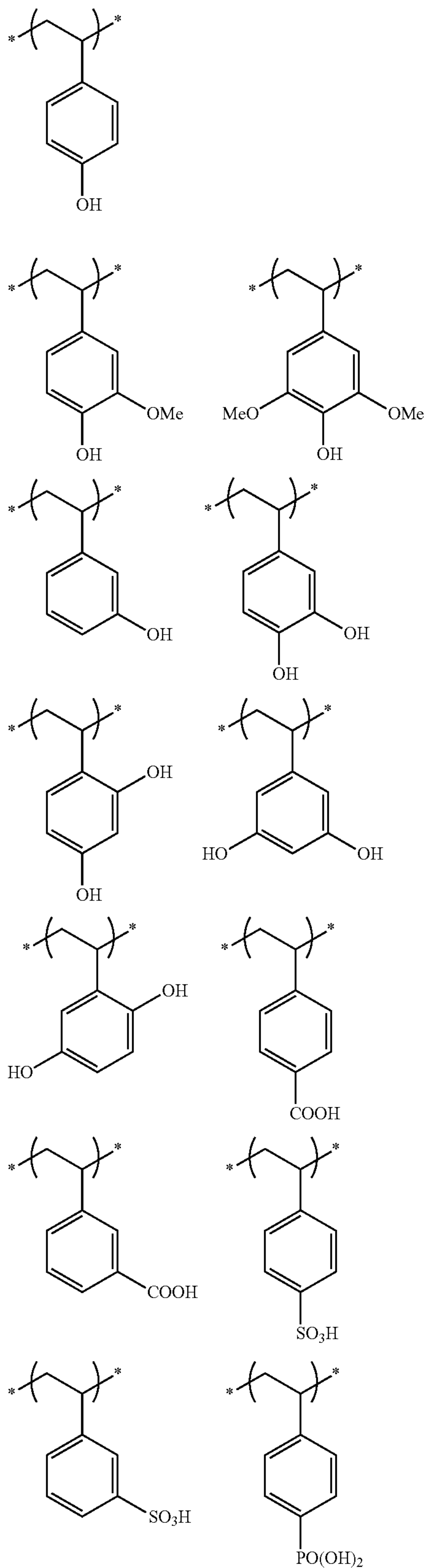
Scheme 6.
