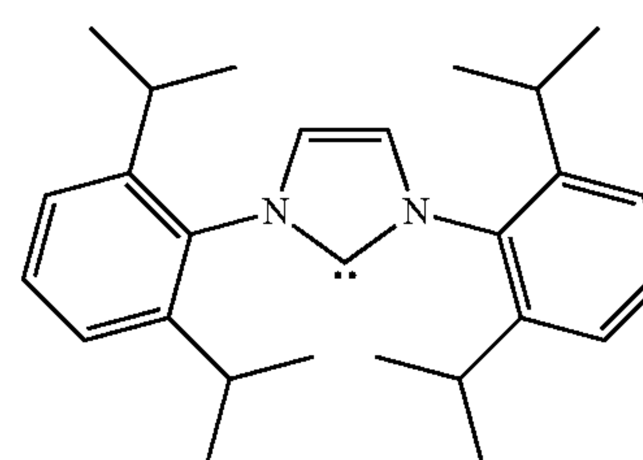
1,3-Bis(2,6-di- i -propylphenyl)imidazol-2-ylidene
