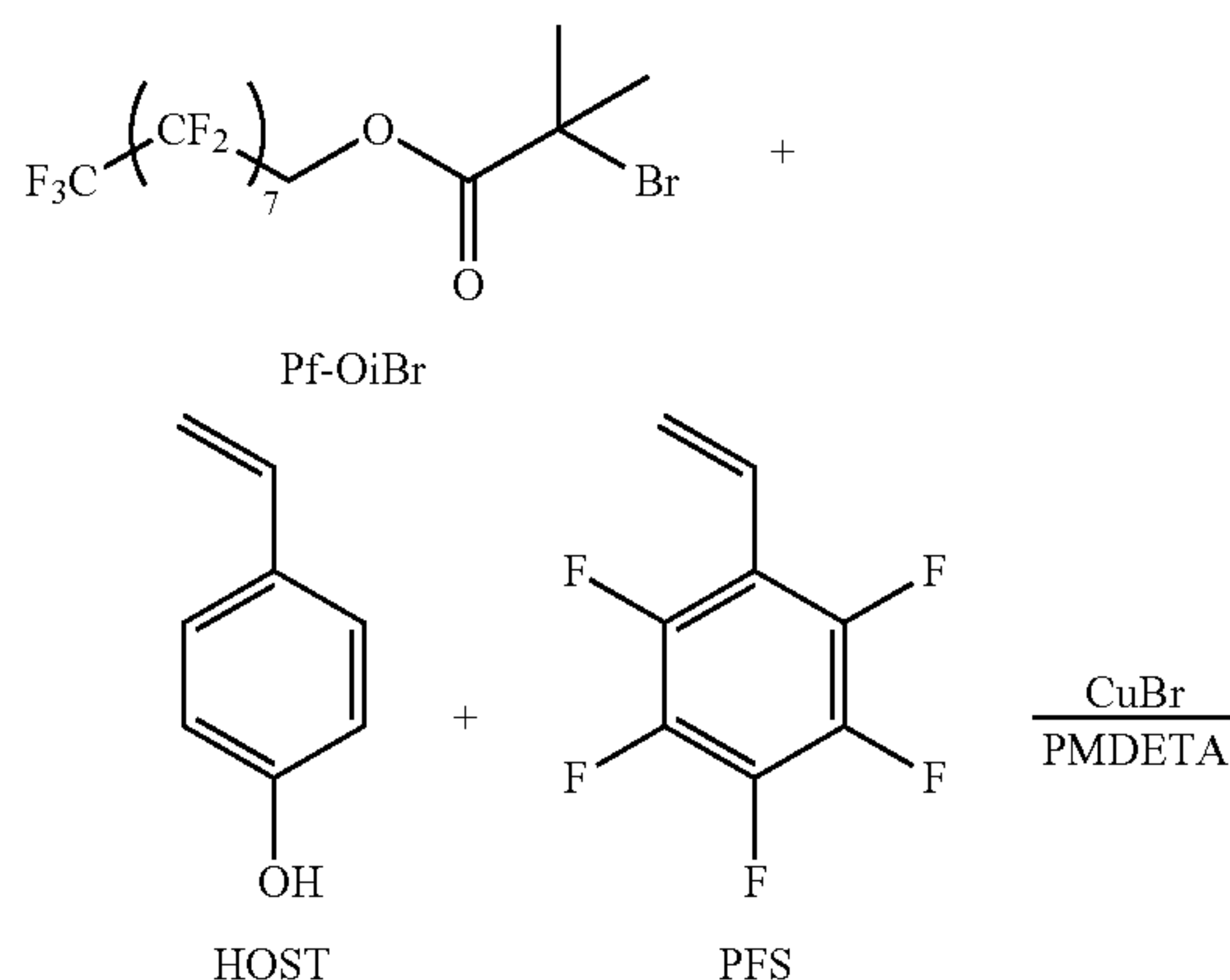
Scheme 9.
