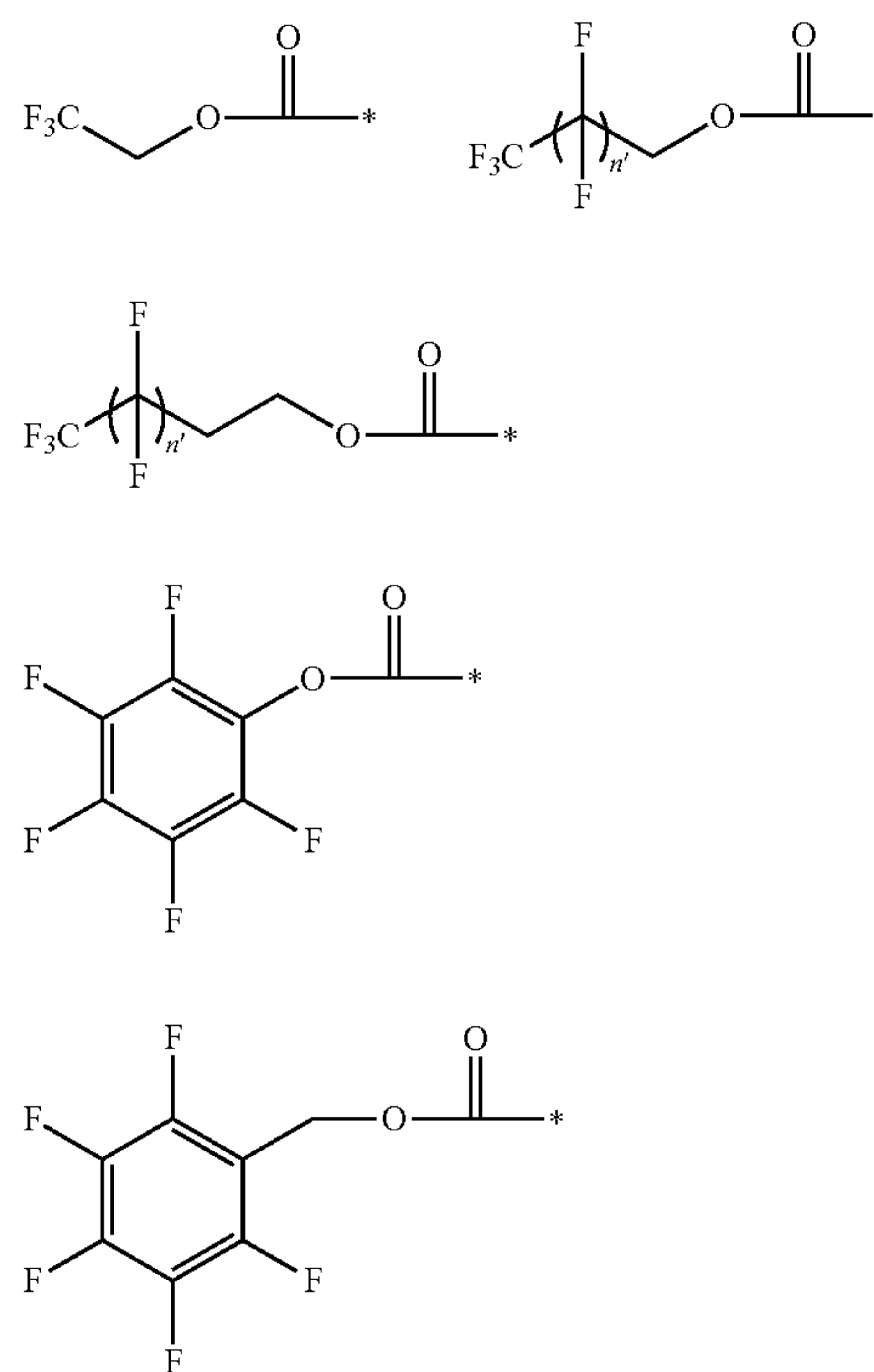
Scheme 8.
