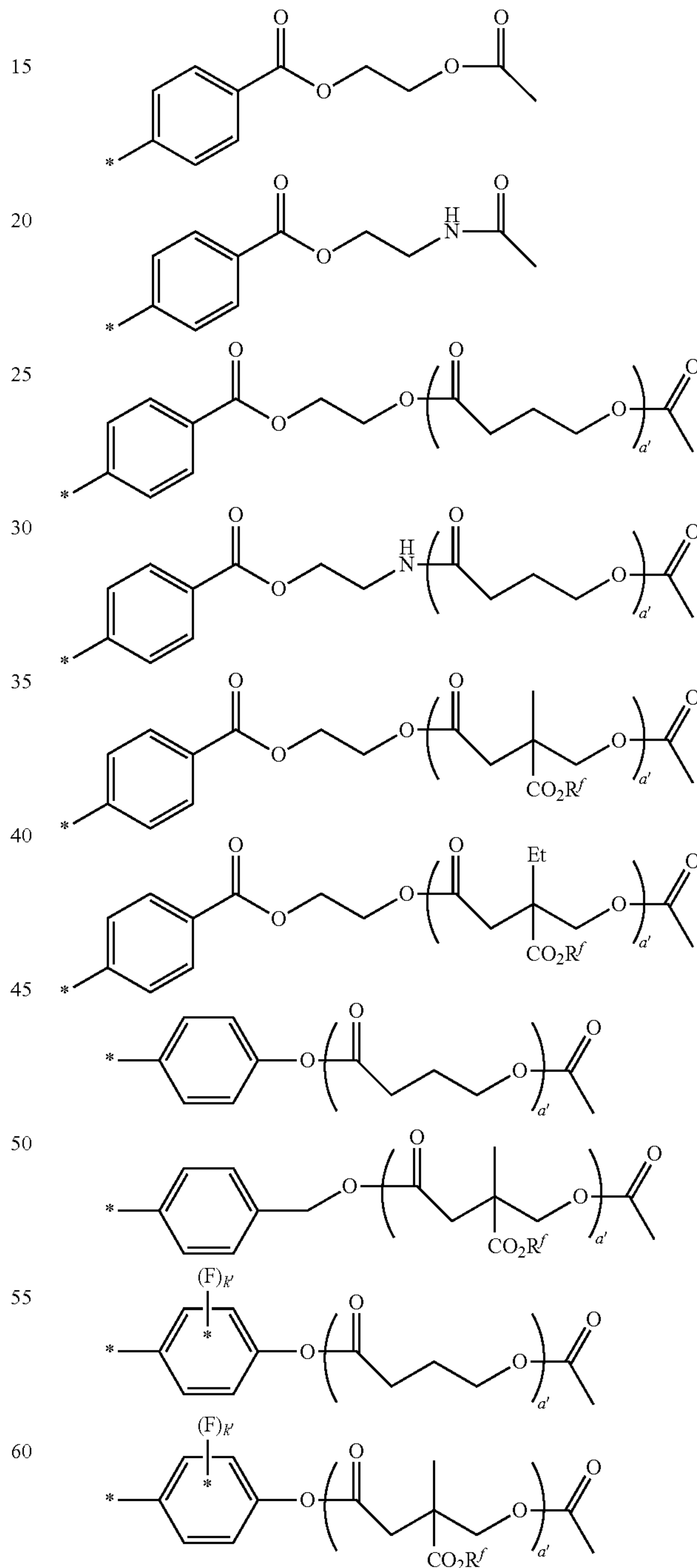
Scheme 13.
