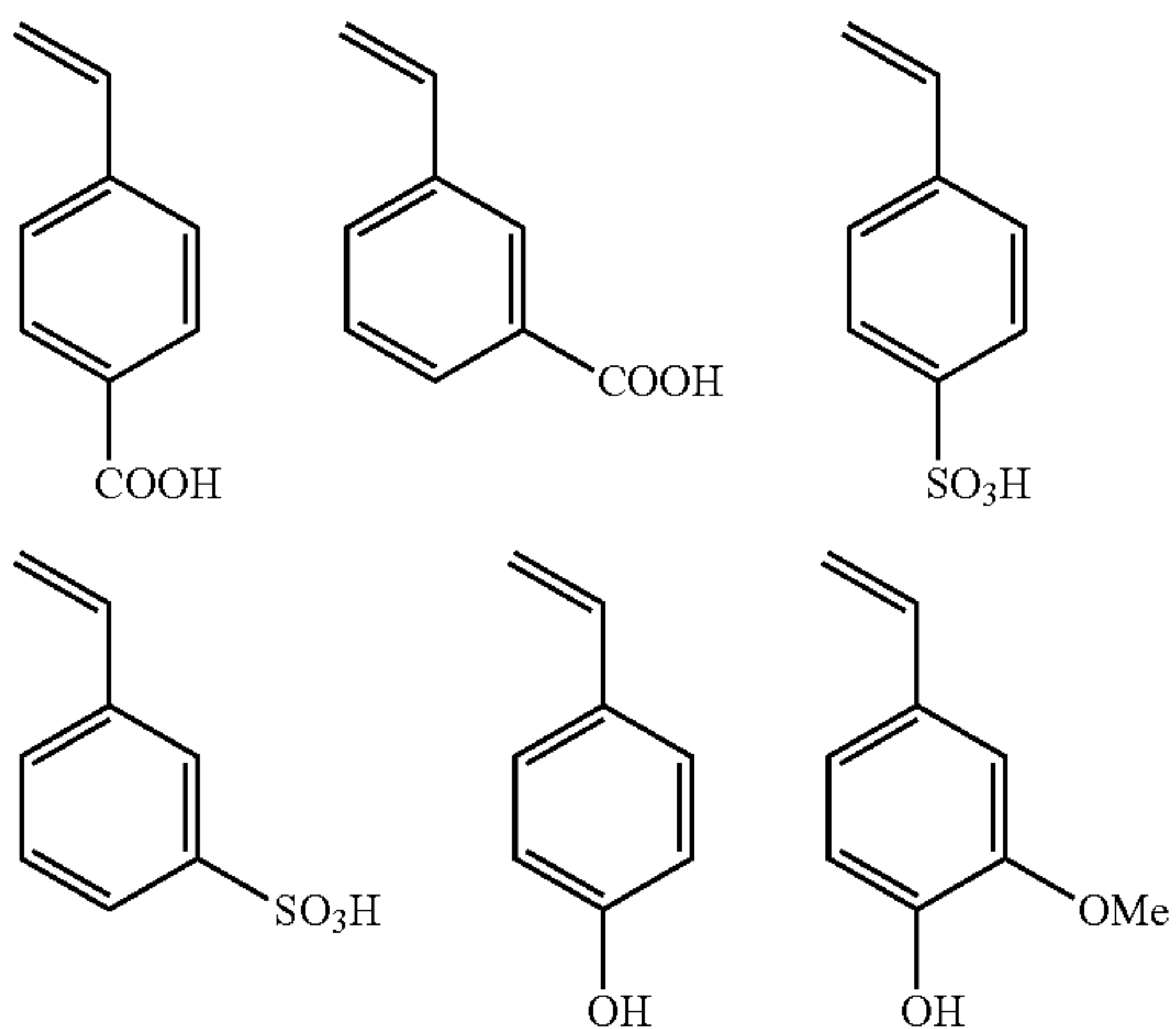
Scheme 7.
