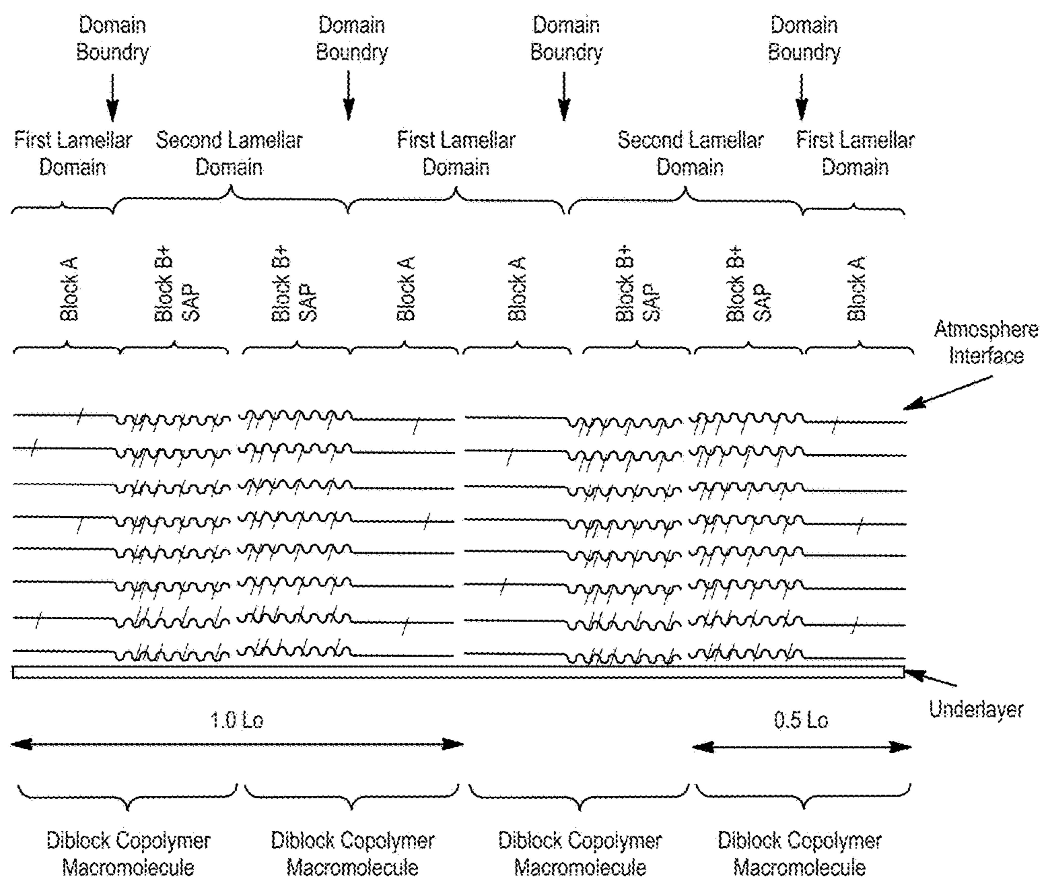
Scheme 3.
