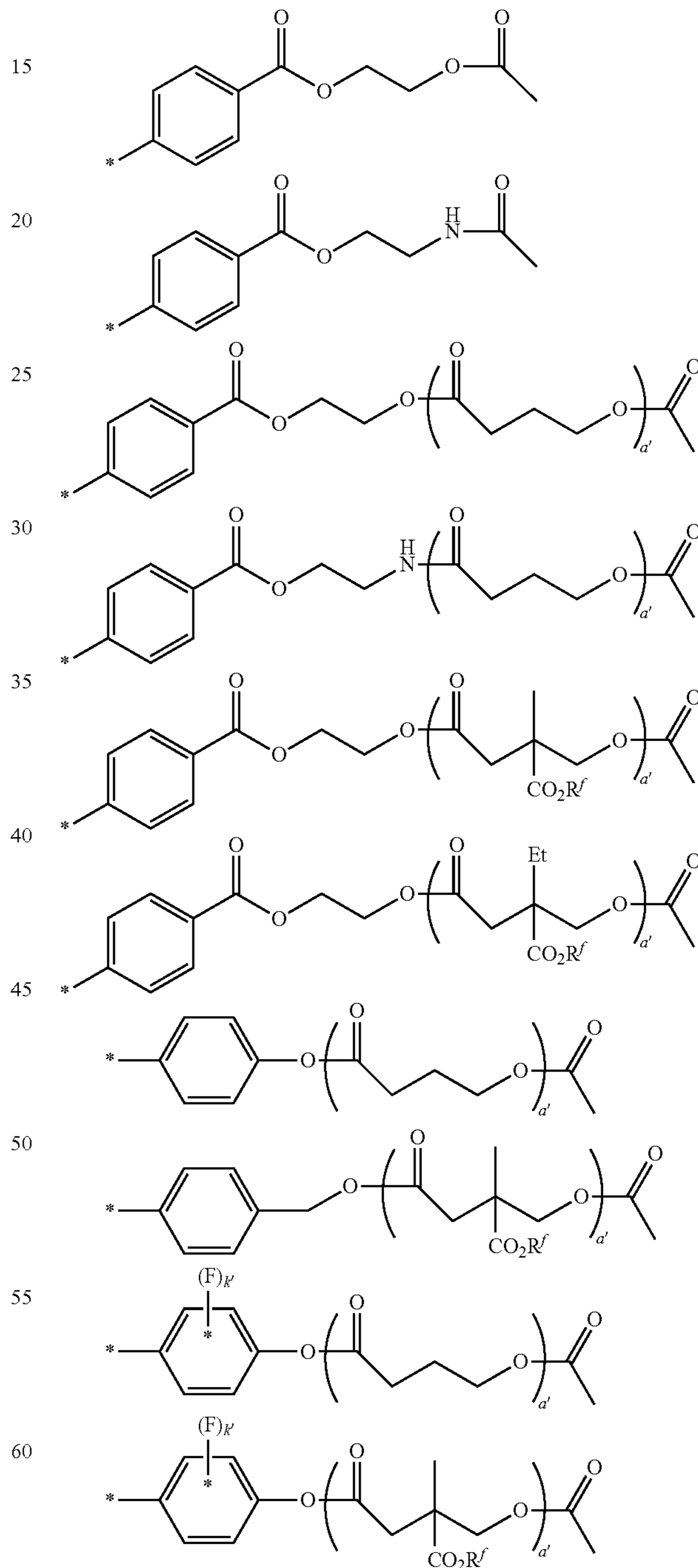
Scheme 13.
