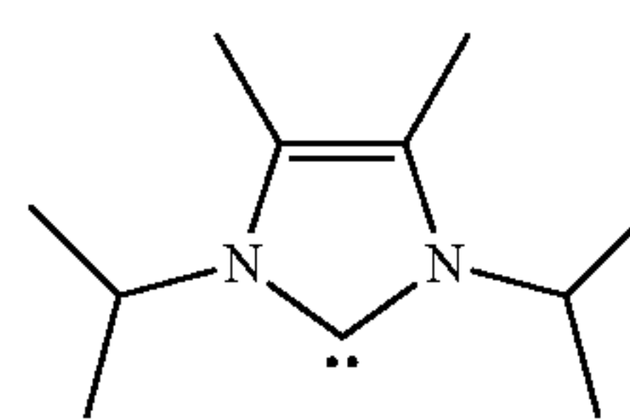
1,3-Bis(2-propyl)-4,5-dimethylimidazol-2-ylidene
