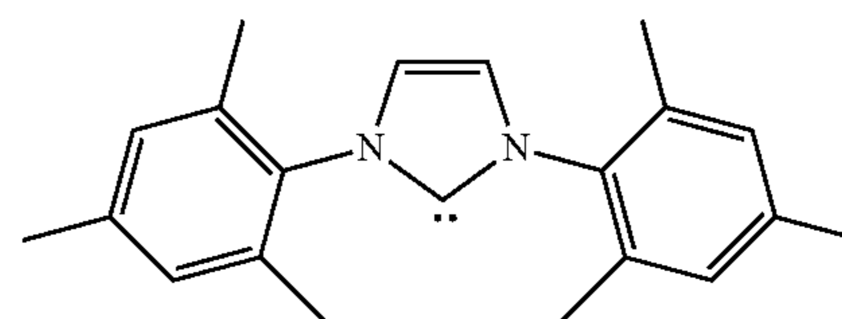
1,3-Bis(2,4,6-trimethylphenyl)imidazol-2-ylidene
