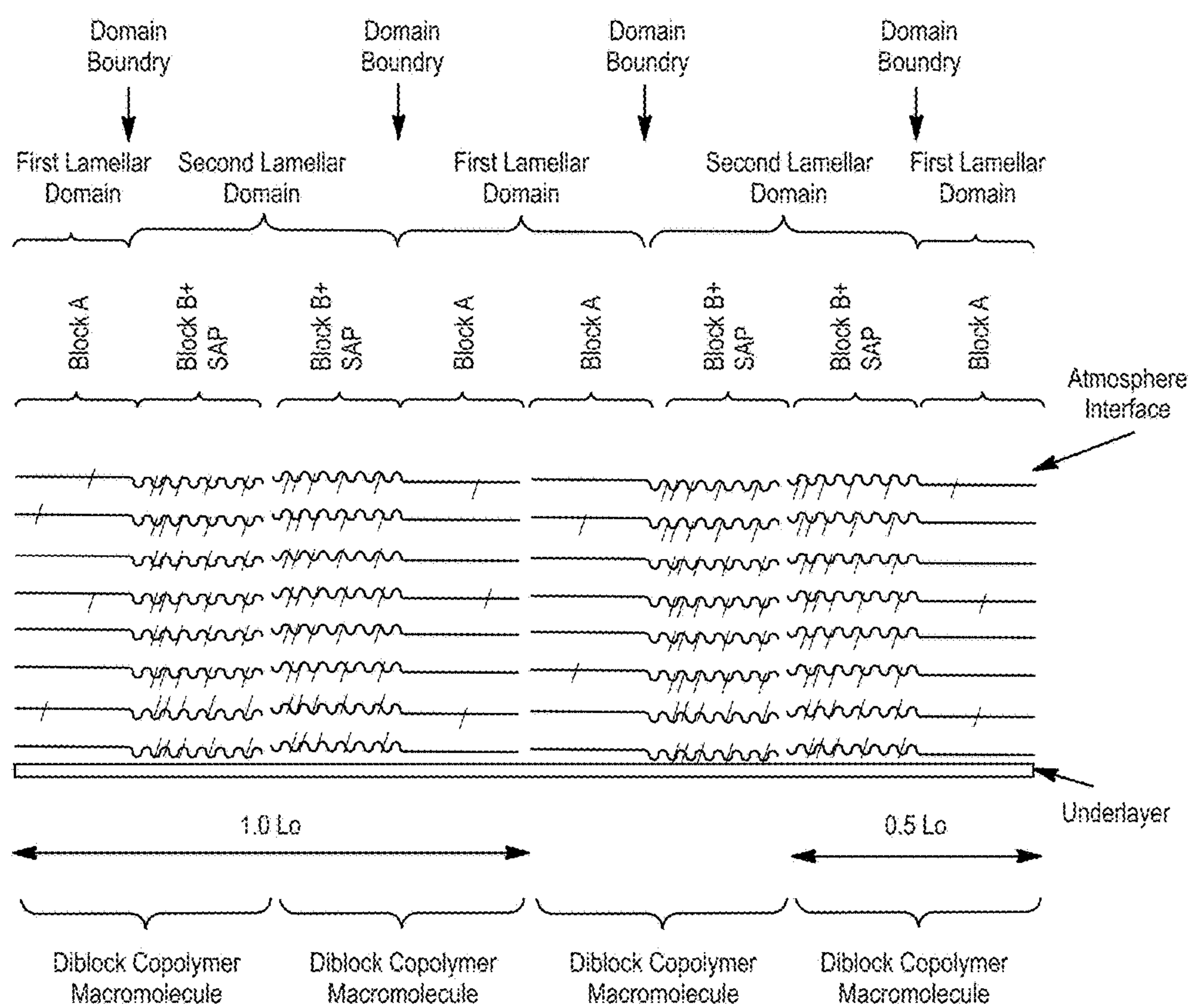
Scheme 3.
