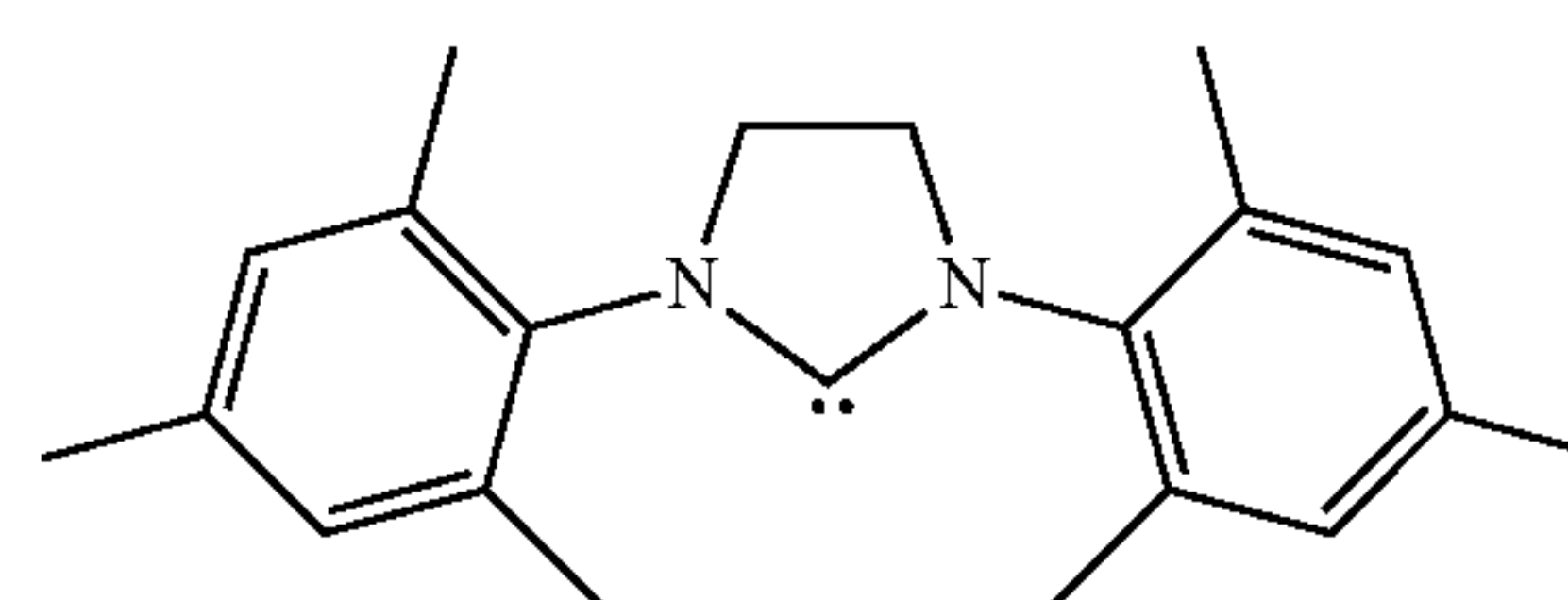
1,3-Bis(2,4,6-trimethylphenyl)-4,5-dihydroimidazol-2-ylidene
