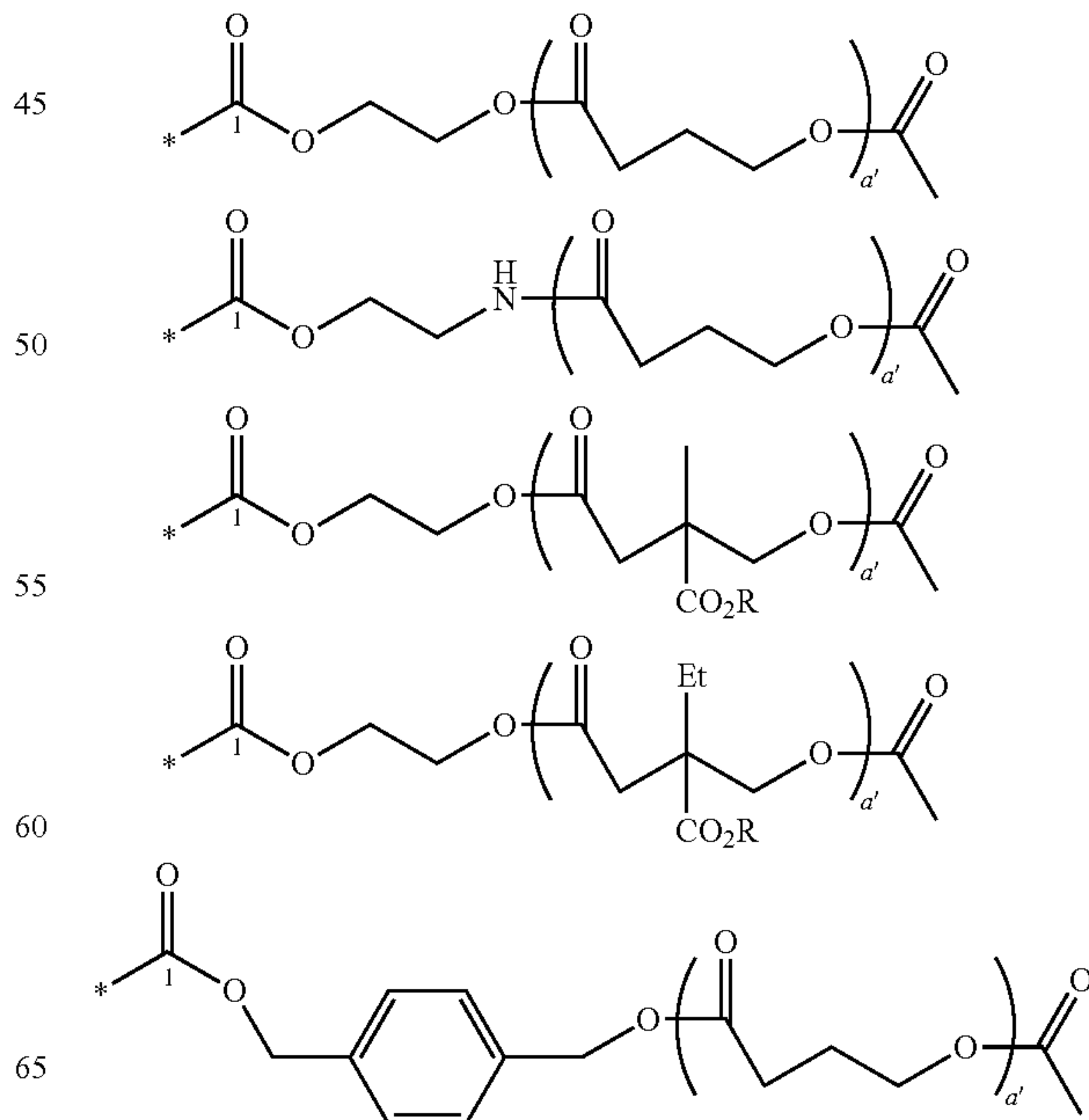
Scheme 12.
