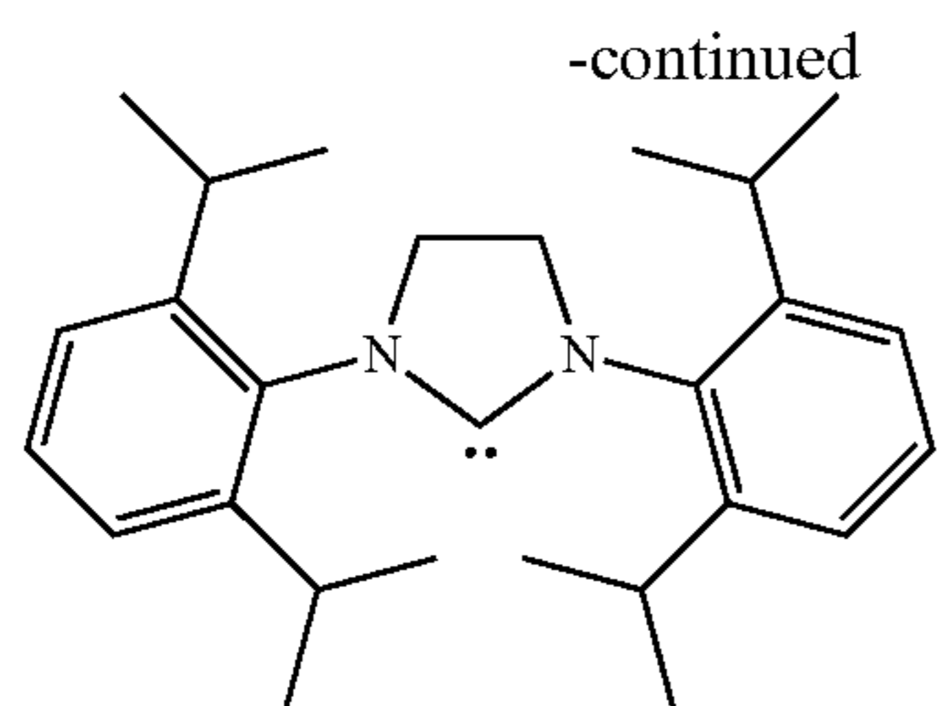
1,3-Bis(2,6-di-i-propylphenyl)-4,5-dihydroimidazol-2-ylidene
