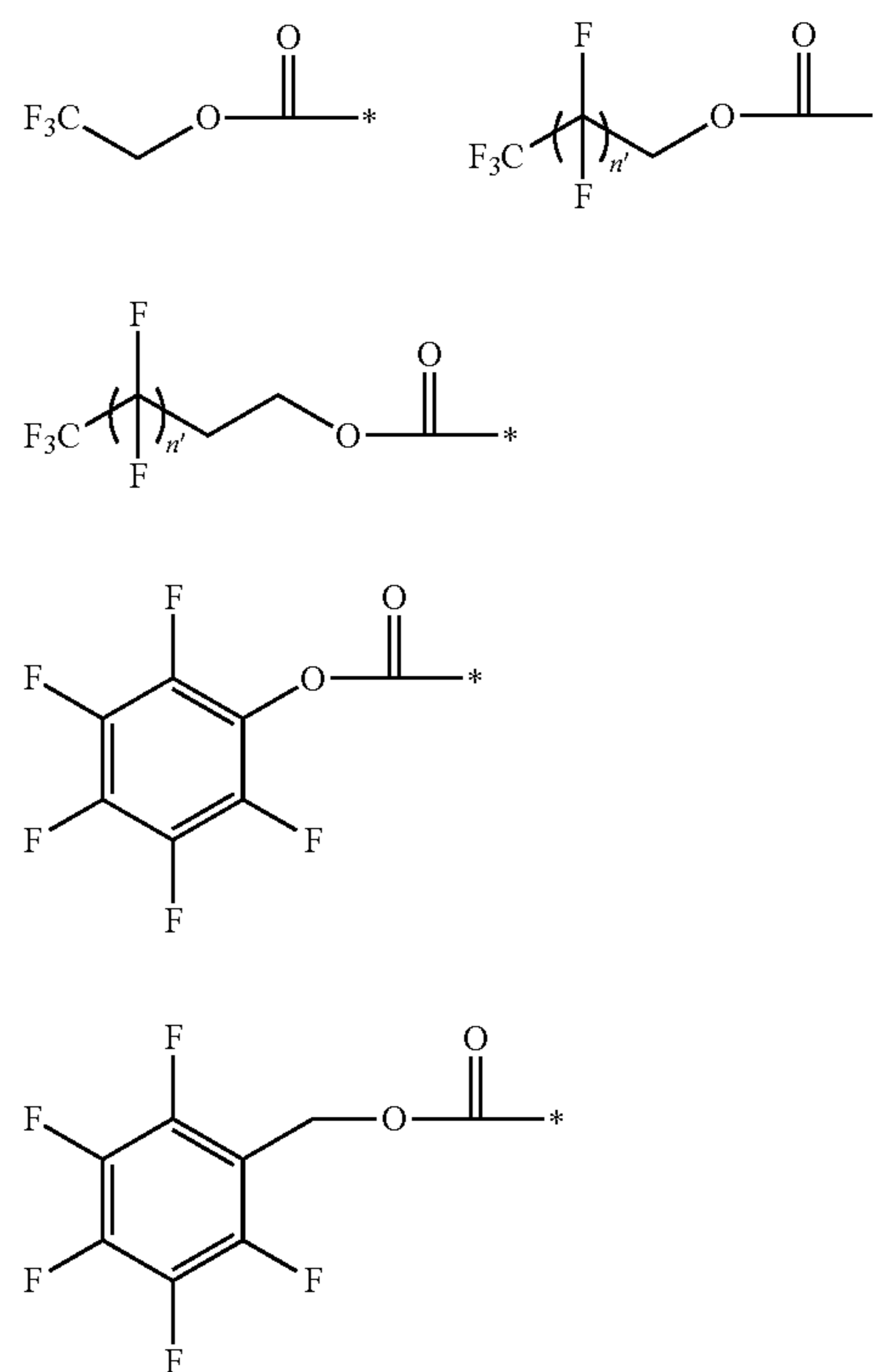
Scheme 8.
