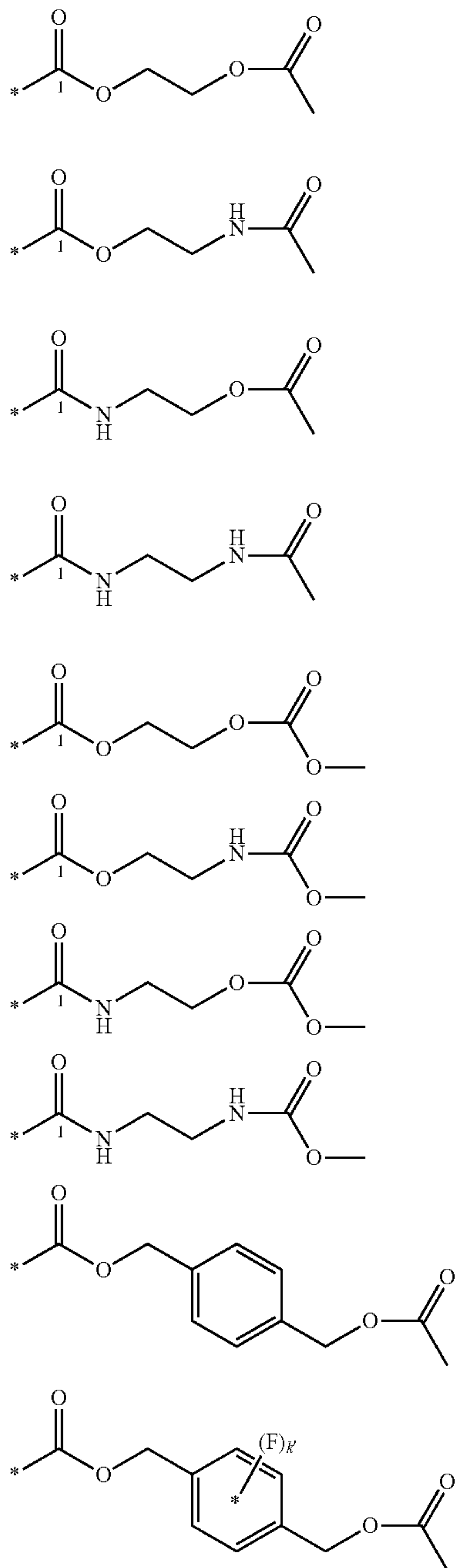
Scheme 11.
