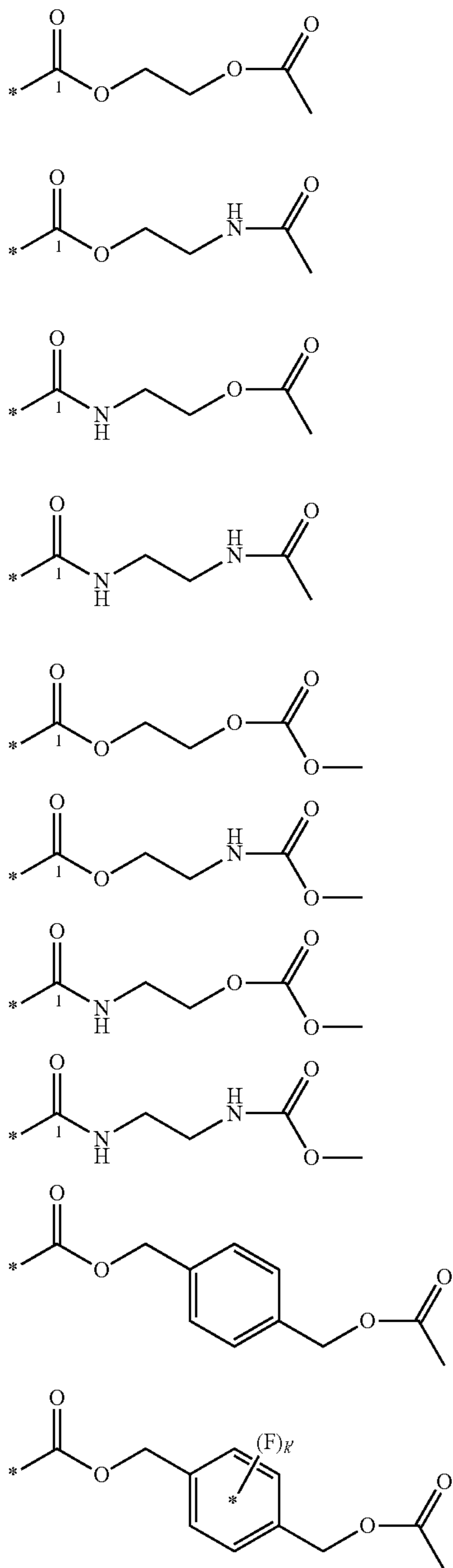
Scheme 11.
