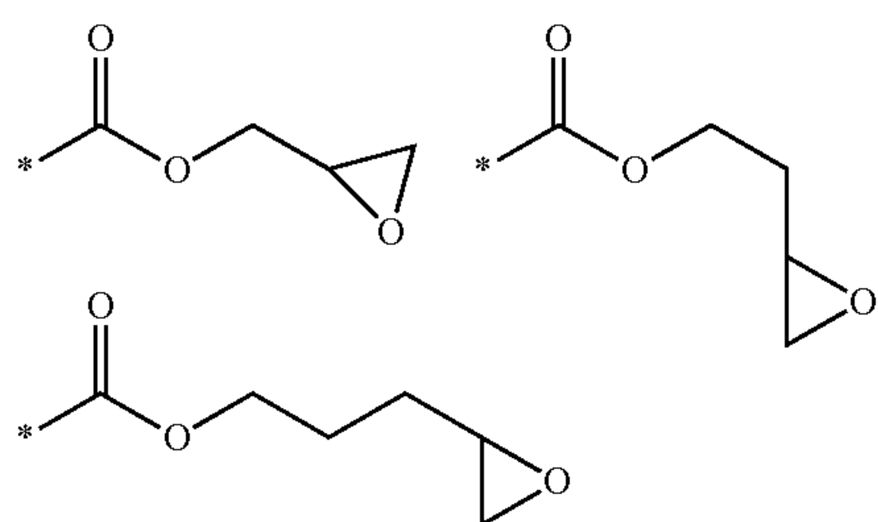
Scheme 15.
