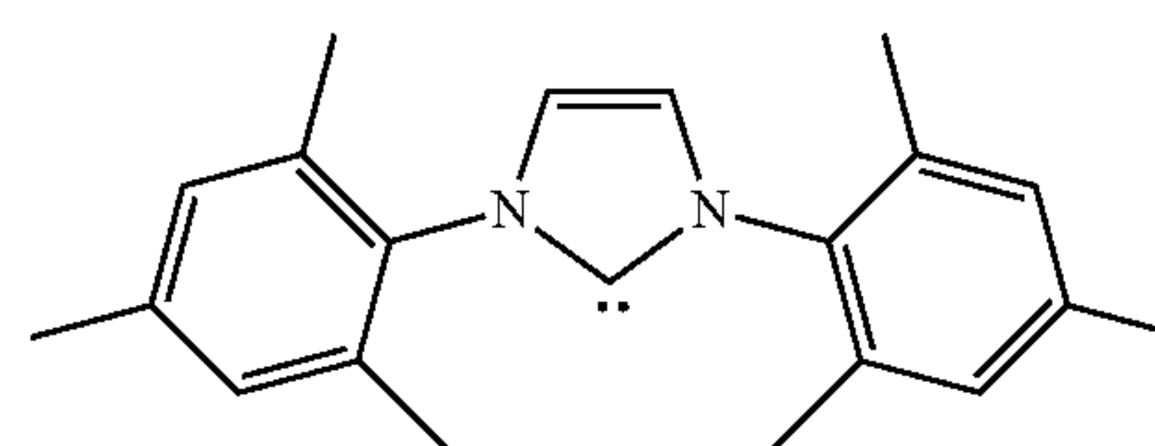
1,3-Bis(2,4,6-trimethylphenyl)imidazol-2-ylidene
