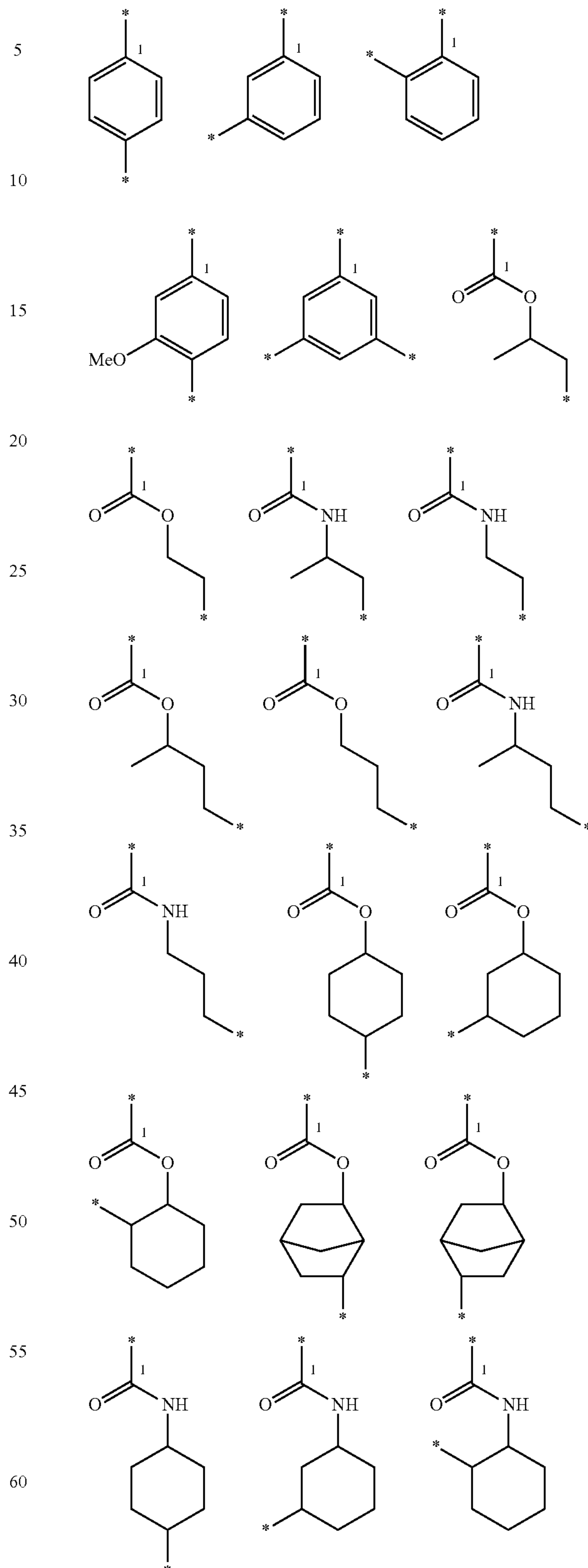
Scheme 5.
