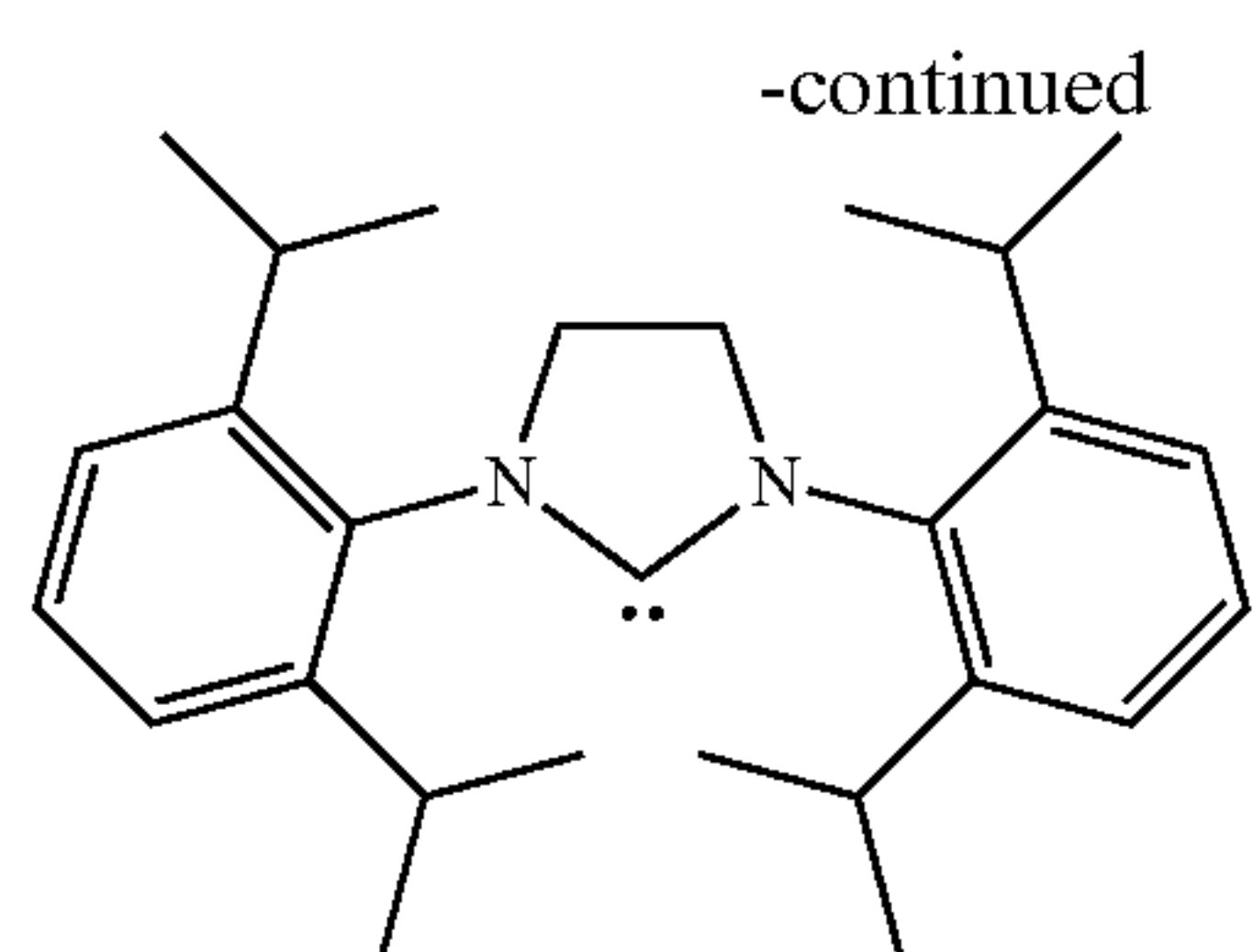
1,3-Bis(2,6-di-i-propylphenyl)-4,5-dihydroimidazol-2-ylidene
