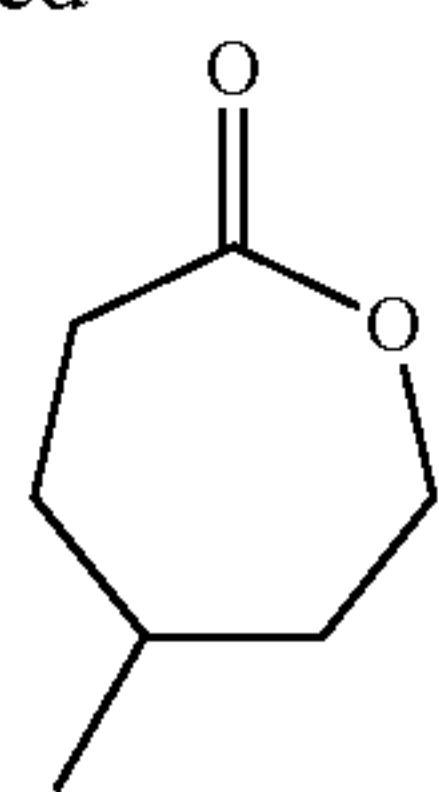
5-Methyloxepan-2-one (MXO)
