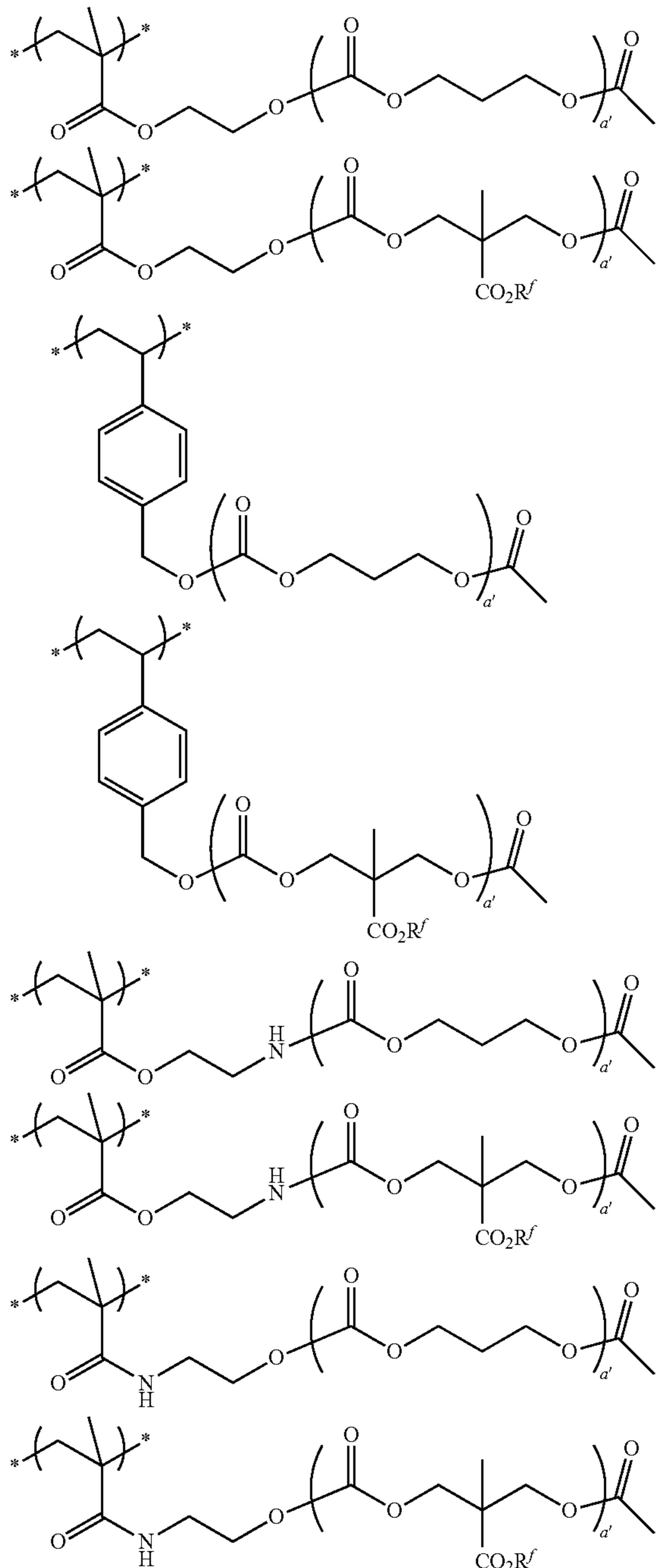
Scheme 13b.
