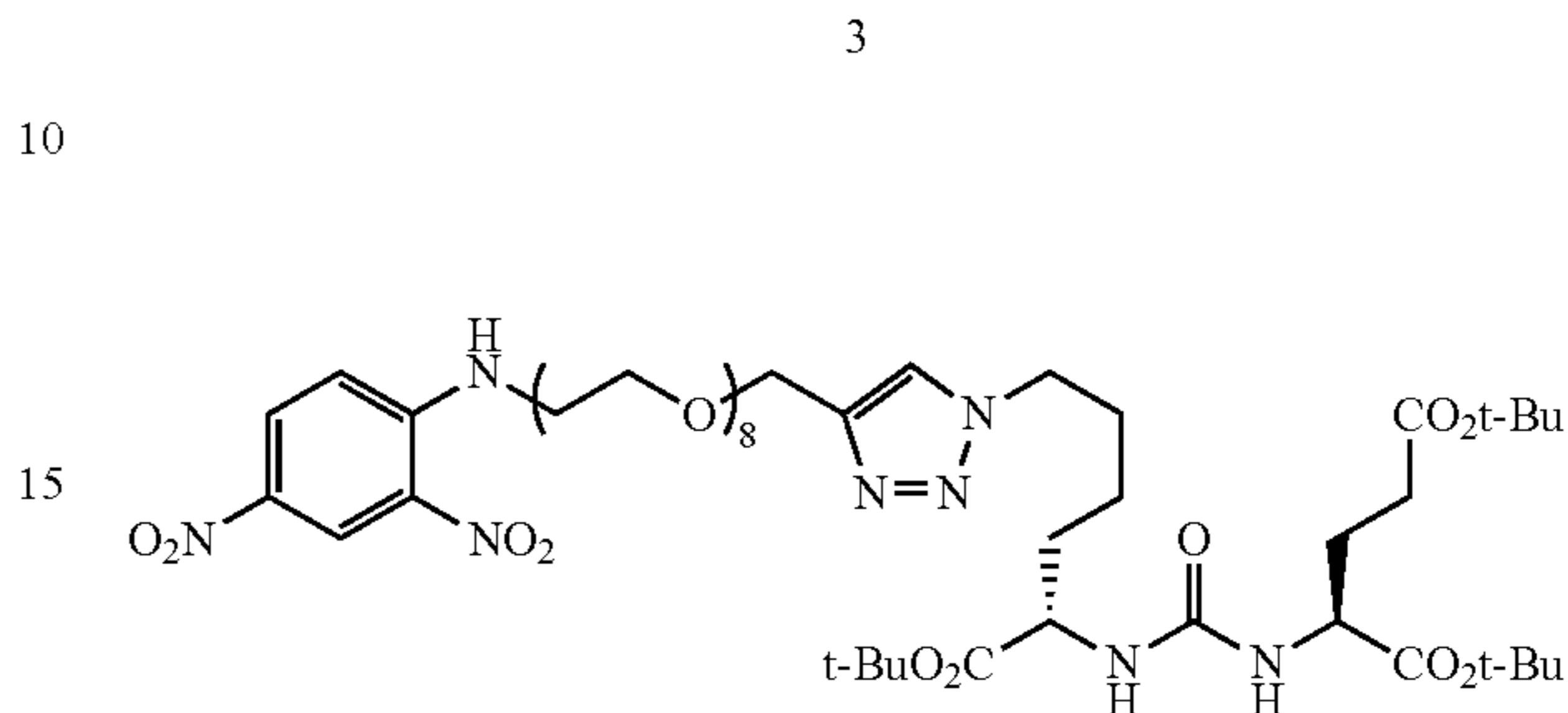
(S)-di-tert-butyl 2-(3-((S)-1-tert-butoxy-6-(4-(13-(2,4-dinitrophenylamino)-2,5,8,11-tetraoxatridecyl)-1H-1,2,3-triazol-1-yl)-1-oxohexan-2-yl)ureido)pentanedioate (3)
