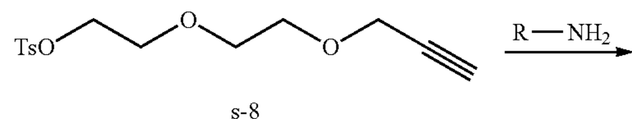
Scheme S-3: General synthesis of (PEG) 2 -alkynes.
