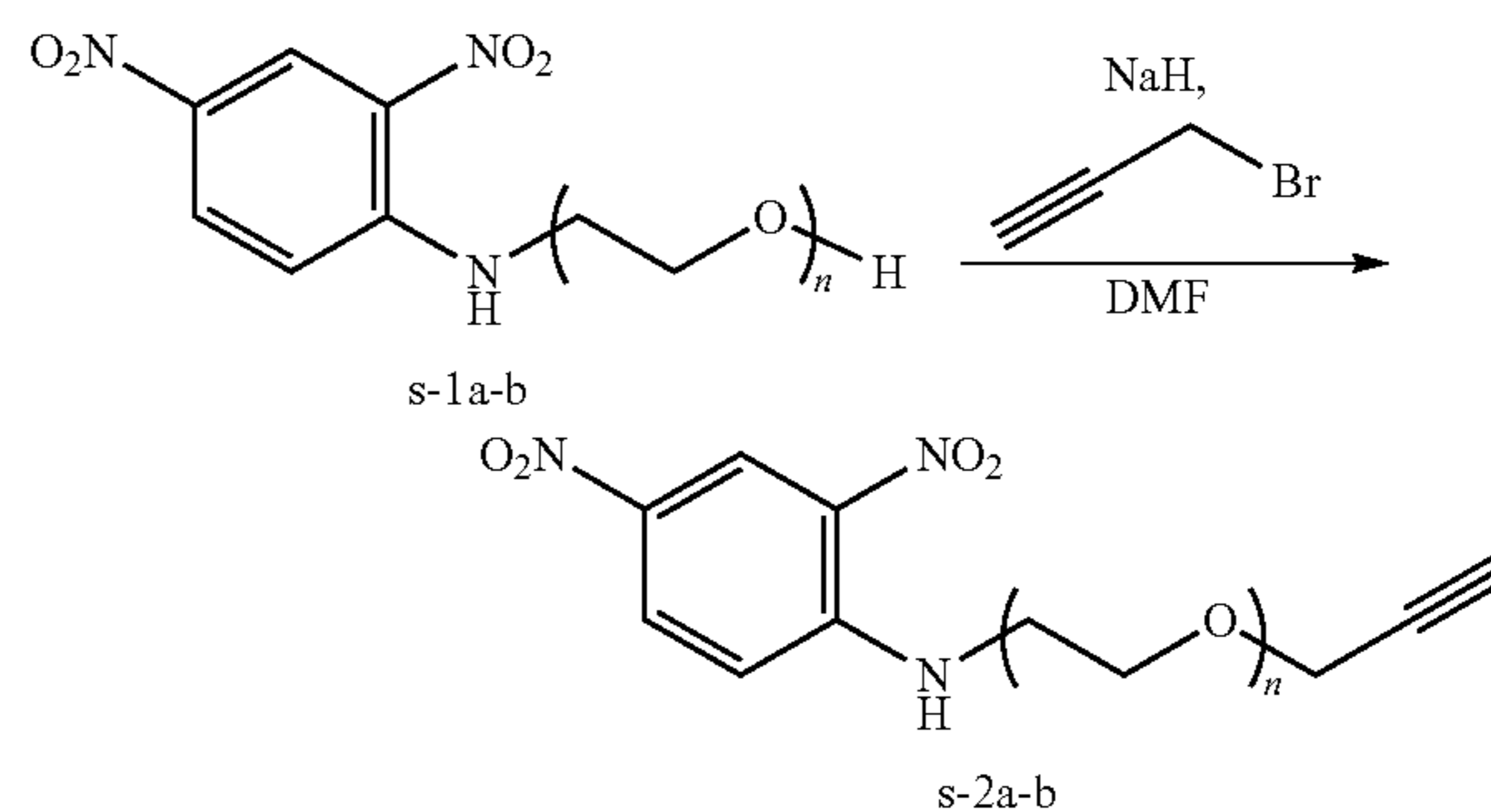
Scheme S-1. General synthesis of DNP-PEG-alkynes from the corresponding DNP-PEG-OH. (a, n = 1; b, n = 2).
