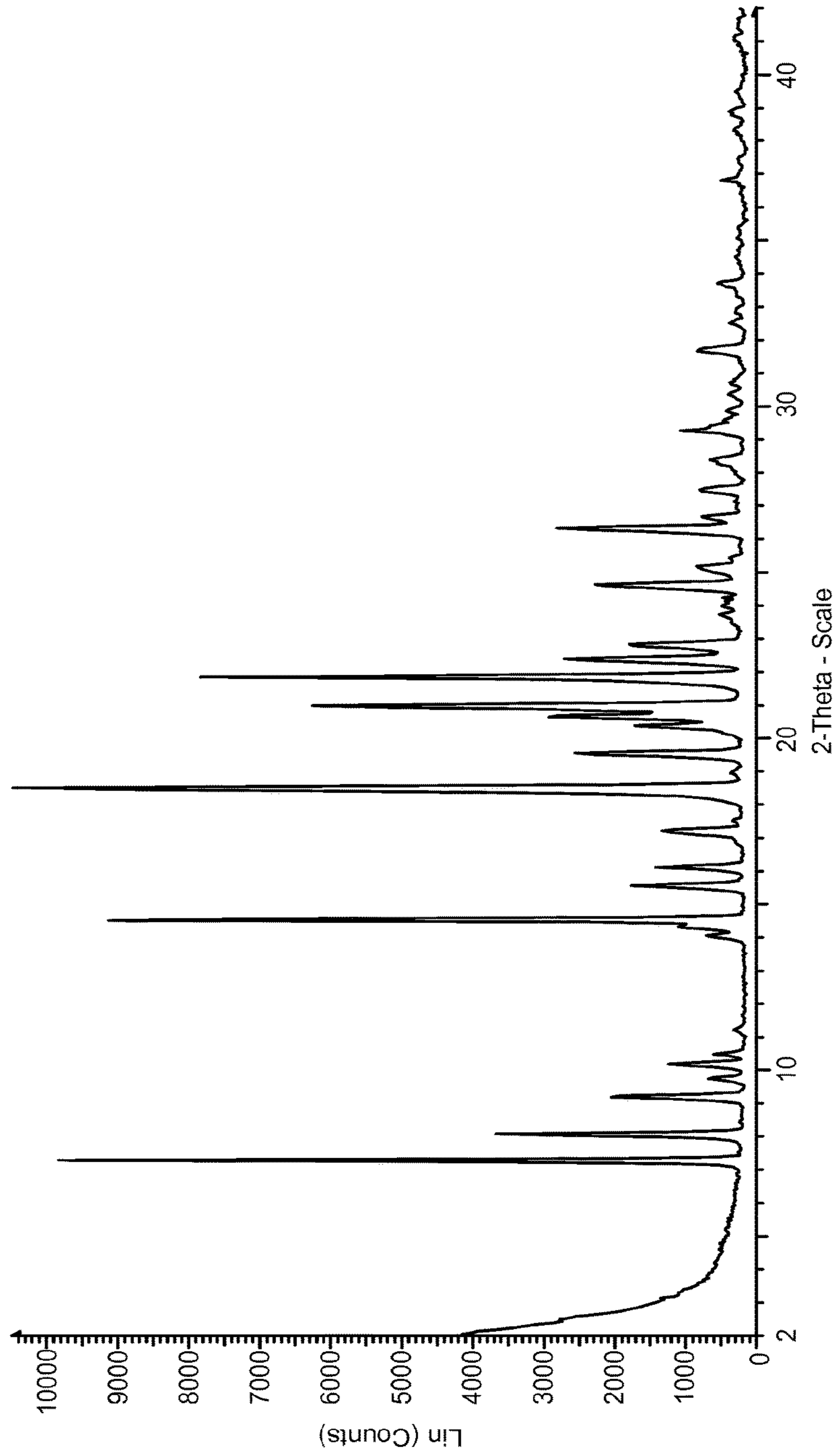
FIG. 12 XRPD Pattern of Form D
