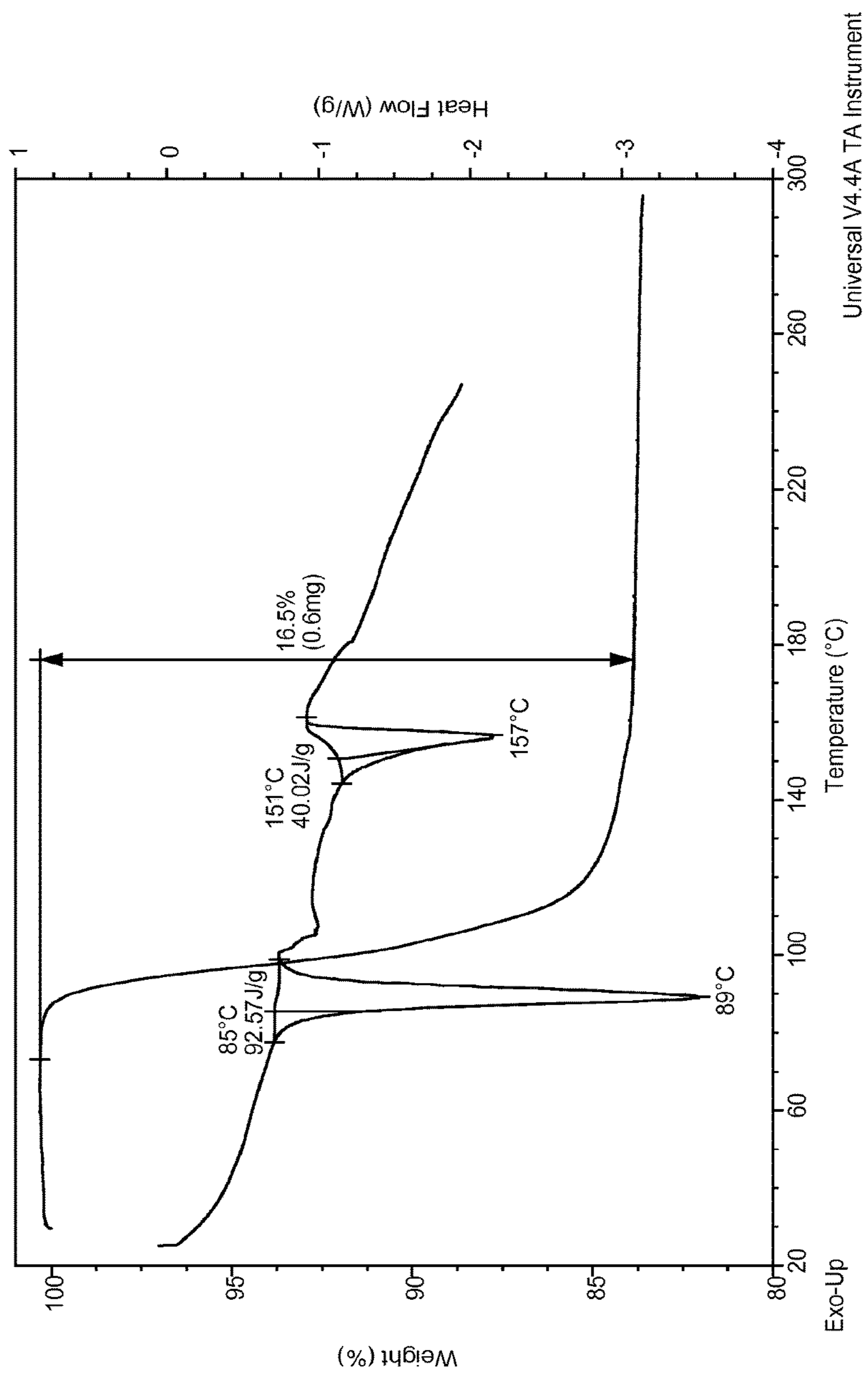
FIG. 15 TGA/DSC Thermograms of Form E
