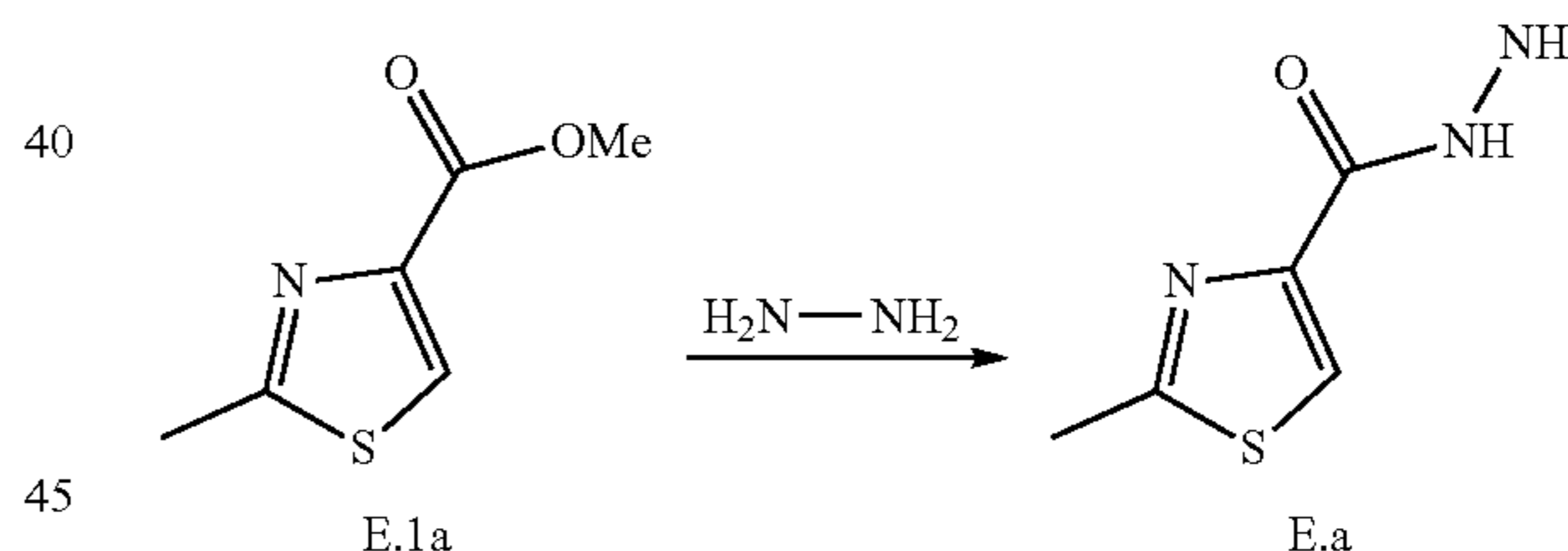
Scheme 31: Synthesis of 2-methylthiazole-4-carbohydrazide E.a
