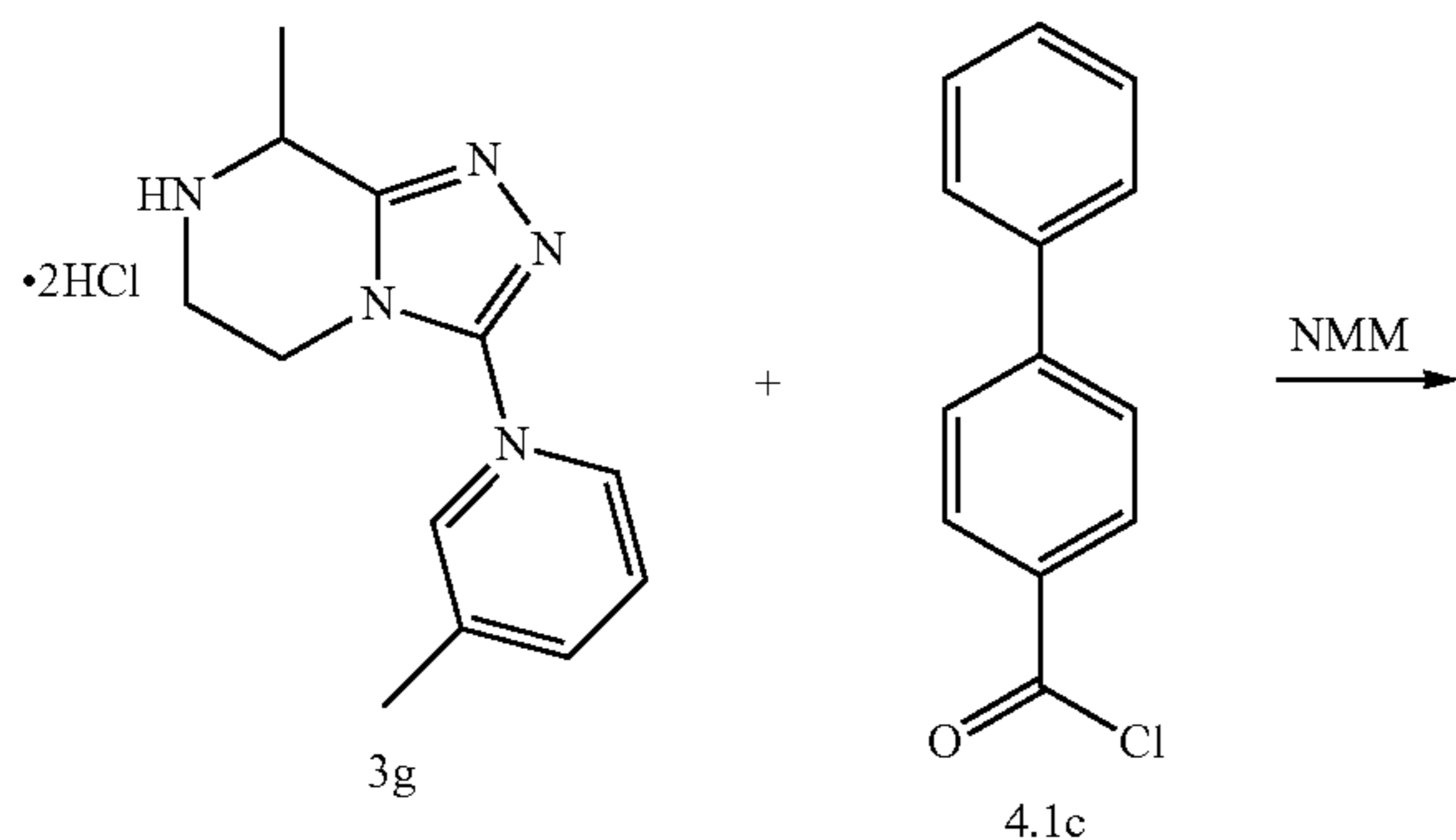
Scheme 28: Synthesis of compounds 4c and n° 29
