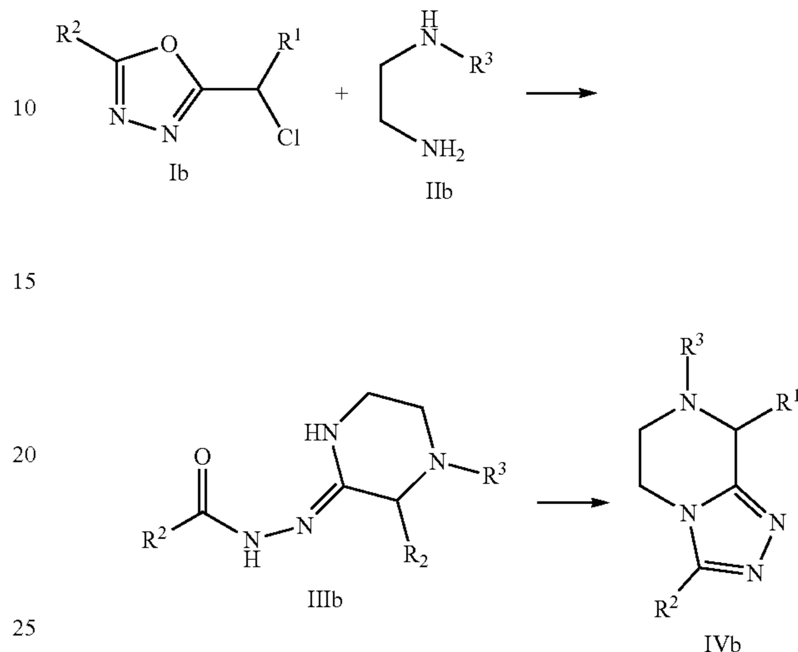
Scheme C: Method B
