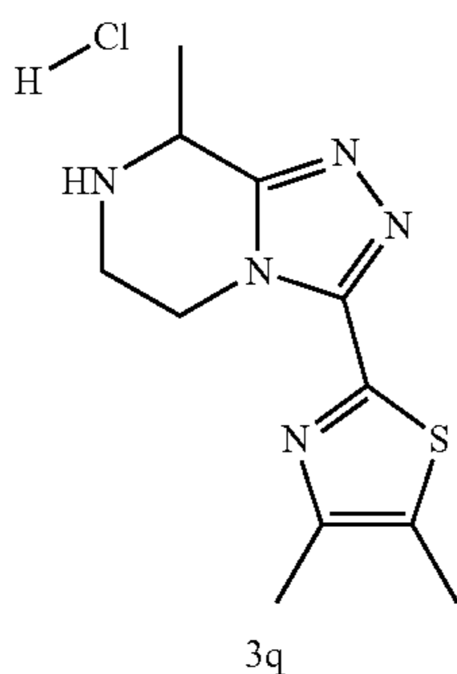
Scheme 23: Cyclodeshydration leading to triazolopiperazine 3
