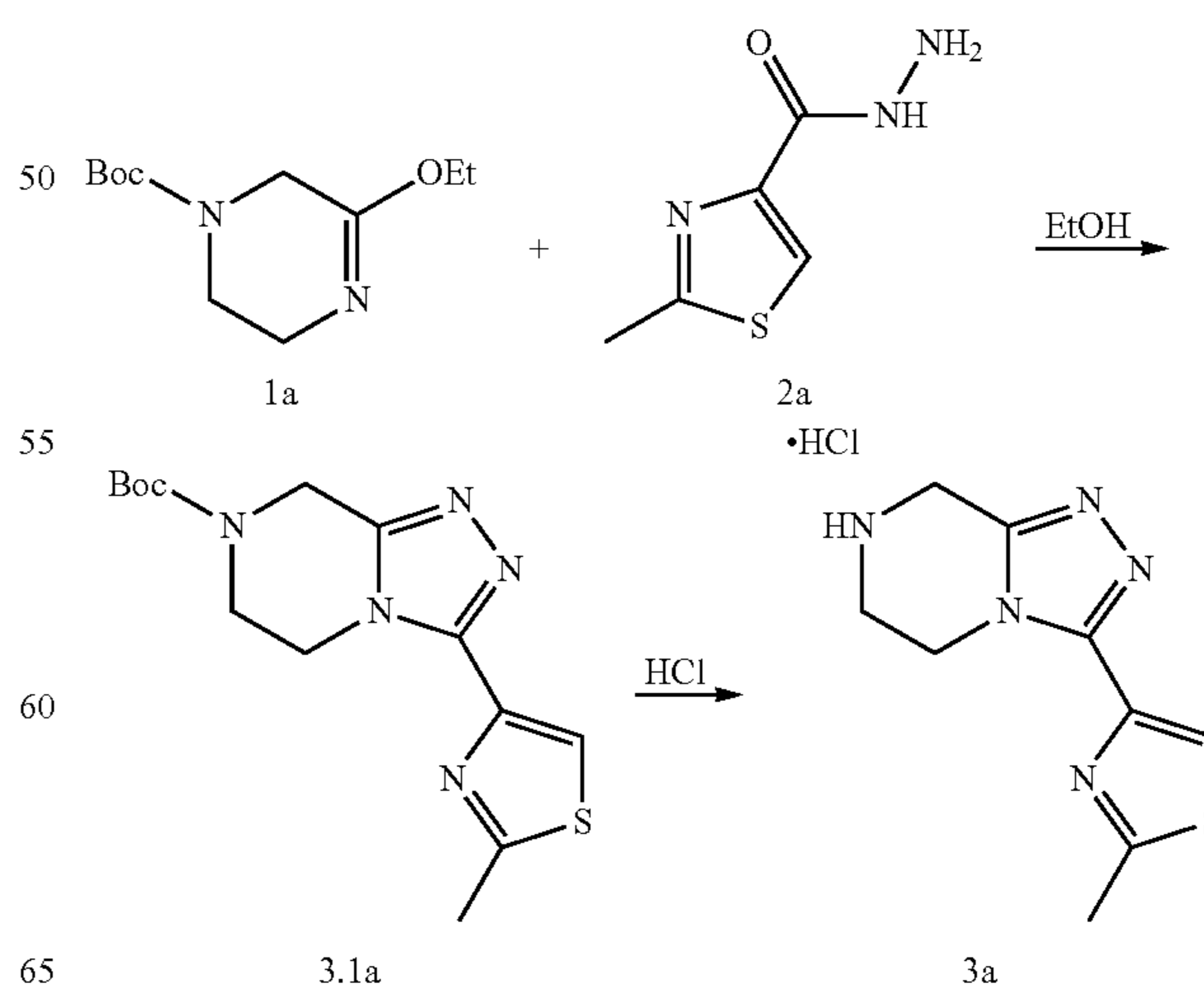
Scheme 17: Synthesis of 2-methyl-4-(5,6,7,8-tetrahydro-[1,2,4]triazolo[4,3-a]pyrazin-3-yl)thiazole hydrochloride 3a
