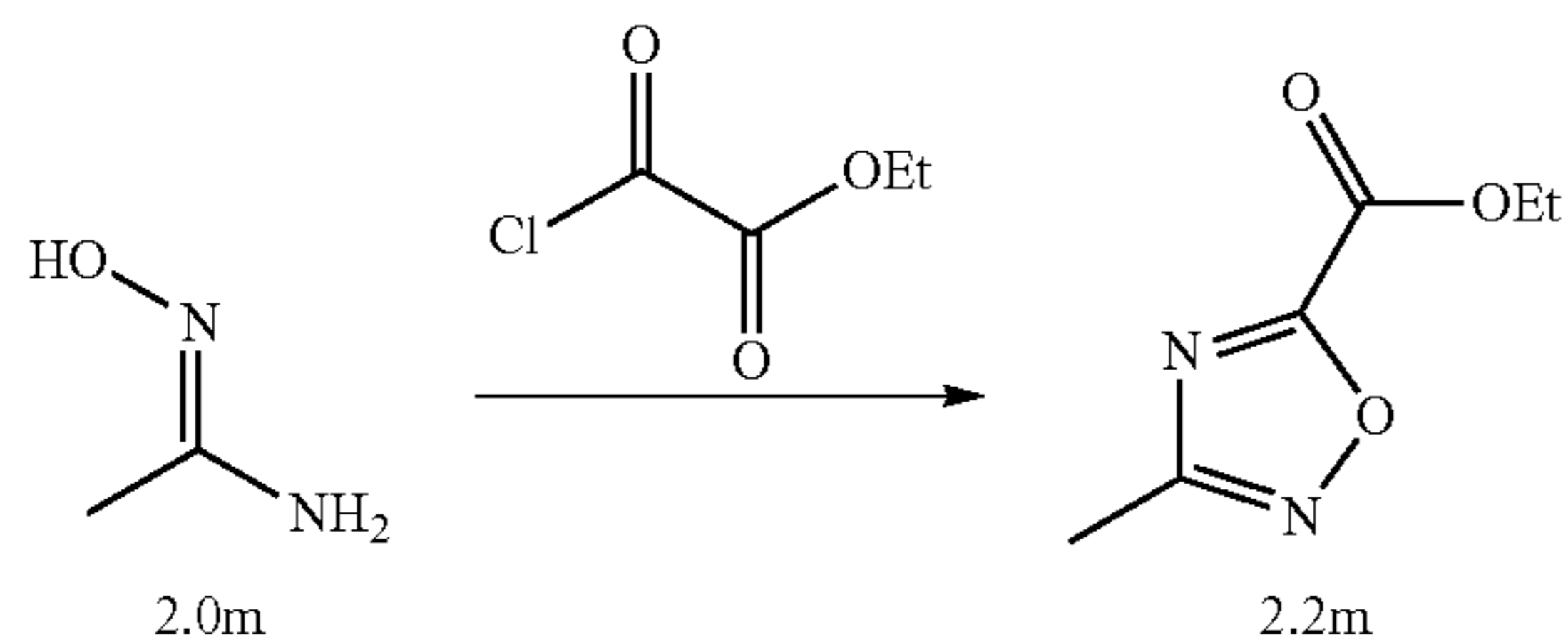
Scheme 11: Synthesis of ethyl 3-methyl-1,2,4-oxadiazole-5-carboxylate 2.2m
