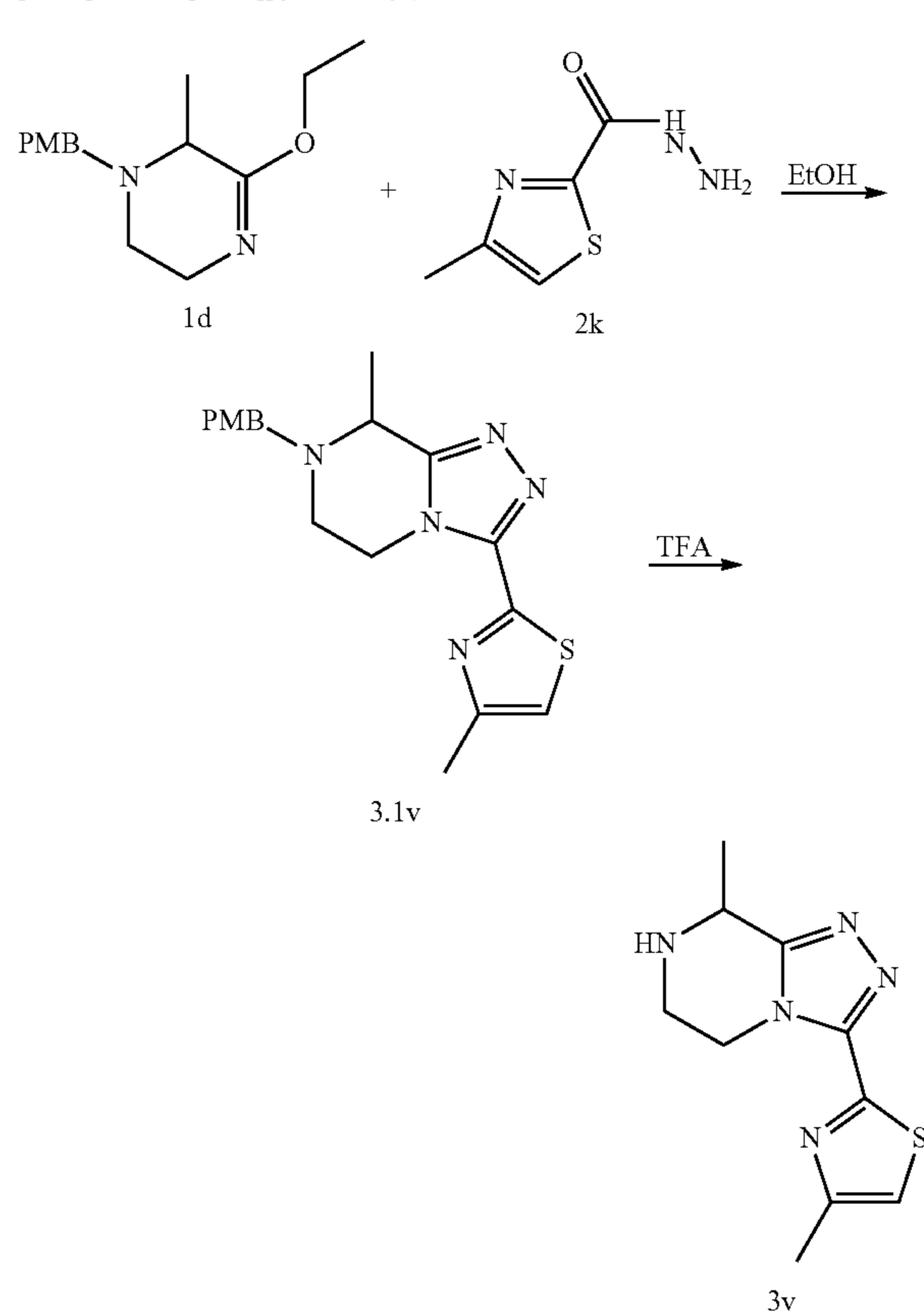
Scheme 24: Synthesis of 4-methyl-2-(8-methyl-5,6,7,8-tetrahydro-[1,2,4]triazolo[4,3-a]pyrazin-3-yl)thiazole 3v
