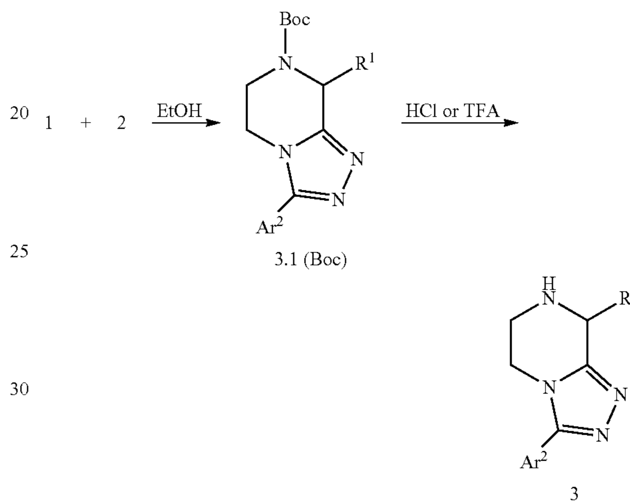
Scheme 16: Cyclodehydration leading to triazolopiperazine 3
