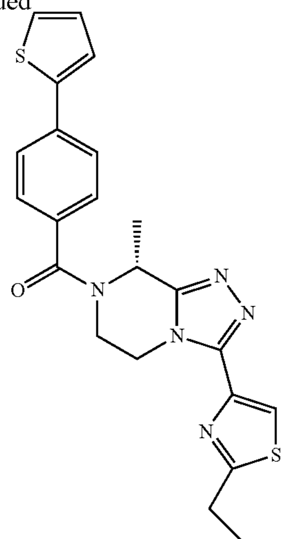
compound n° 5
