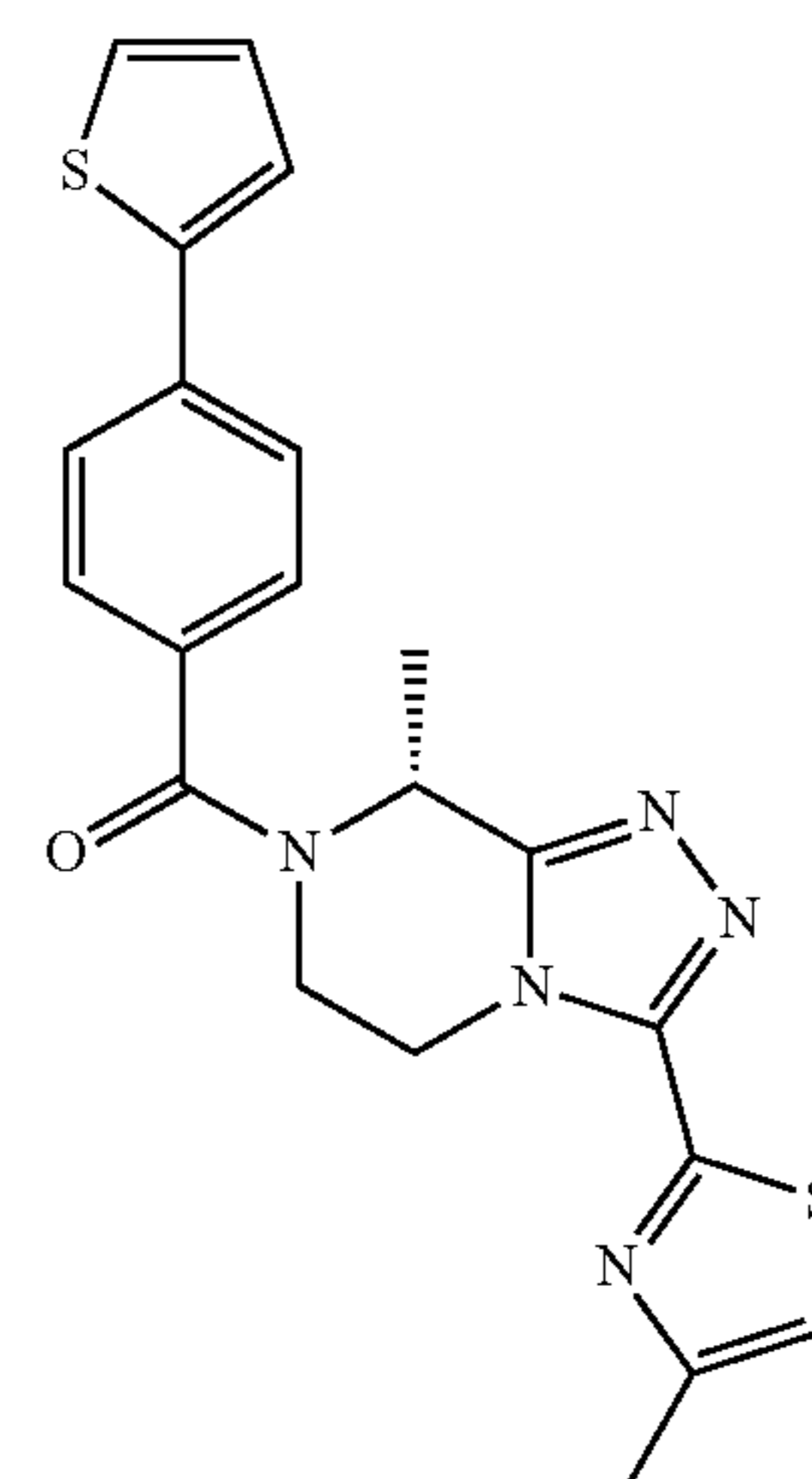
compound n° 19
