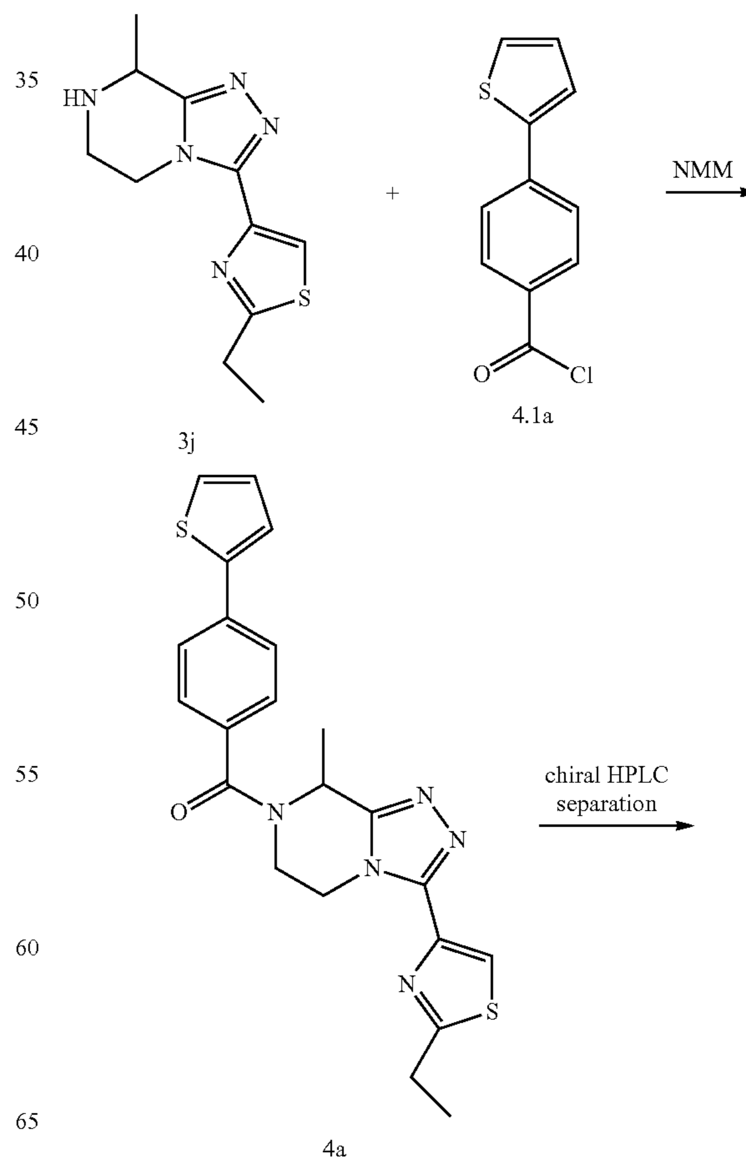
Scheme 26: Synthesis of compounds 4a and n° 5
