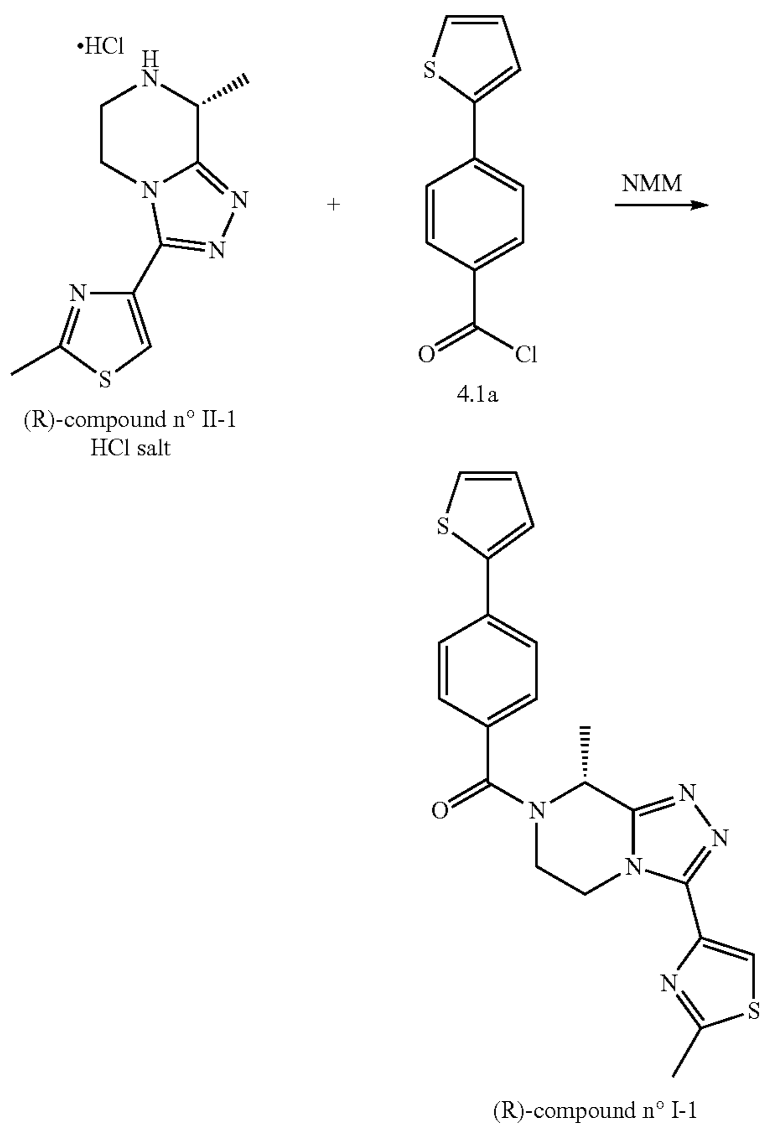
Scheme 34: Synthesis of (R)-I-1
