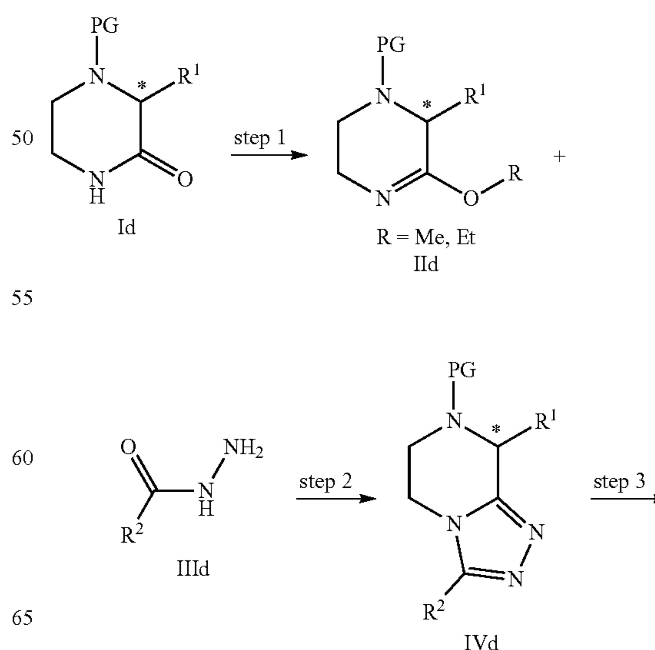
Scheme D: Method C
