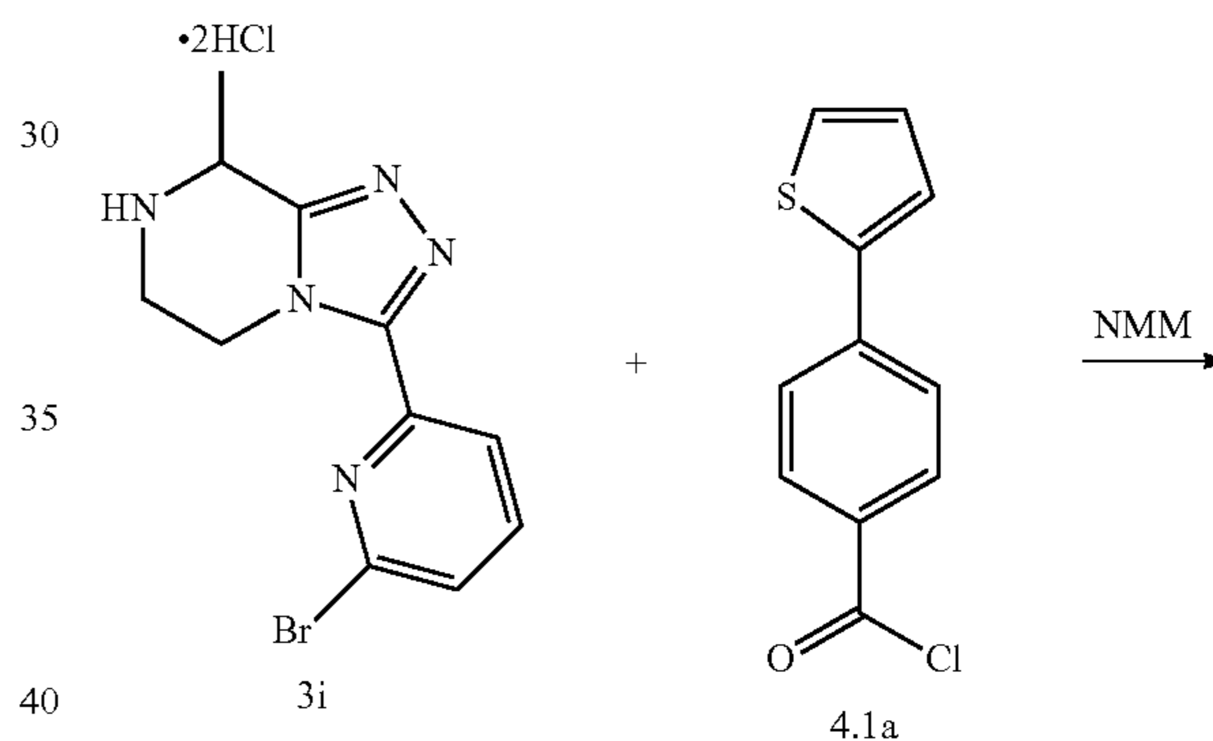
Scheme 29: Synthesis of compound n° 33.
