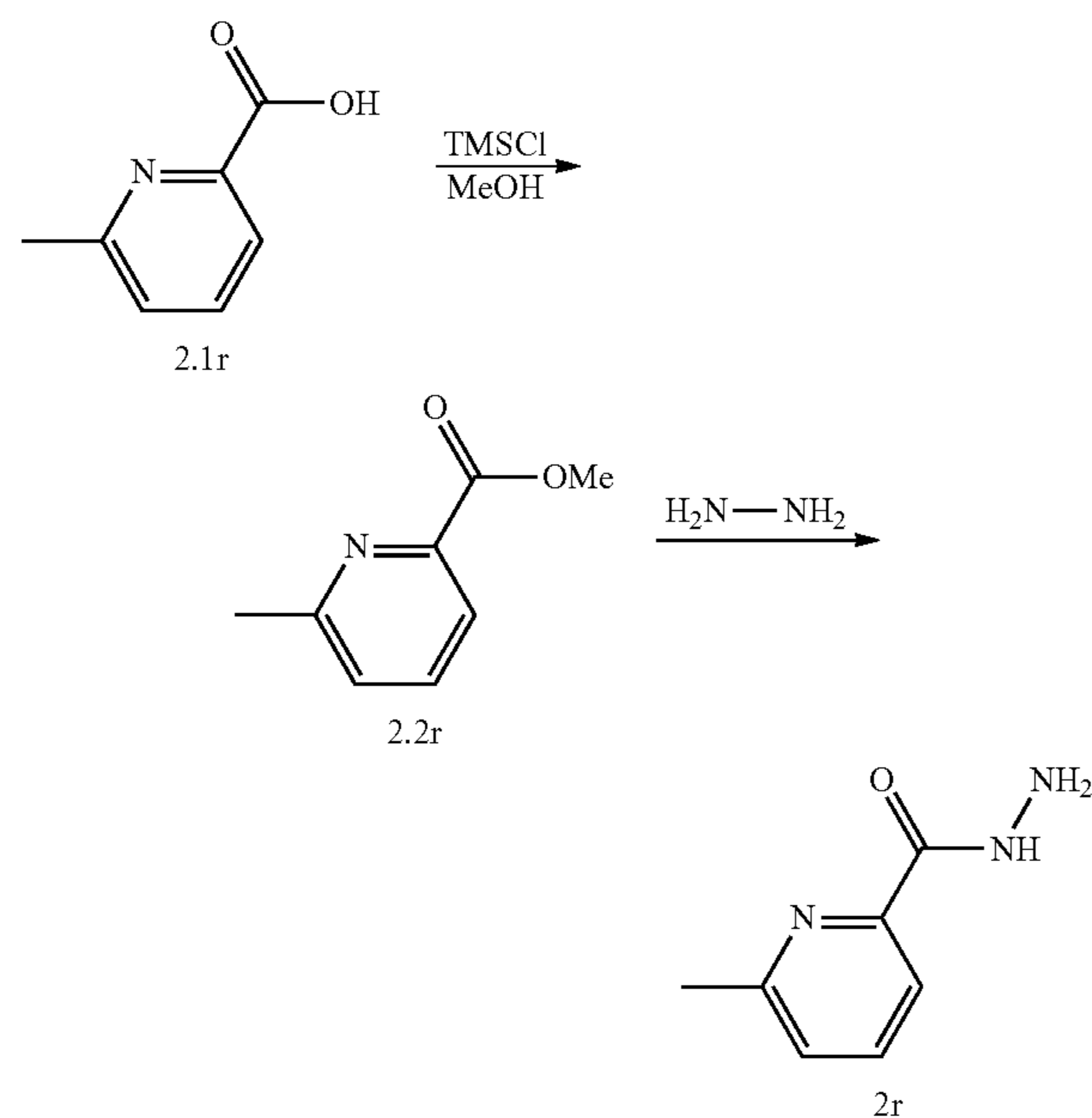
Scheme 15: Synthesis of 6-methylpicolinohydrazide 2r.
