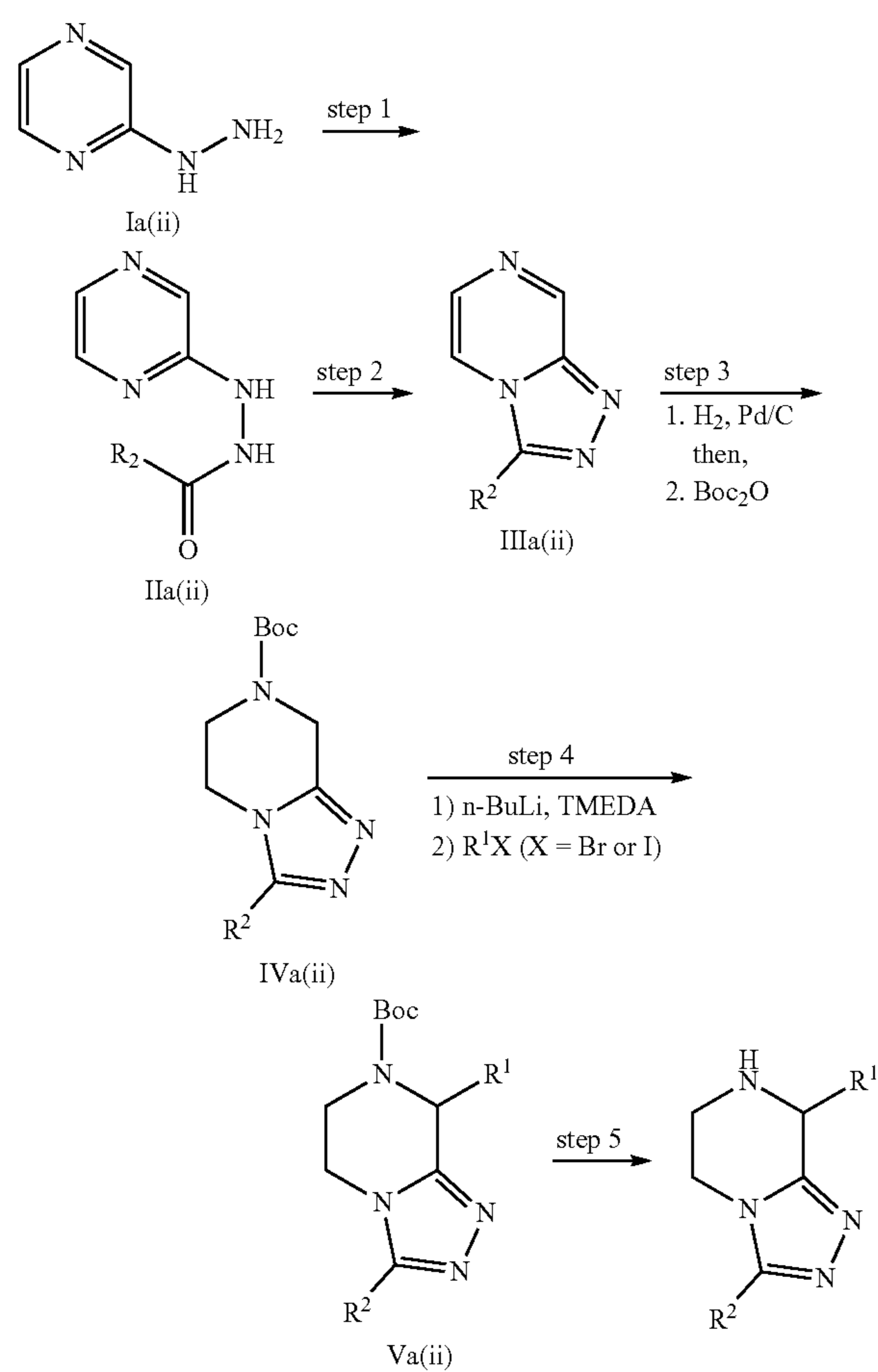
Scheme B: Method A(ii)
