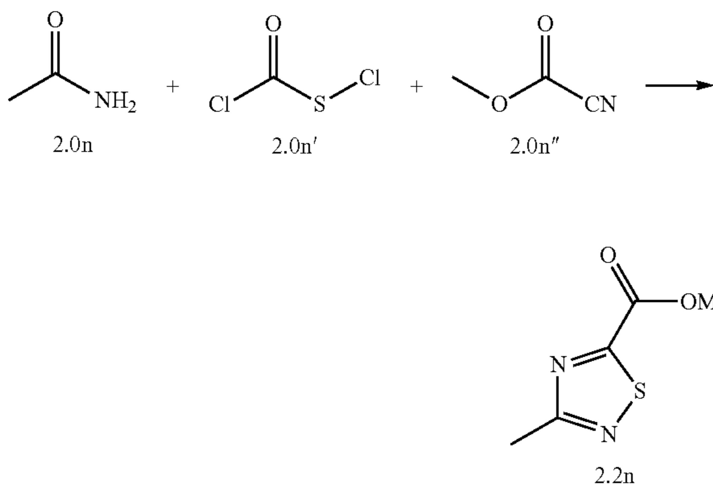
Scheme 12: Synthesis of methyl 3-methyl-1,2,4-thiadiazole-5-carboxylate 2.2n
