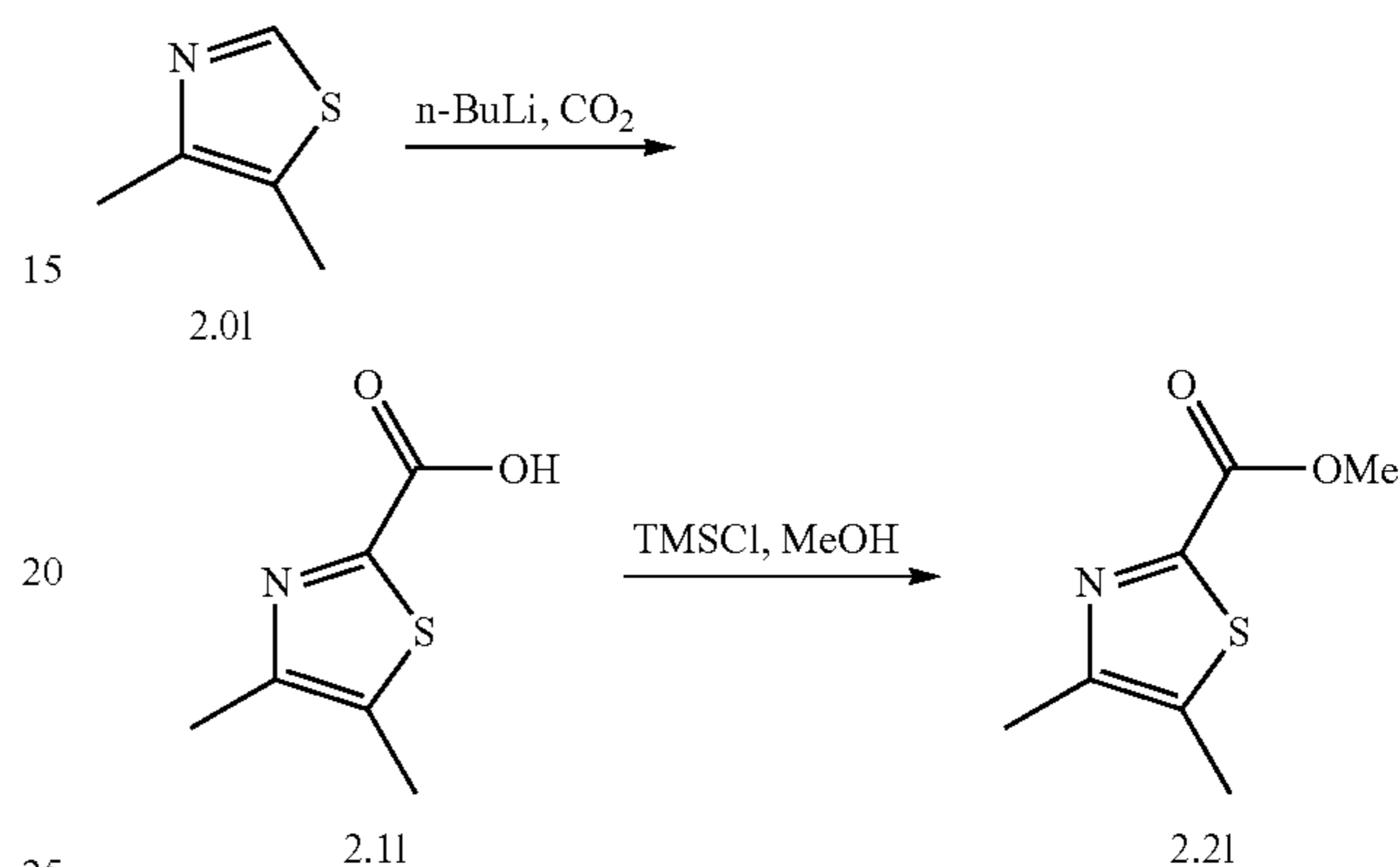
Scheme 10: Synthesis of methyl 4,5-dimethylthiazole-2-carboxylate 2.2l
