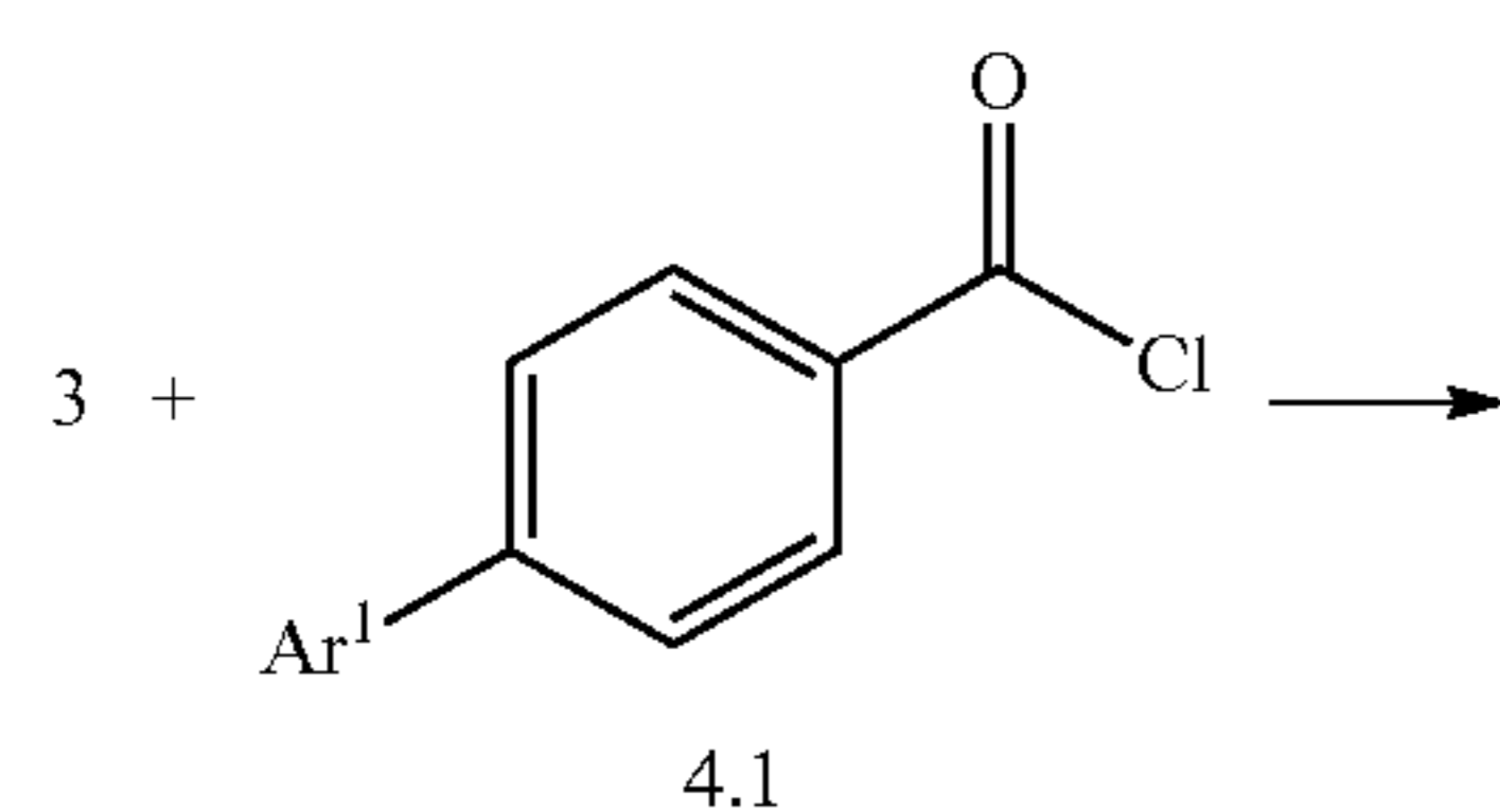
Scheme 25: Acylation and chiral HPLC purification
