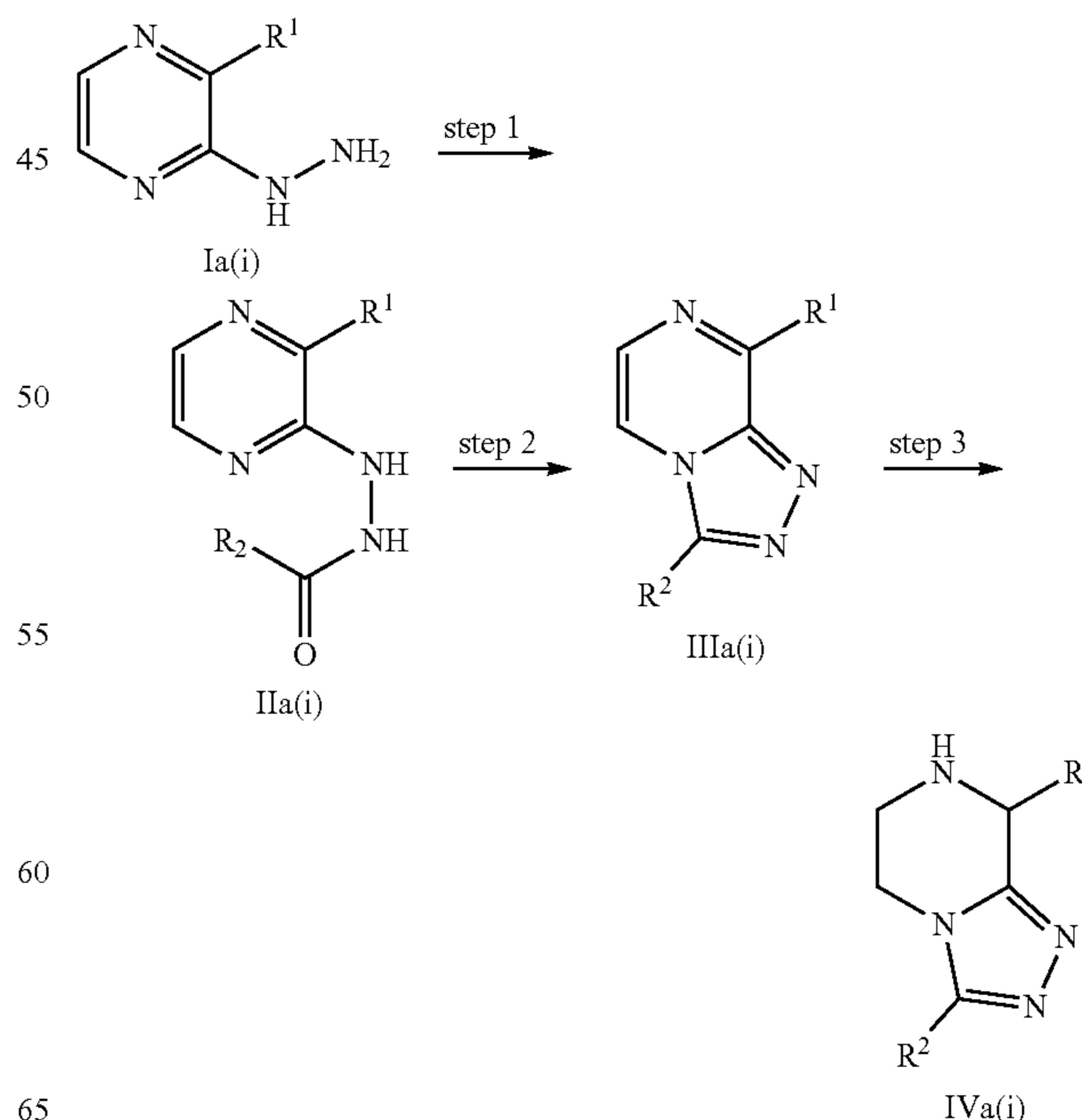
Scheme A: Method A(i)
