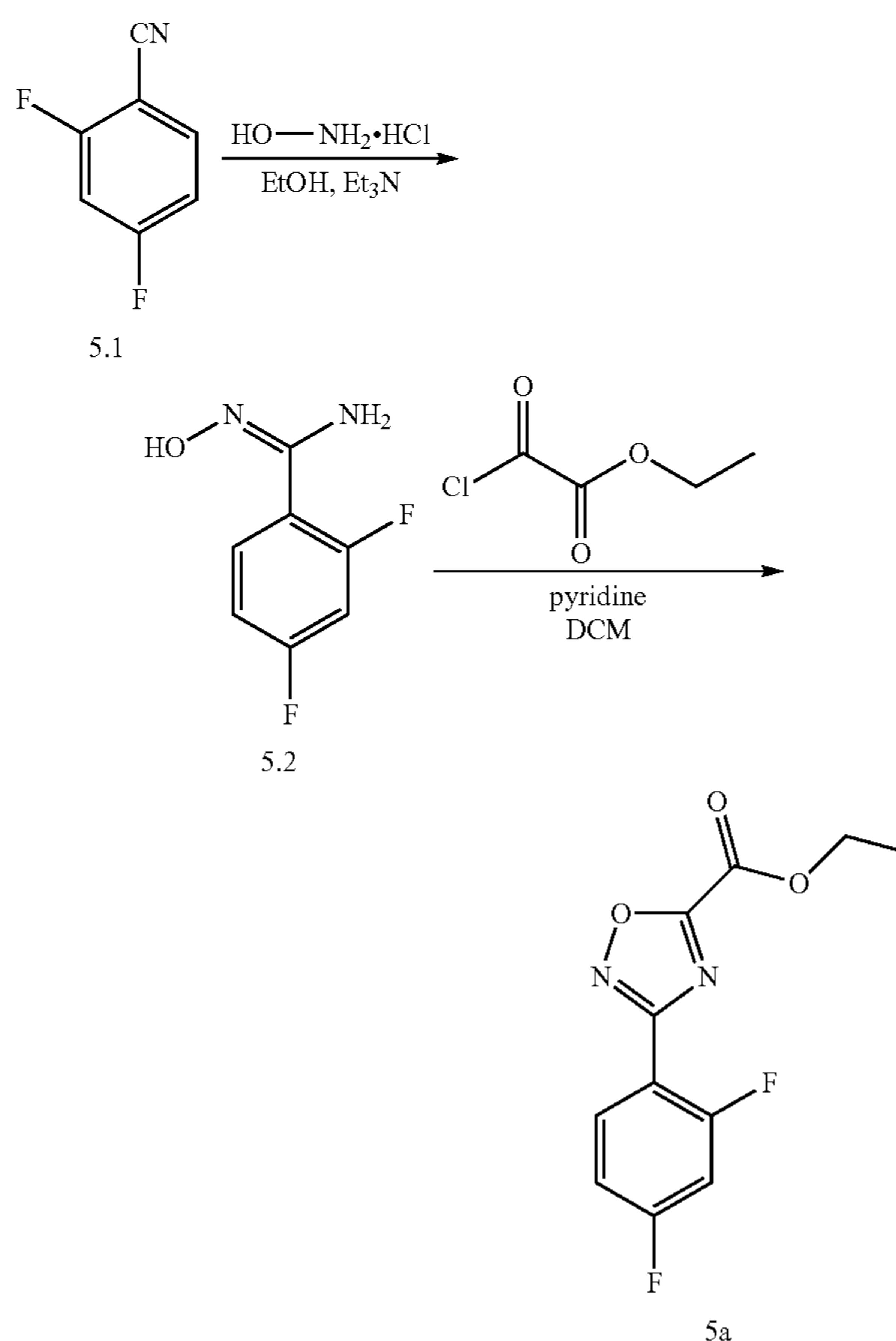
Scheme 6: synthesis of intermediate 5a
