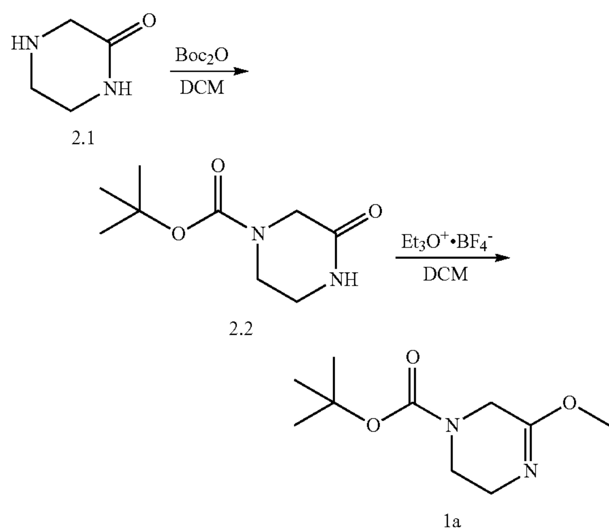
Scheme 2: Synthesis of tert-butyl 3-ethoxy-5,6-dihydropyrazine-1(2H)-carboxylate
