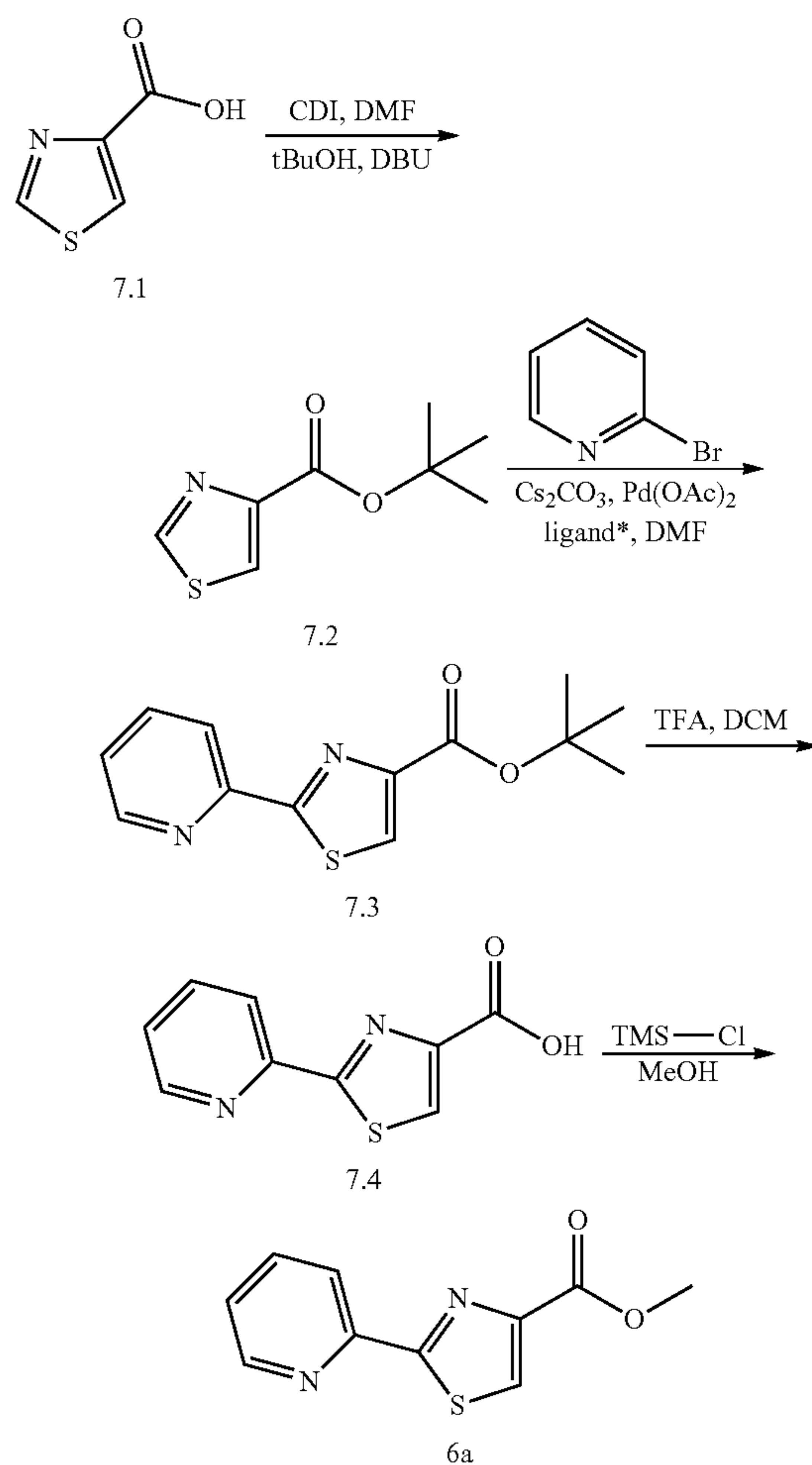
Scheme 7: Synthesis of intermediate 6a
