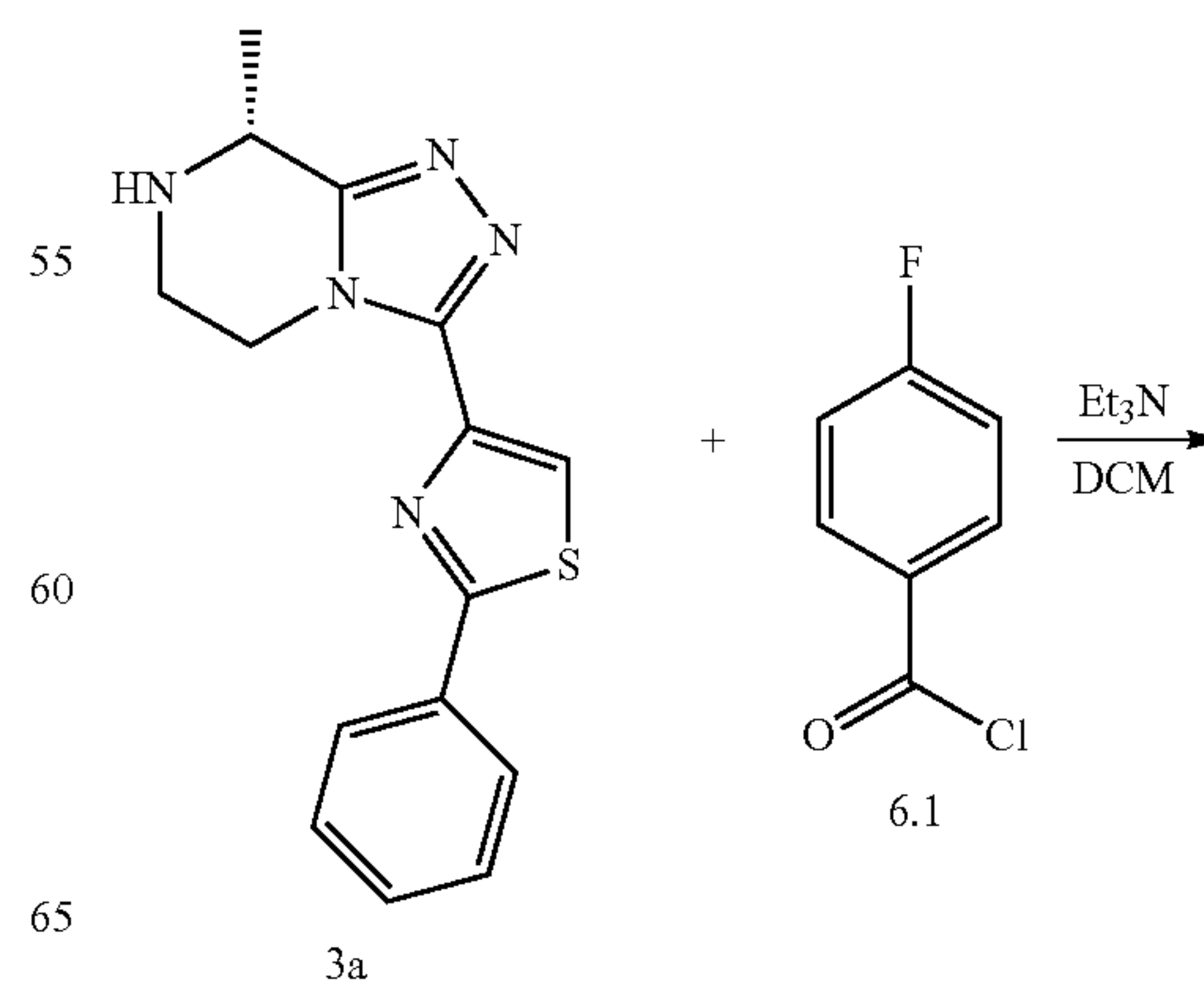
Scheme 12: synthesis of (R)-(4-fluorophenyl)(8-methyl-3-(2-phenylthiazol-4-yl)-5,6-dihydro-[1,2,4]triazolo[4,3-a]pyrazin-7(8H)-yl)methanone (compound n° 45).
