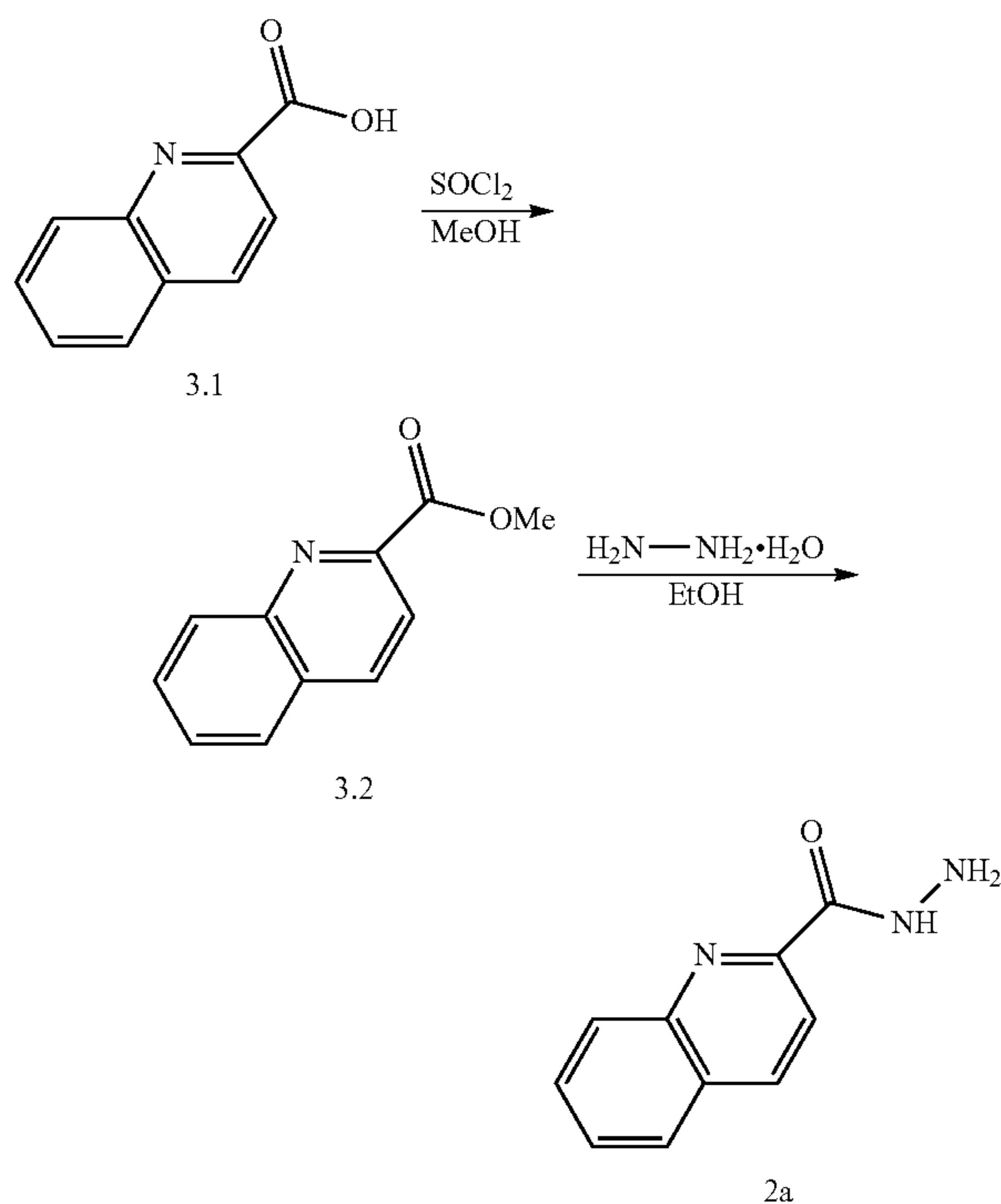
Scheme 3: Synthesis of quinoline-2-carbohydrazide 2a
