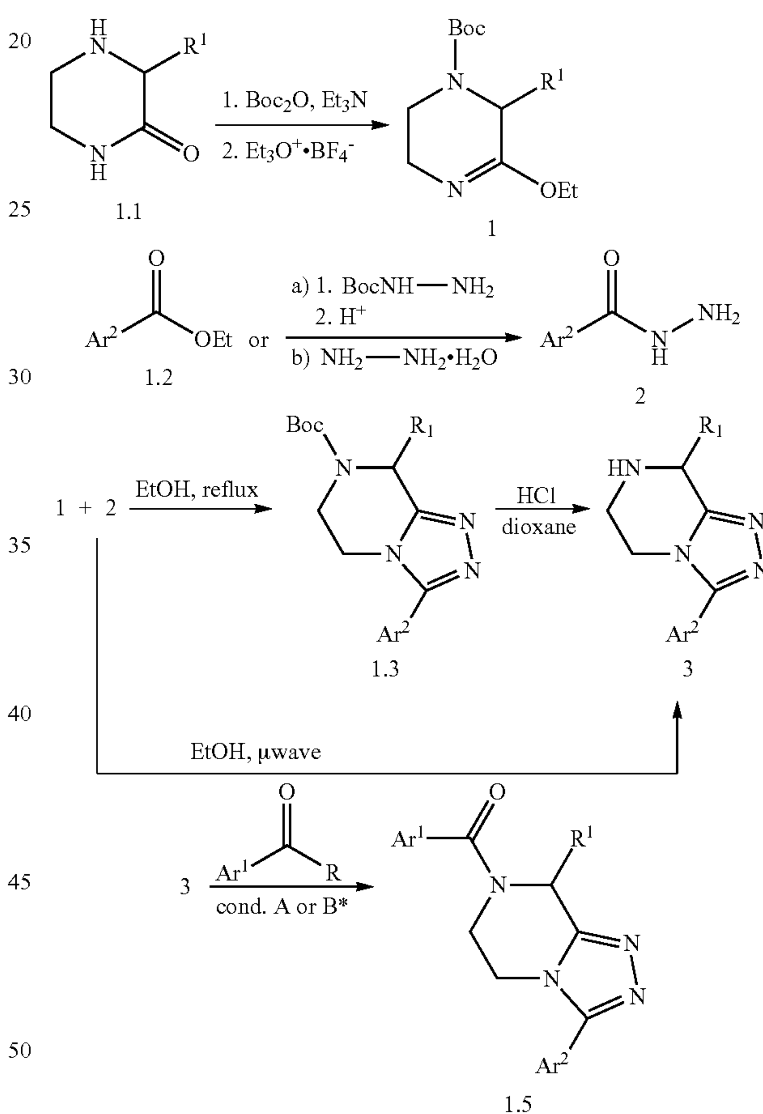
Scheme 1: General synthetic scheme for the preparation of the majority of compounds in the present invention
