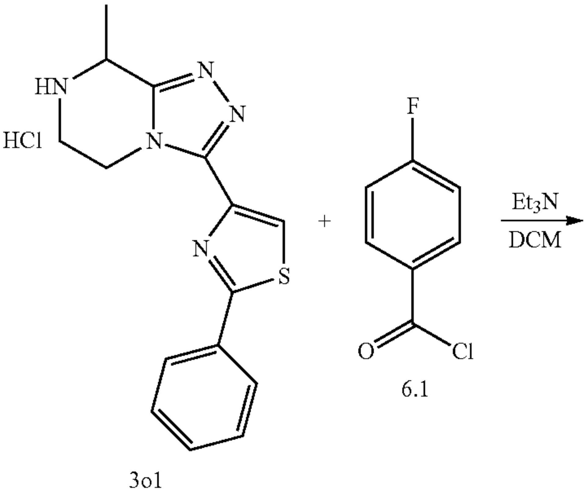
Scheme 13: synthesis of (4-fluorophenyl)(8-methyl-3-(2-phenylthiazol- 4-yl)-5,6-dihydro-[1,2,4]triazolo[4,3-a]pyrazin-7(8H)-yl)methanone (compound n° 166).
