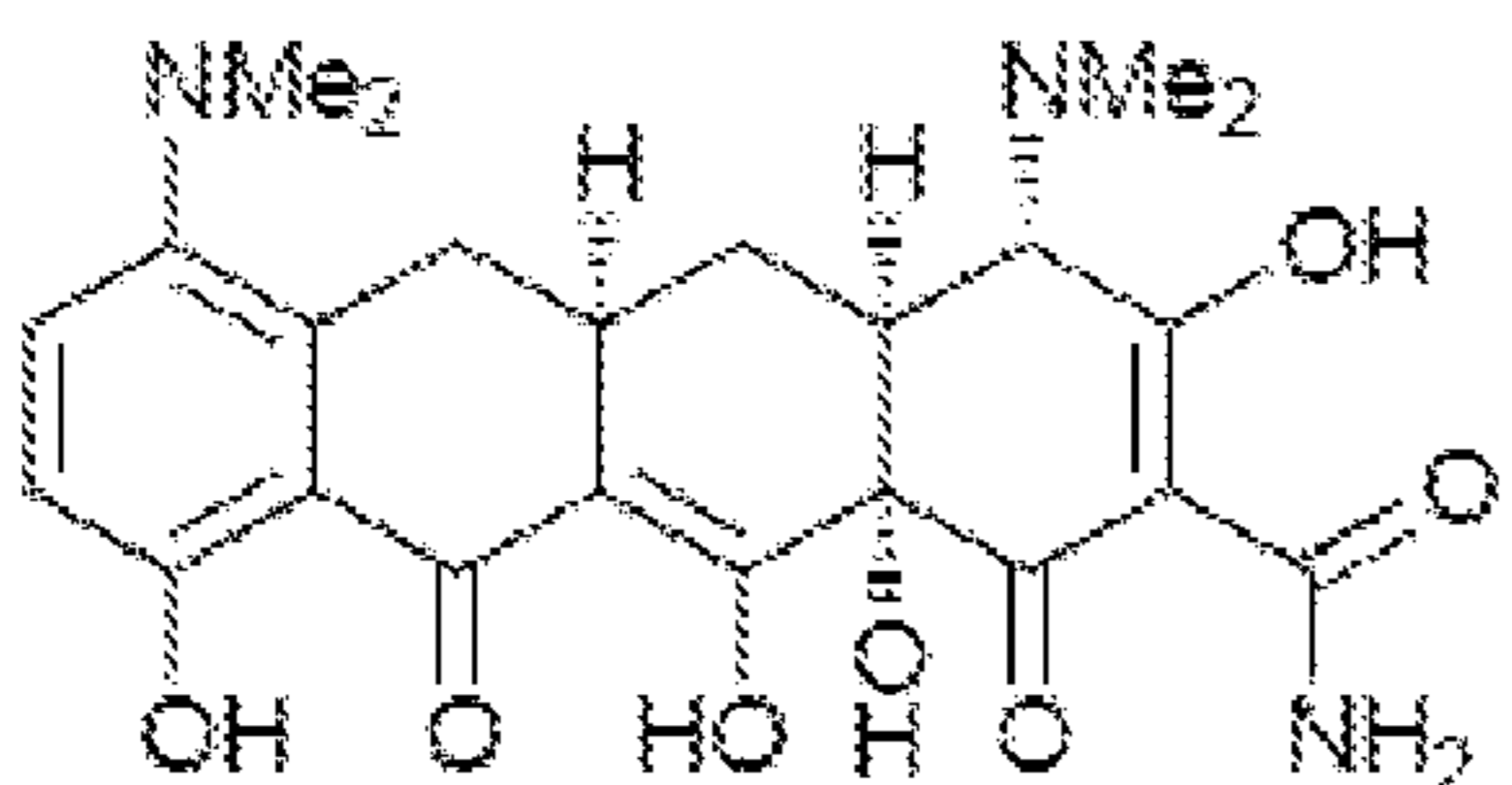
7: minocycline (Minocin®)
