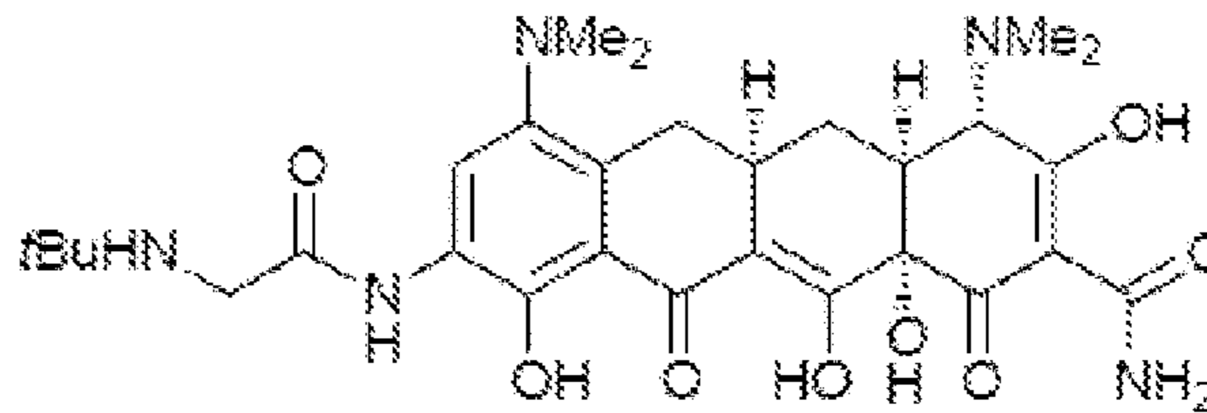
9: tigecycline (Tygacil®)
