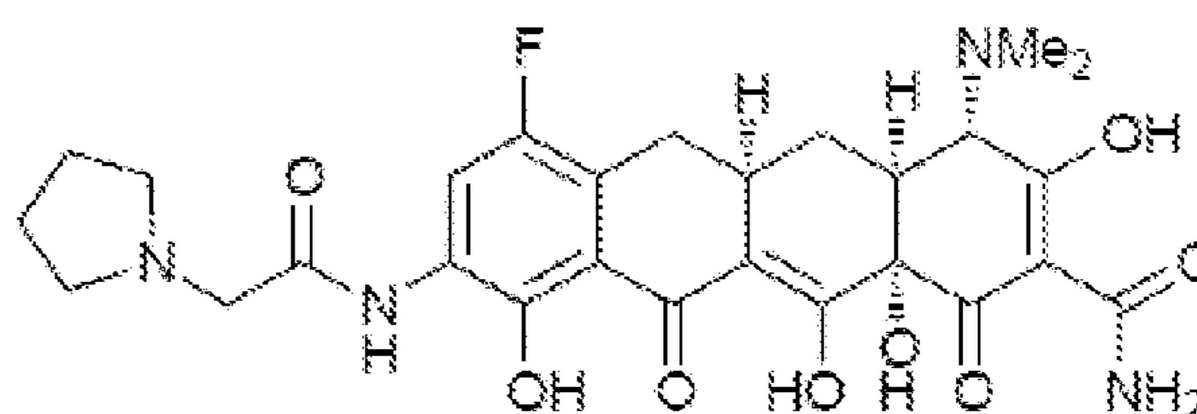
10: eravacycline (TP-434)
