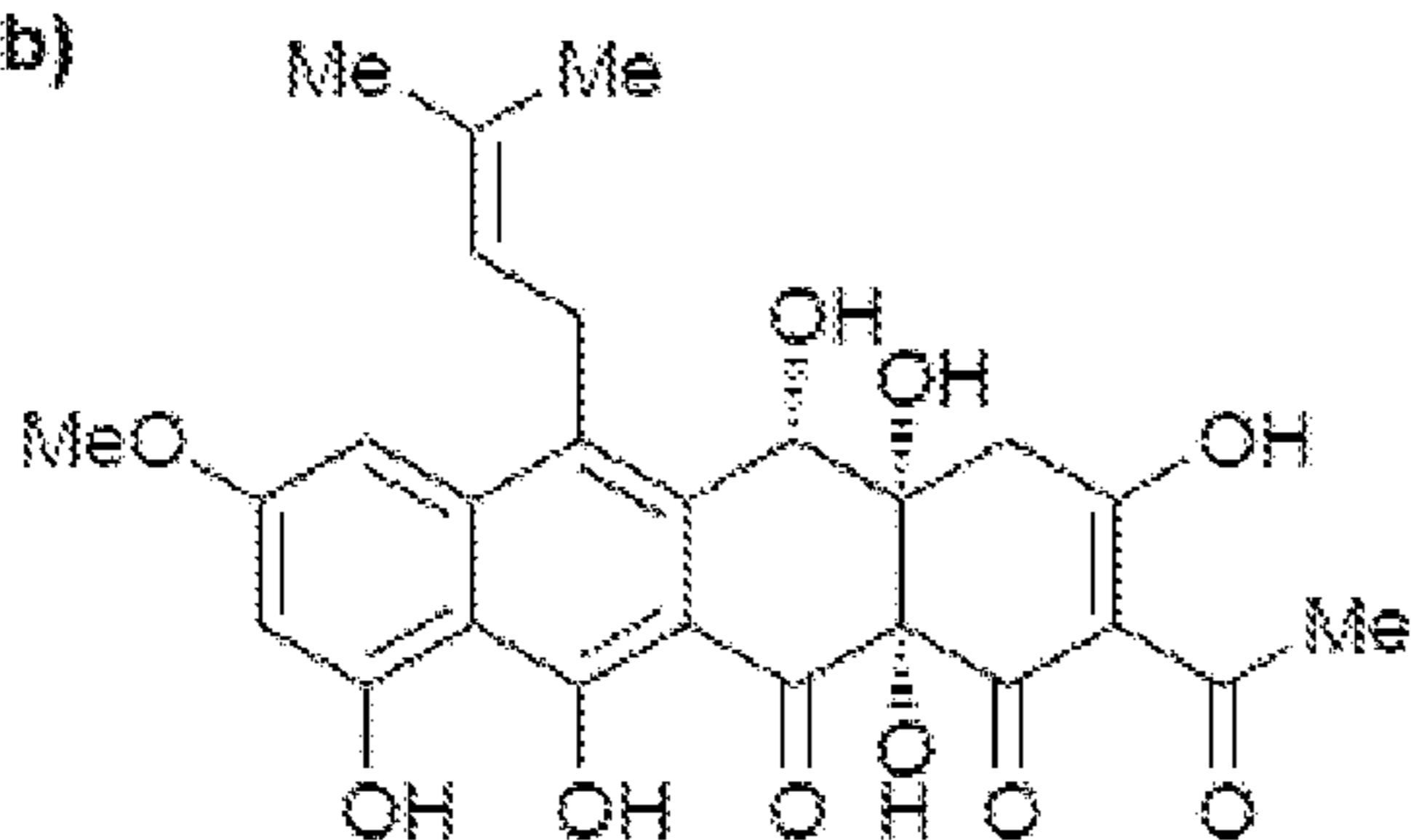
11: hypomycetin
