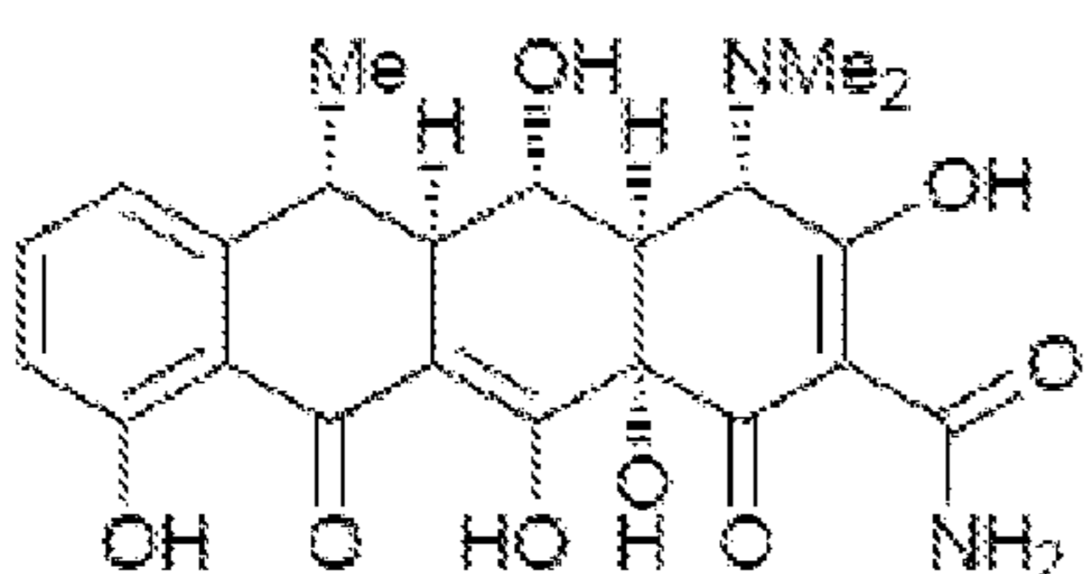
8: doxycycline (Vibramycin®)
