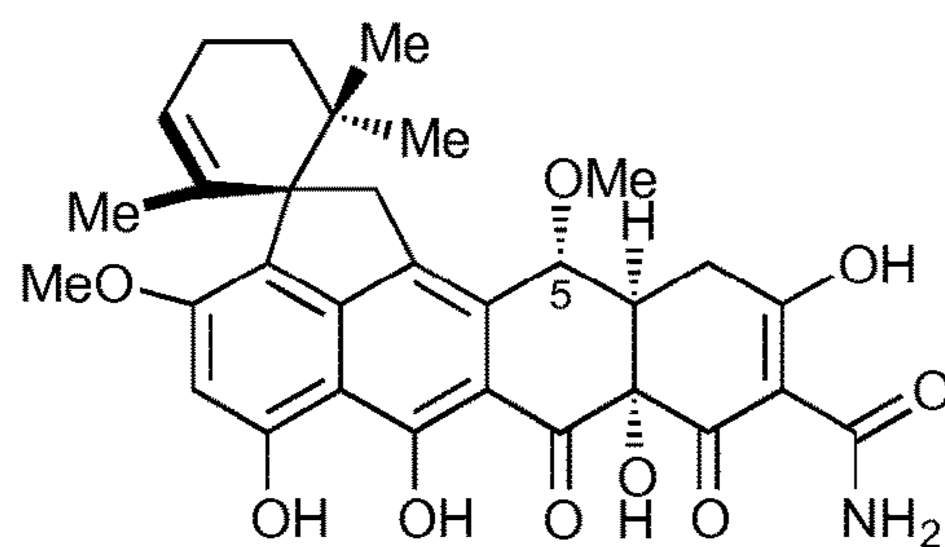
(±)-V5
