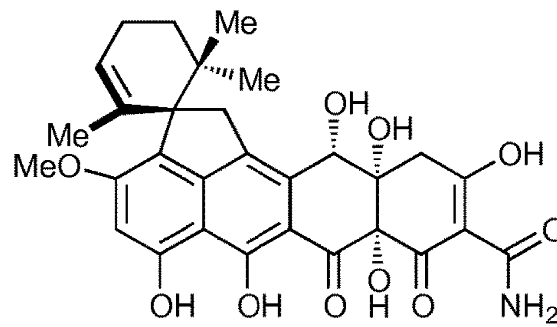
(+)-2: viridicatumtoxin A
