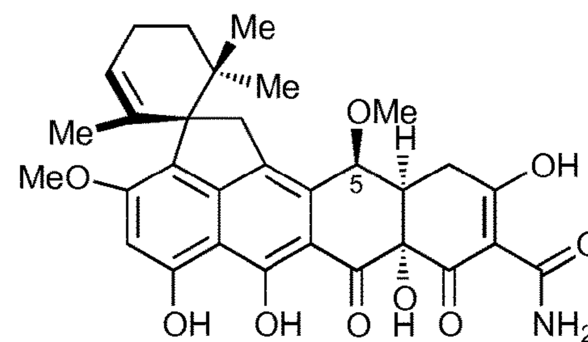
(±)-V6
