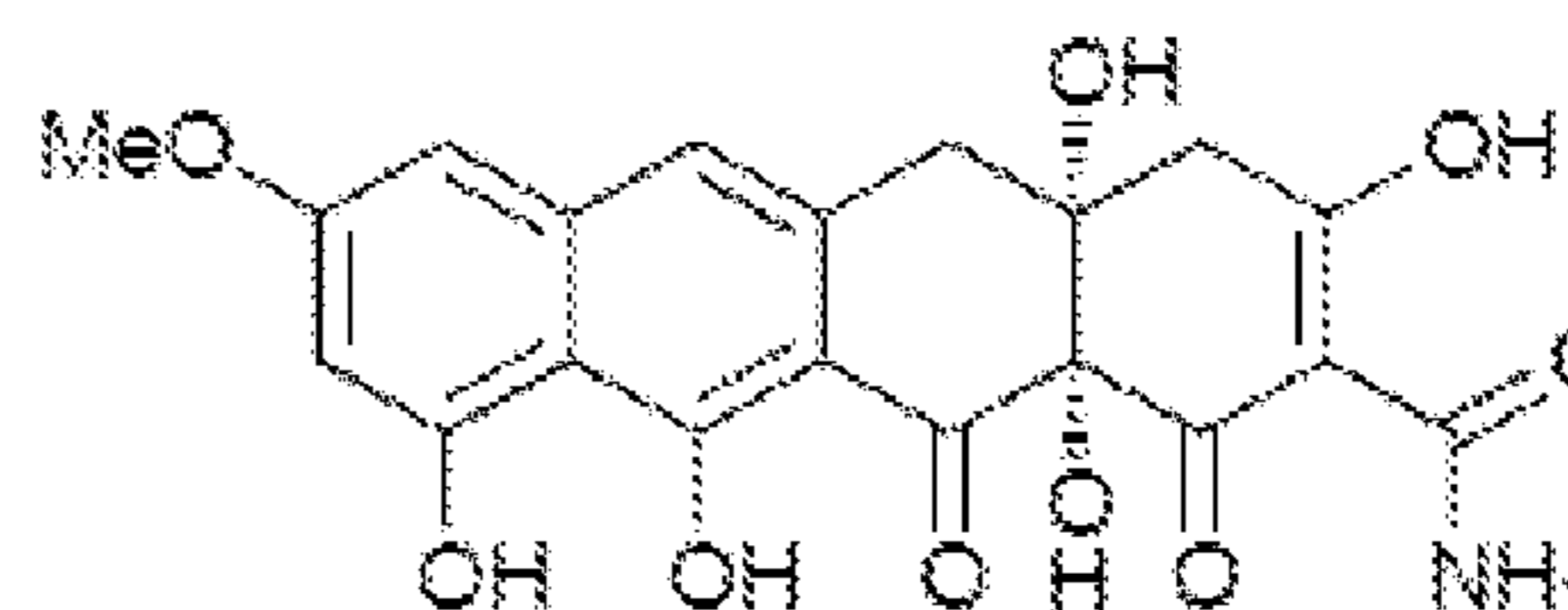
12: anthrotainin (TAN-1652)
