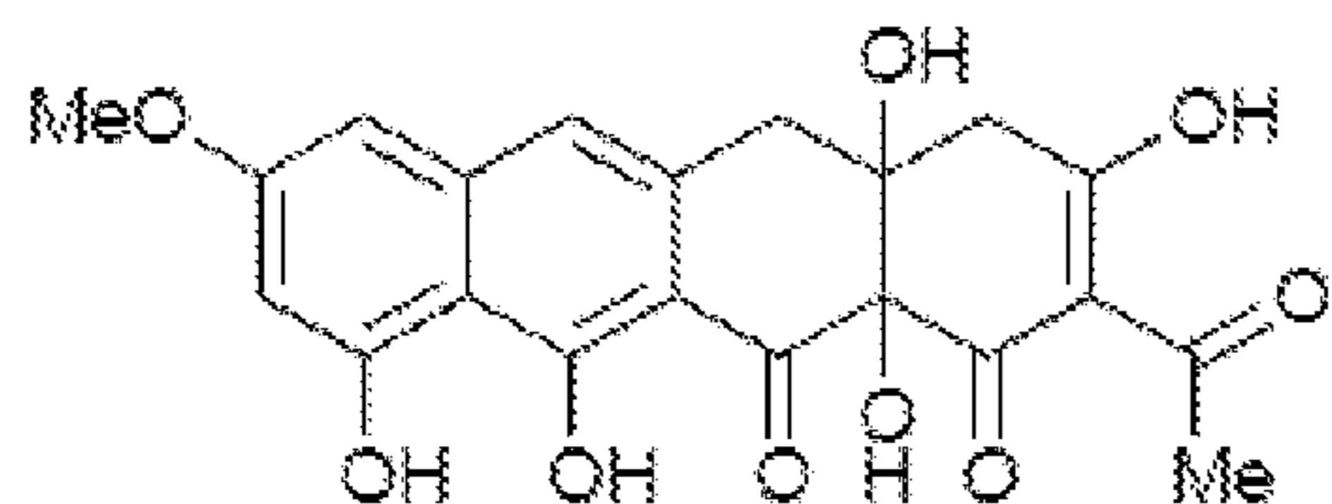
13: TAN-1612
