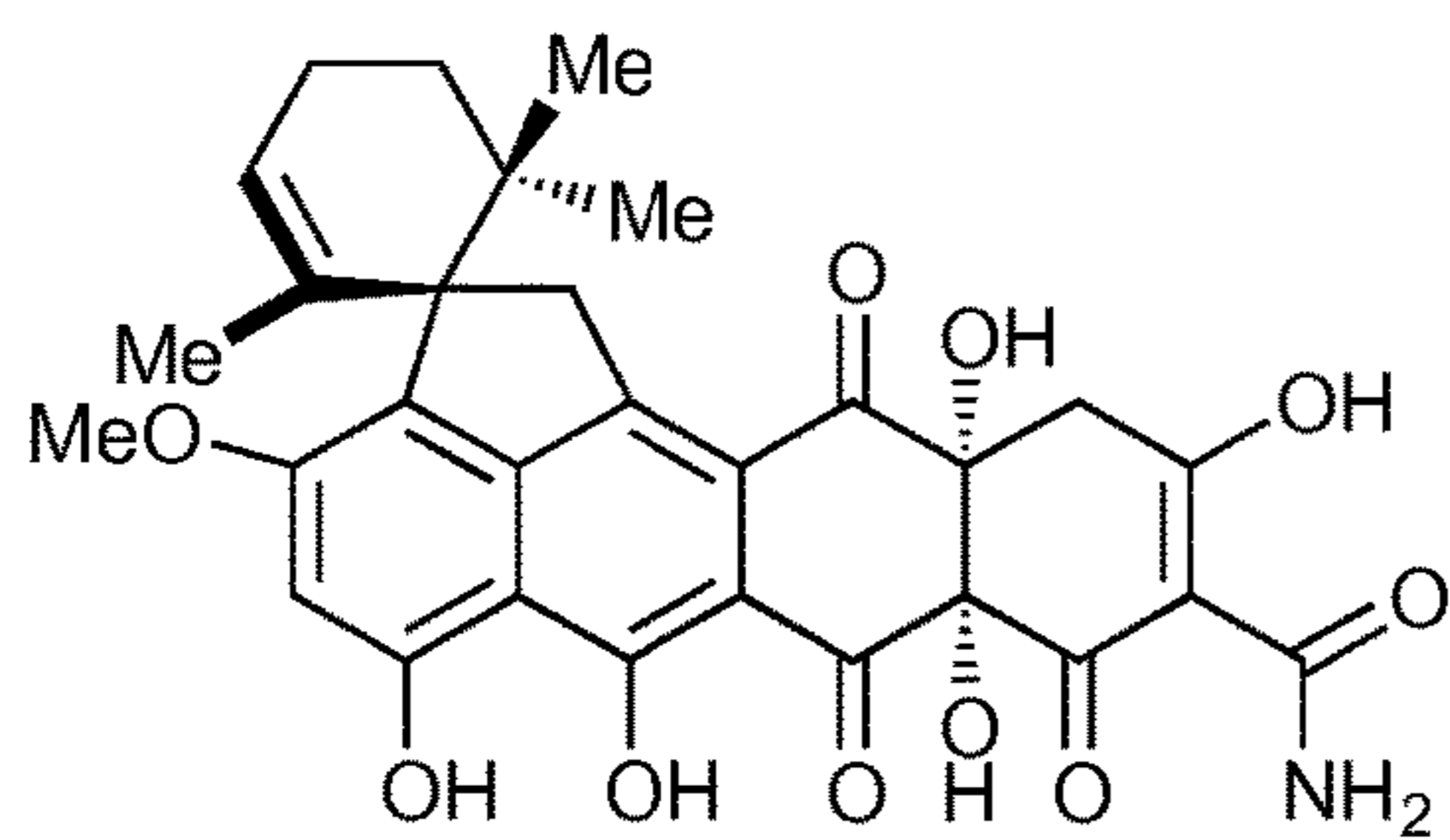
(+)-1: viridicatumtoxin B
