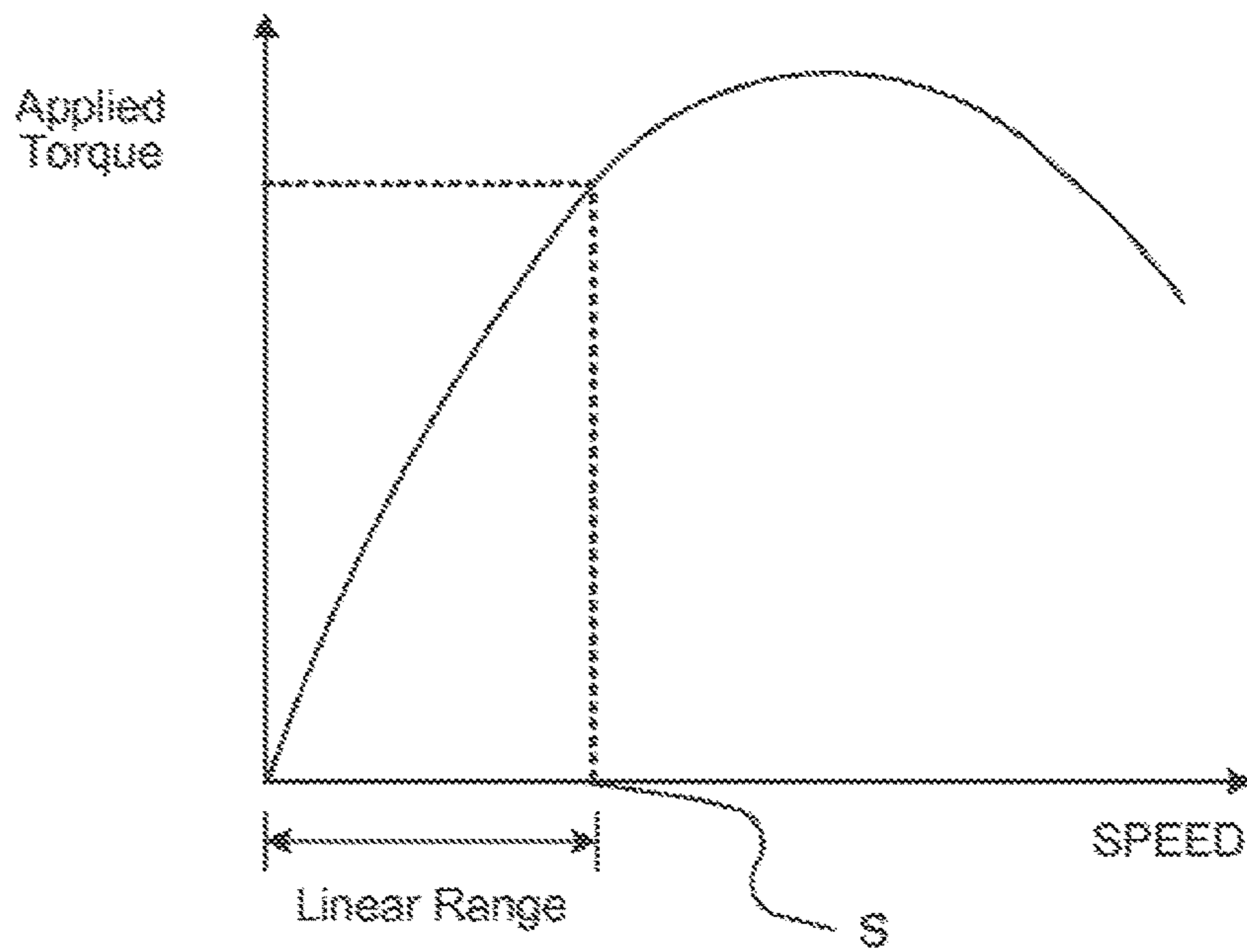
Figure 1 - Prior Art
