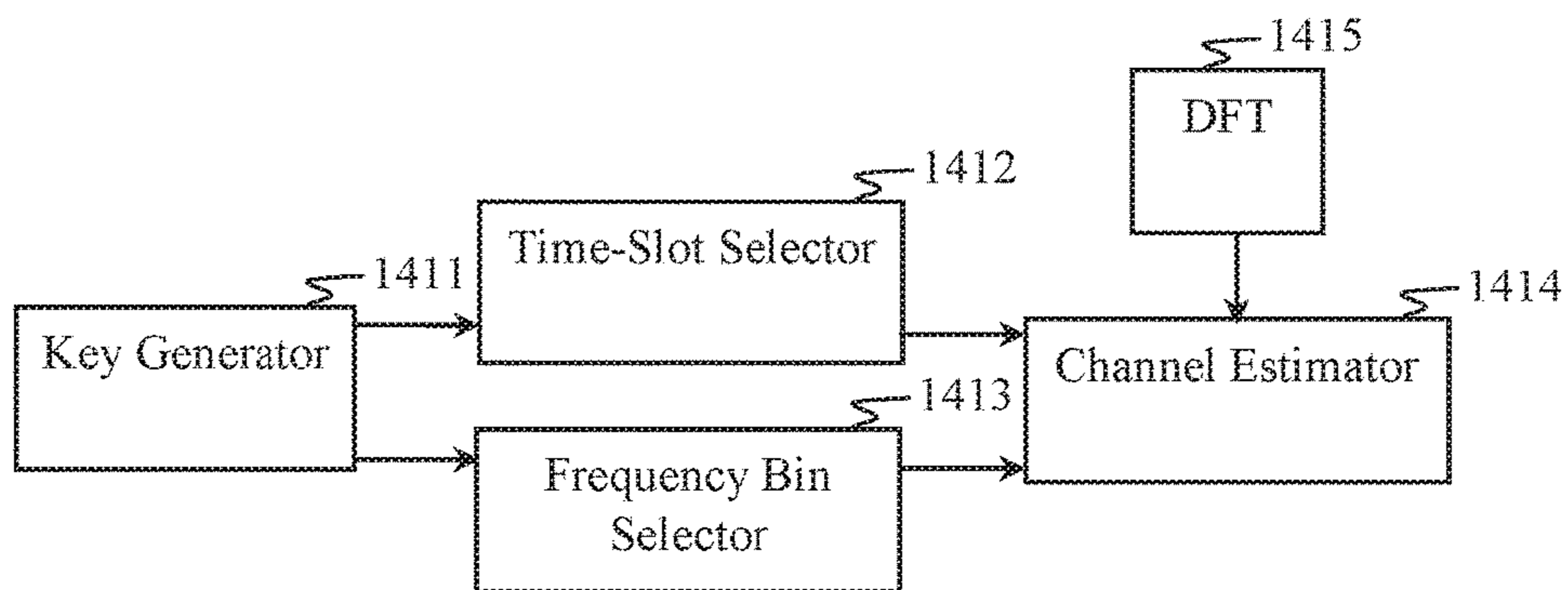
Figure 14B
