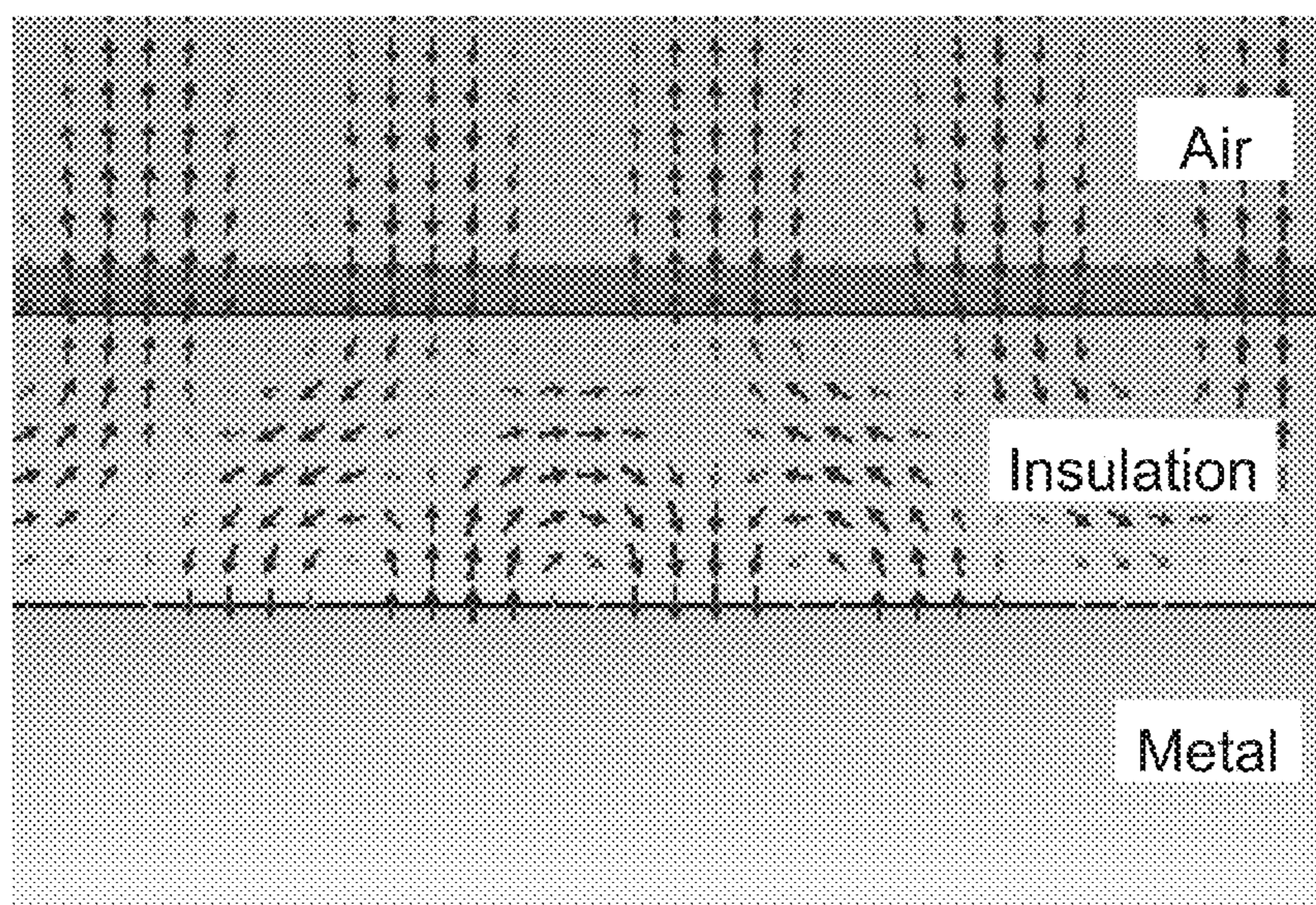
Longitudinal Section of Cable showing e-fields of TM 01 waves at 40 GHz
