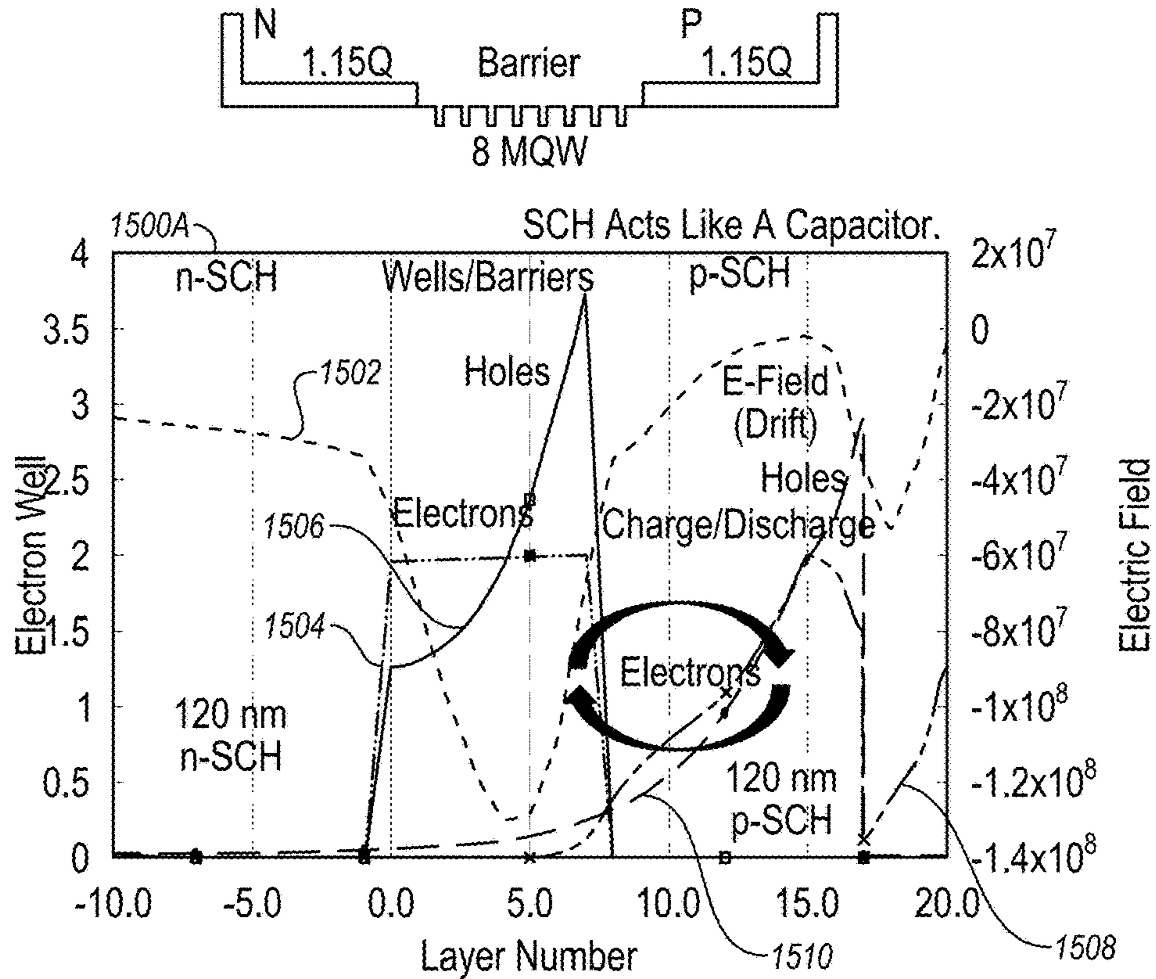
Carriers In SCH Charges/Discharges Due To Transport Effect, And Damps Overshooting.
