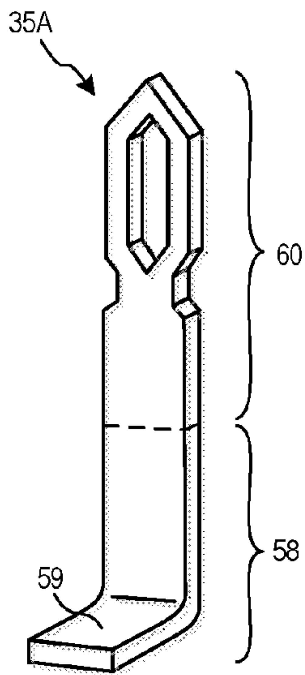
EYE-OF-THE-NEEDLE ELECTRICAL PRESS-FIT TERMINAL
