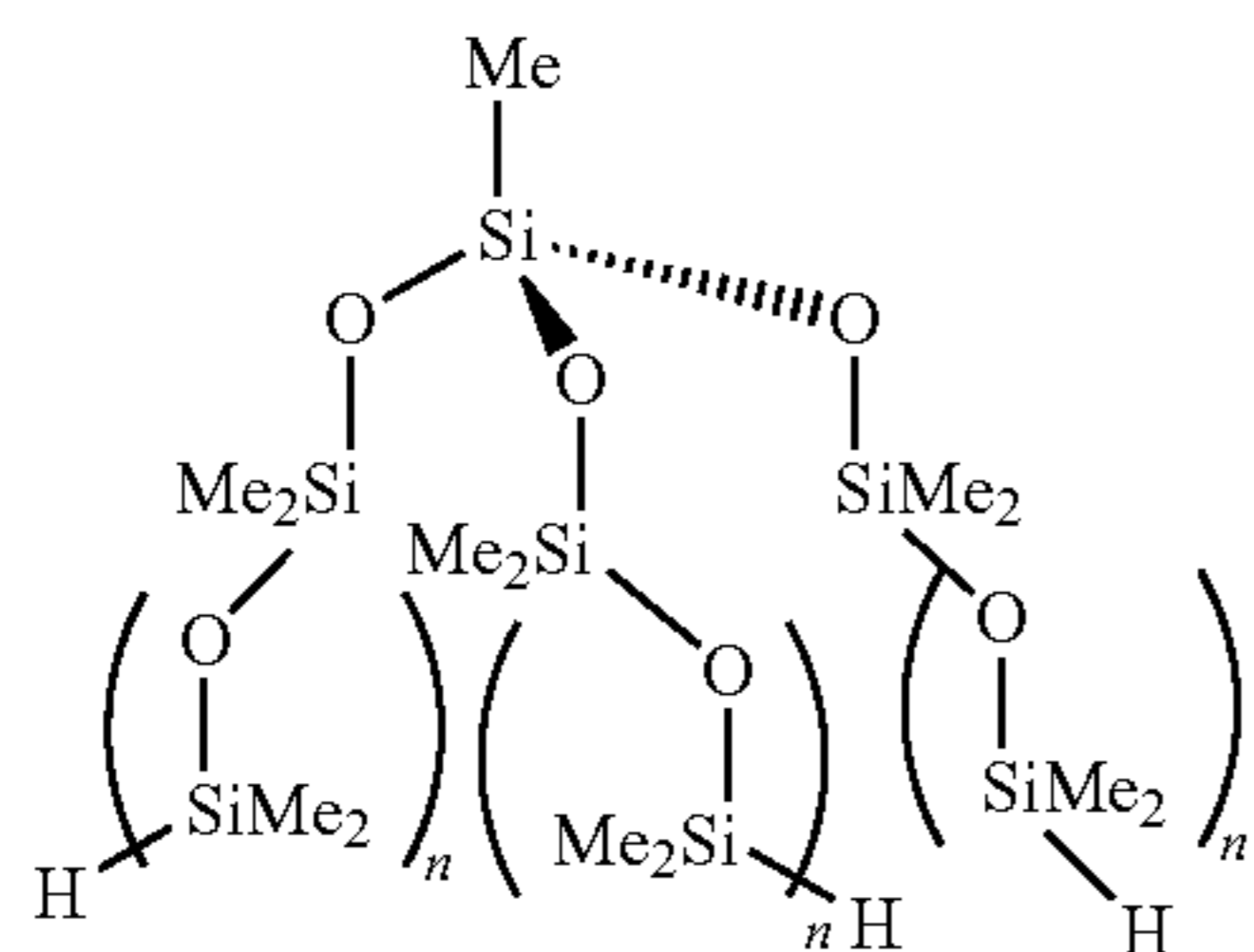
\alpha, \alpha', \alpha'' -(methylsilylydyne)tris- [ \omega [(dimethylhydrosilyl)oxy]poly(dimethylsilylene)]] (9Cl) intermediate.
