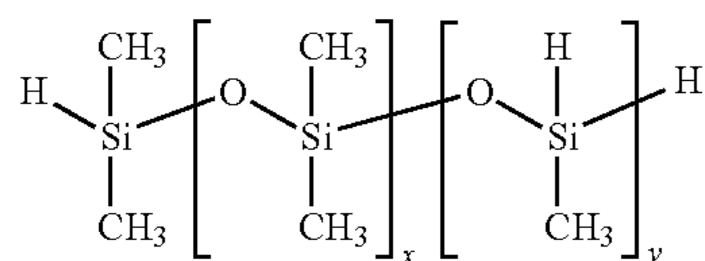
hydride terminated (methylhydrosiloxane) (dimethylsiloxane) intermediate
