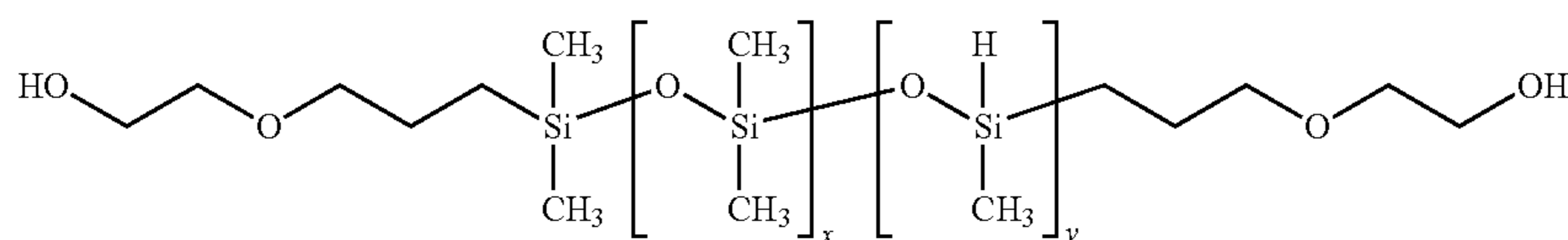
hydroxyethoxypropyl terminated (methylhydrosiloxane)(dimethylsiloxane) copolymer intermediate
