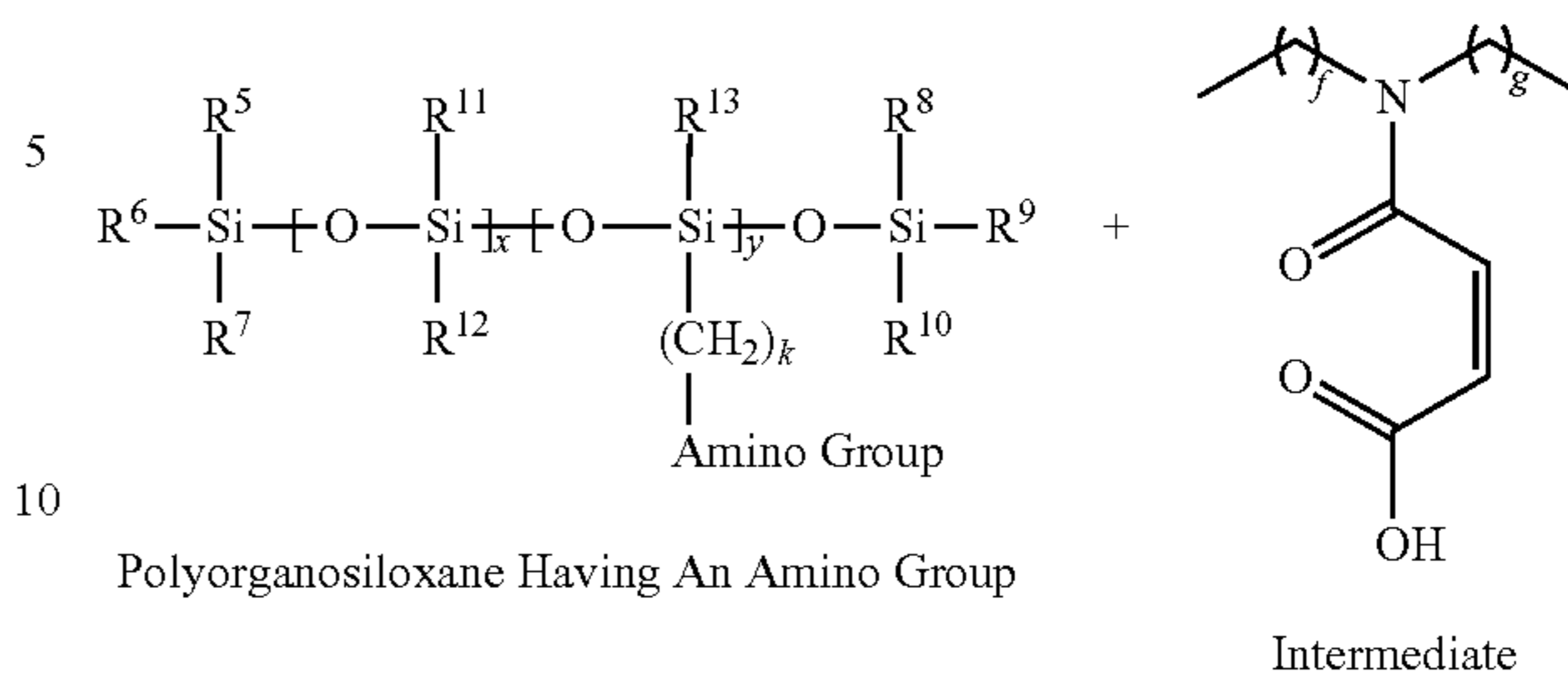
Reaction Scheme Eleven
