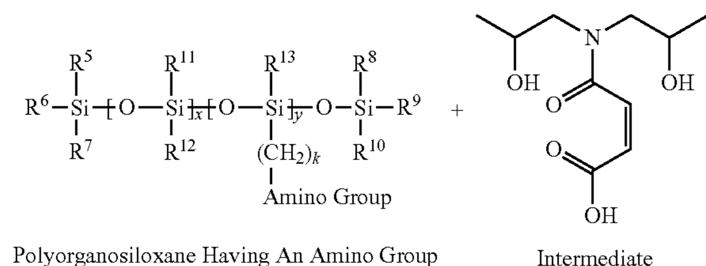
Reaction Scheme Ten
