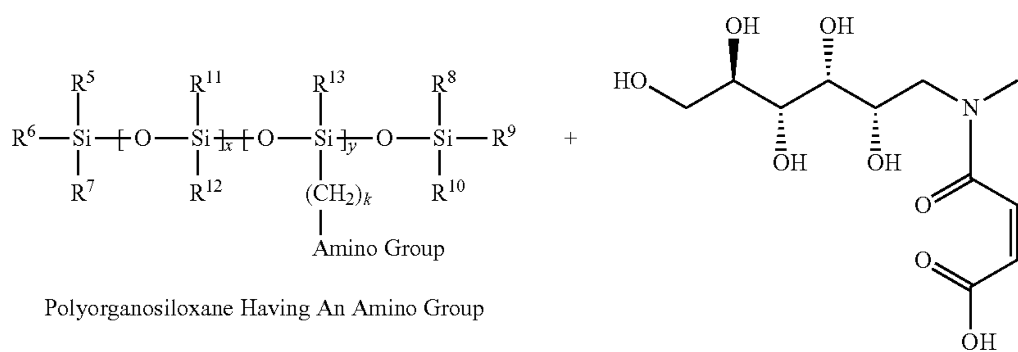
Reaction Scheme Twelve
