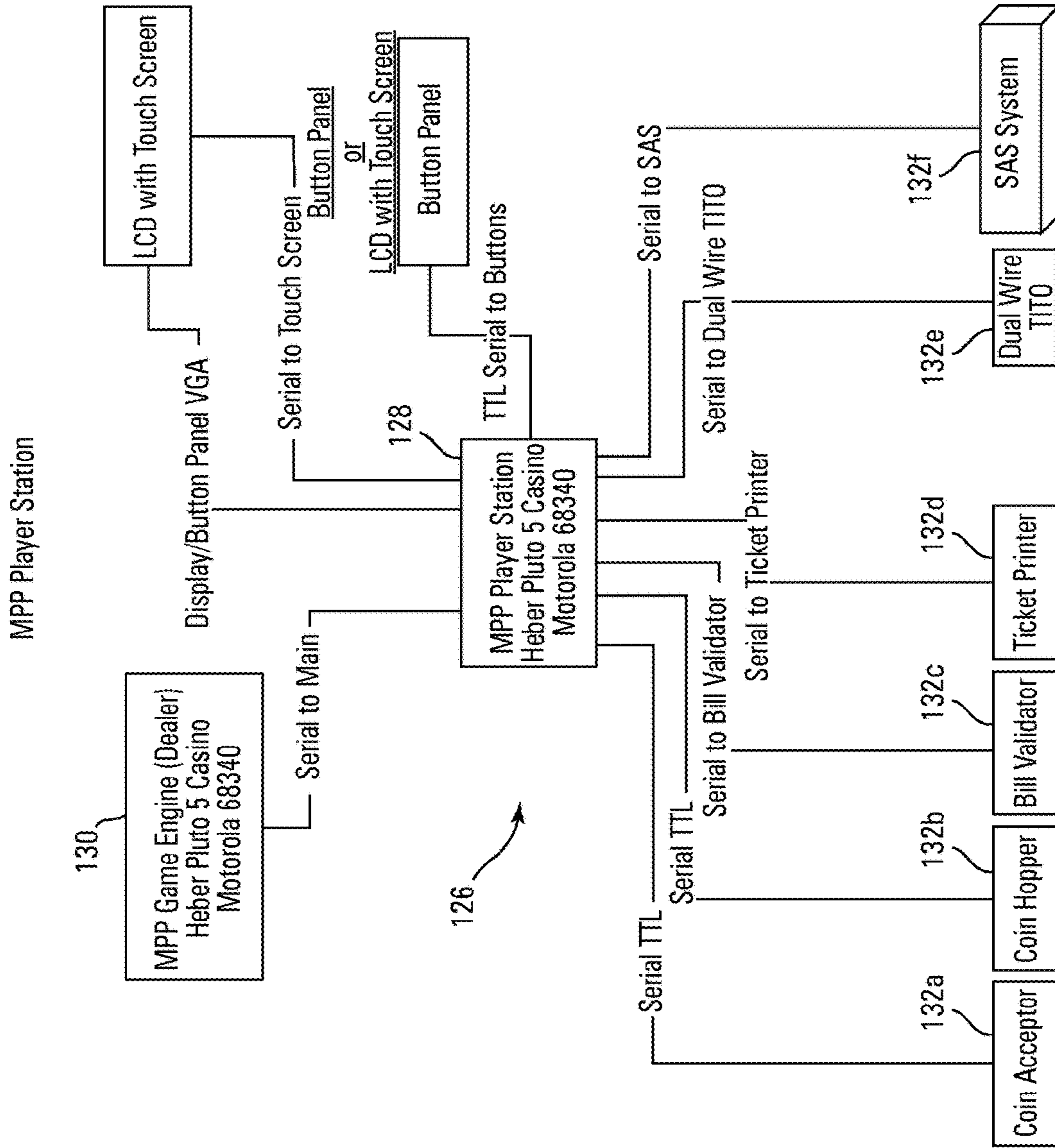
Fig. 7 Prior Art
