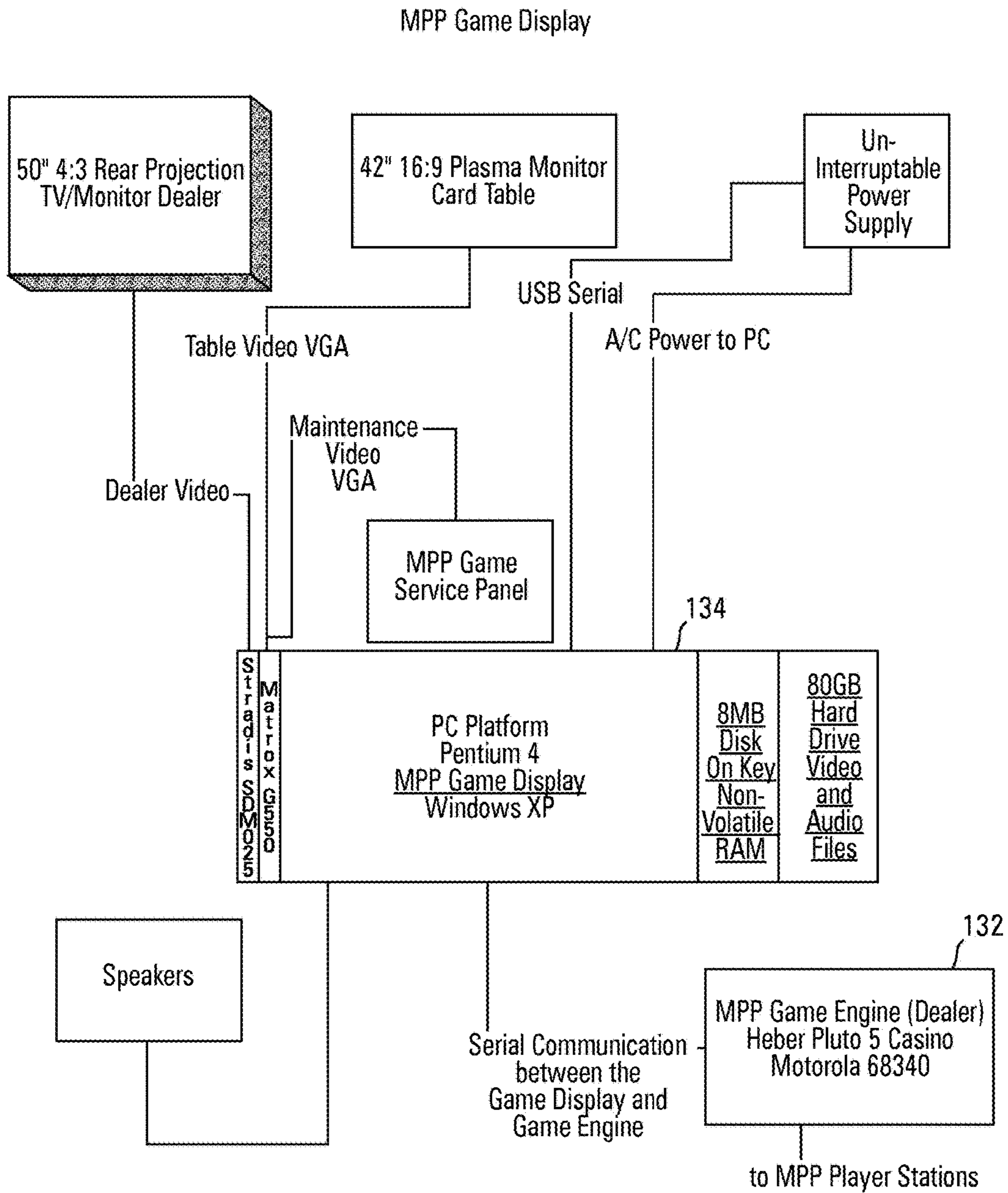
Fig. 8 Prior Art
