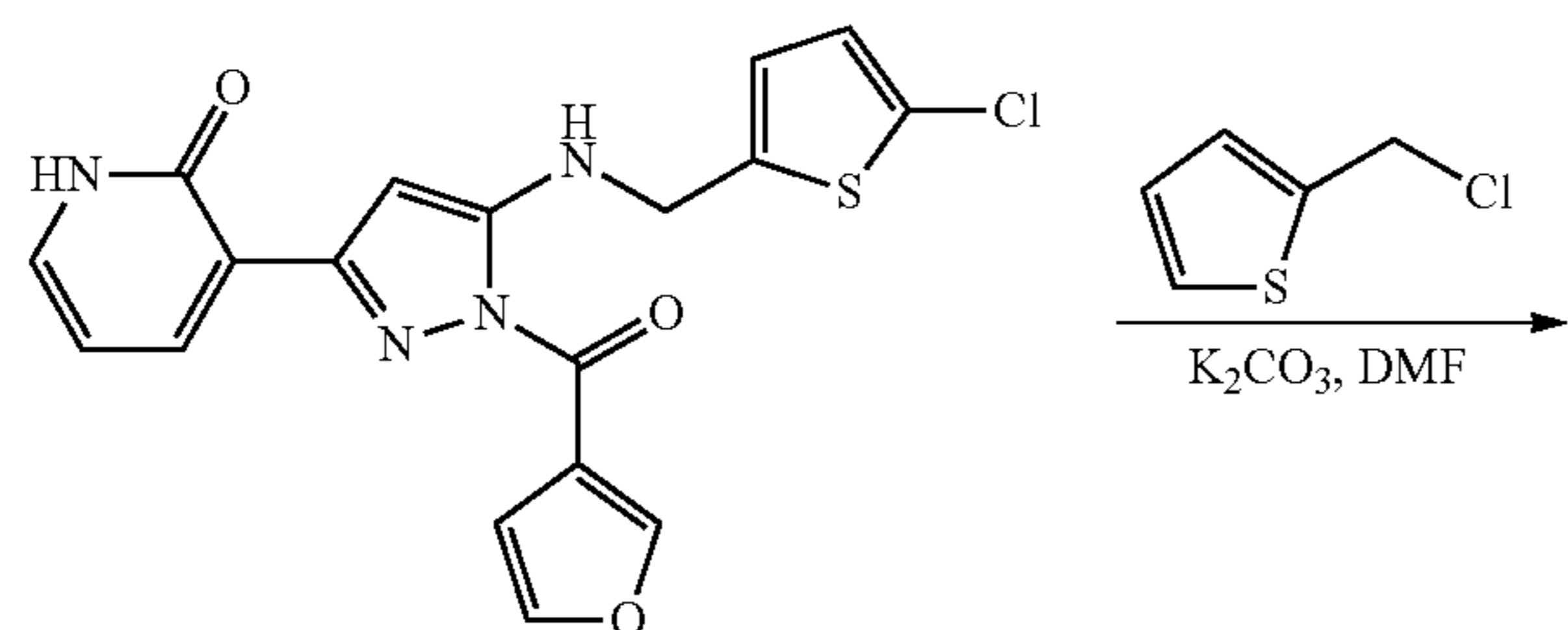
Compound 4
