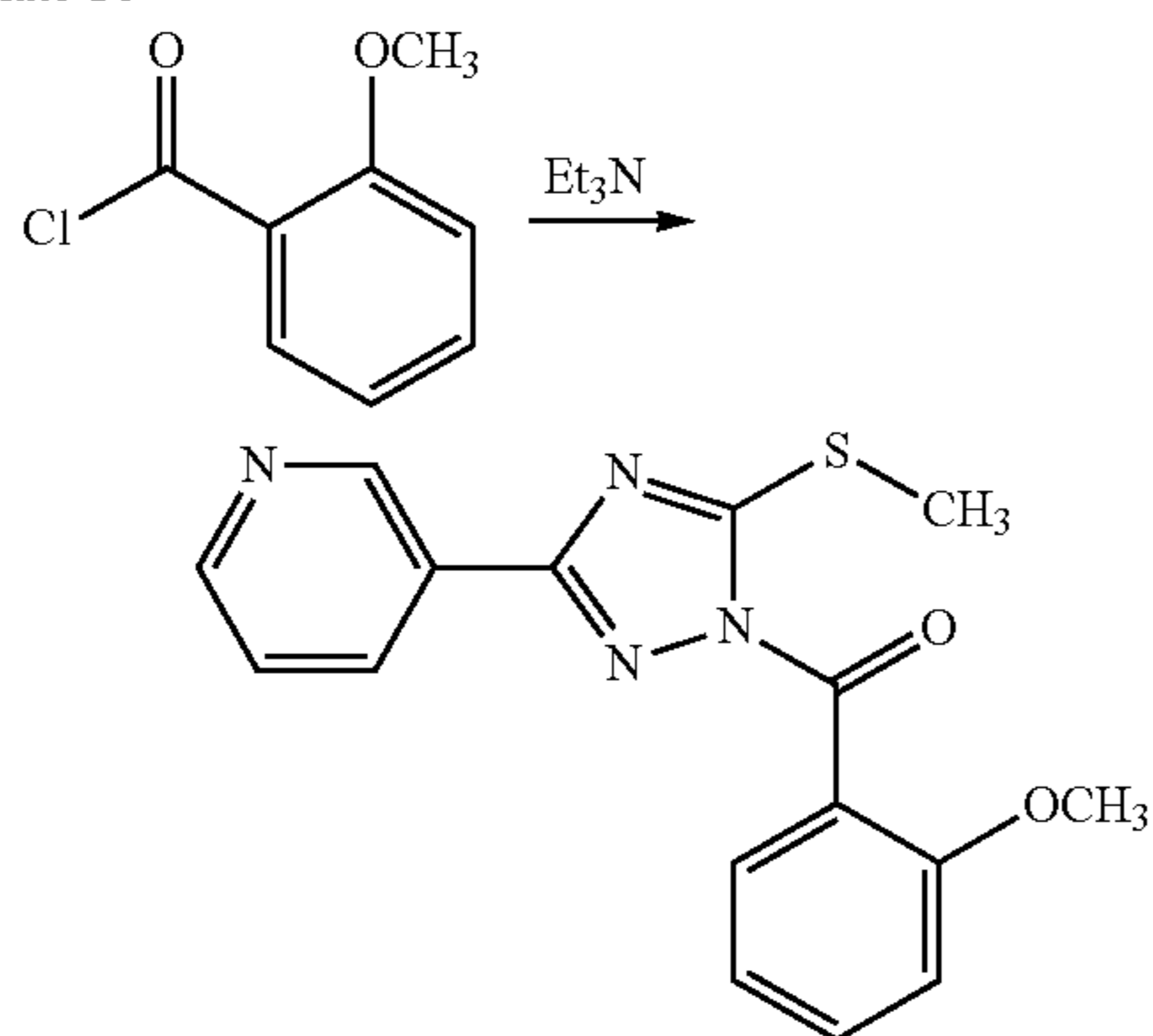
Compound 15
