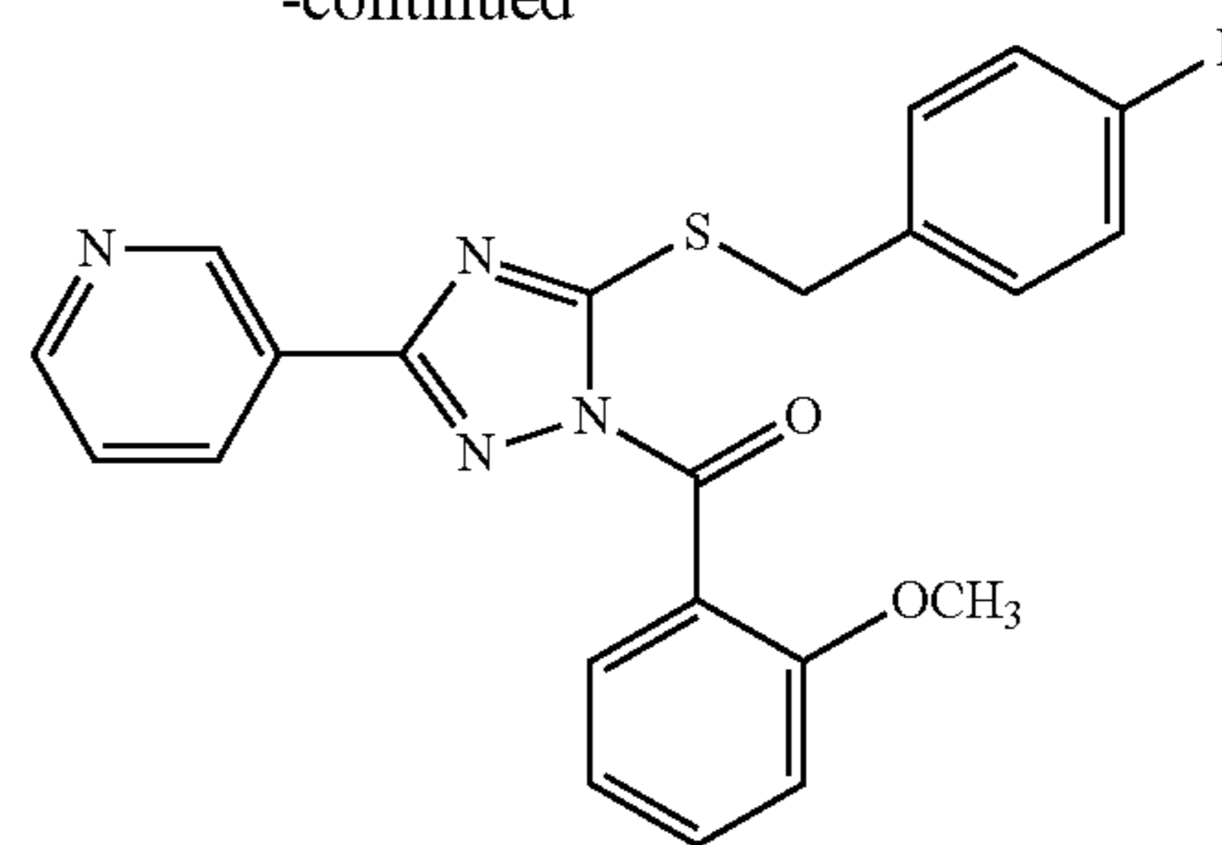
Compound 14
