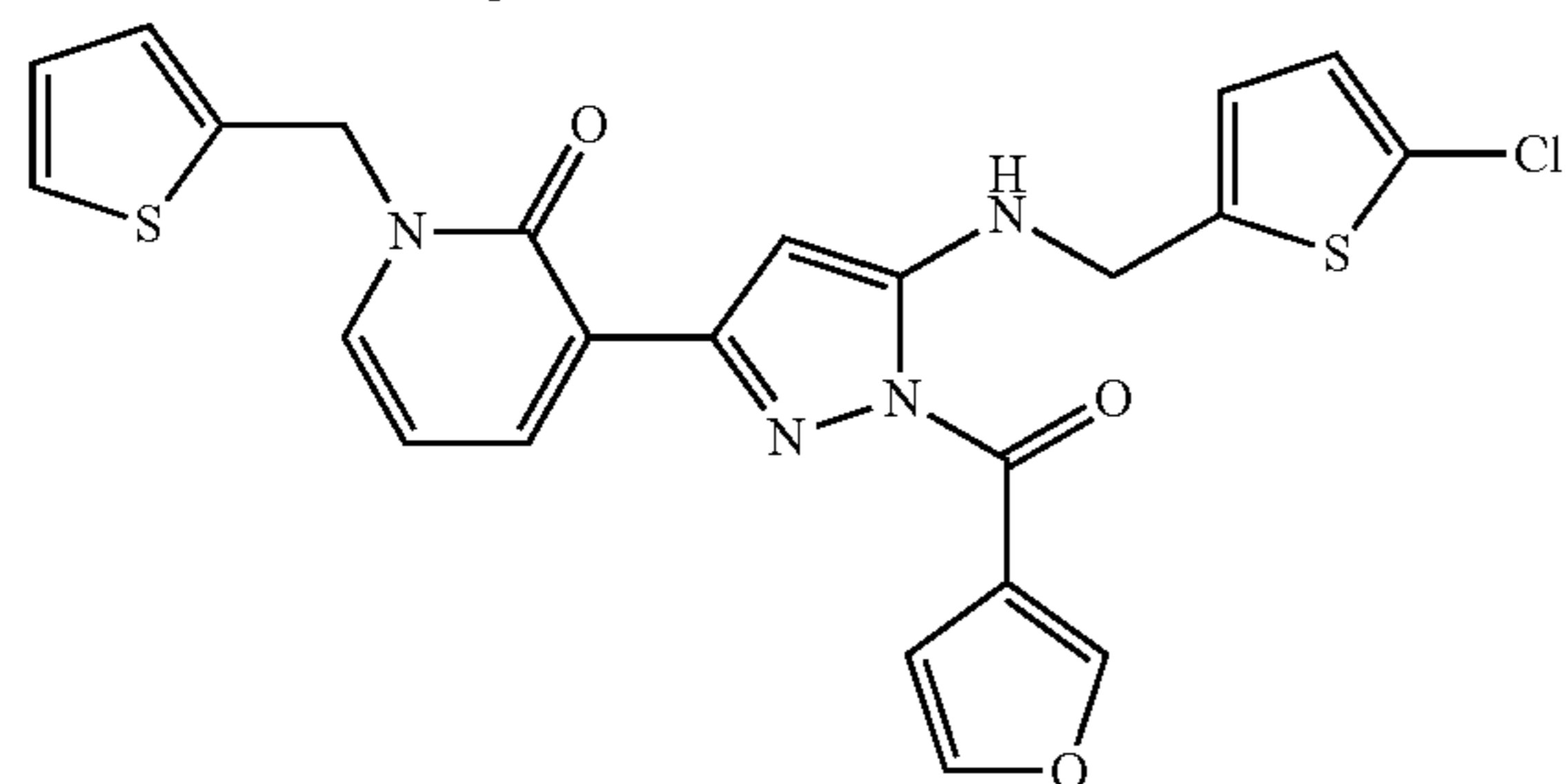
Compound 5
