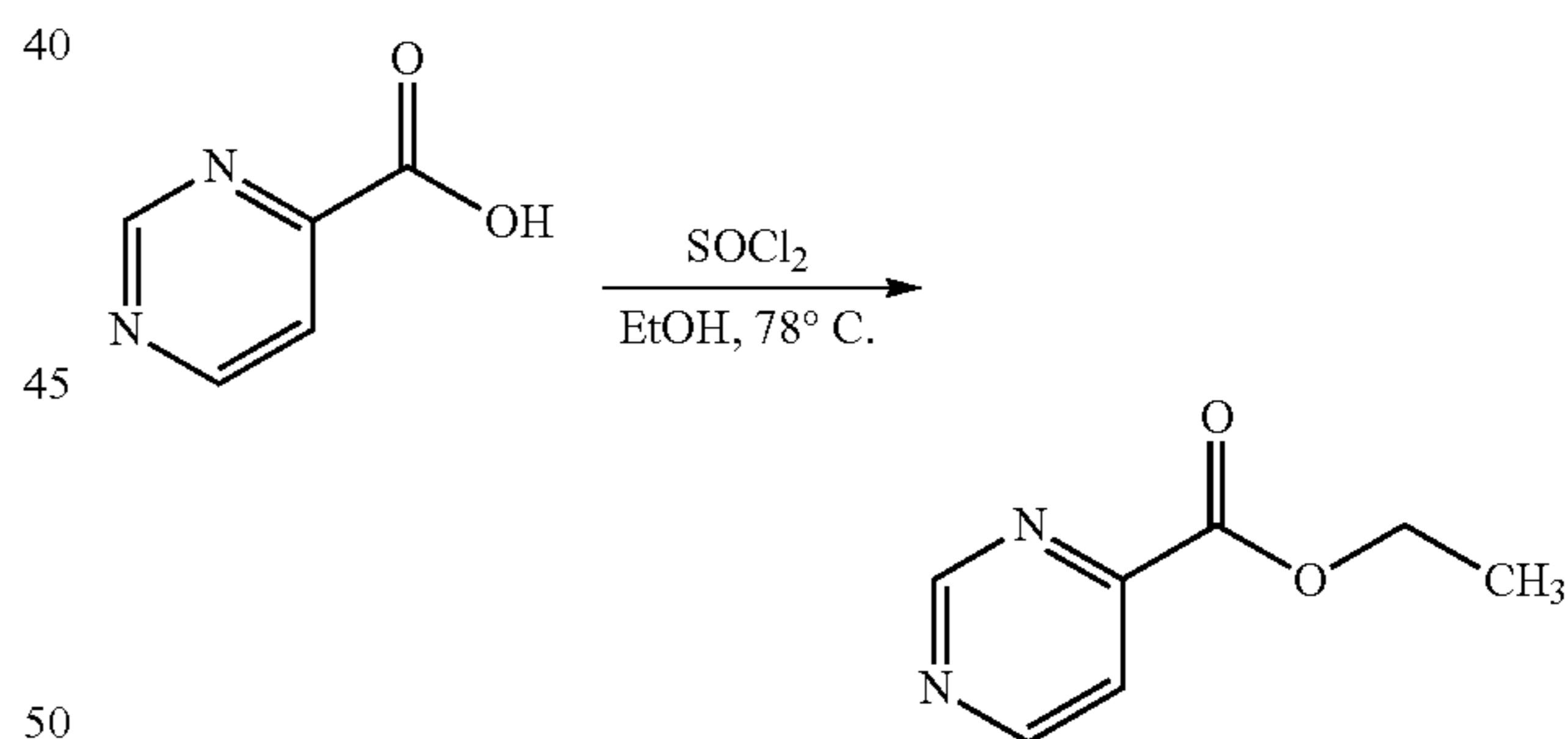
Intermediate 19
