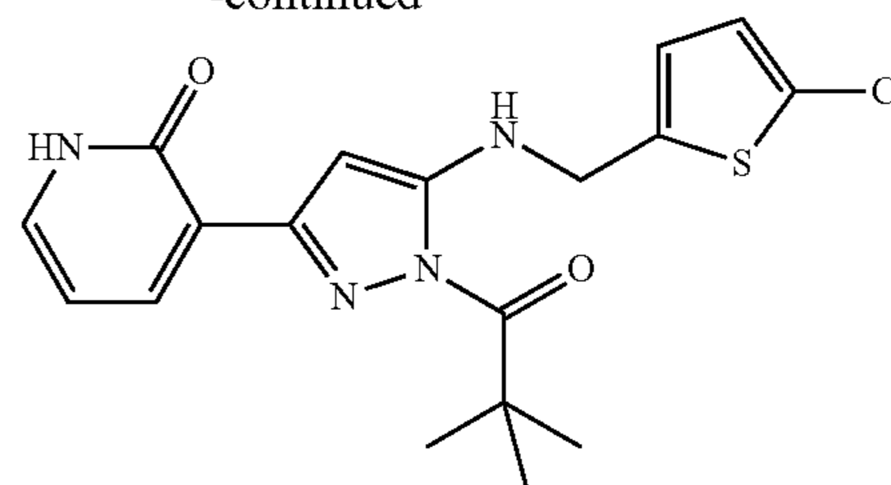
Compound 3
