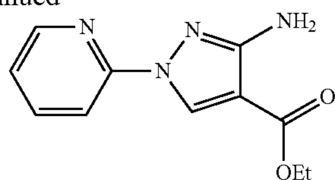
Intermediate 33
