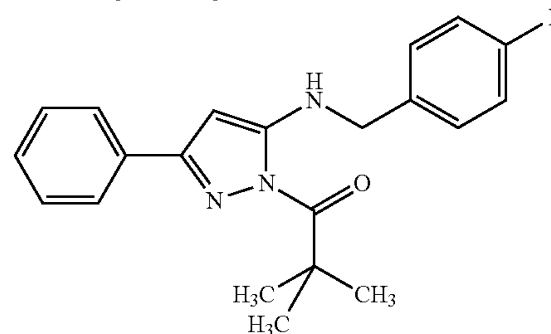
Compound 19
