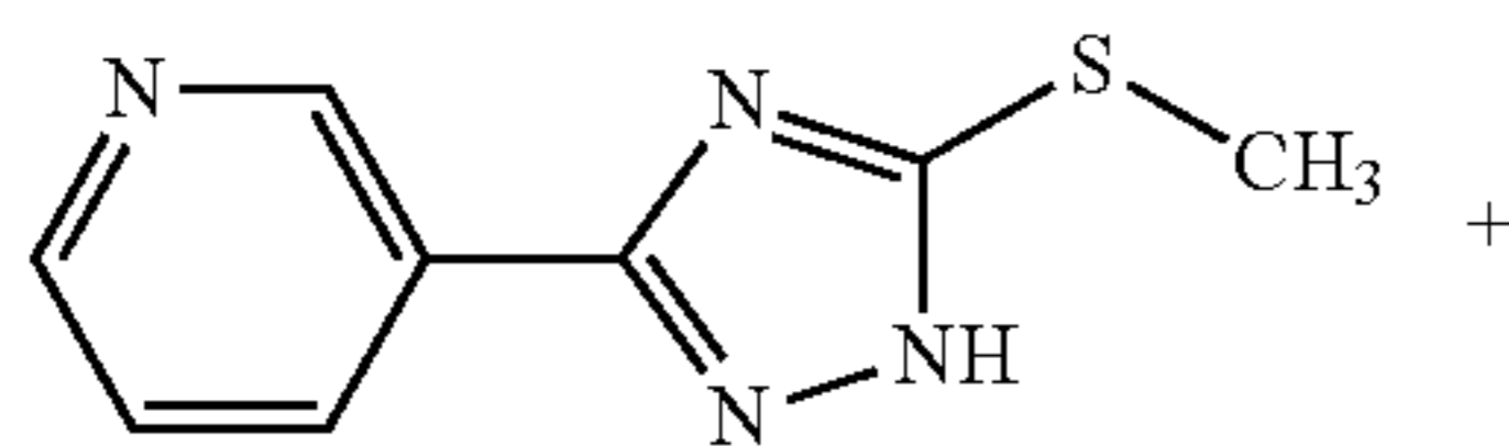
Intermediate 18
