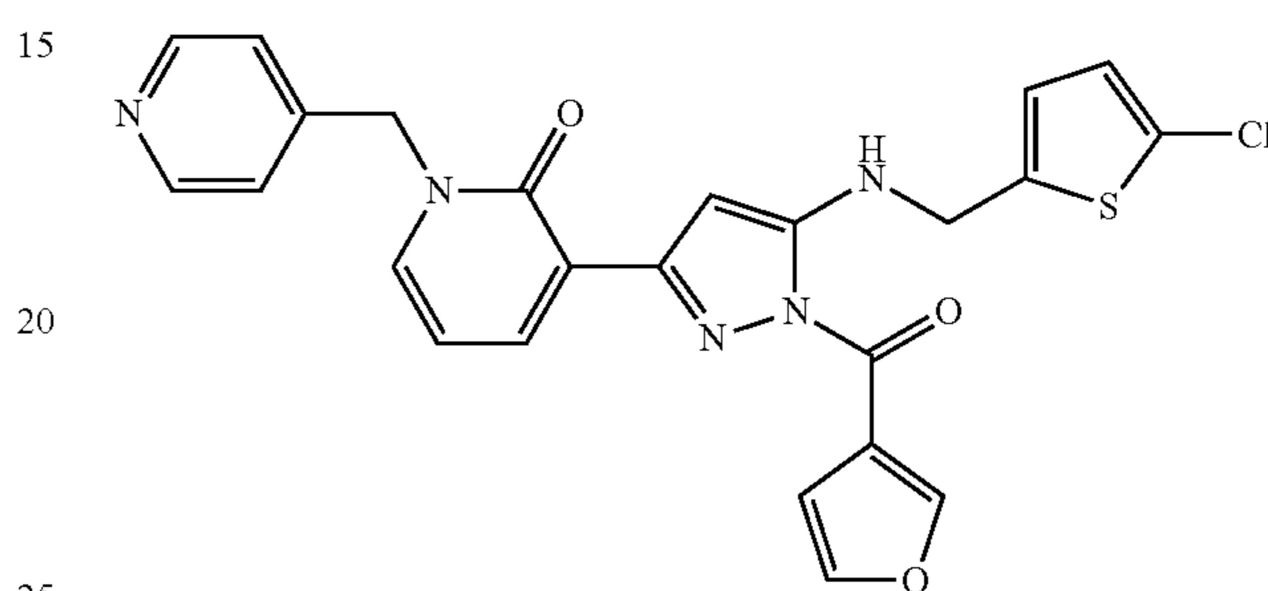
Compound 6
