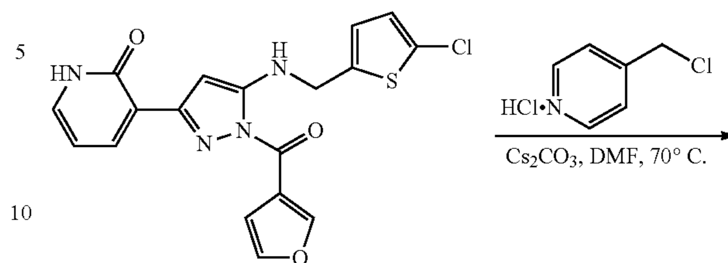
Compound 4
