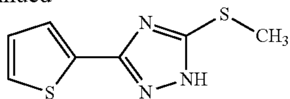
Intermediate 17
