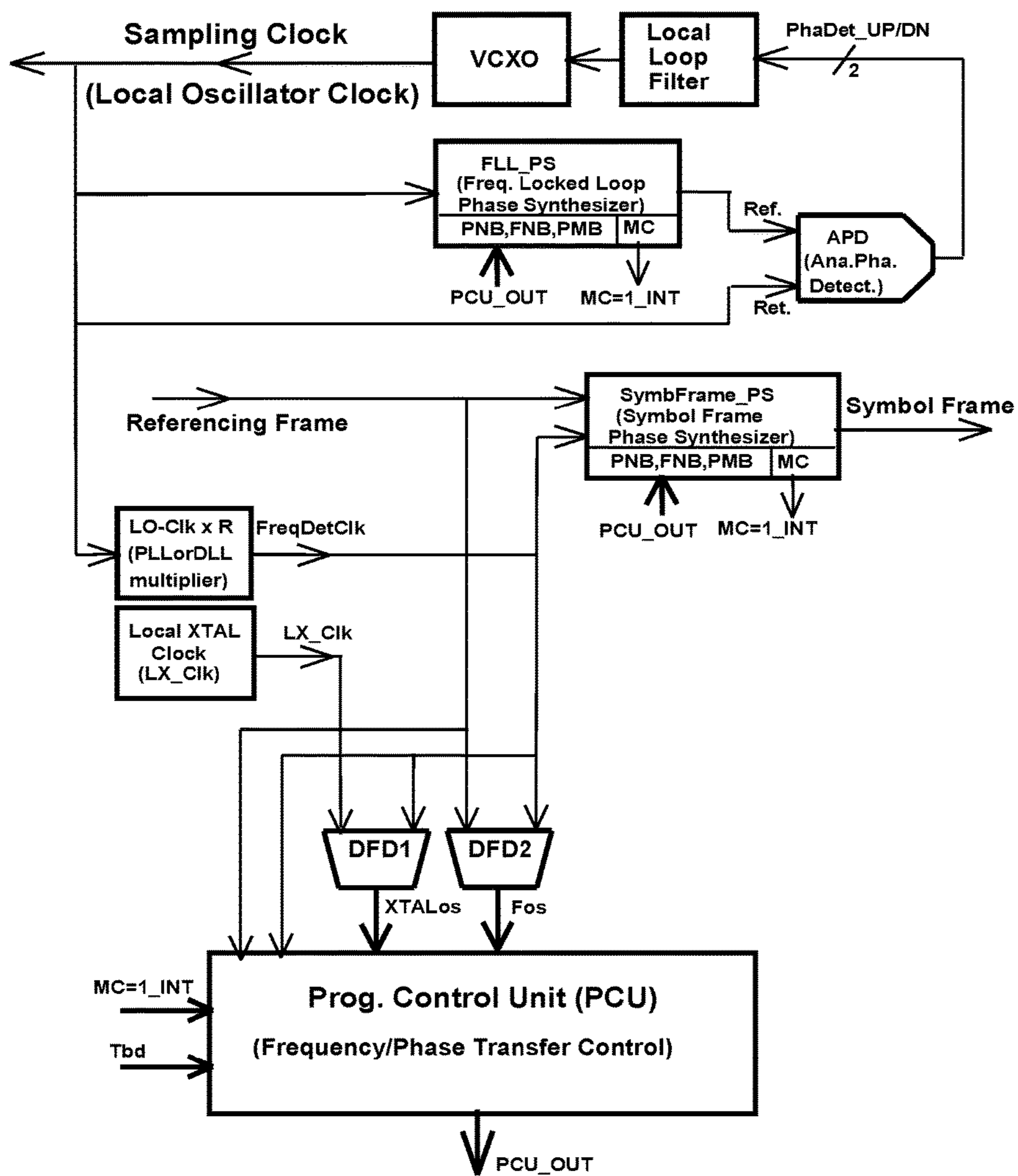
FIG.18 High Accuracy FLPS
