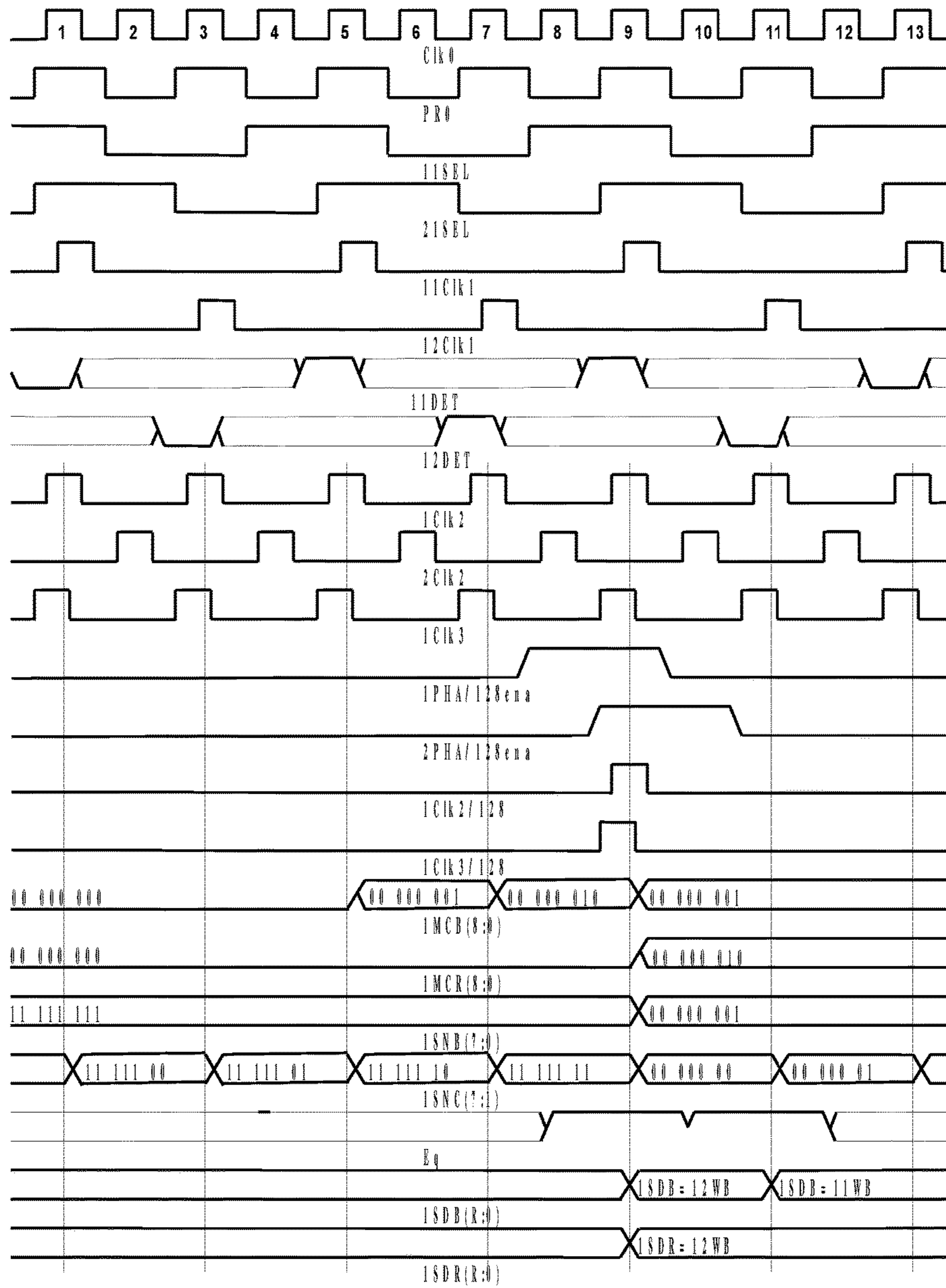
FIG.12 Timing Diagrams of the WFSC
