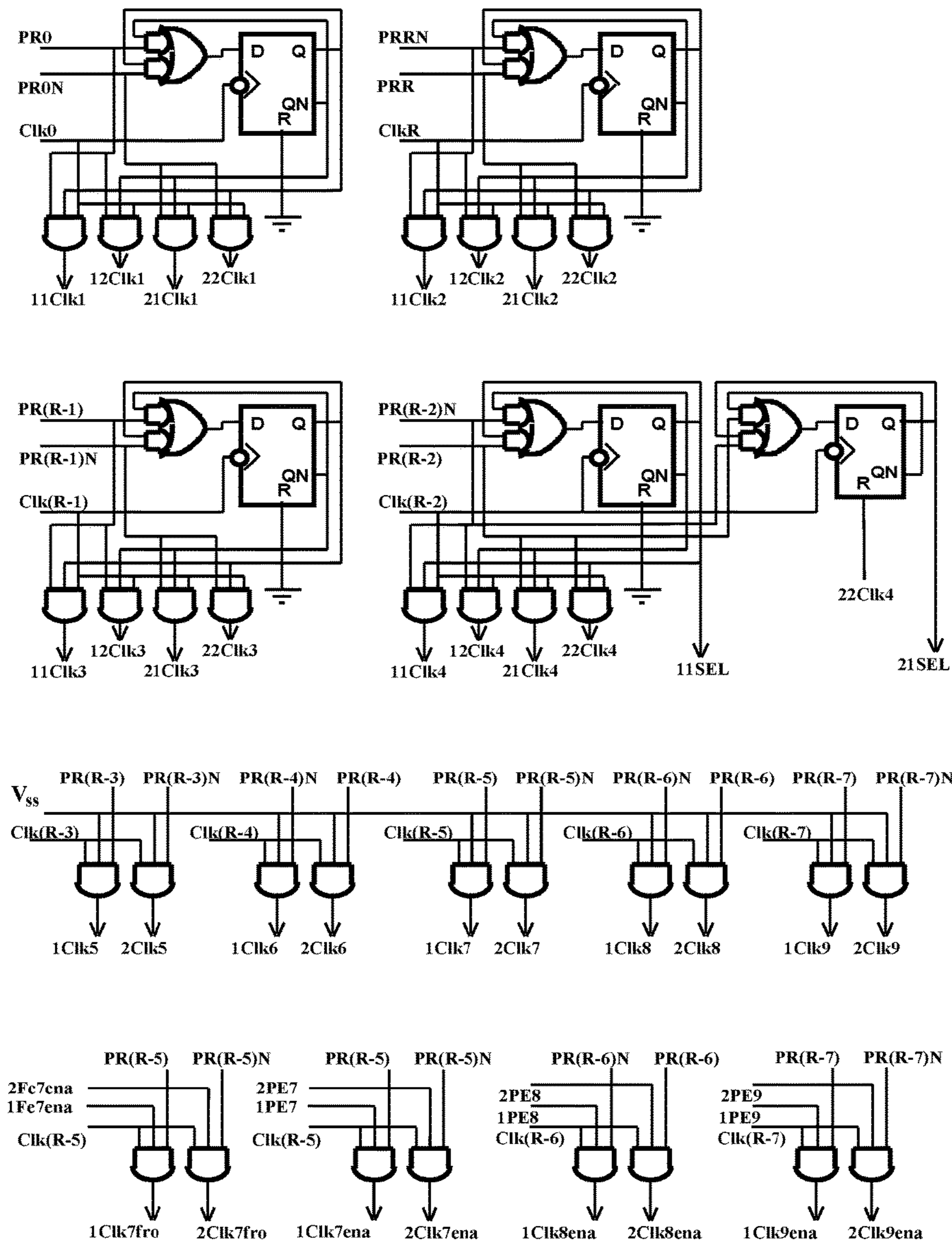
FIG.9 Sequential Clocks Generation for the NFED(SCG NFED)
