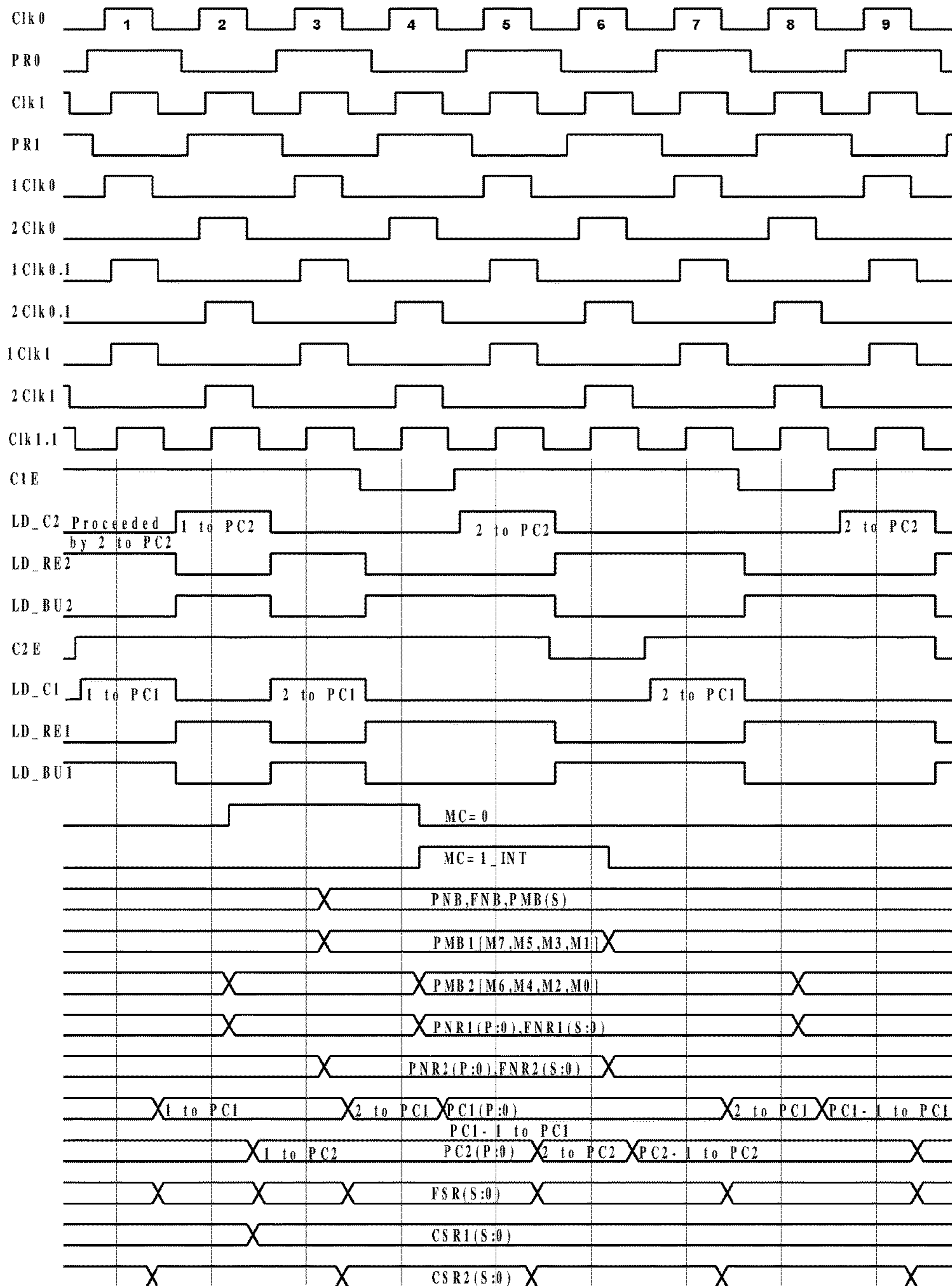
FIG.7 Timing Diagram of Phase Synthesizer
