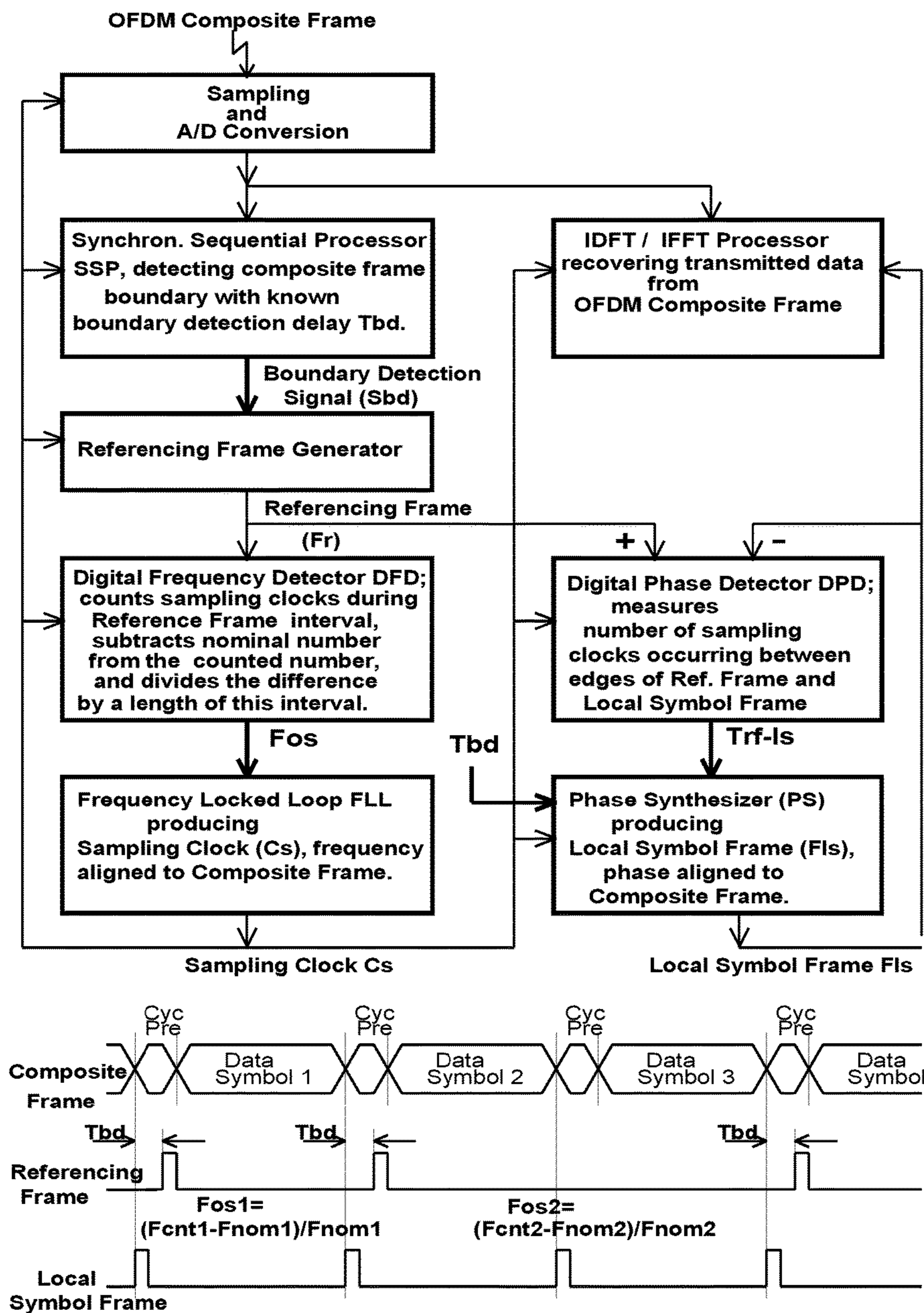
FIG.14 Synchronization System with Improved Stability
