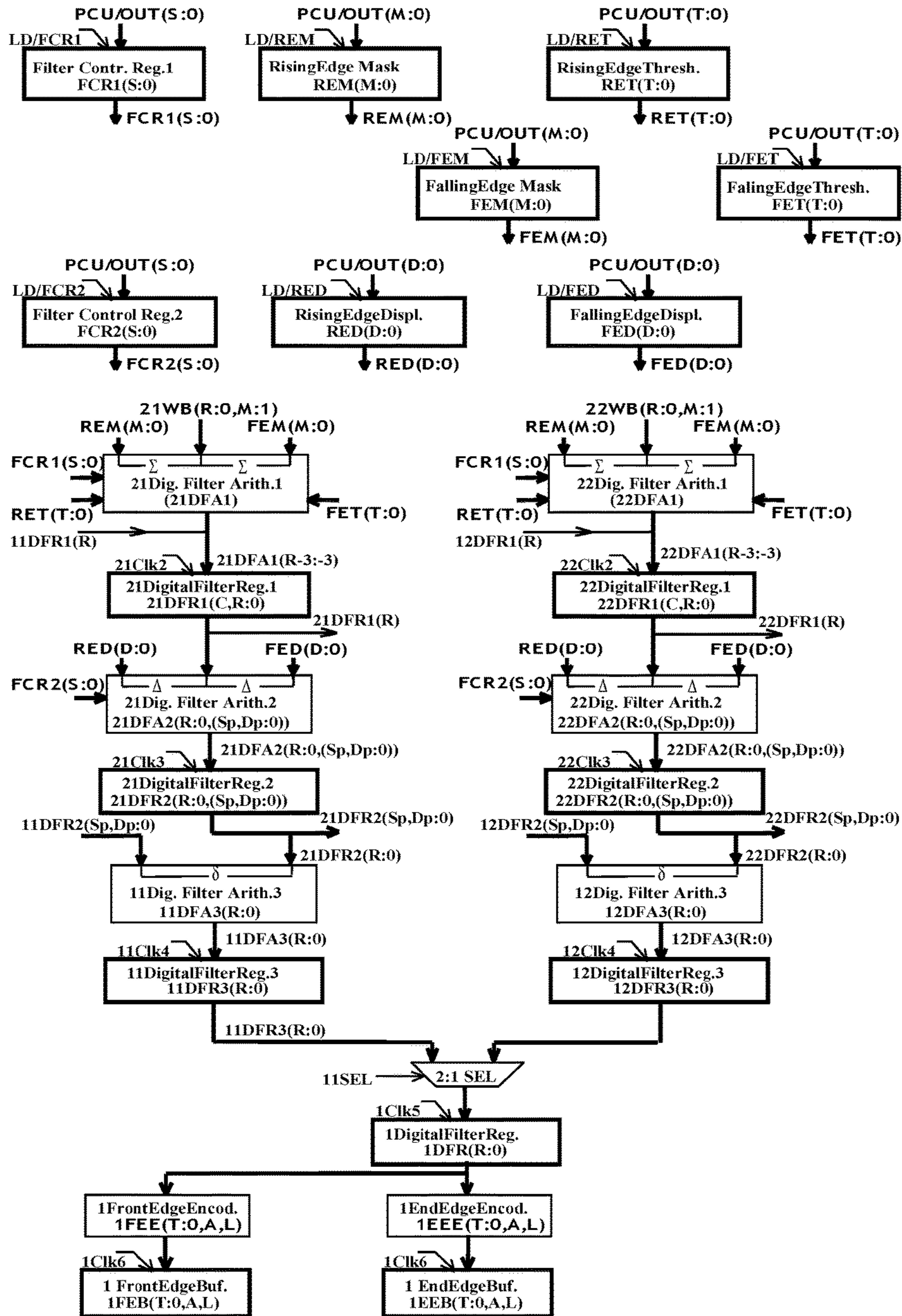
FIG.10 Noise Filtering Edge Detectors (NFED)
