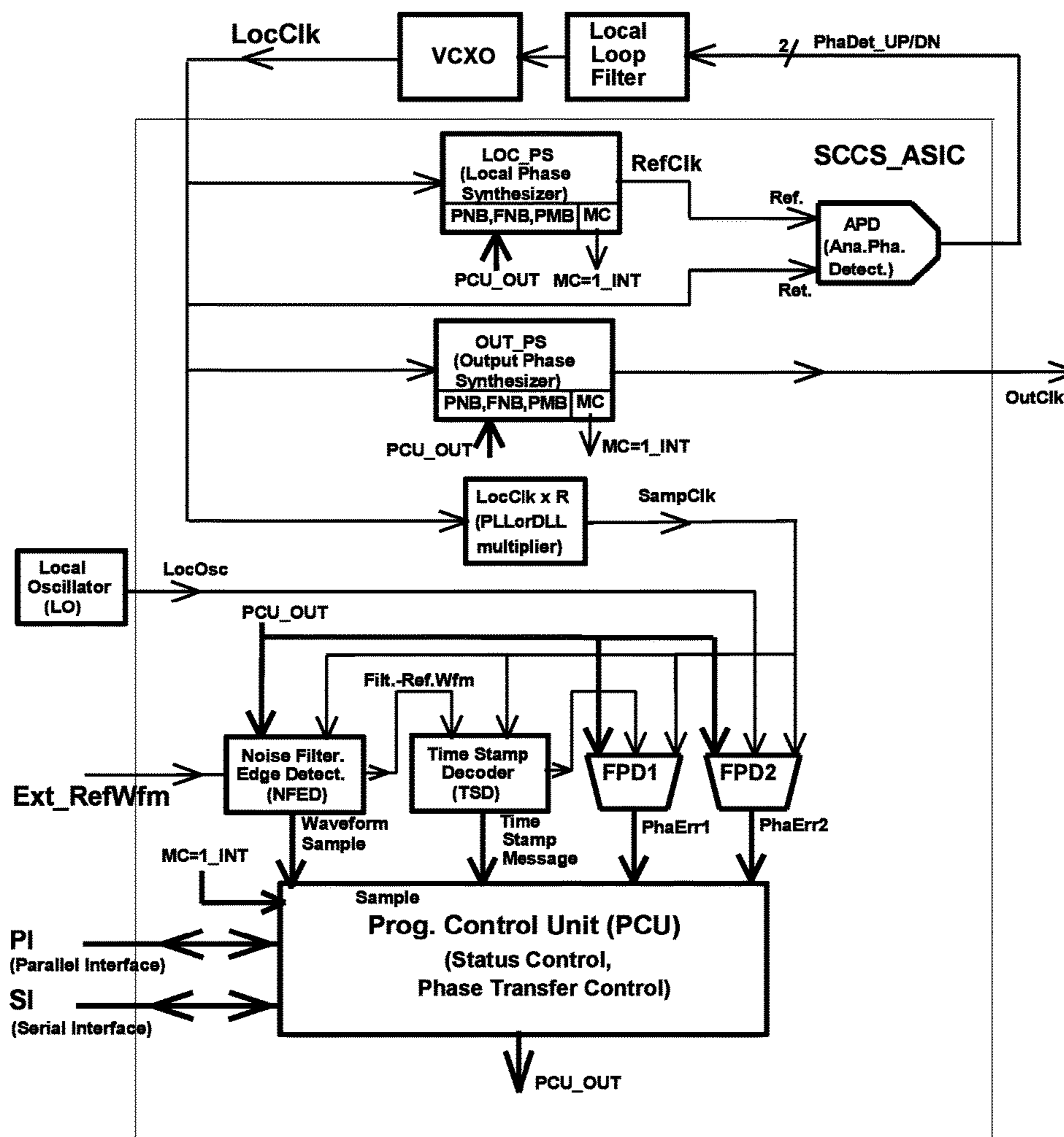
FIG.1 Open Ended Configuration of SCCS
