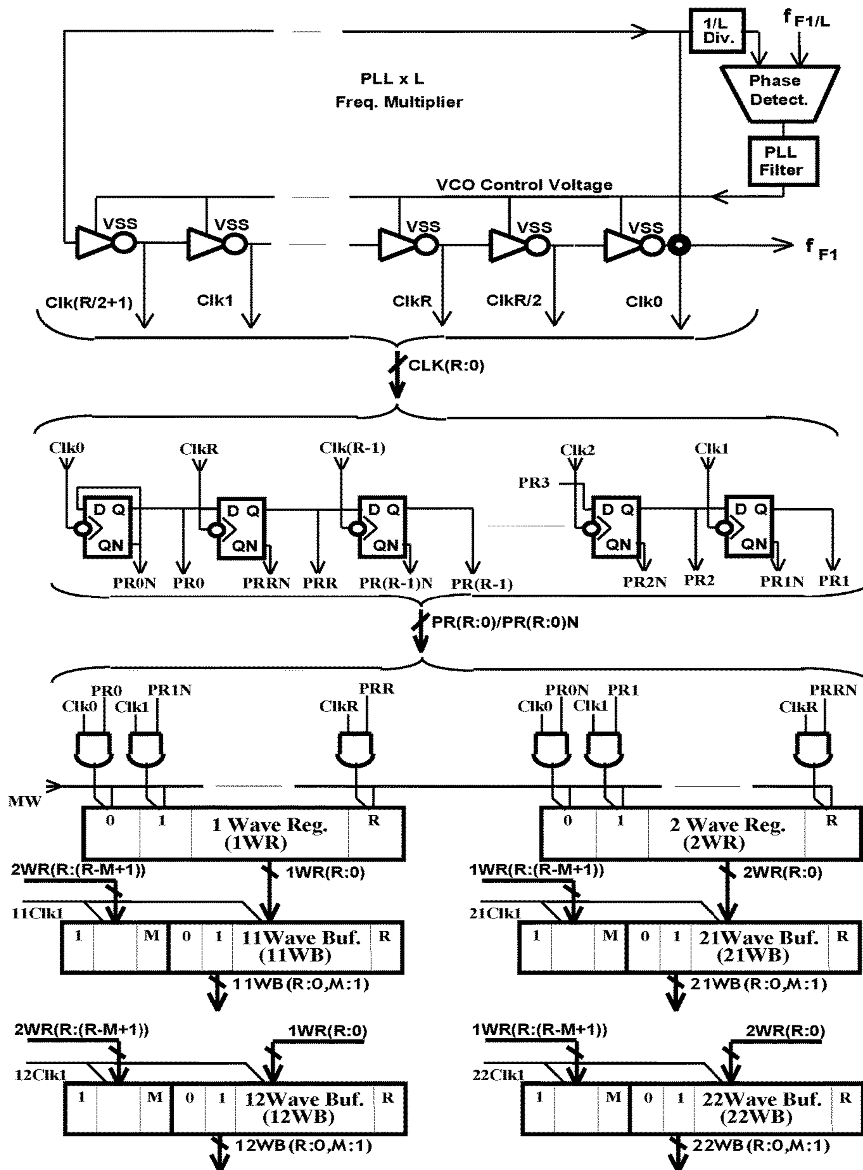
FIG.8 Wave Capturing including Edge Regions (WCER)
