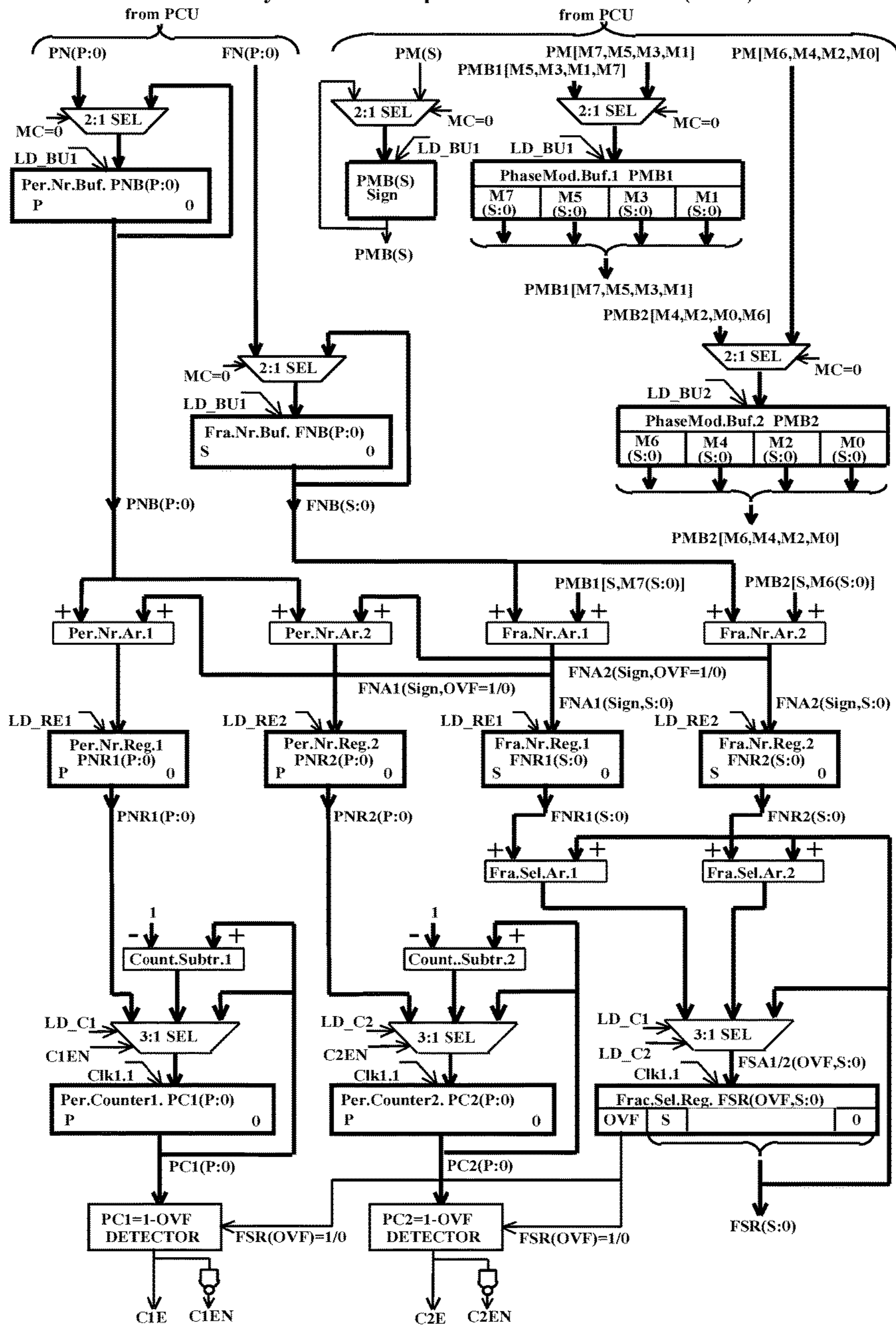
FIG.6 Synchronous Sequential Phase Processor (SSPP)
