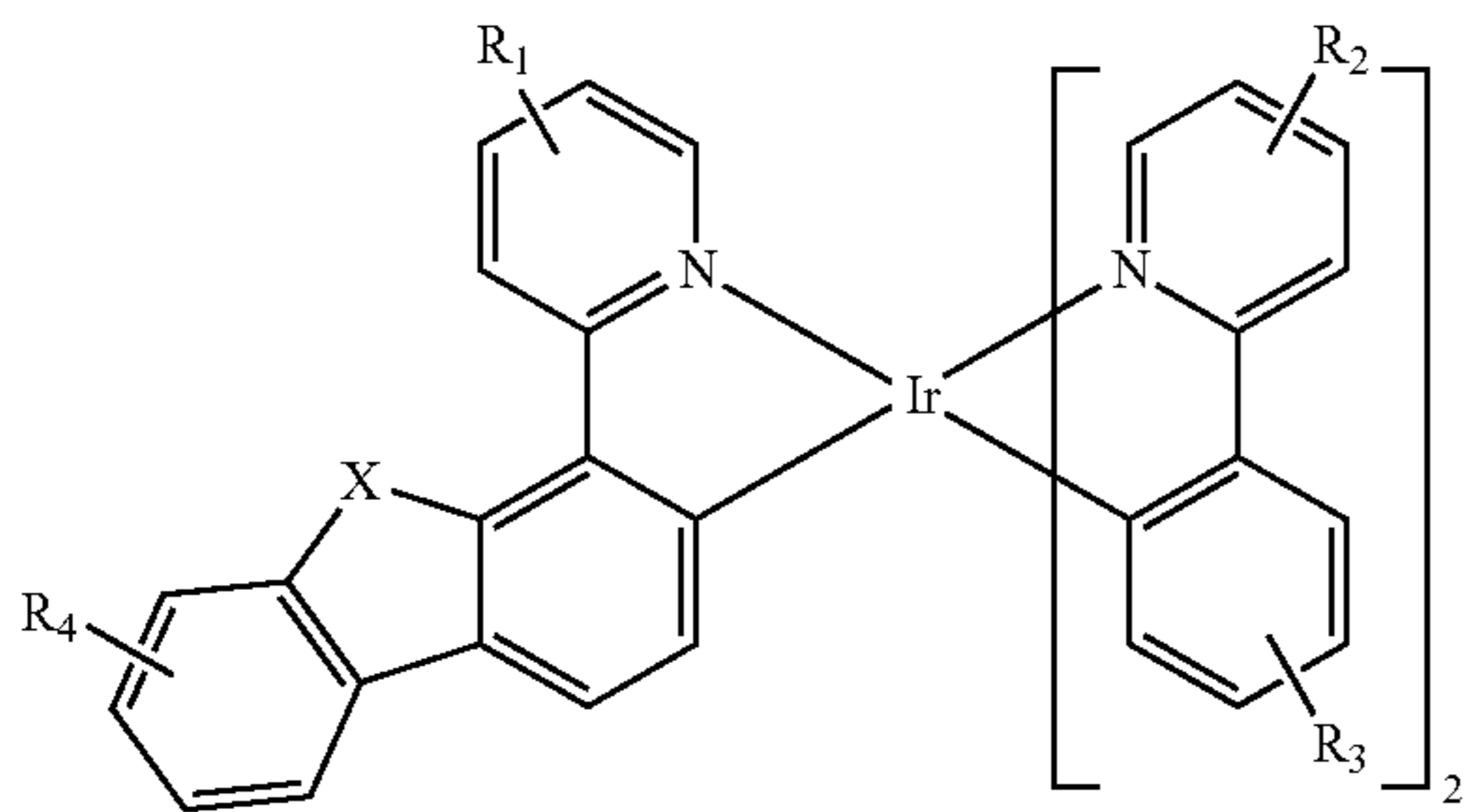
FORMULA IV
