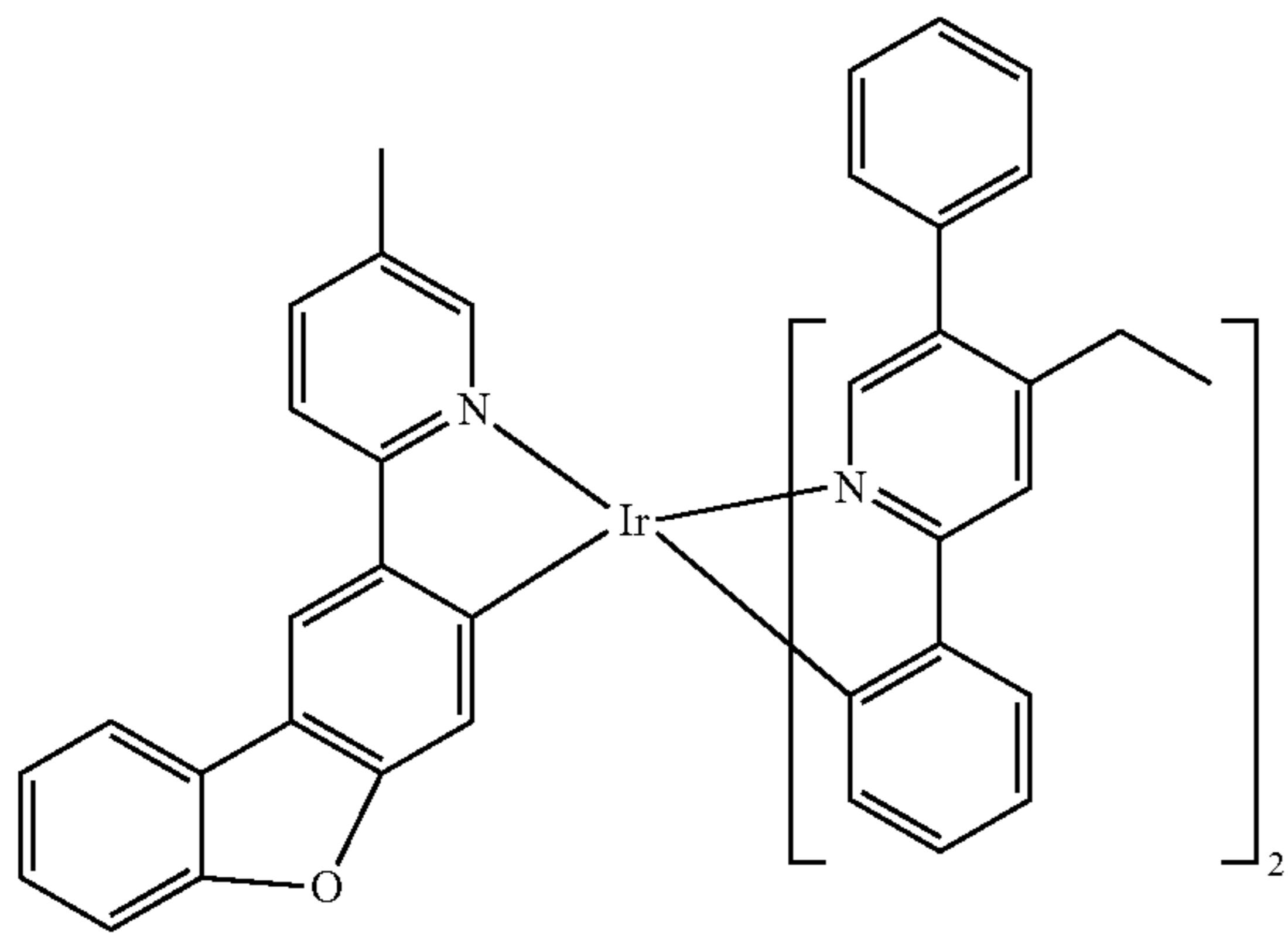
Compound 54
