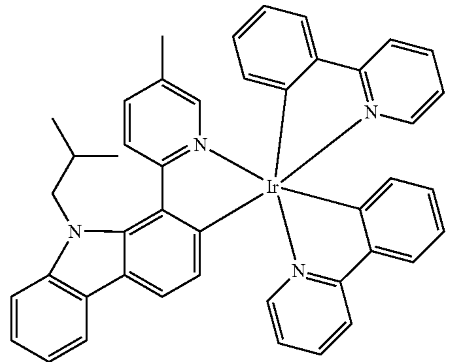
Compound 104
