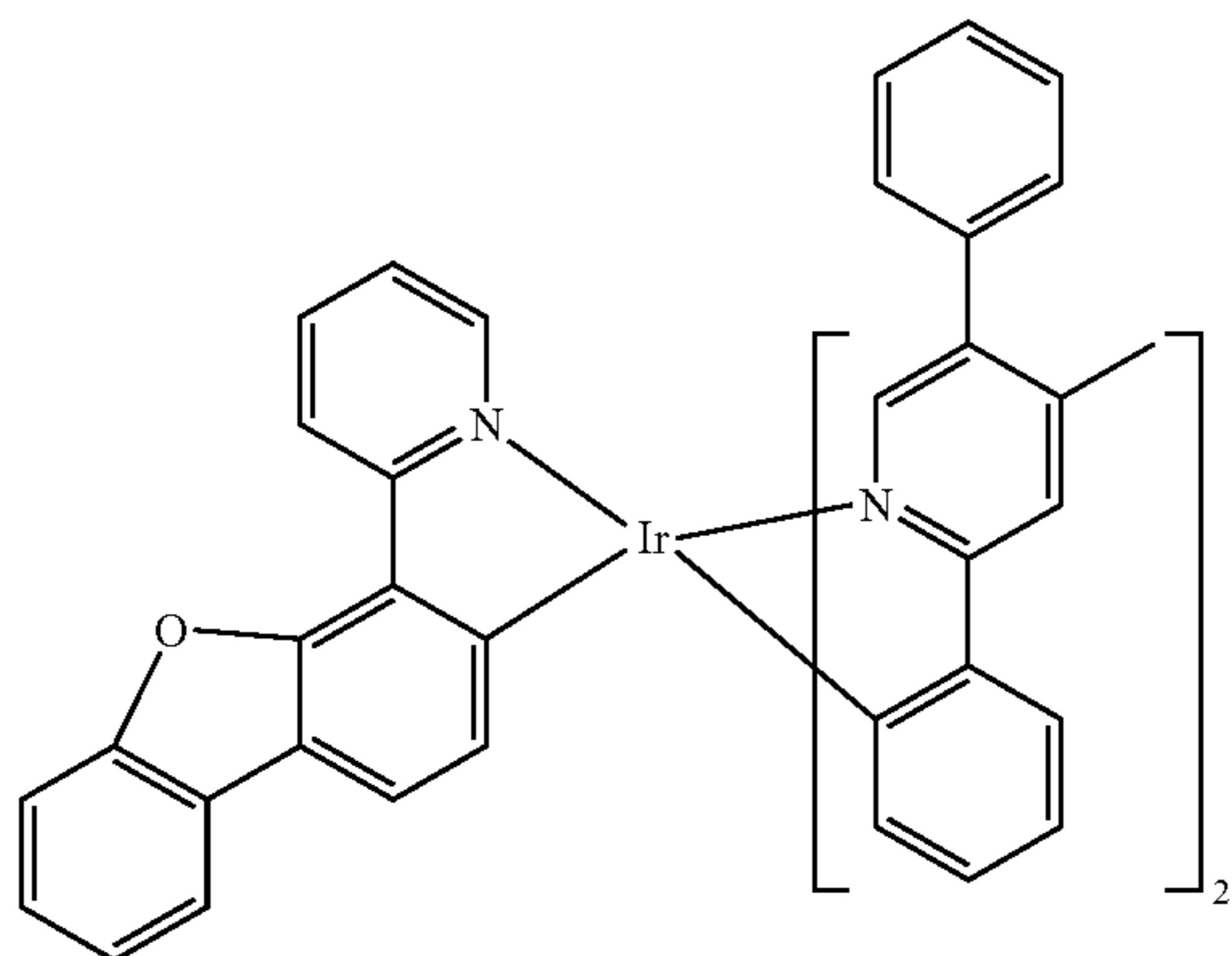
Compound 37
