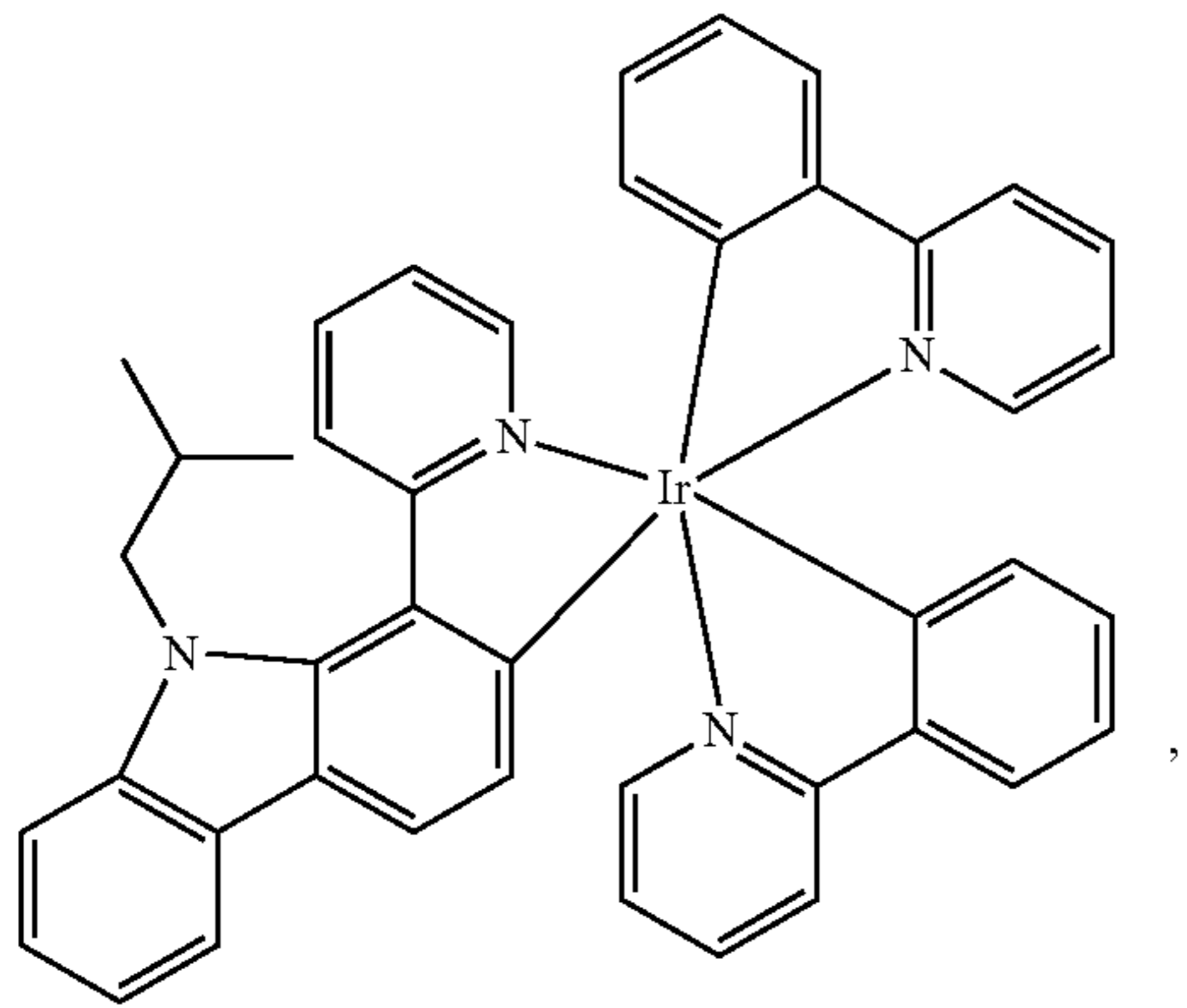
Compound 25
