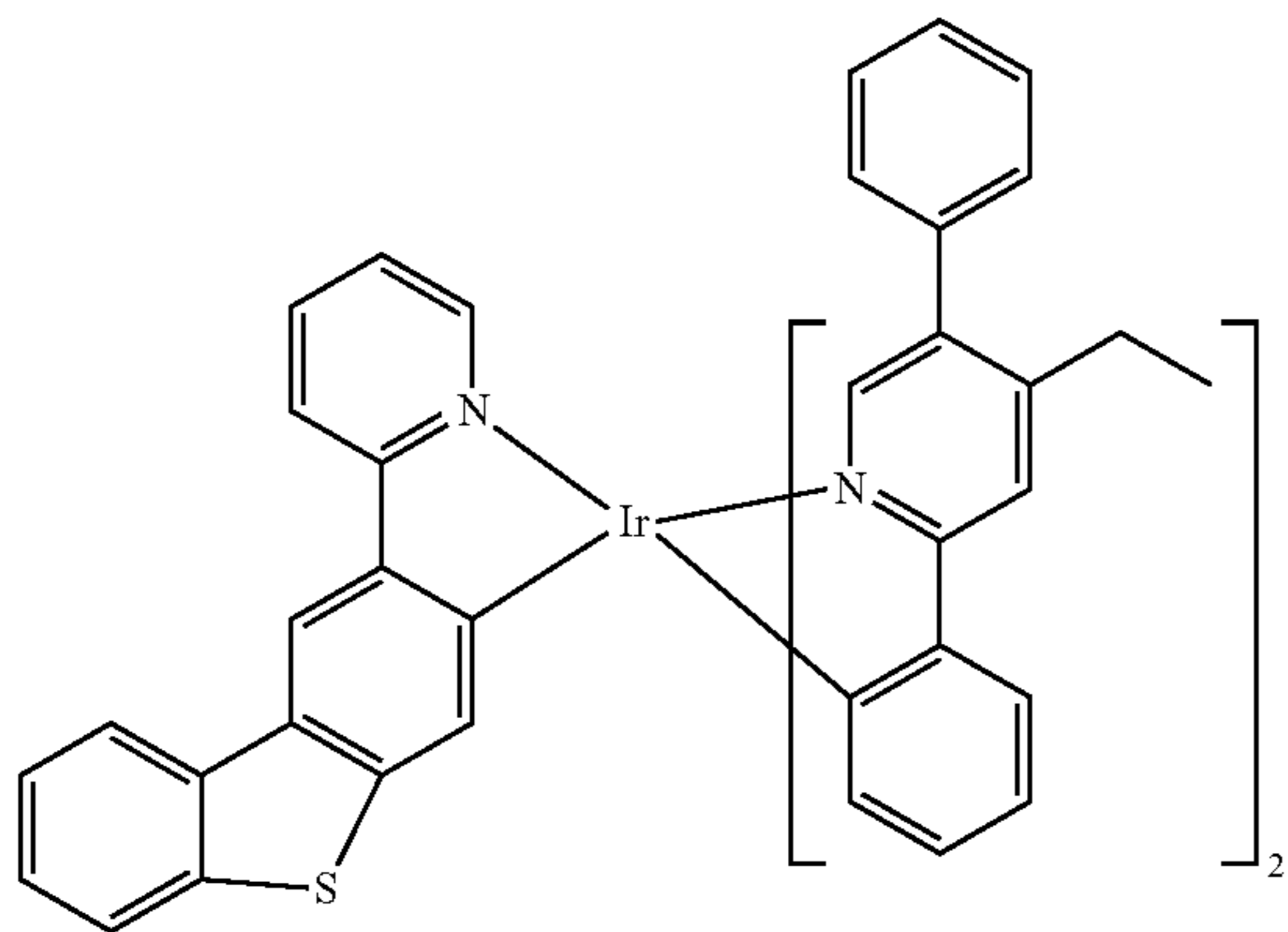
Compound 72
