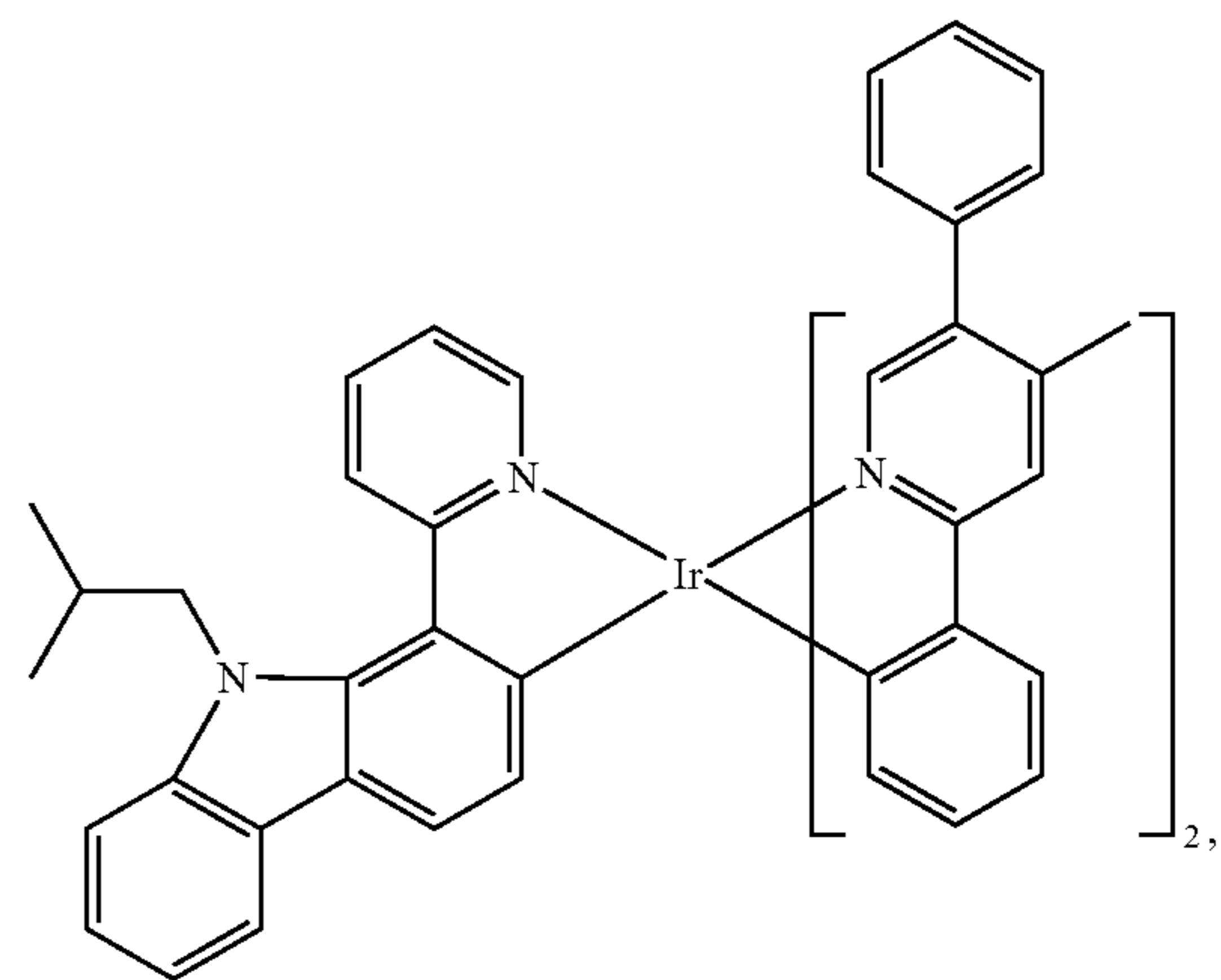
Compound 85
