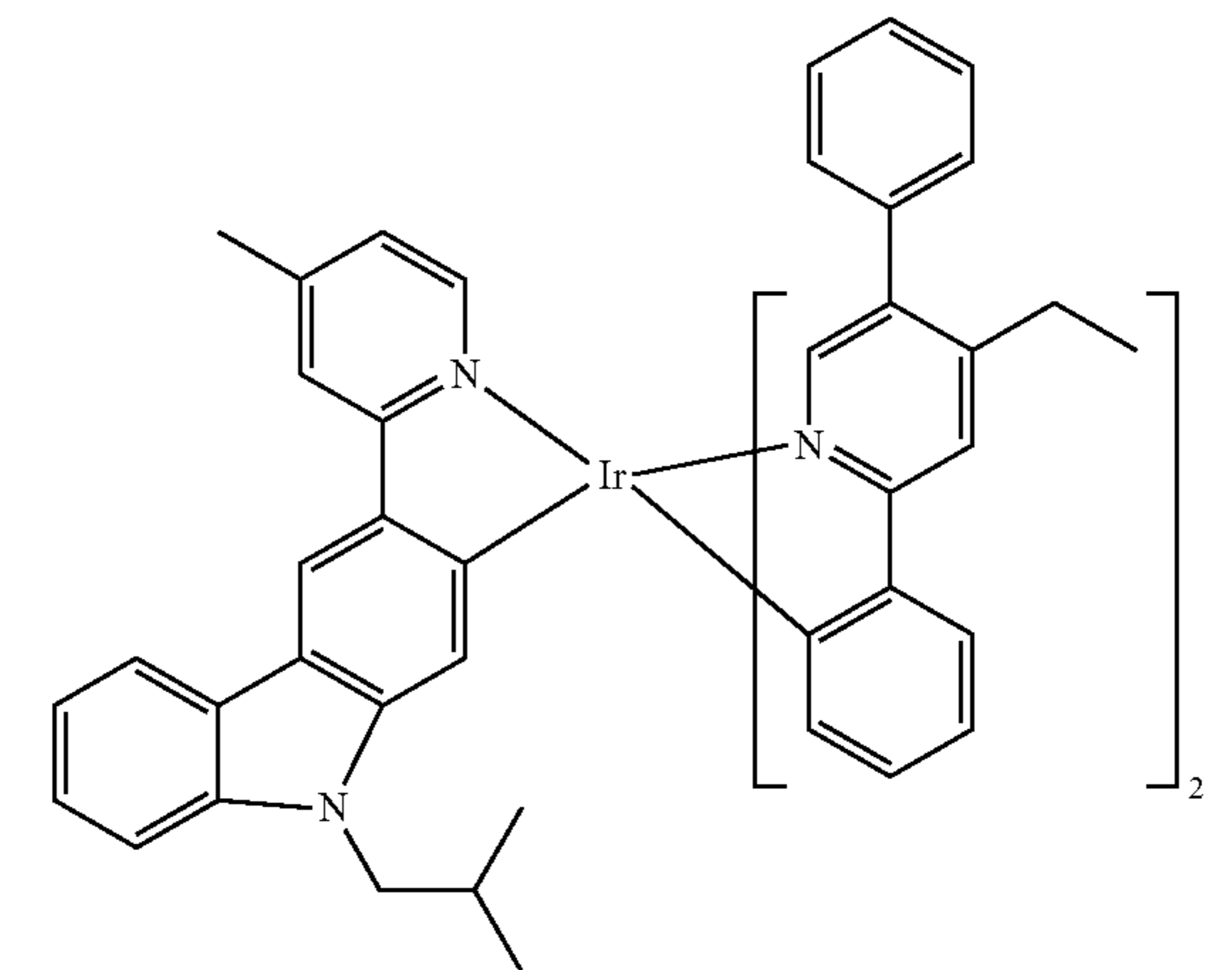
Compound 99
