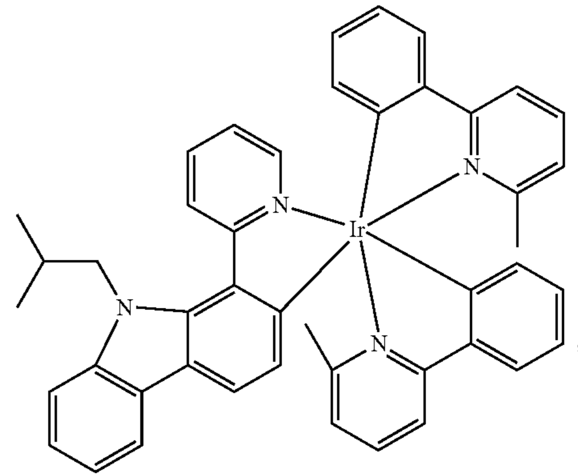
Compound 28
