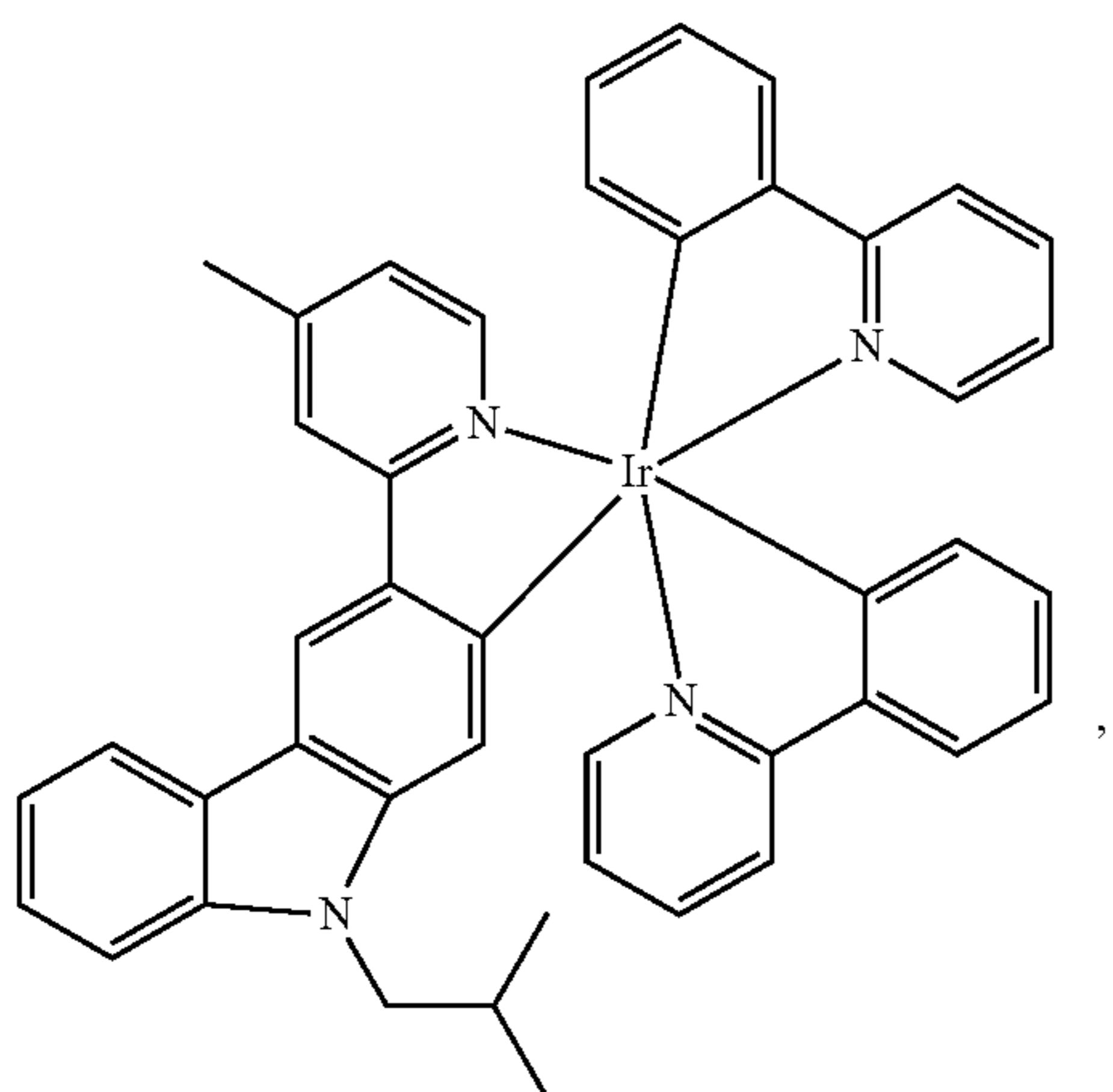
Compound 33
