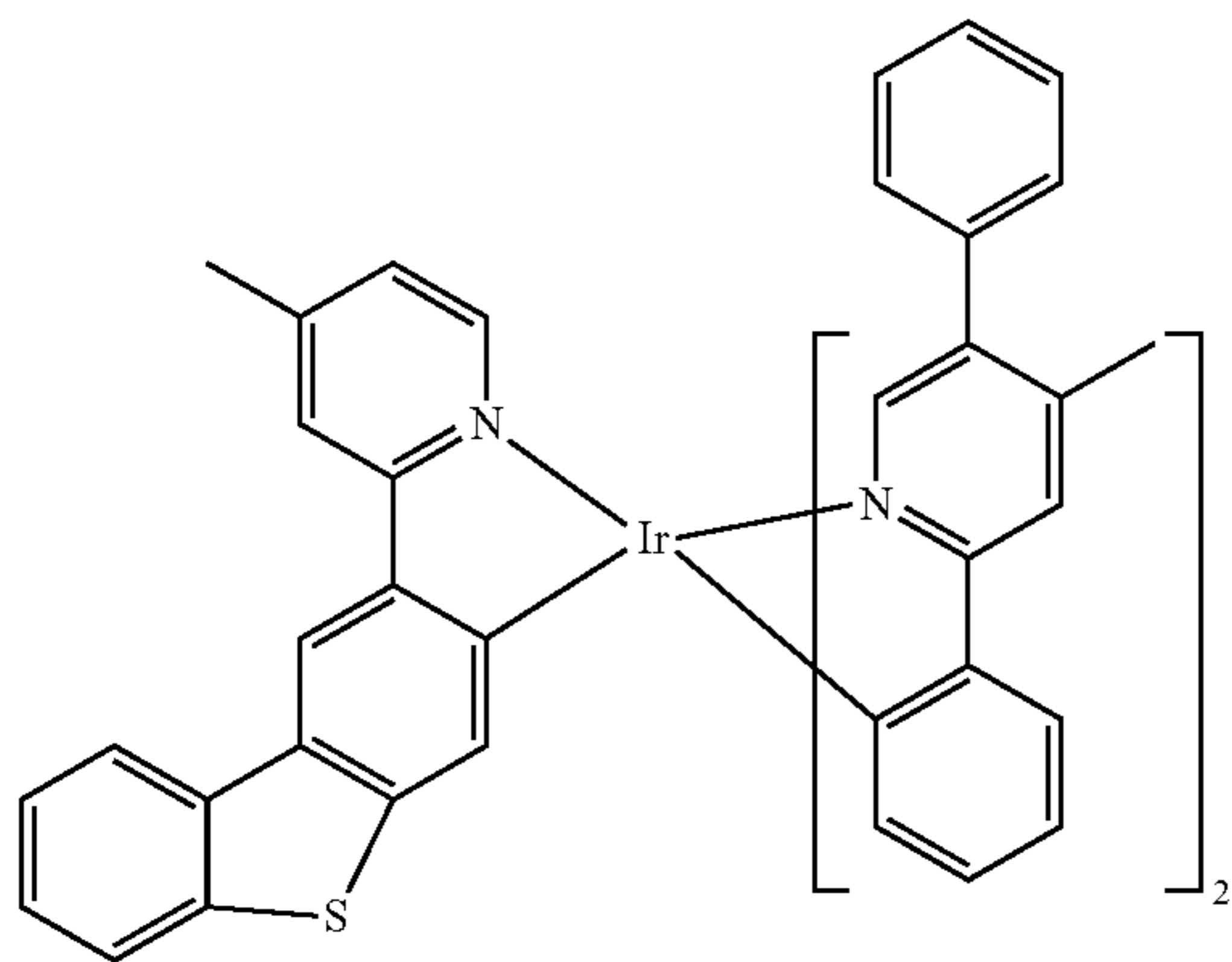
Compound 66
