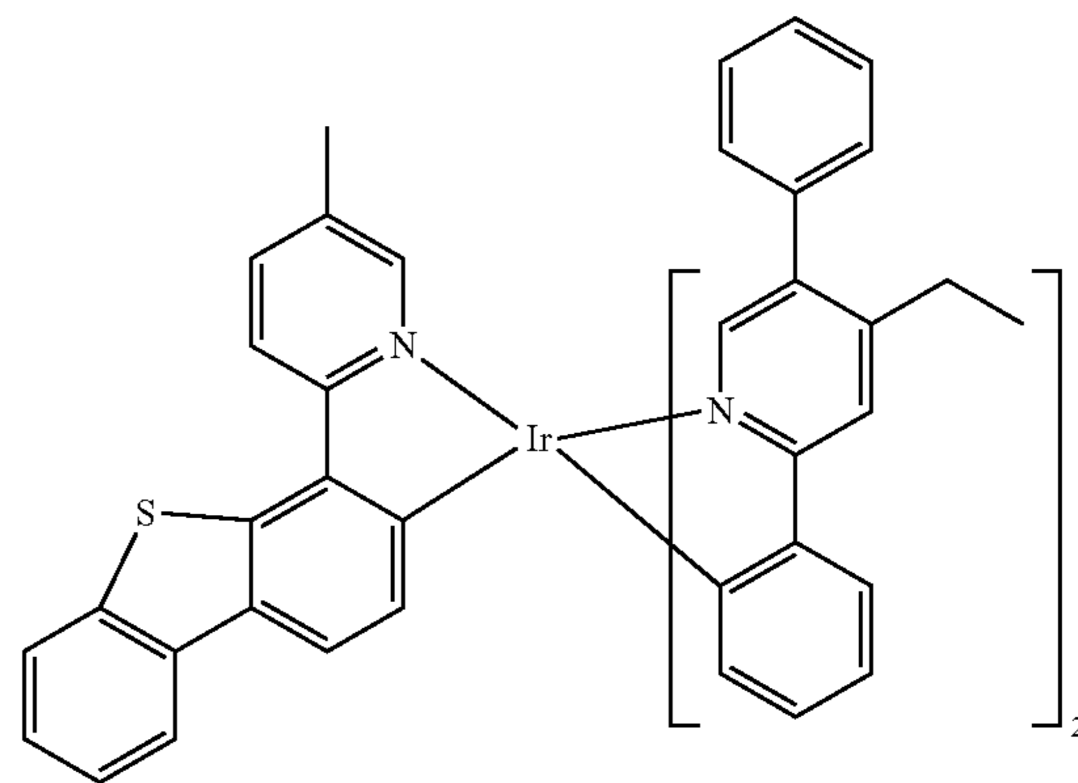
Compound 76
