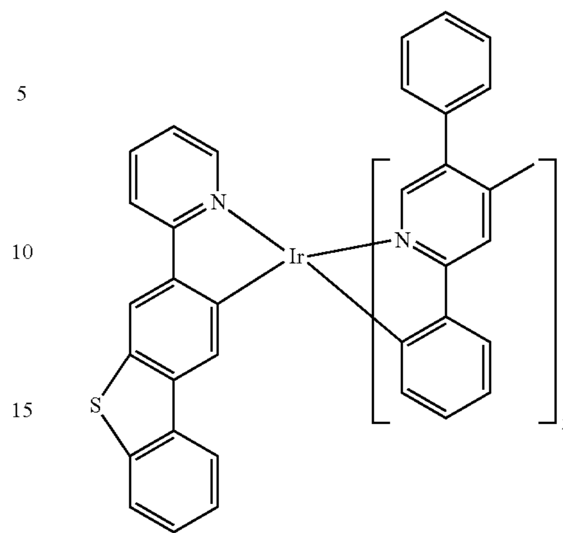
Compound 59
