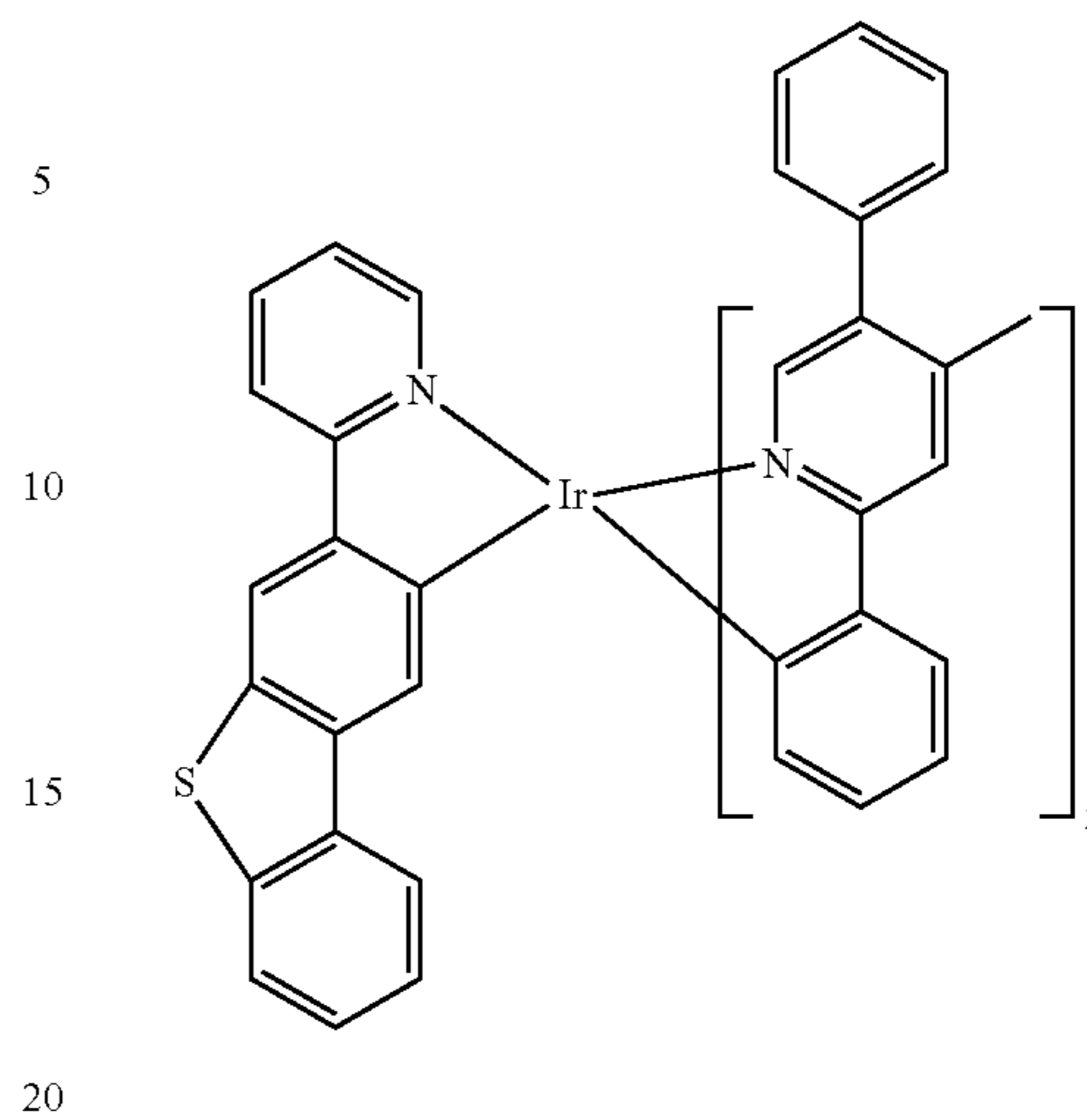
Compound 59
