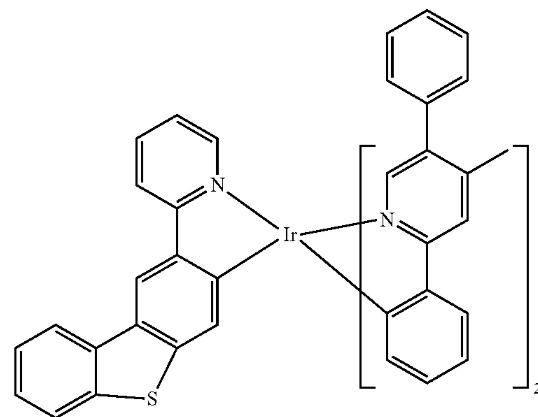
Compound 63
