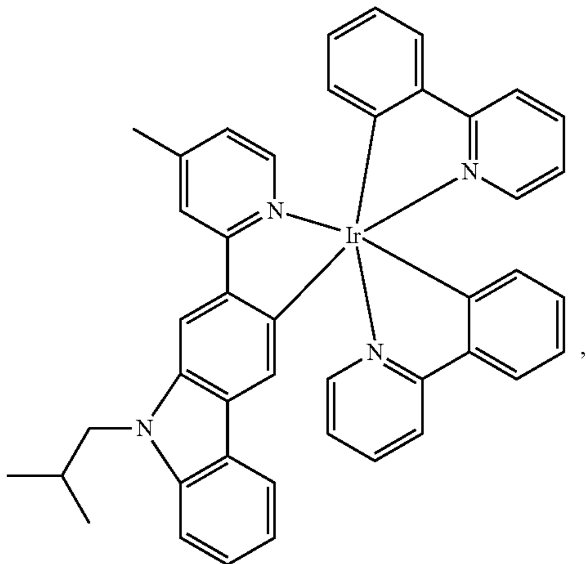
Compound 32
