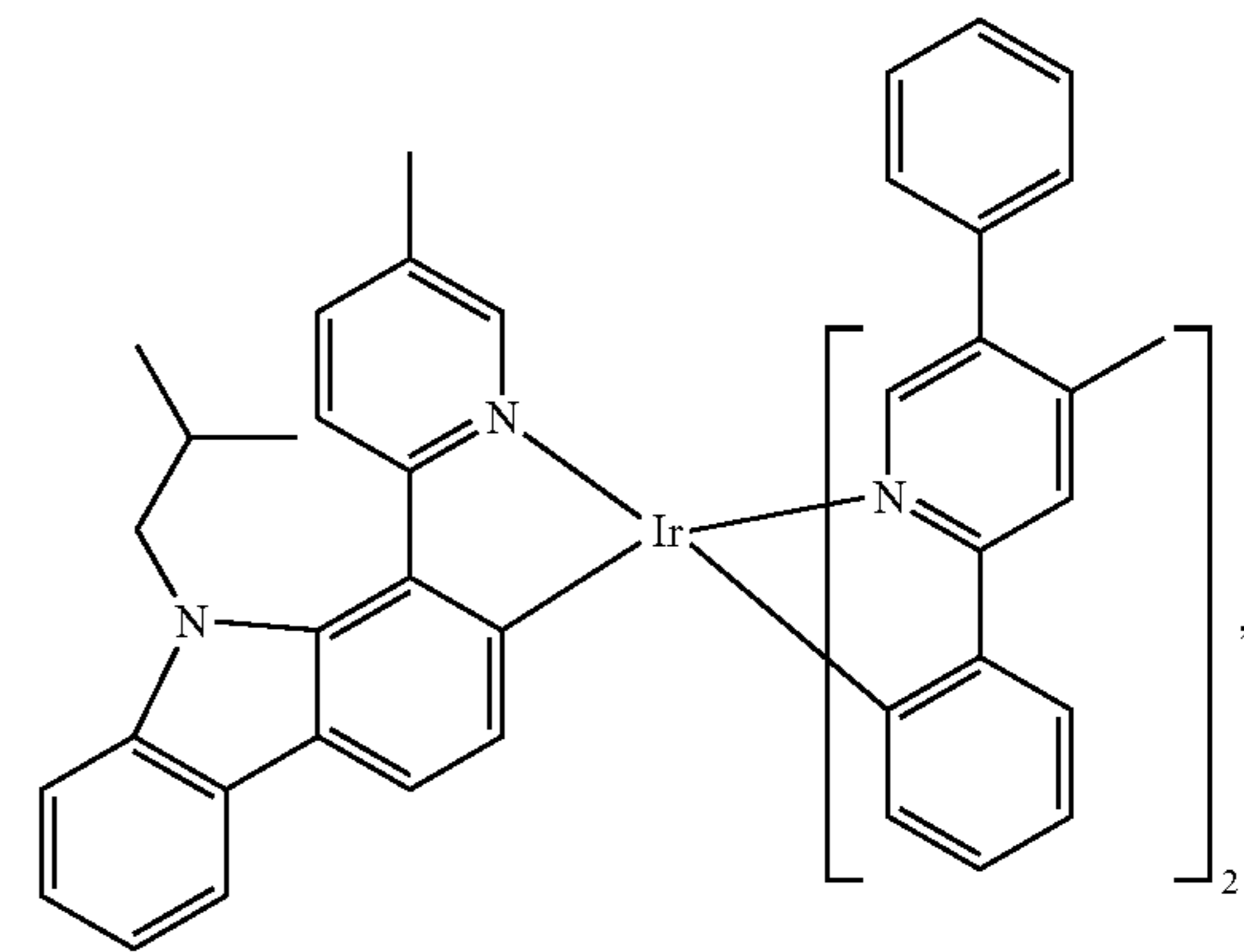
Compound 91
