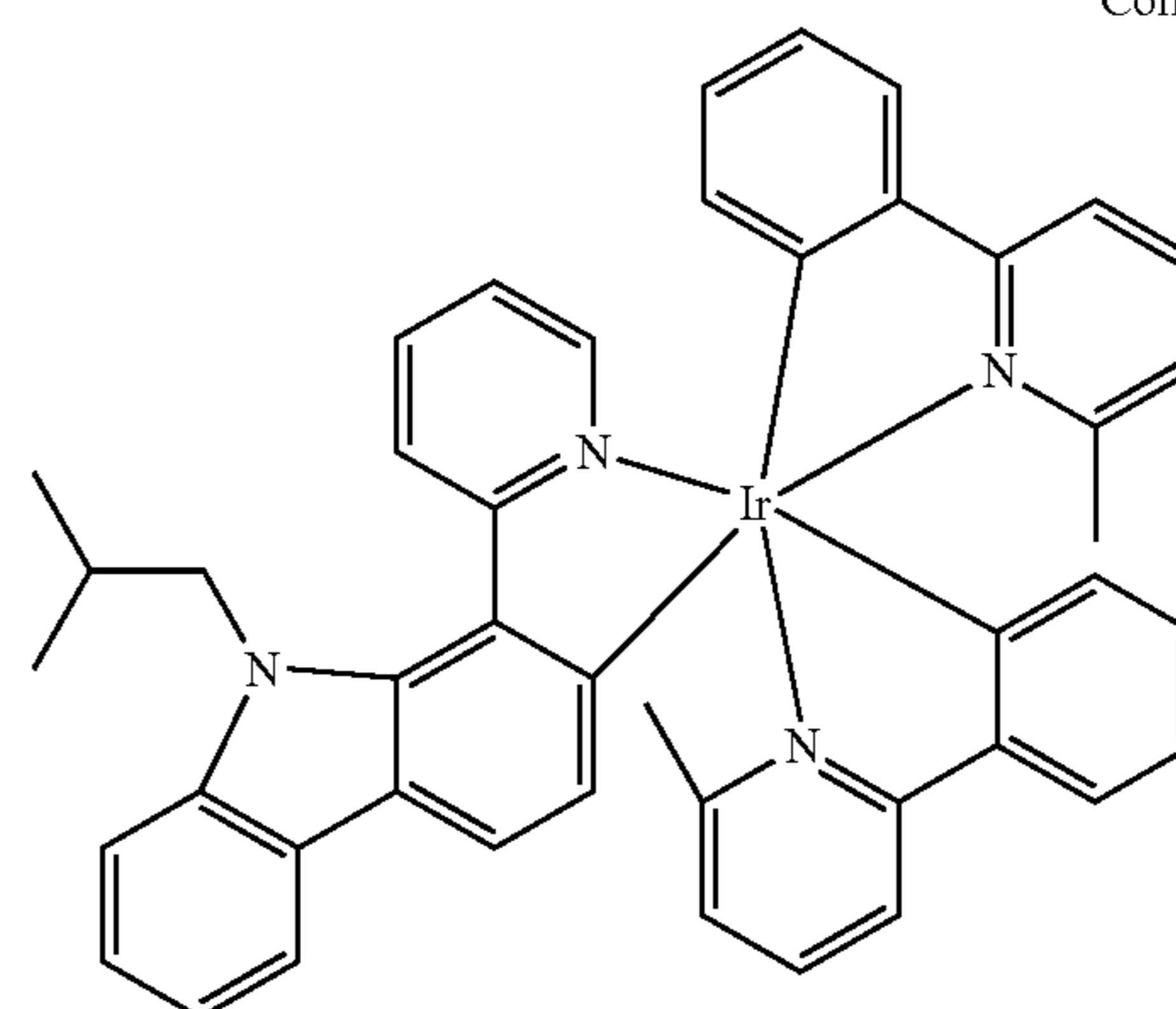
Compound 28
