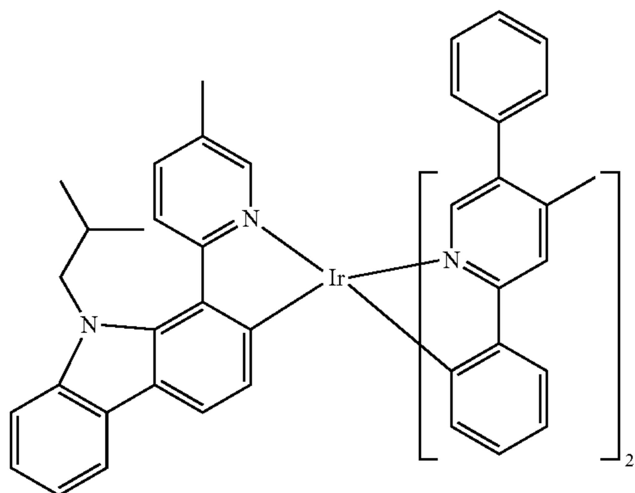
Compound 91
