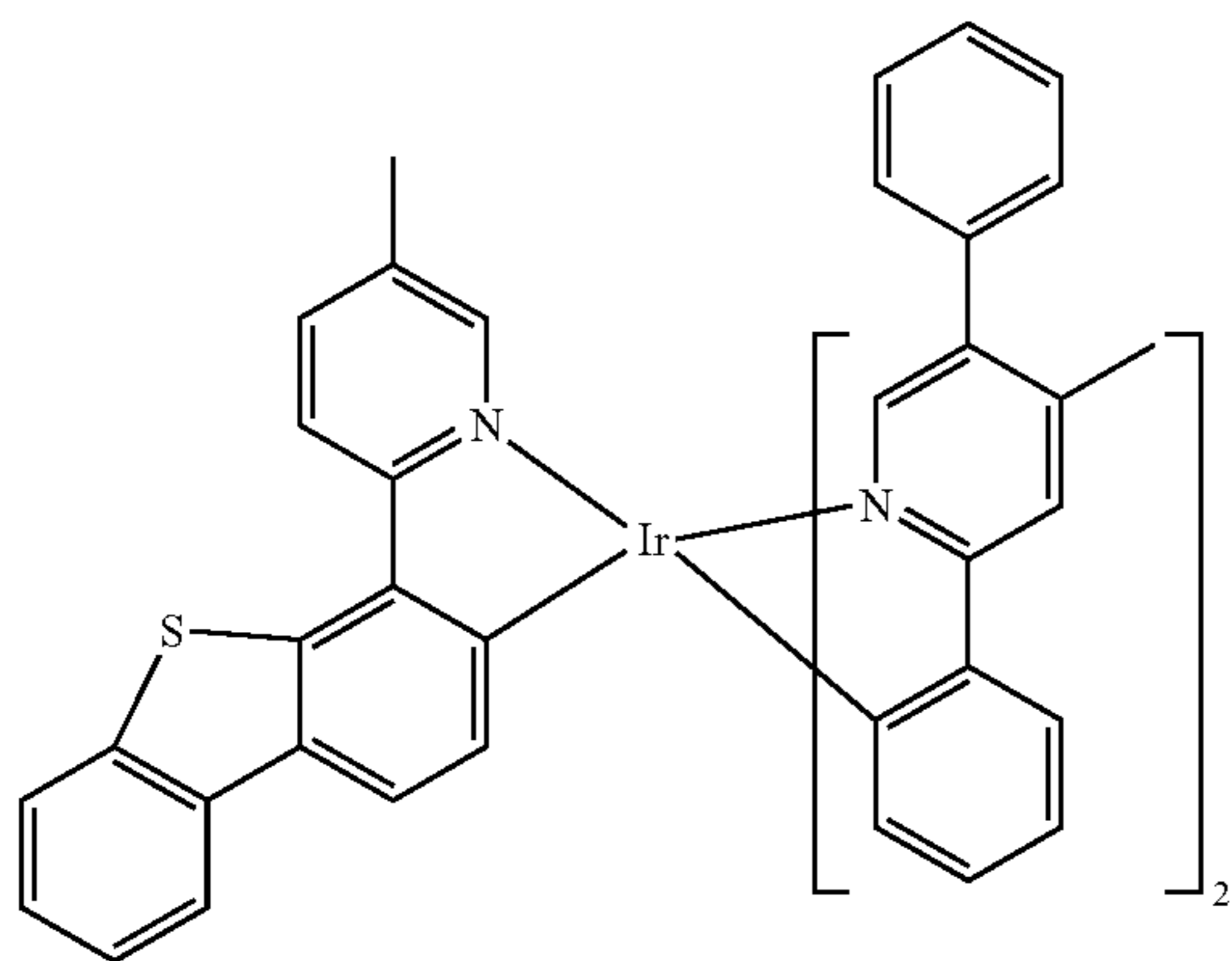
Compound 67
