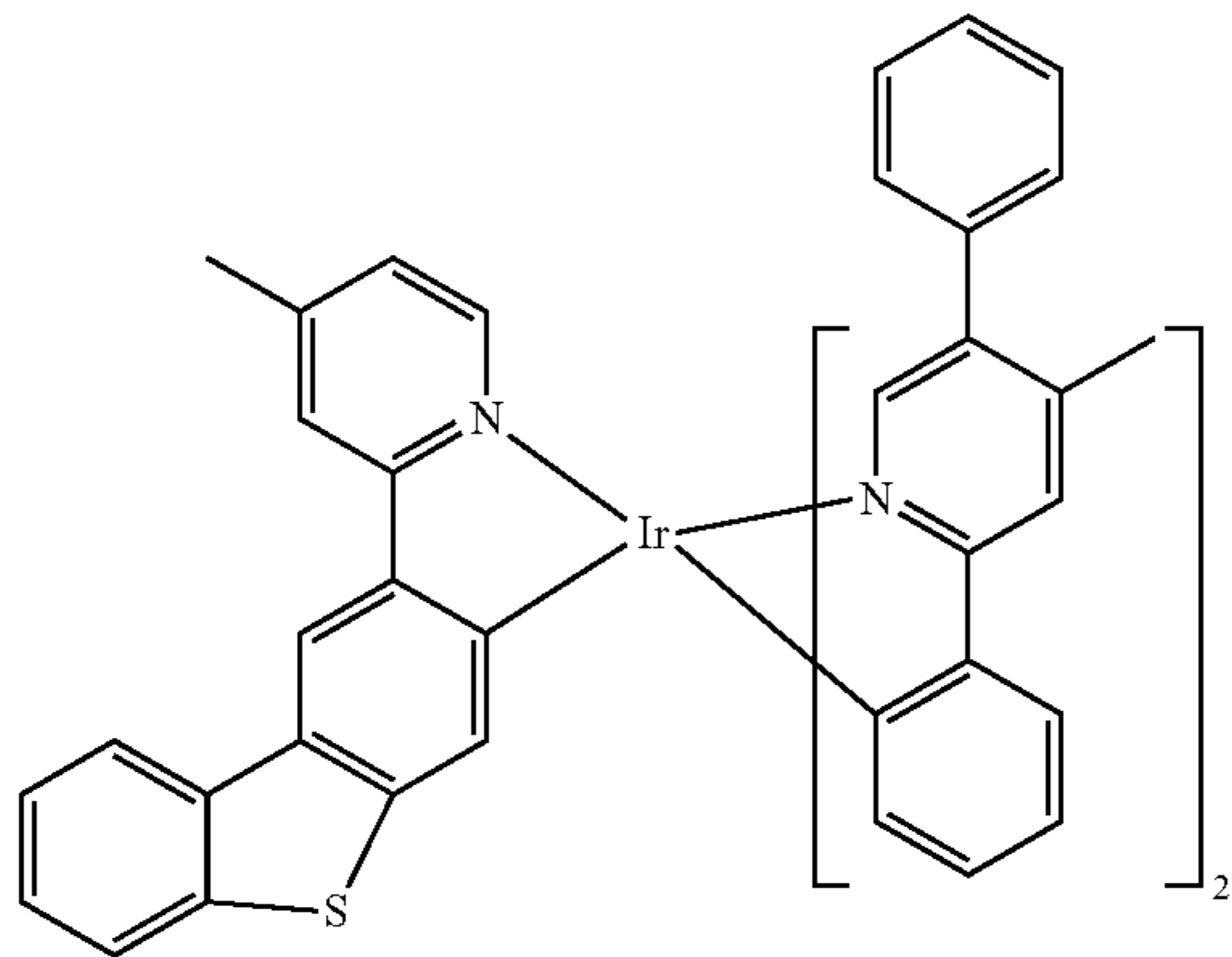
Compound 66
