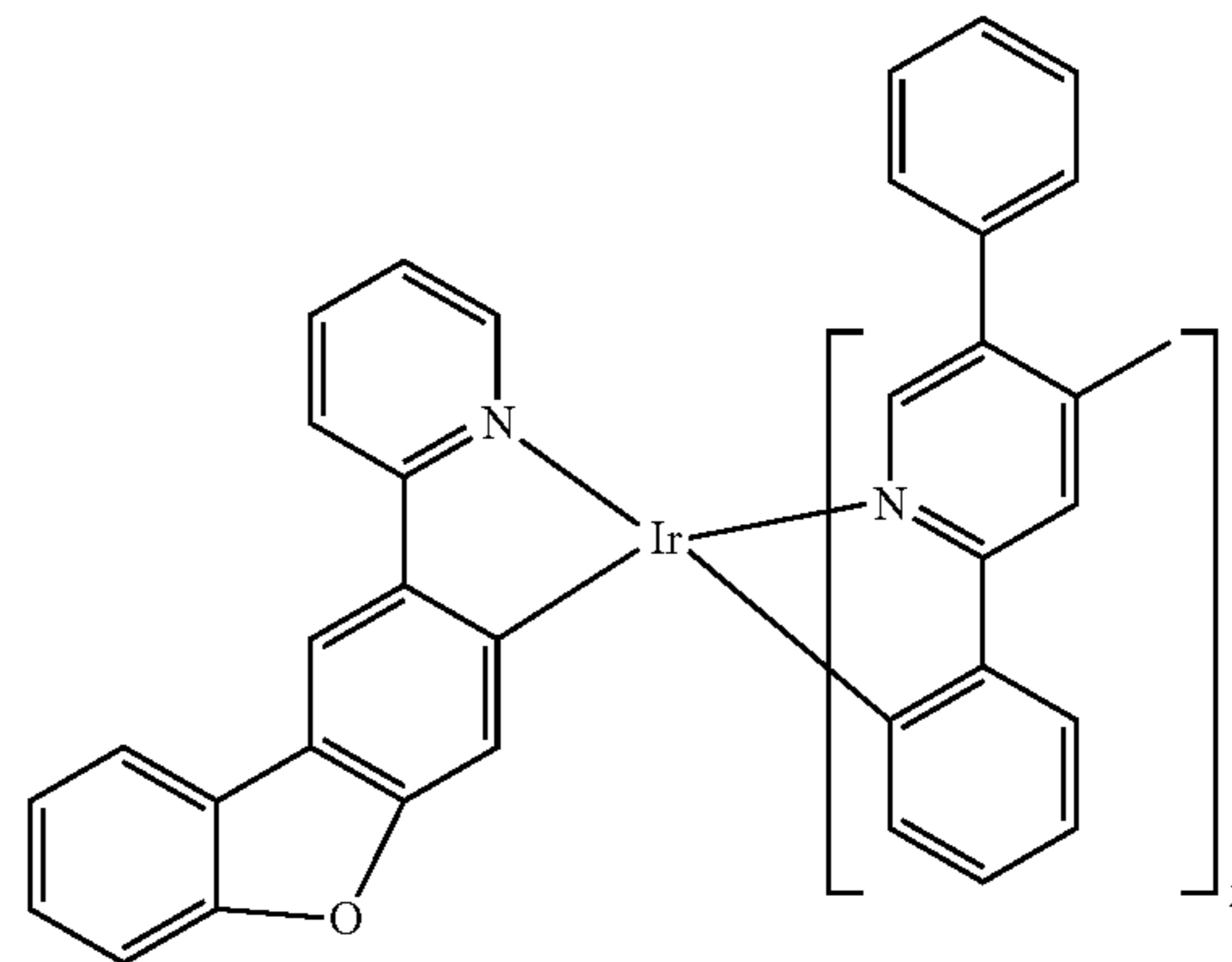
Compound 39
