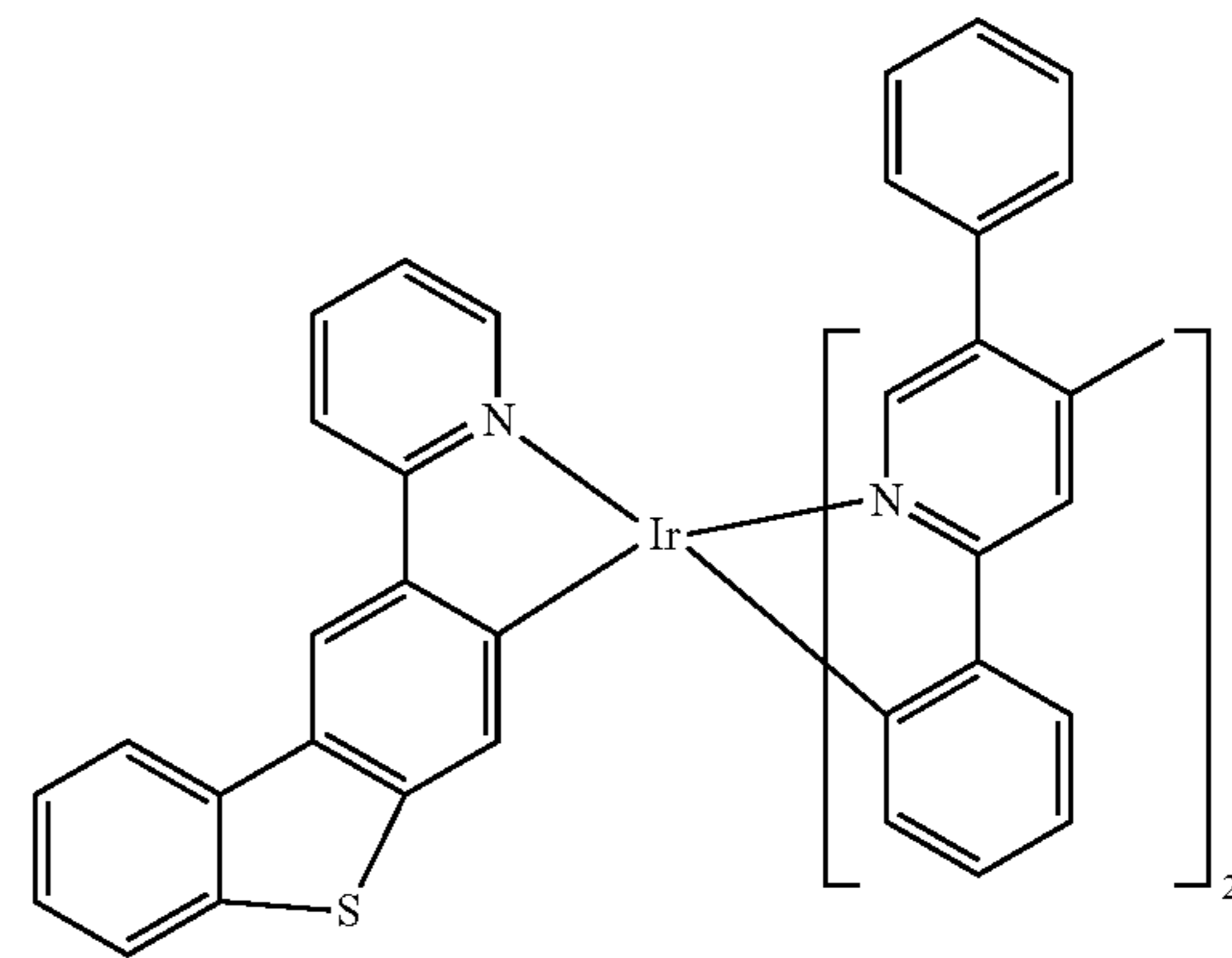
Compound 63
