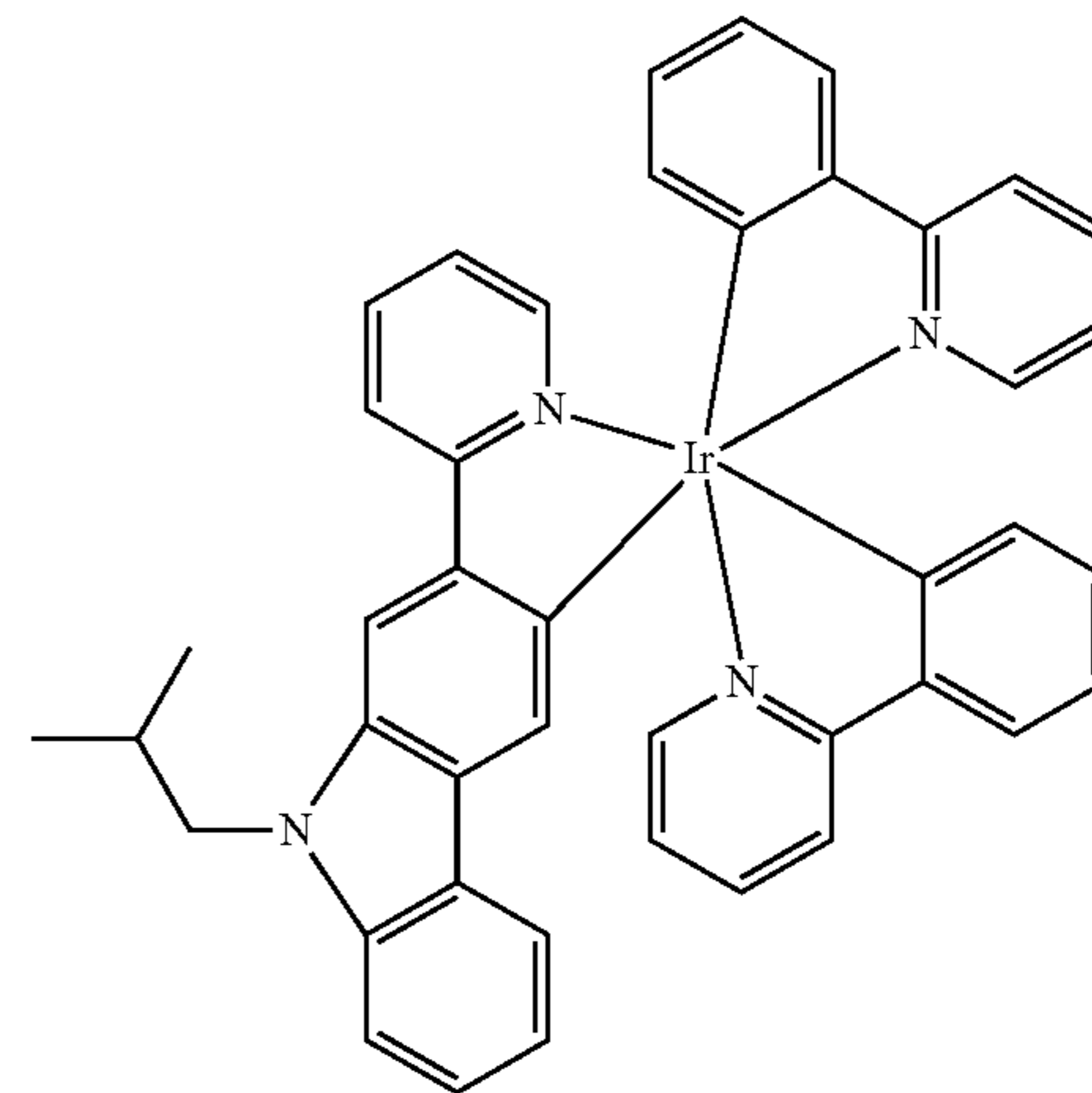
Compound 26
