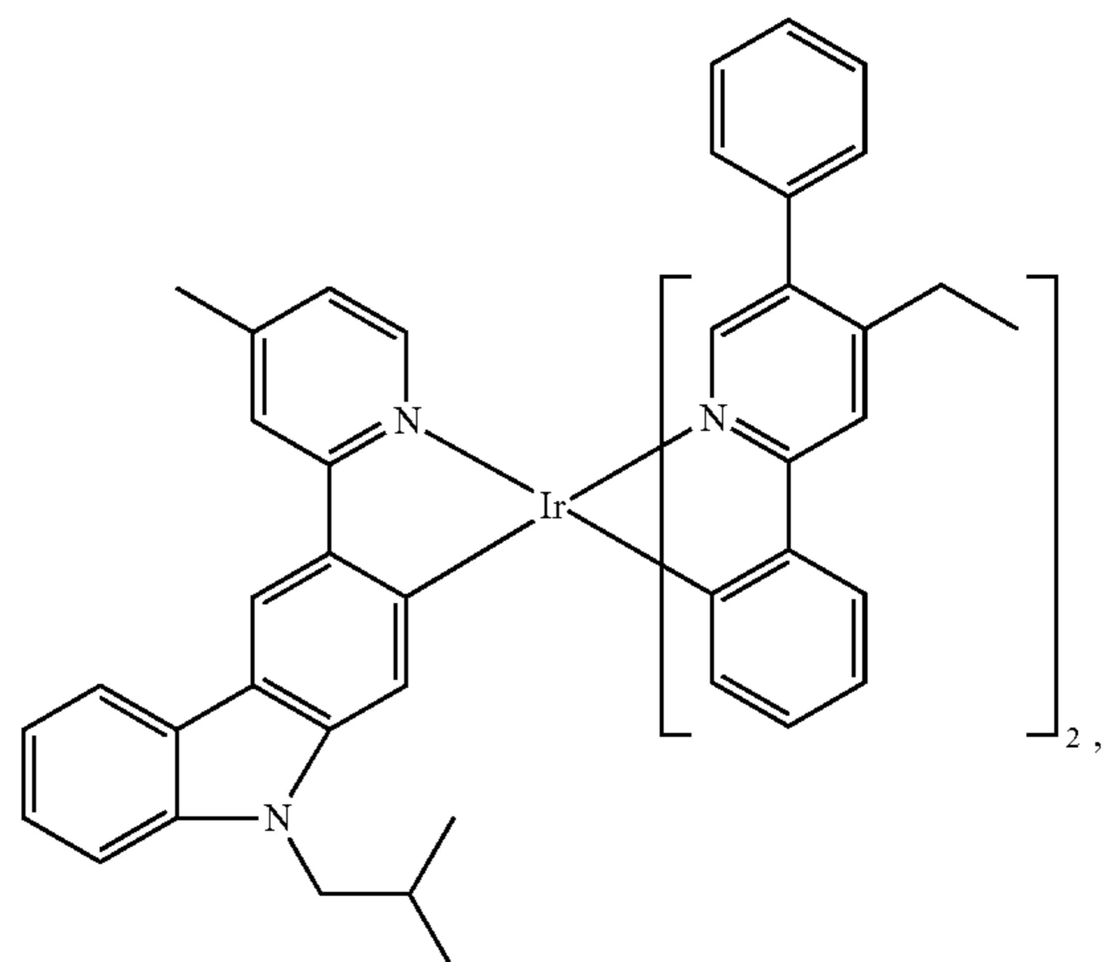
Compound 99
