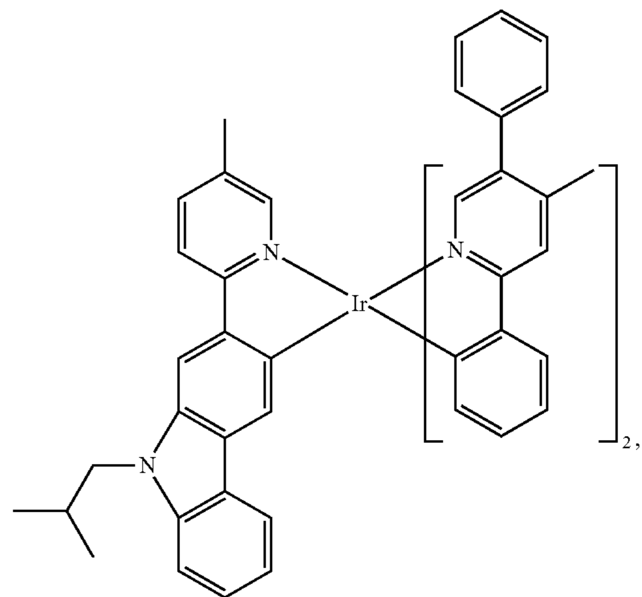
Compound 92
