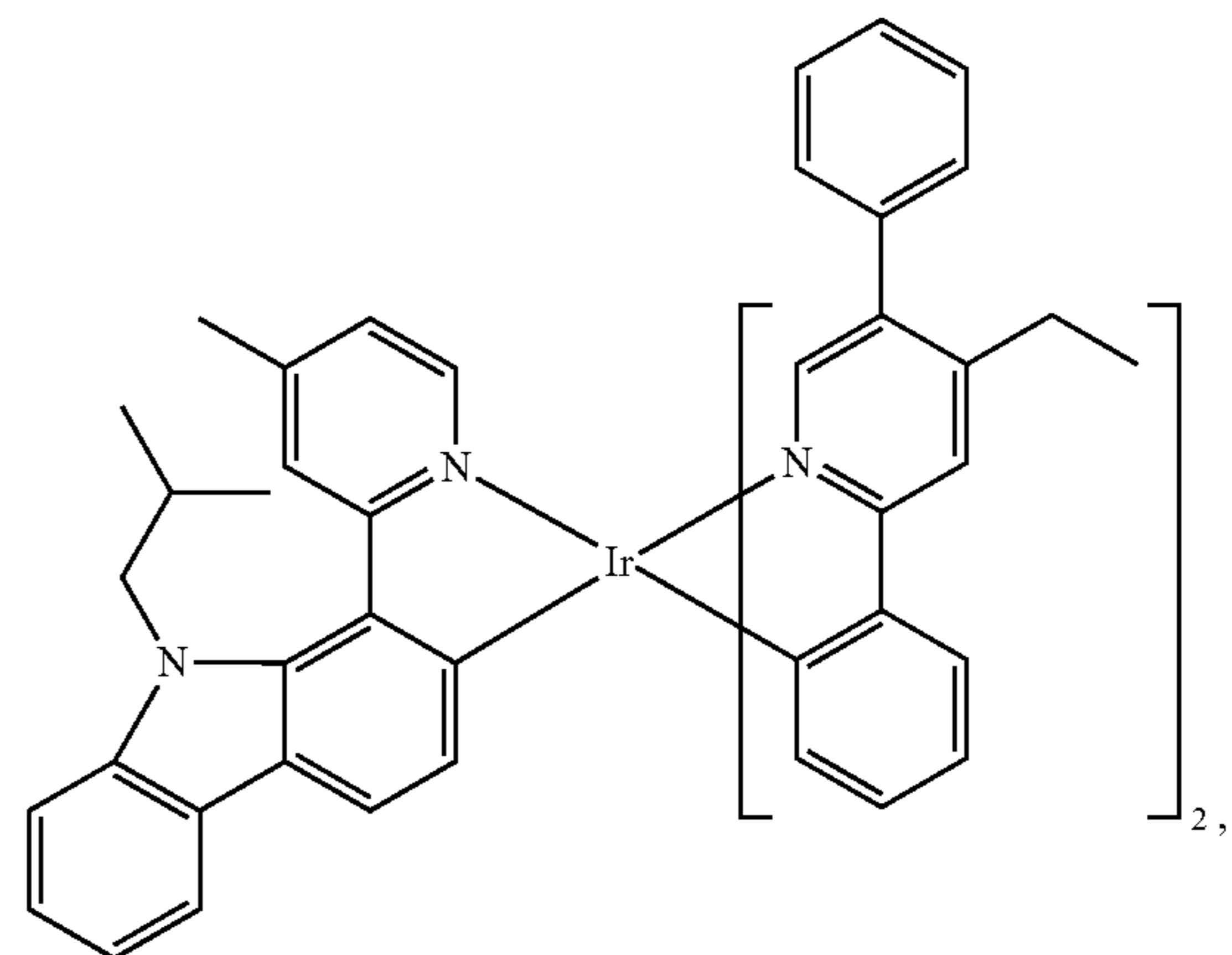
Compound 97
