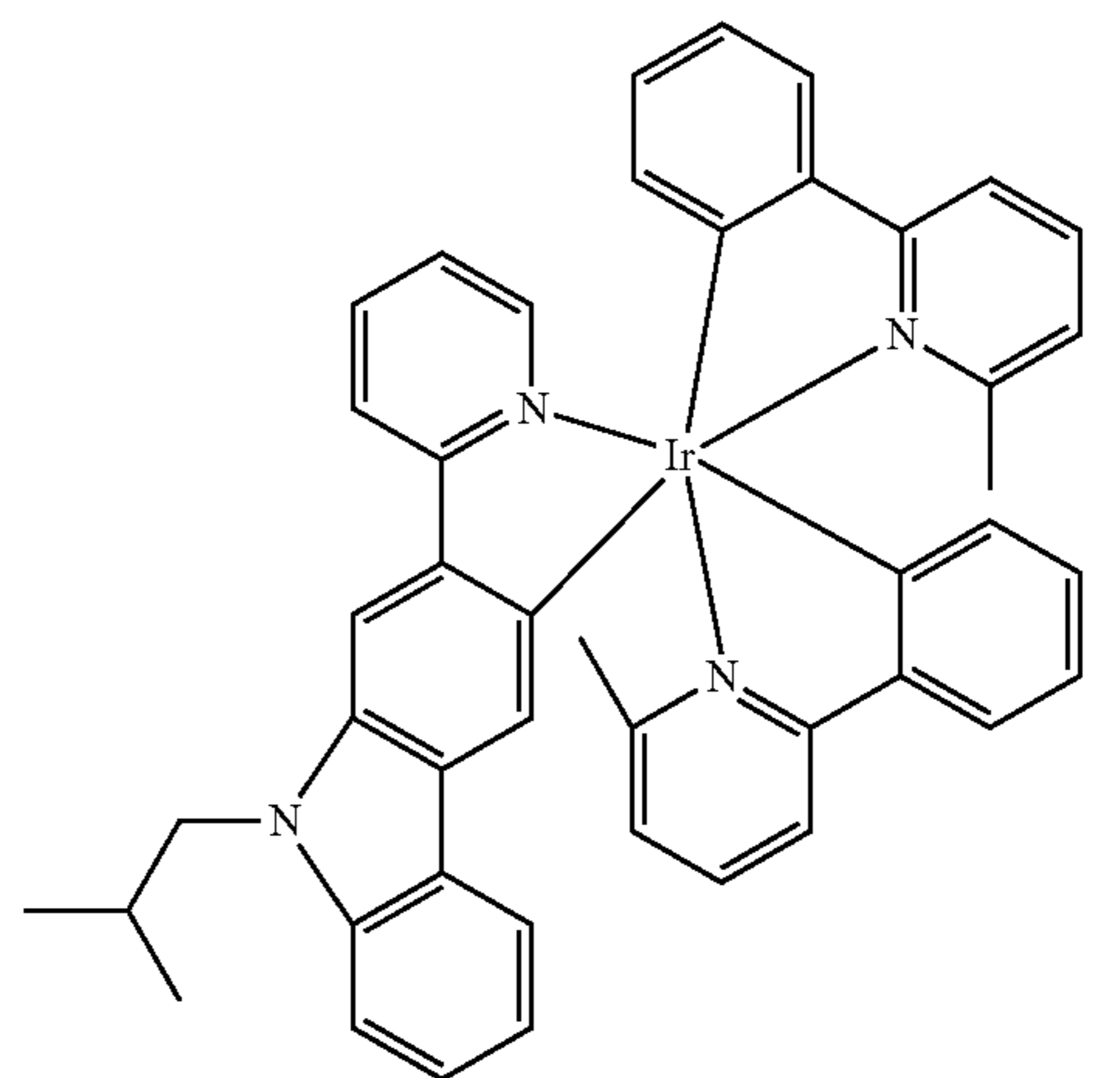
Compound 29
