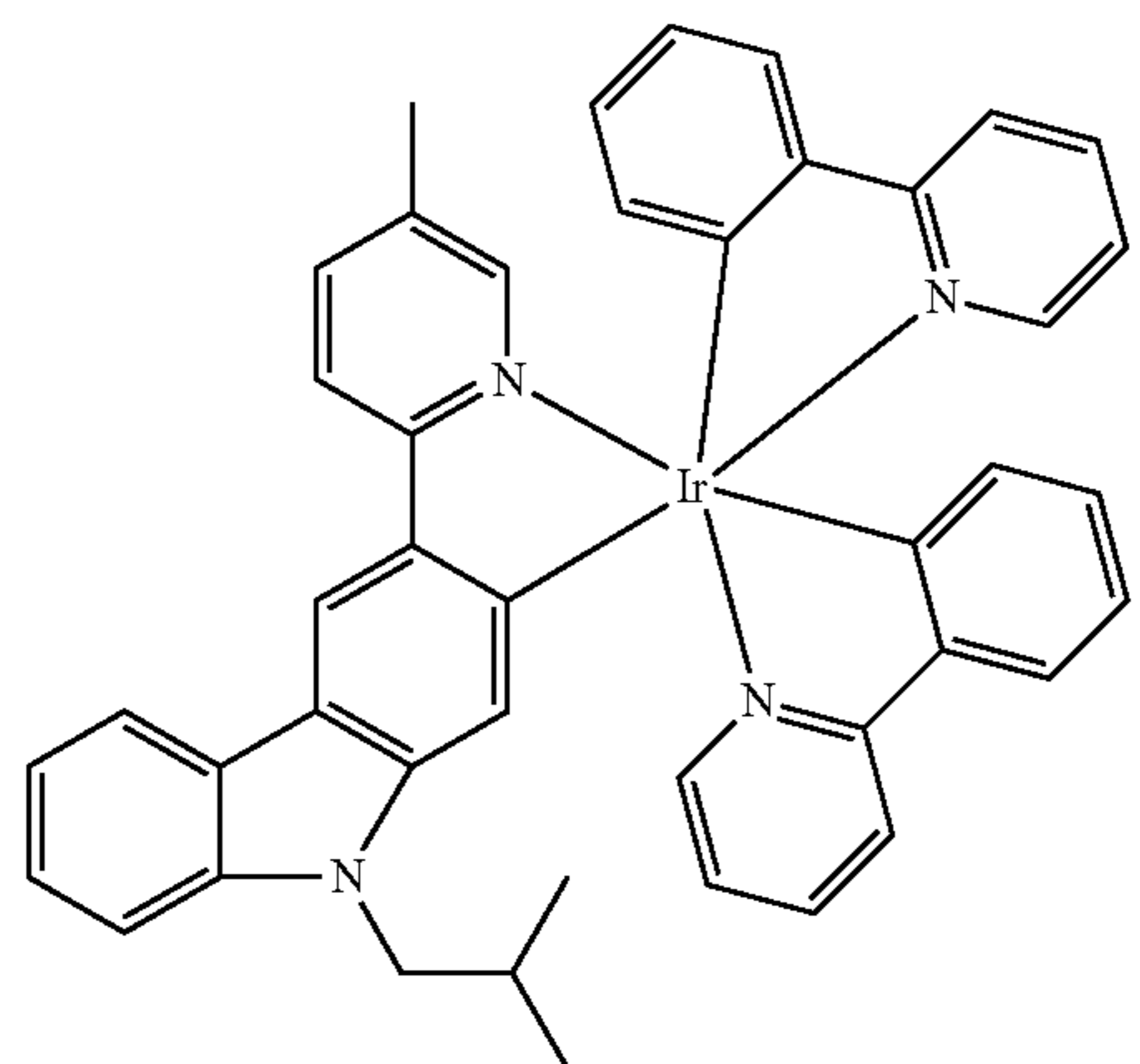
Compound 106
