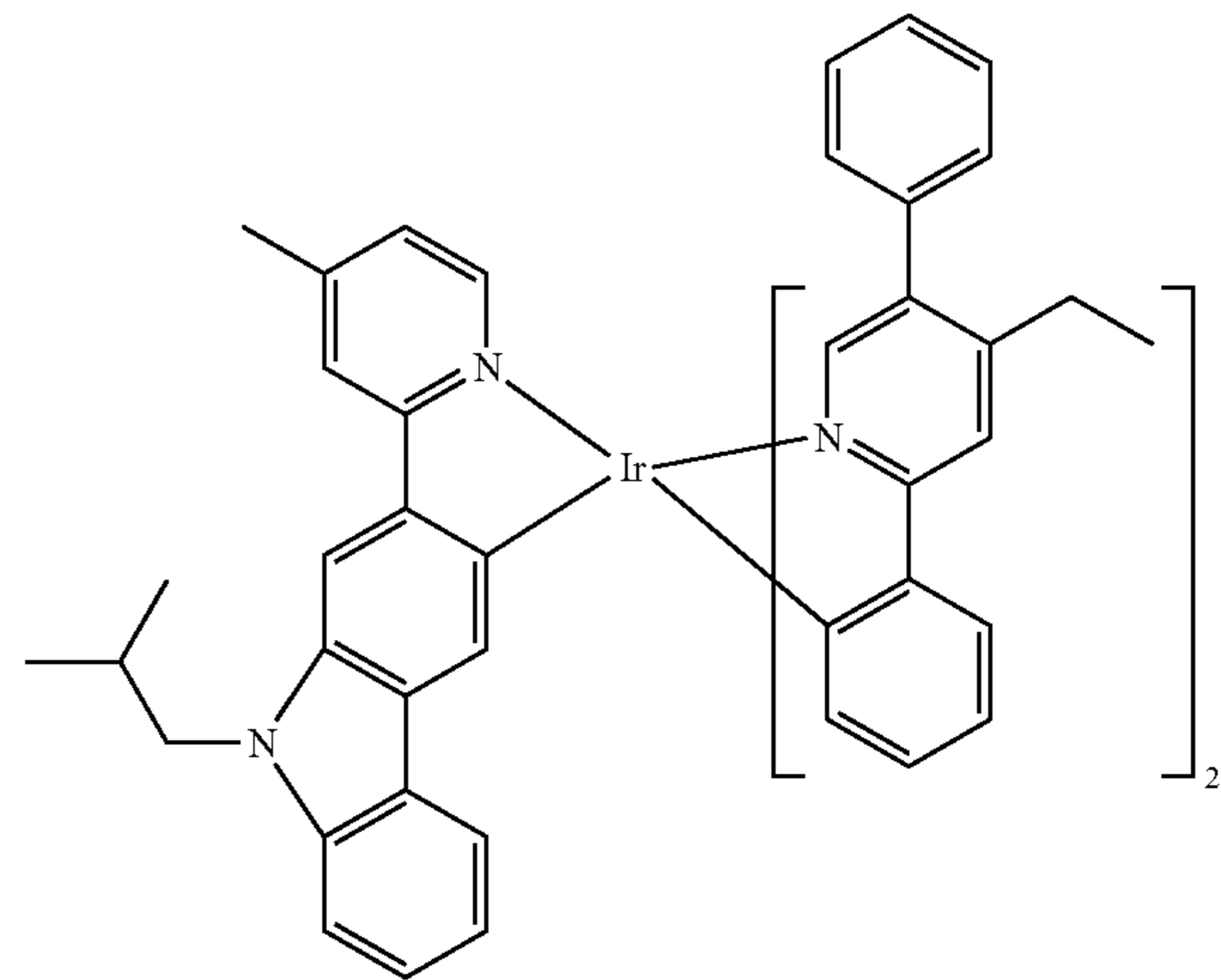
Compound 98
