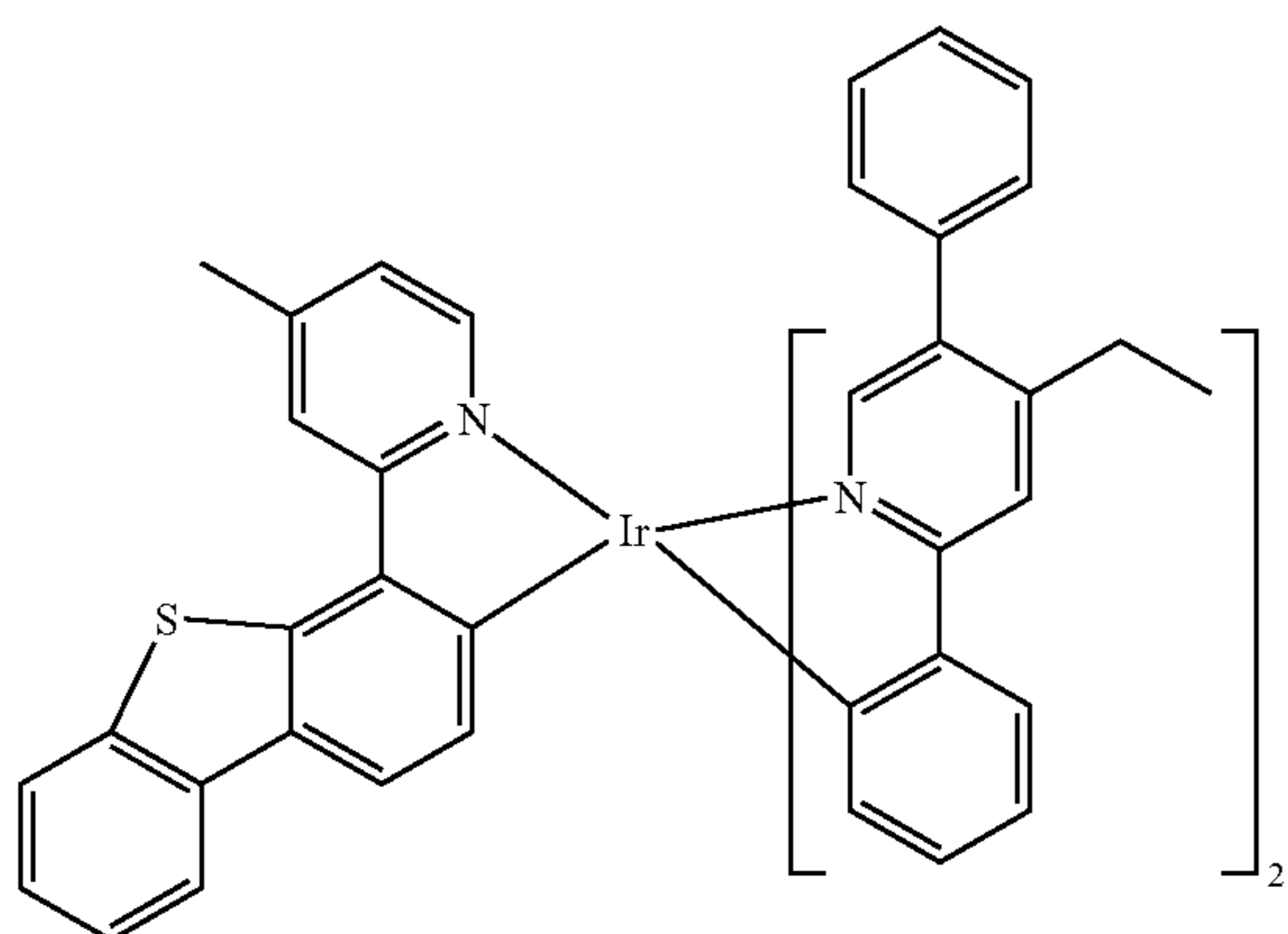
Compound 73
