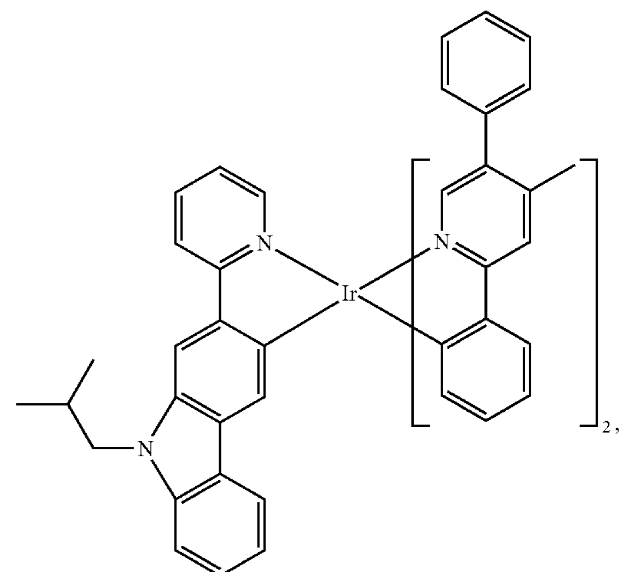
Compound 86
