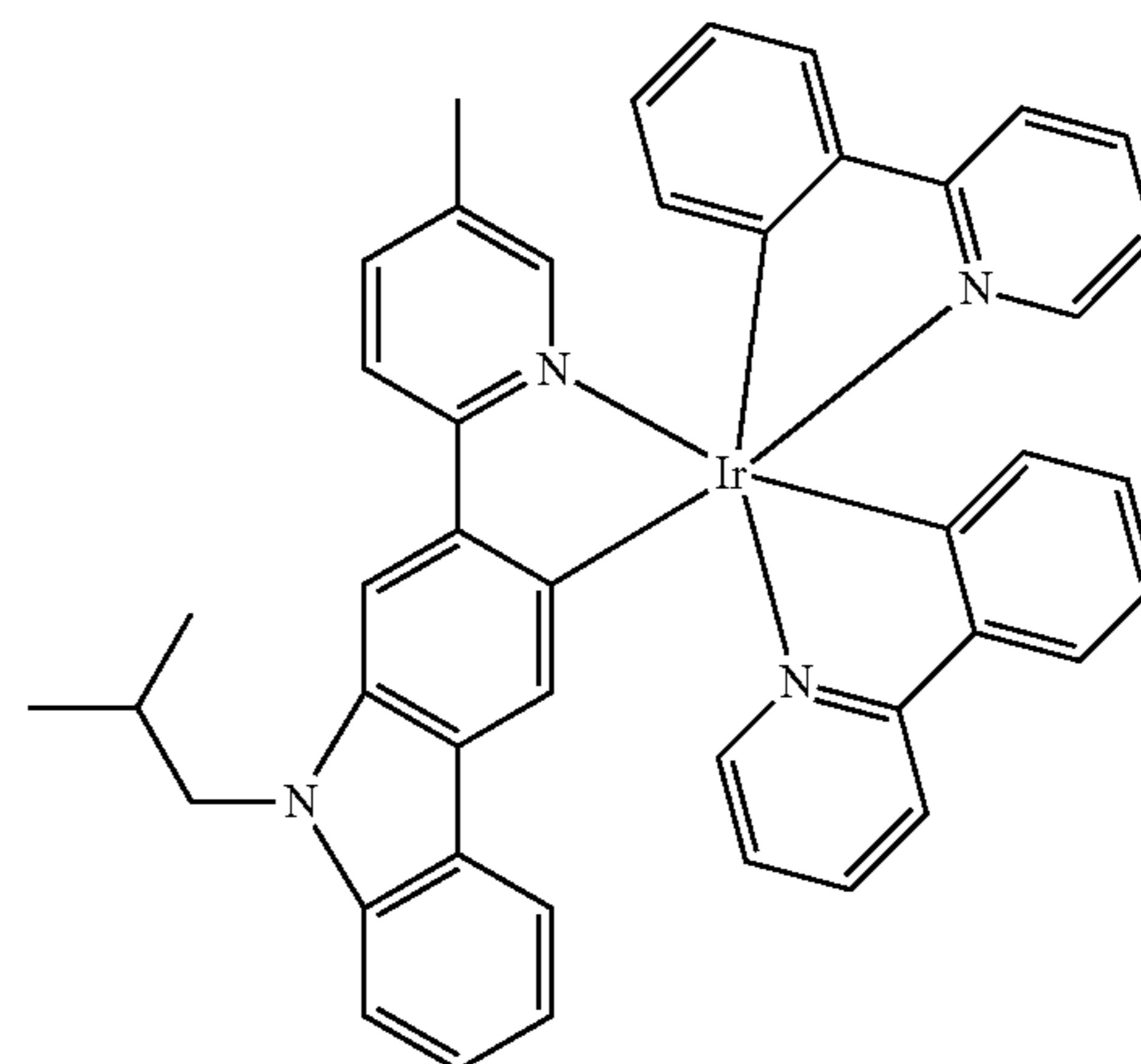
Compound 105
