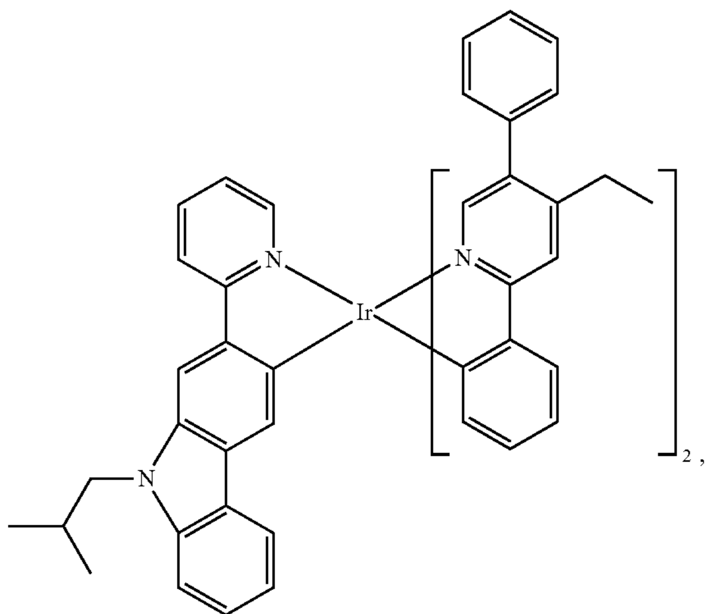
Compound 95
