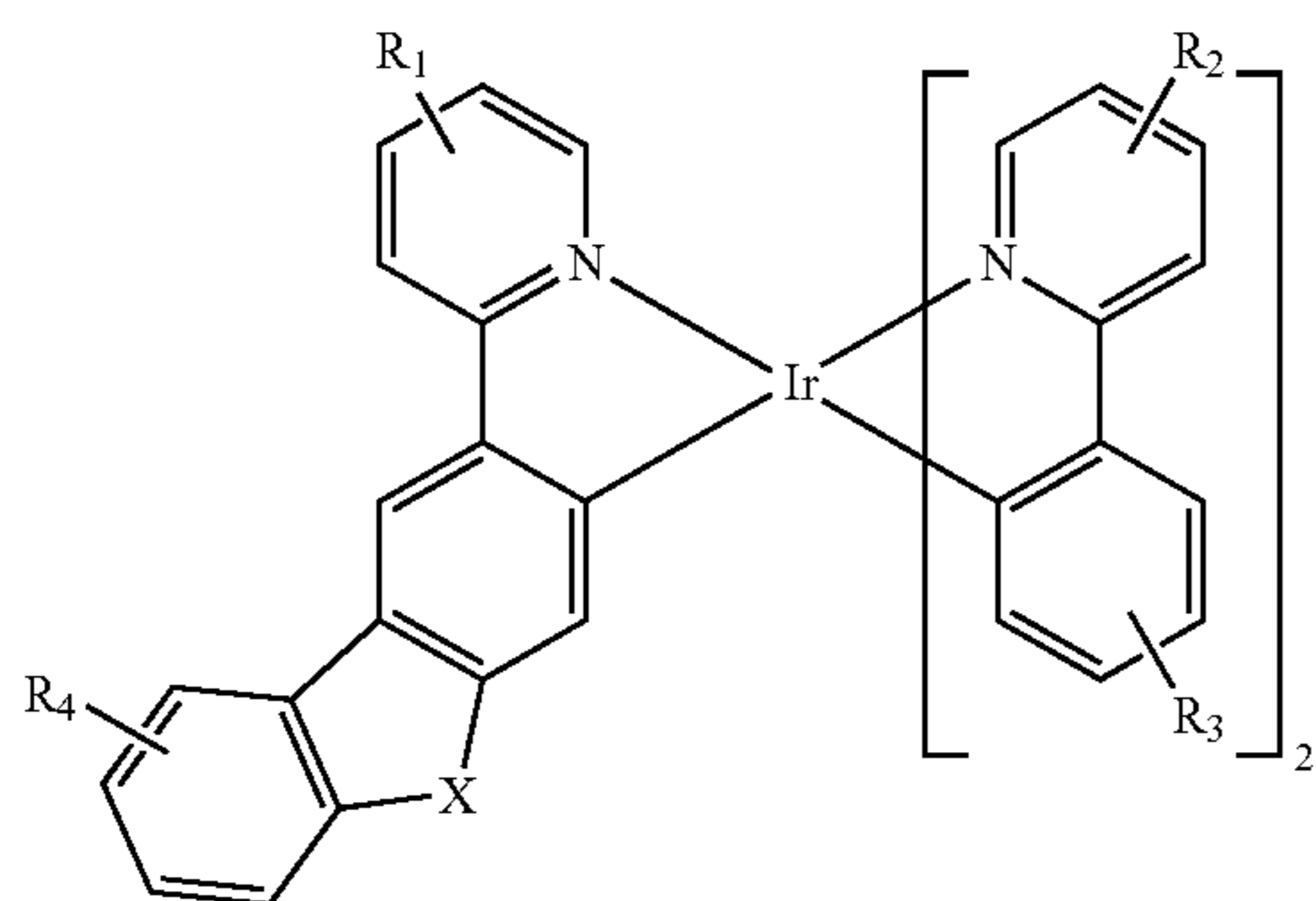
FORMULA V
