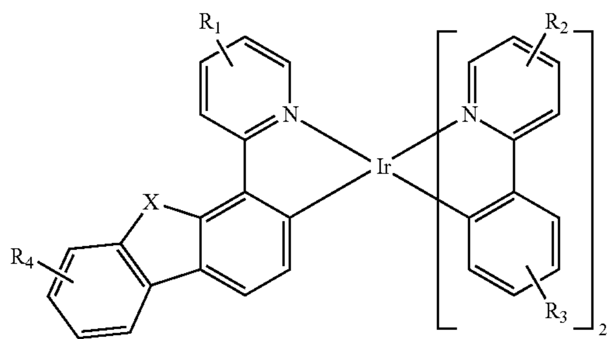
FORMULA IV
