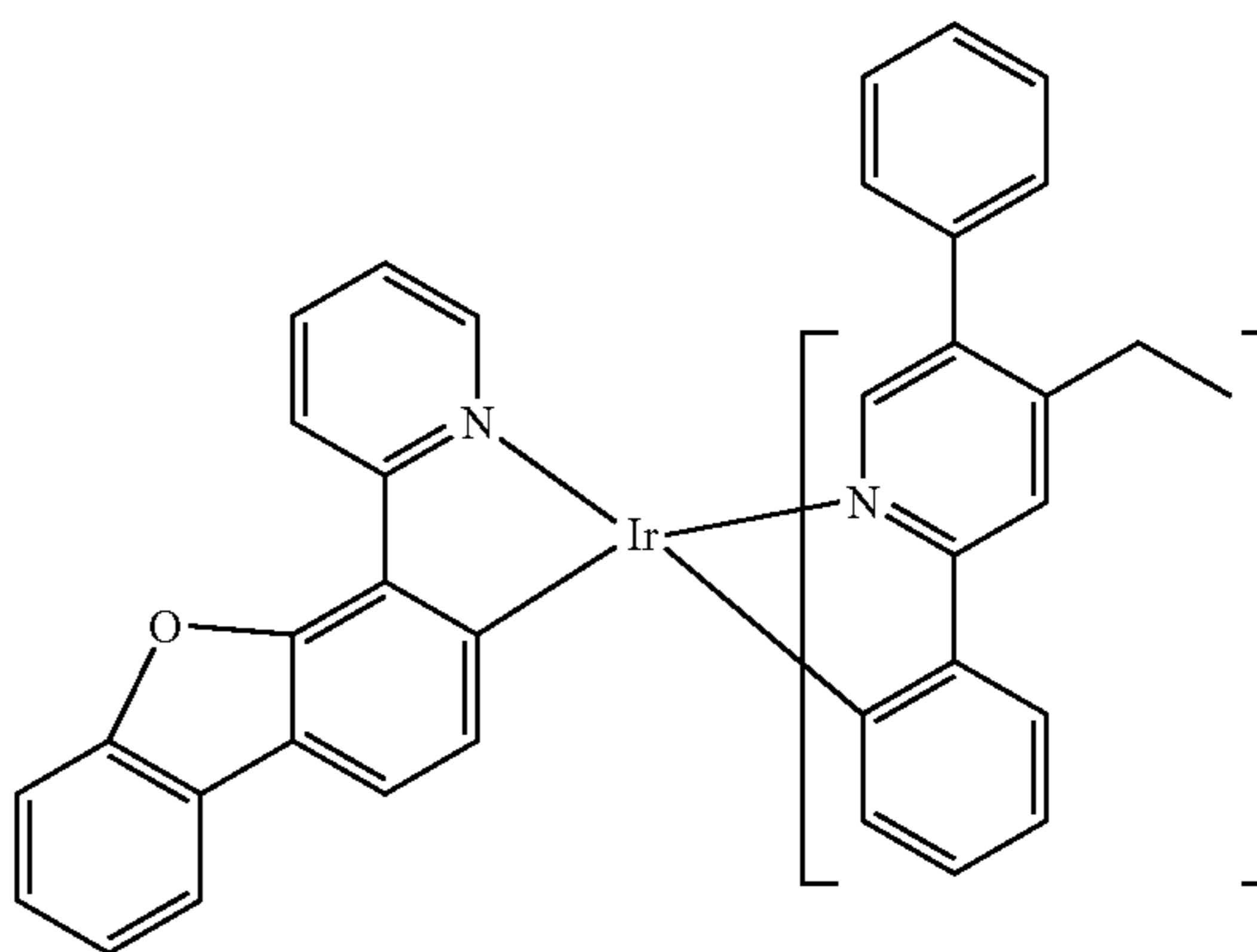
Compound 46
