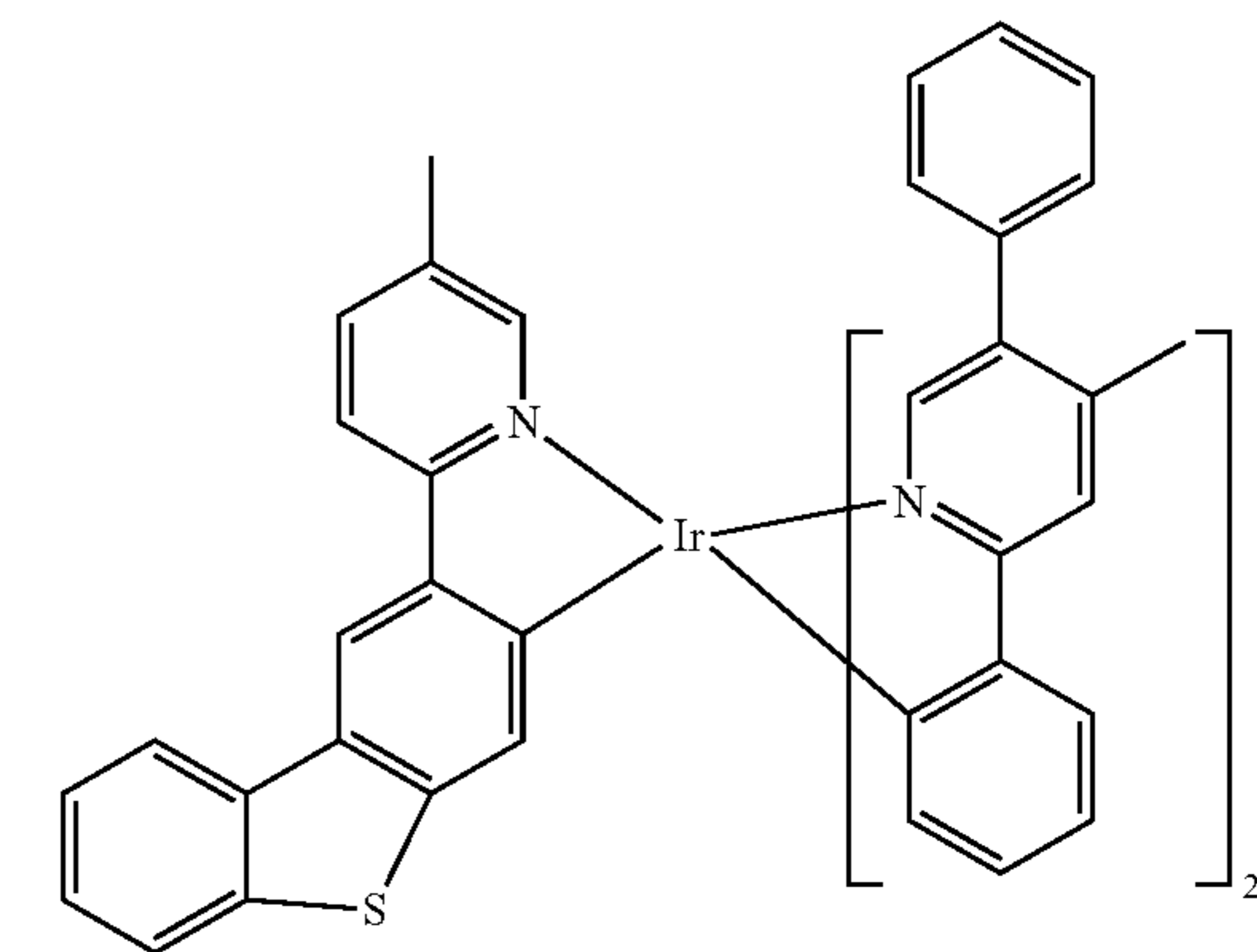
Compound 69
