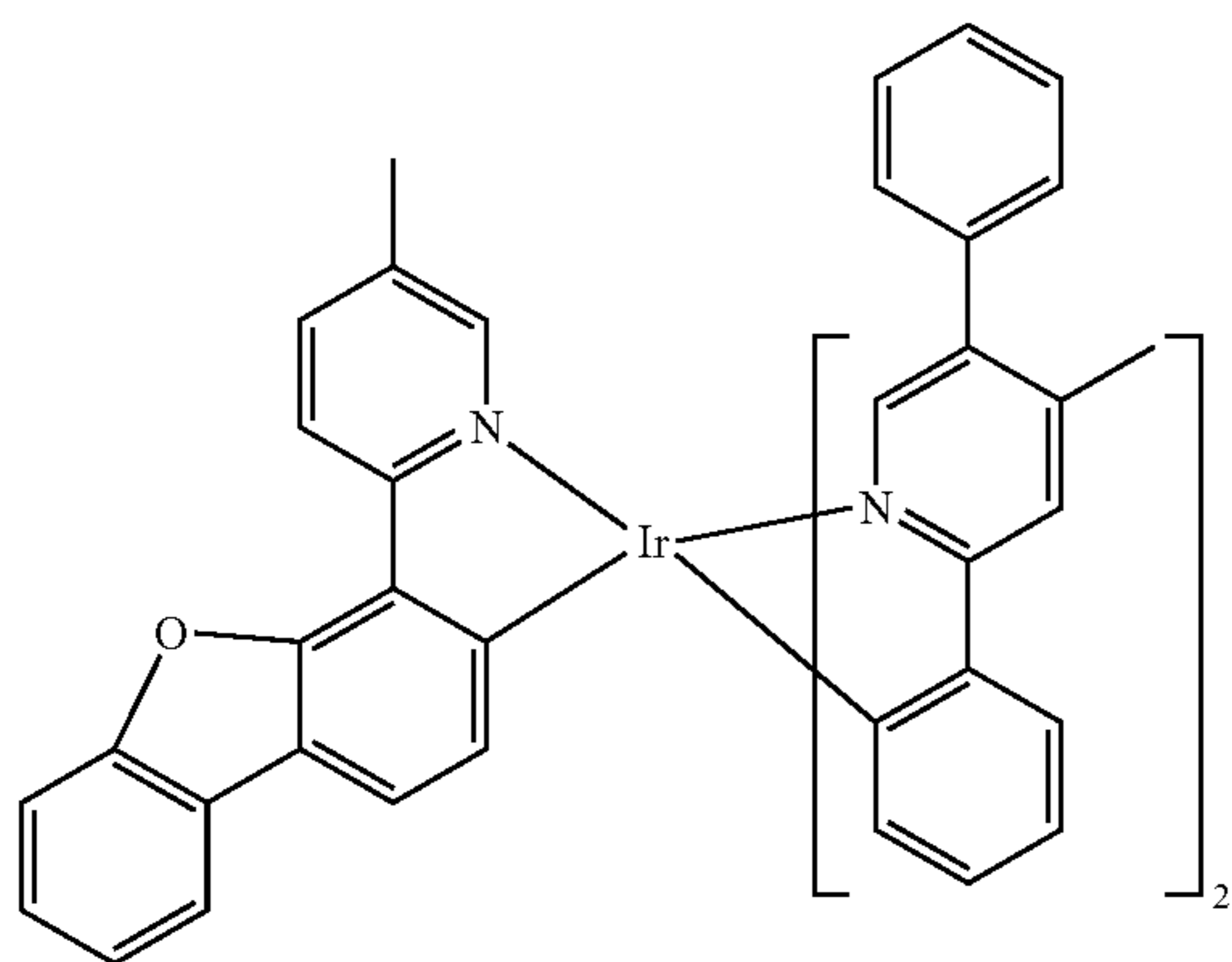
Compound 43
