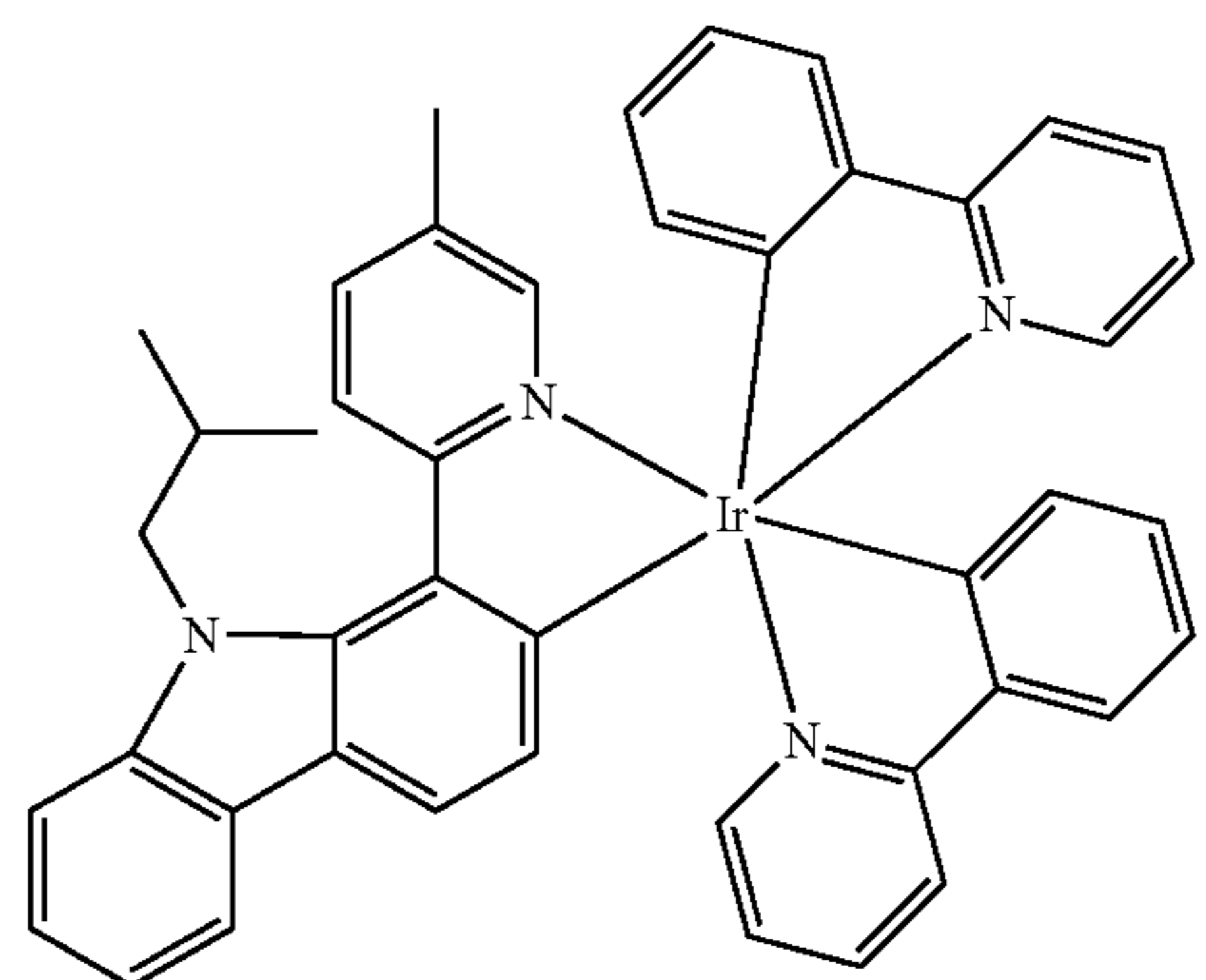
Compound 104
