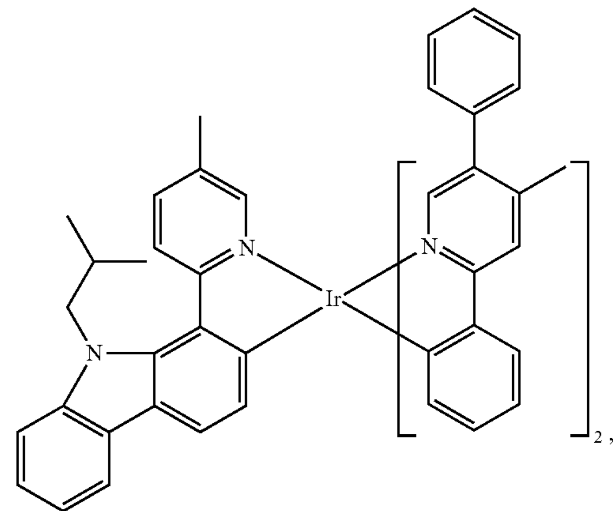
Compound 91
