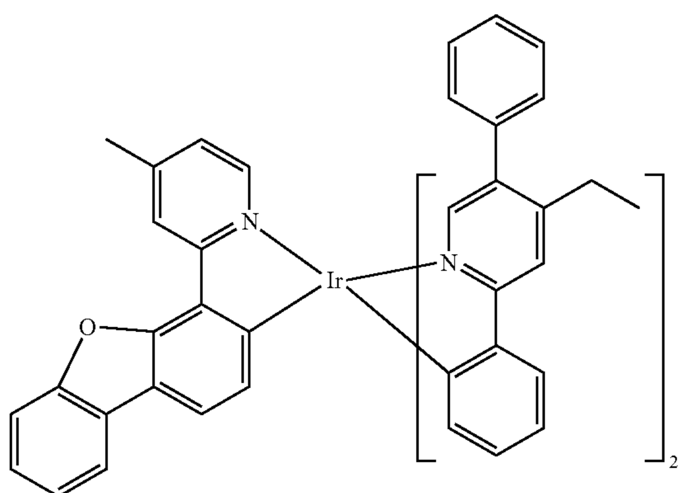
Compound 49
