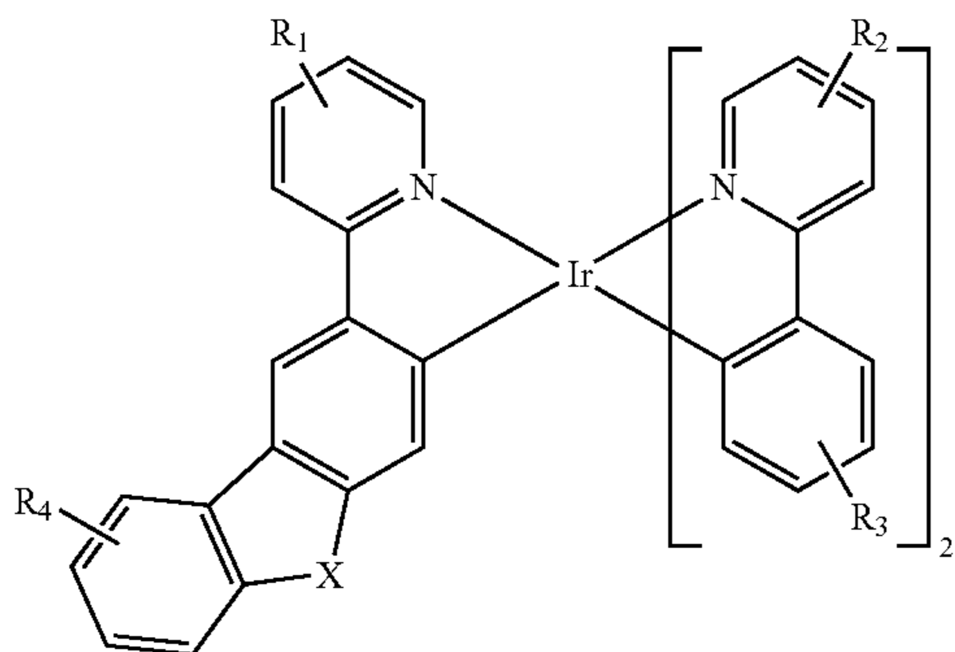
FORMULA V
