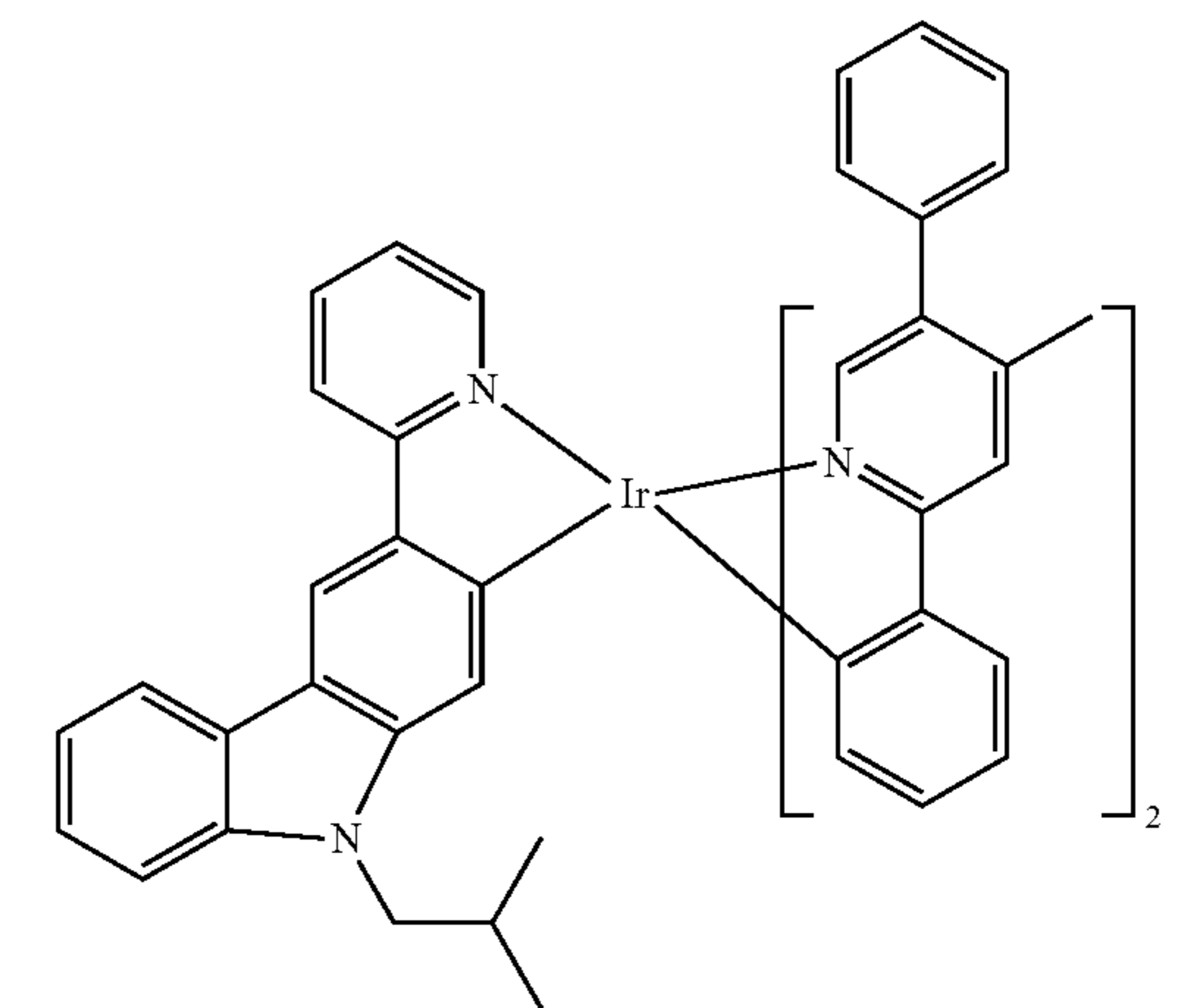
Compound 87
