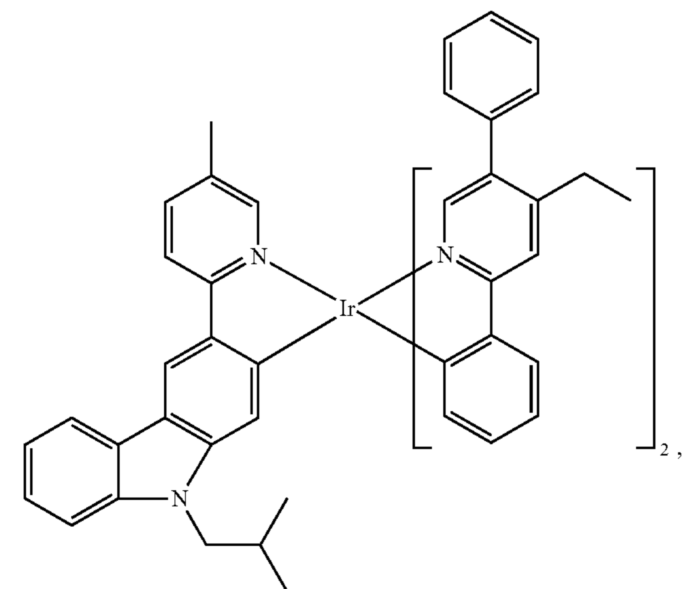
Compound 102
