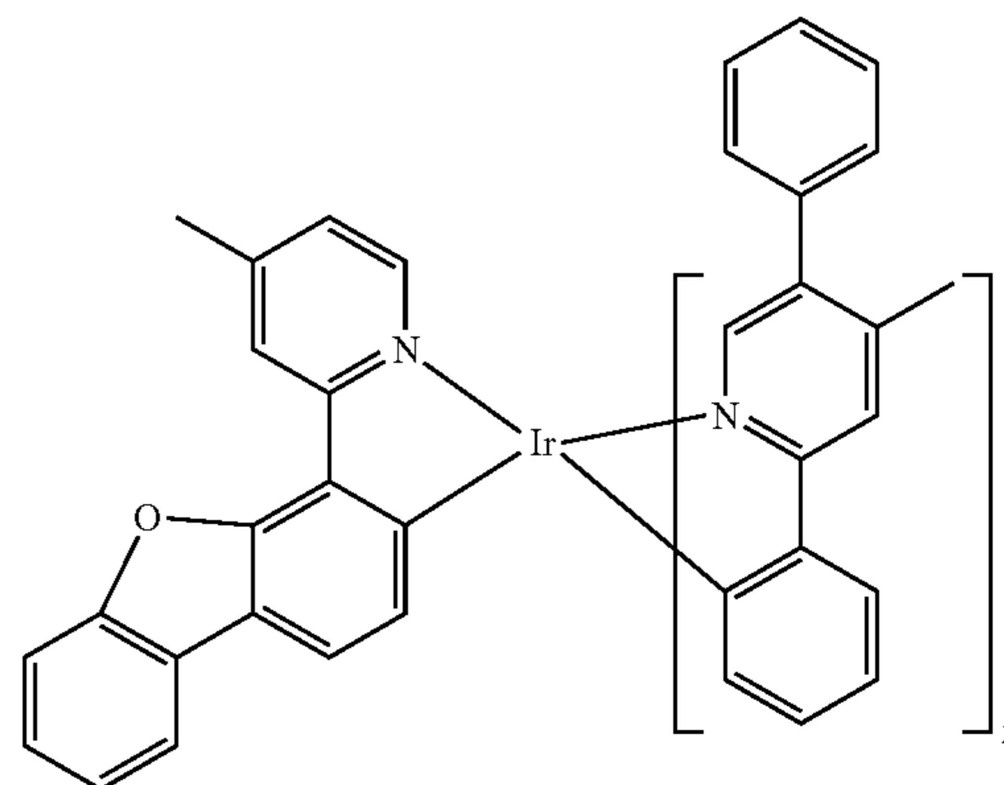
Compound 40
