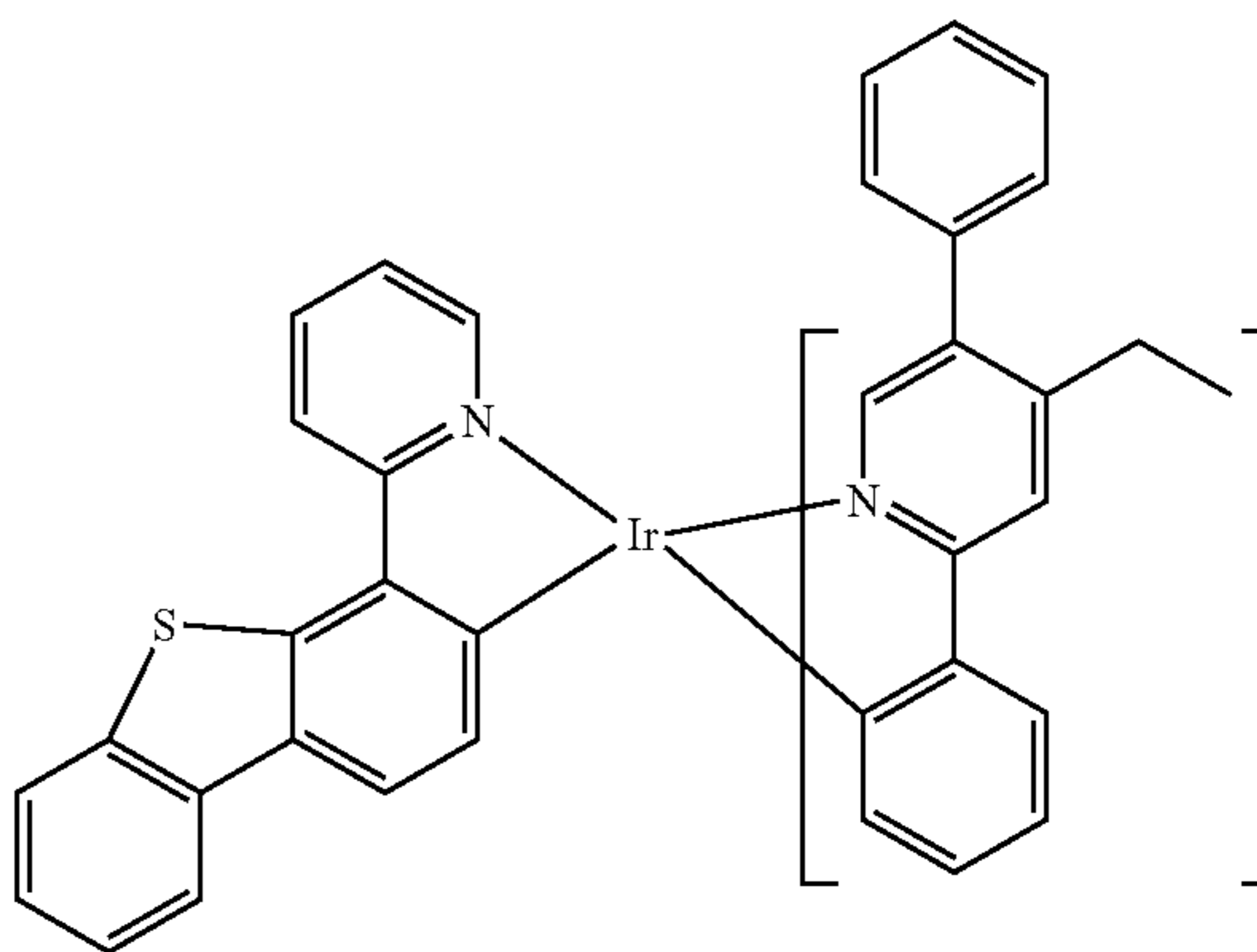
Compound 70
