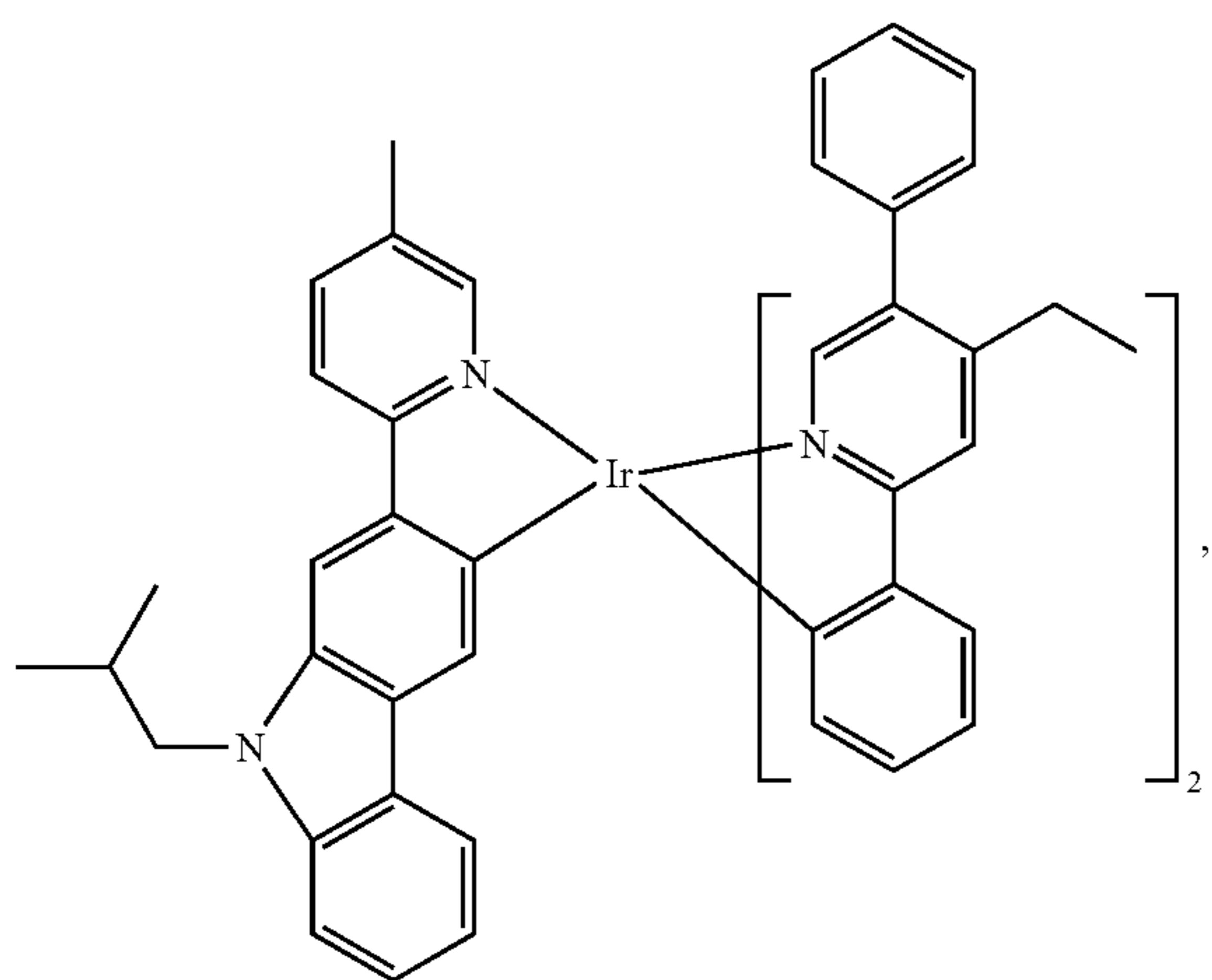
Compound 101
