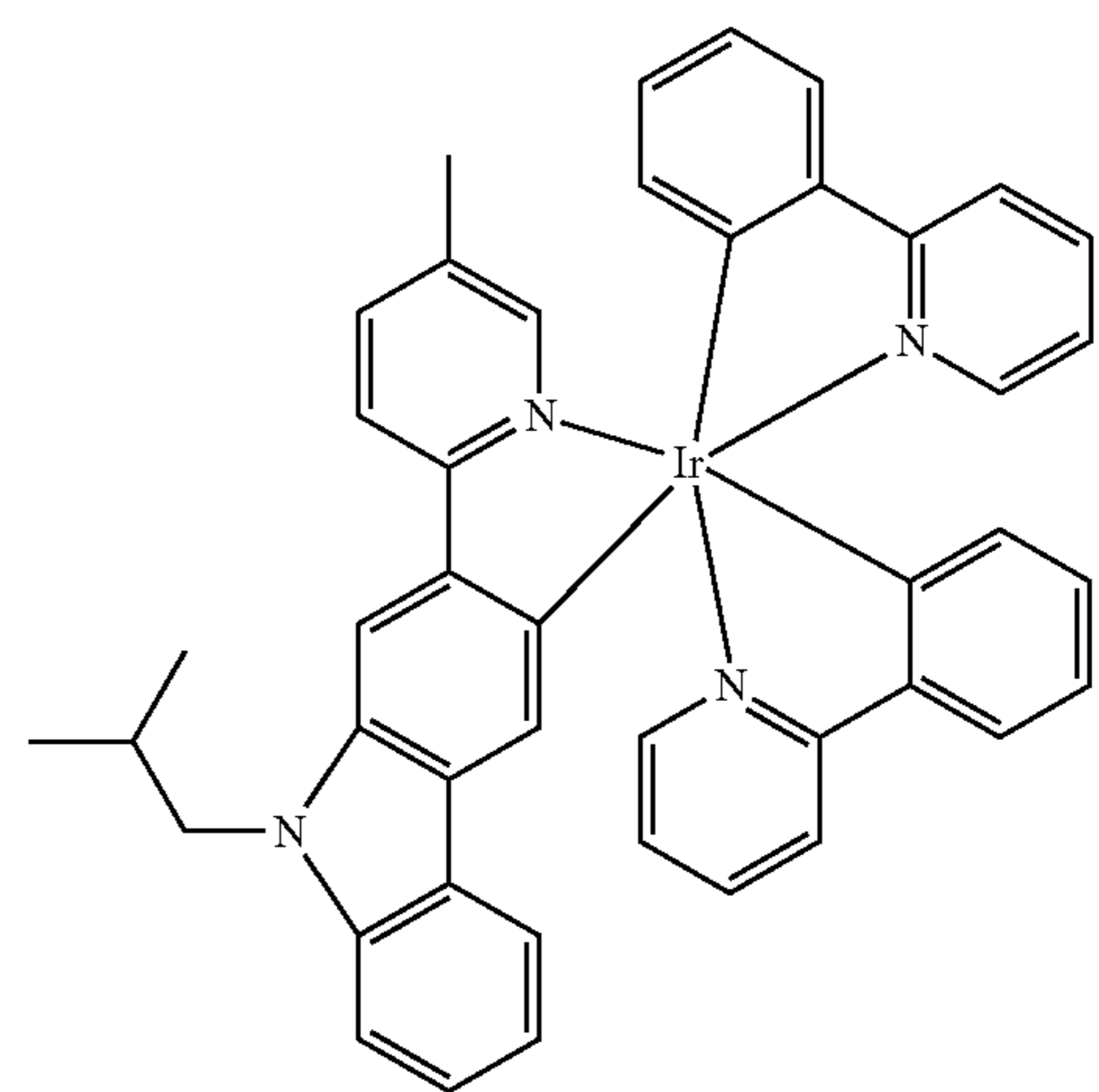
Compound 104
