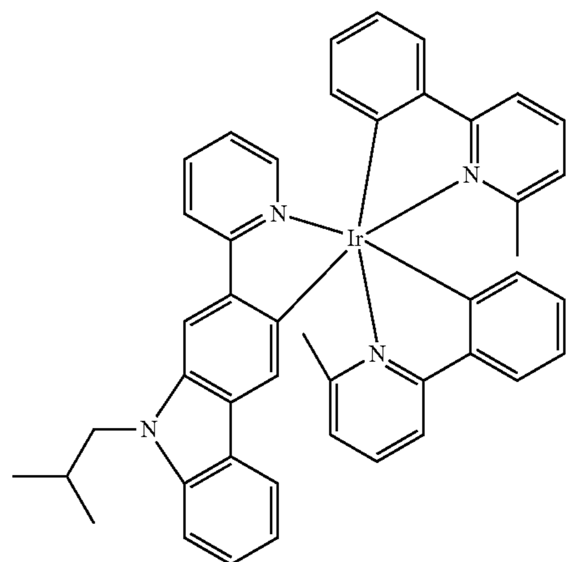
Compound 29
