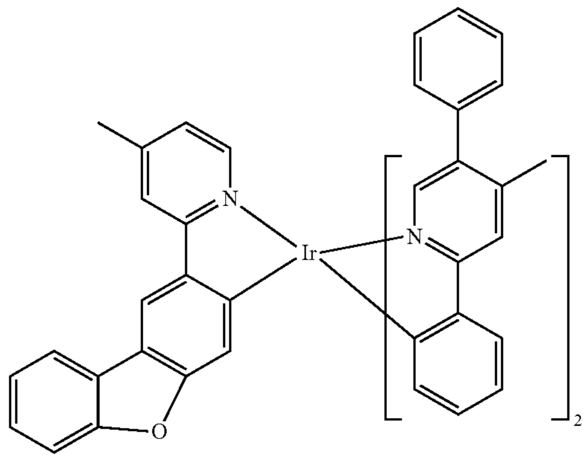
Compound 42
