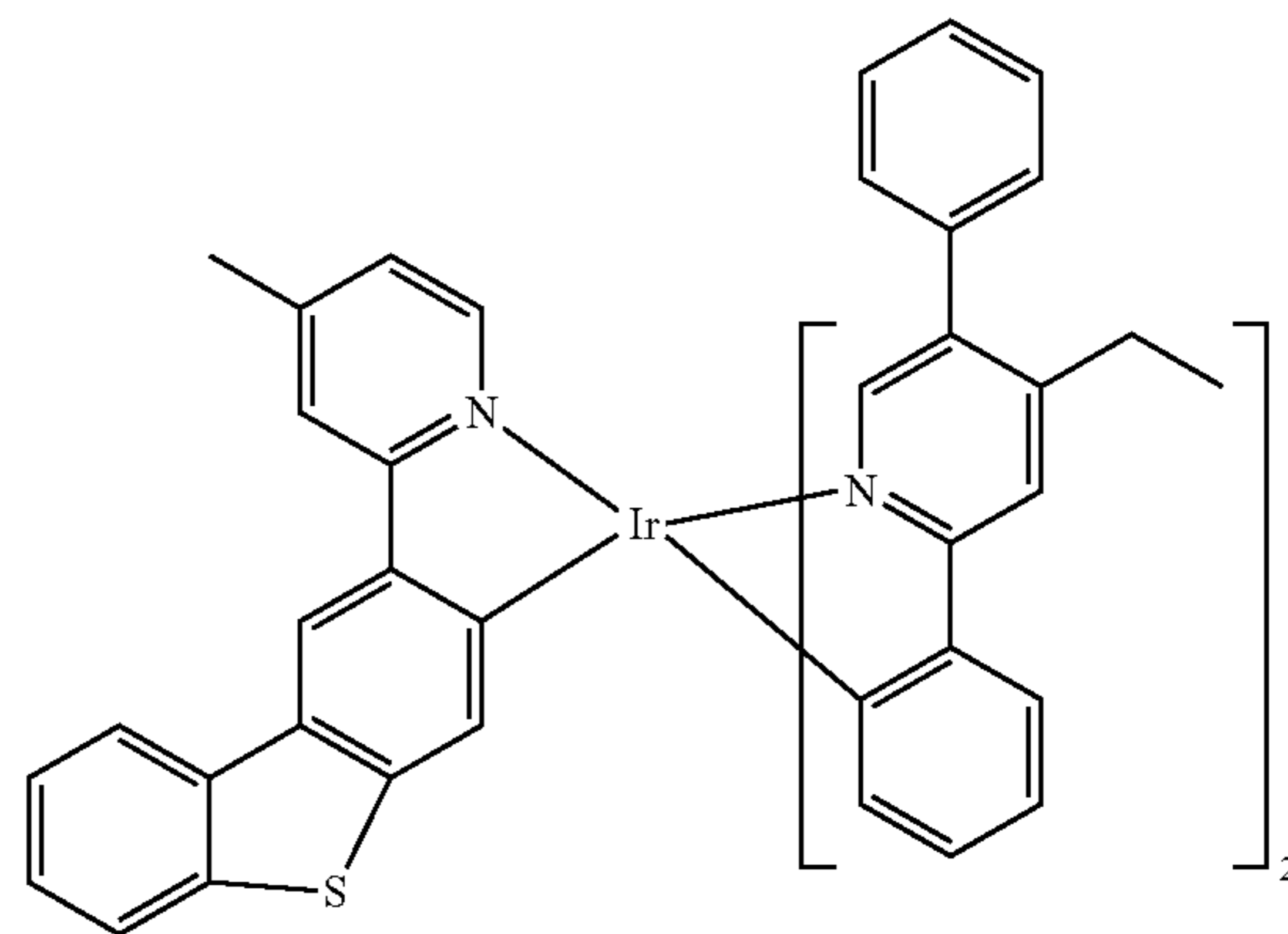
Compound 75
