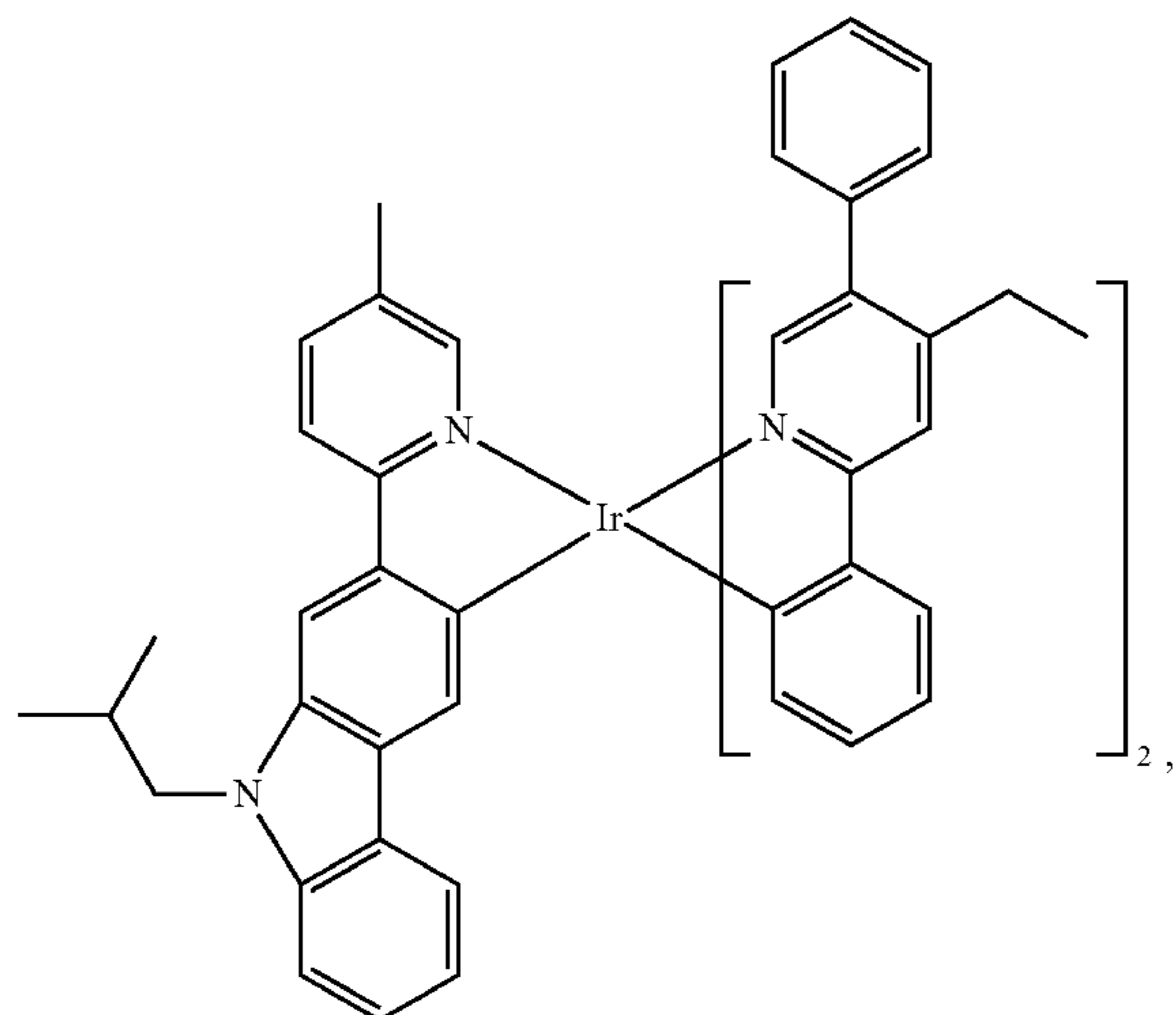
Compound 101
