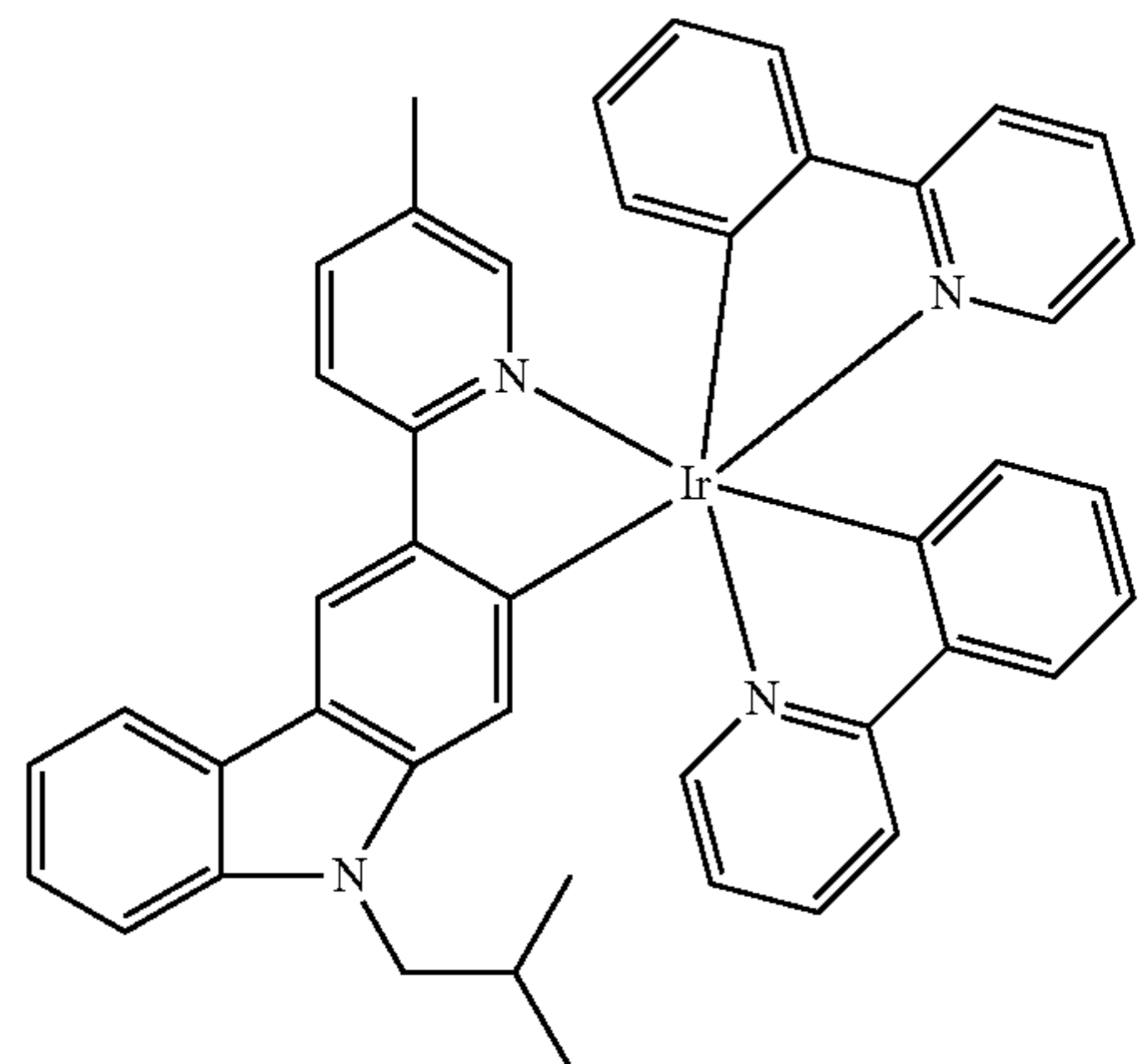
Compound 106
