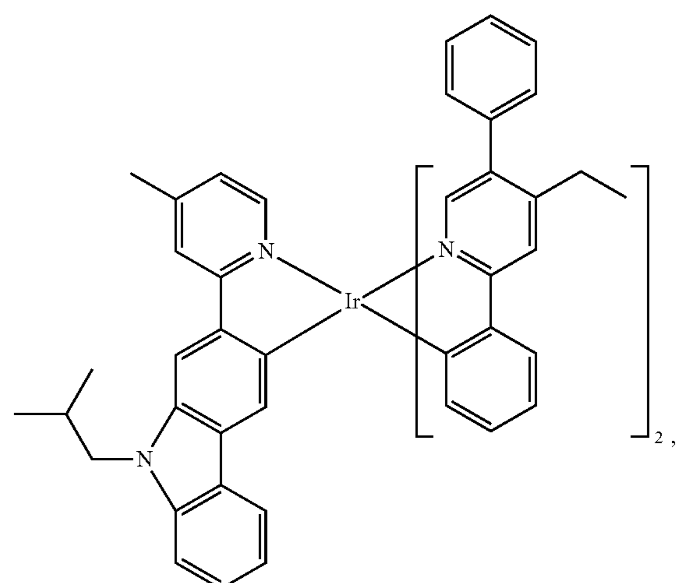
Compound 98
