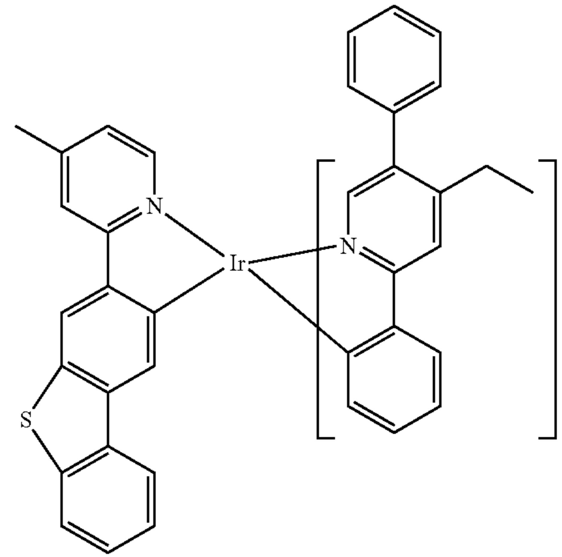
Compound 74
