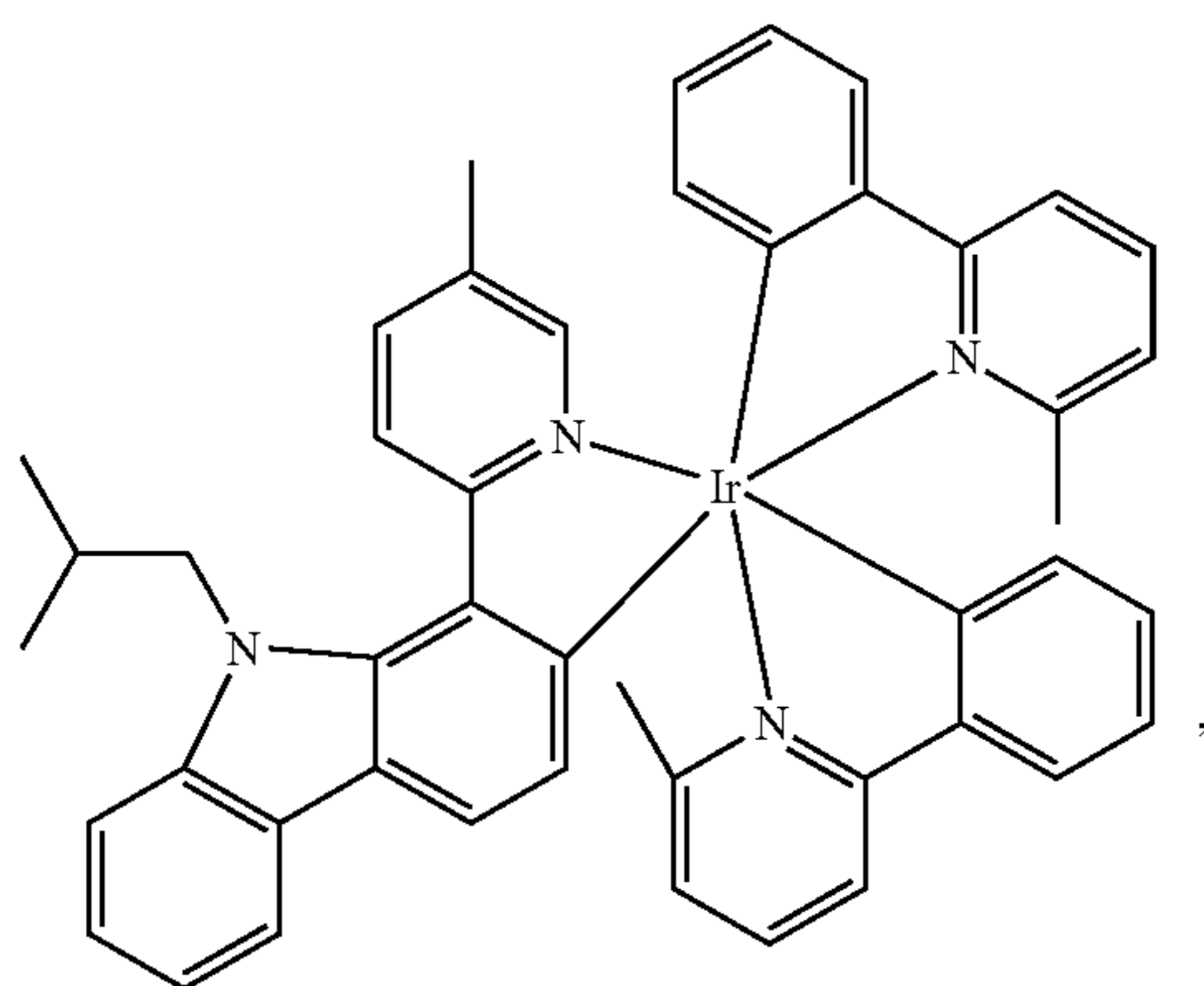
Compound 106
