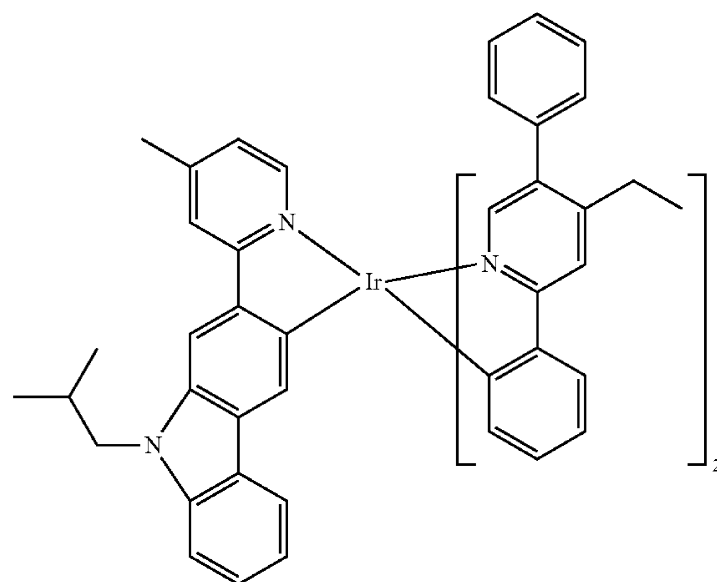
Compound 98
