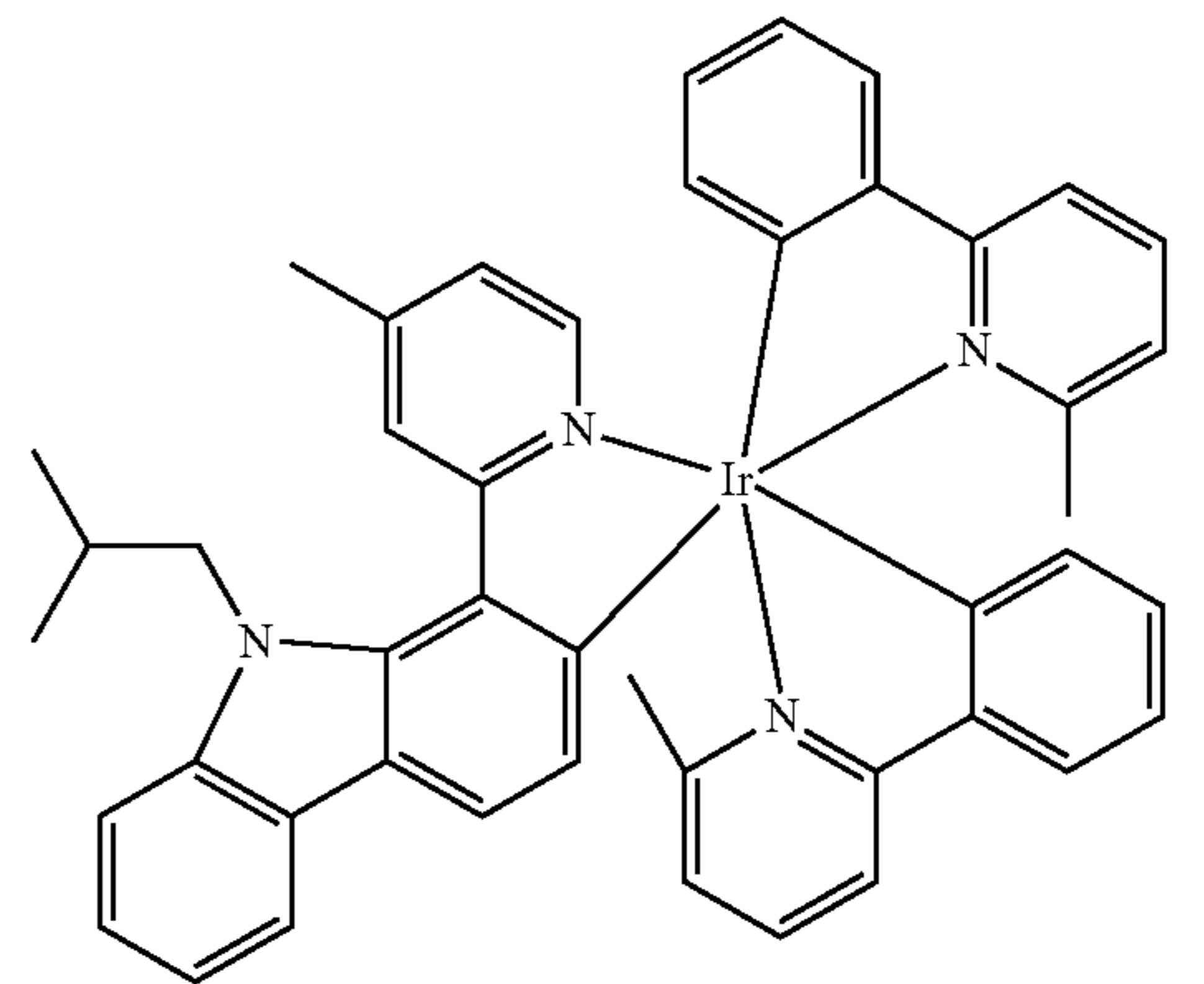
Compound 34
