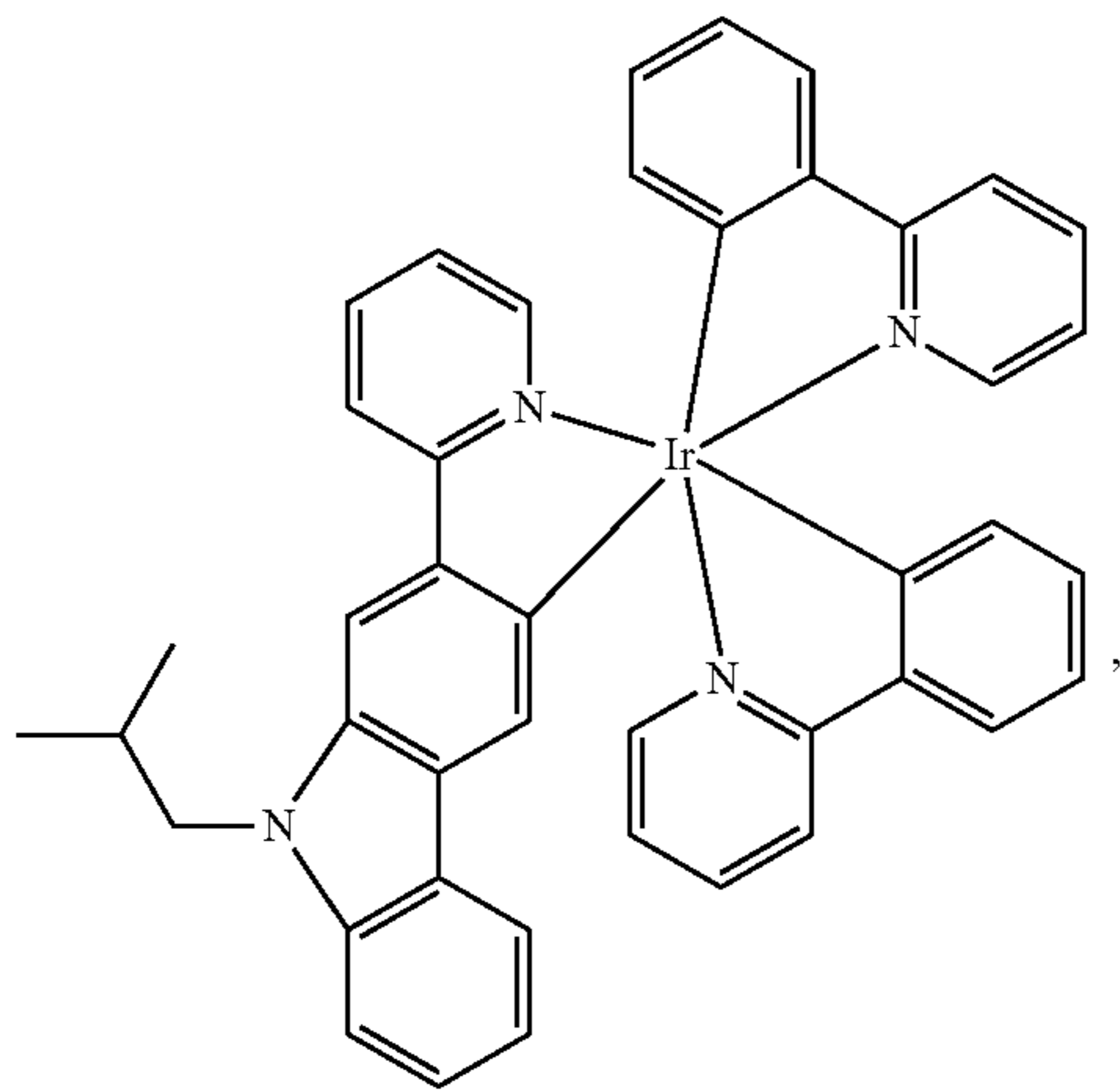
Compound 26
