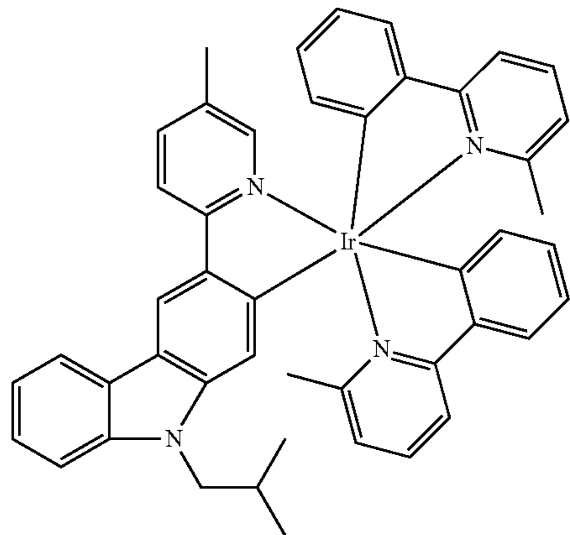
Compound 108
