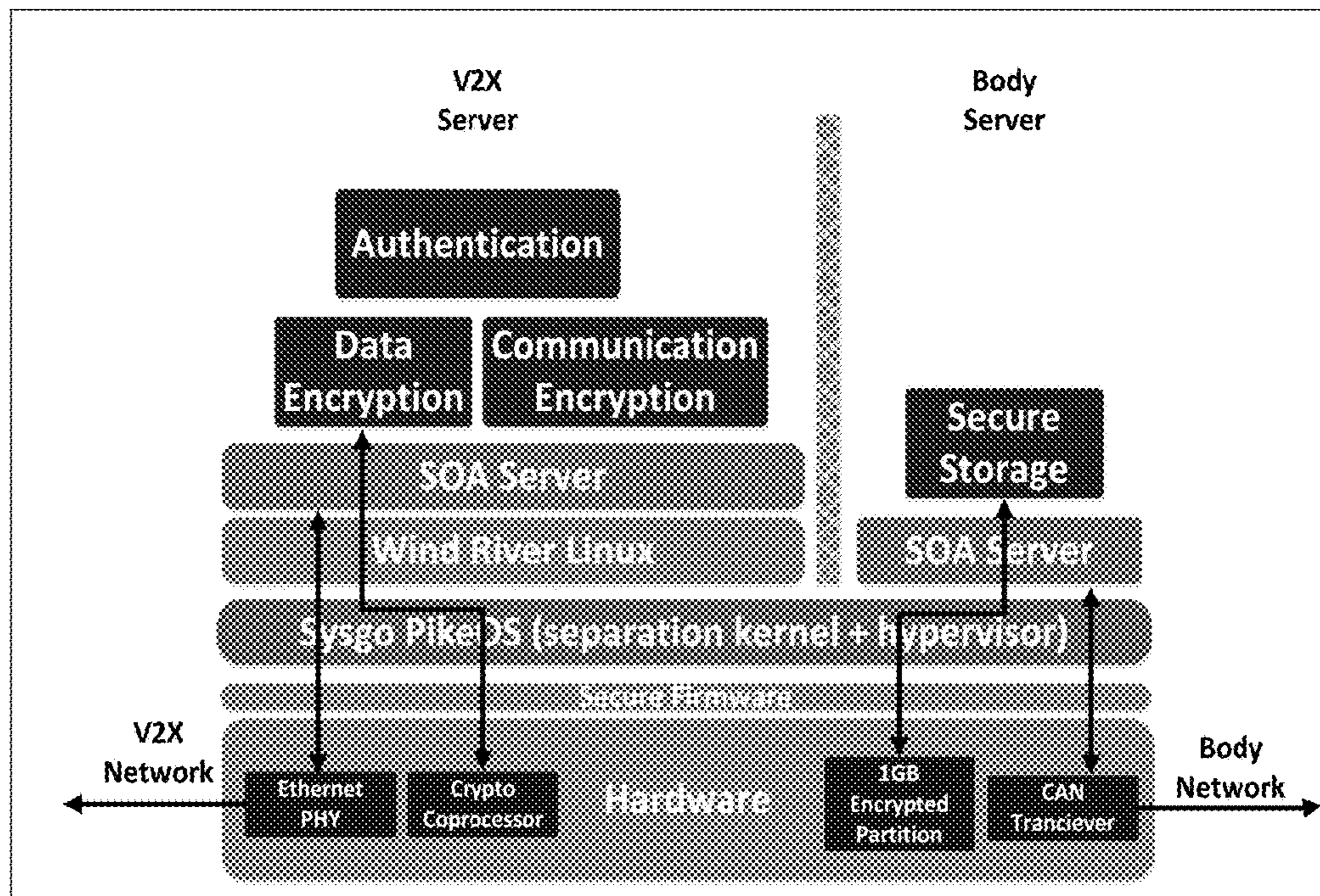
Figure 10. The inventive SOA security server architecture example
