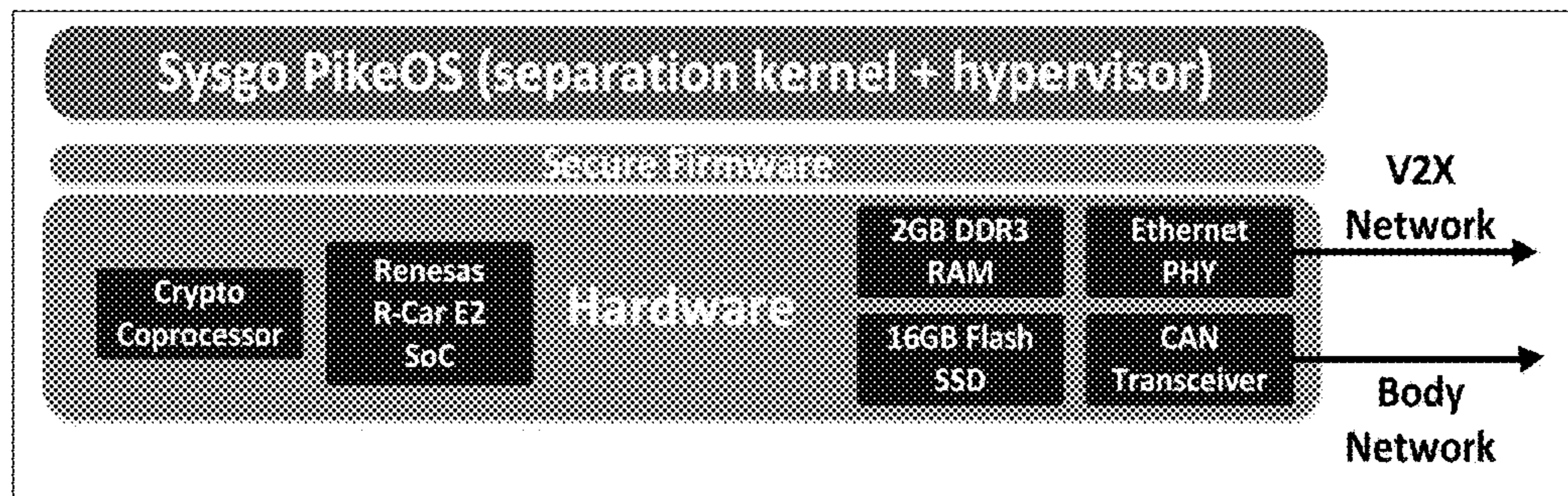
Figure 9. Example security server ECU architecture
