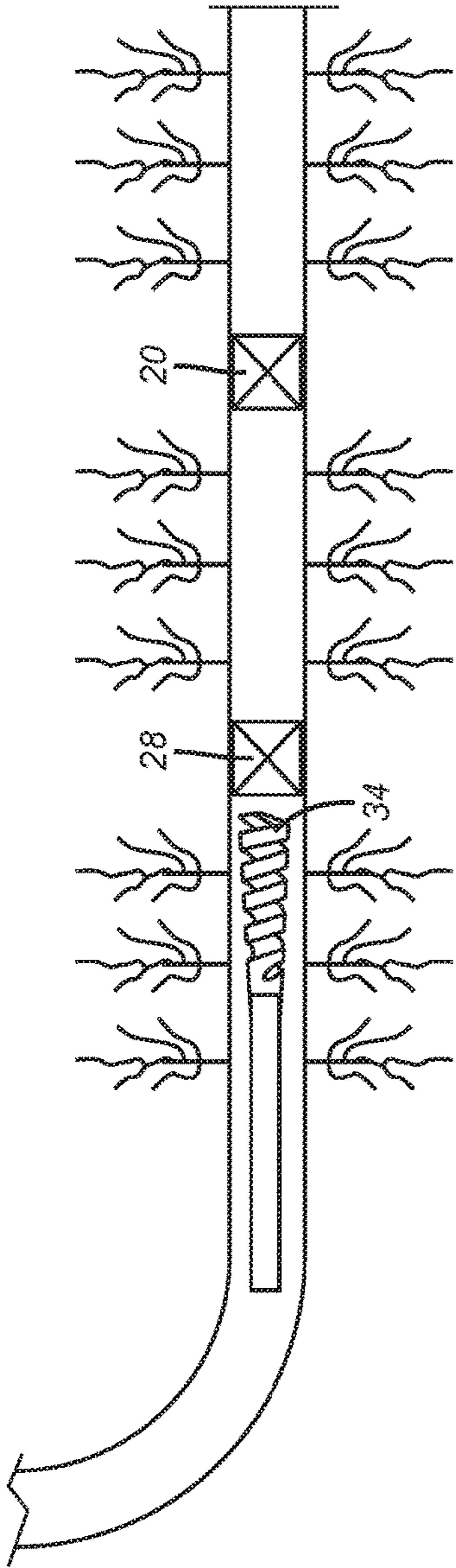
(PRIOR ART) FIG. 10
