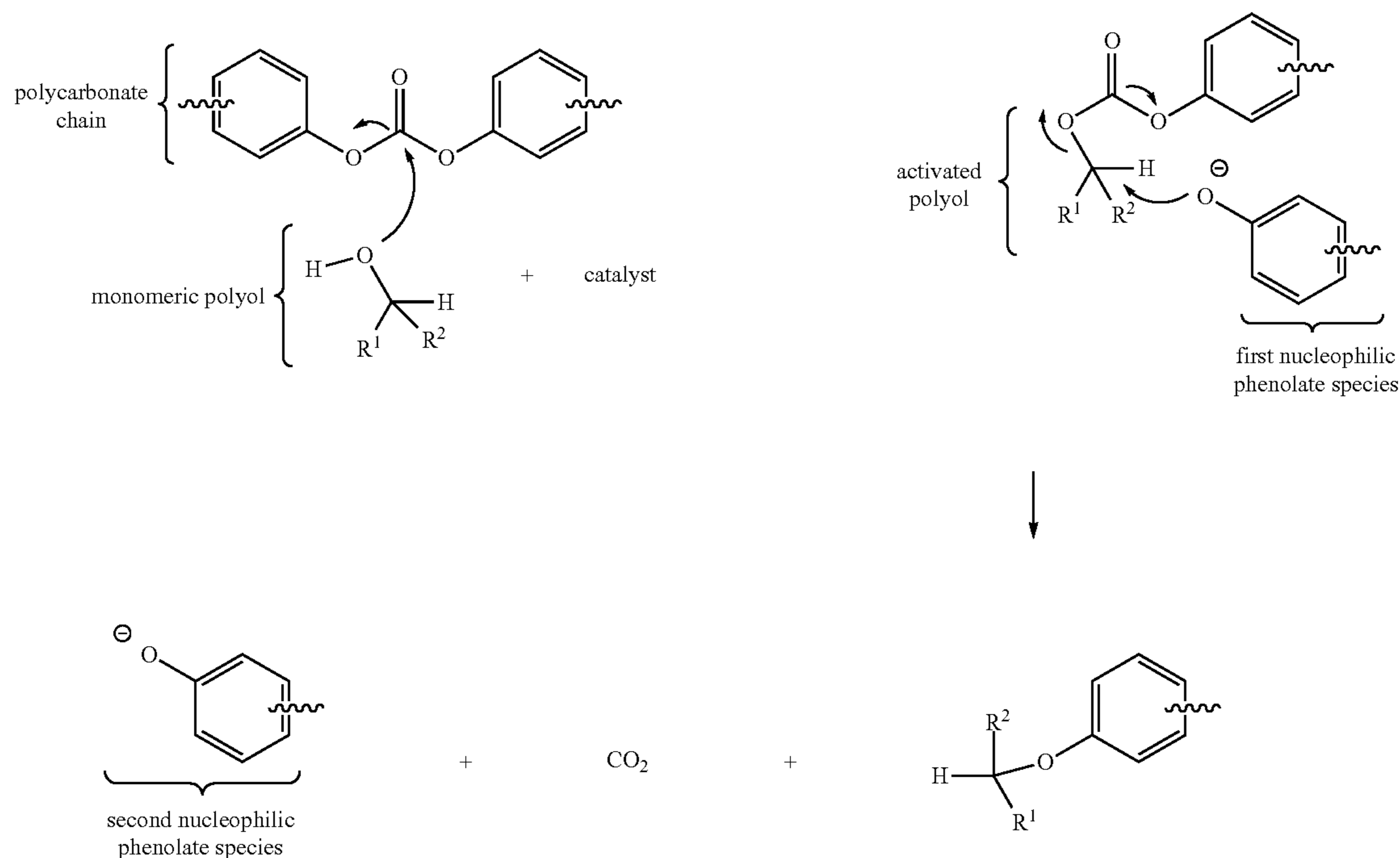
Scheme 1
