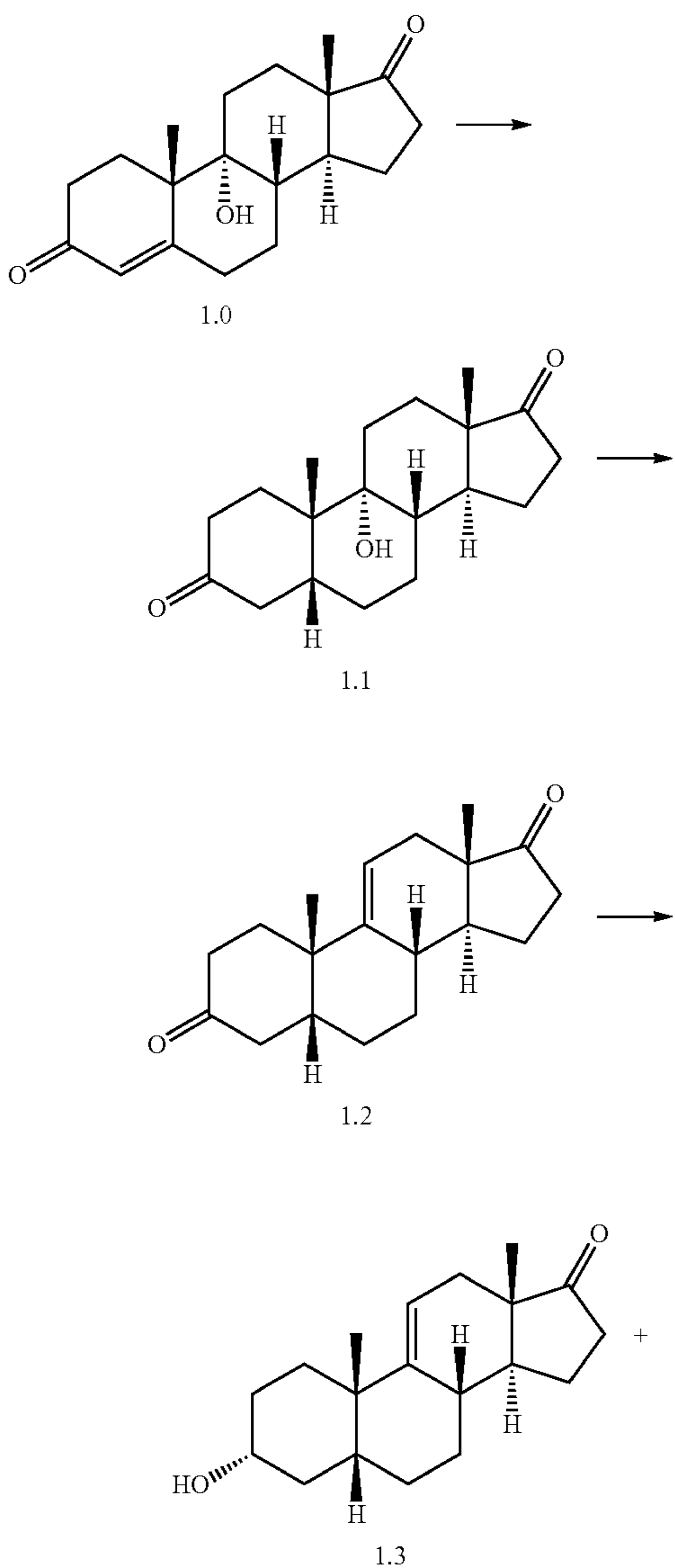
Scheme 1. Synthesis of Deoxycholic Acid (DCA)
