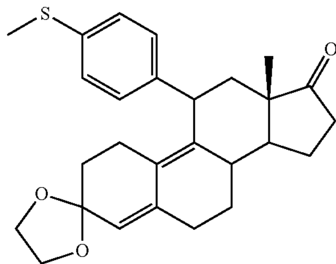
3,3-Ethylendioxy-5 \alpha -hidroxy-11 \beta -[4-p-(methylthio)phenyl]estra-4,9-dien-17-one (4j)
