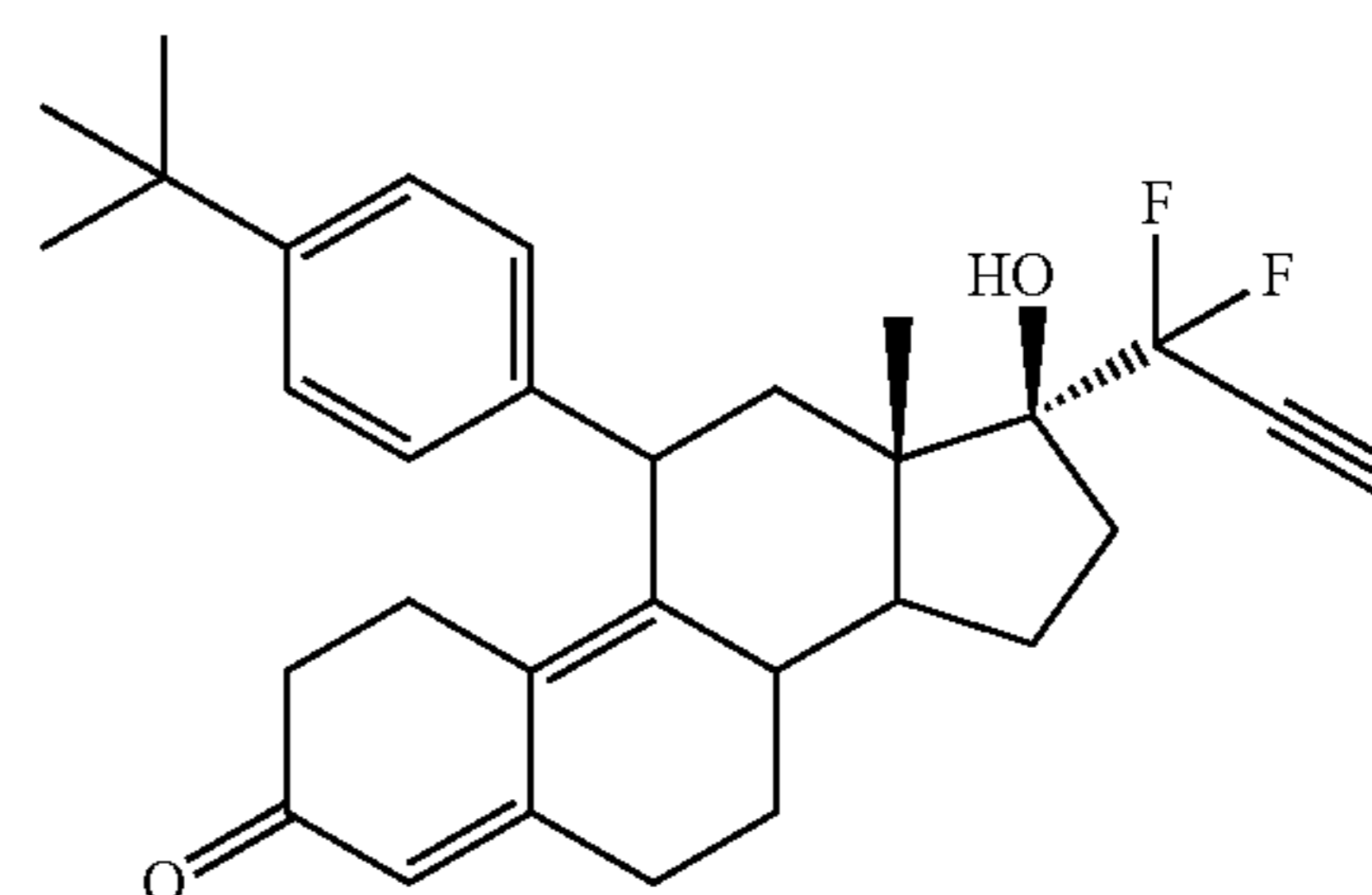
17 \alpha -(1,1-difluoro-2-propyn-1-yl)-17 \beta -hydroxy-11 \beta -[4-p-(t-butyl)phenyl]estra-4,9-dien-3-one (EC357)
