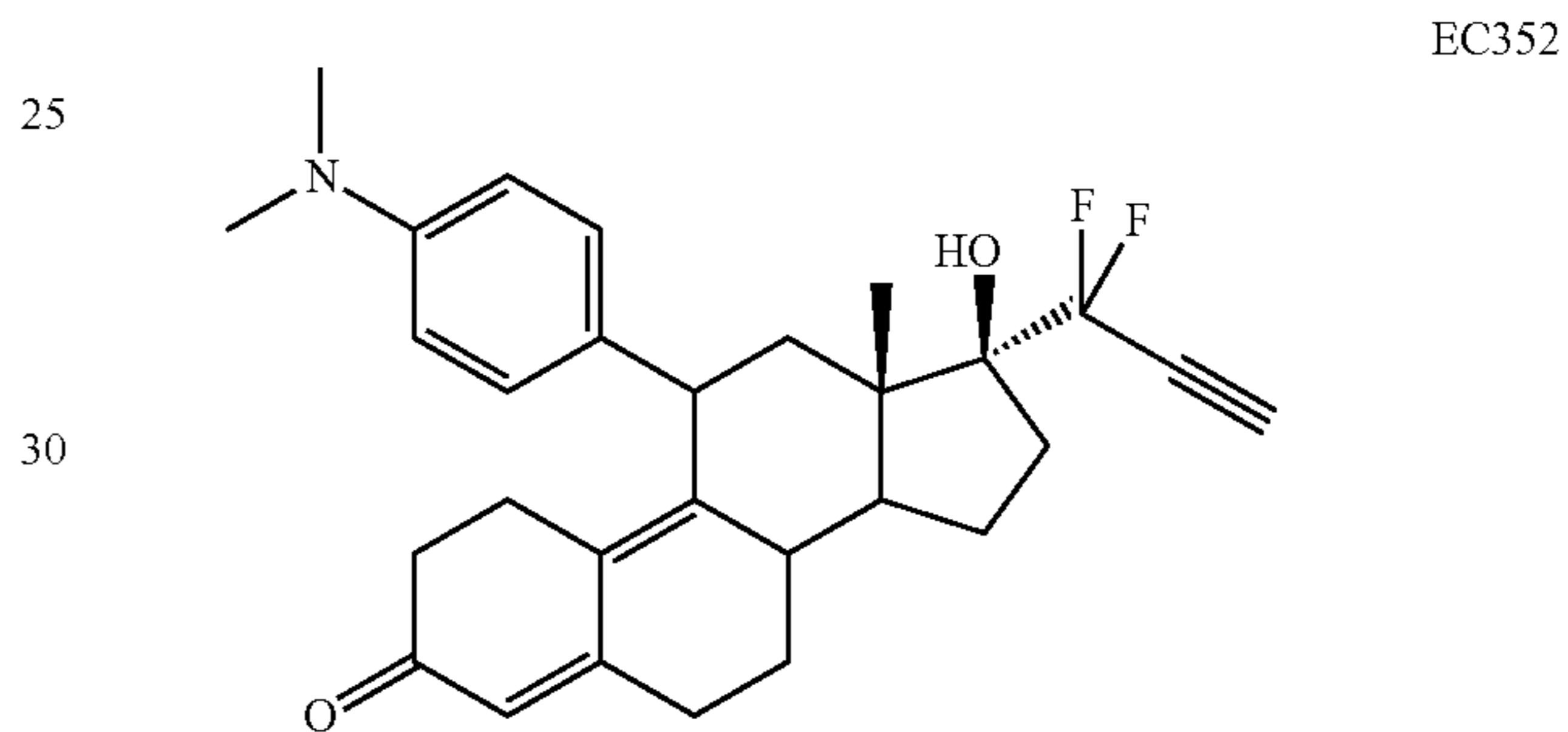
17 \alpha -(1,1-difluoro-2-propyn-1-yl)-17 \beta -hydroxy-11 \beta -[4-p-(dimethylamino)phenyl]estra-4,9-dien-3-one (EC352)
