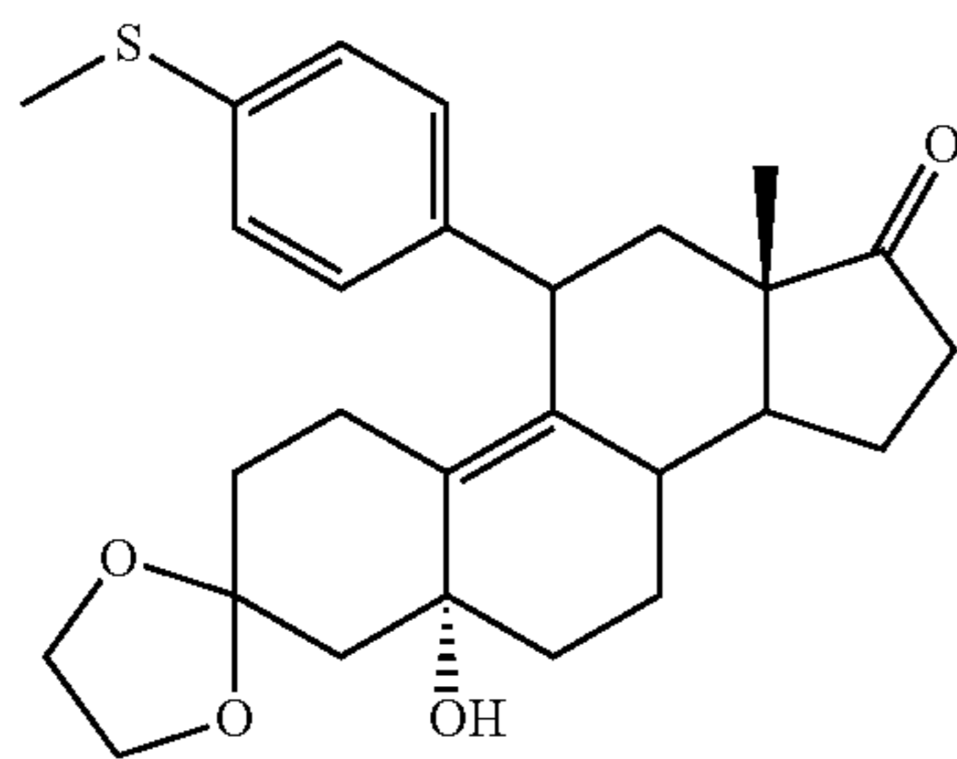
3,3-Ethylendioxy-5 \alpha -hidroxy-11 \beta -[4-p-(methylthio)phenyl]estra-4,9-dien-17-one (3j)
