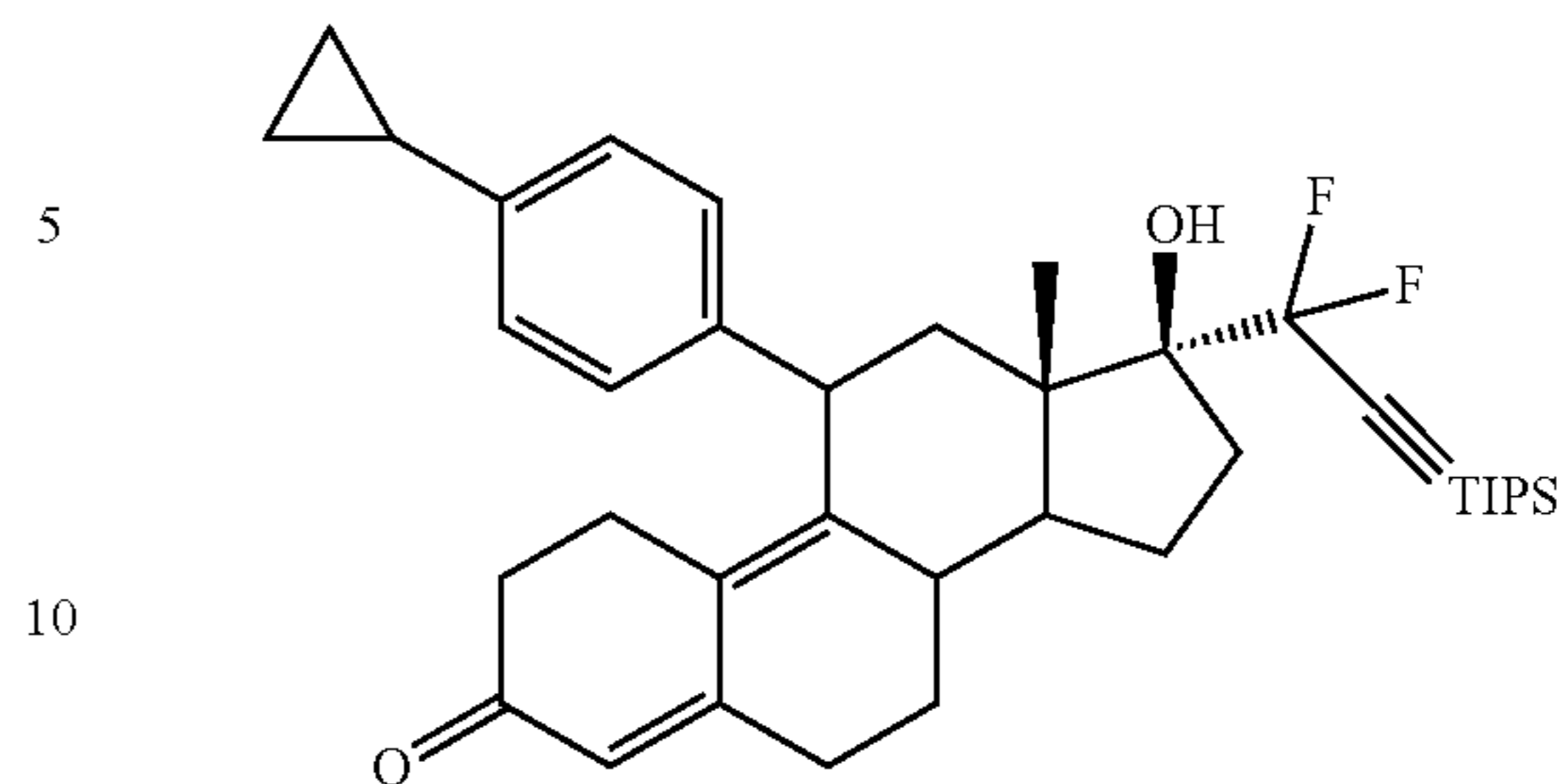
17α-[1,1-difluoro-3-[tris(1-methylethyl)silyl]-2-propyn-1-yl]-17β-hydroxy-11β-[4-p-(cyclopropyl)phenyl]estra-4,9-dien-3-one. (6a)
