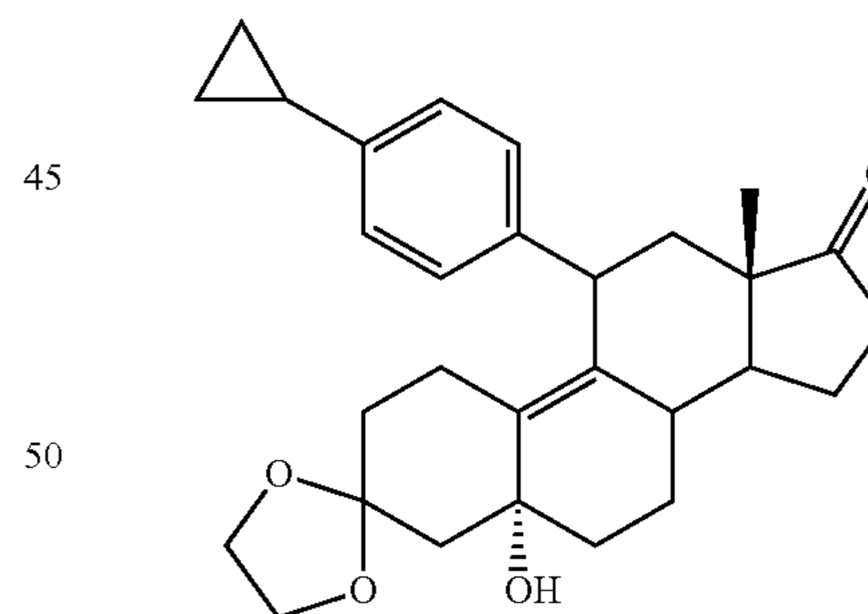
3,3-Ethylenedioxy-5α-hydroxy-11β-[4'-cyclopropylphenyl]-estr-9-ene-17-one (3a)
