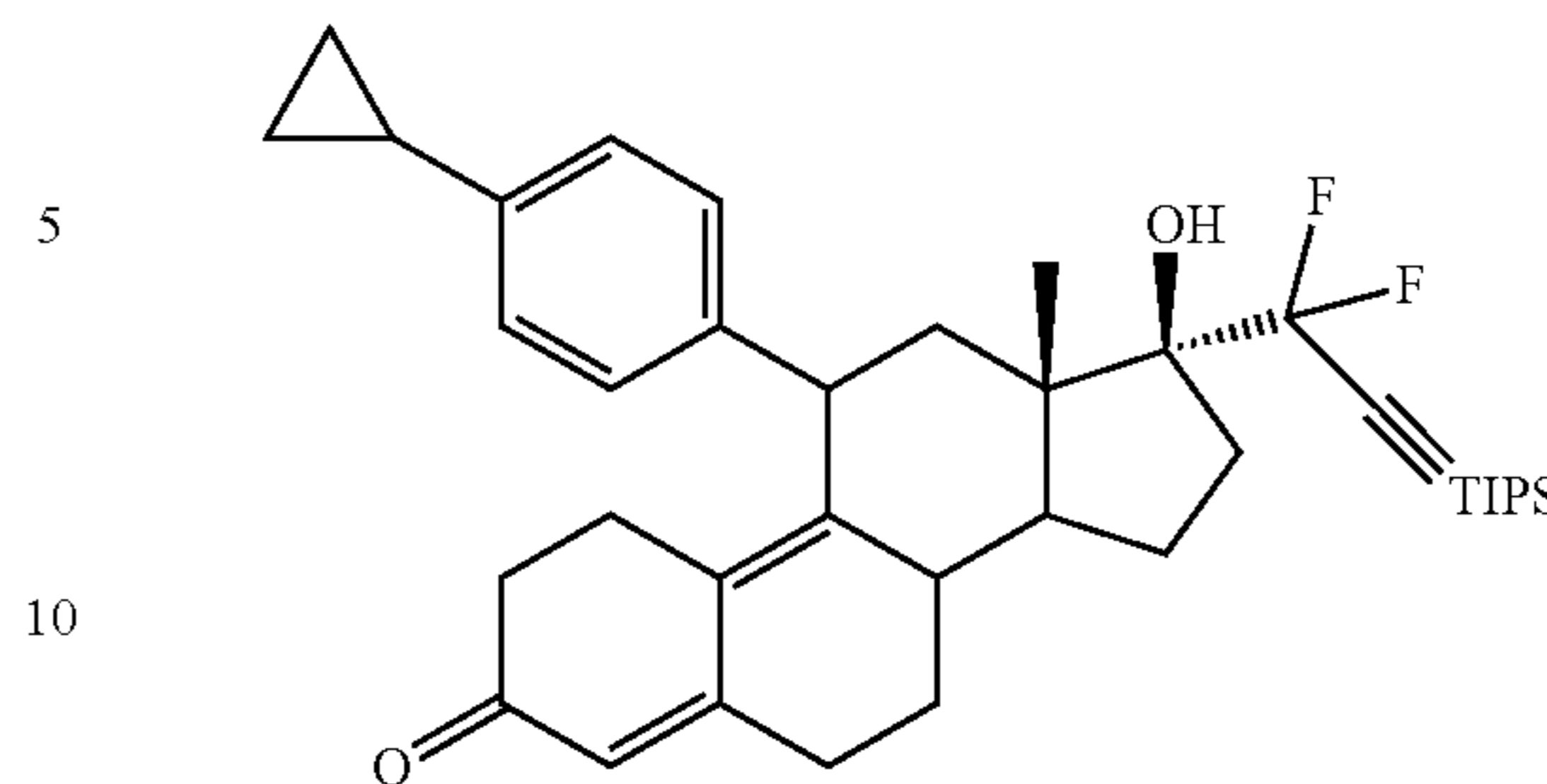
17α-[1,1-difluoro-3-[tris(1-methylethyl)silyl]-2-propyn-1-yl]-17β-hydroxy-11β-[4-p-(cyclopropyl)phenyl]estra-4,9-dien-3-one. (6a)
