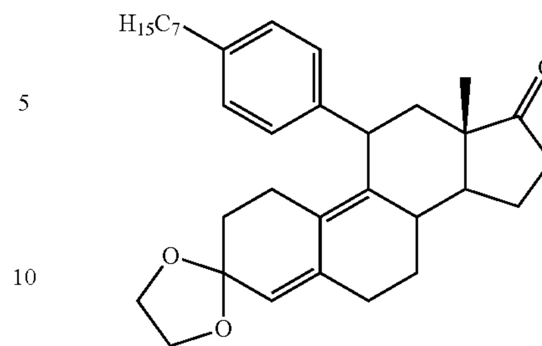
3,3-Ethylendioxy-11 \beta -[4-p-(n-heptyl)phenyl]estra-9-en-17-one (4i)
