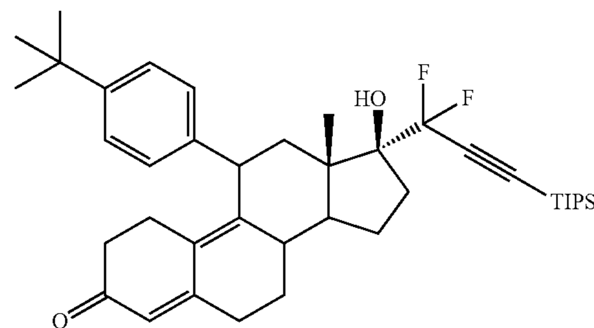
17 \alpha -[1,1-difluoro-3-[tris(1-methylethyl)silyl]-2-propyn-1-yl]-17 \beta -hydroxy-11 \beta -[4-p-(t-butyl)phenyl]estra-4,9-dien-3-one (6f)
