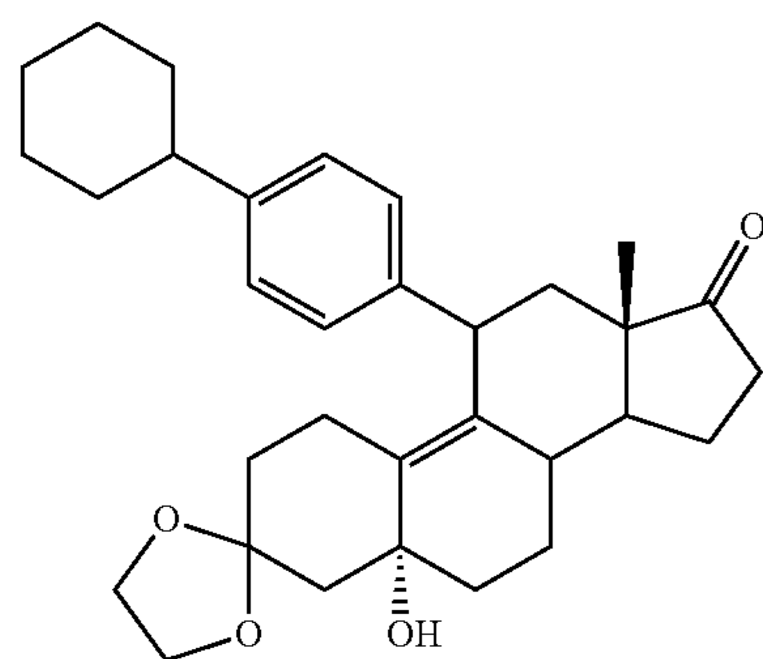
3,3-Ethylendioxy-5 \alpha -hidroxy-11 \beta -[4-p-(cyclohexyl) phenyl]estra-9-en-17-one (3h)
