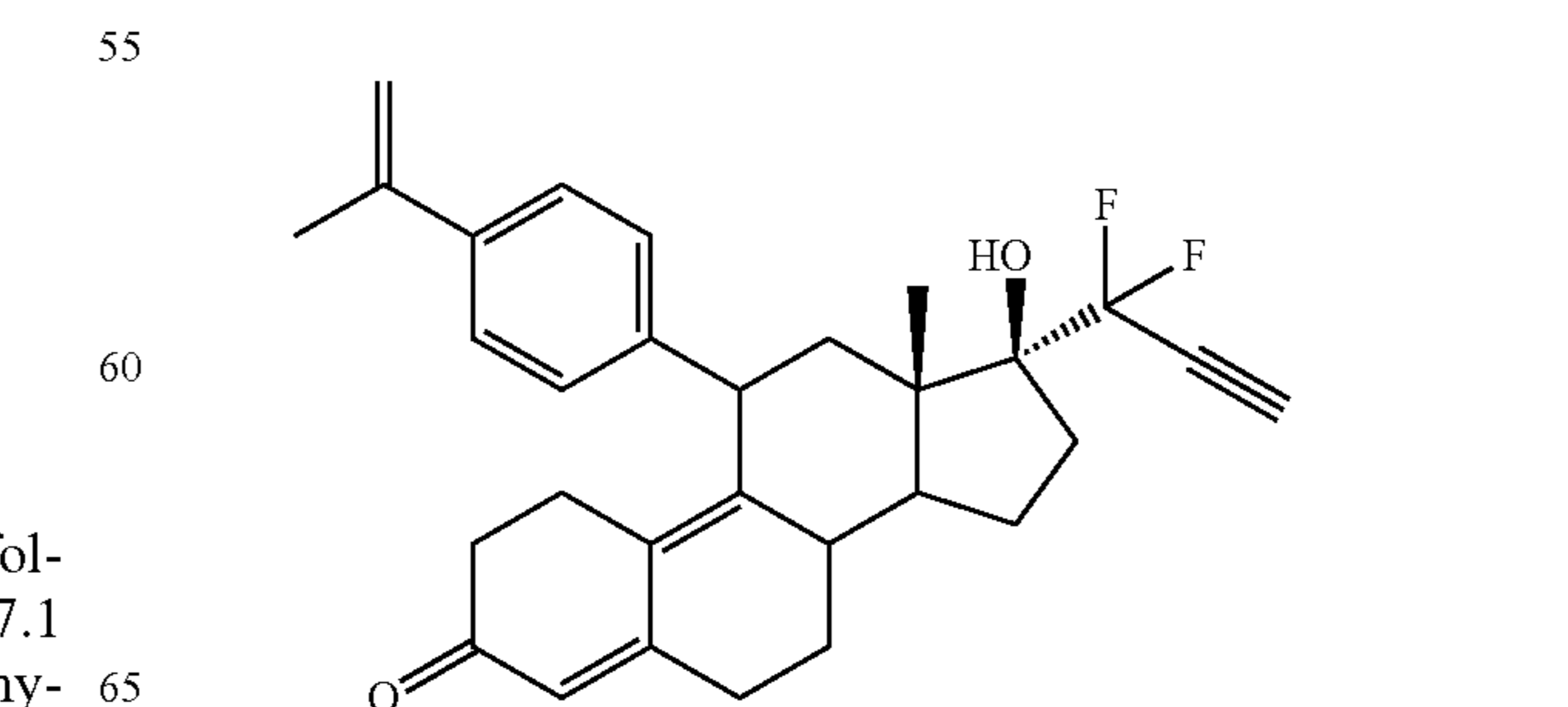
3,3-Ethylendioxy-11 \beta -[4-p-(1-methylethenyl)phenyl]estra-4,9-dien-17-one (4 g)
