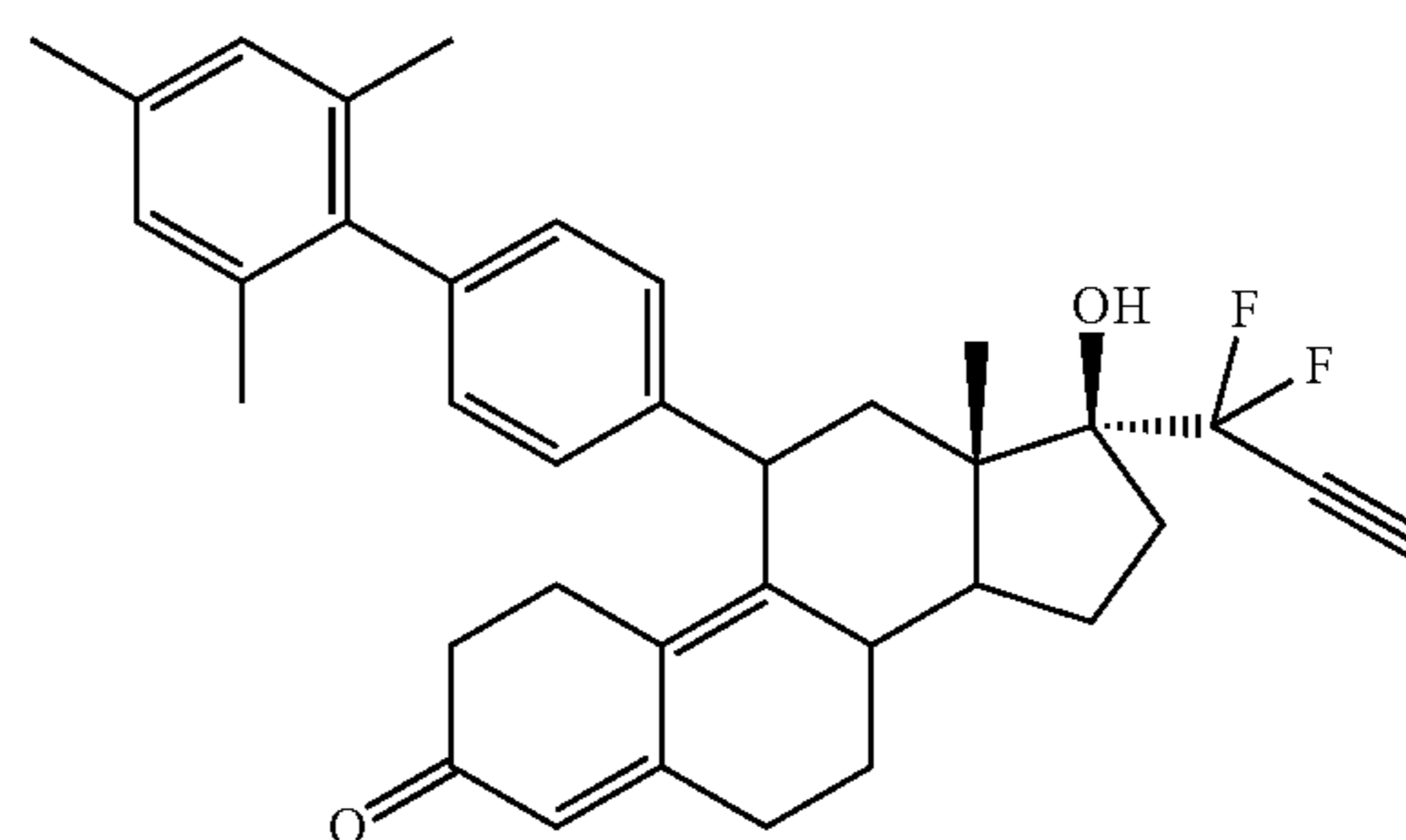
17α-(1,1-difluoro-2-propyn-1-yl)-17β-hydroxy-11β-[4-p-(2,4,6-trimethylphenyl)phenyl]estra-4,9-dien-3-one (EC359)
