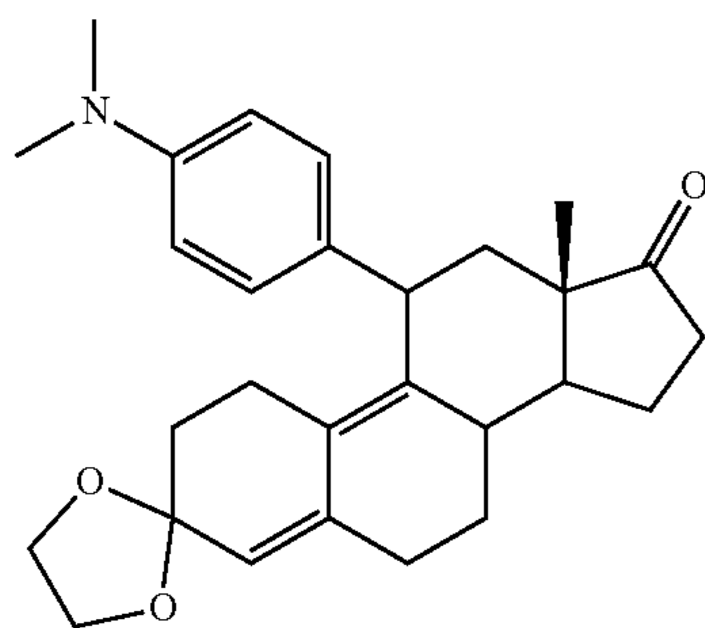
3,3-Ethyldioxy-11 \beta -[4-p-(dimethylamino)phenyl]estra-4,9-dien-17-one (4d)
