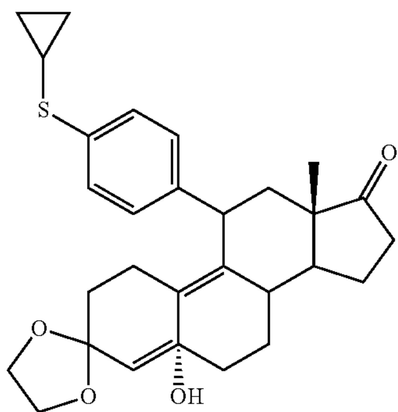
3,3-Ethylendioxy-5 \alpha -hidroxy-11 \beta -[4-p-(cyclopropylthio)phenyl]estra-9-en-17-one (31)
