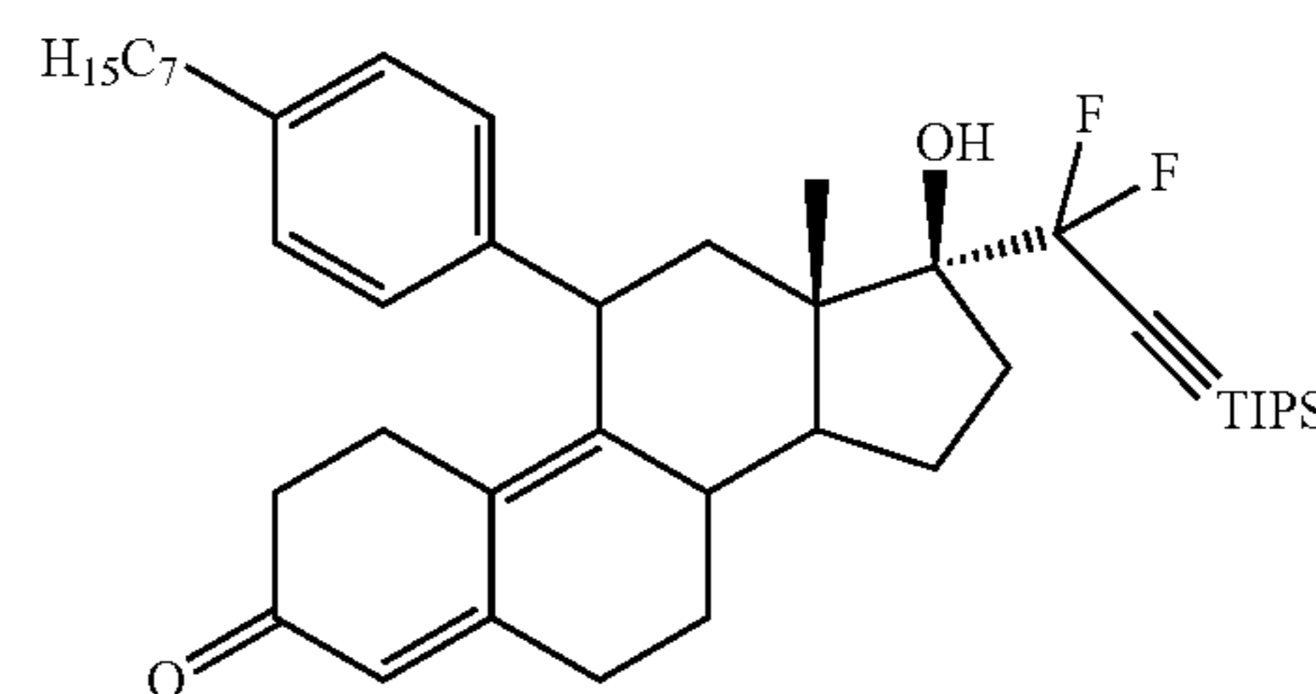
17 \alpha -[1,1-difluoro-3-[tris(1-methylethyl)silyl]-2-propyn-1-yl]-17 \beta -hydroxy-11 \beta -[4-p-(n-heptyl)phenyl]estra-4,9-dien-3-one (6i)
