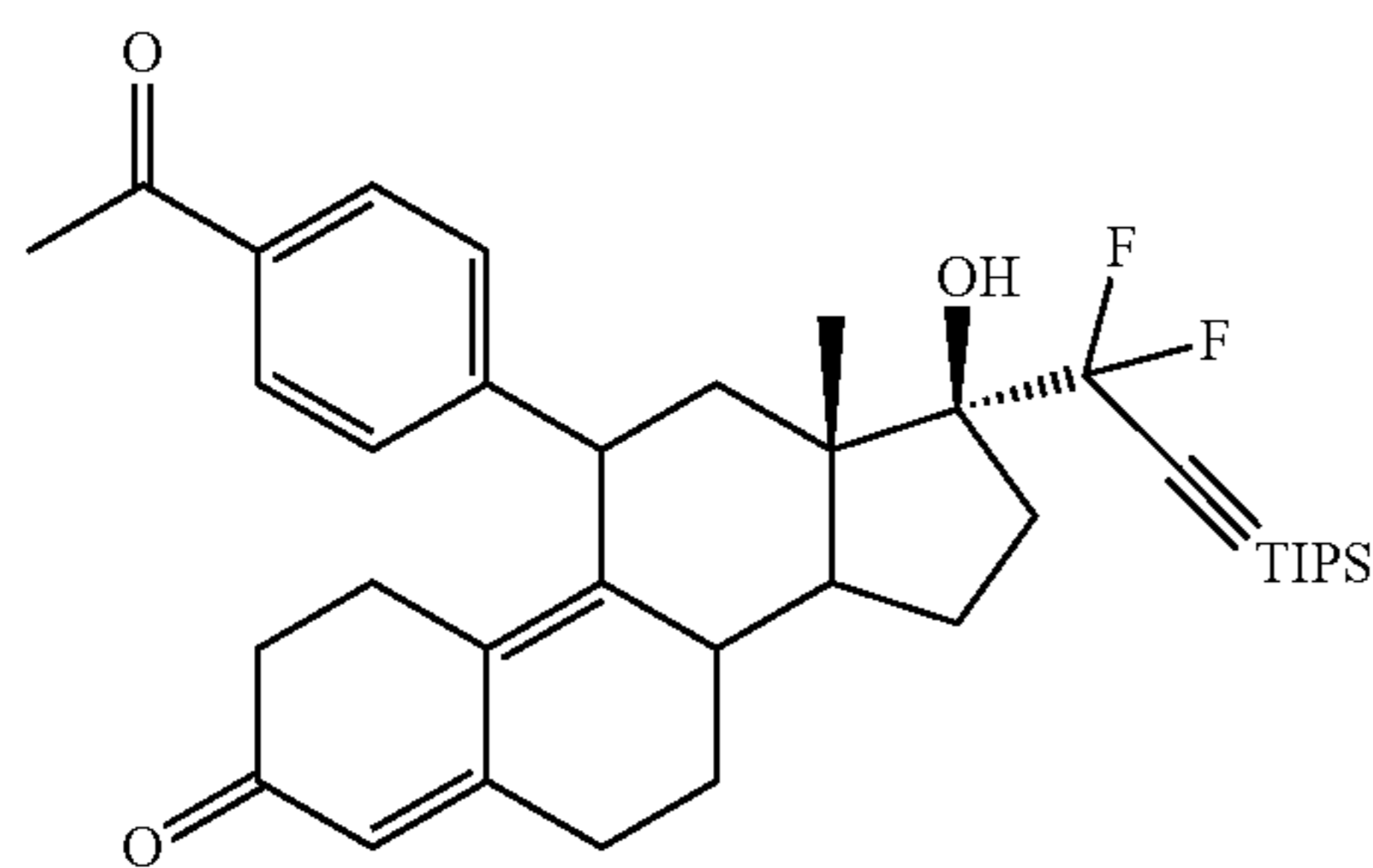
17 \alpha -[1,1-difluoro-3-[tris(1-methylethyl)silyl]-2-propyn-1-yl]-17 \beta -hydroxy-11 \beta -[4-p-(acetyl)phenyl]estra-4,9-dien-3-one. (6b)
