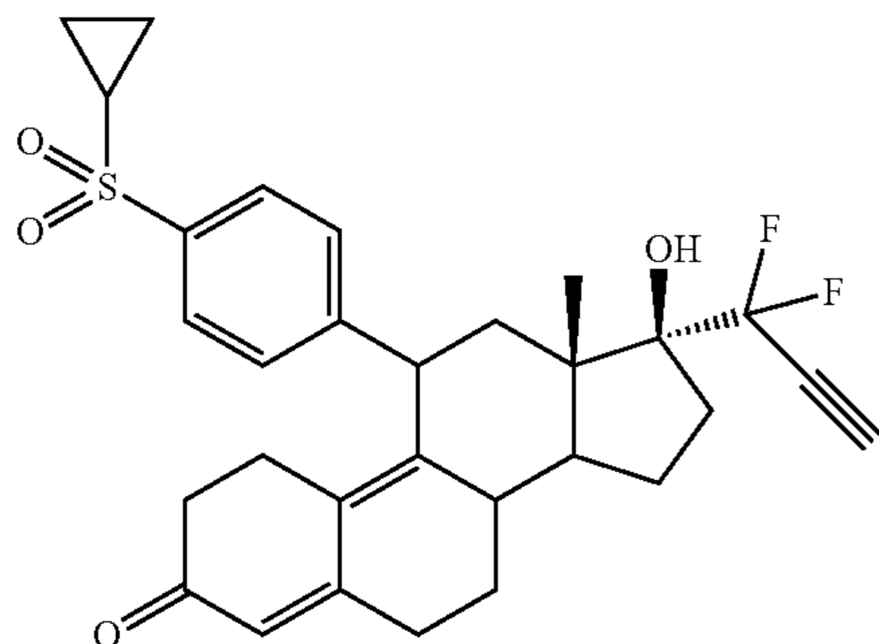
17 \alpha -(1,1-difluoro-2-propyn-1-yl)-17 \beta -hydroxy-11 \beta -[4-p-(cyclopropylsulfonyl)phenyl]estra-4,9-dien-3-one (EC361)
