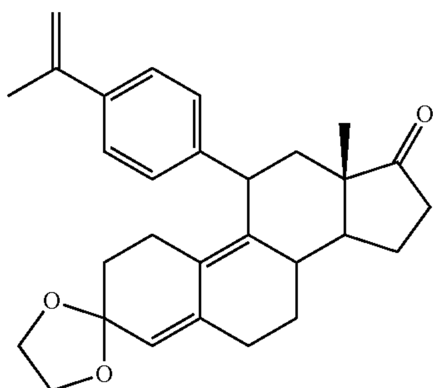
3,3-Ethylendioxy-11 \beta -[4-p-(1-methylethenyl)phenyl]estra-4,9-dien-17-one (4 g)
