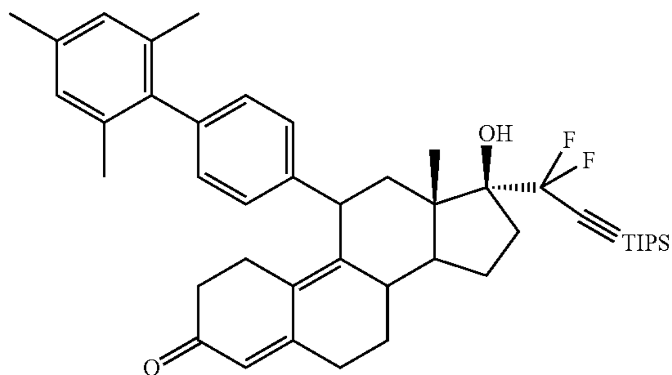
17α-[1,1-difluoro-3-[tris(1-methylethyl)silyl]-2-propyn-1-yl]-17β-hydroxy-11β-[4-p-(2,4,6-trimethylphenyl)phenyl]estra-4,9-dien-3-one (6k)
