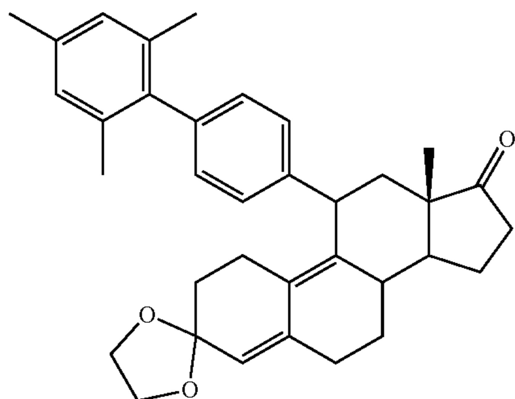
3,3-Ethylendioxy-11β-[4-p-(2,4,6-trimethylphenyl)phenyl]estra-4,9-dien-17-one (4k)
