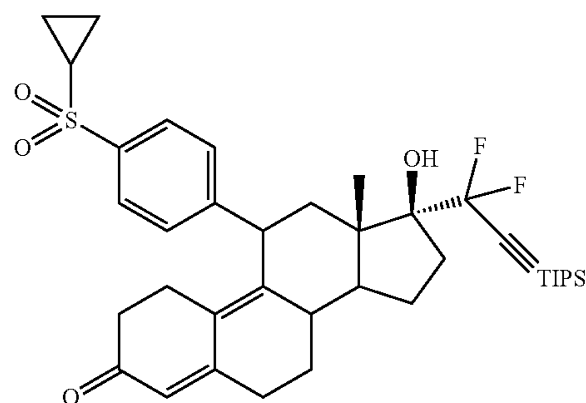
17 \alpha -[1,1-difluoro-3-[tris(1-methylethyl)silyl]-2-propyn-1-yl]-17 \beta -hidroxy-11 \beta -[4-p-(cyclopropylsulfonyl)phenyl]estra-4,9-dien-3-one (61)
