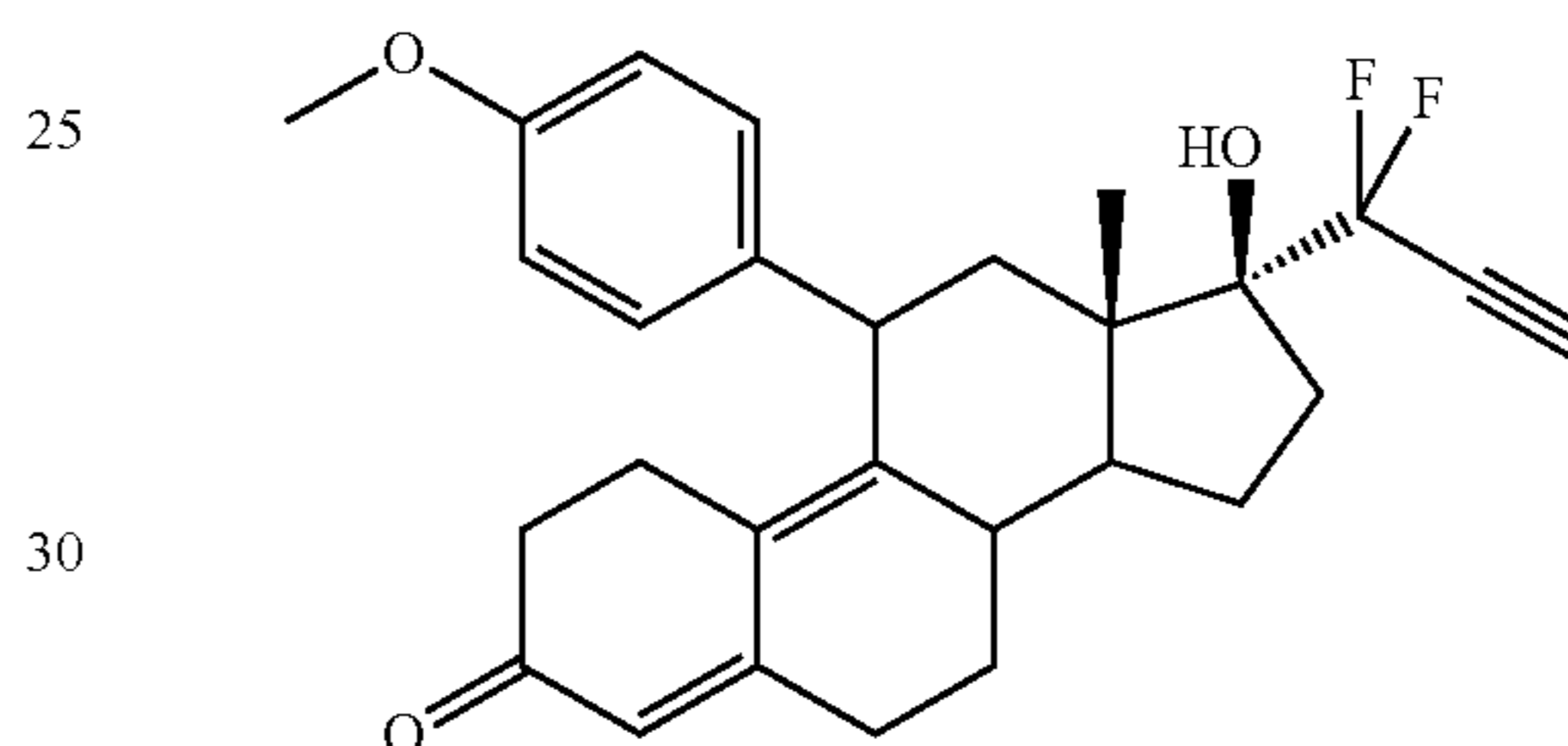
17 \alpha -(1,1-difluoro-2-propyn-1-yl)-17 \beta -hidroxy-11 \beta -[4-p-(methoxy)phenyl]estra-4,9-dien-3-one (EC356)
