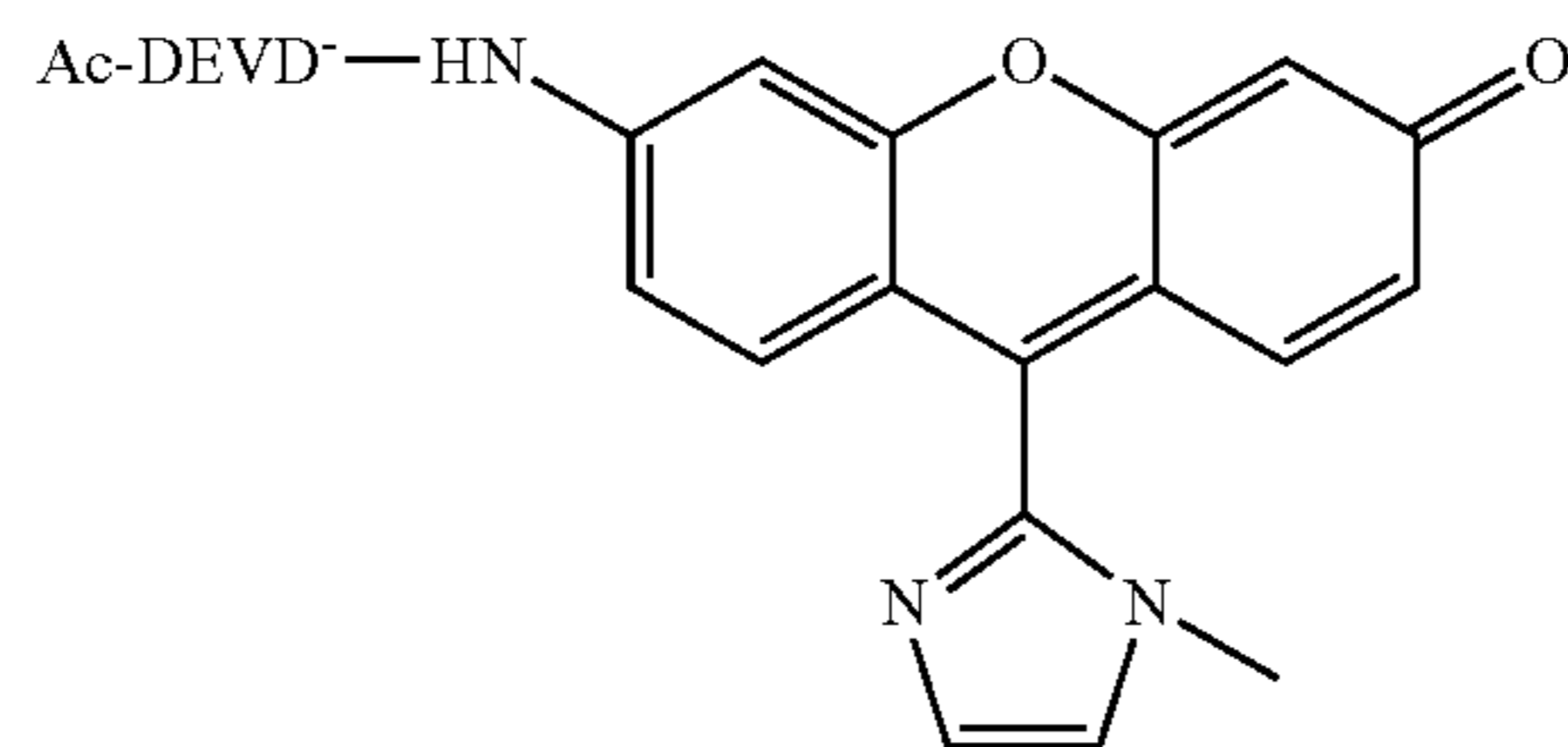
Caspase-3 substrate
