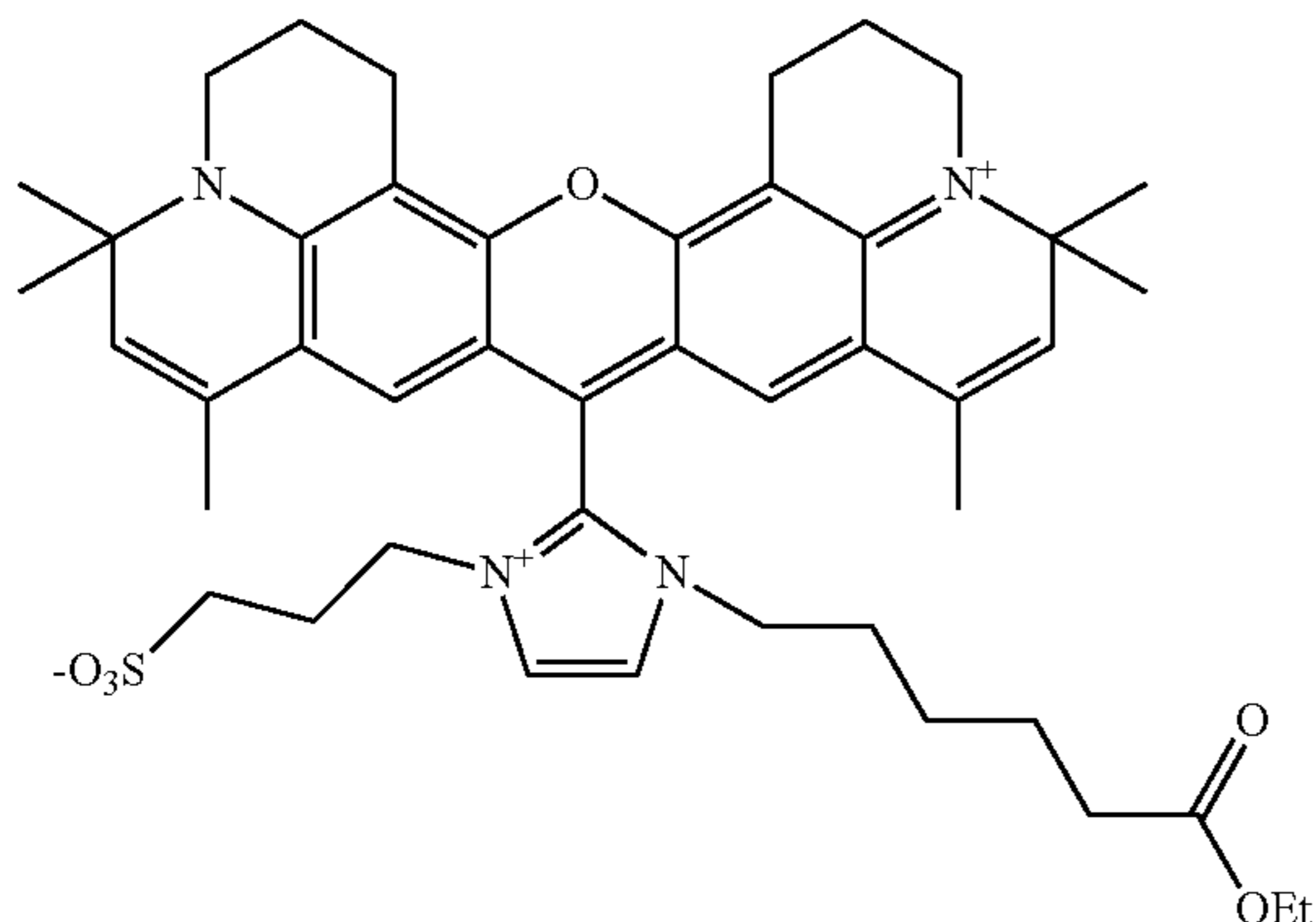
Compound No. 90
