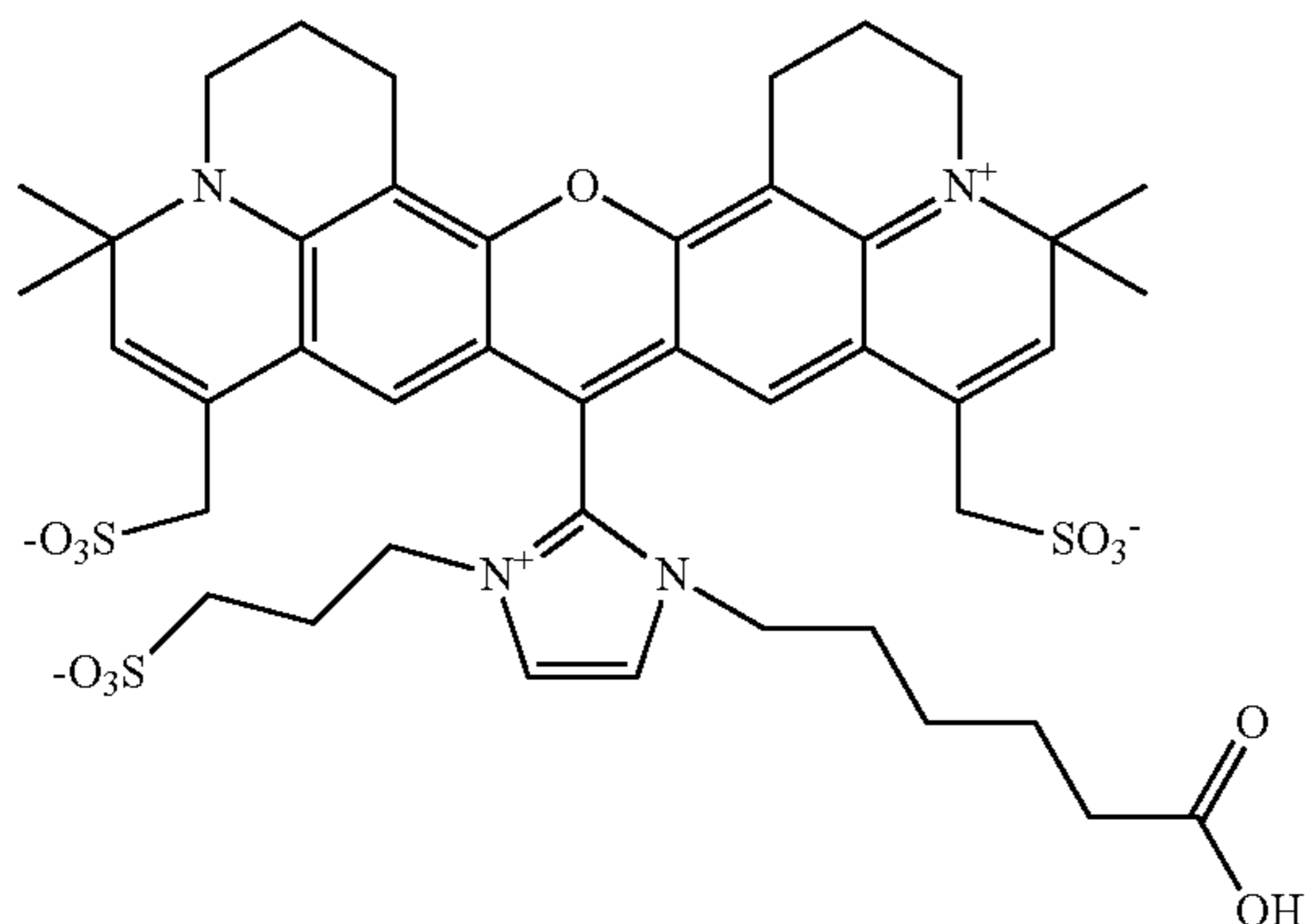
Compound No. 91
