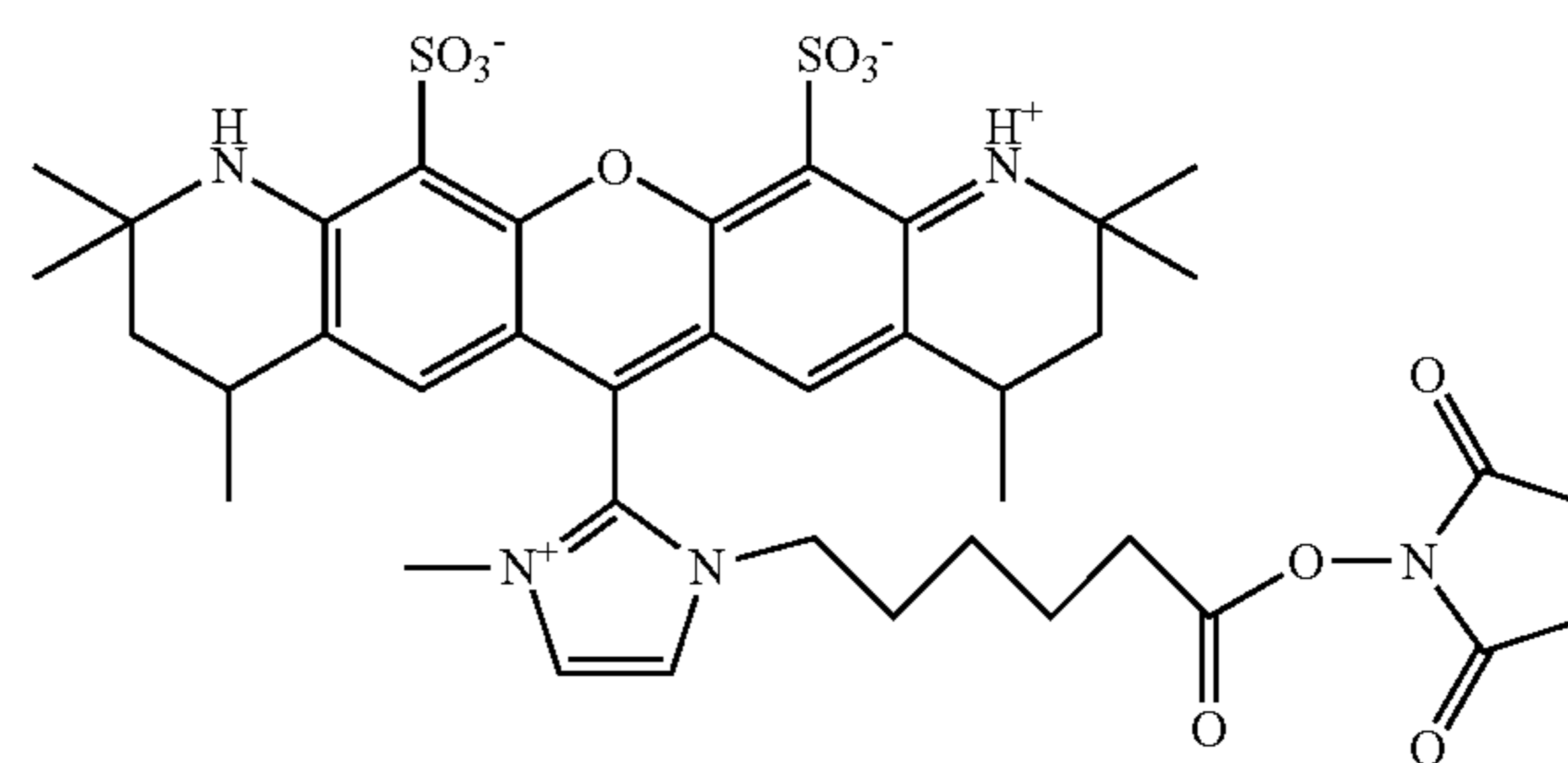
Compound No. 29
