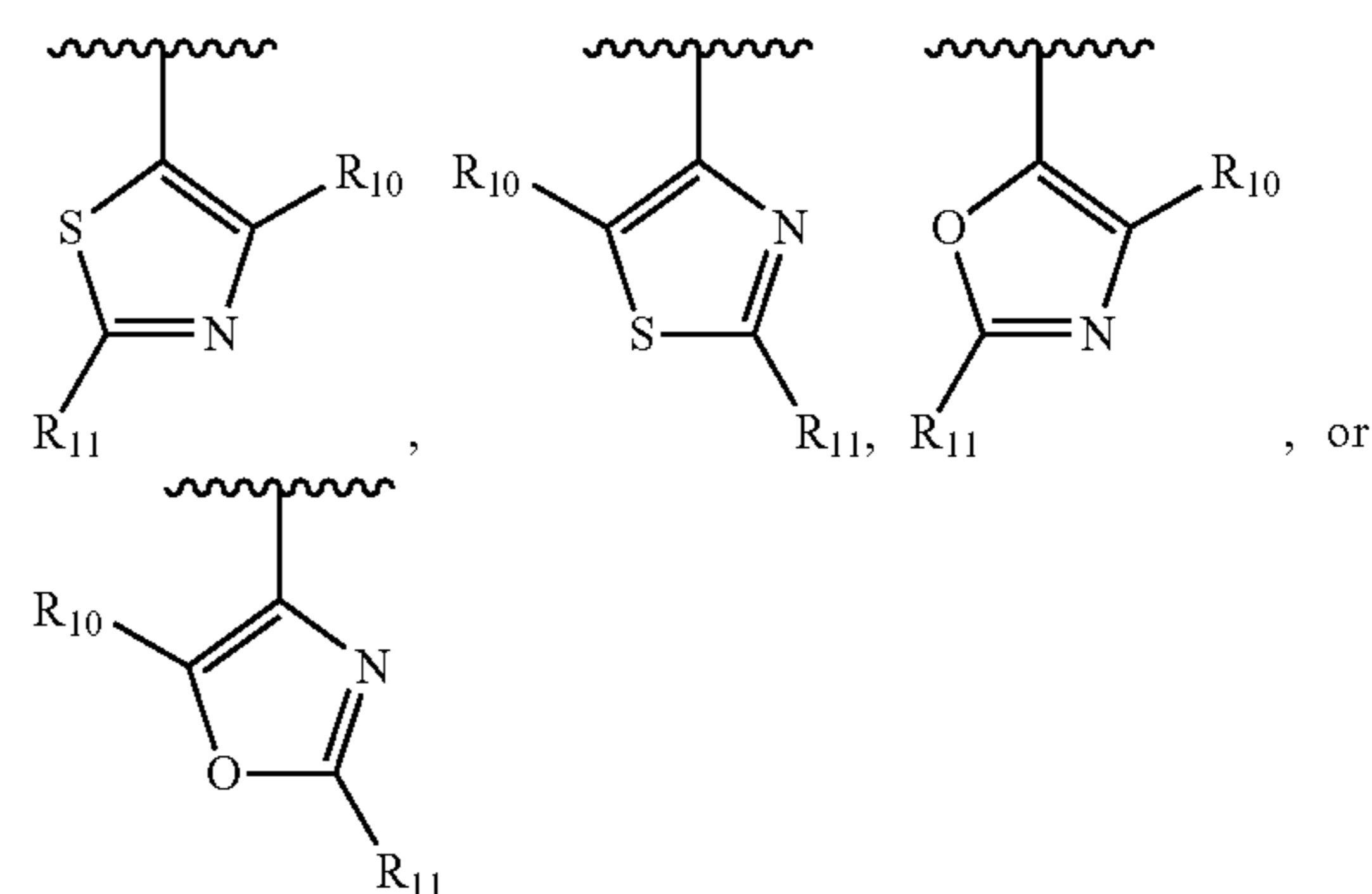
Formula 1a
