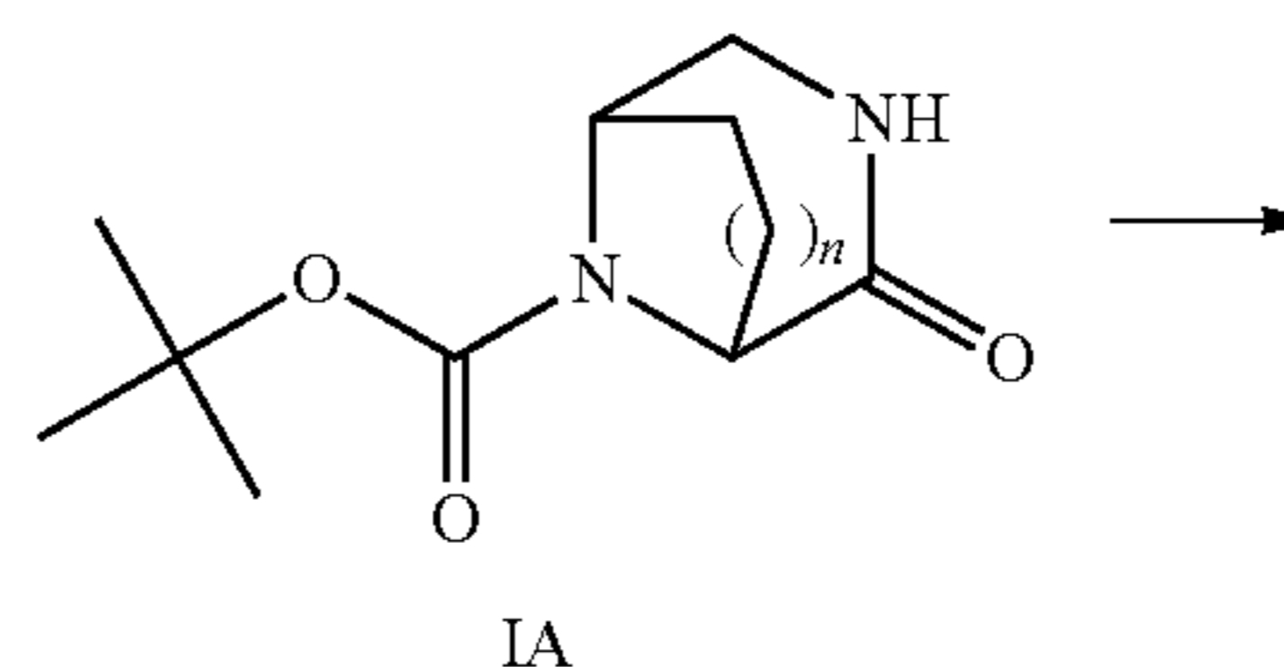
Scheme 1
