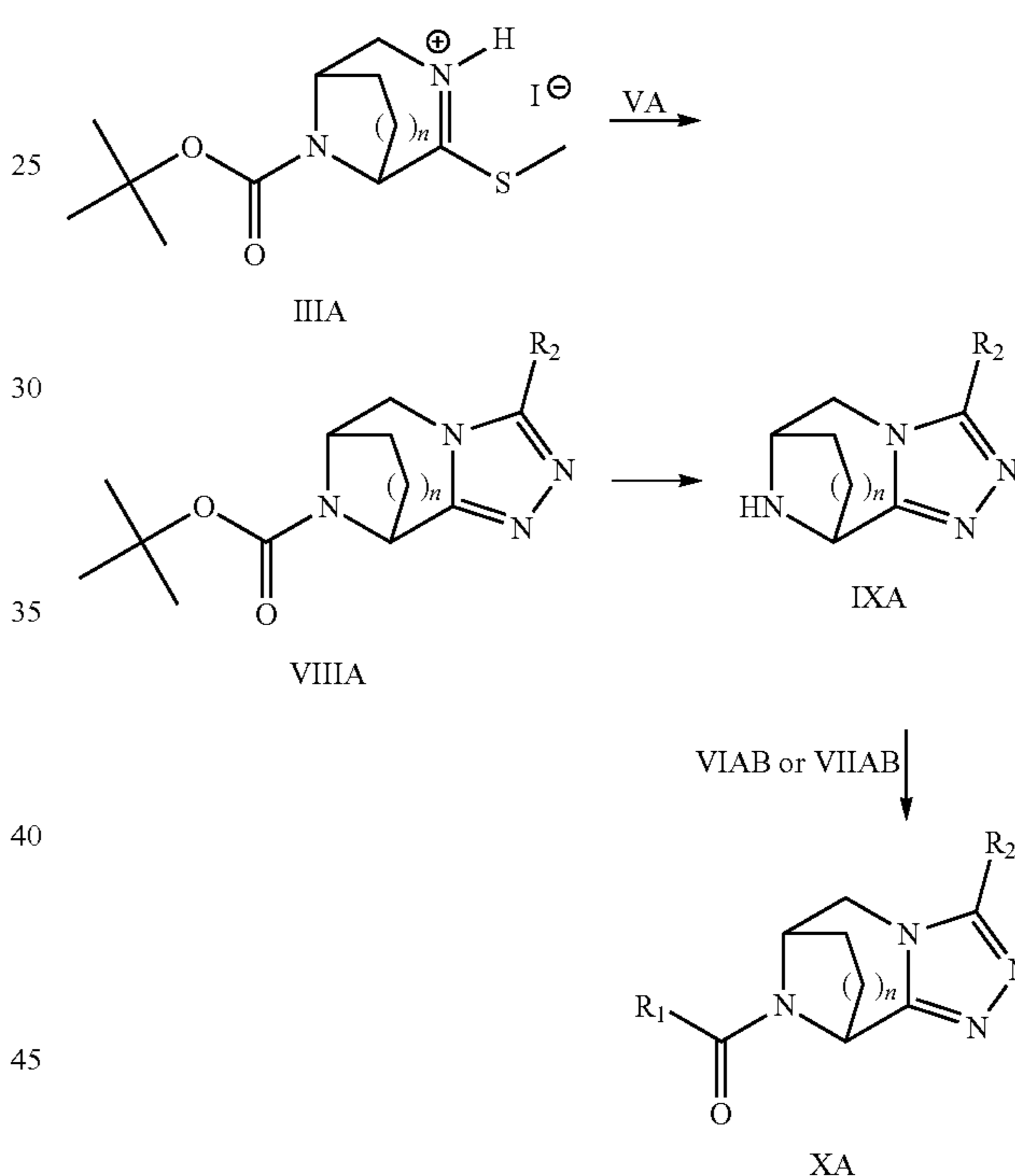
Scheme 3
