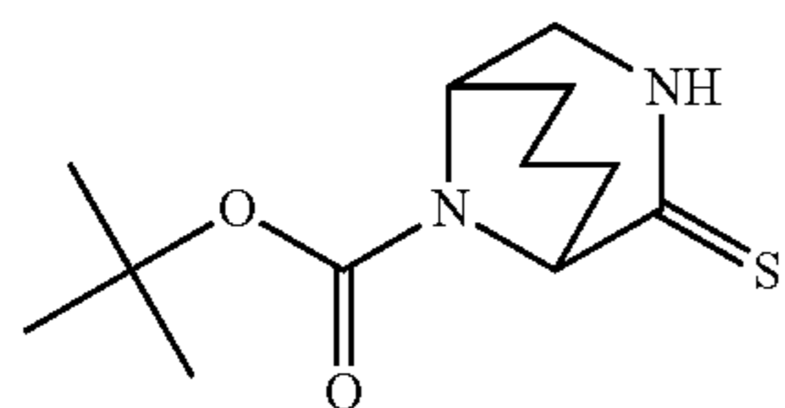
Intermediate B: tert-Butyl 2-thioxo-3,9-diazabicyclo[3.3.1]nonane-9-carboxylate
