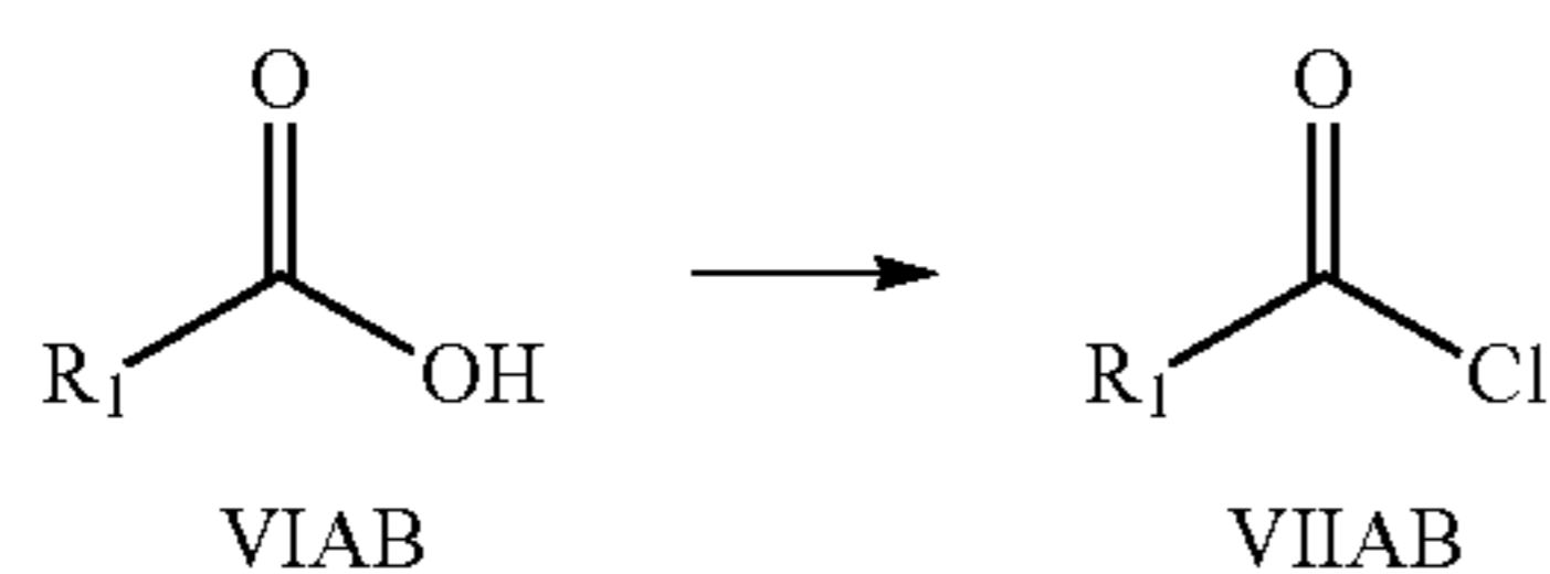
Scheme 2B
