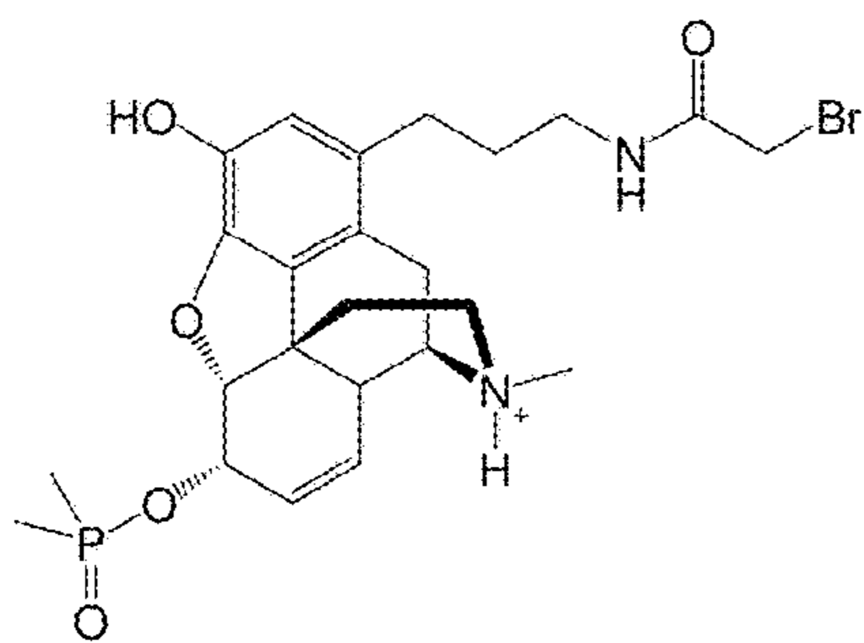
1-Aminopropyl-N-Bromoacetyl-6PM
