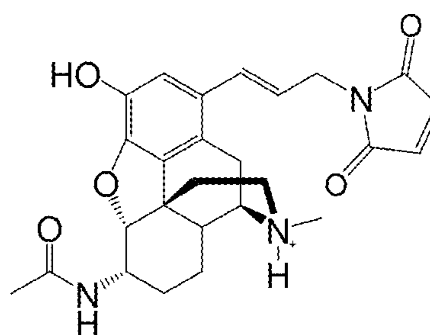
1-Maleimido-N-propenyl-6-AHM
