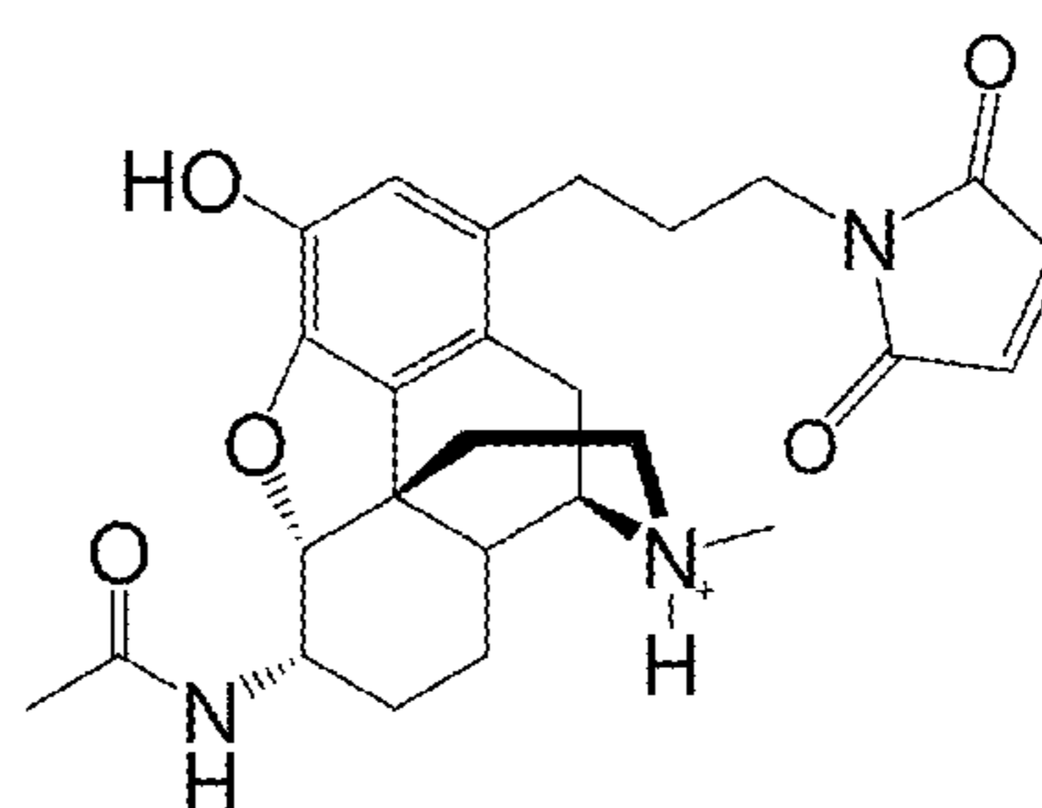
1-Maleimido-N-propyl-6-AHM
