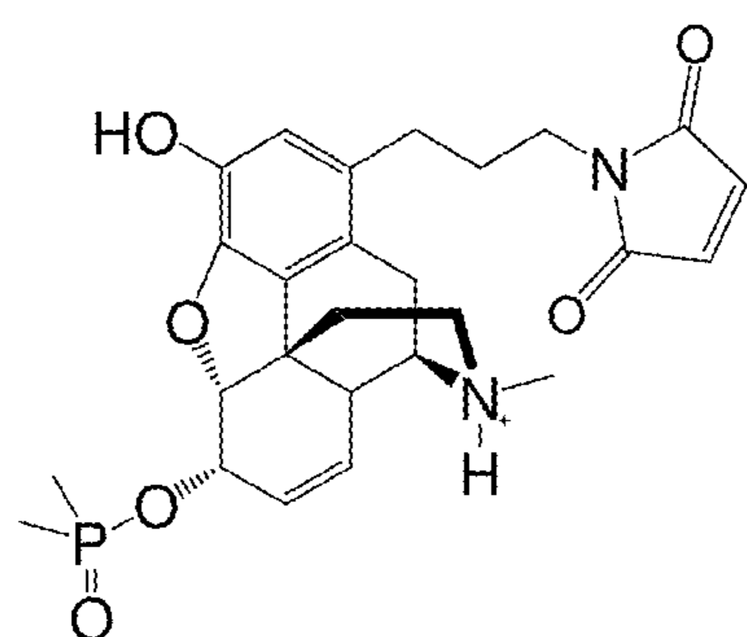
1-Maleimido-N-propyl-6PM
