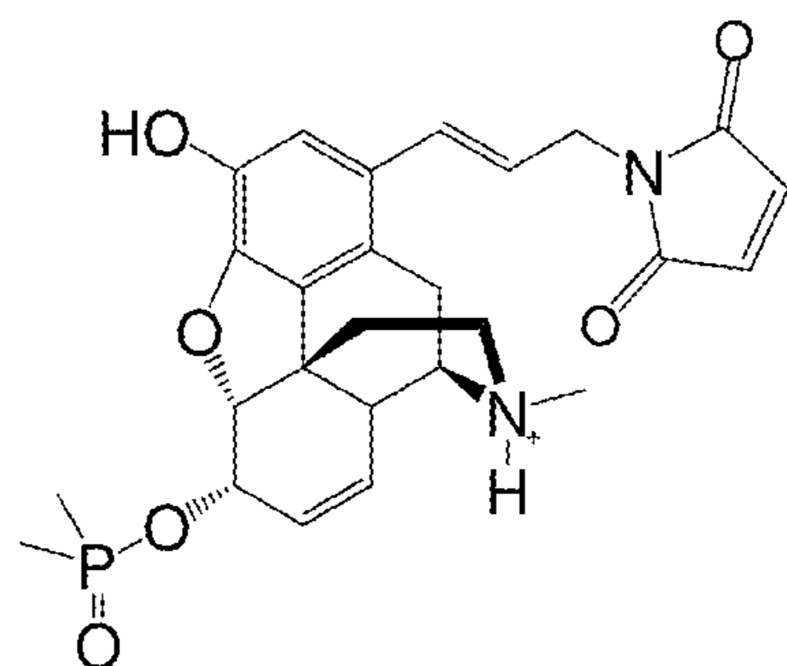
1-Maleimido-N-propenyl-6PM
