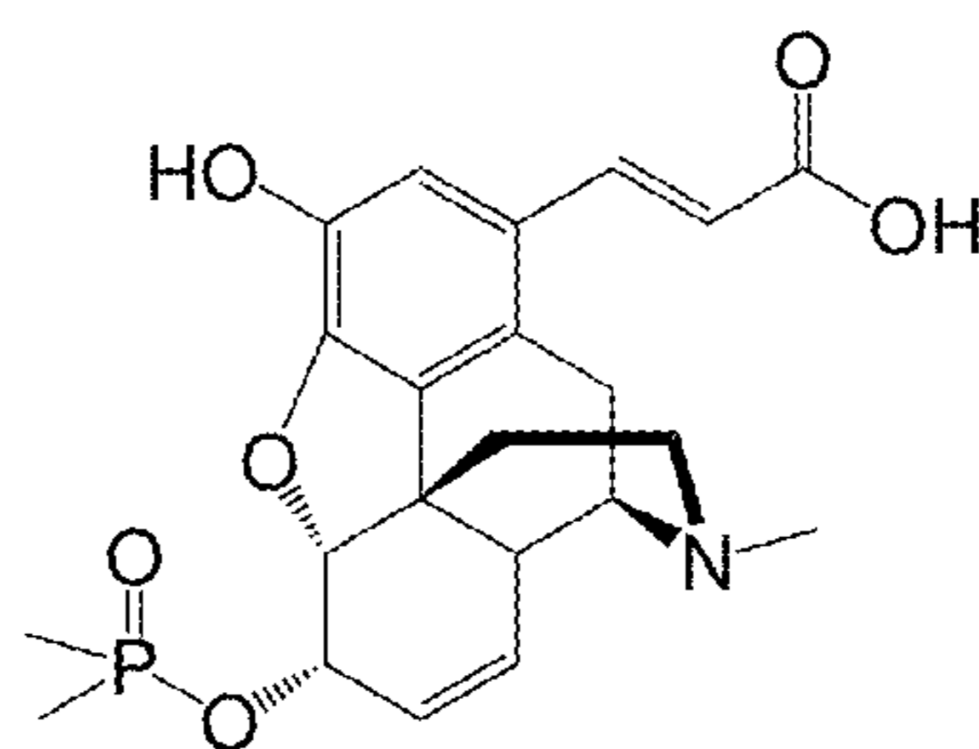
6-Phosphinyl Alkene
