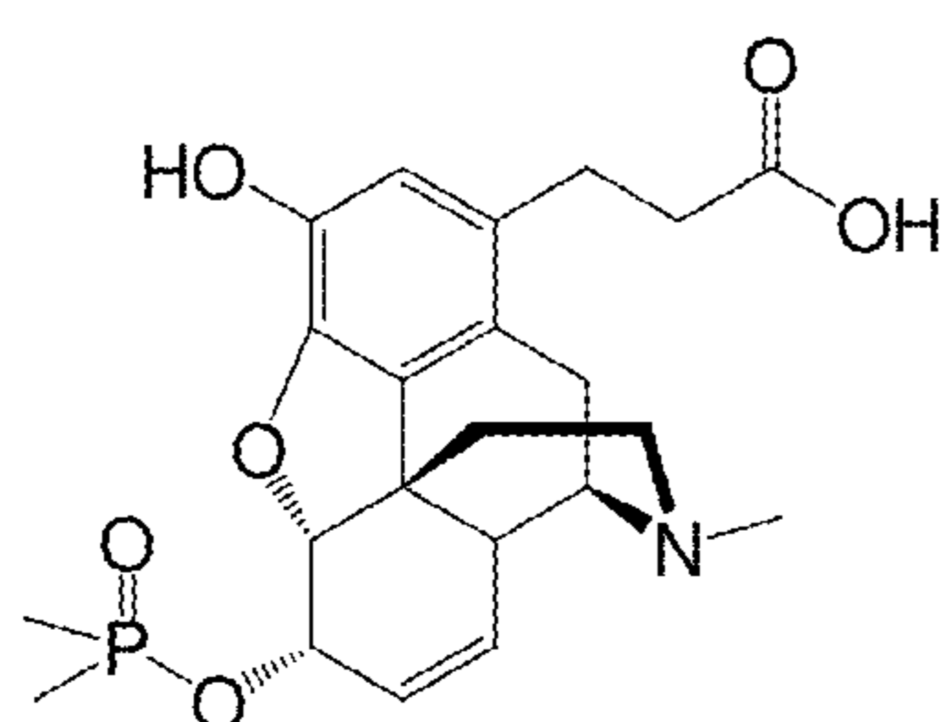
6-Phosphinyl Alkane
