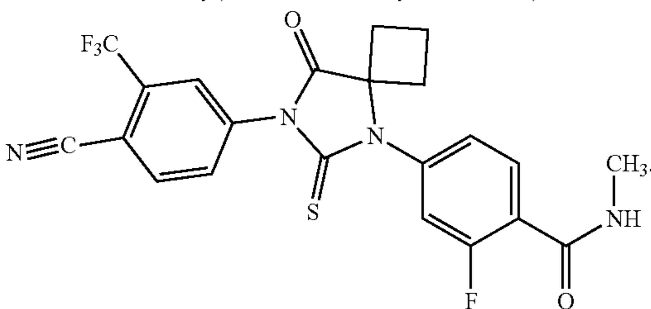
4-[7-(4-cyano-3-trifluoromethylphenyl)-8-oxo-6-thioxo-5,7-diazaspiro[3.4]oct-5-yl]-2-fluoro-N-methylbenzamide (RD162)
