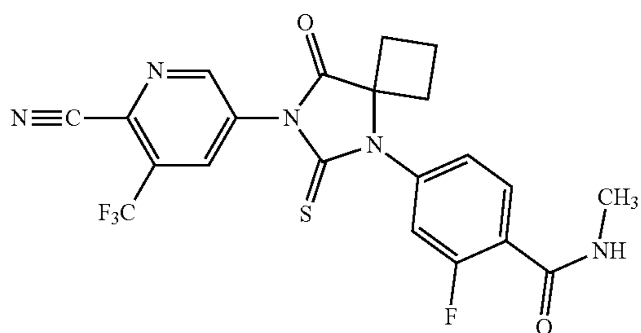
4-[7-(6-cyano-5-trifluoromethylpyridin-3-yl)-8-oxo-6-thioxo-5,7-diazaspiro[3.4]oct-5-yl]-2-fluoro-N-methylbenzamide (ARN-509)
