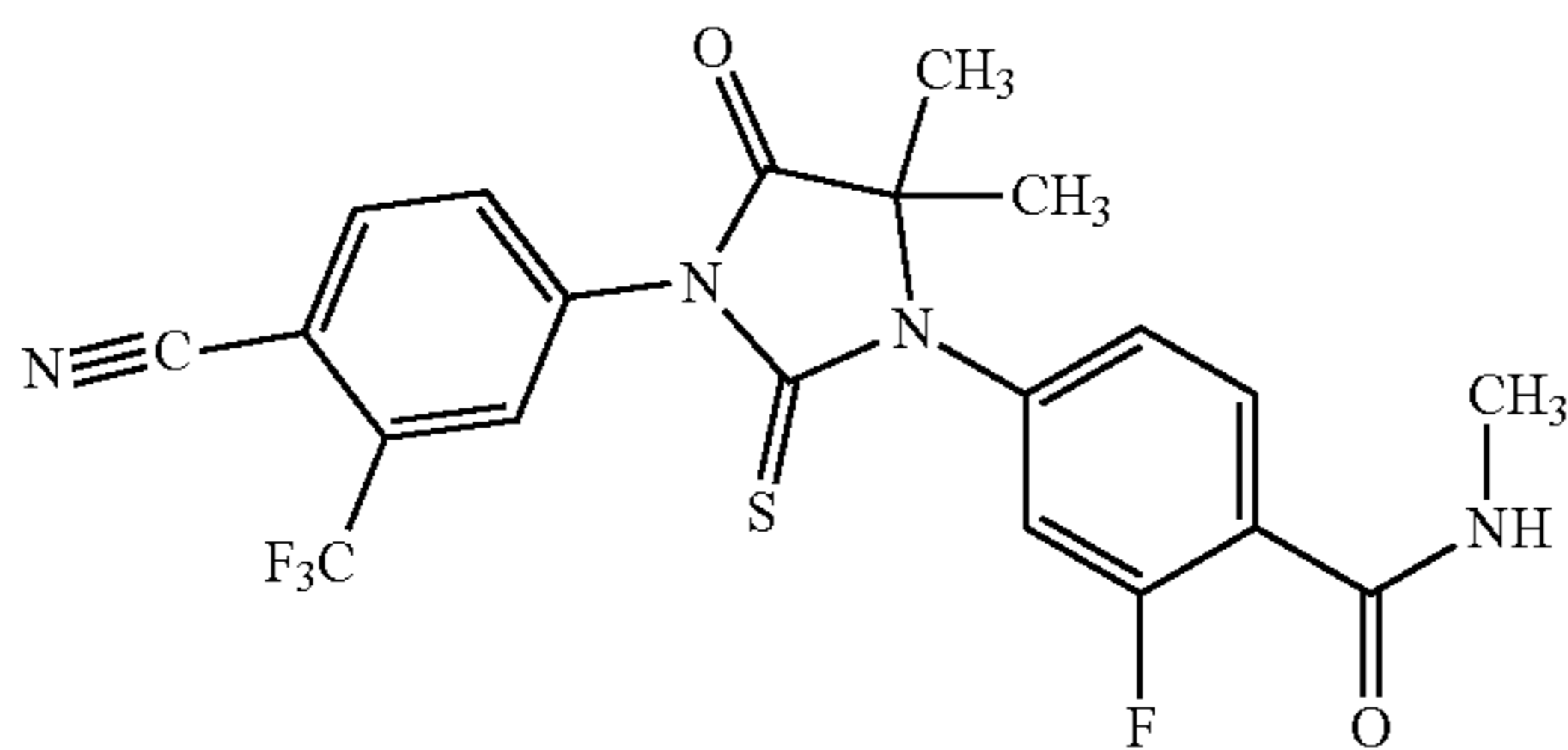
4-(3-(4-cyano-3-(trifluoromethyl)phenyl)-5,5-dimethyl-4-oxo-2-thioxoimidazolidin-1-yl)-2-fluoro-N-methylbenzamide (enzalutamide)
