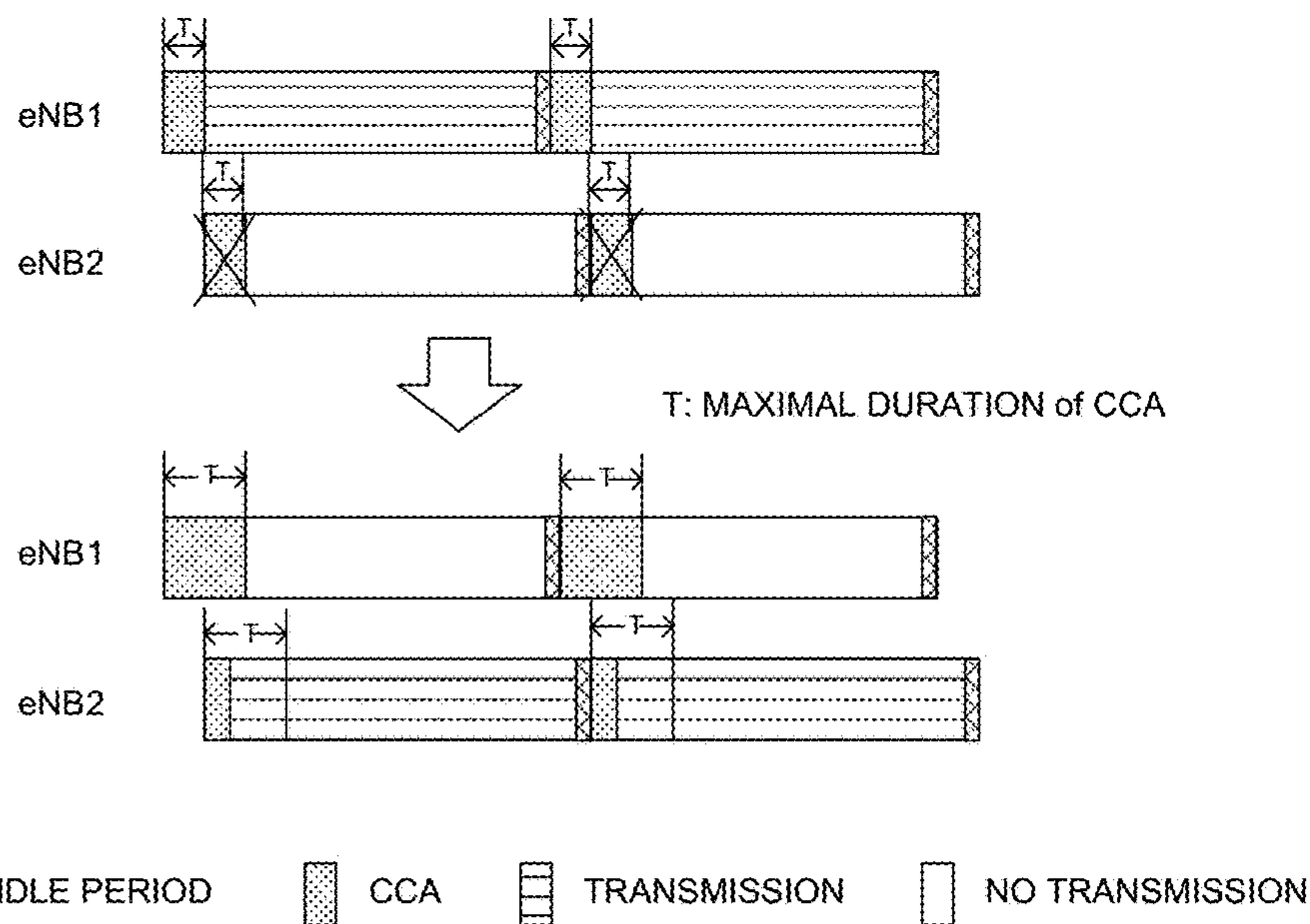
ASYNCHRONOUS NETWORK
