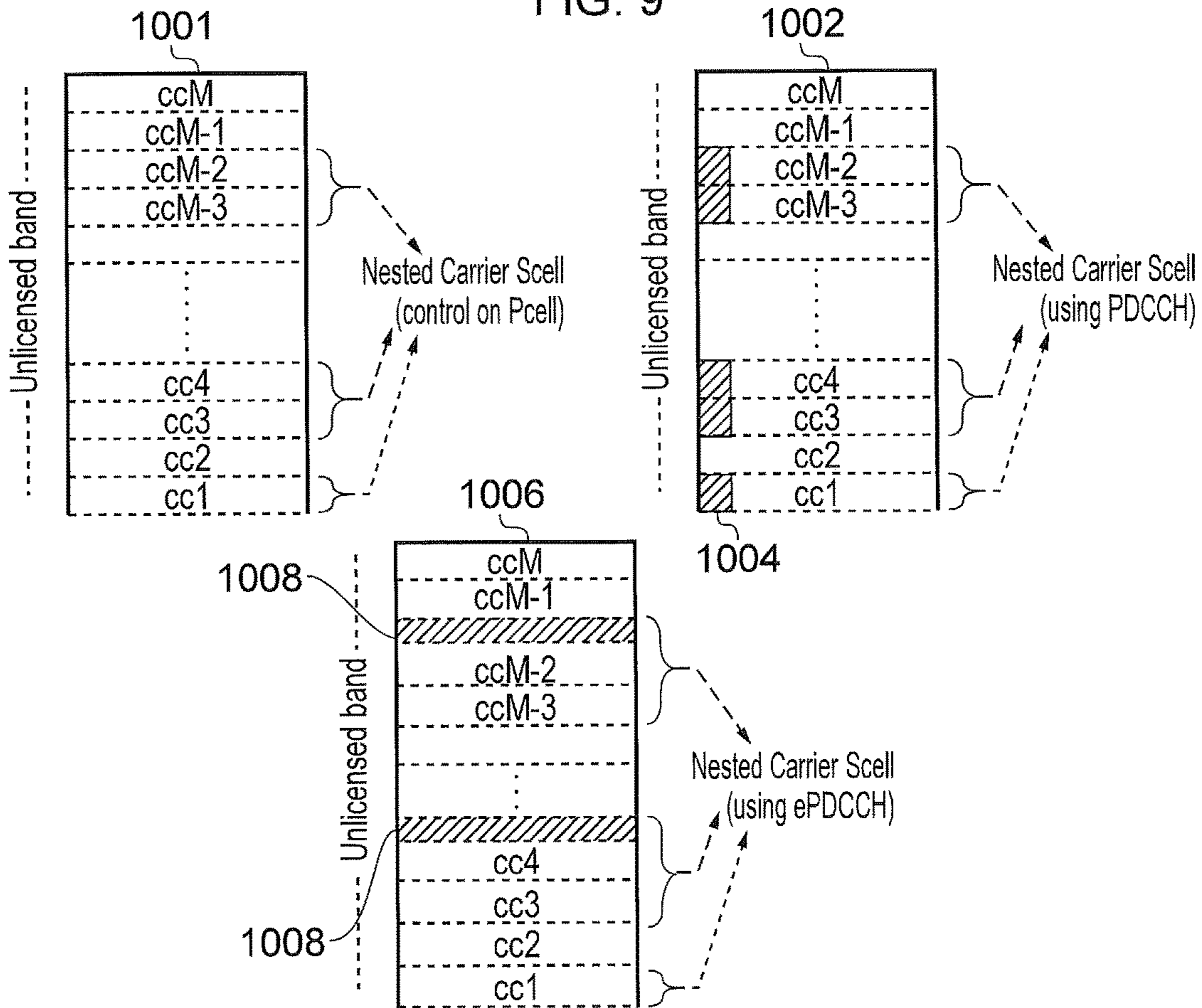
PDCCH and EPDCCH arrangement in the candidate channels comprising a nested carrier.
