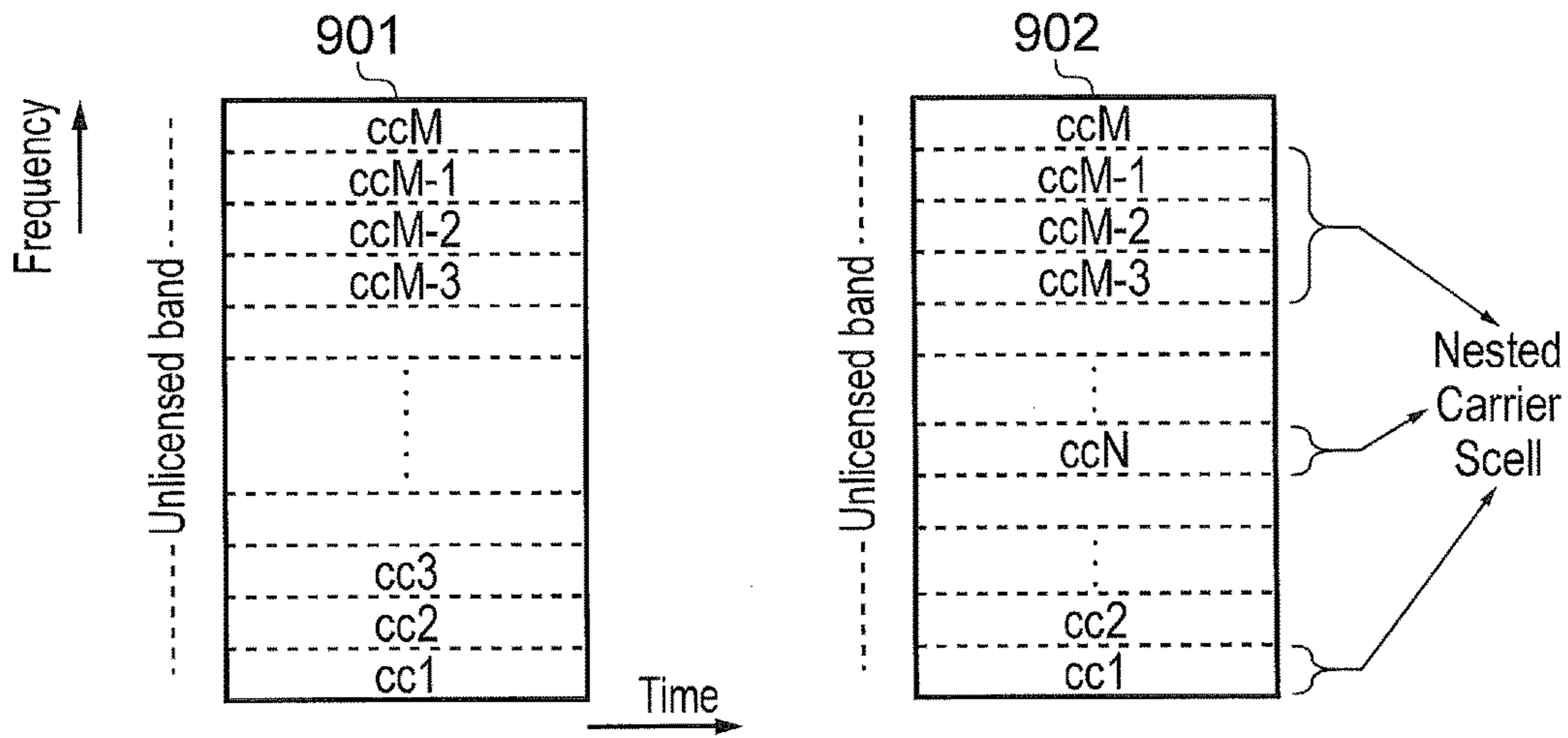
Definition of candidate channels within U-resources and logical aggregation of some candidate channels into a nested carrier. (NB other wireless systems are transmitting in any parts of the unlicensed band, including those not used by any activated candidate channel).
