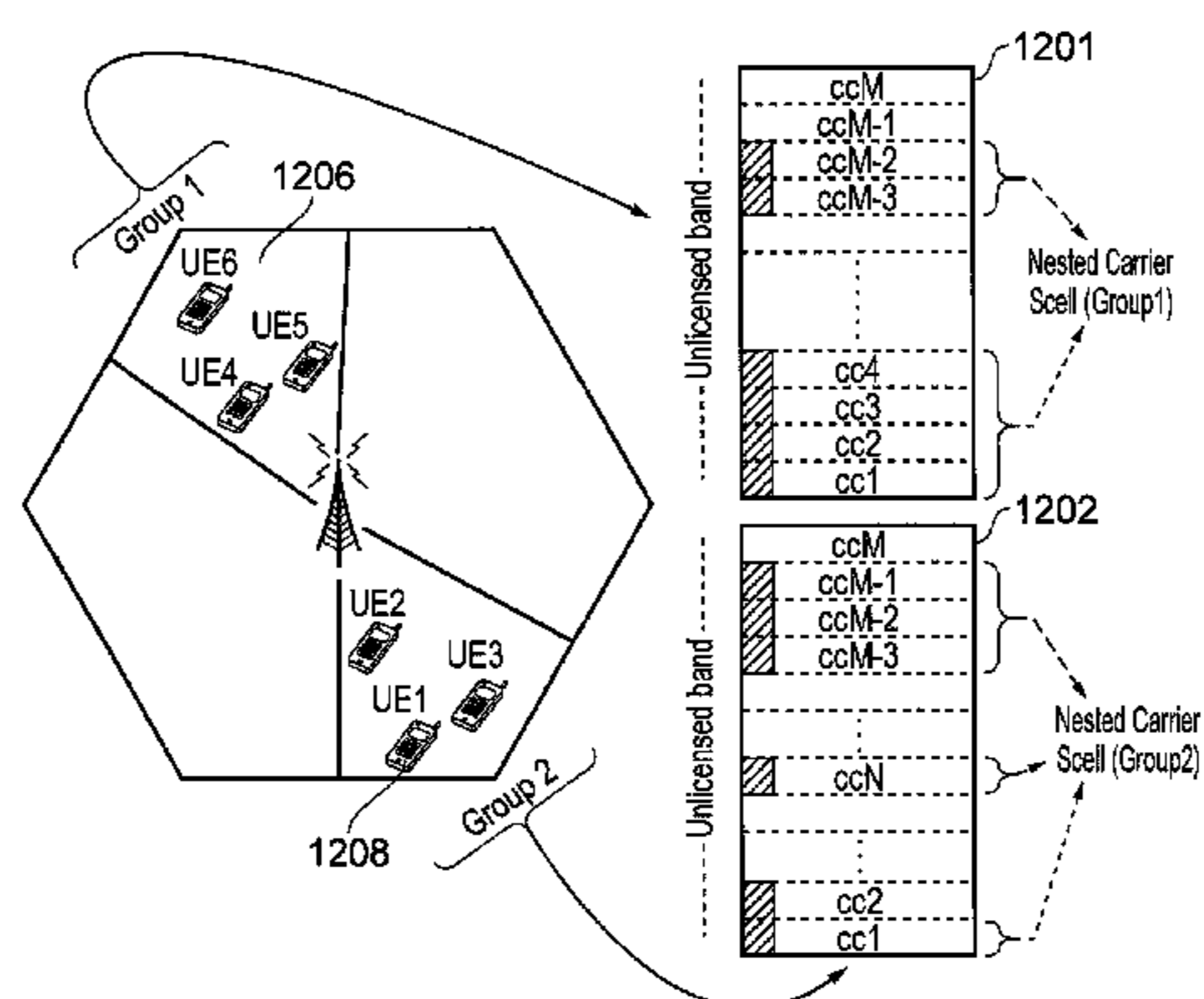
Spatial re-use of candidate channels within a macrocell
