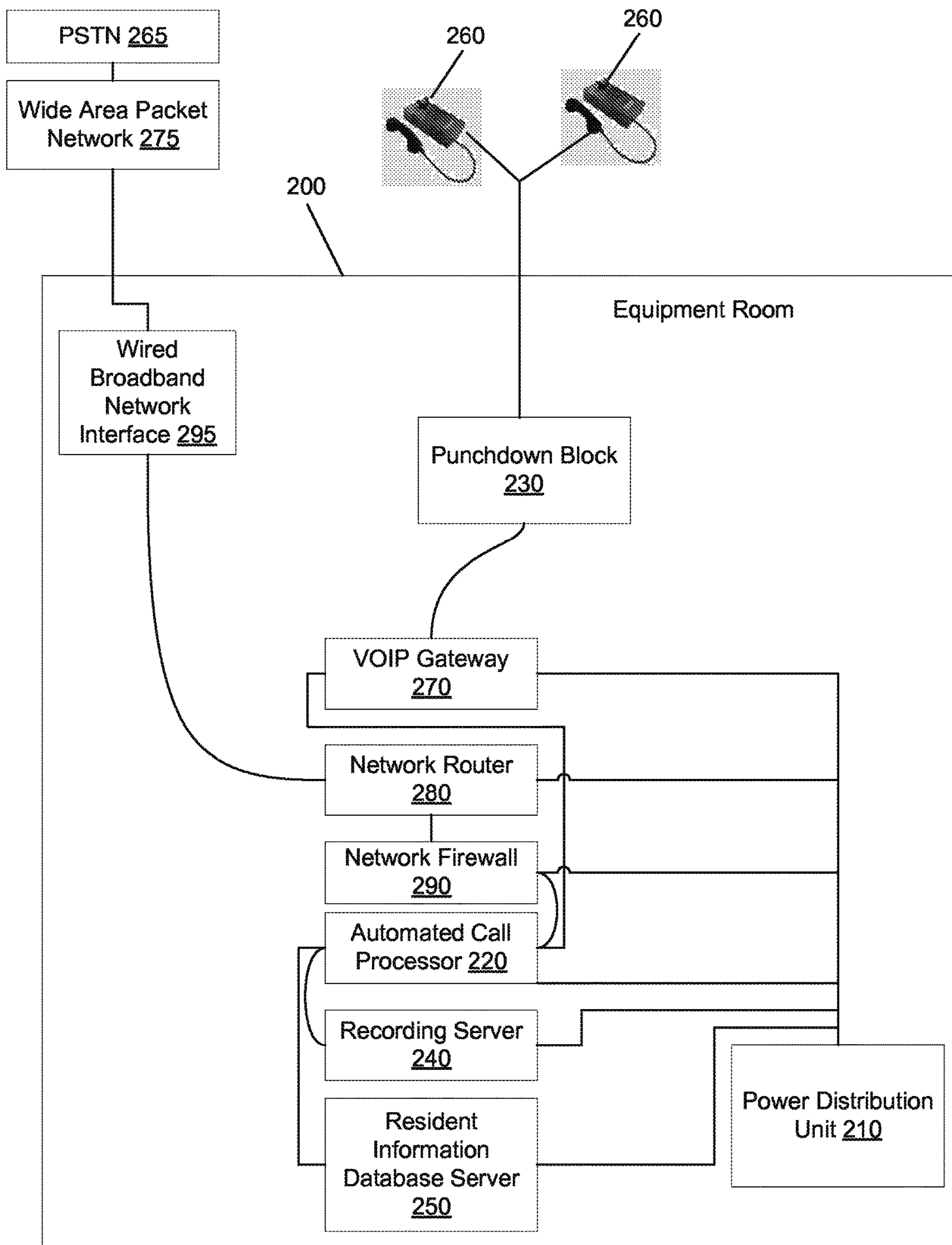
Figure 2 (Prior Art)
