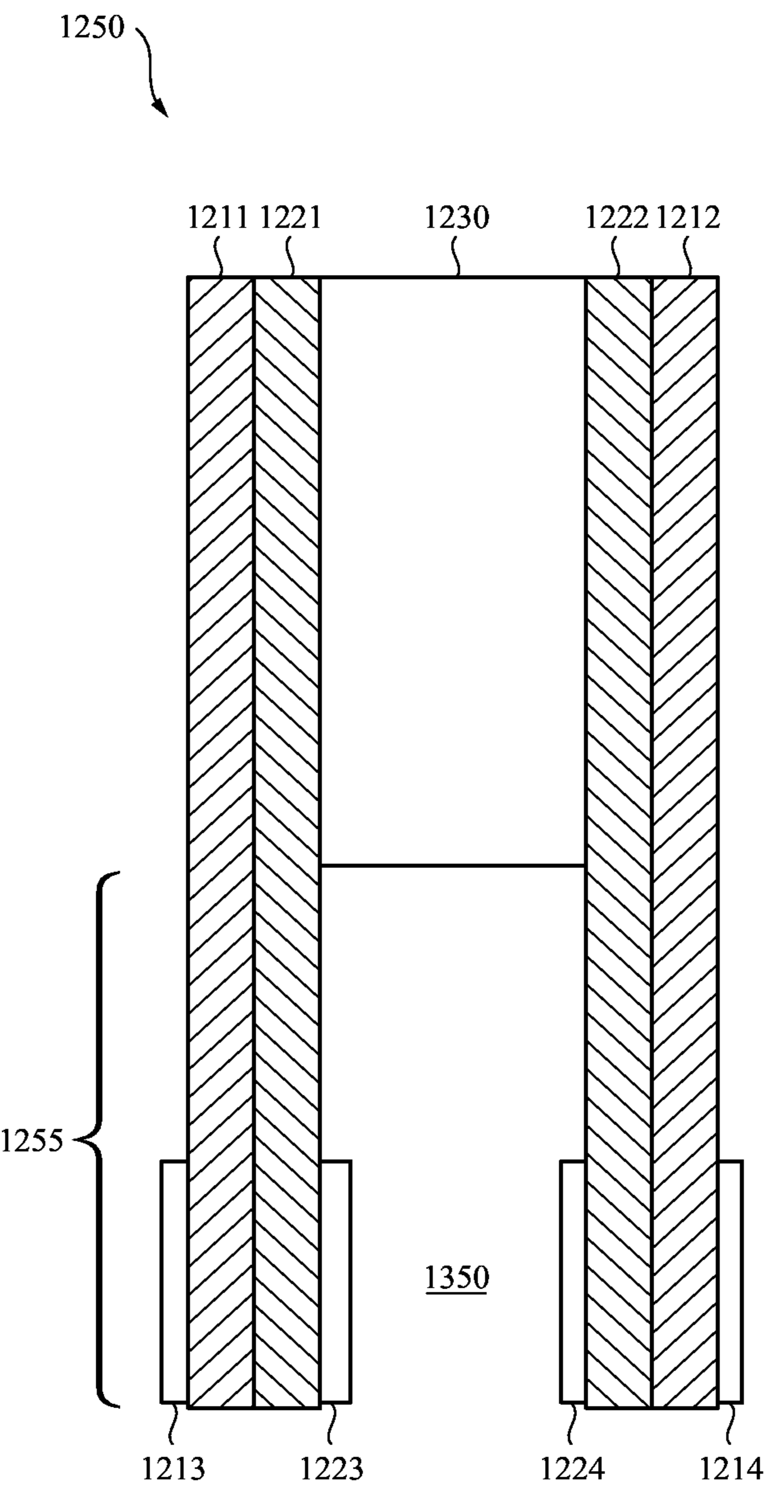
SECTION 3-3 FIG. 13
