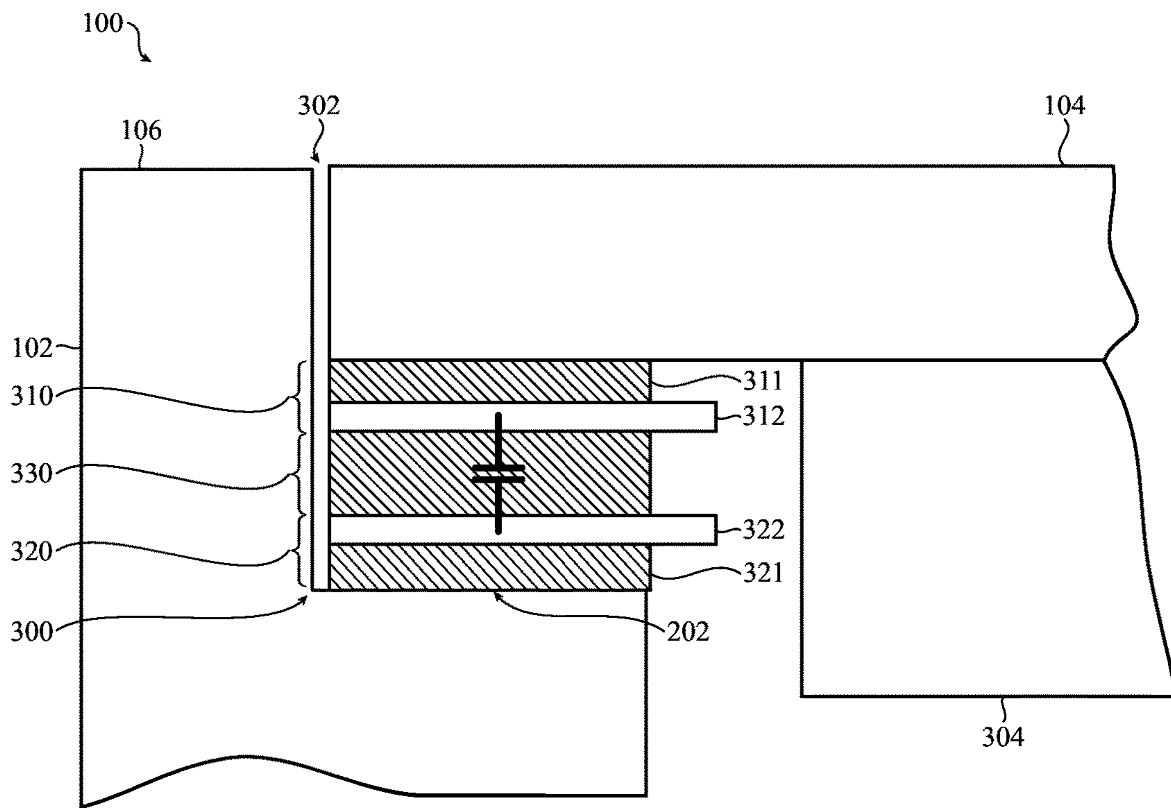
SECTION 2-2 FIG. 3
