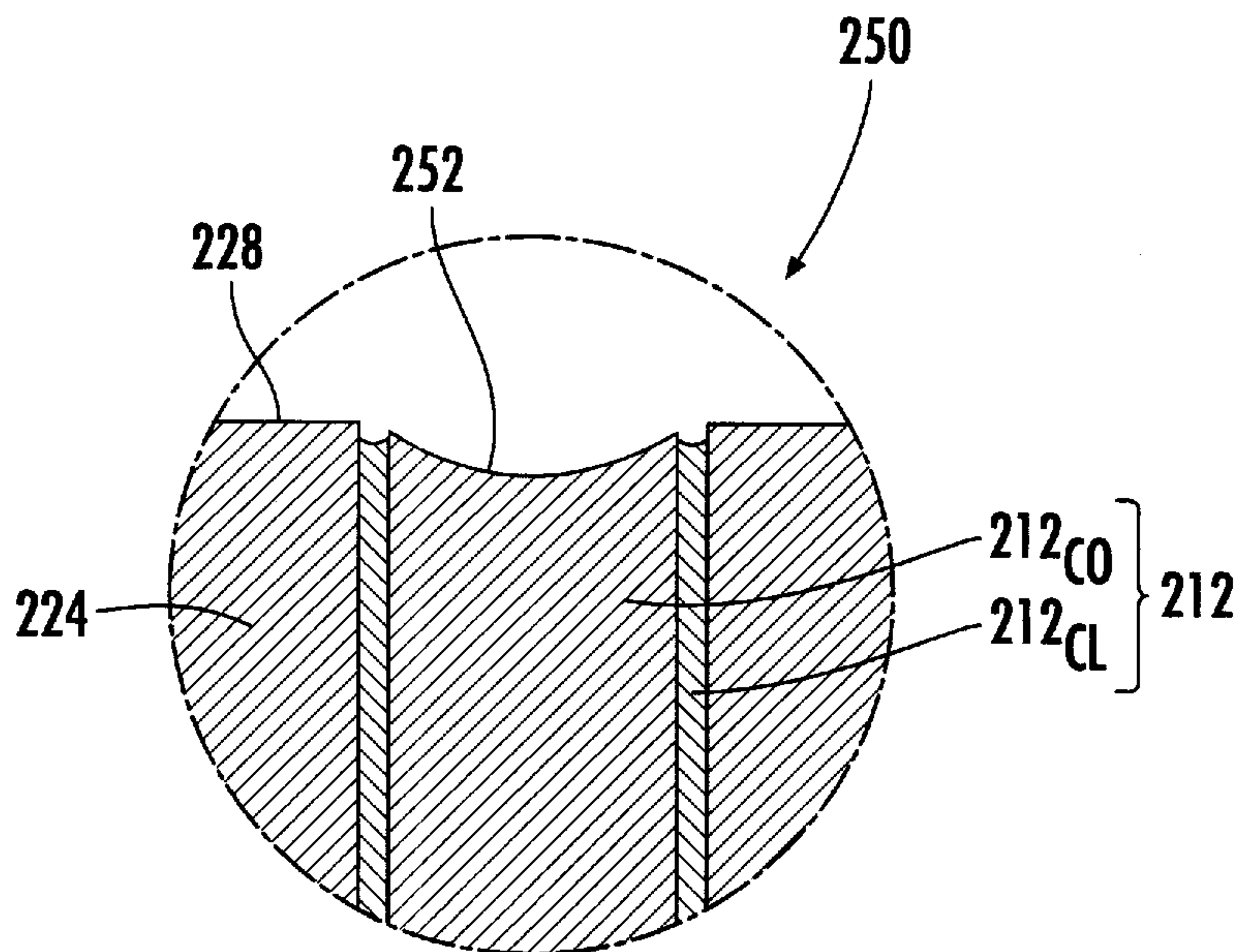
FIG. 21 (PRIOR ART)
