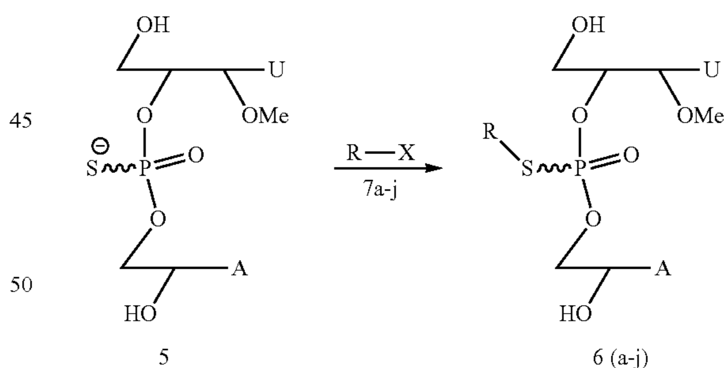
Scheme 4
