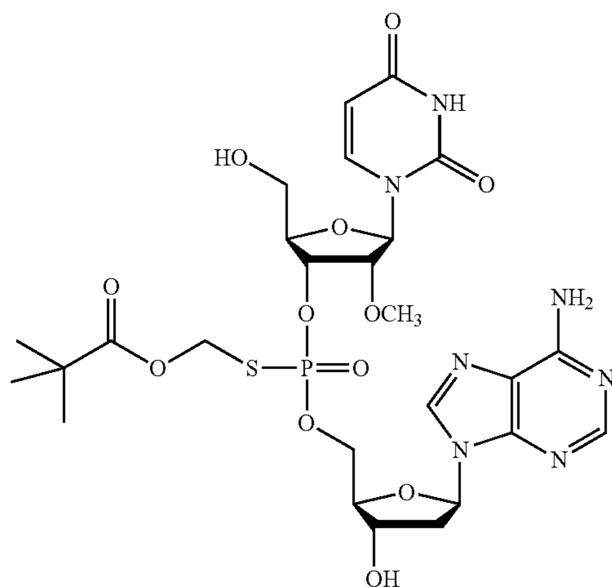
Compound 1
