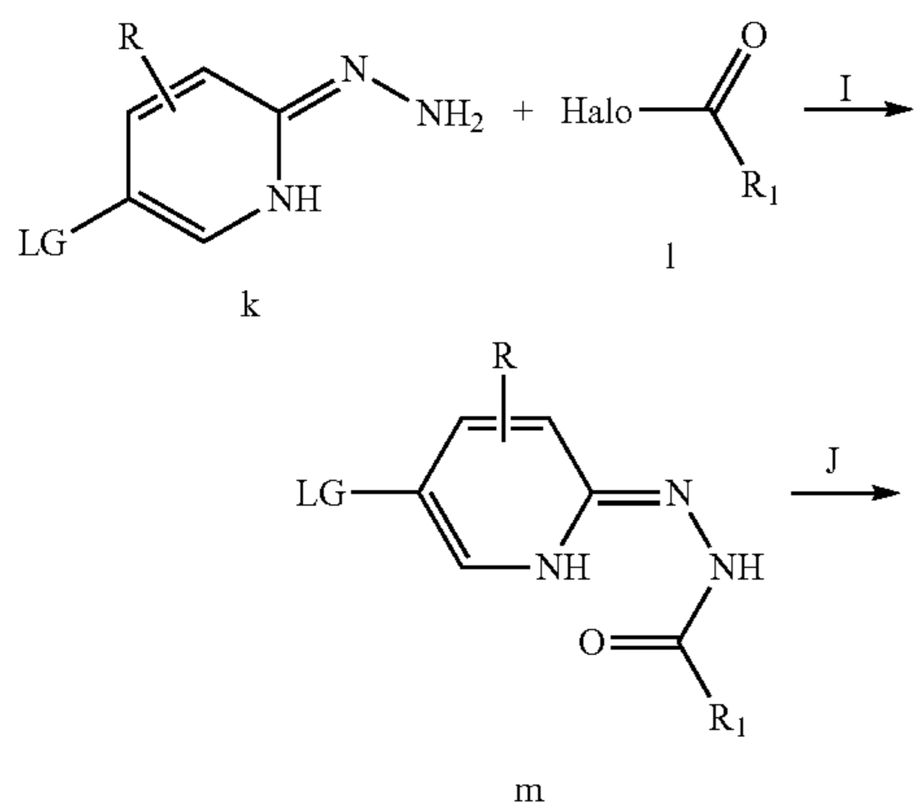
General Reaction Scheme III
