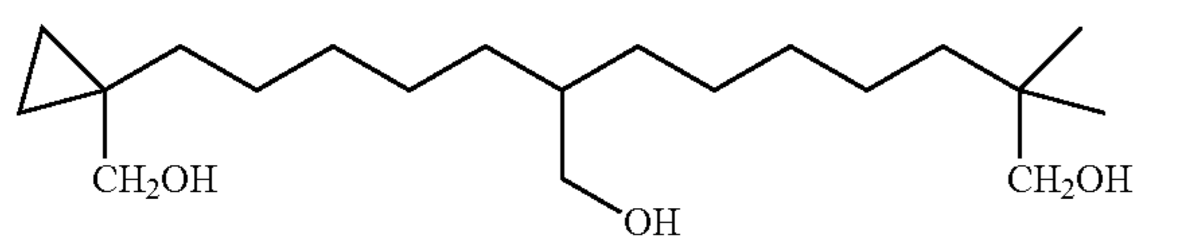
8-[5-(1-Hydroxymethyl-cyclopropyl)-pentyl]-2,2-dimethyl-nonane-1,9-diol
