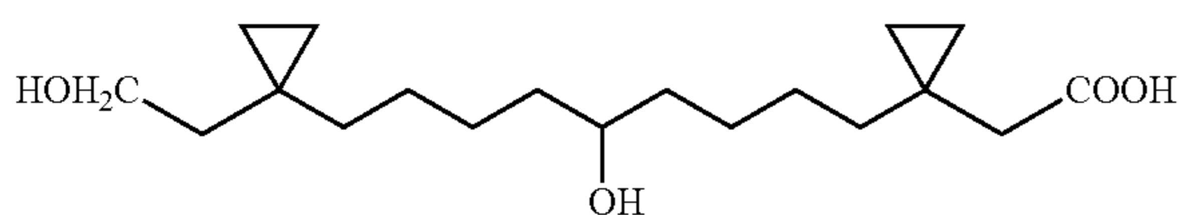
(1-{5-Hydroxy-9-[1-(2-hydroxy-ethyl)-cyclopropyl]-nonyl}-cyclopropyl)-acetic acid
