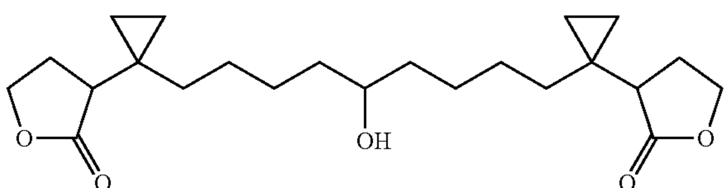
1,9-Bis-[1-(2-oxo-tetrahydrofuran-3-yl)-cyclopropyl]-nonan-5-ol
