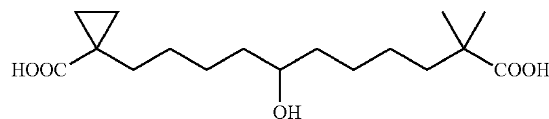
1-(10-Carboxy-5-hydroxy-10-methyl-undecyl)-cyclopropanecarboxylic acid
