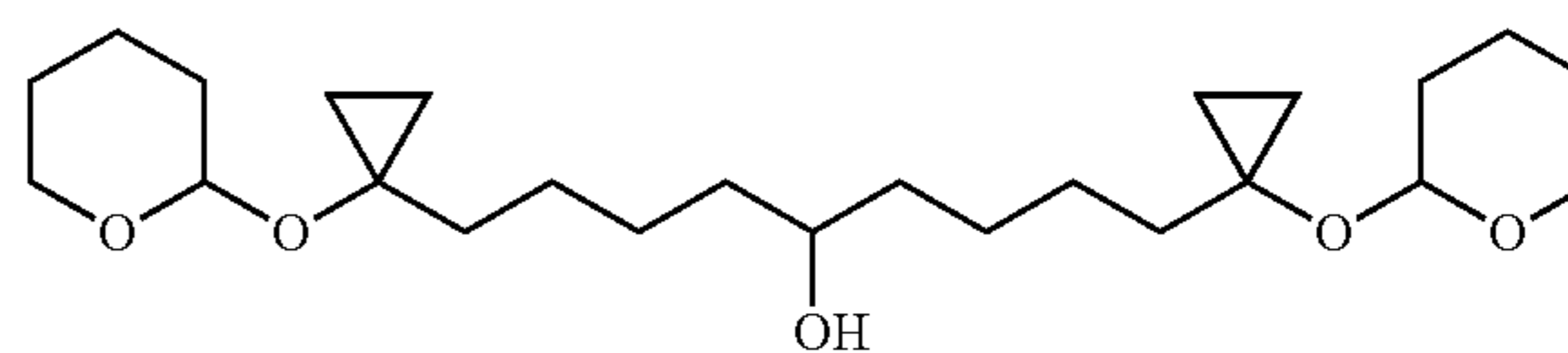
1,9-Bis-[1-(tetrahydro-pyran-2-yloxy)-cyclopropyl]-nonan-5-ol
