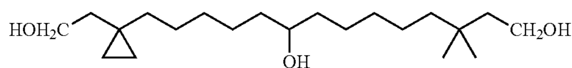
14-[1-(2-Hydroxy-ethyl)-cyclopropyl]-3,3-dimethyl-tetradecane-1,9-diol
