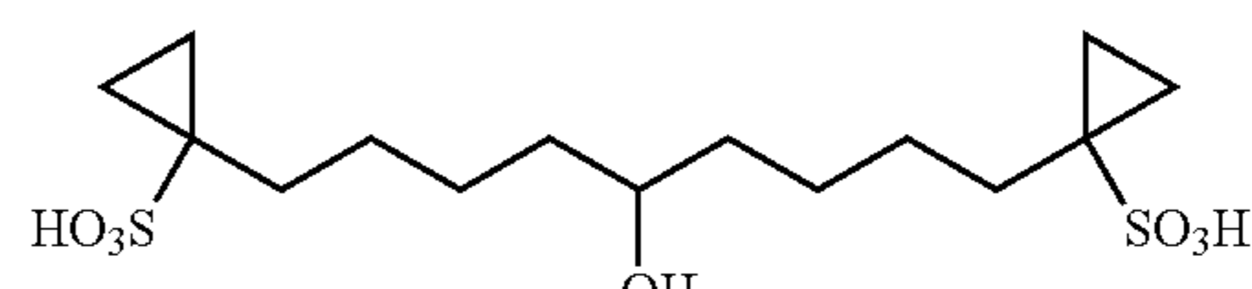
1,9-Bis-(1-sulfonyloxy-cyclopropyl)-nonan-5-ol
