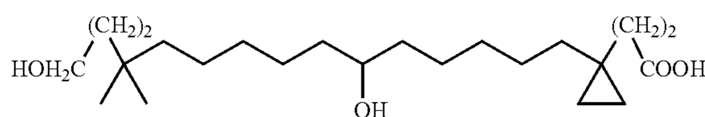
3-[1-(6,15-Dihydroxy-12,12-dimethyl-pentadecyl)-cyclopropyl]-propionic acid
