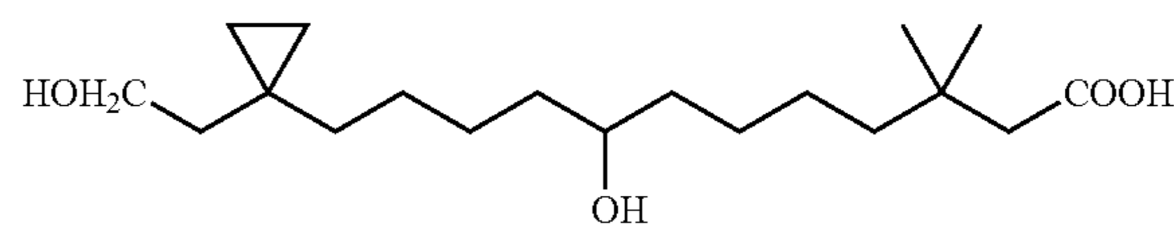
8-Hydroxy-12-[1-(2-hydroxy-ethyl)-cyclopropyl]-3,3-dimethyl-dodecanoic acid
