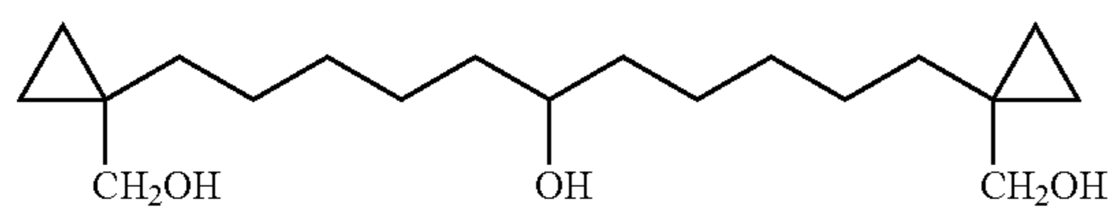
1,11-Bis-(1-hydroxymethyl-cyclopropyl)-undecan-6-ol
