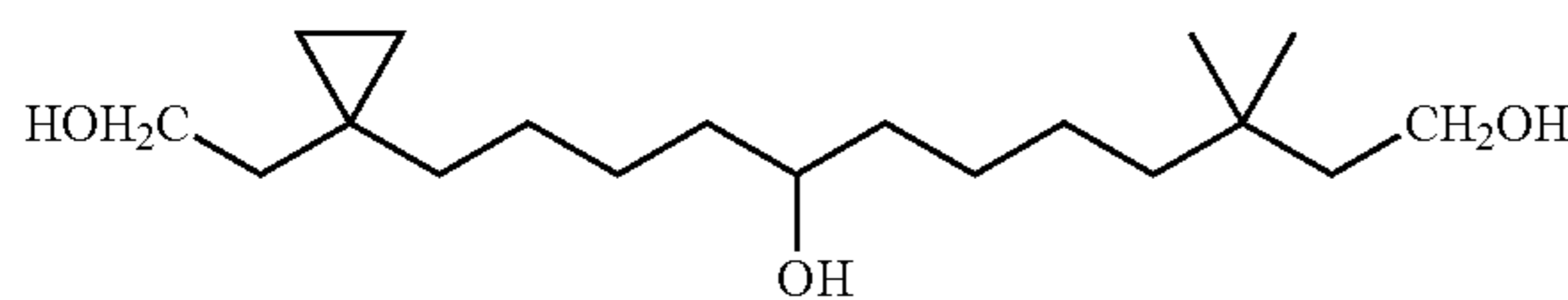
12-[1-(2-Hydroxy-ethyl)-cyclopropyl]-3,3-dimethyl-dodecane-1,8-diol
