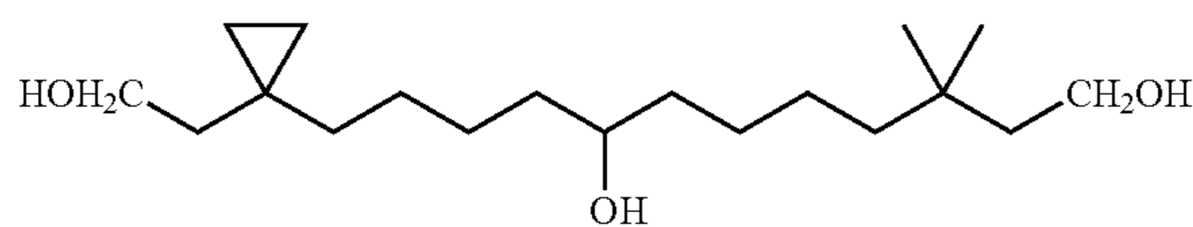
12-[1-(2-Hydroxy-ethyl)-cyclopropyl]-3,3-dimethyl-dodecane-1,8-diol
