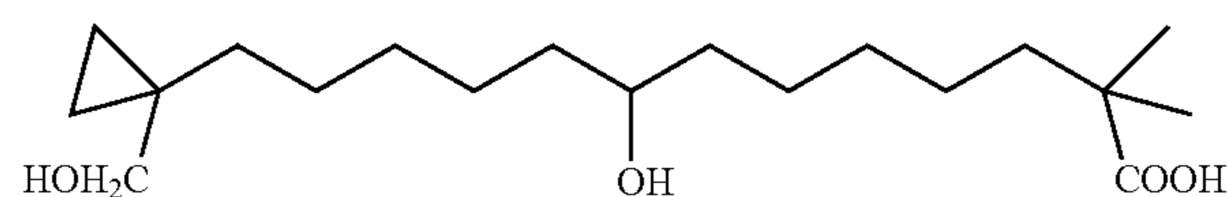
8-Hydroxy-13-(1-hydroxymethyl-cyclopropyl)-2,2-dimethyl-tridecanoic acid
