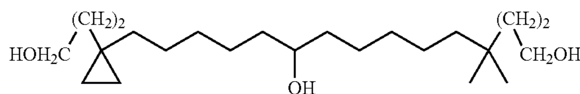
15-[1-(3-Hydroxy-propyl)-cyclopropyl]-4,4-dimethyl-pentadecane-1,10-diol
