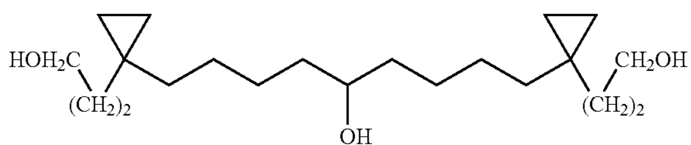
1,9-Bis-[1-(3-hydroxy-propyl)-cyclopropyl]-nonan-5-ol
