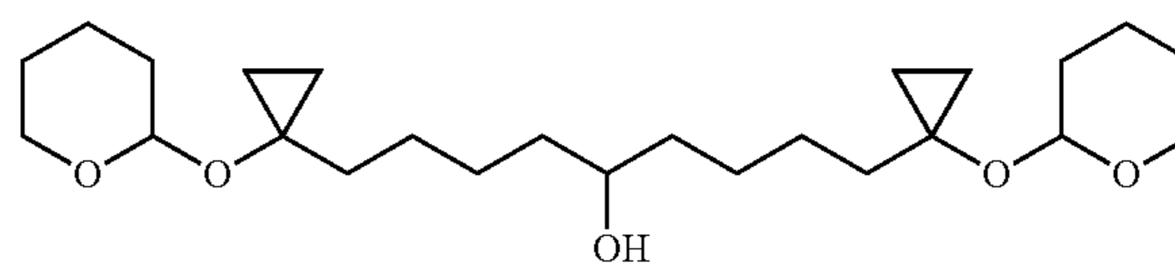
1,9-Bis-[1-(tetrahydro-pyran-2-yloxy)-cyclopropyl]-nonan-5-ol
