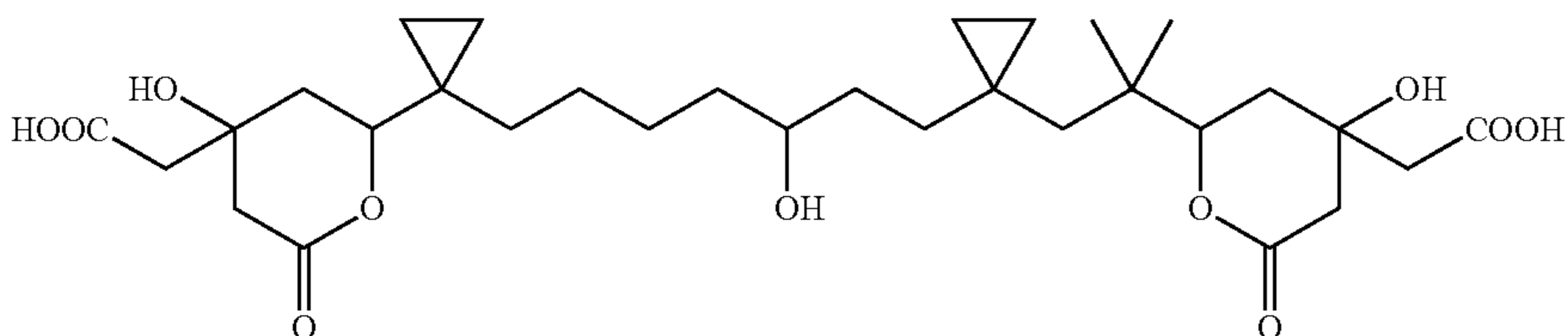
1,9-Bis {1-[9-(4-carboxymethyl-4-hydroxy-6-oxo-tetrahydro-pyran-2-yl)-(cyclopropyl)]}-5-hydroxy-nonane
