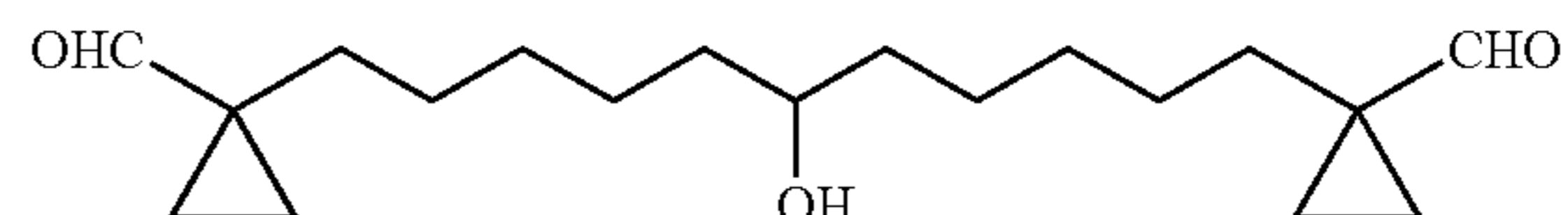
1,11-Bis-(1-oxa-cyclopropyl)-undecan-6-ol
