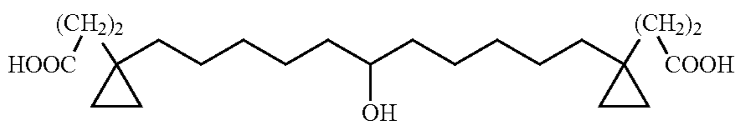
Compound 39
