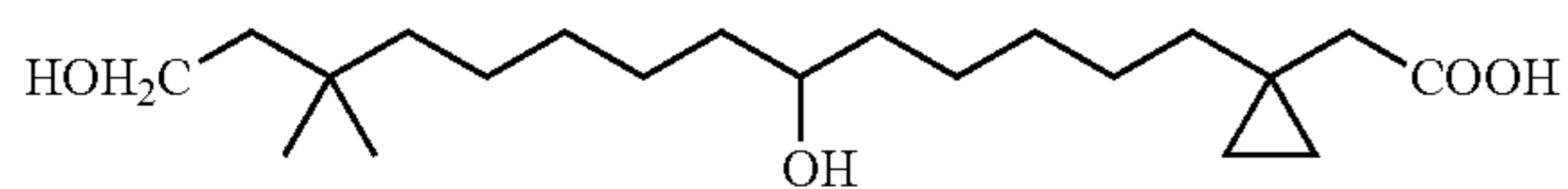
[1-(6,14-Dihydroxy-12,12-dimethyl-tetradecyl)-cyclopropyl]-acetic acid
