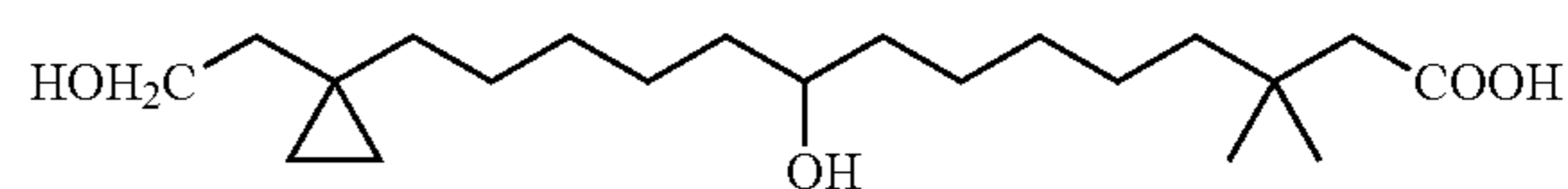
9-Hydroxy-14-[1-(2-hydroxy-ethyl)-cyclopropyl]-3,3-dimethyl-tetradecanoic acid
