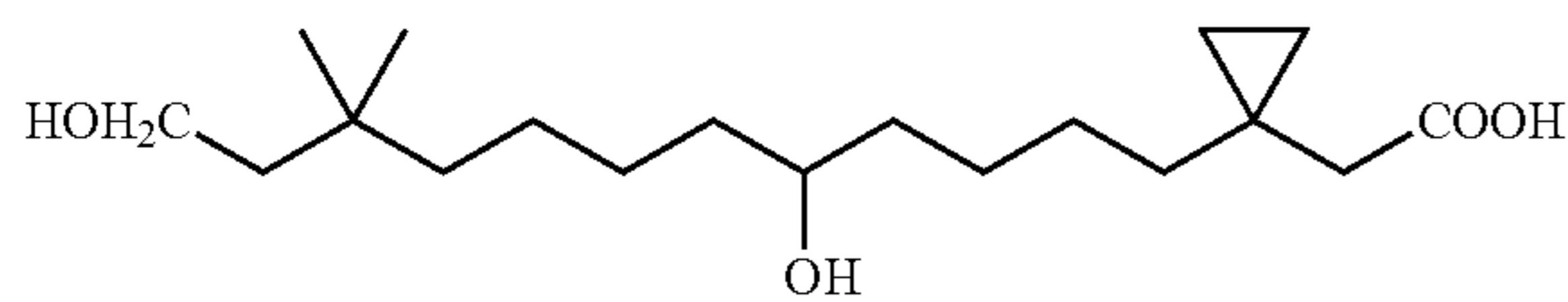
[1-(5,12-Dihydroxy-10,10-dimethyl-dodecyl)-cyclopropyl]-acetic acid
