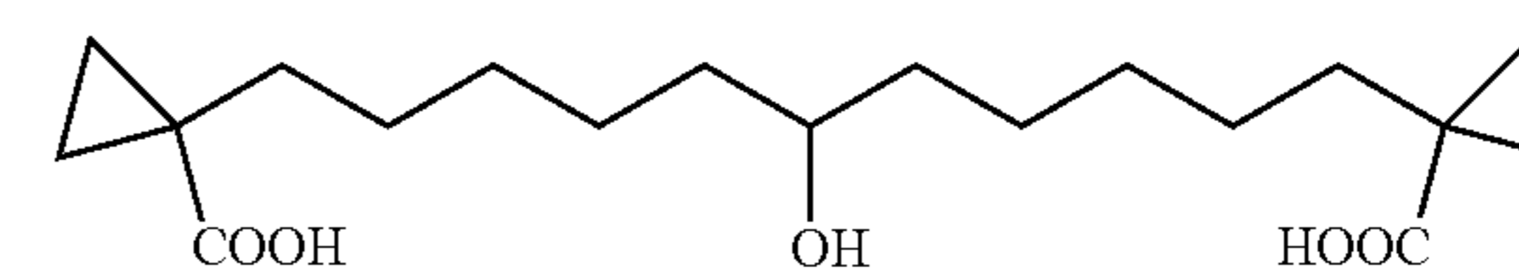
1-(12-Carboxy-6-hydroxy-12-methyl-tridecyl)-cyclopropanecarboxylic acid
