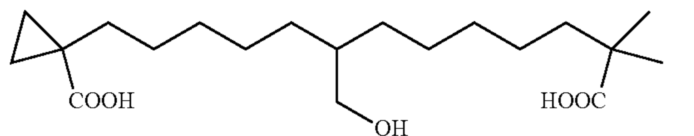
1-(12-Carboxy-6-hydroxymethyl-12-methyl-tridecyl)-cyclopropanecarboxylic acid
