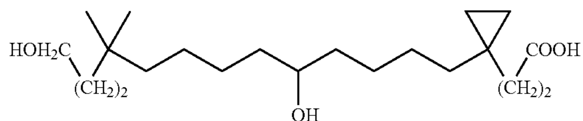
3-[1-(5,13-Dihydroxy-10,10-dimethyl-tridecyl)-cyclopropyl]-propionic acid
