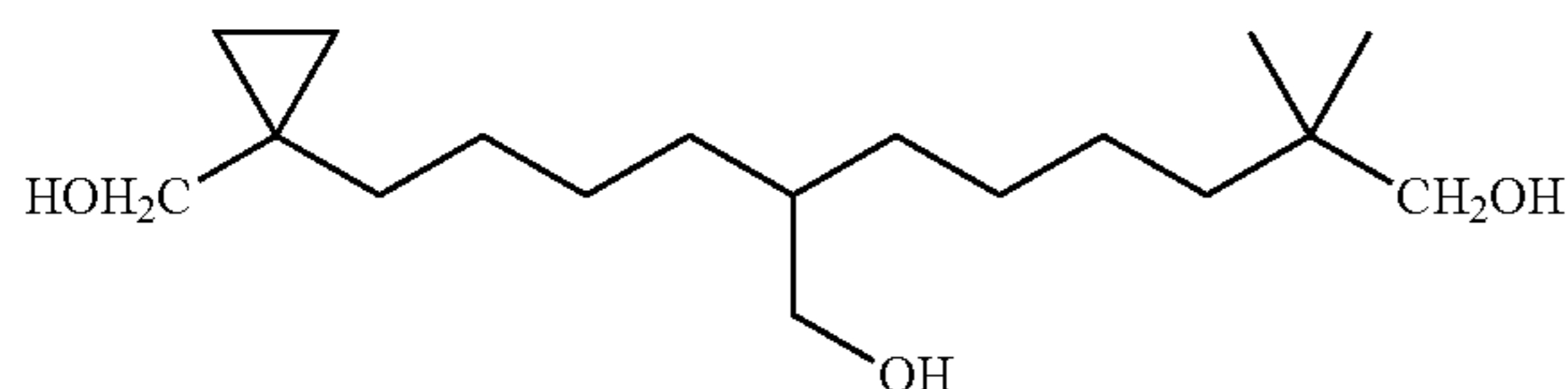
7-[4-(1-Hydroxymethyl-cyclopropyl)-butyl] 2,2-dimethyl-octane-1,8-diol
