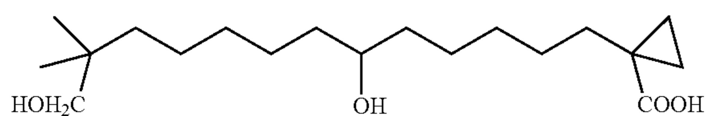
1-(6,13-Dihydroxy-12,12-dimethyl-tridecyl)-cyclopropanecarboxylic acid
