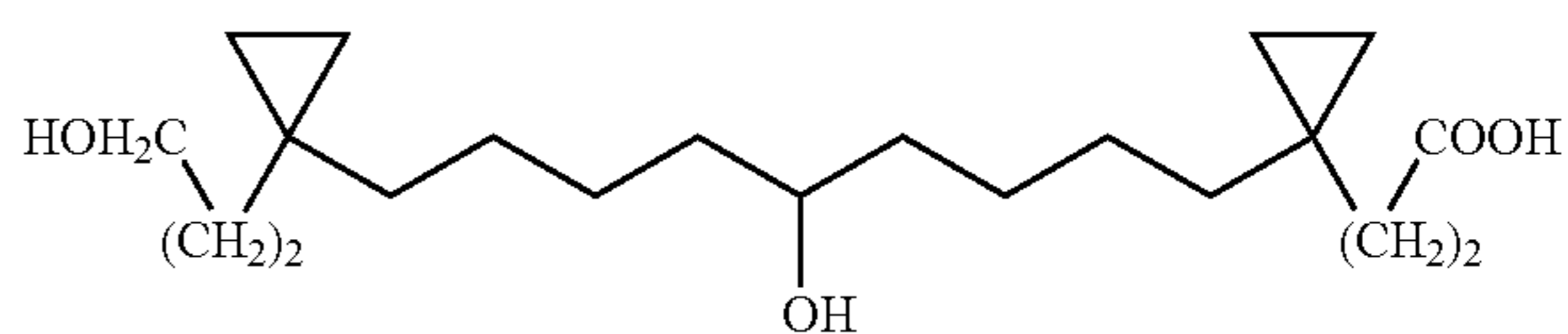
3-(1-{5-Hydroxy-9-[1-(3-hydroxy-propyl)-cyclopropyl]-nonyl}-cyclopropyl)-propionic acid
