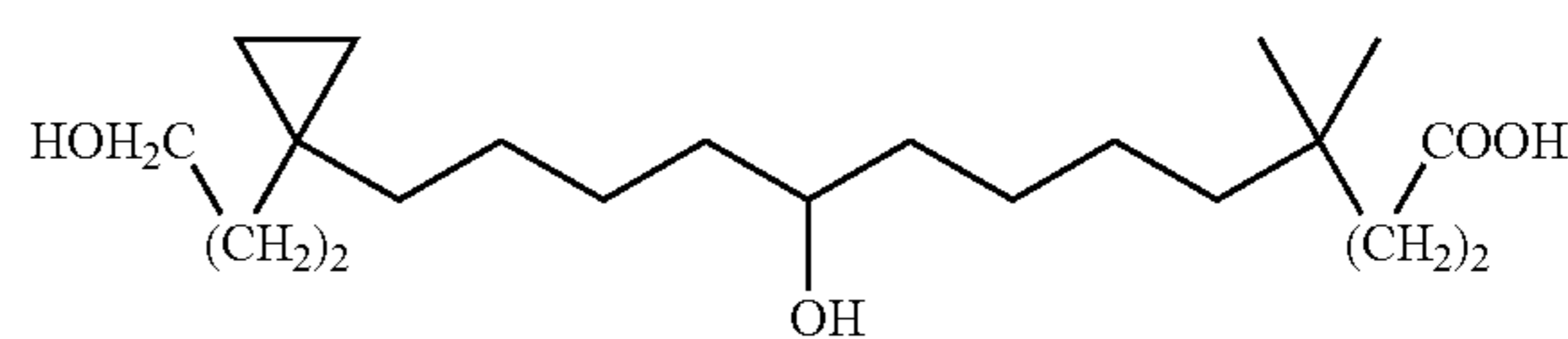
4,4-Dimethyl-9-hydroxy-13-[1-(3-hydroxypropyl)-cyclopropyl]-tridecanoic acid
