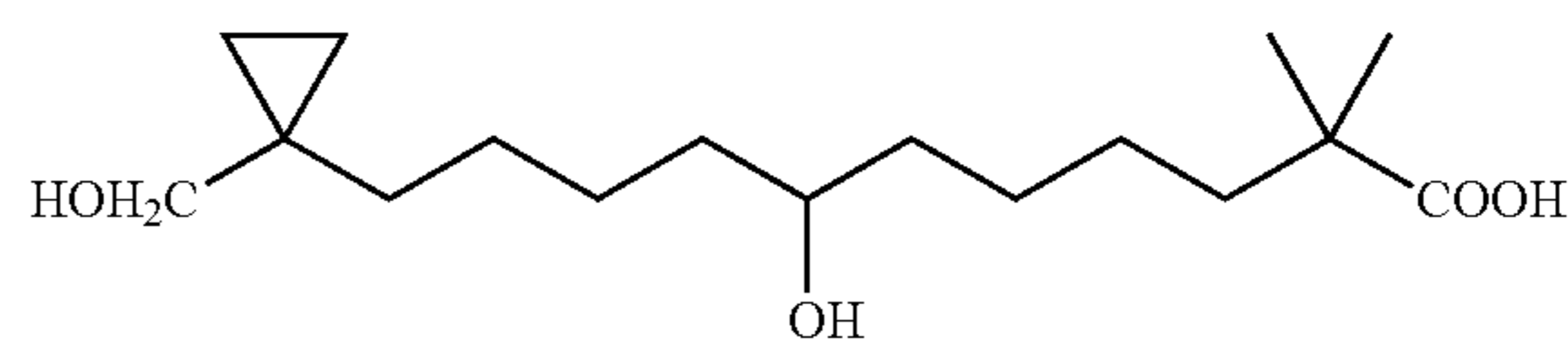
7-Hydroxy-11-(1-hydroxymethyl-cyclopropyl)-2,2-dimethyl-undecanoic acid
