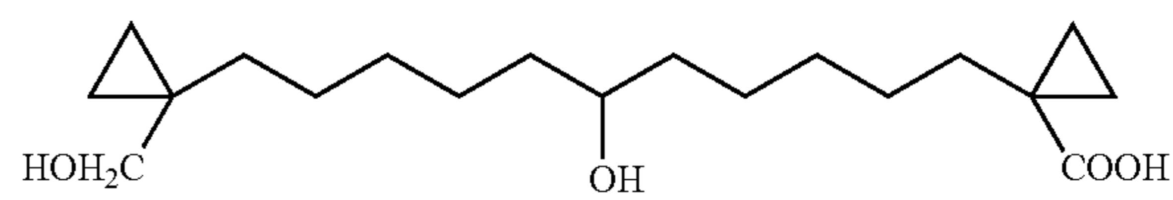
1-[6-Hydroxy-11-(1-hydroxymethyl-cyclopropyl)-undecyl]-cyclopropanecarboxylic acid
