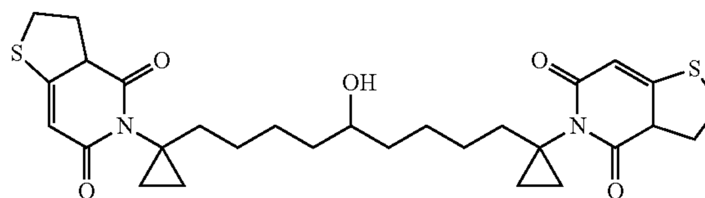
2,9-Bis-(4,6-dioxo-2,3,3a,6-tetrahydro-4H-thieno[3,2-c]pyridin-5-yl)-2,9-bis-(cyclopropyl)-5-hydroxy-nonane
