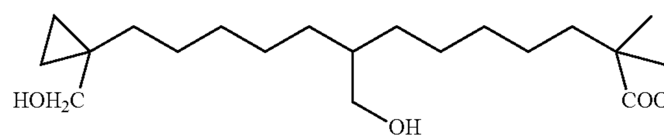
8-Hydroxymethyl-13-(1-hydroxymethyl-cyclopropyl)-2,2-dimethyl-tridecanoic acid
