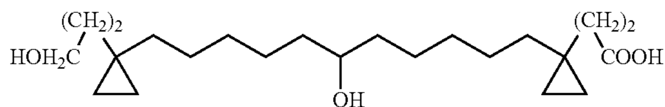
3-(1-(6-Hydroxy-11-[1-(3-hydroxy-propyl)-cyclopropyl]-undecyl)-cyclopropyl)-propionic acid
