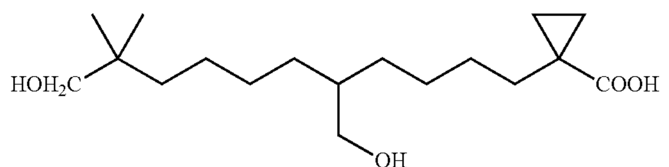
1-(11-Hydroxy-5-hydroxymethyl-10,10-dimethyl-undecyl)-cyclopropanecarboxylic acid
