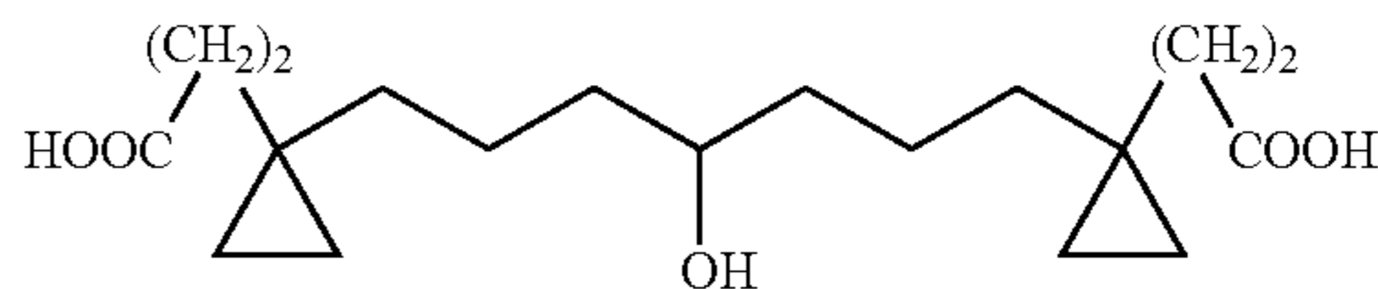
3-(1-(7-[1-(2-Carboxy-ethyl)-cyclopropyl]-4-hydroxy-heptyl)-cyclopropyl)-propionic acid
