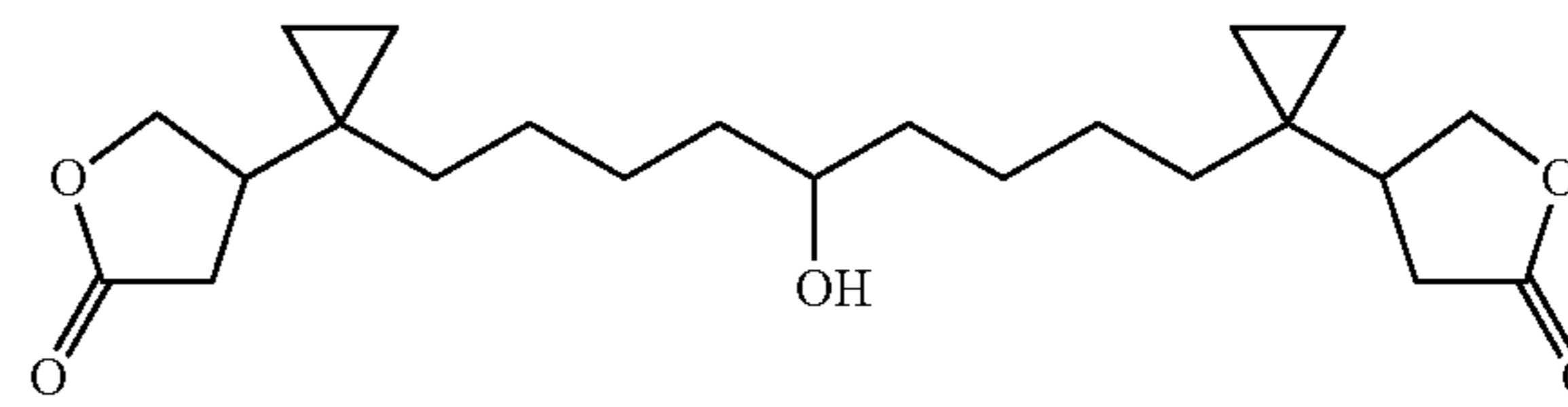
1,9-Bis-[1-(2-oxo-tetrahydrofuran-4-yl)-cyclopropyl]-nonan-5-ol
