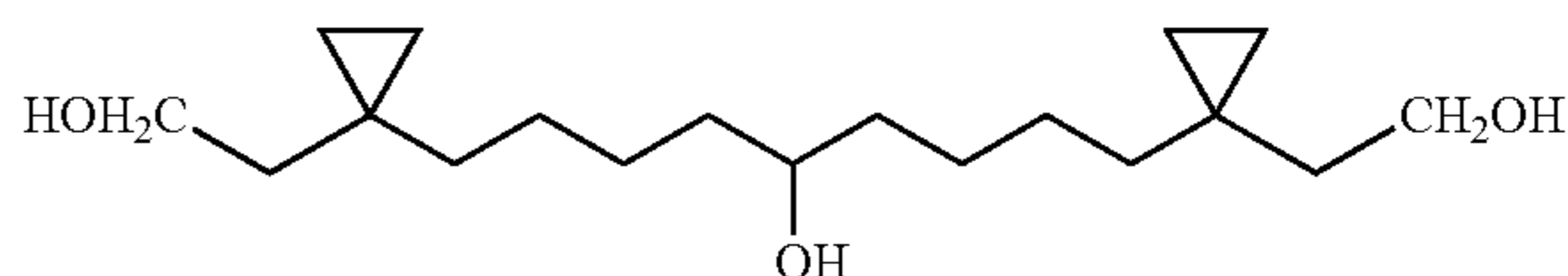
1,9-Bis-[1-(2-hydroxy-ethyl)-cyclopropyl]-nonan-5-ol
