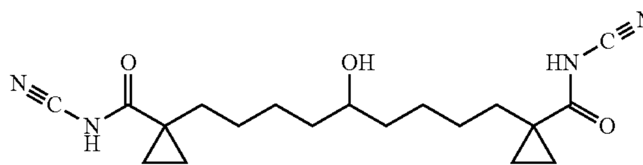
1,7-Bis-(1-dicyanimido-cyclopropyl)-5-hydroxy-nonane
