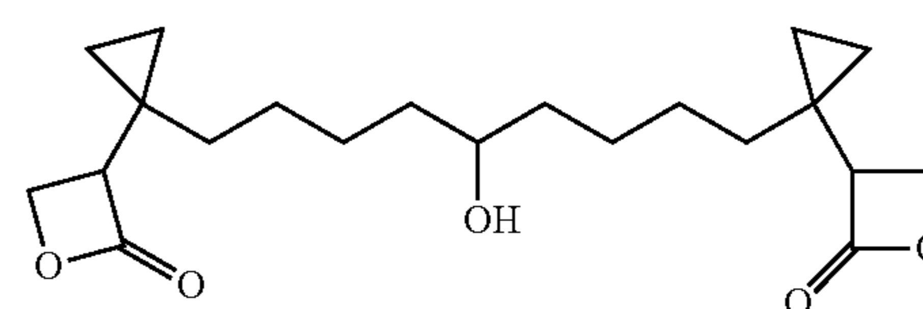
1,9-Bis-[1-(2-oxo-oxoethan-3-yl)-cyclopropyl]-nonan-5-ol
