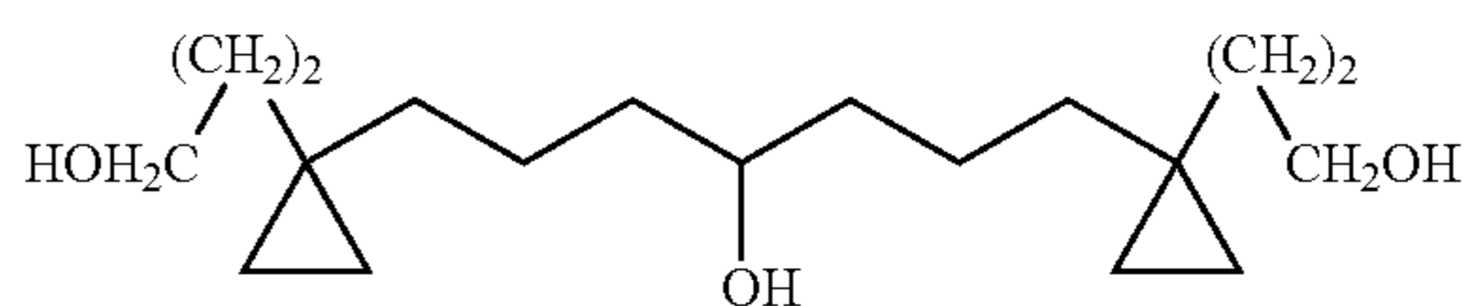
1,7-Bis-[1-(3-hydroxy-propyl)-cyclopropyl]-heptan-4-ol
