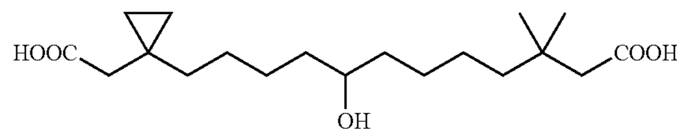
12-(1-Carboxymethyl-cyclopropyl)-8-hydroxy-3,3-dimethyl-dodecanoic acid
