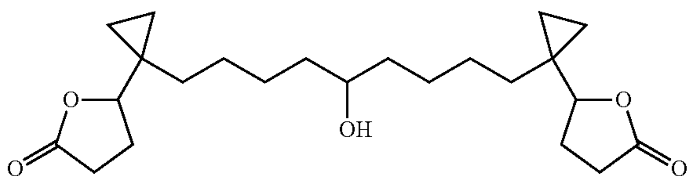
1,9-Bis-[1-(2-oxo-tetrahydrofuran-5-yl)-cyclopropyl]-nonan-5-ol
