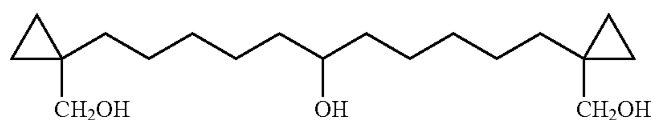
1,11-Bis-(1-hydroxymethyl-cyclopropyl)-undecan-6-ol
