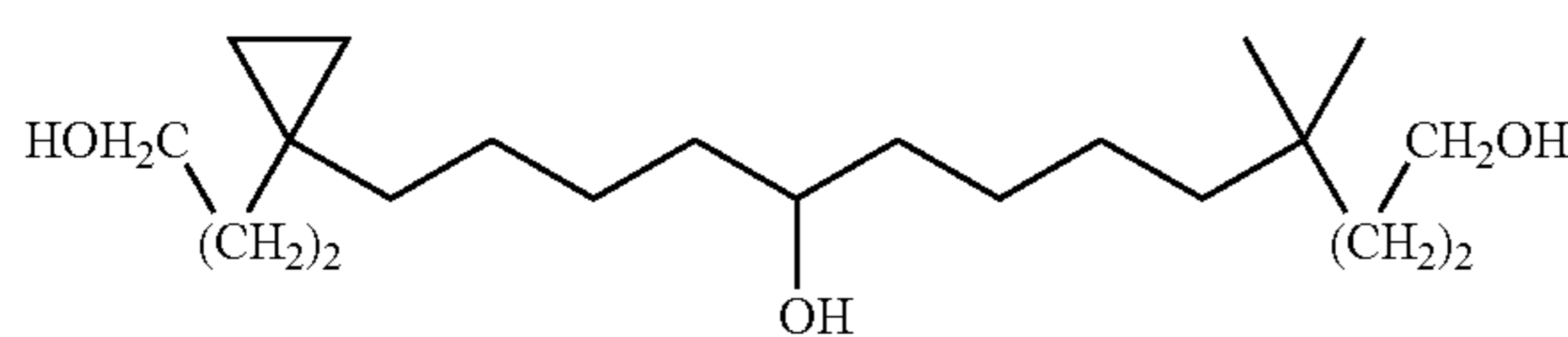
13-[1-(3-Hydroxy-propyl)-cyclopropyl]-4,4-dimethyl-tridecane-1,9-diol
