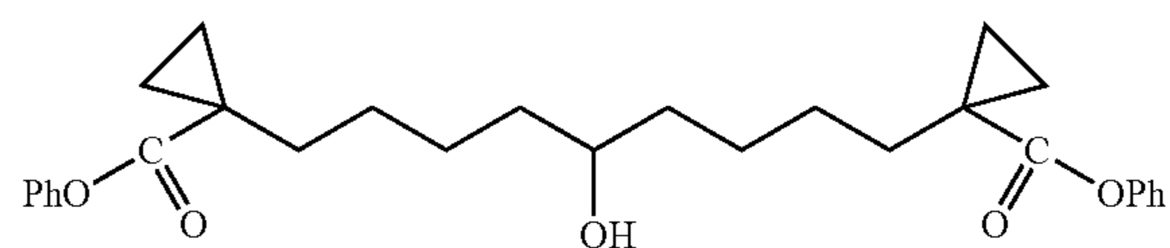
1,9-Bis-(1-phenoxy-carbonyl-cyclopropyl)-nonan-5-ol
