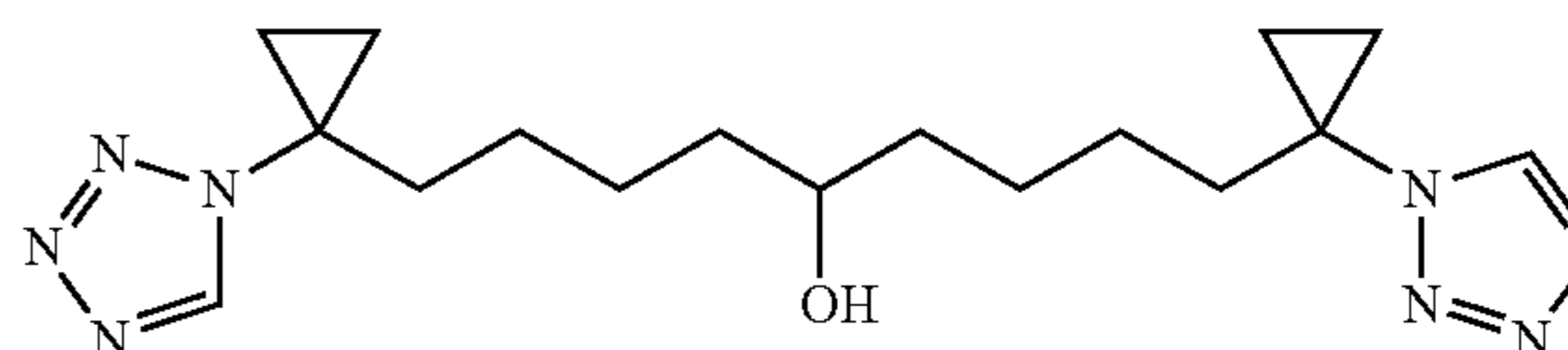
Compound 48
