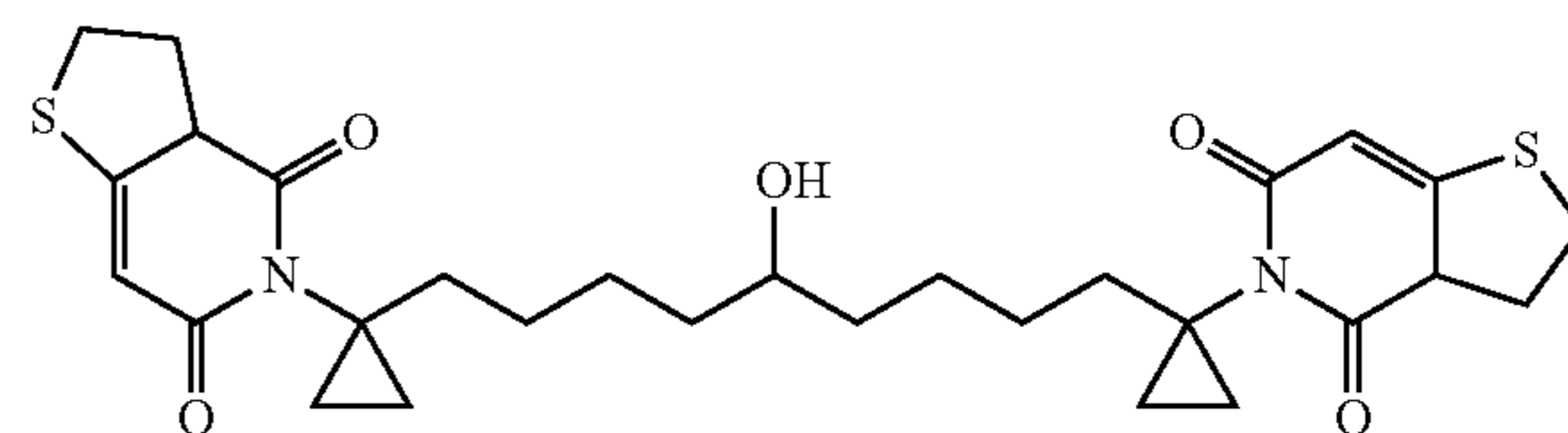
2,9-Bis-(4,6-dioxo-2,3,3a,6-tetrahydro-4H-thieno[3,2-c]pyridin-5-yl)-2,9-bis-(cyclopropyl)-5-hydroxy-nonane
