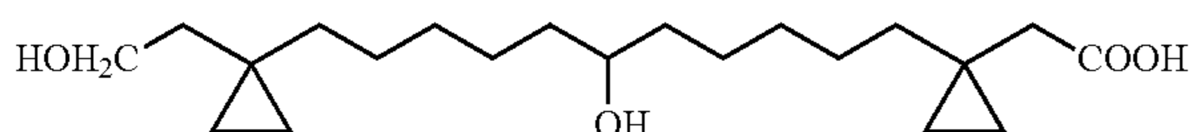
(1-{6-Hydroxy-11-[1-(2-hydroxy-ethyl)-cyclopropyl]-undecyl}-cyclopropyl)-acetic acid
