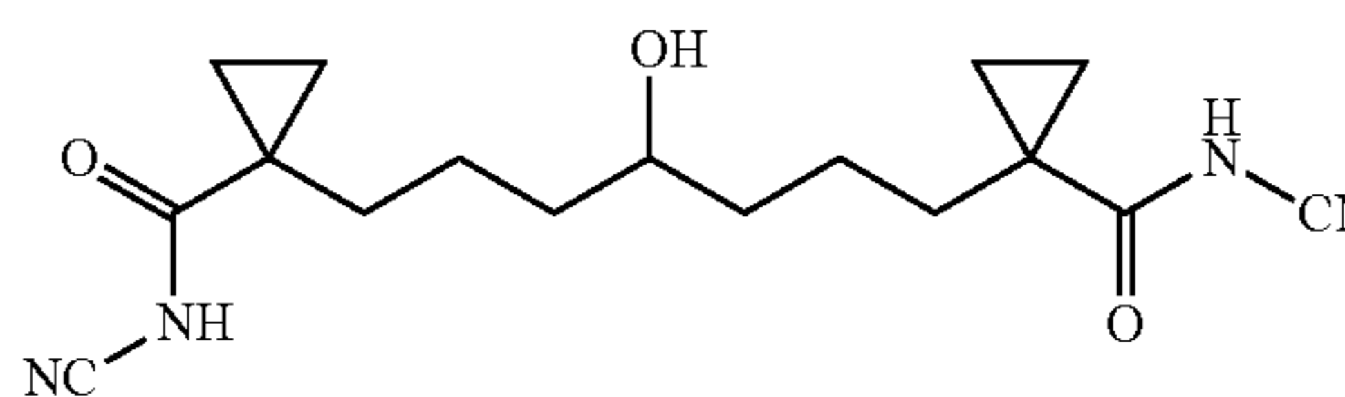
1,7-Bis-(1-dicyanimido-cyclopropyl)-4-hydroxy-heptane
