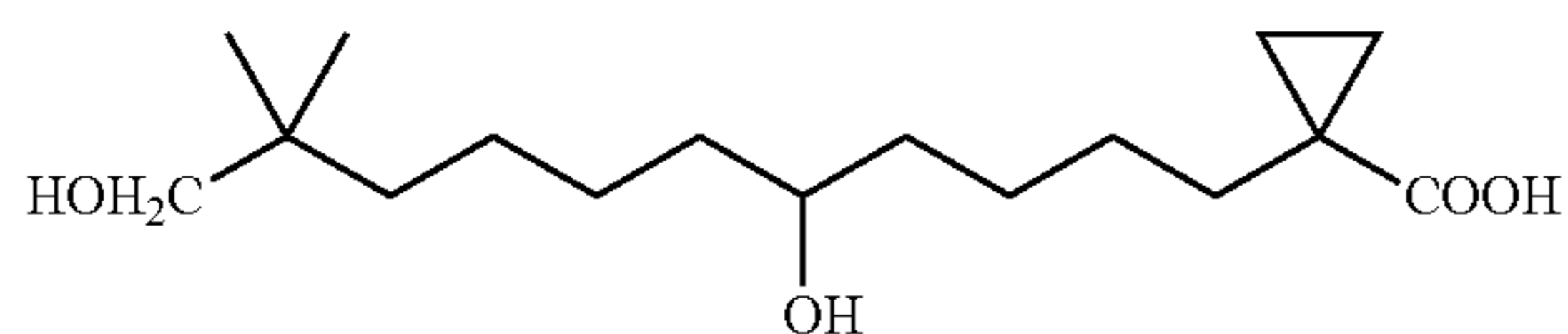
1-(5,11-Dihydroxy-10,10-dimethyl-undecyl)-cyclopropanecarboxylic acid
