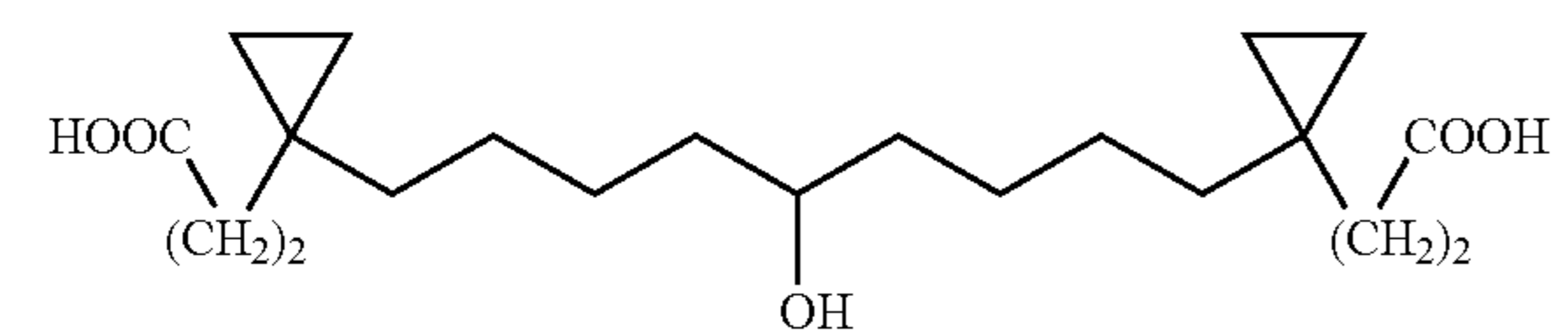
3-(1-{9-[1-(3-Carboxy-ethyl)-5-hydroxy-cyclopropyl]-nonyl}-cyclopropyl)-propionic acid
