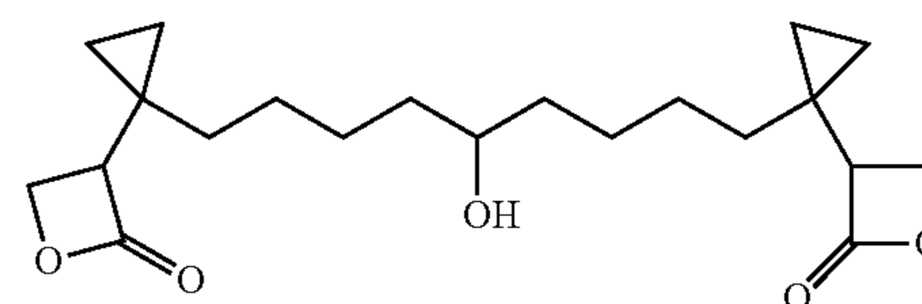
1,9-Bis-[1-(2-oxo-oxoethan-3-yl)-cyclopropyl]-nonan-5-ol
