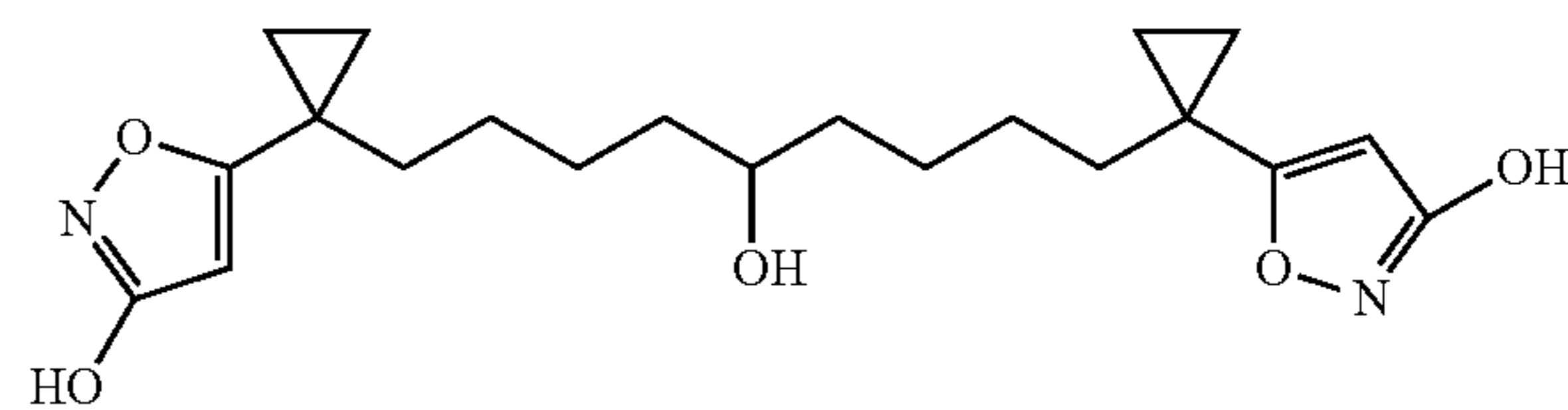
1,9-Bis-[1-(3-hydroxy-isoxazol-5-yl)-cyclopropyl]-nonan-5-ol
