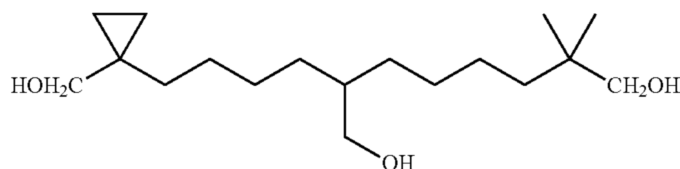
7-[4-(1-Hydroxymethyl-cyclopropyl)-butyl] 2,2-dimethyl-octane-1,8-diol
