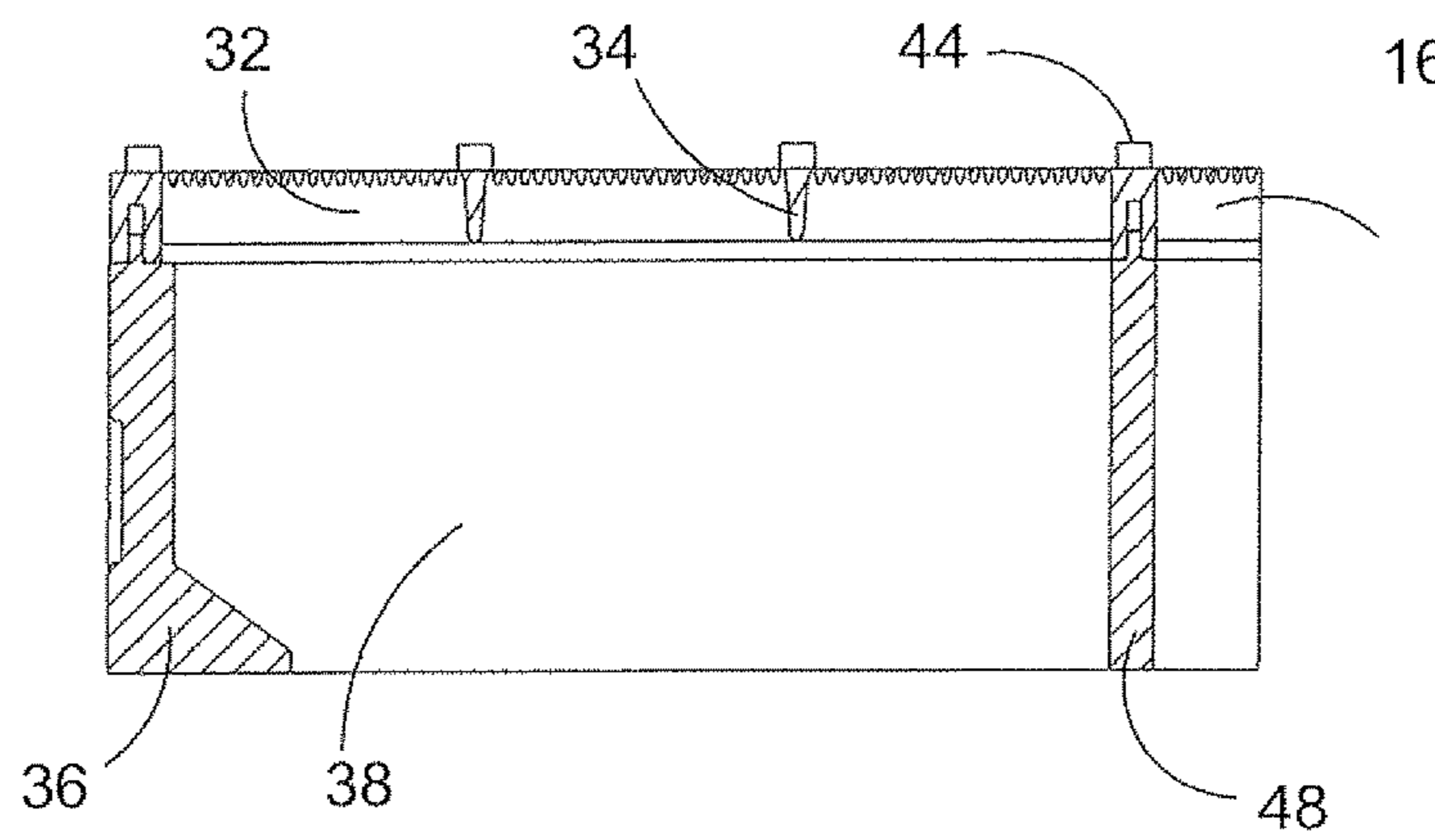
SECTION B-B
