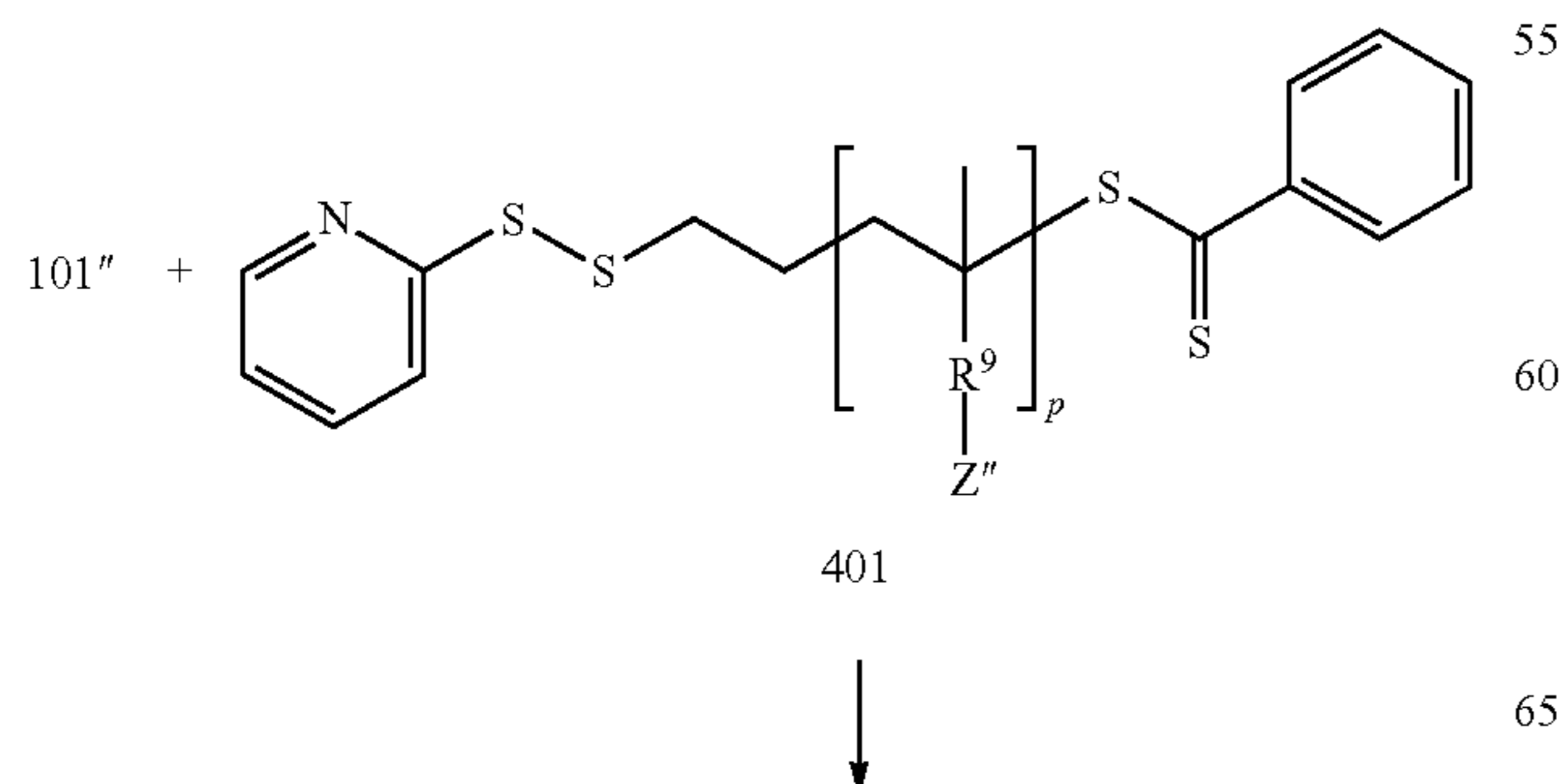
Reaction Scheme 4
