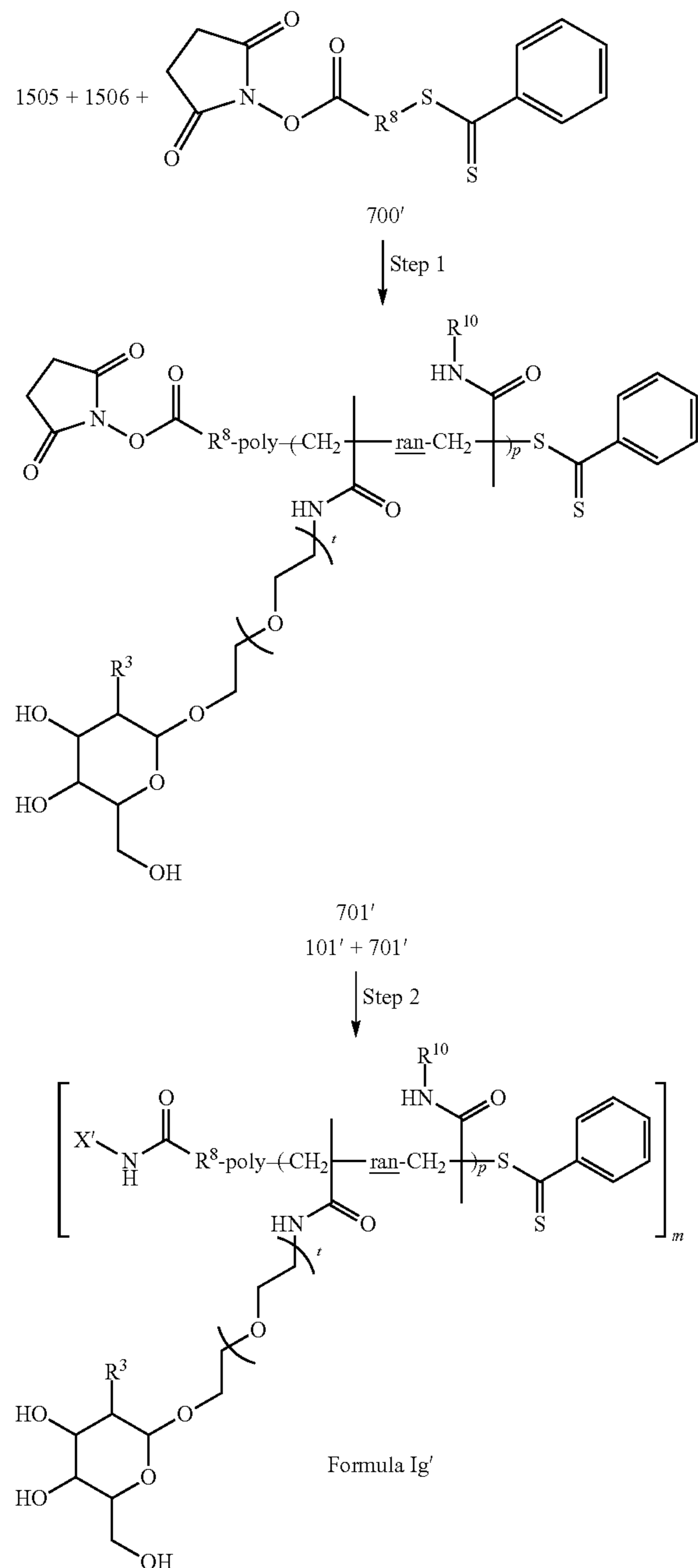
Reaction Scheme 18
