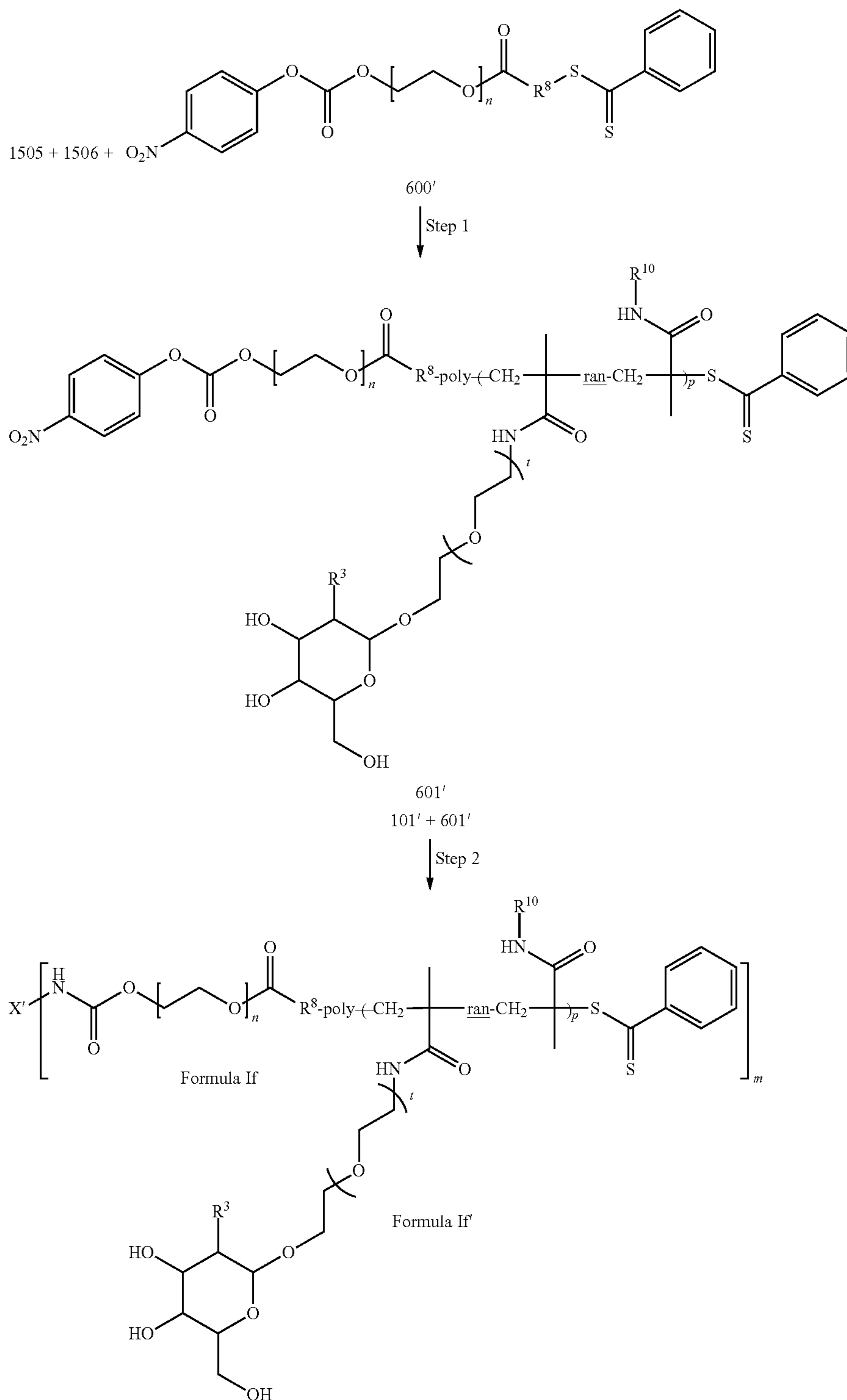
Reaction Scheme 17
