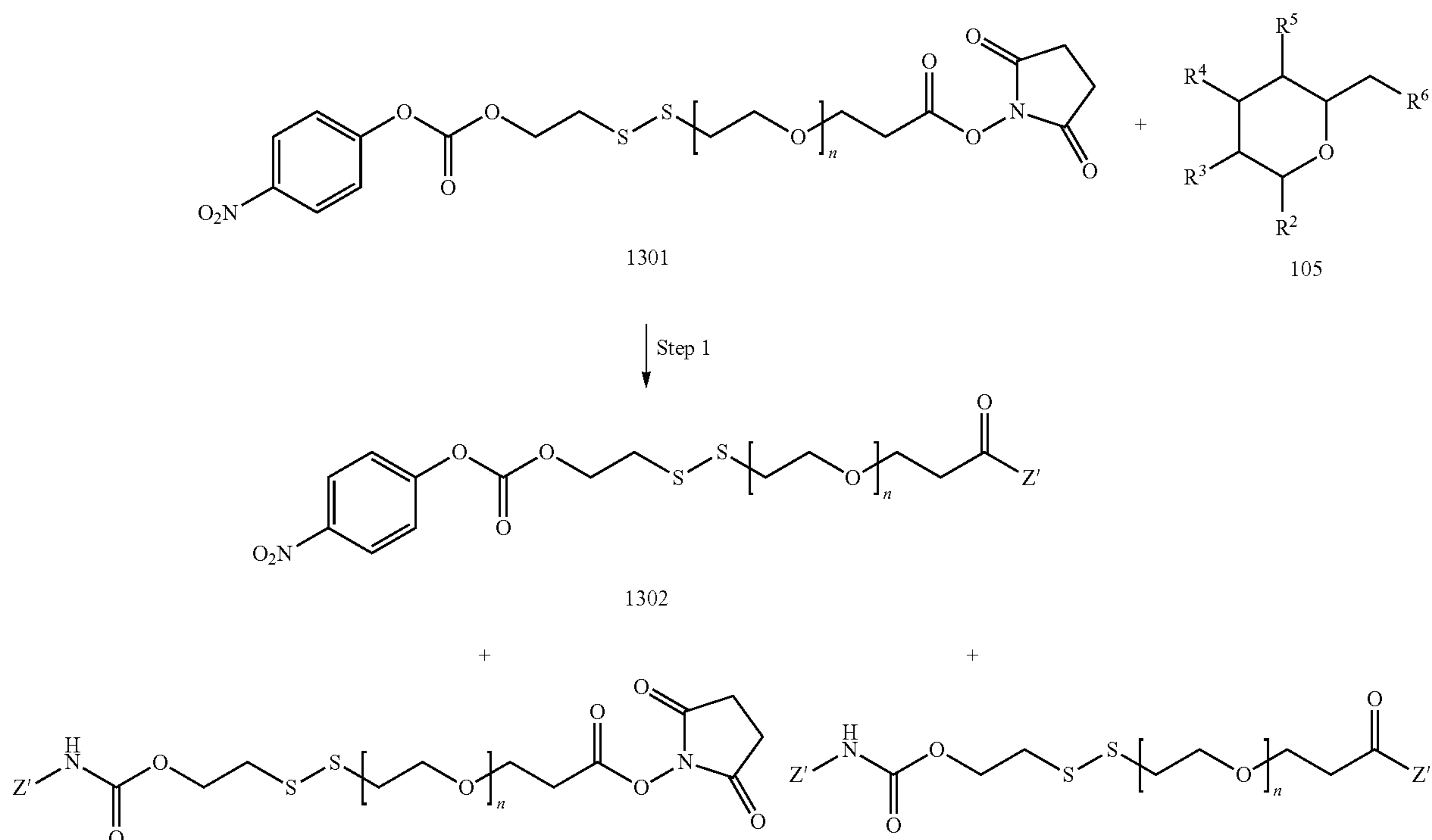
Reaction Scheme 13
