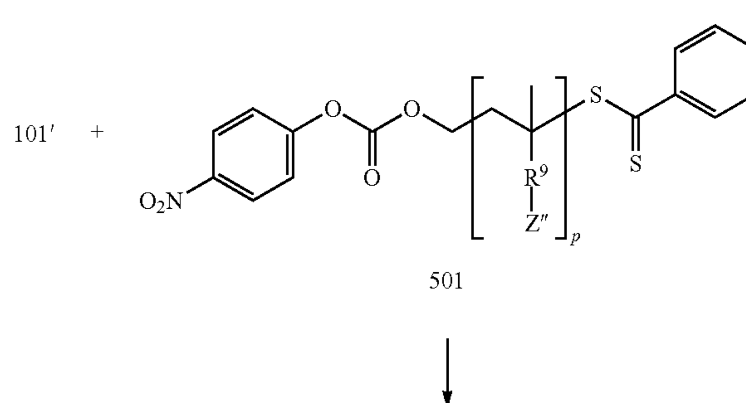
Reaction Scheme 5
