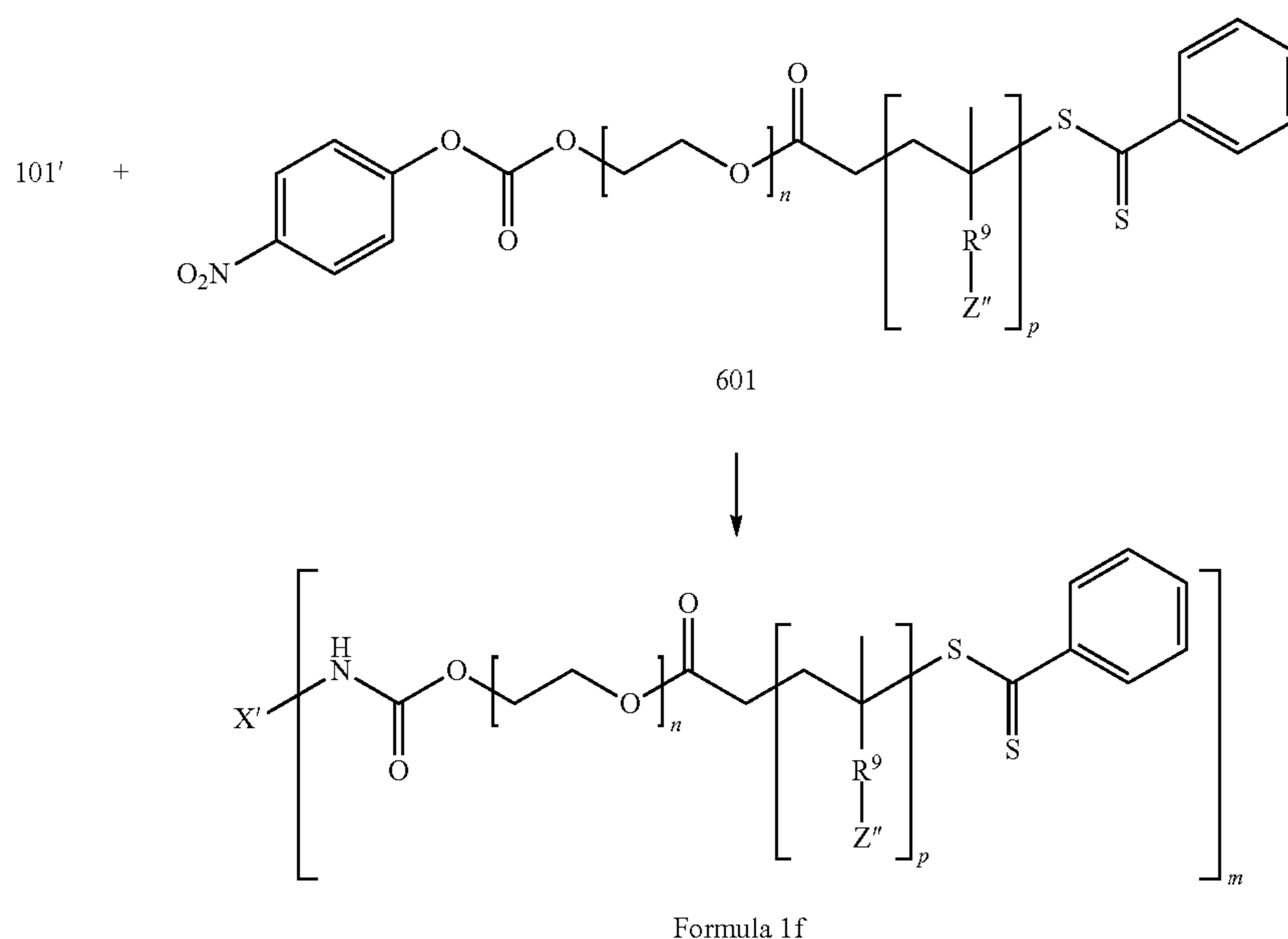
Reaction Scheme 6
