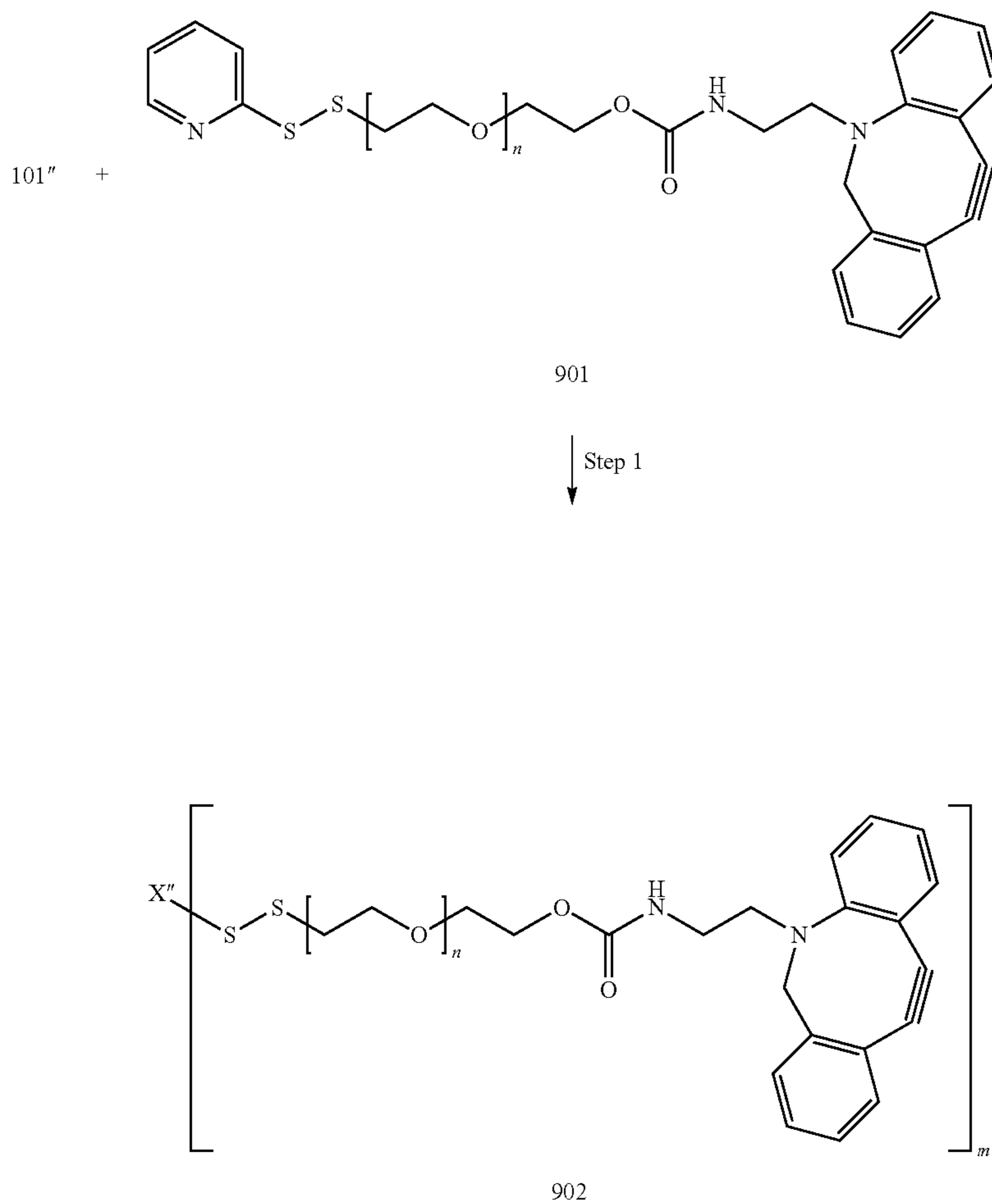
Reaction Scheme 9
