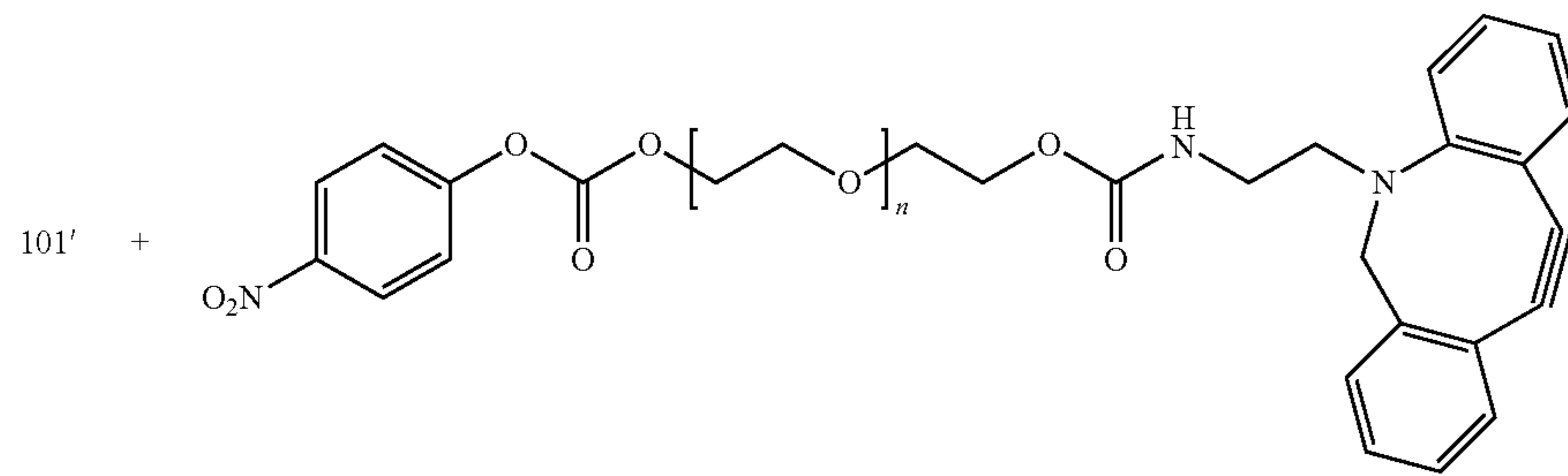
Reaction Scheme 8
