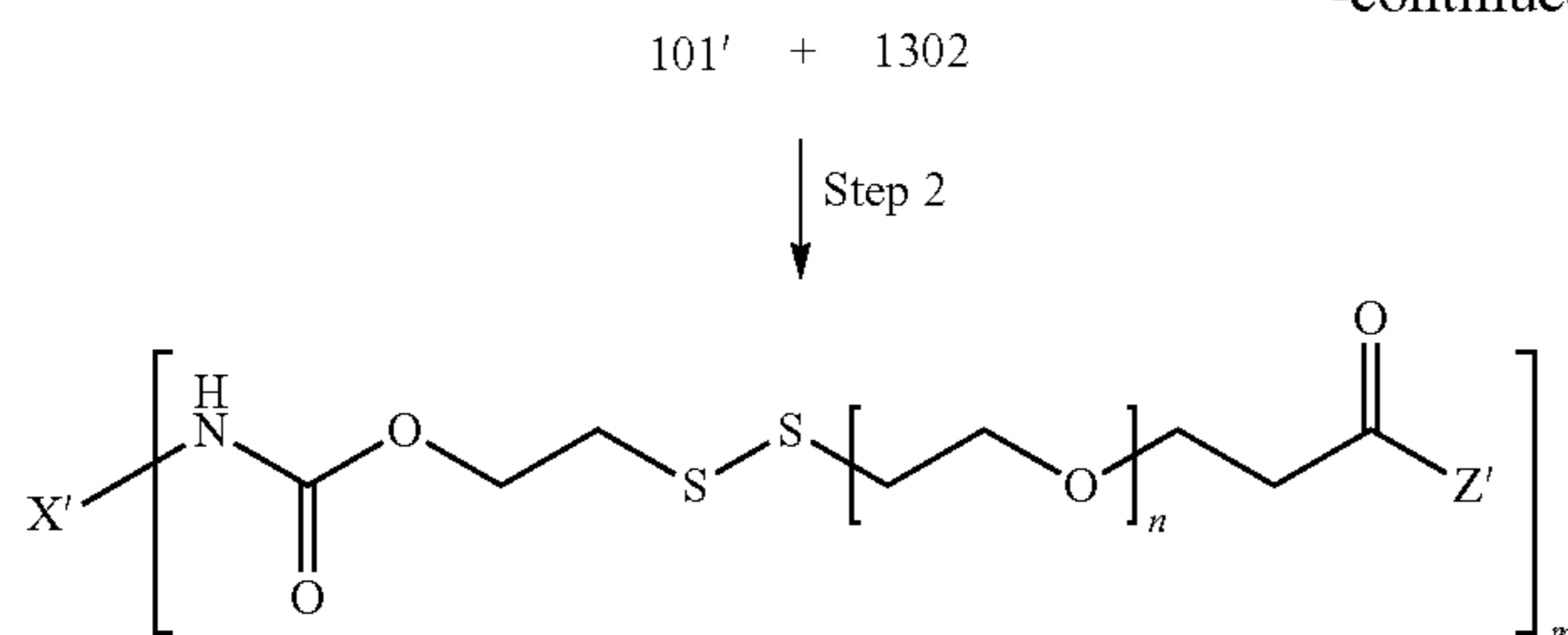
Formula 1o
