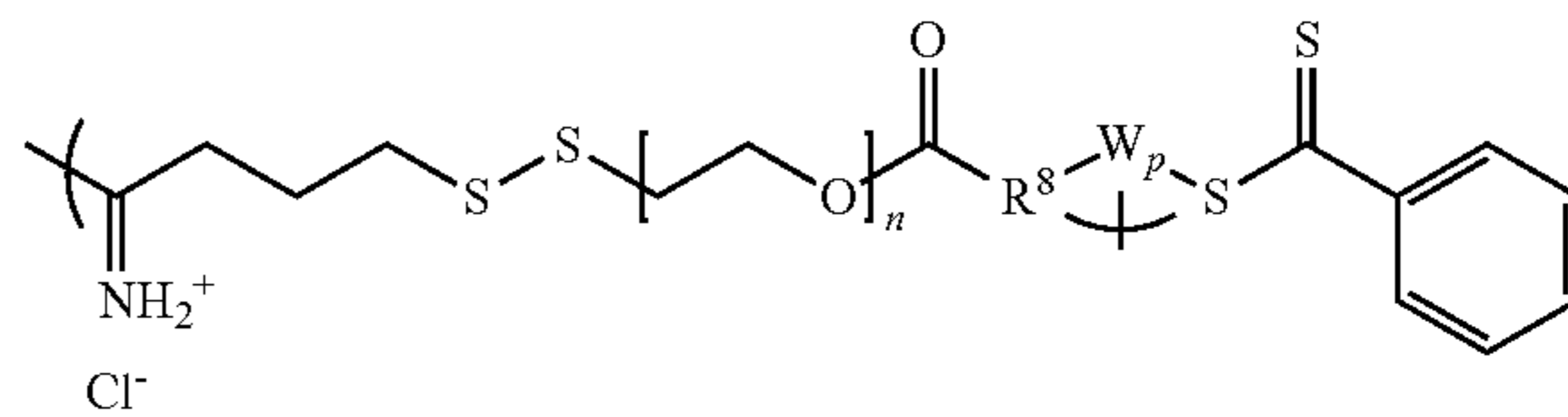
Formula Yb
