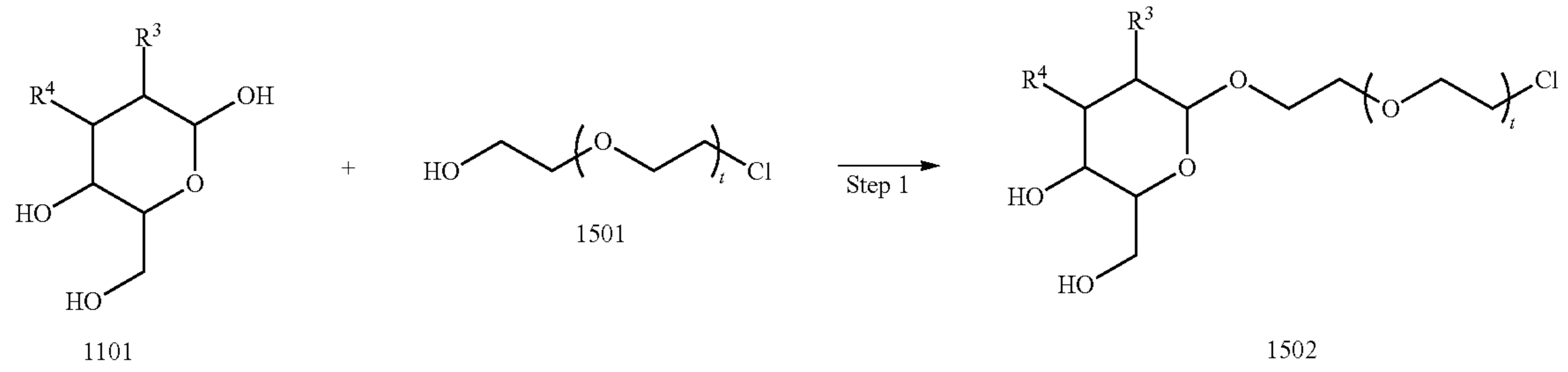
Reaction Scheme 15
