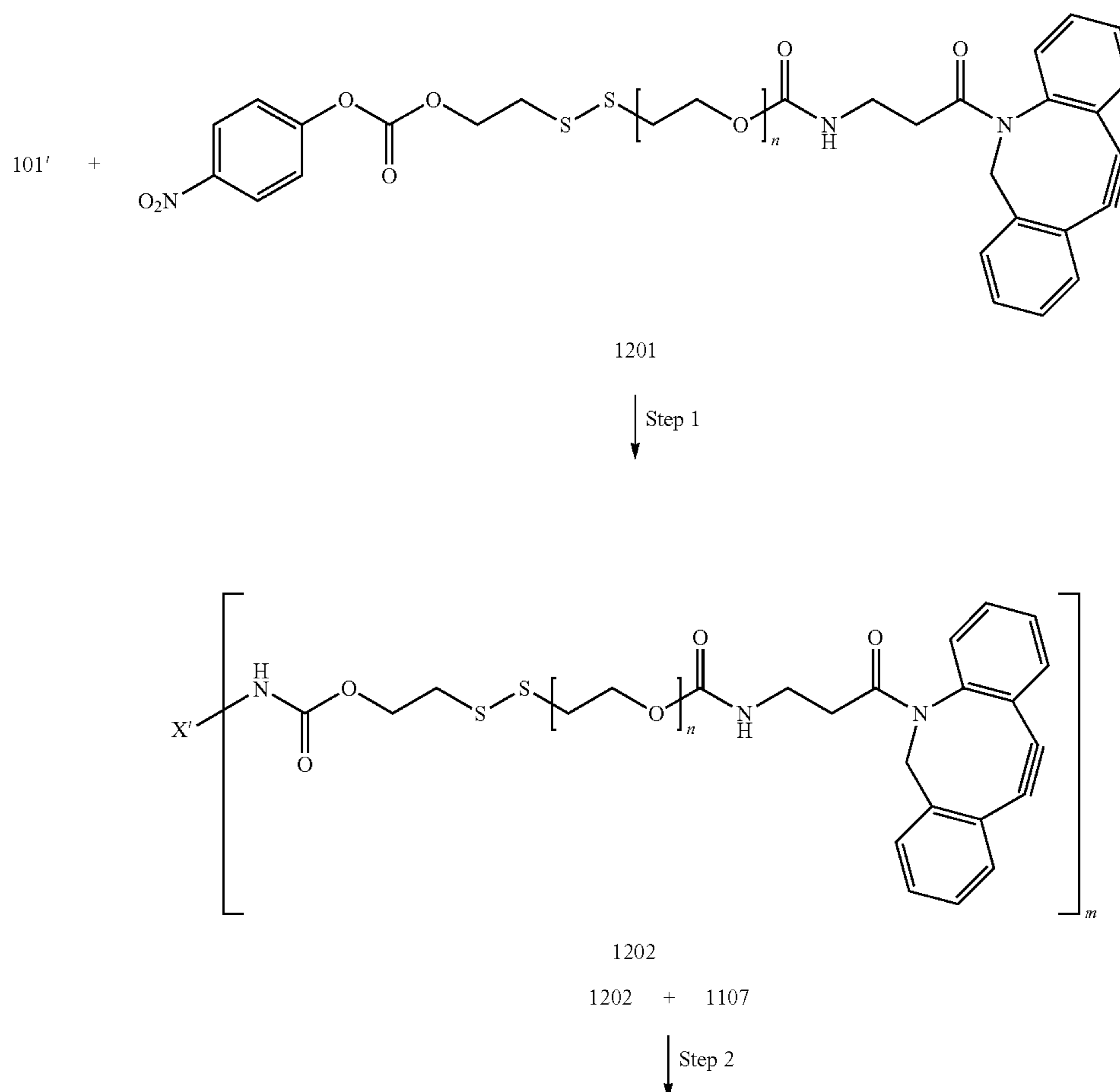
Reaction Scheme 12
