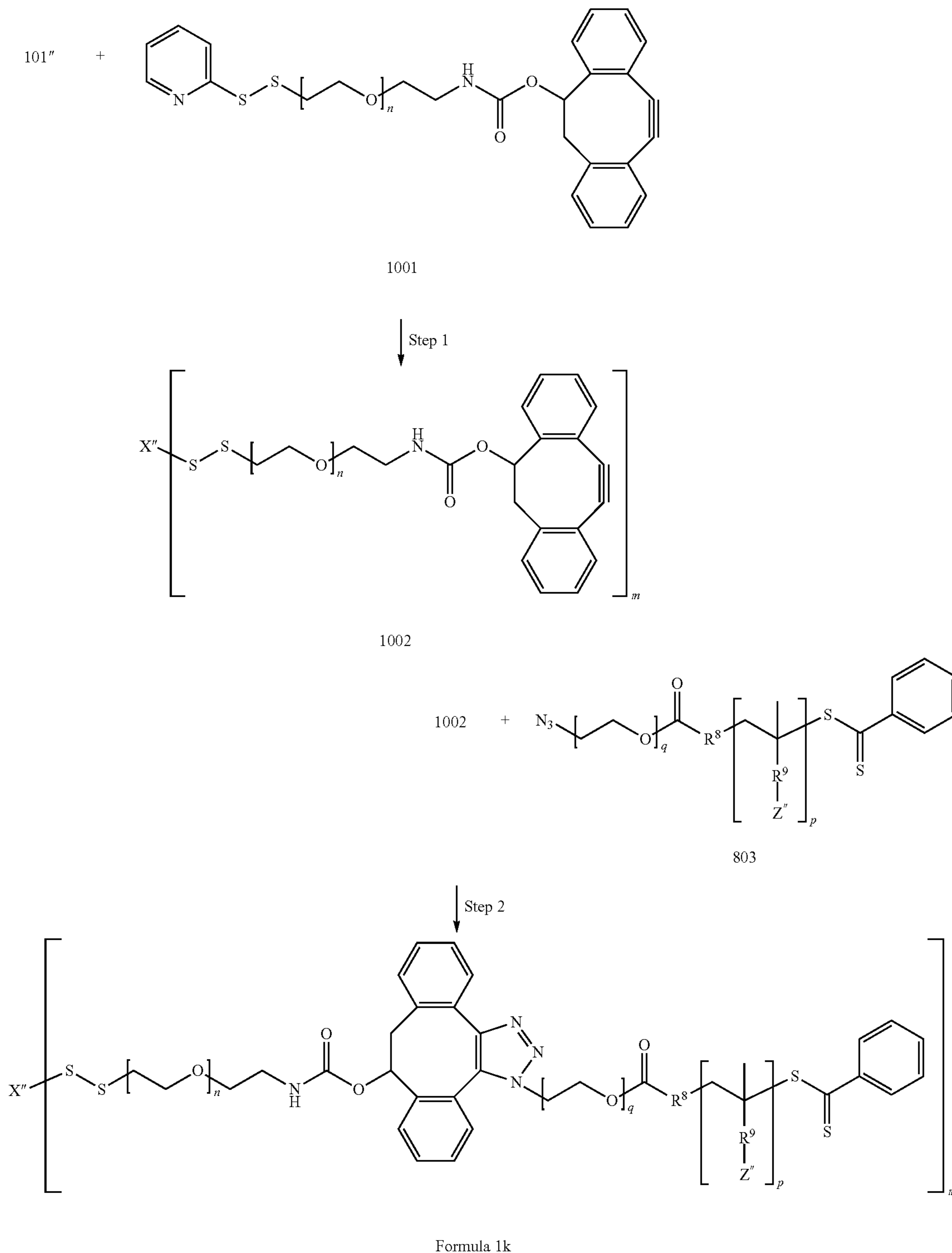
Reaction Scheme 10
