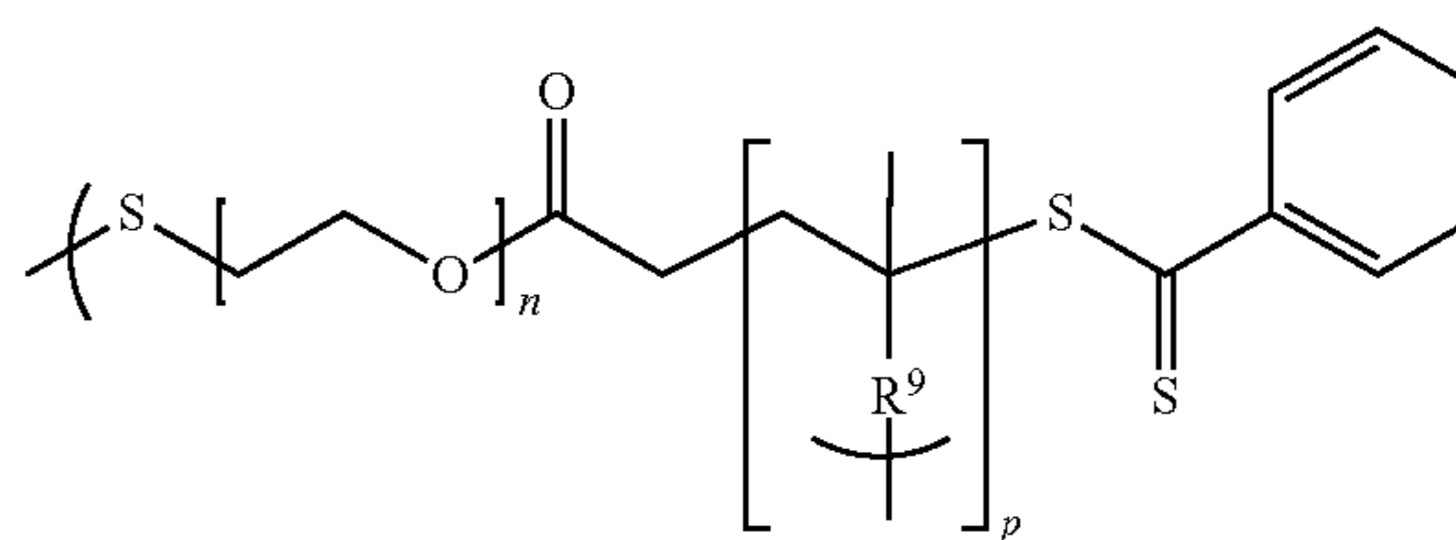
Formula Ym
