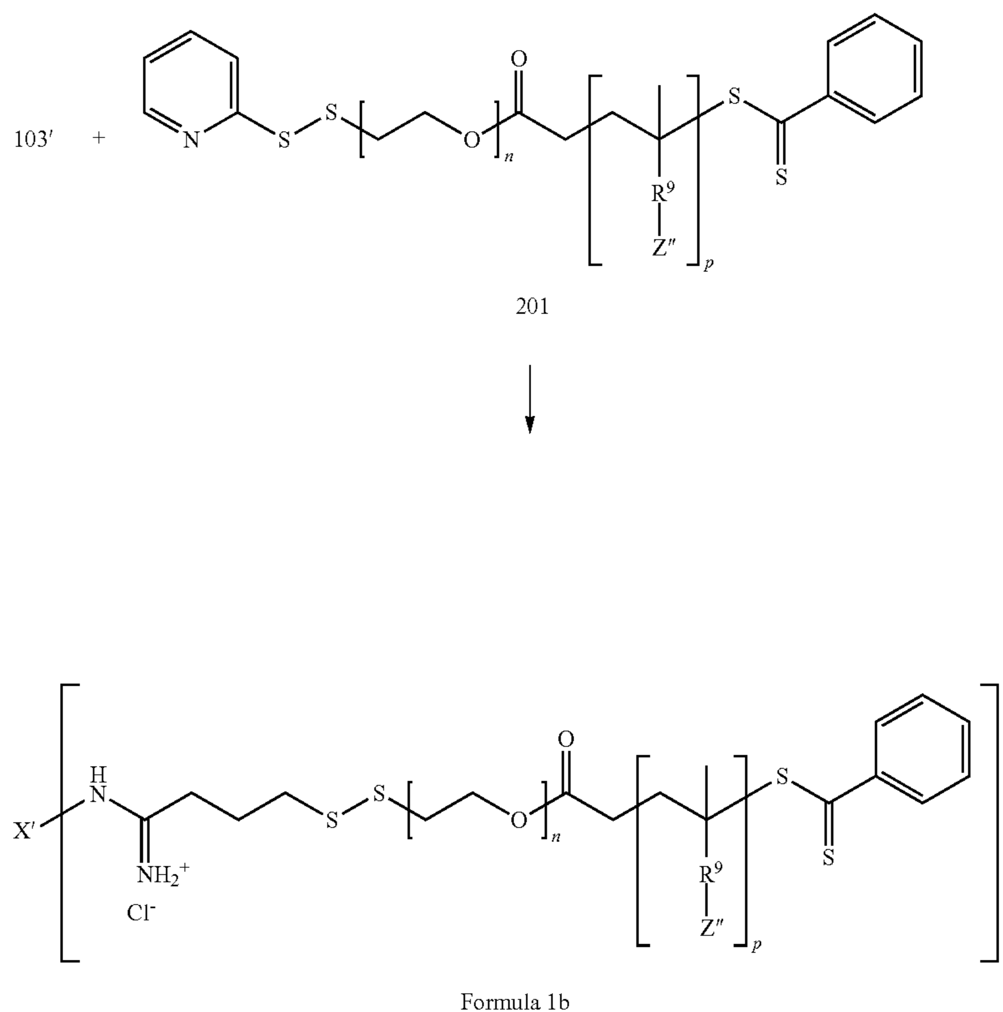
Reaction Scheme 2
