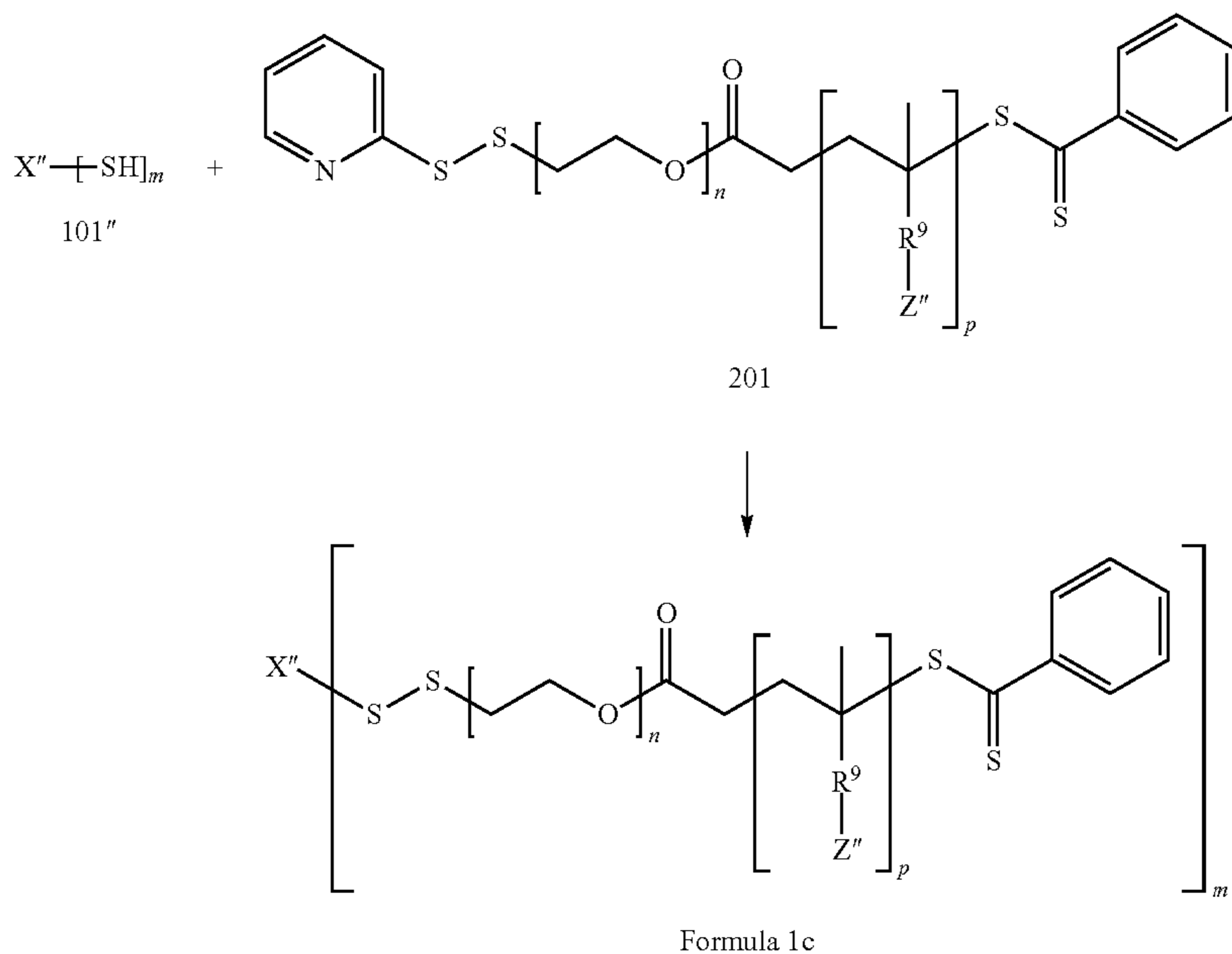
Reaction Scheme 3
