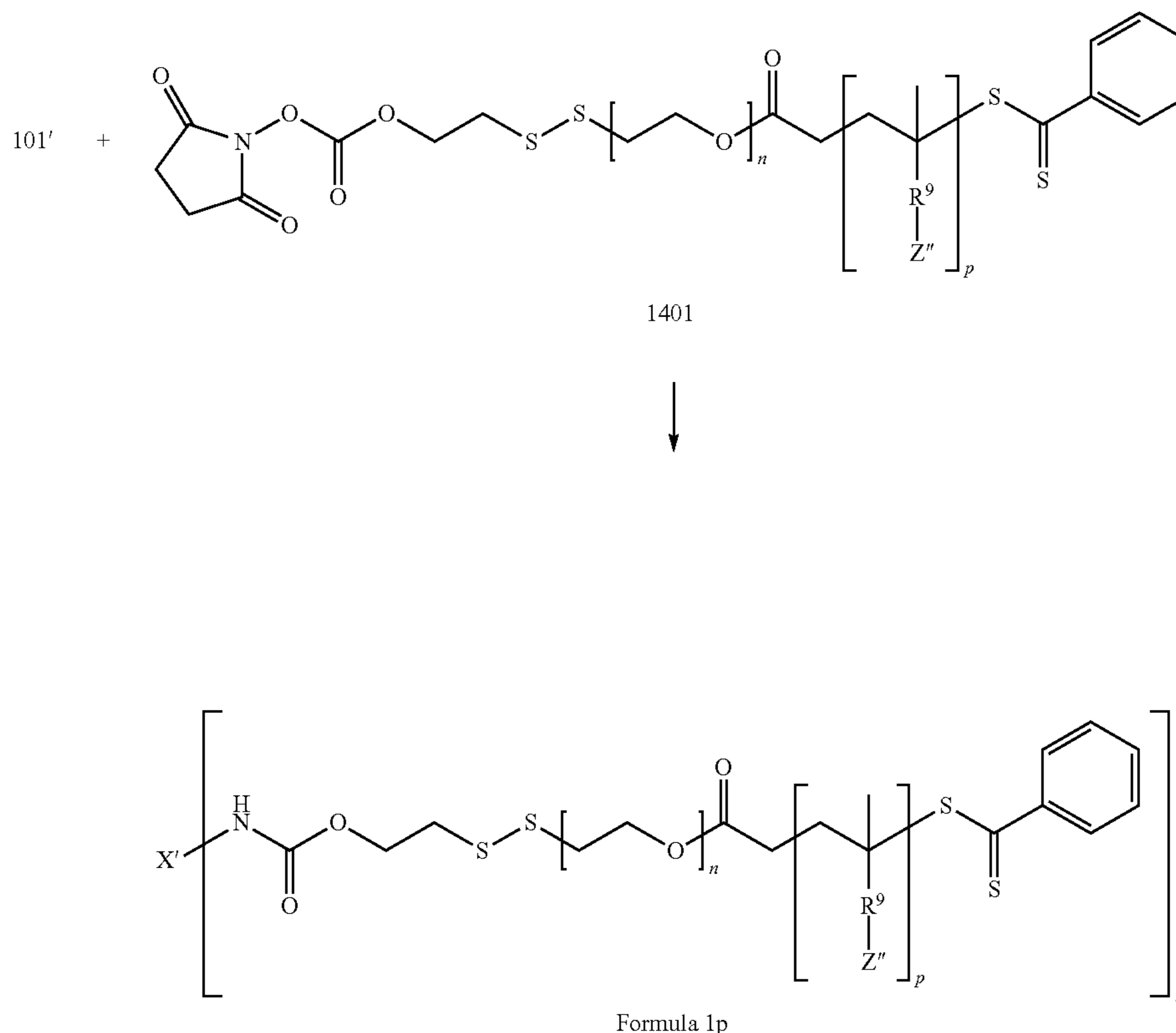
Reaction Scheme 14
