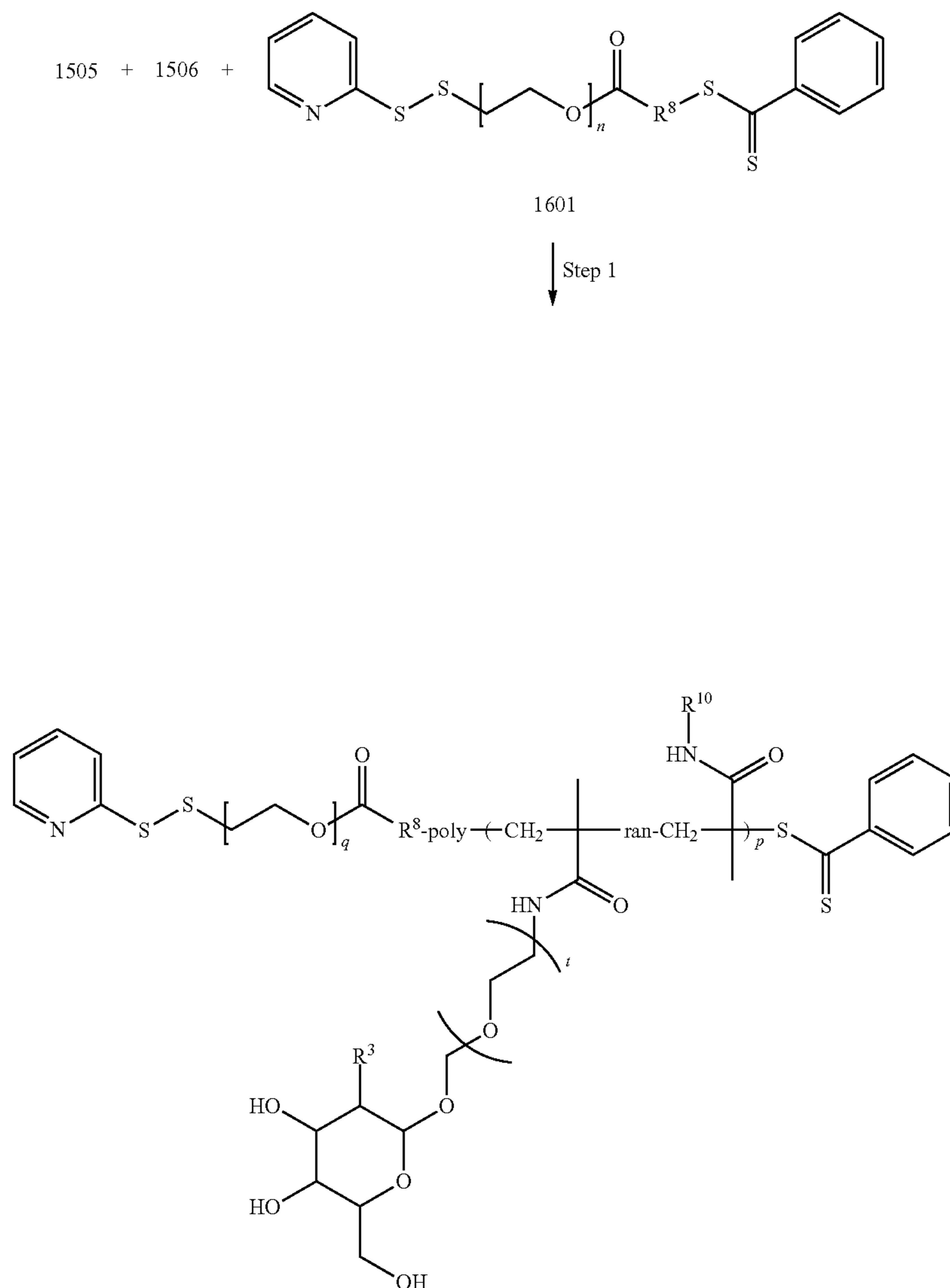
Reaction Scheme 16
