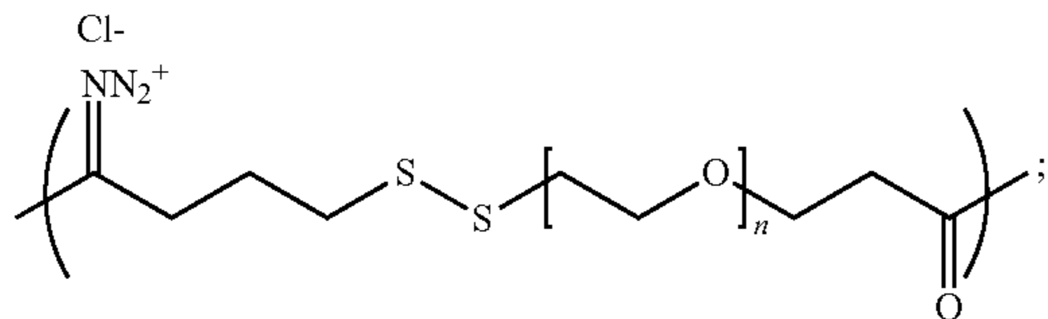
Formula Ya 20
