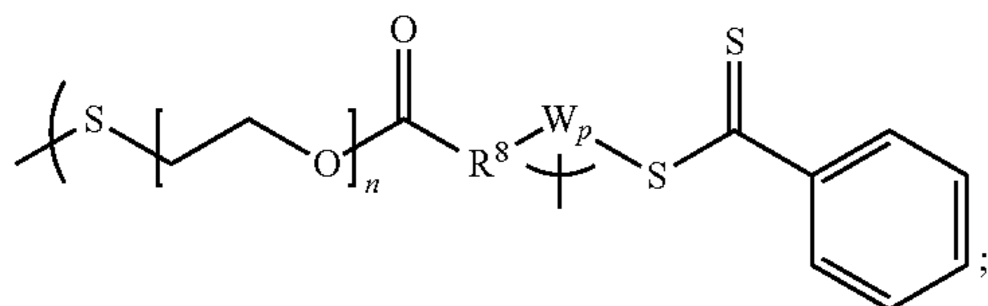
Formula Yc
