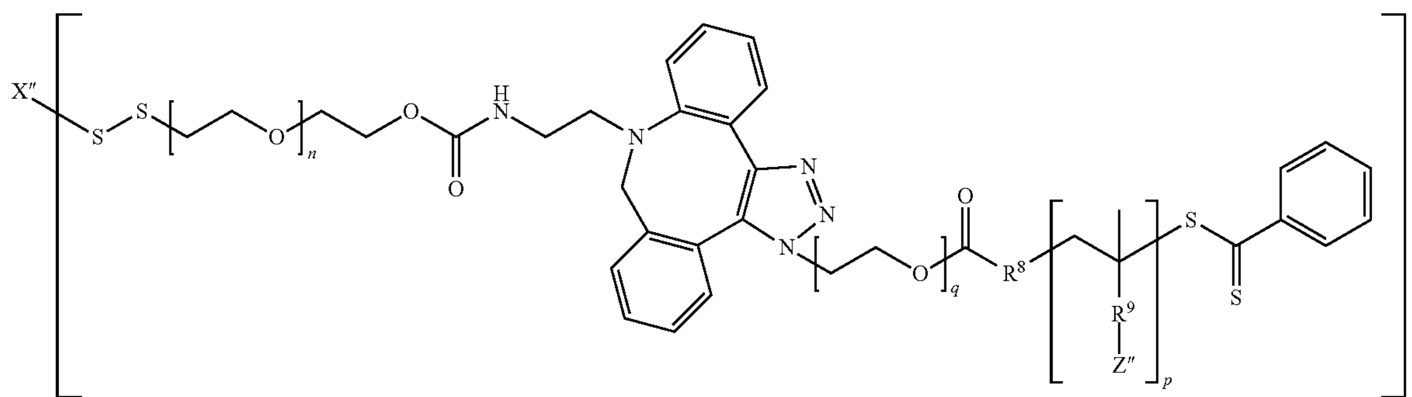
Formula 1i
