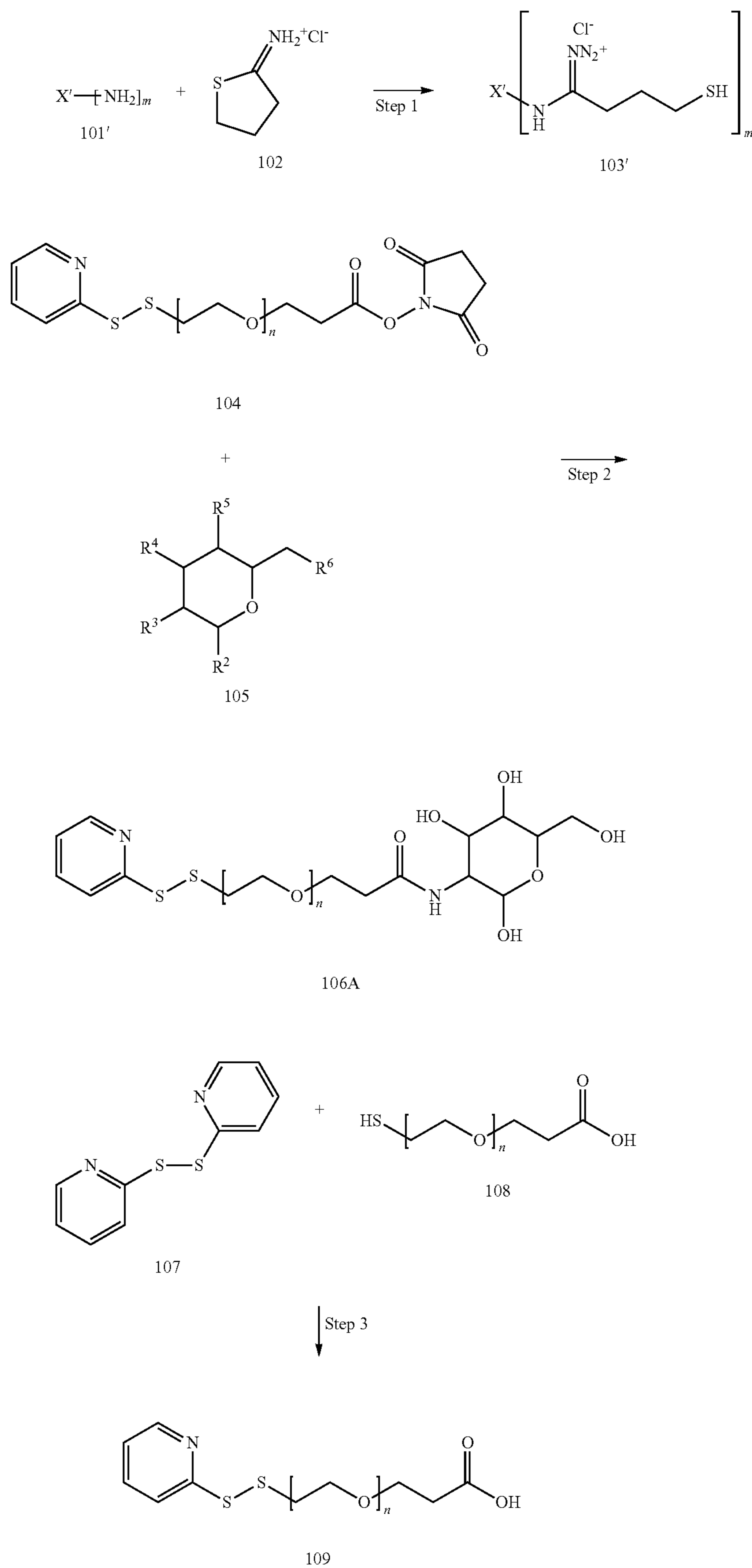
Reaction Scheme 1
