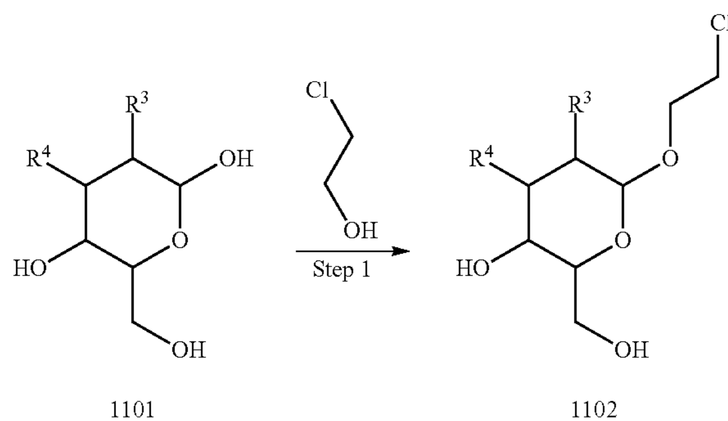
Reaction Scheme 11
