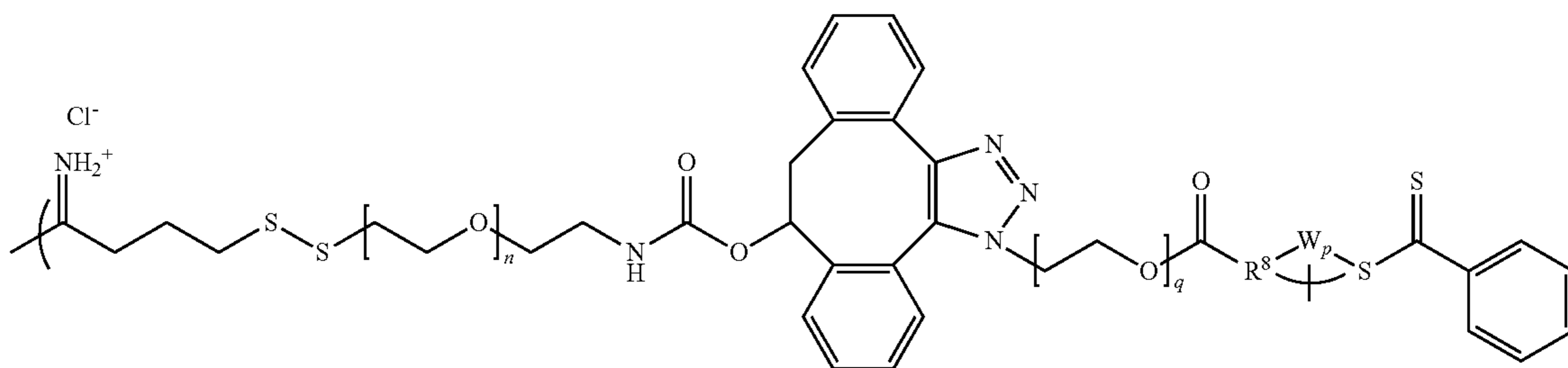
Formula YL
