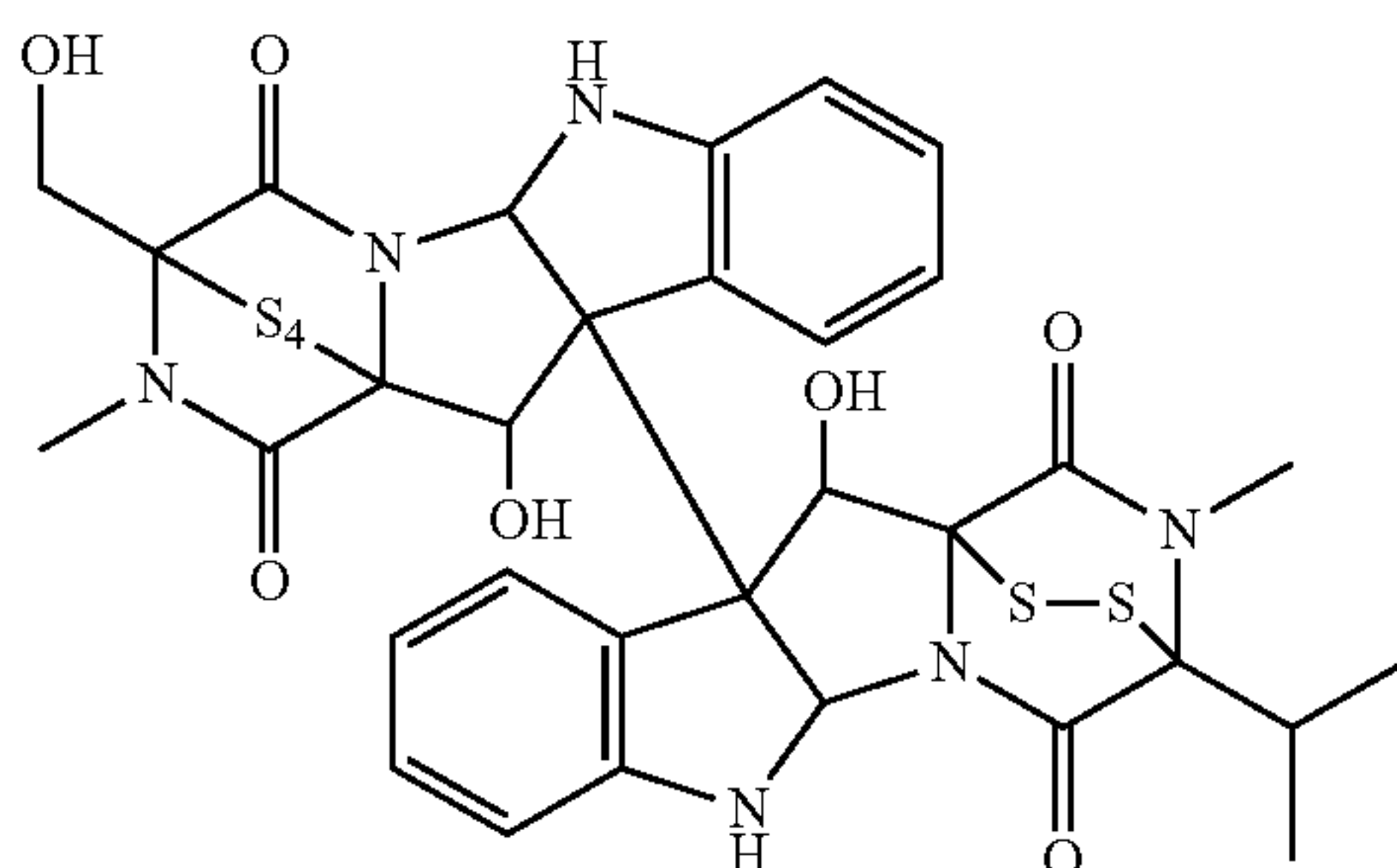
Chemical Formula 24
