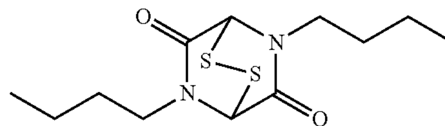
[Chemical Formula 14]
