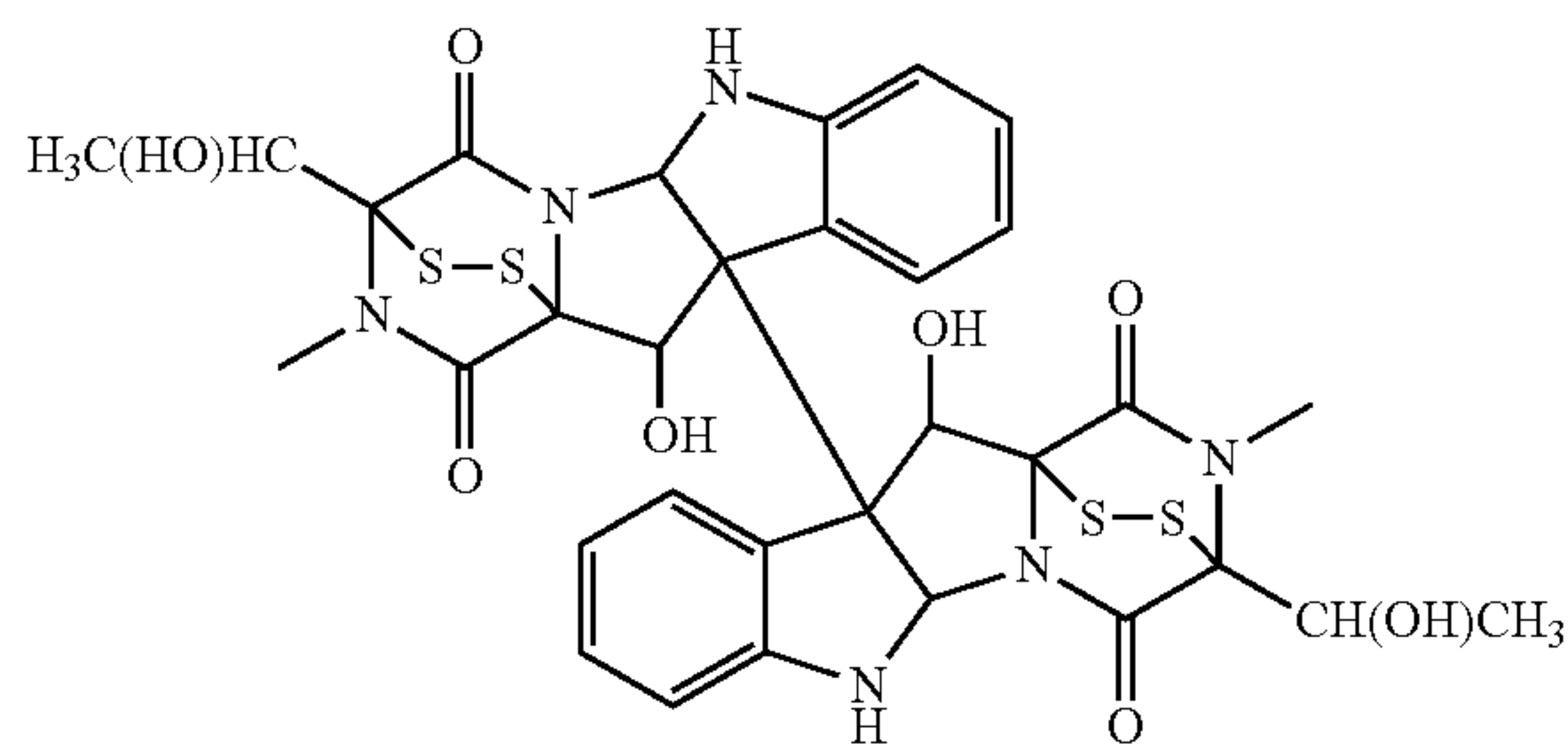
Chemical Formula 31
