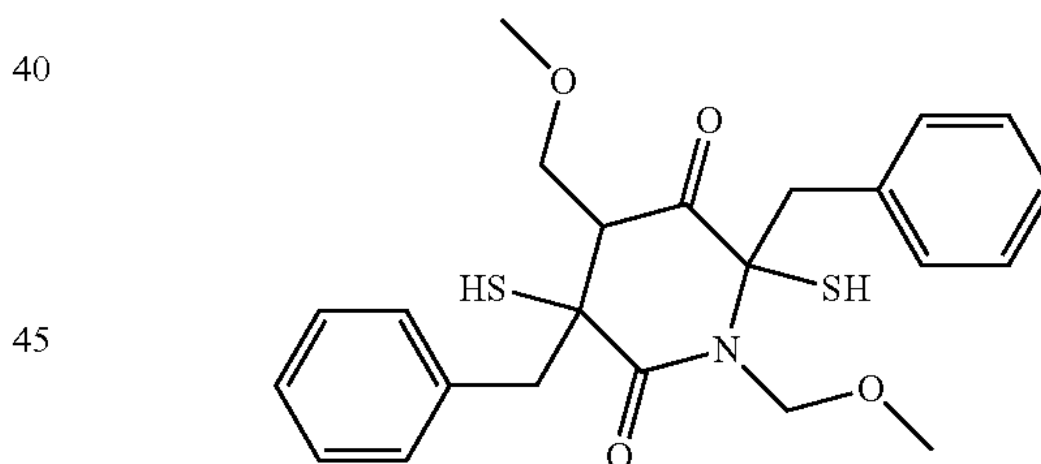
Chemical Formula 44
