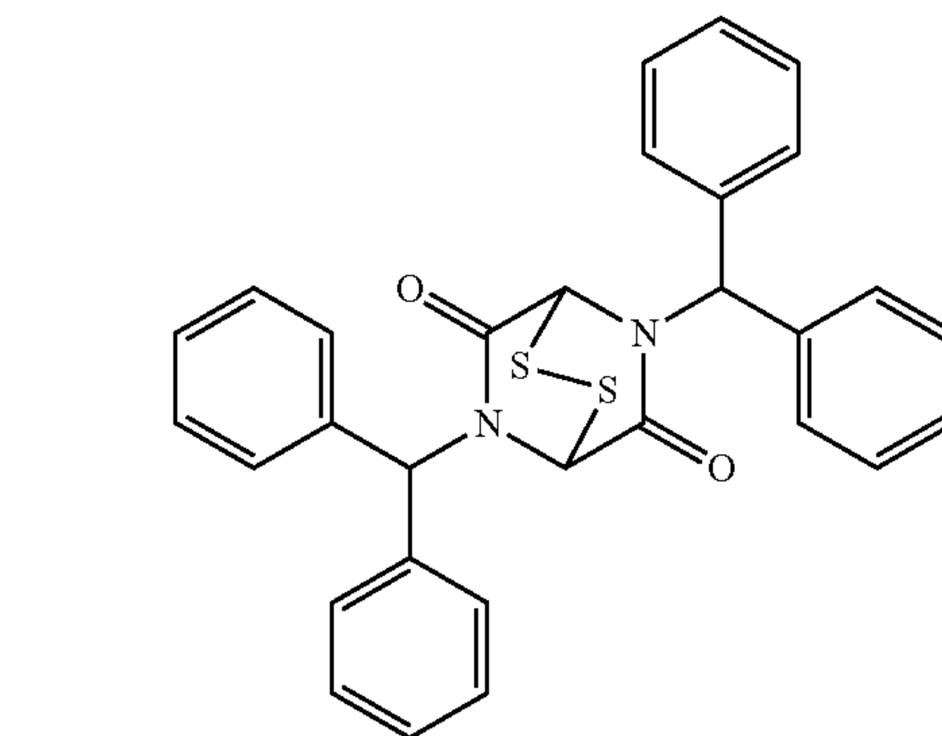
[Chemical Formula 13]
