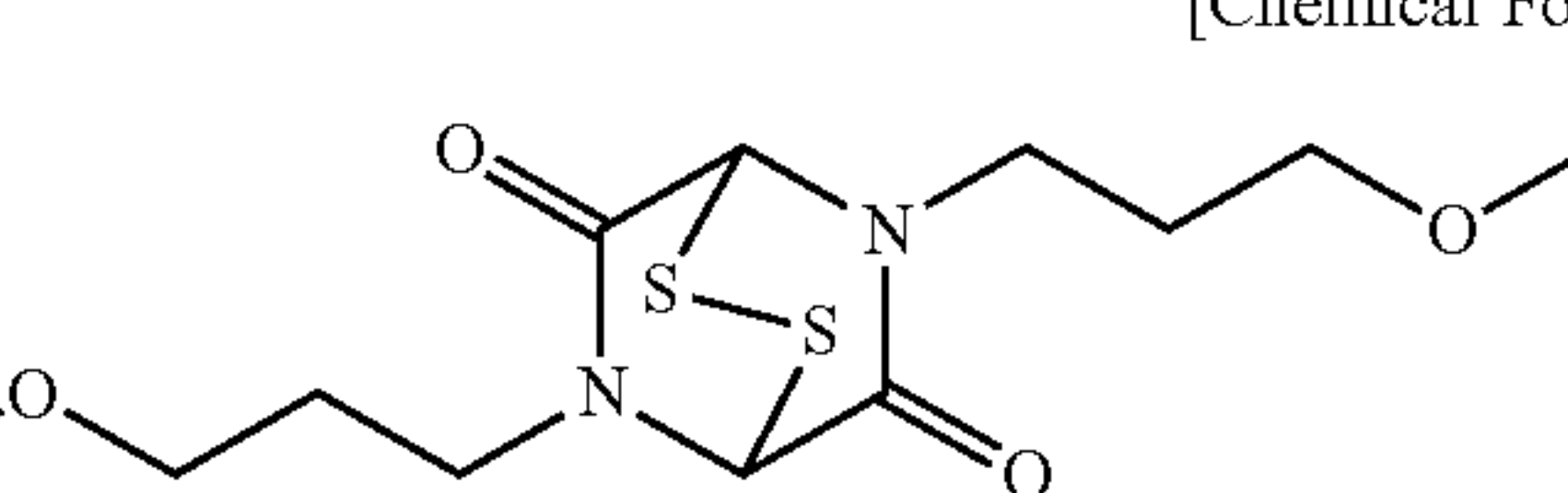
[Chemical Formula 15]
