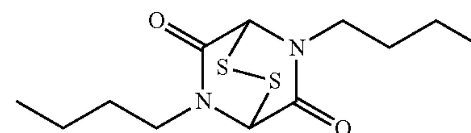
[Chemical Formula 14]
