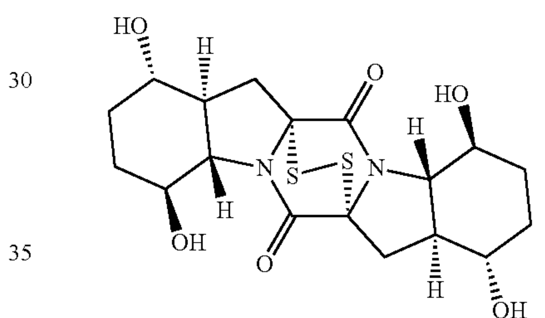
Chemical Formula 35
