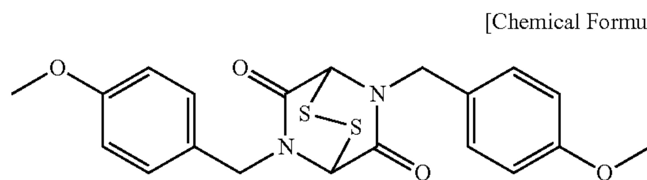
[Chemical Formula 10]
