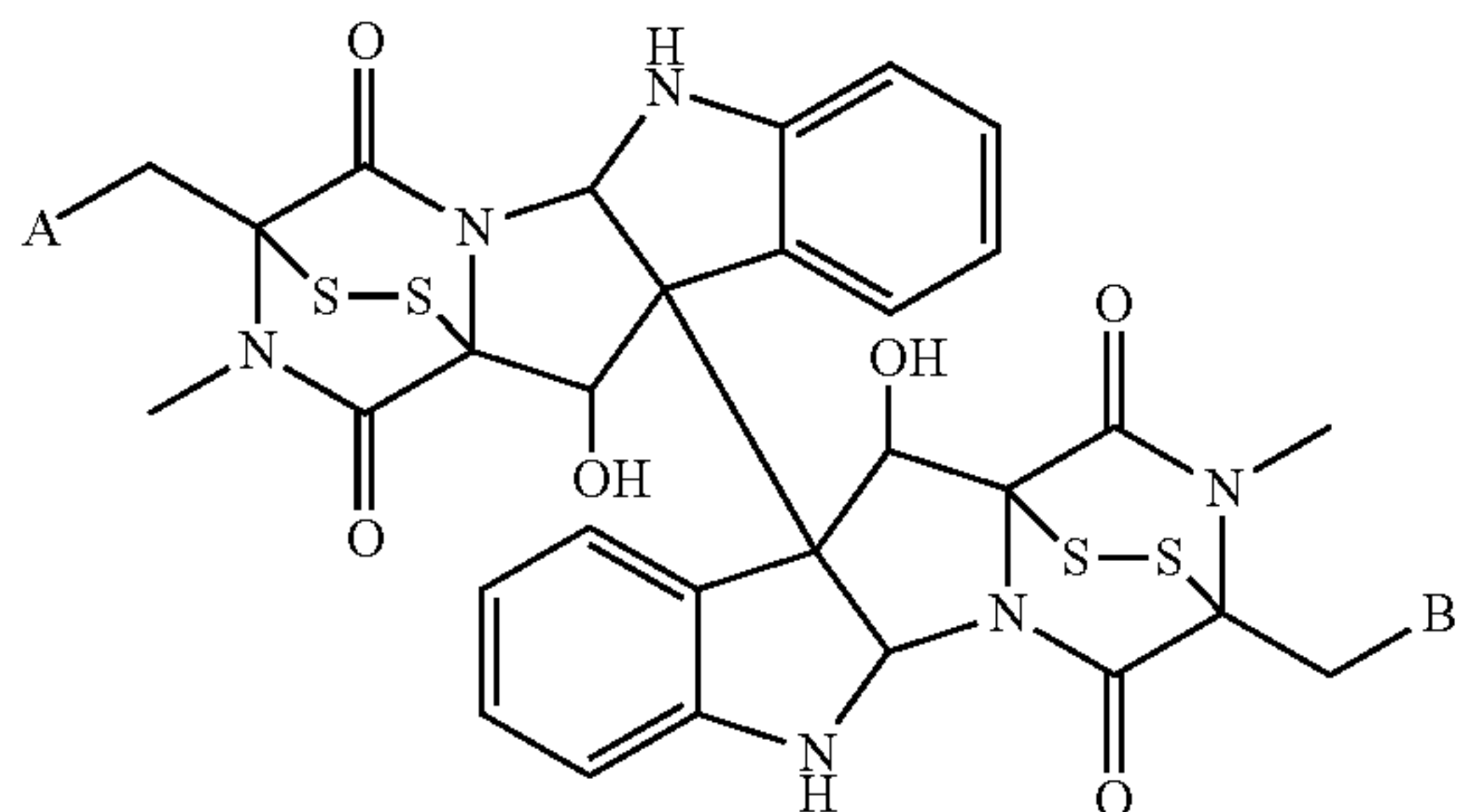
Chemical Formula 22
