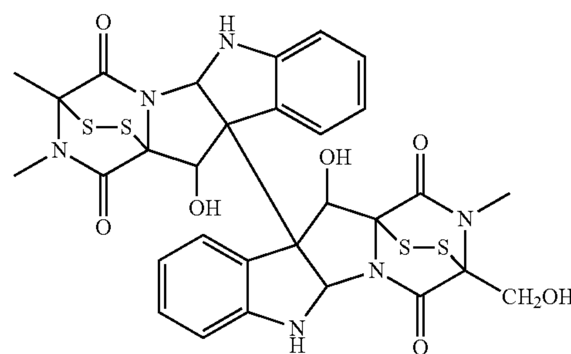
Chemical Formula 31
