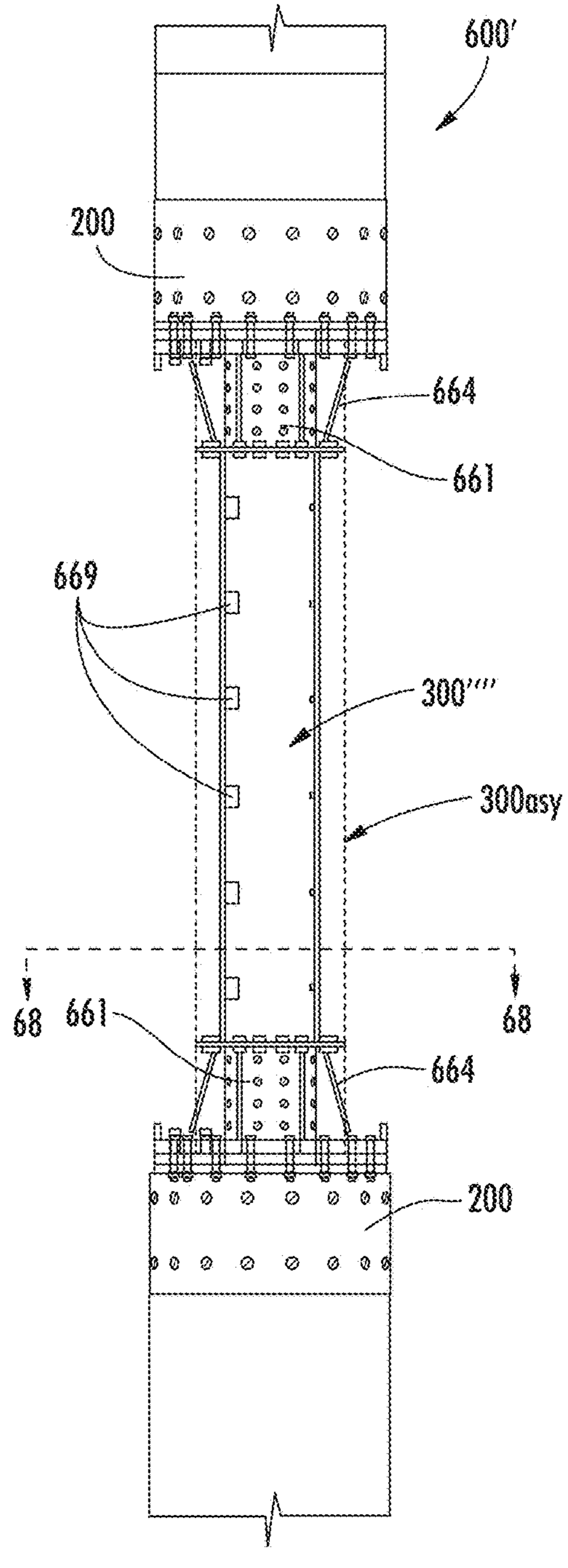
REMOVE TEMPORARY SUPPORT STEP 8
