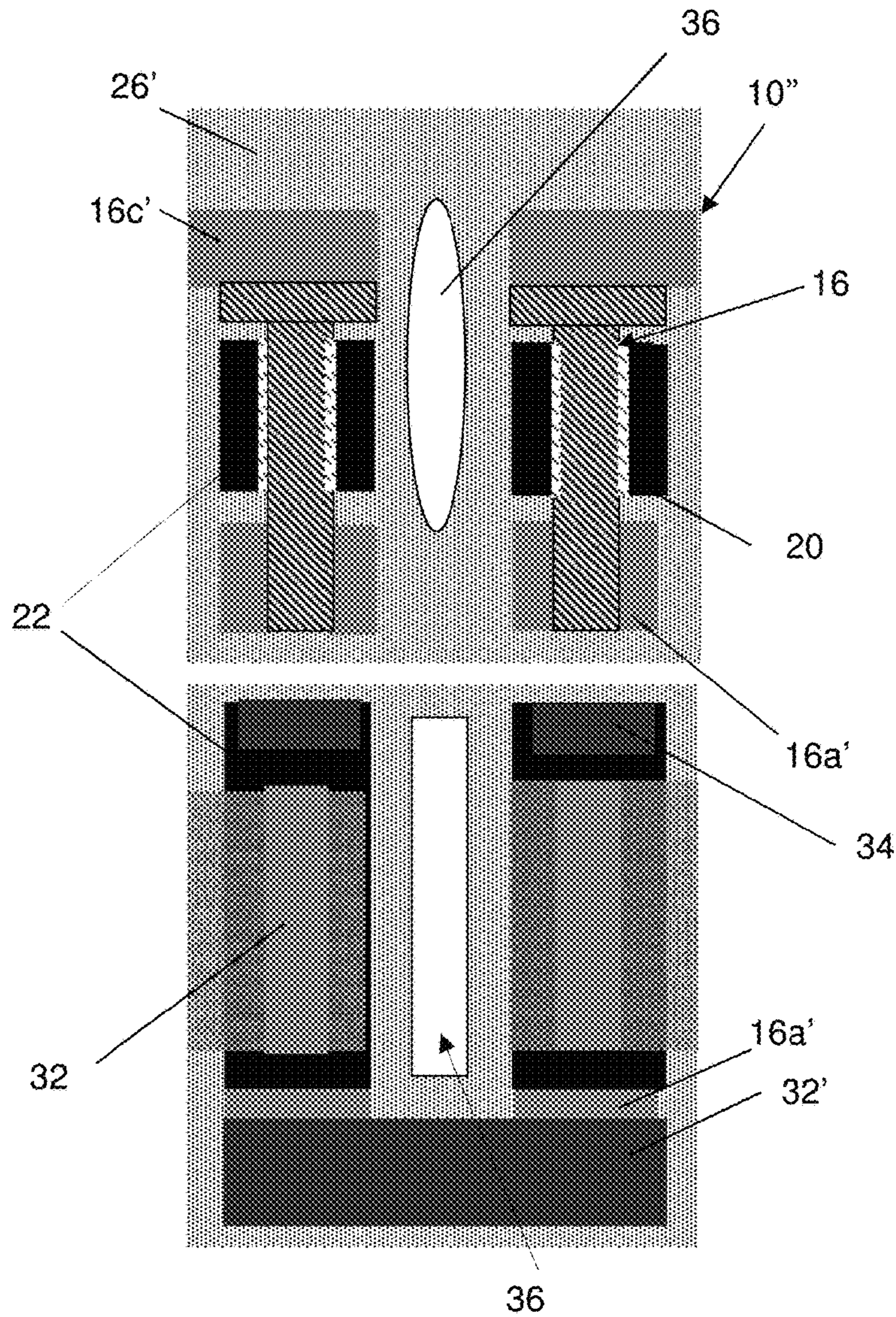
FIG. 9b (Top-down)
