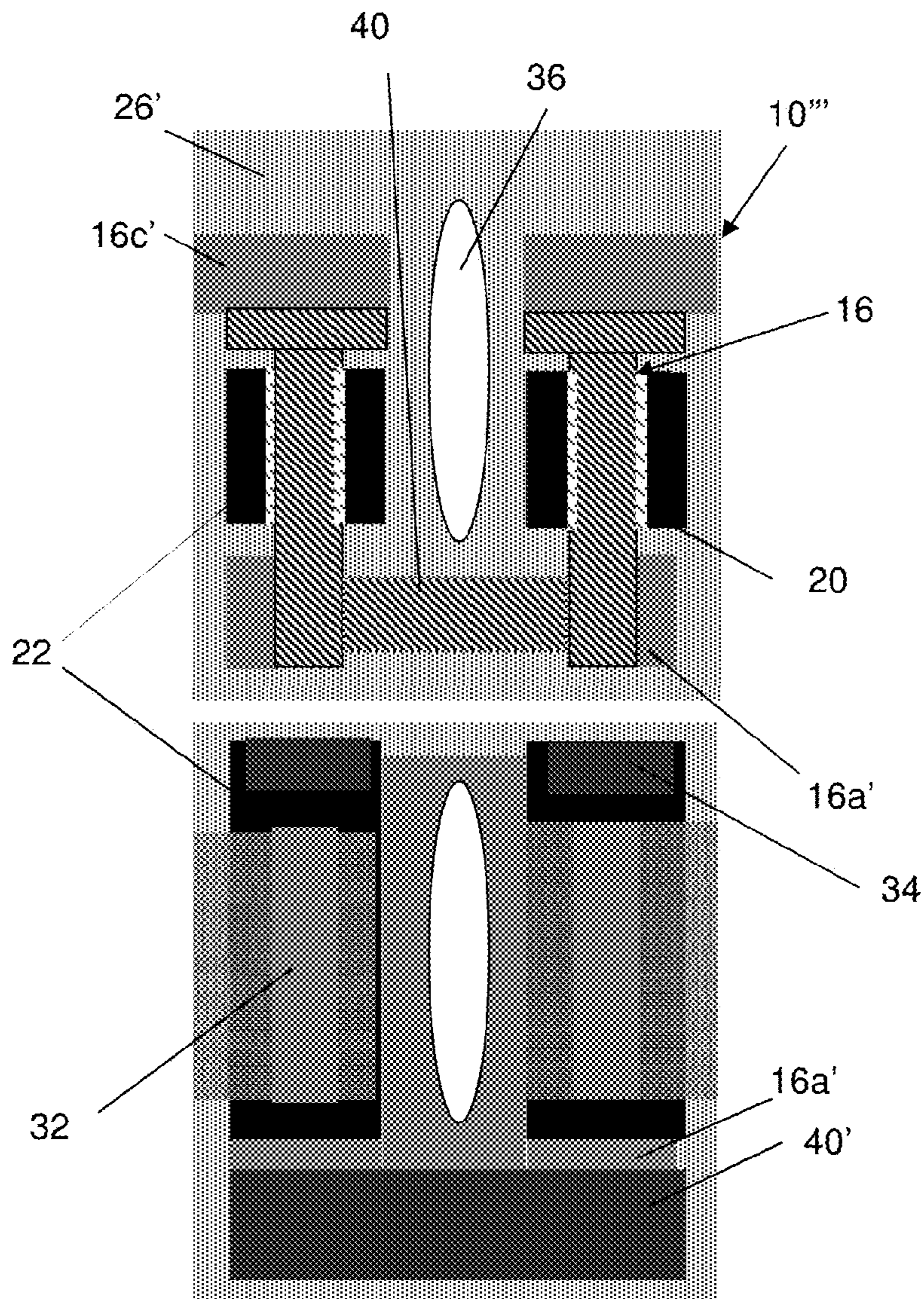
FIG. 10b (Top-down)
