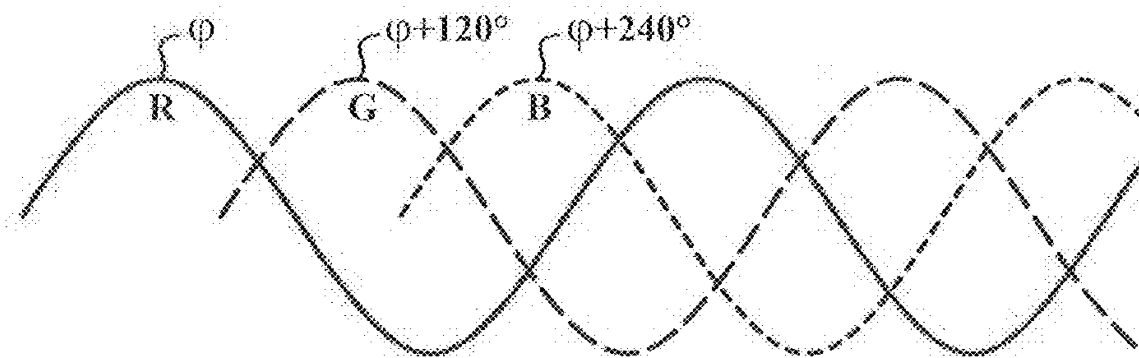
3 Phase 3 Color Beam Modulation
