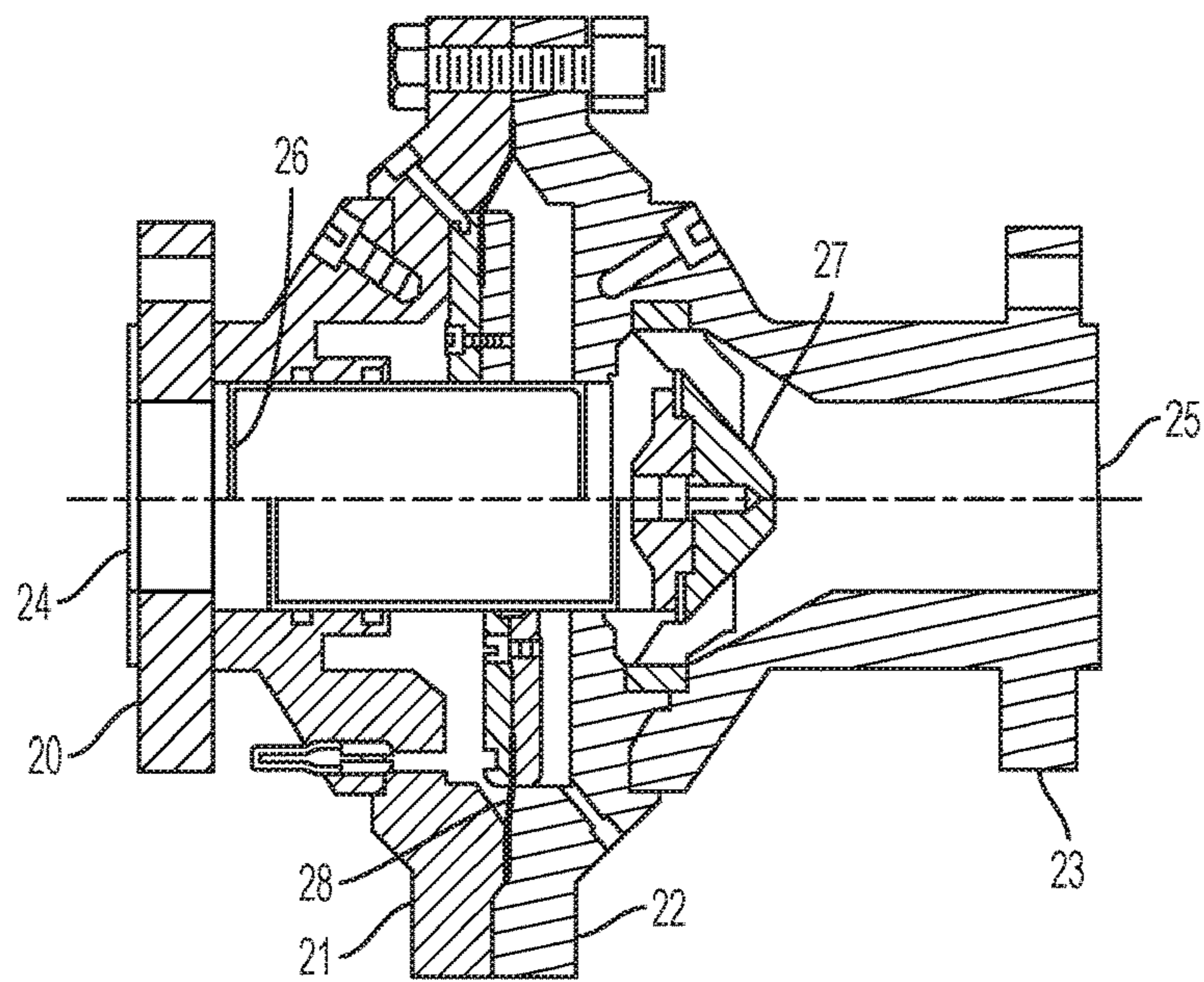
FIG. 2 PRIOR ART
